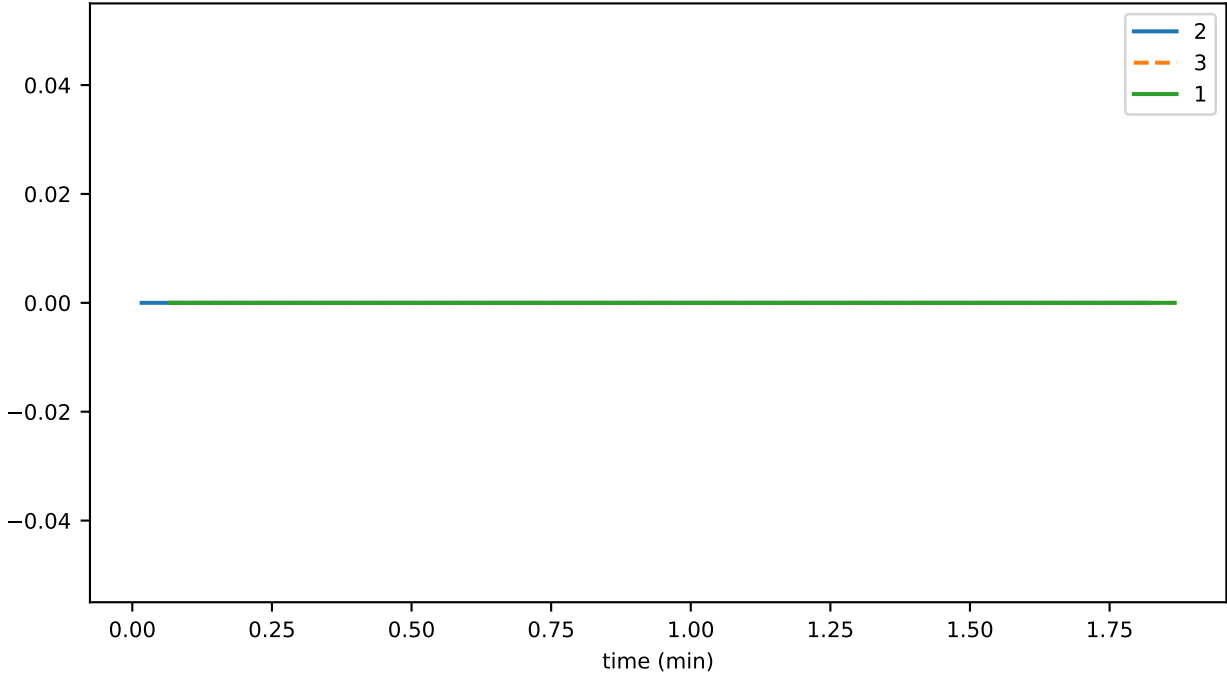
sync_phase_00_fraction_SENDING_EVENTS
