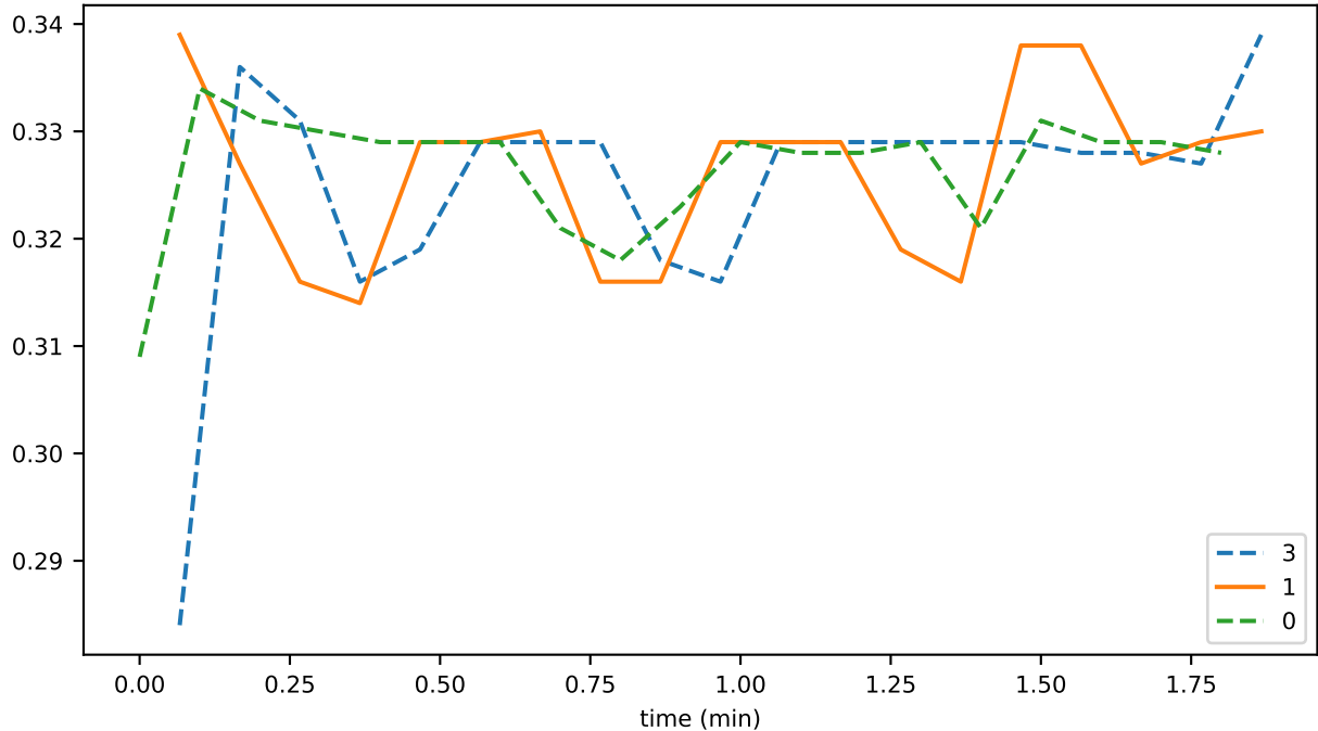
sync_phase_02_fraction_SENDING_EVENTS
