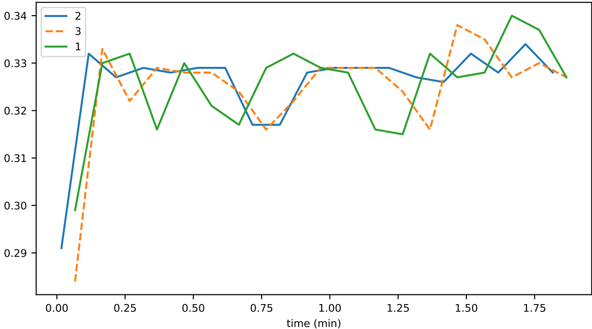
sync_phase_00_fraction_SENDING_EVENTS
