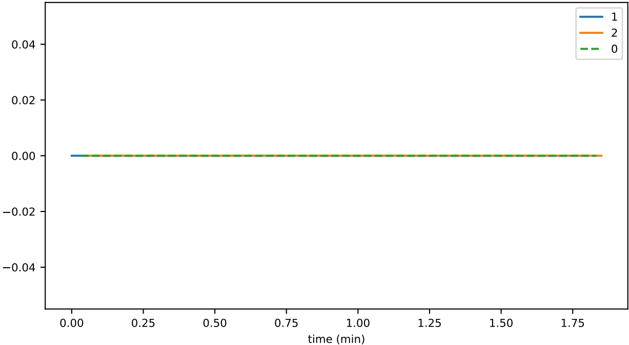
sync_phase_03_fraction_SELF_FALLEN_BEHIND
