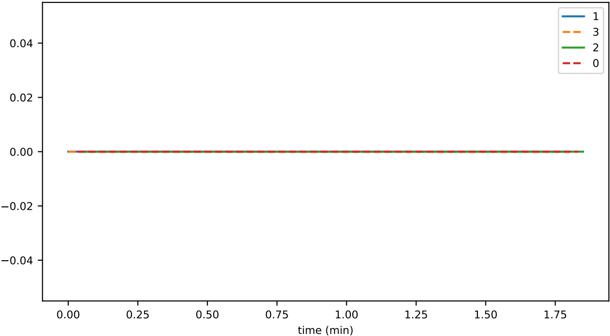
ds_files_level_5_leavesFileSizeByLevelMb_accounts
