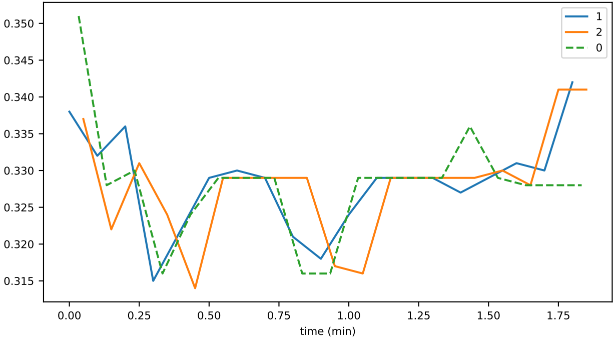
sync_phase_03_fraction_SENDING_EVENTS
