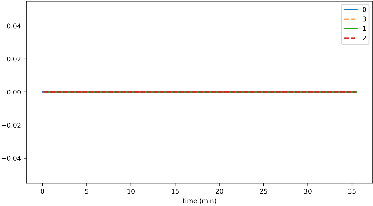
SmartContractService:SystemContractMethodCall_FREEZE_UNFREEZE_failed
