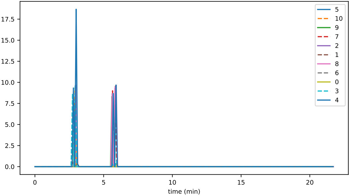
ds_compactions_level_0_hashesSavedSpaceMb_accounts
