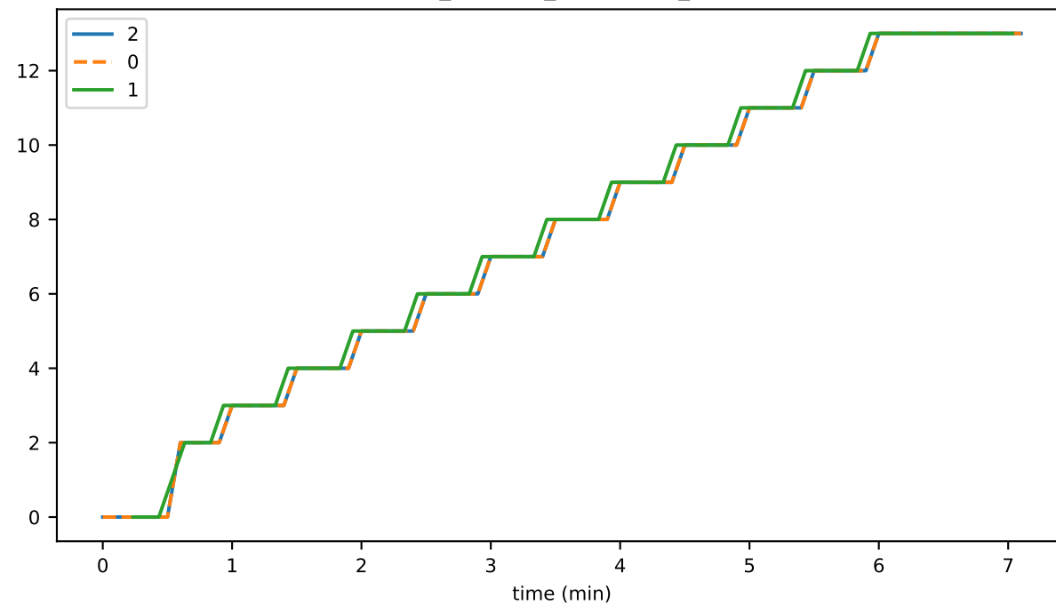
vmap_lifecycle_flushCount_state
