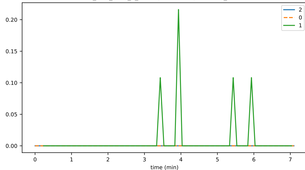
ds_files_level_3_hashesFileSizeByLevelMb_state
