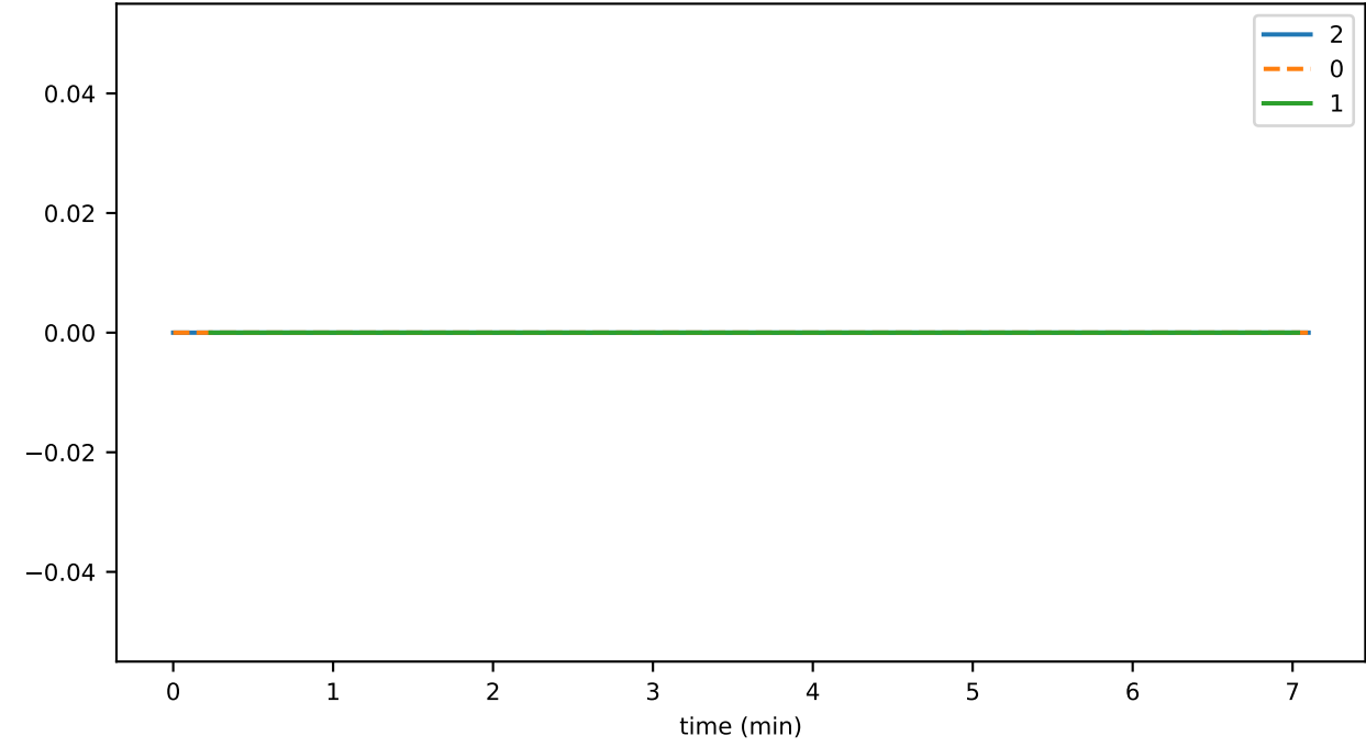
OrphanBuffer_unhandled_task_count
