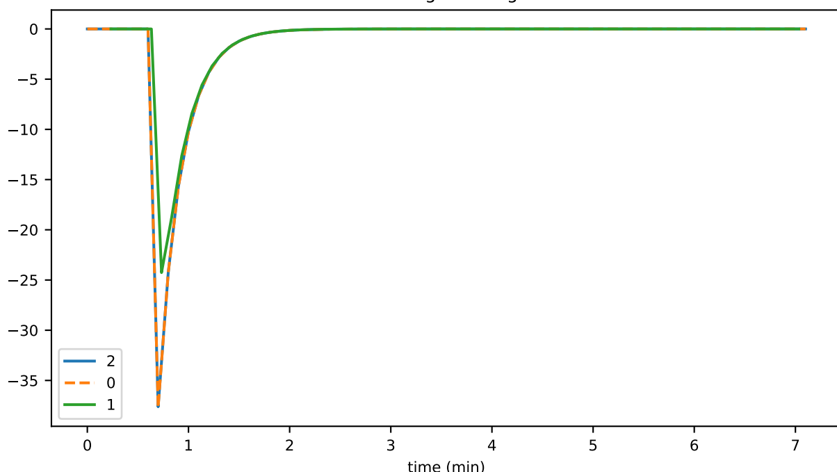
stateSignatureAge
