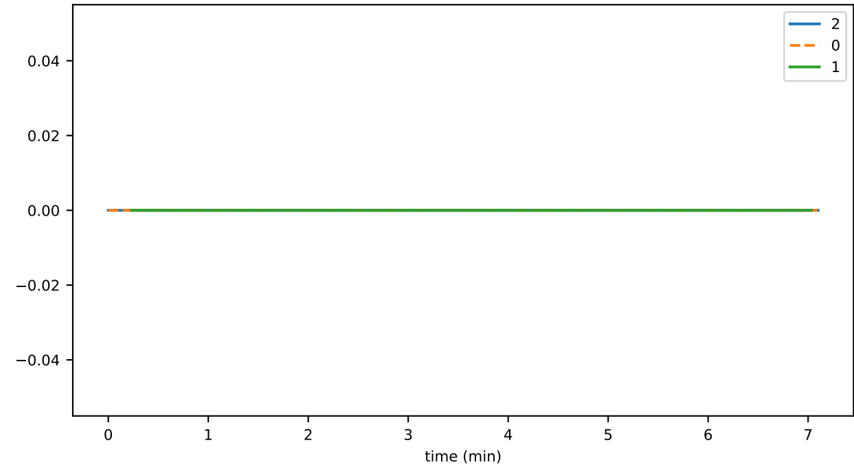
ds_compactions_level_9_hashesTimeMs_state
