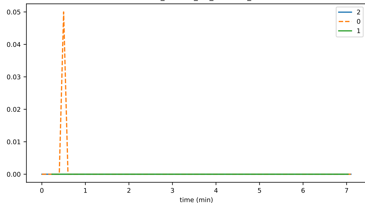
eventCreation_fraction_PIPELINE_INSERTION
