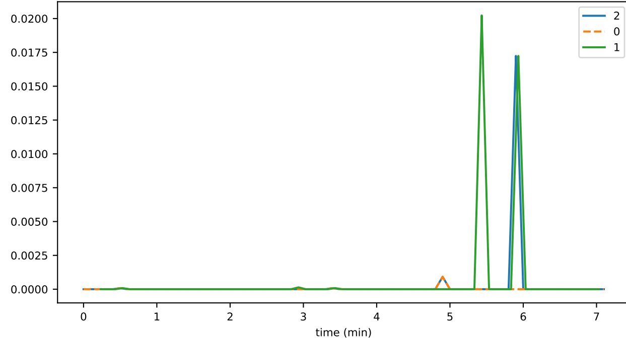
ds_flushes_leafKeysStoreFileSizeMb_state
