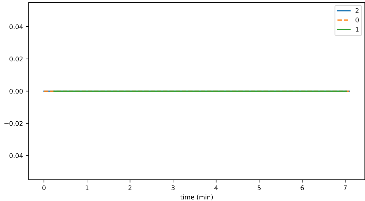
ds_compactions_level_9_leavesTimeMs_state
