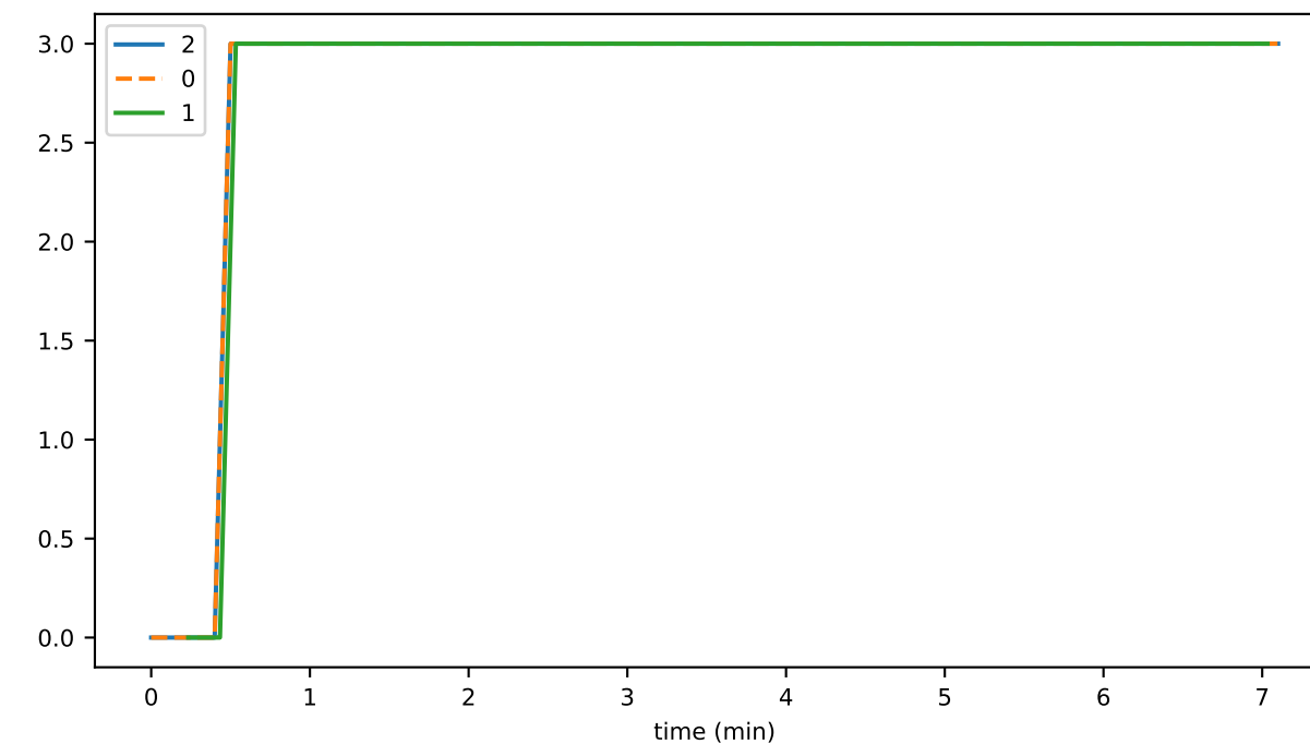
nodeUpdateDurationMax
