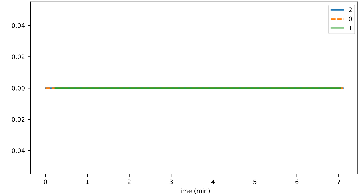
tokenCancelAirdropThrottledTxns
