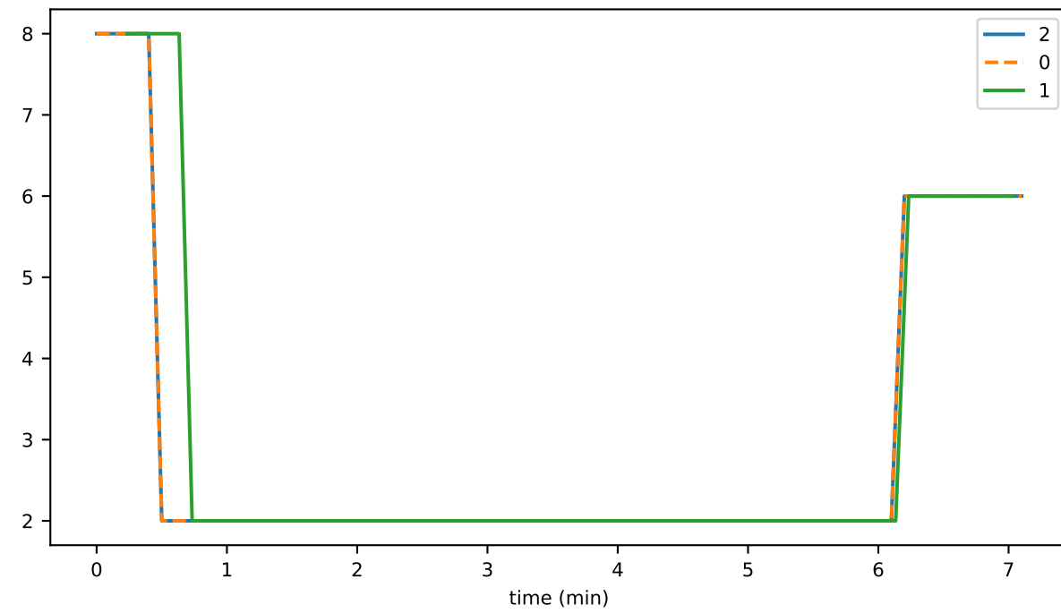
PlatformStatus
