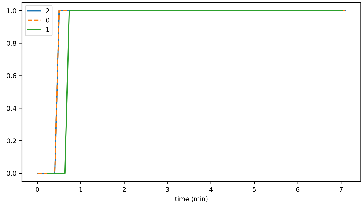
createdEventParents
