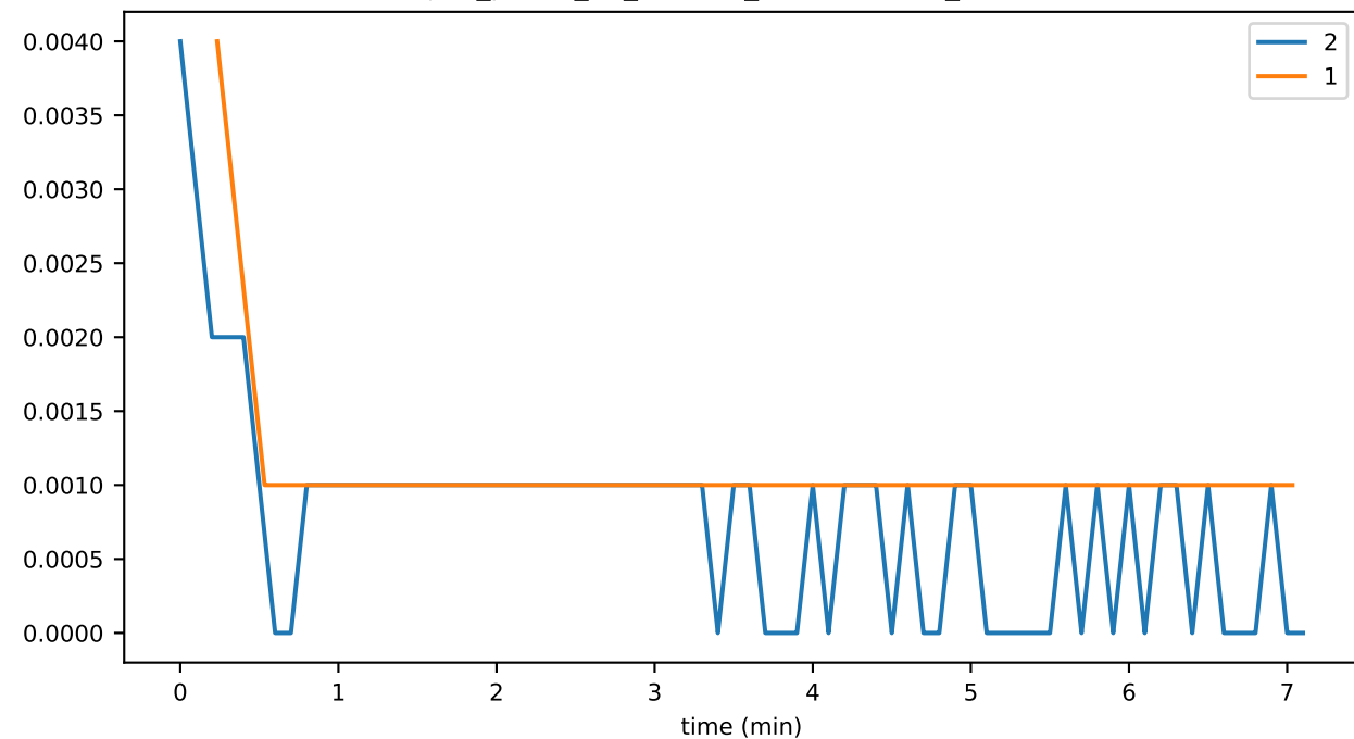
sync_phase_00_fraction_EXCHANGING_WINDOWS
