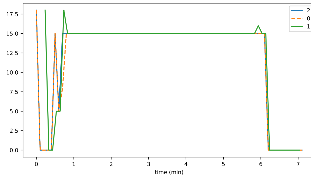
numEventsAddedUntilConsensusMAX
