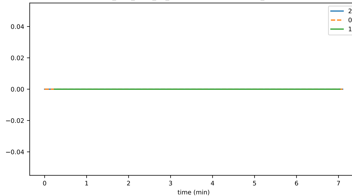
ds_files_level_10_leavesFileSizeByLevelMb_state
