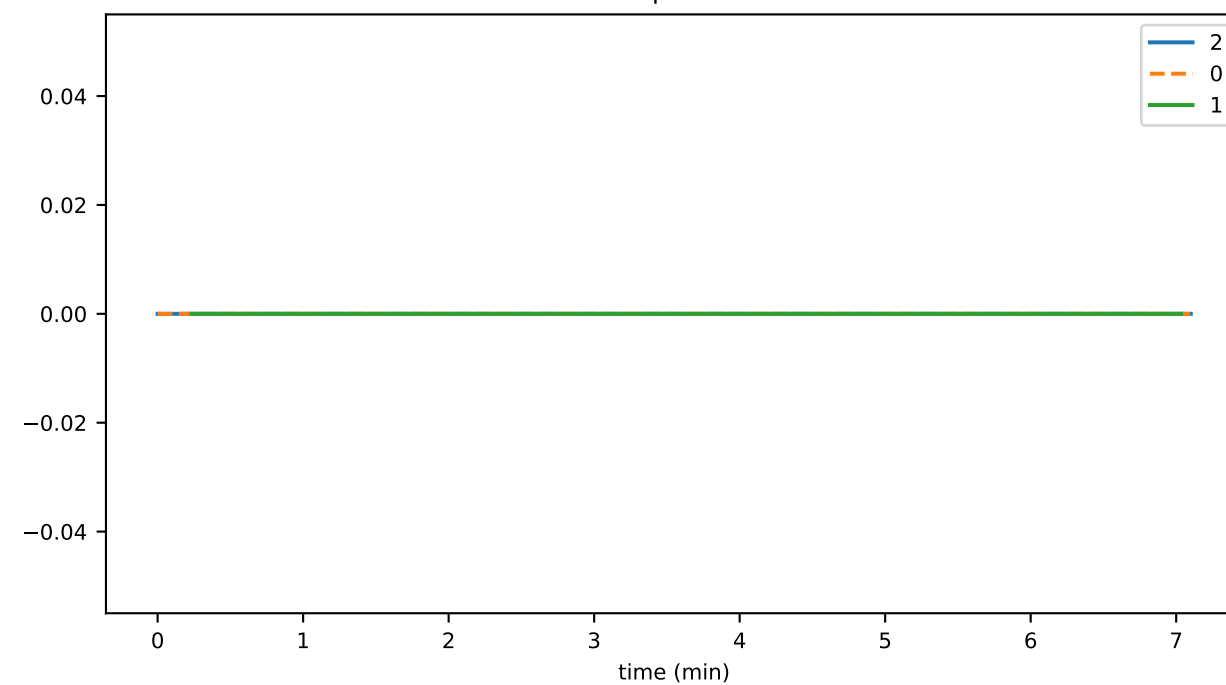
consensusGetTopicInfoDurationMax
