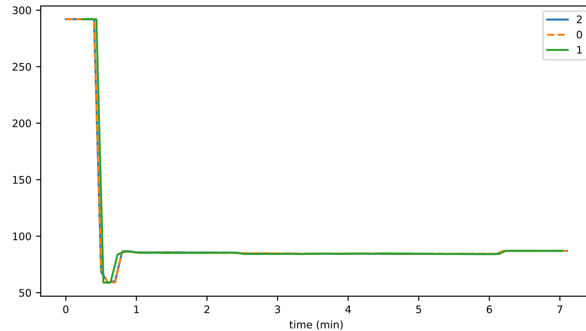
knownSetSize
