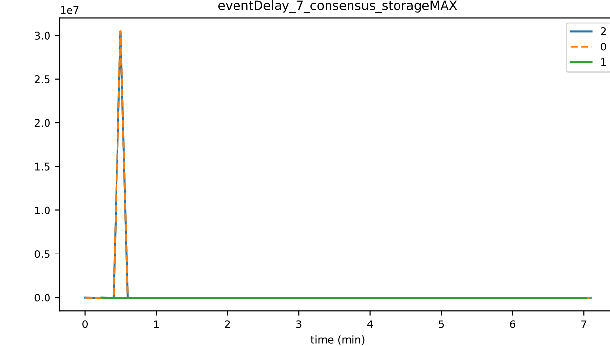
eventDelay_7_consensus_storageMAX
