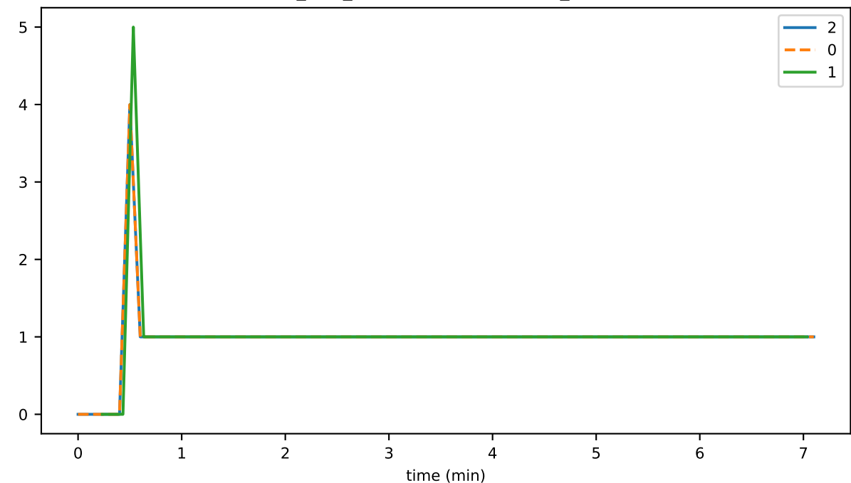
ds_files_leafKeysStoreFileSizeMb_state
