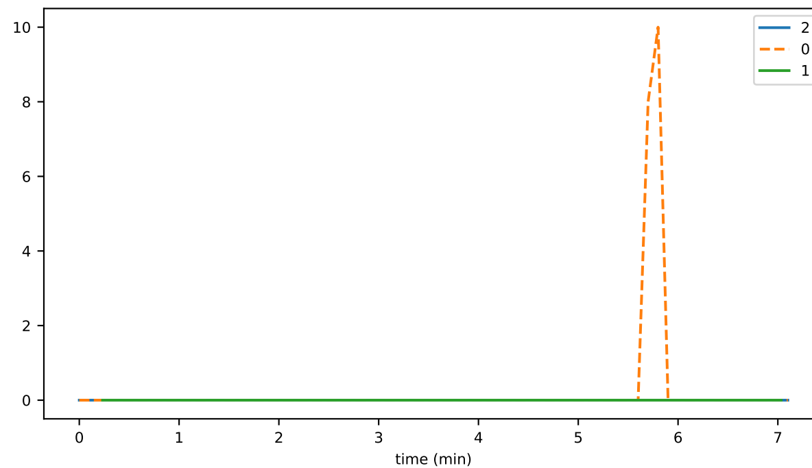
bufferedTransactions
