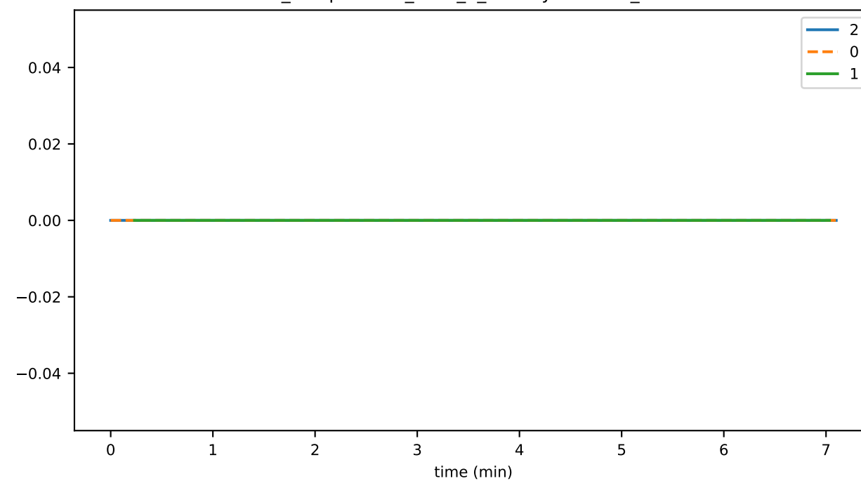
ds_compactions_level_6_leafKeysTimeMs_state
