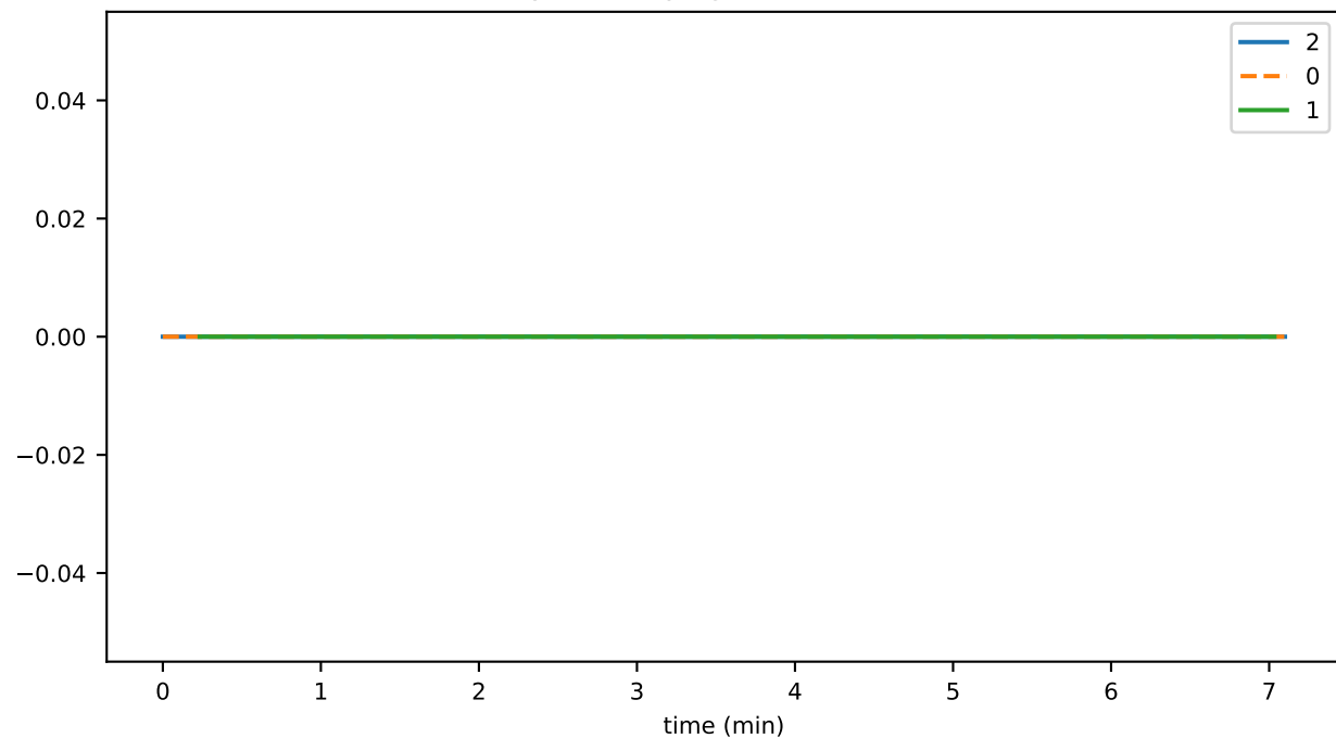
historyProofKeyPublicationDurationAvg
