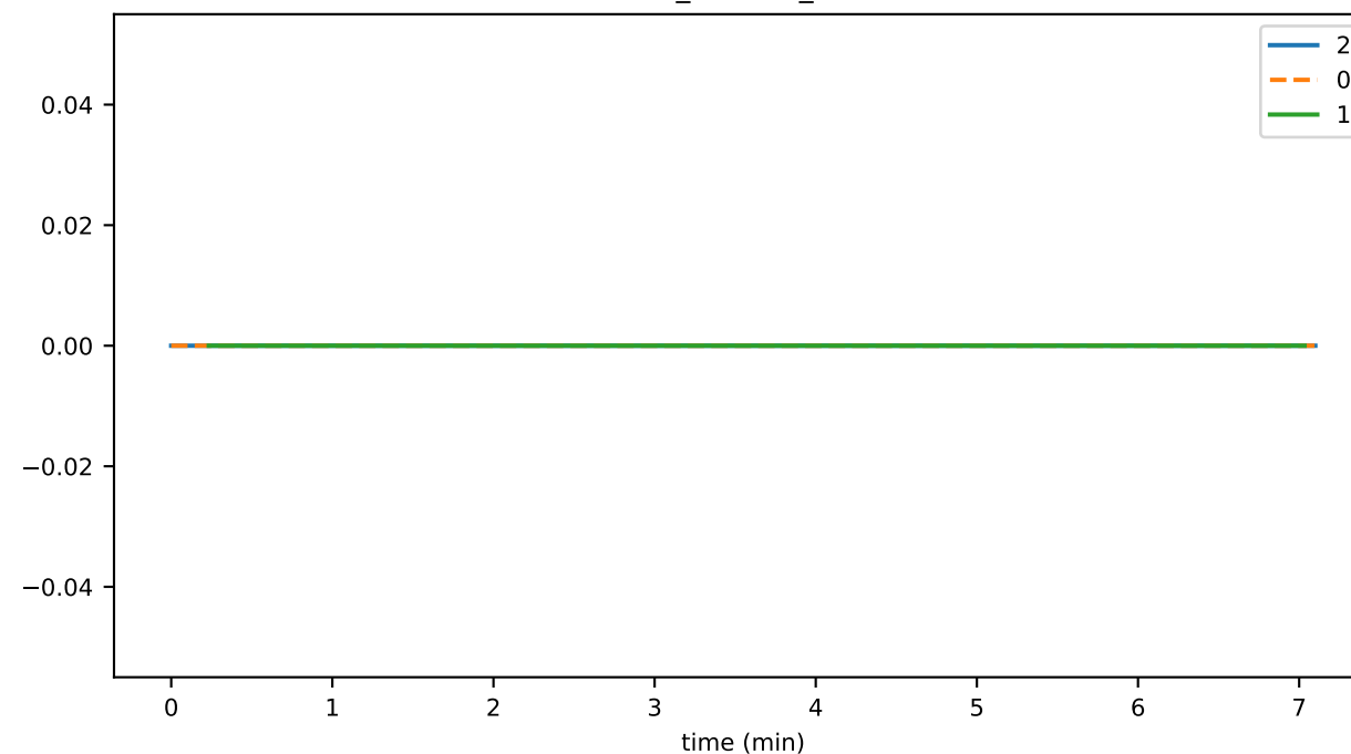
eventCreation_fraction_PLATFORM_STATUS
