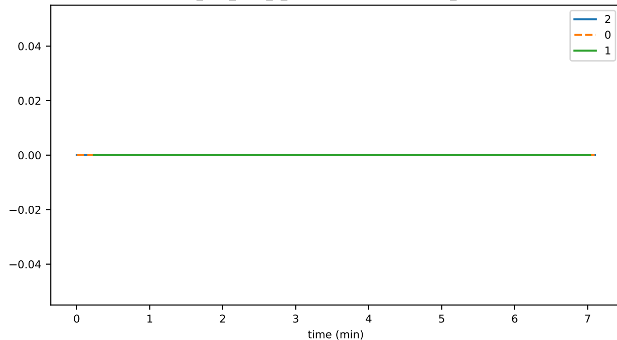
ds_files_level_3_hashesFileSizeByLevelMb_state
