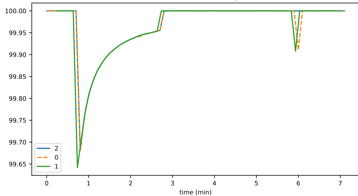
nodeActivePercentSnapshot_node2
