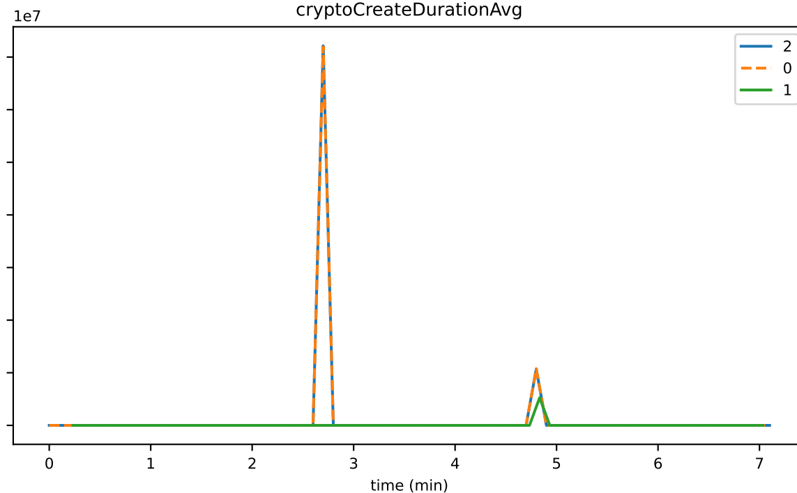
cryptoCreateDurationAvg
