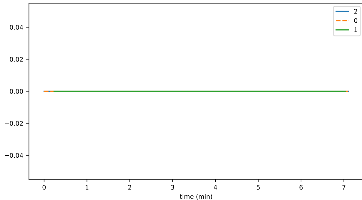
ds_files_level_8_leafKeysFileSizeByLevelMb_state
