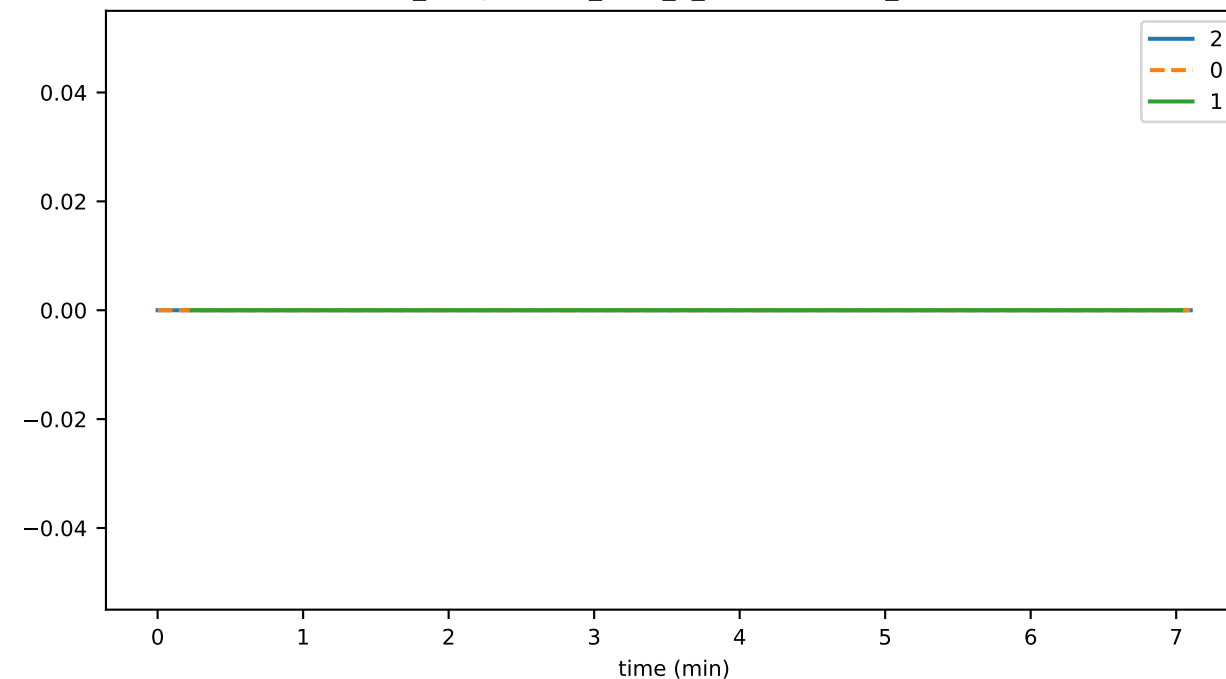
ds_compactions_level_5_hashesTimeMs_state
