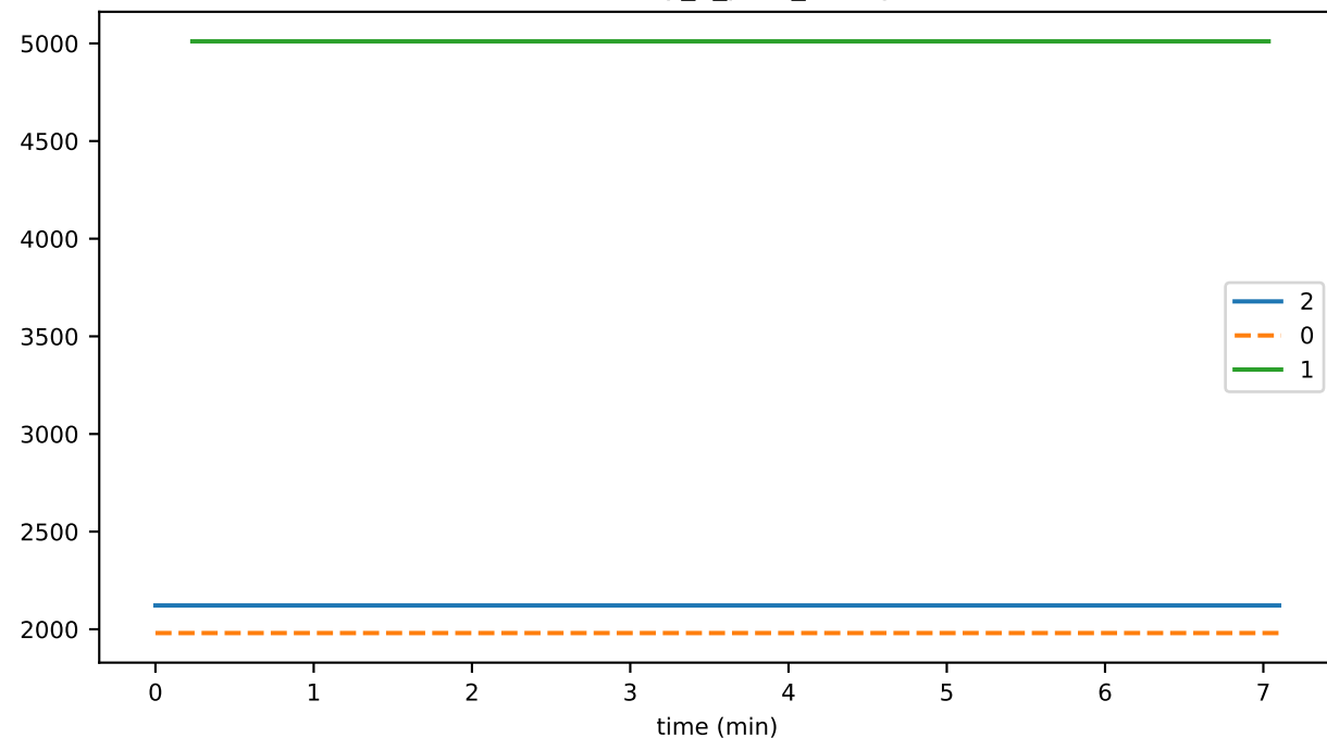
eventDelay_7_consensus_gossip
