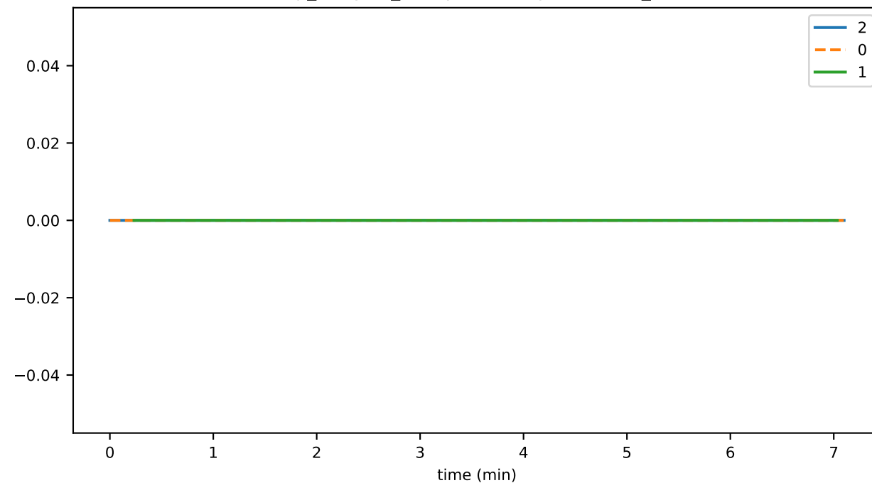
vmap_lifecycle_flushCount_state
