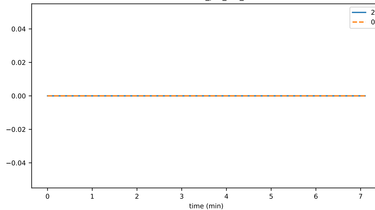
disconnects_per_sec_01
