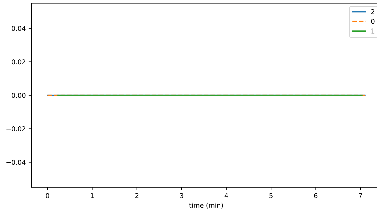
conn_connClose_connectionStalled
