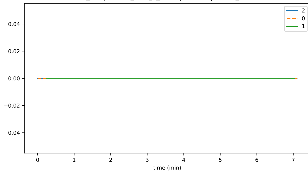
ds_compactions_level_6_leafKeysSavedSpaceMb_state
