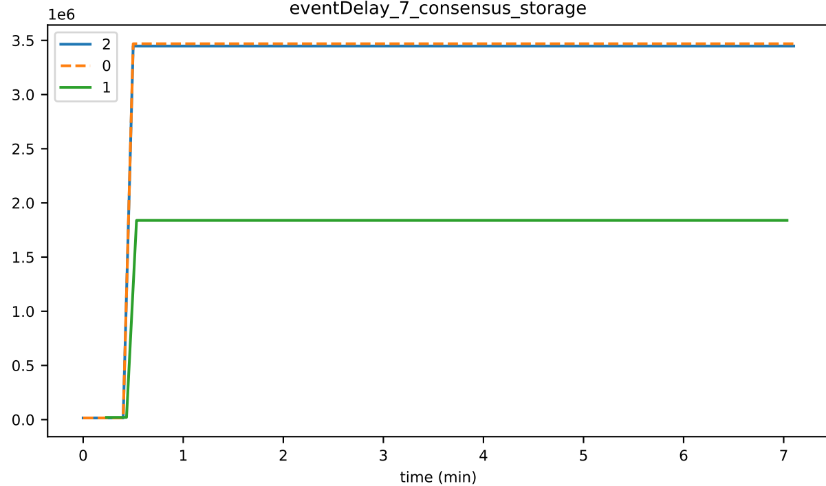
eventDelay_7_consensus_storage
