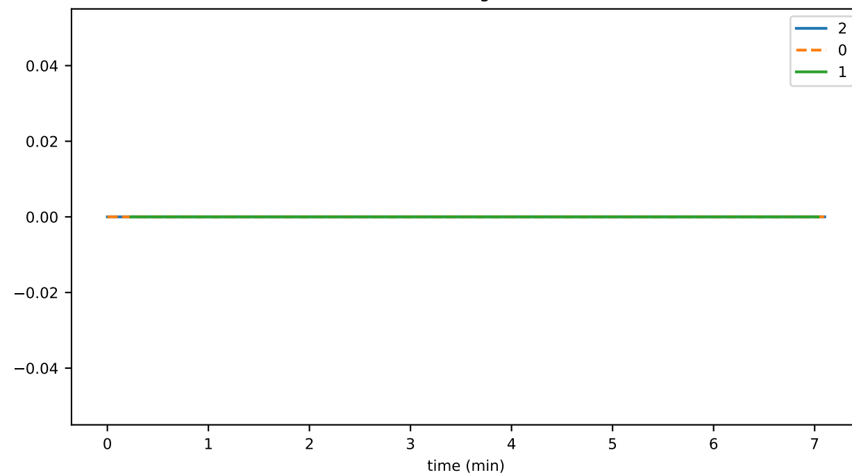
knownSetSize
