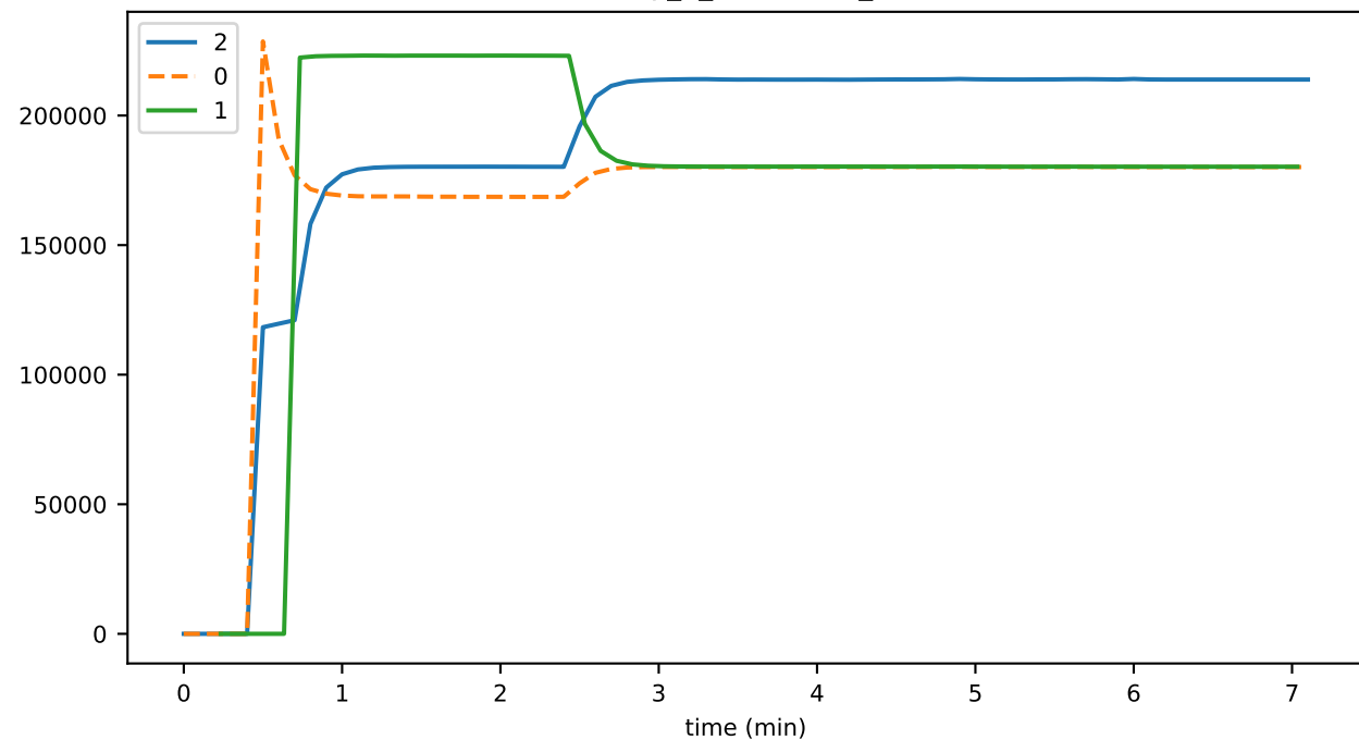
eventDelay_7_consensus_storage
