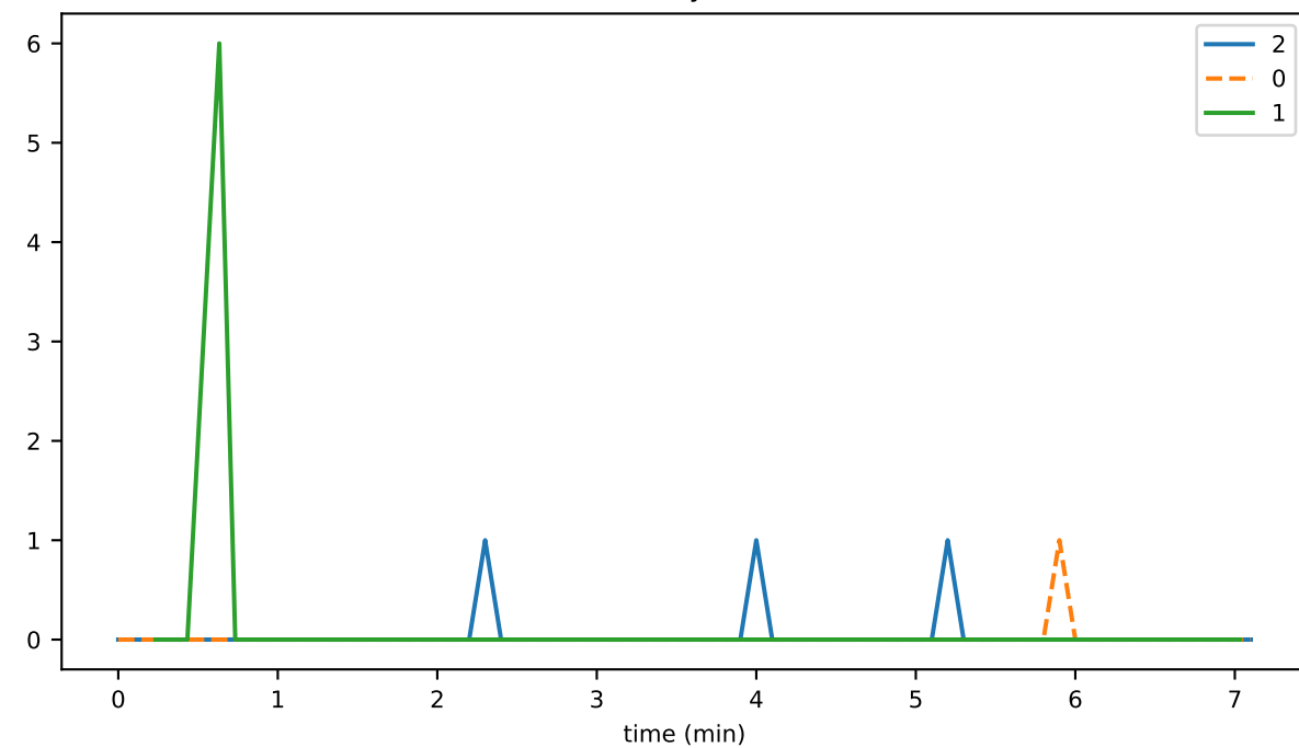
bufferedPriorityTransactions
