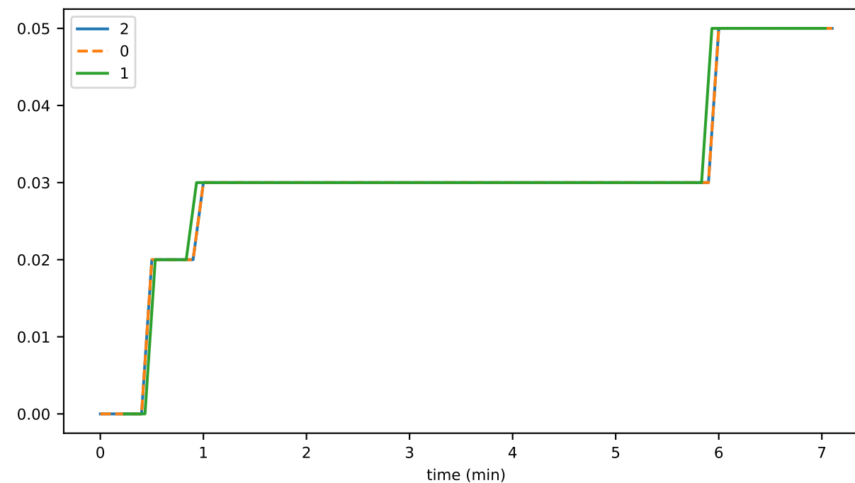
disconnects_per_sec_01
