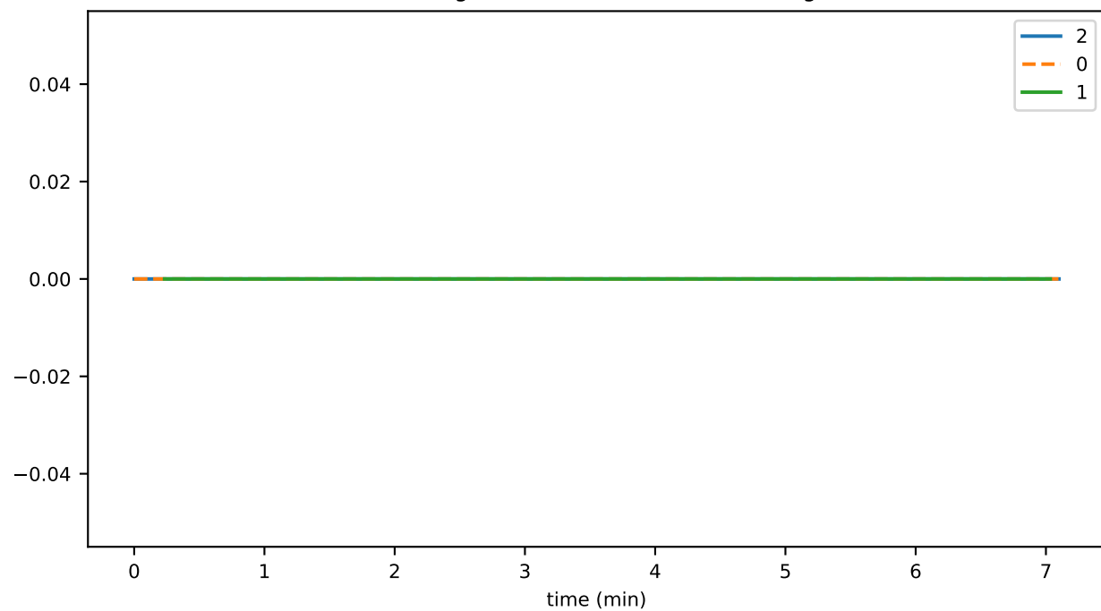
stateSignatureTransactionDurationAvg
