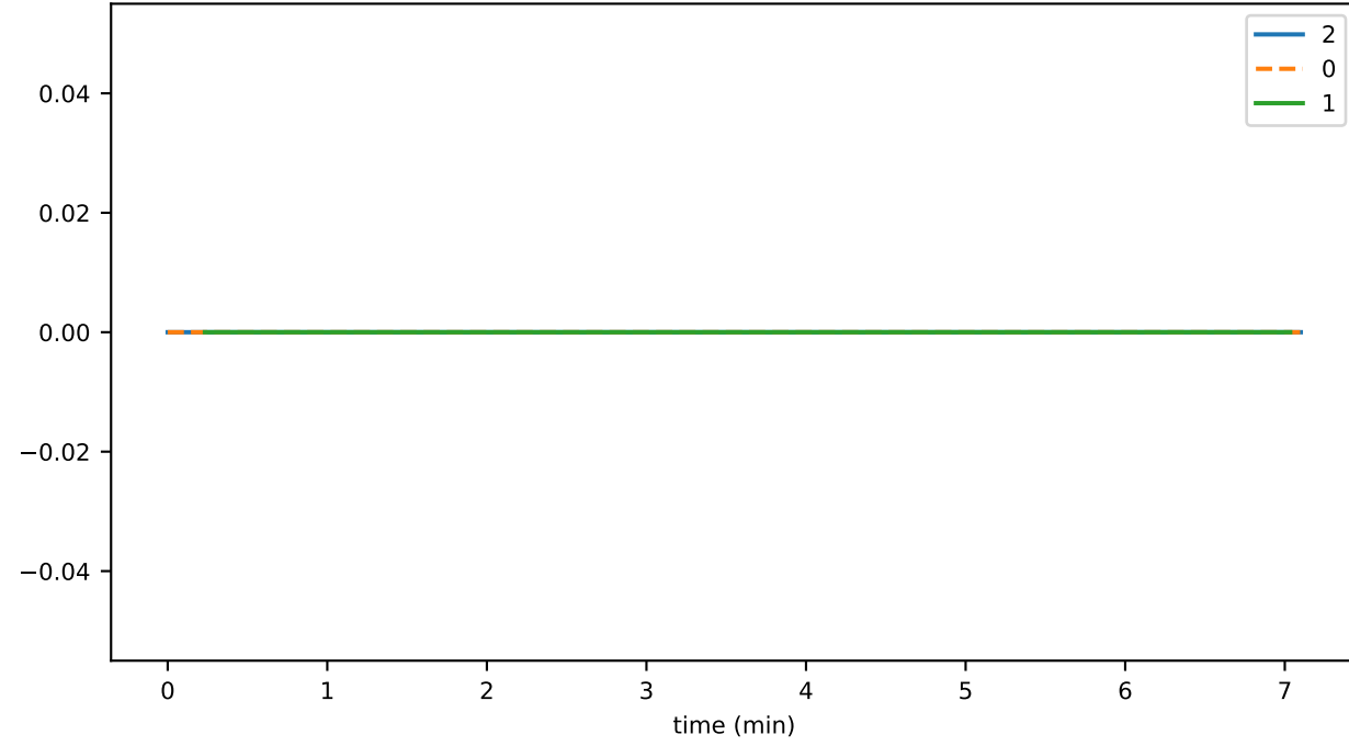
migrationRootHashVoteThrottledTxns
