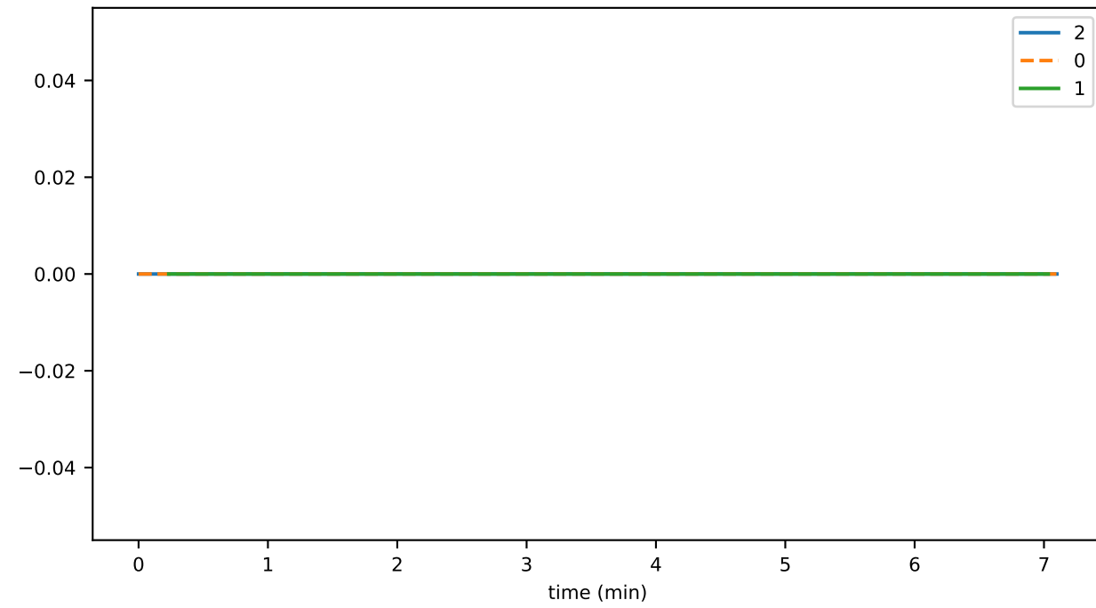
PlatformStatus
