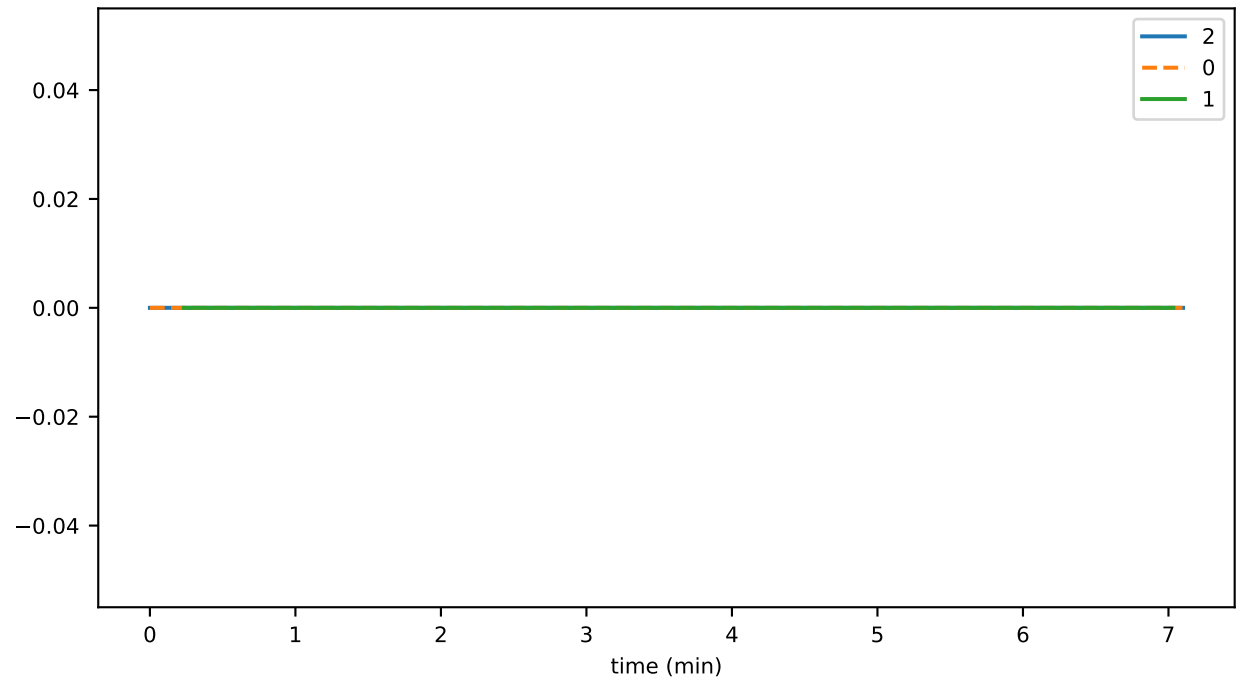
ds_compactions_level_9_leavesSavedSpaceMb_state
