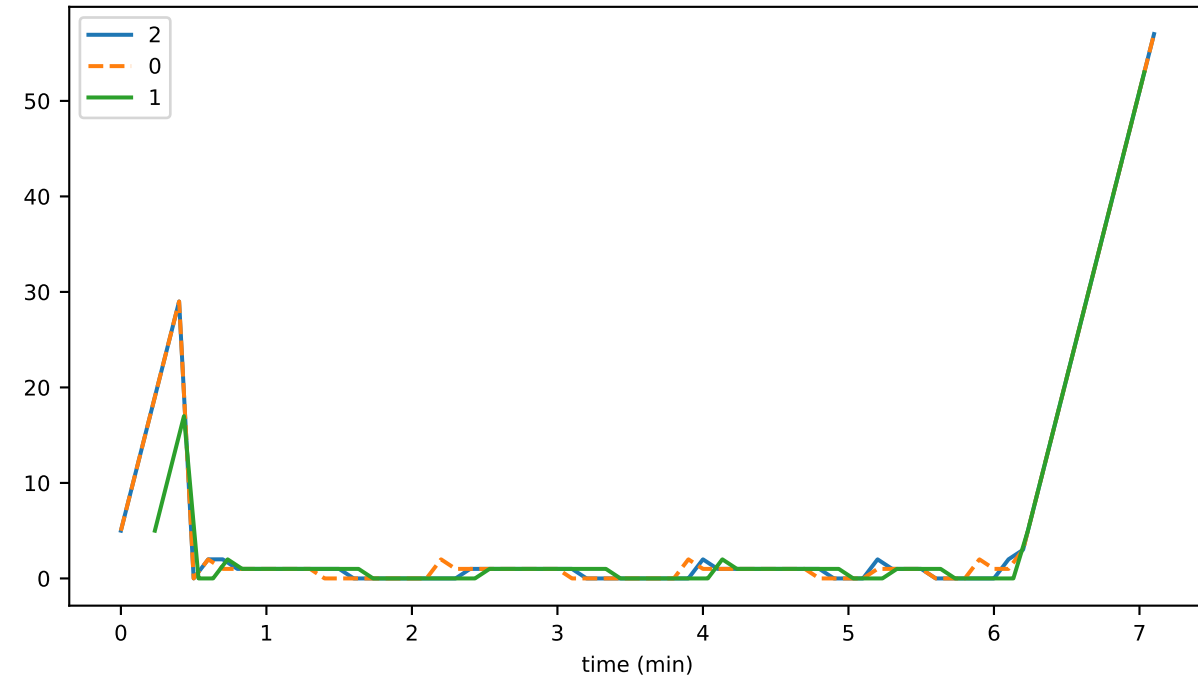
OrphanBuffer_busy_fraction
