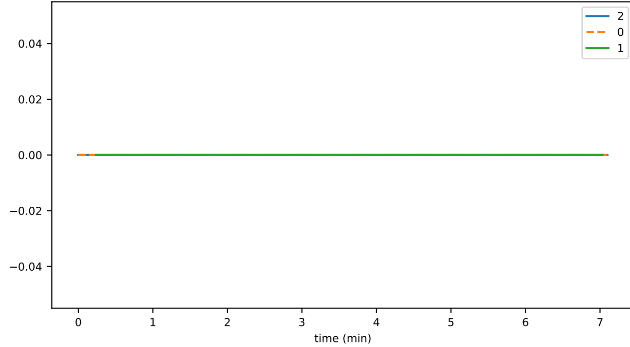
ds_compactions_level_9_hashesSavedSpaceMb_state
