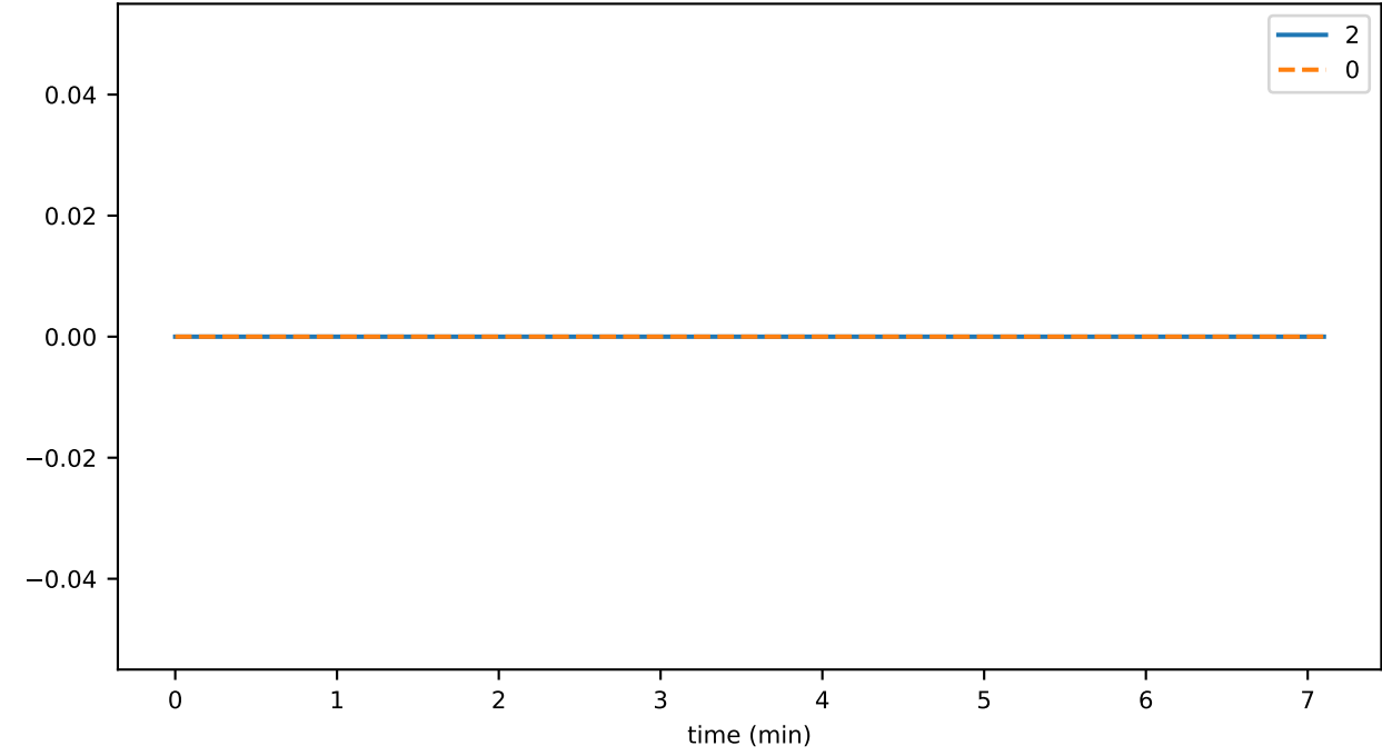
sync_phase_01_fraction_SENDING_EVENTS
