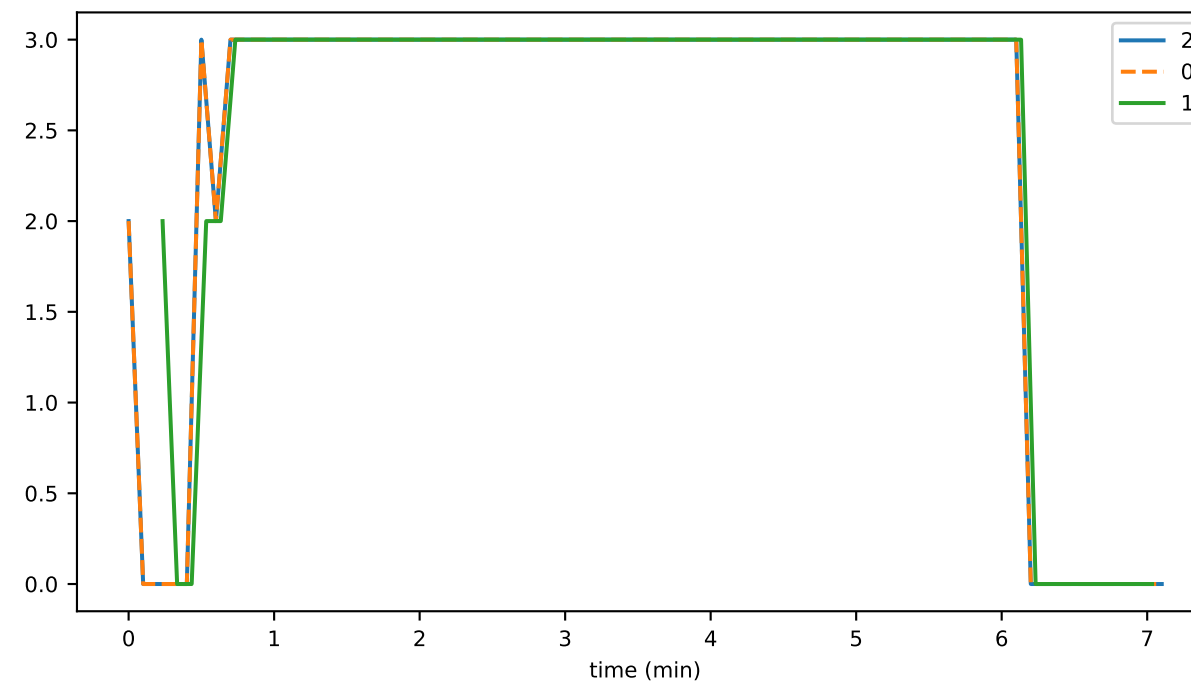
witnessesSeenMAX
