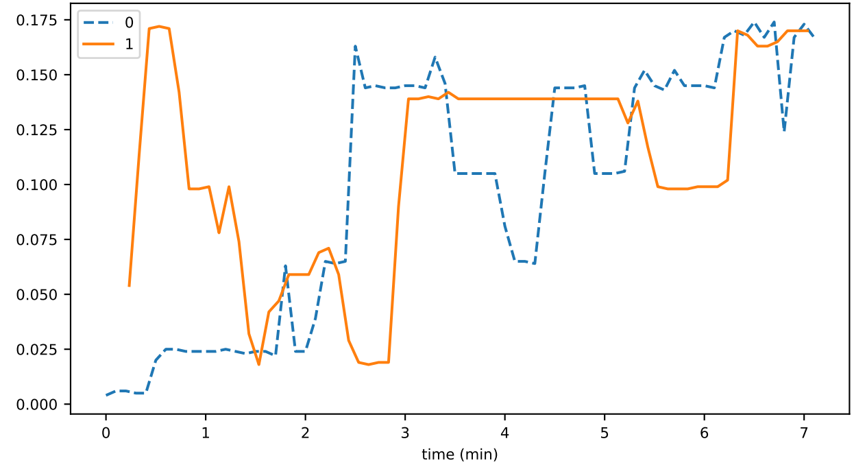
sync_phase_02_fraction_GOSSIP_HALTED
