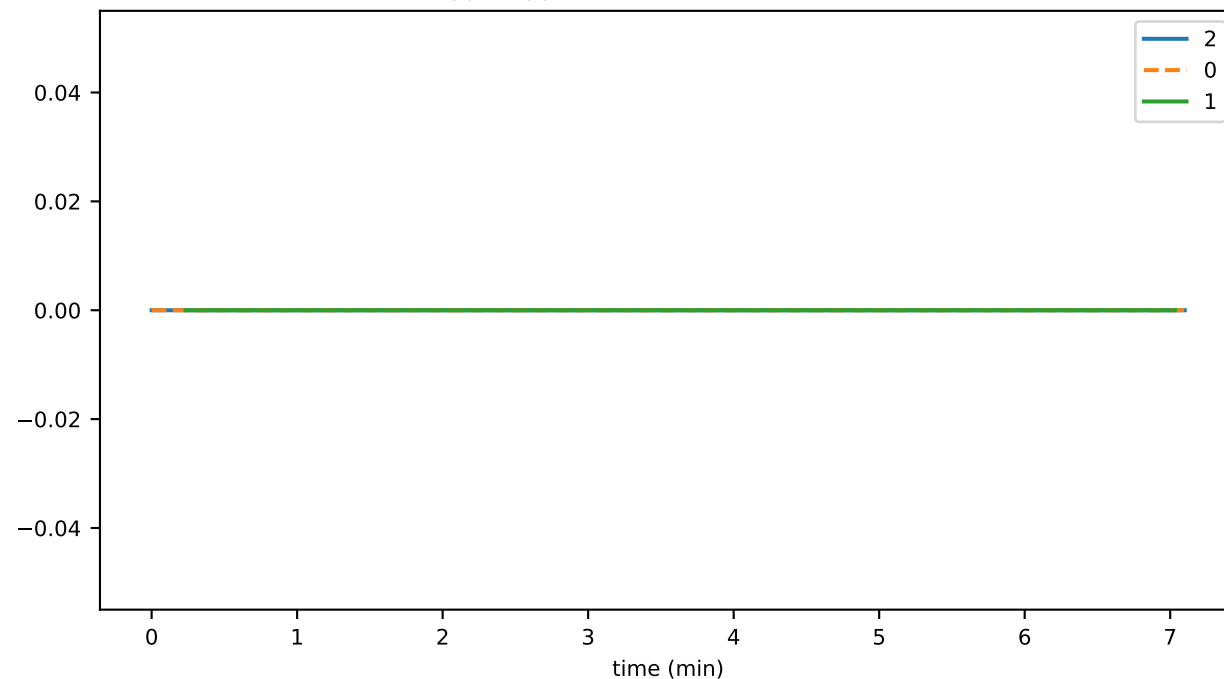
cryptoCreateDurationAvg
