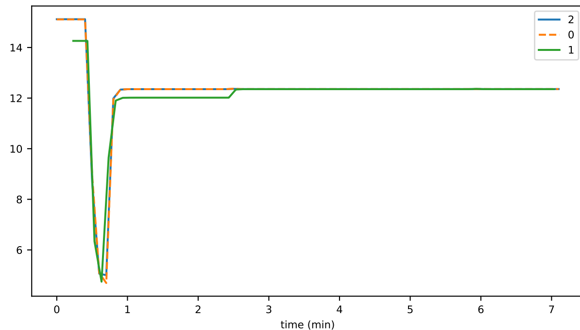
numEventsAddedUntilConsensus
