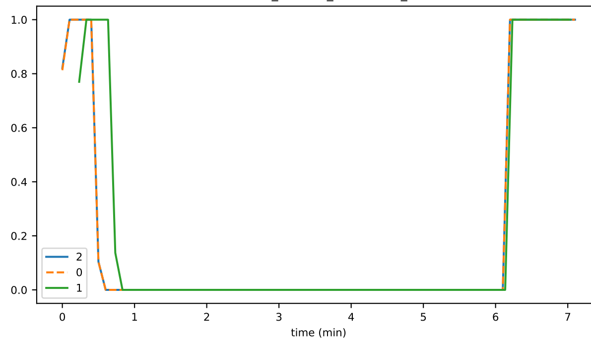
eventCreation_fraction_PLATFORM_STATUS
