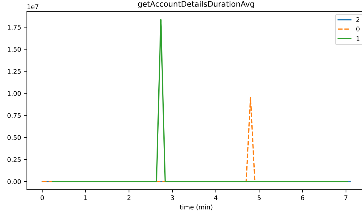
getAccountDetailsDurationAvg
