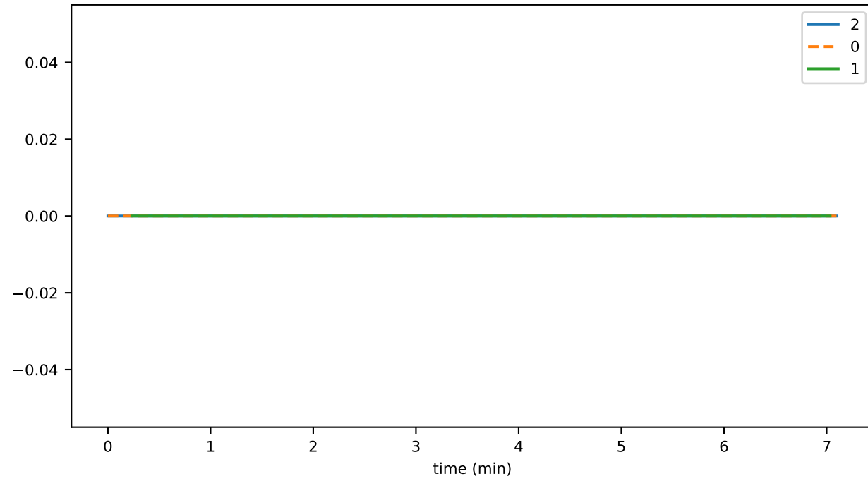
migrationRootHashVoteThrottledTxns
