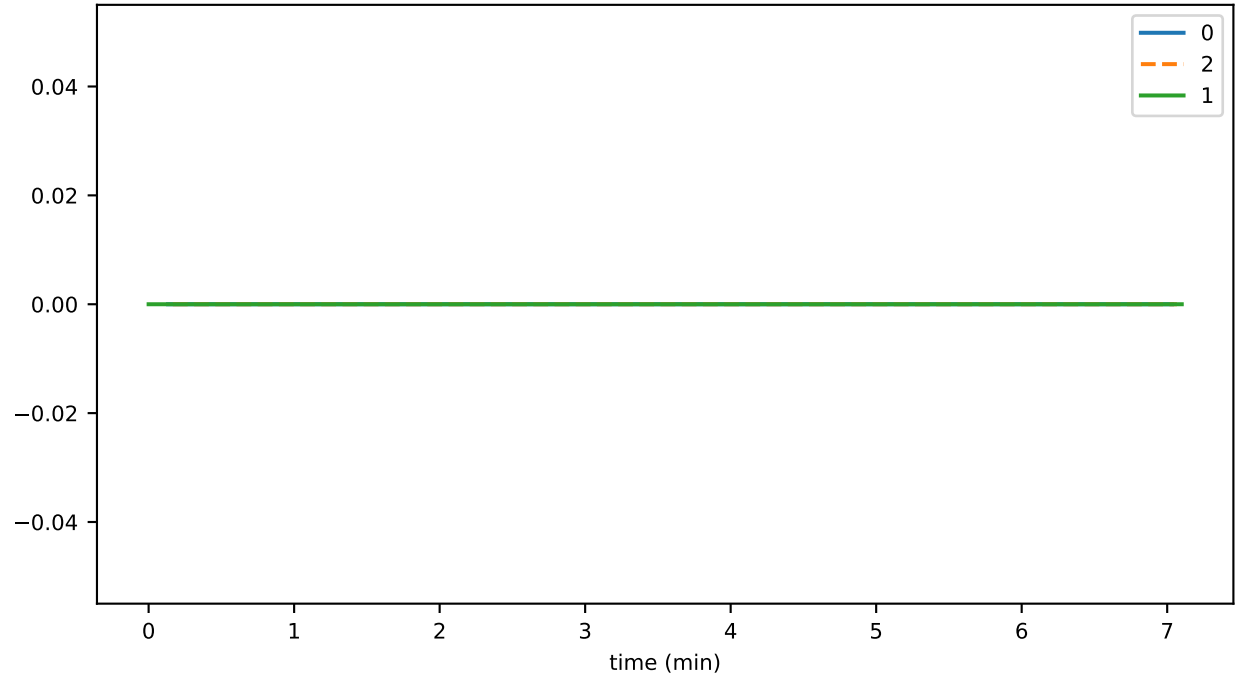
cryptoTransferDurationAvg
