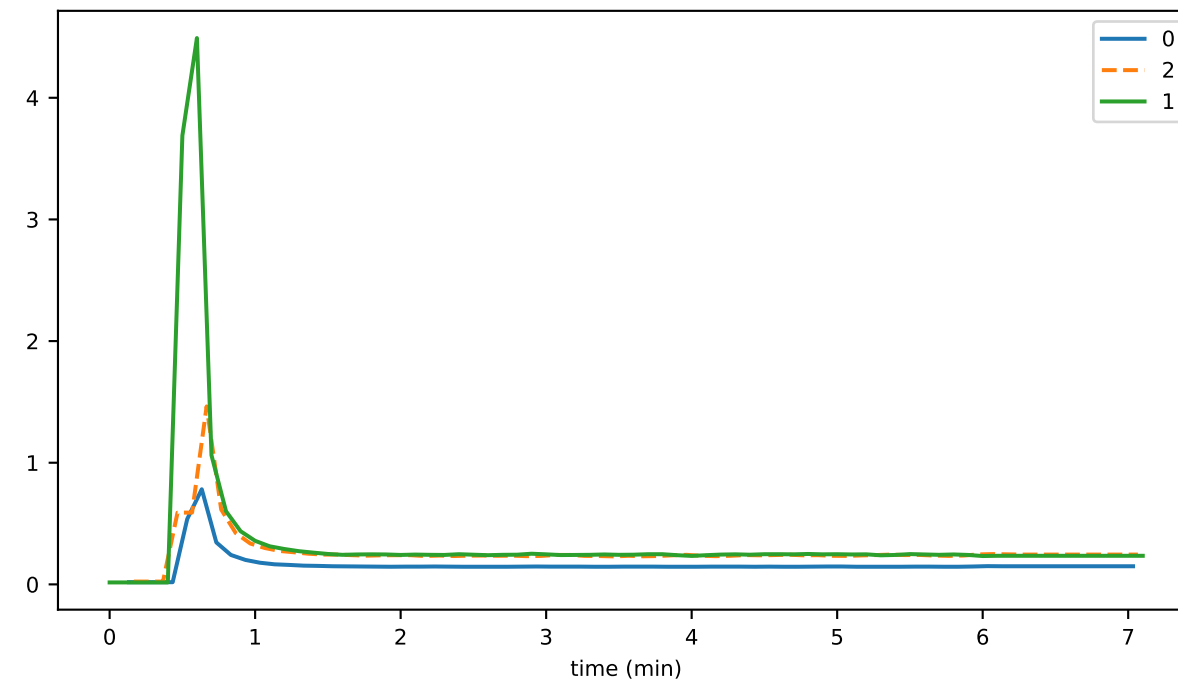
memFree
