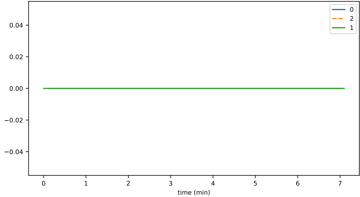
cryptoGetStakersThrottledTxns
