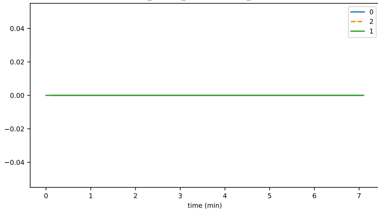
ds_offheap_leavesIndexMb_state
