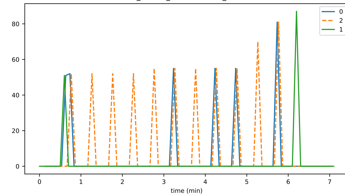
ds_flushes_leafKeysWritten_state
