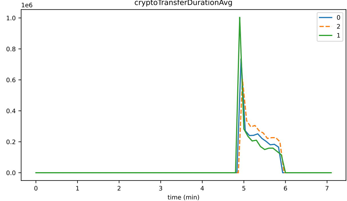
cryptoTransferDurationAvg
