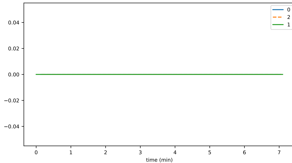
receiverReconnectDurationSeconds
