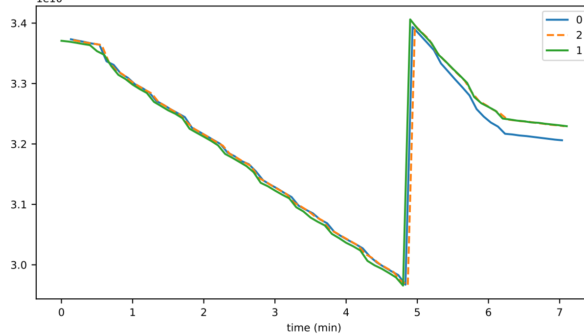
memFree
