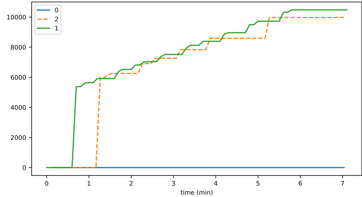
getAccountDetailsDurationAvg
