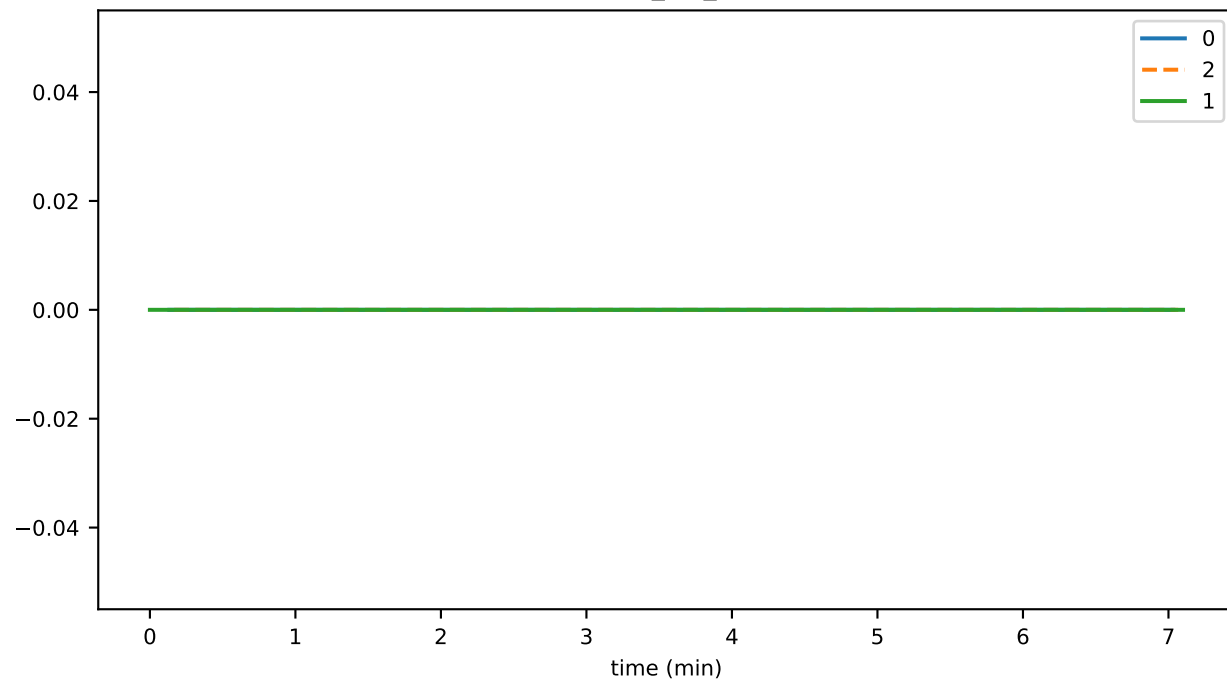
recycled_file_count
