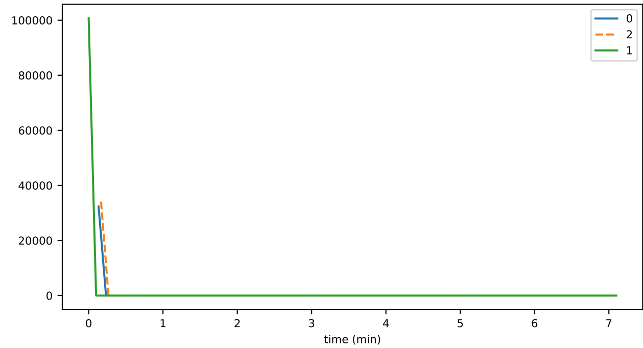
eventDelay_5_orphanBuffer_storageMAX
