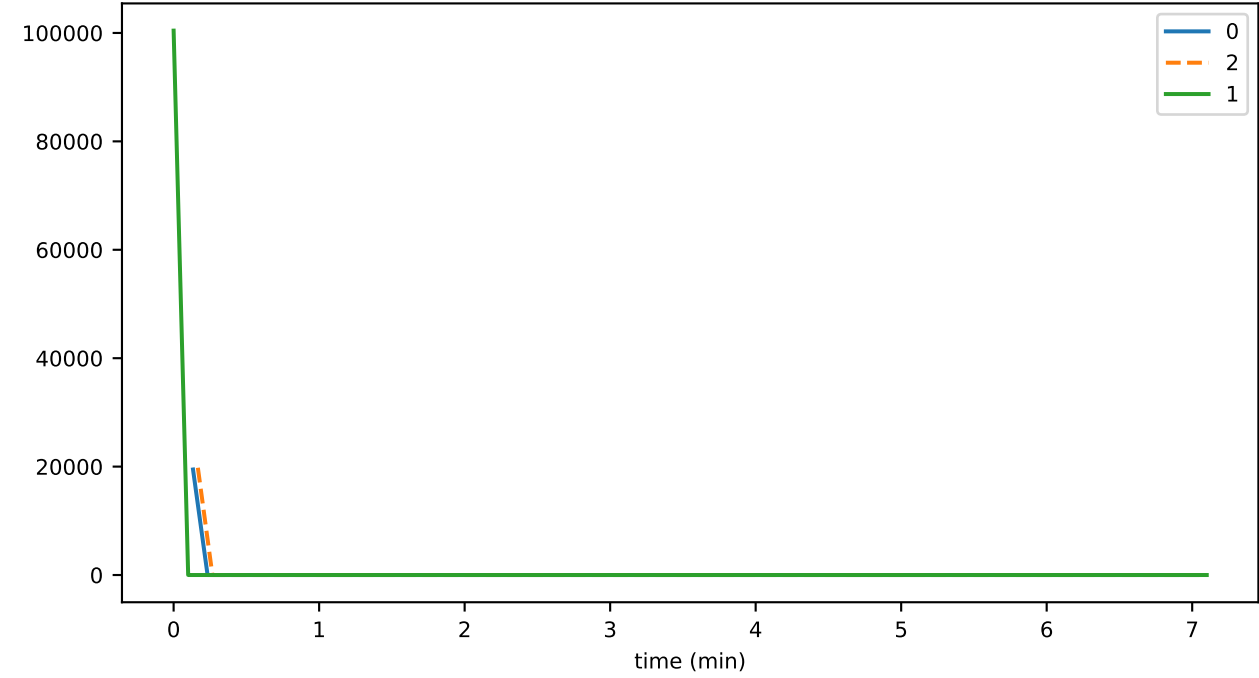
eventDelay_3_deduplication_storageMAX
