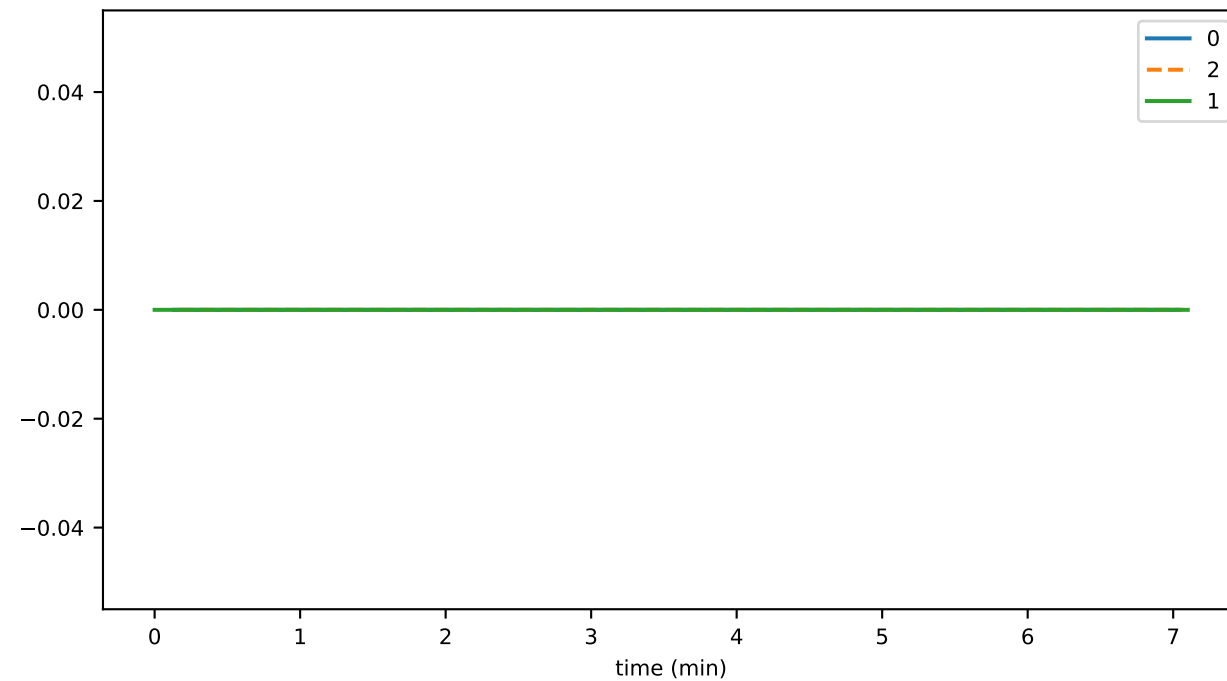
scheduleGetInfoDurationMax
