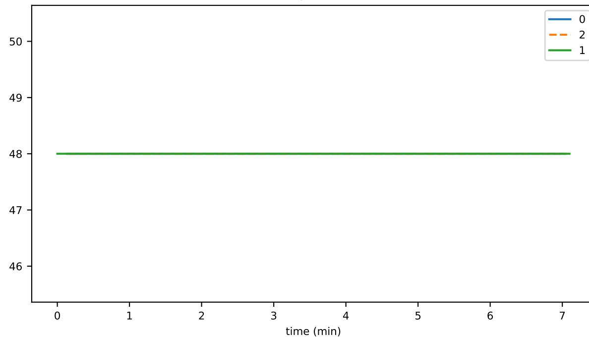
receiverReconnectDurationSeconds
