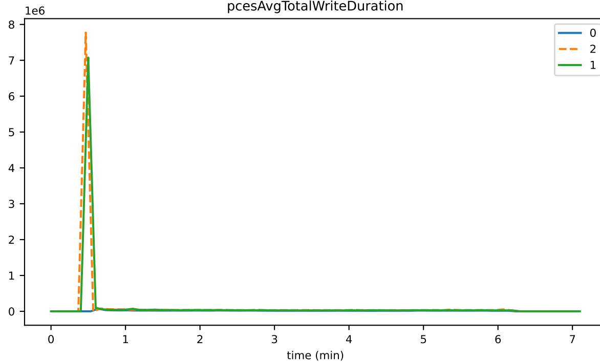
pcesAvgTotalWriteDuration
