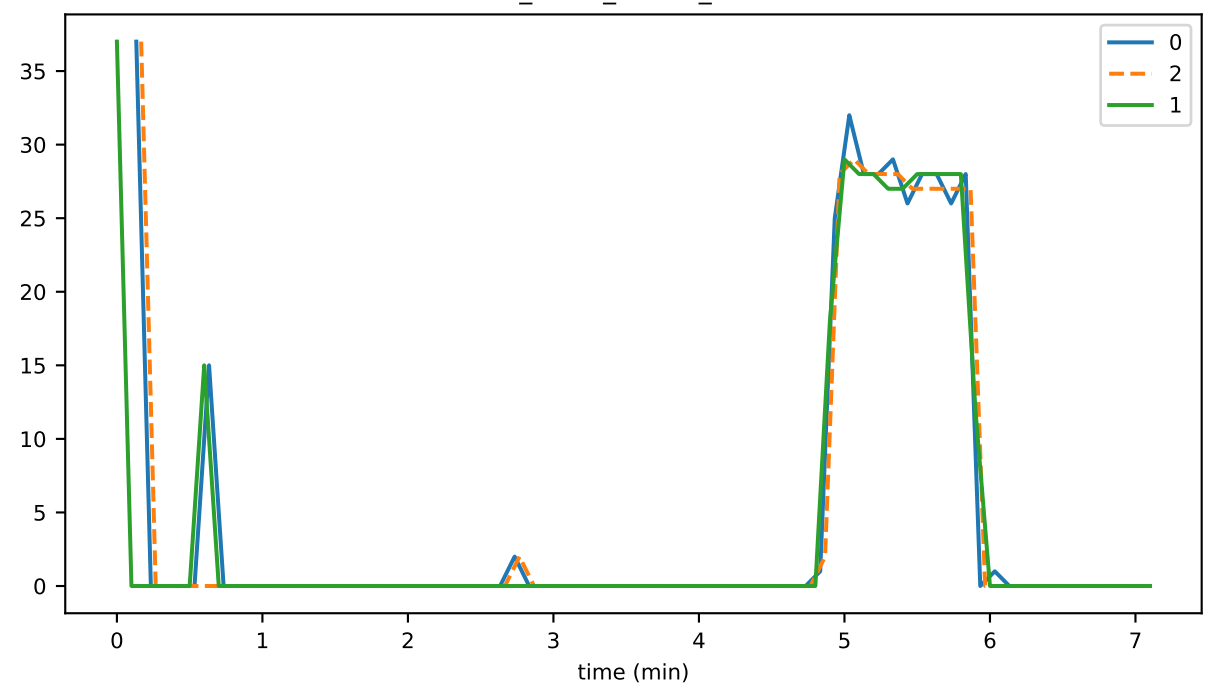
ds_reads_leaves_state
