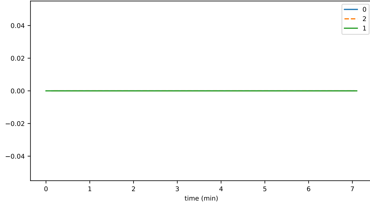
scheduleSignDurationMax
