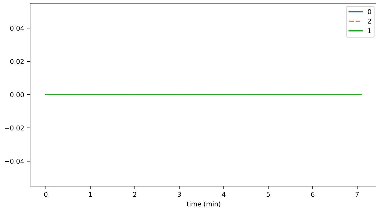
scheduleGetInfoDurationAvg
