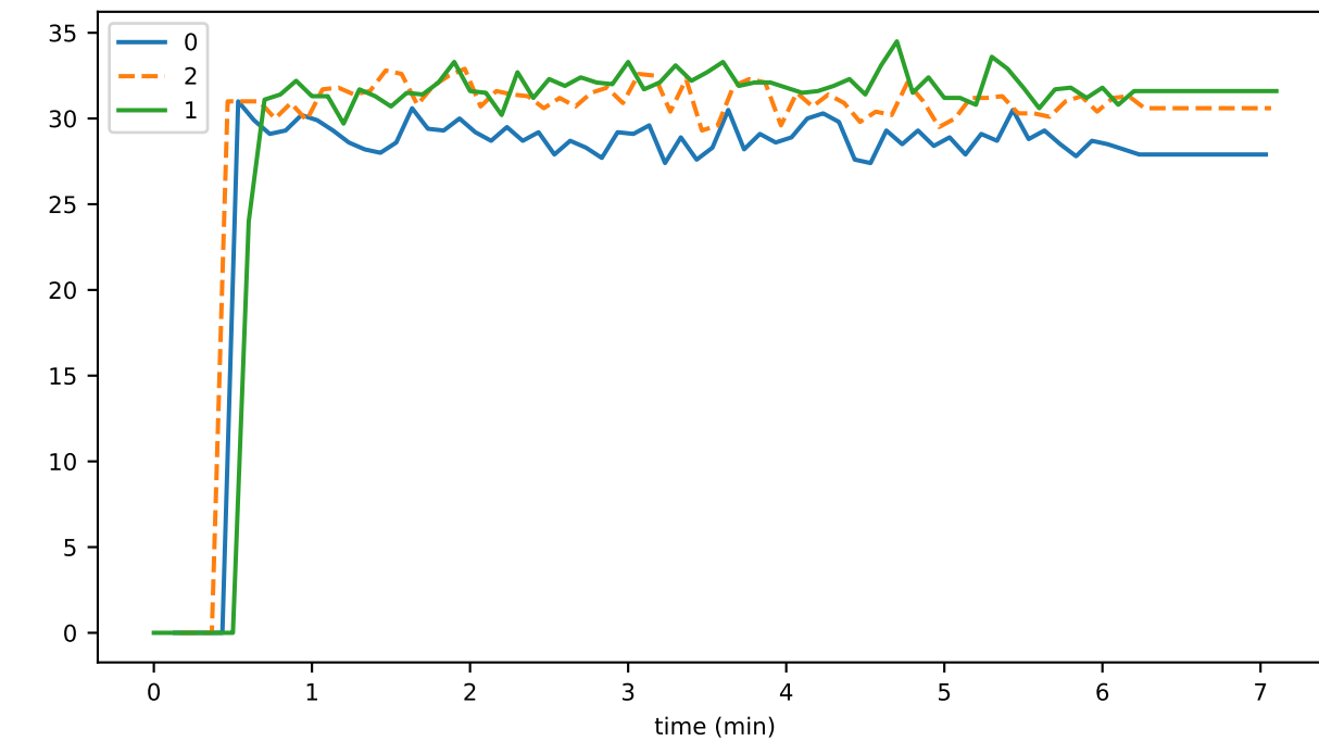
eventsFailedSignatureValidation
