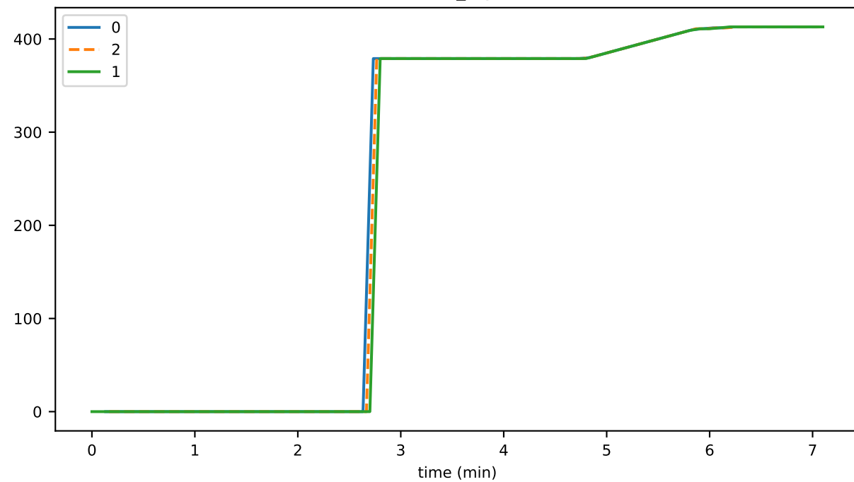
recycled_file_count
