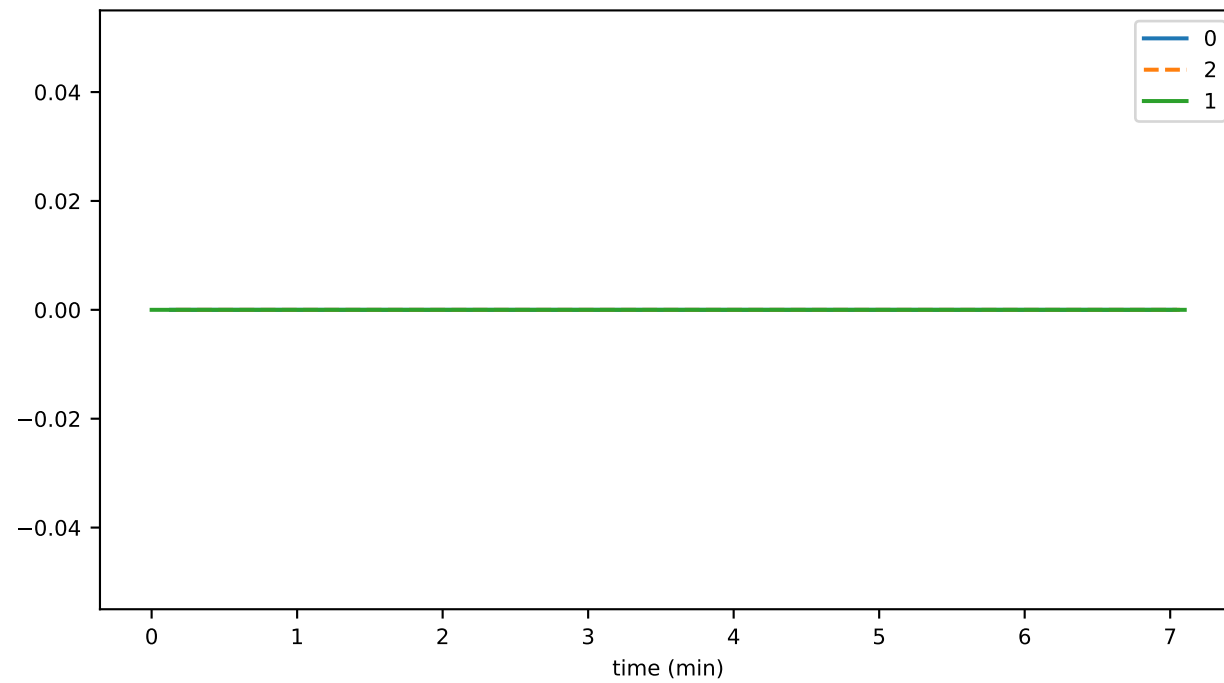
systemDeleteThrottledTxns
