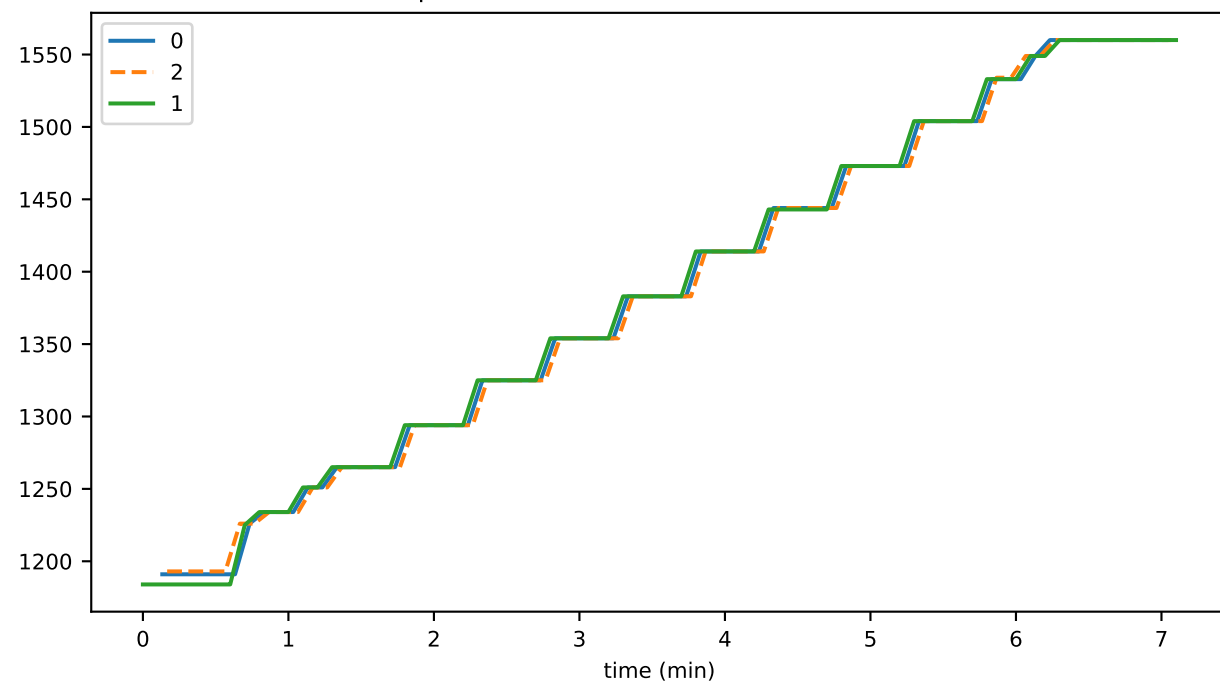
preconsensusEventFileTotalSizeGB
