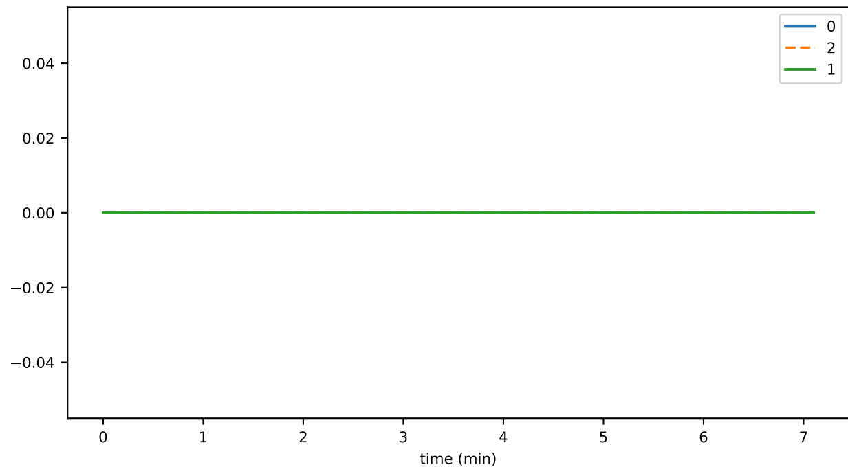
systemDeleteDurationMax
