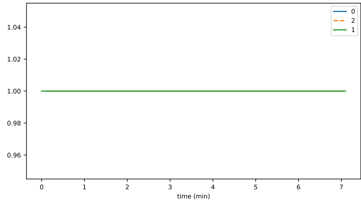
hintsKeyPublicationDurationAvg
