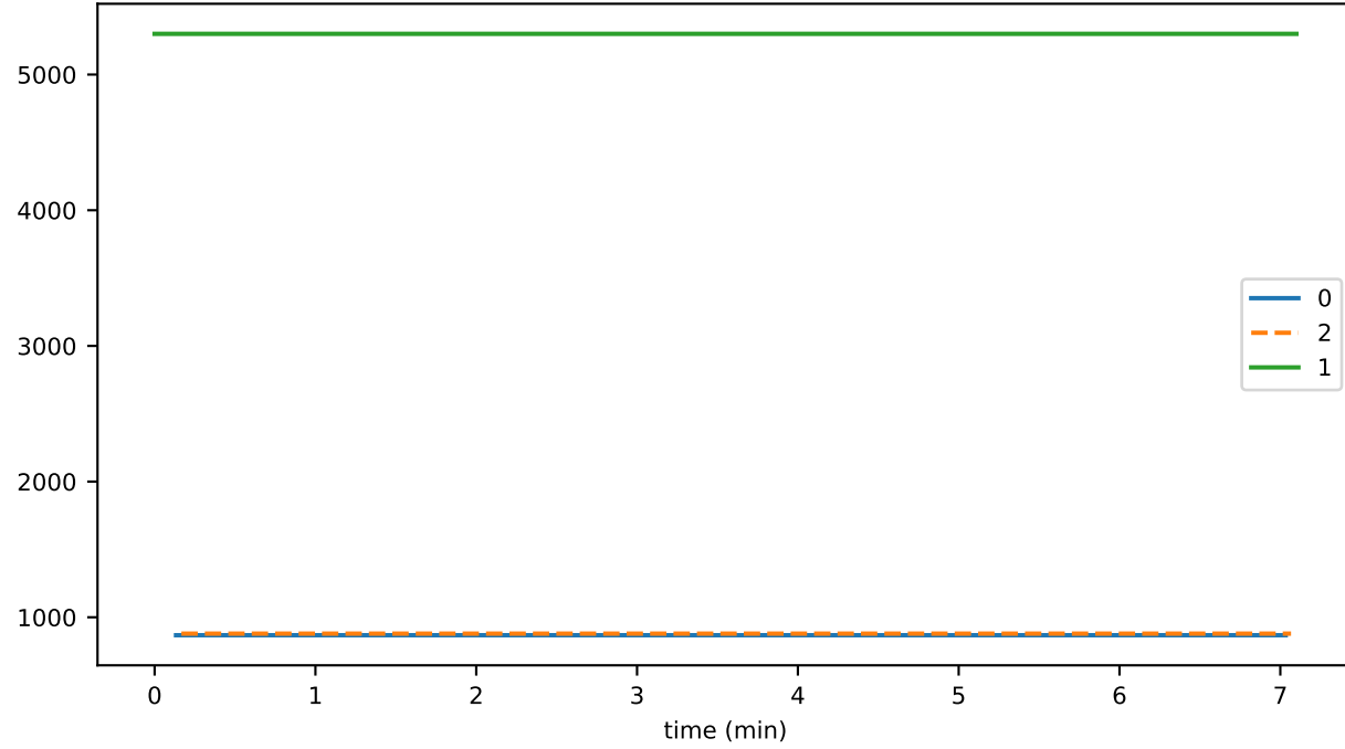
eventDelay_3_deduplication_storage
