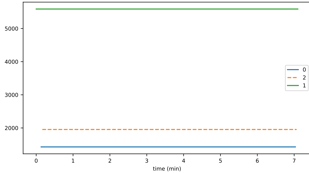
eventDelay_5_orphanBuffer_storage
