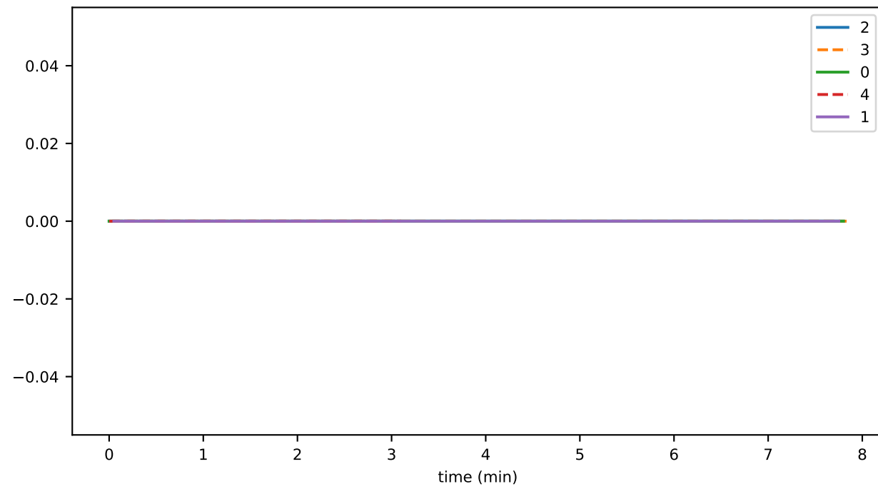
totalNeverSignedDiskStates
