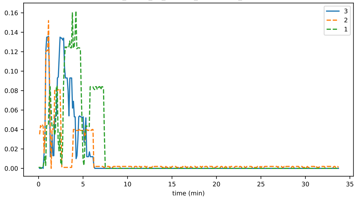
sync_phase_00_fraction_RECEIVING_EVENTS
