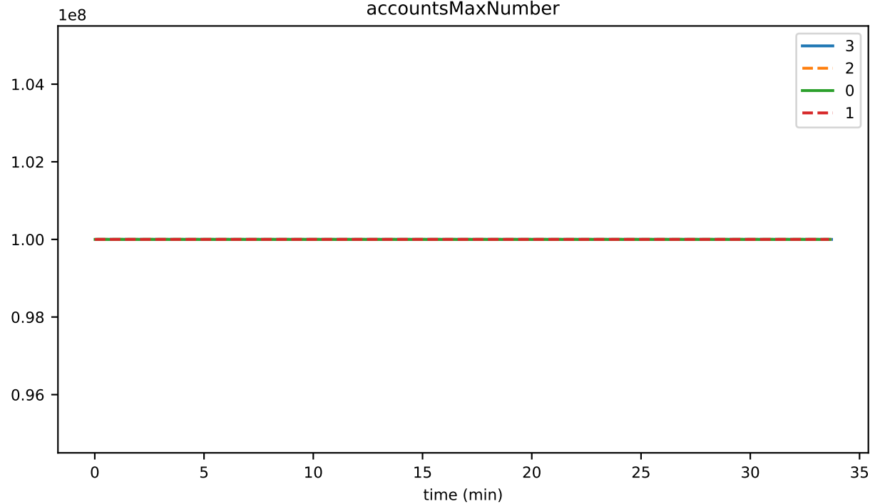
accountsMaxNumber
