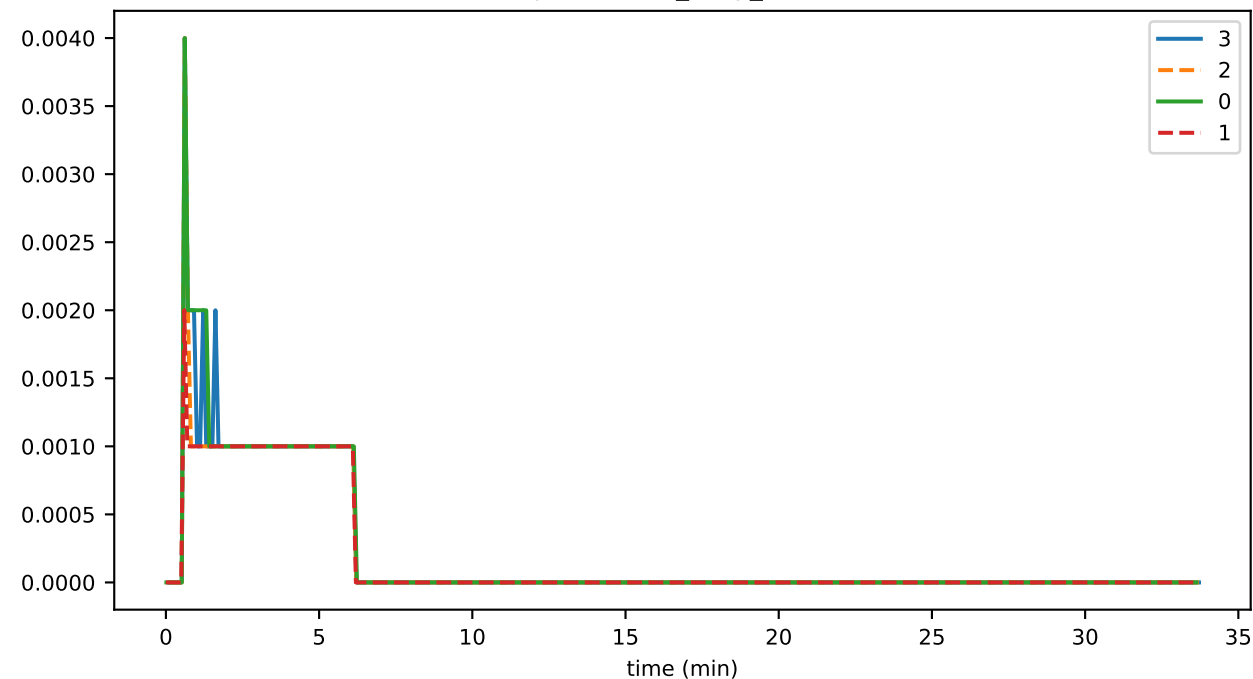
orphanBufferSize
