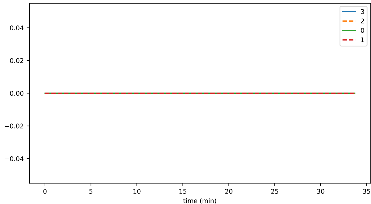
SigIntakePulseTime
