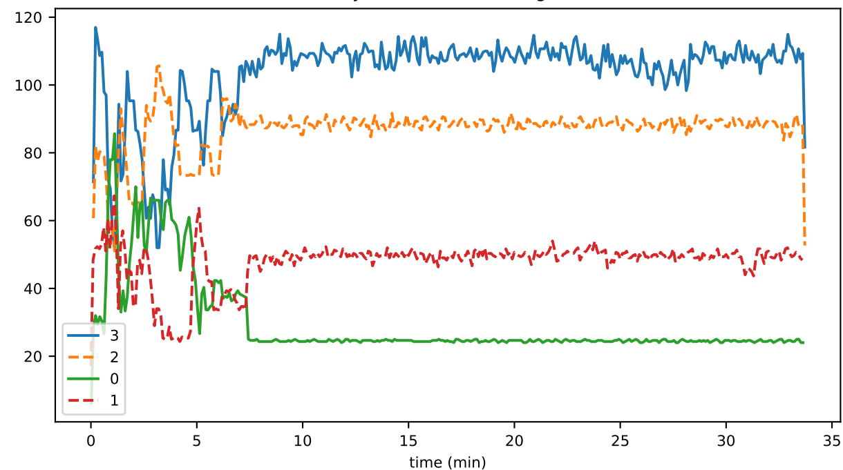
doNotSyncRemoteProcessingEvents
