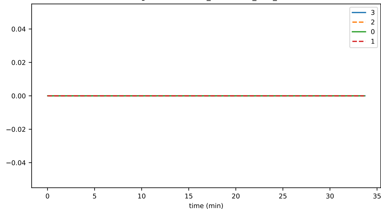
StateSigner_unhandled_task_count
