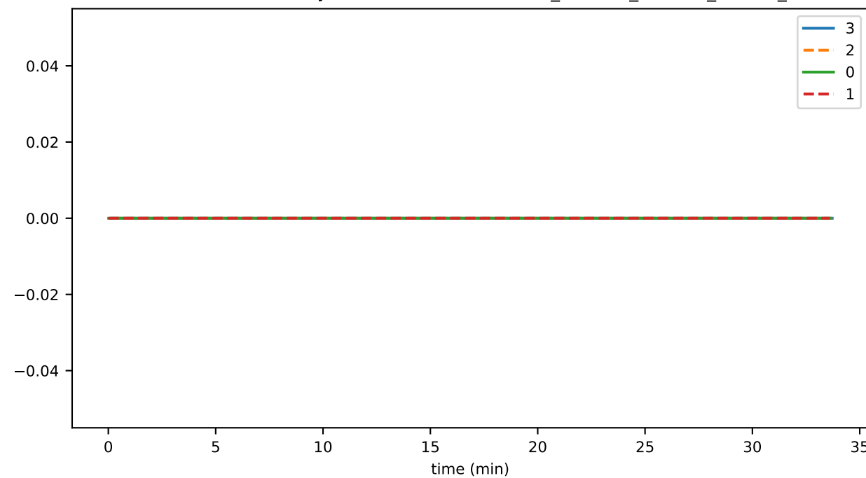
SmartContractService:SystemContractMethodCall_CREATE_DELETE_TOKEN_failed
