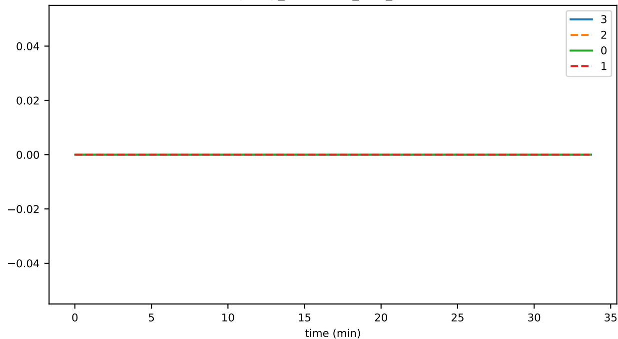
graphDepthUntilConsensusMAX
