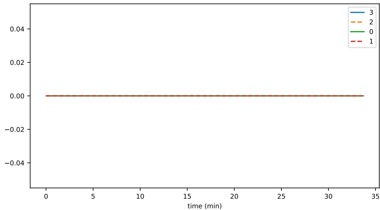
startsReconnectAsReceiver
