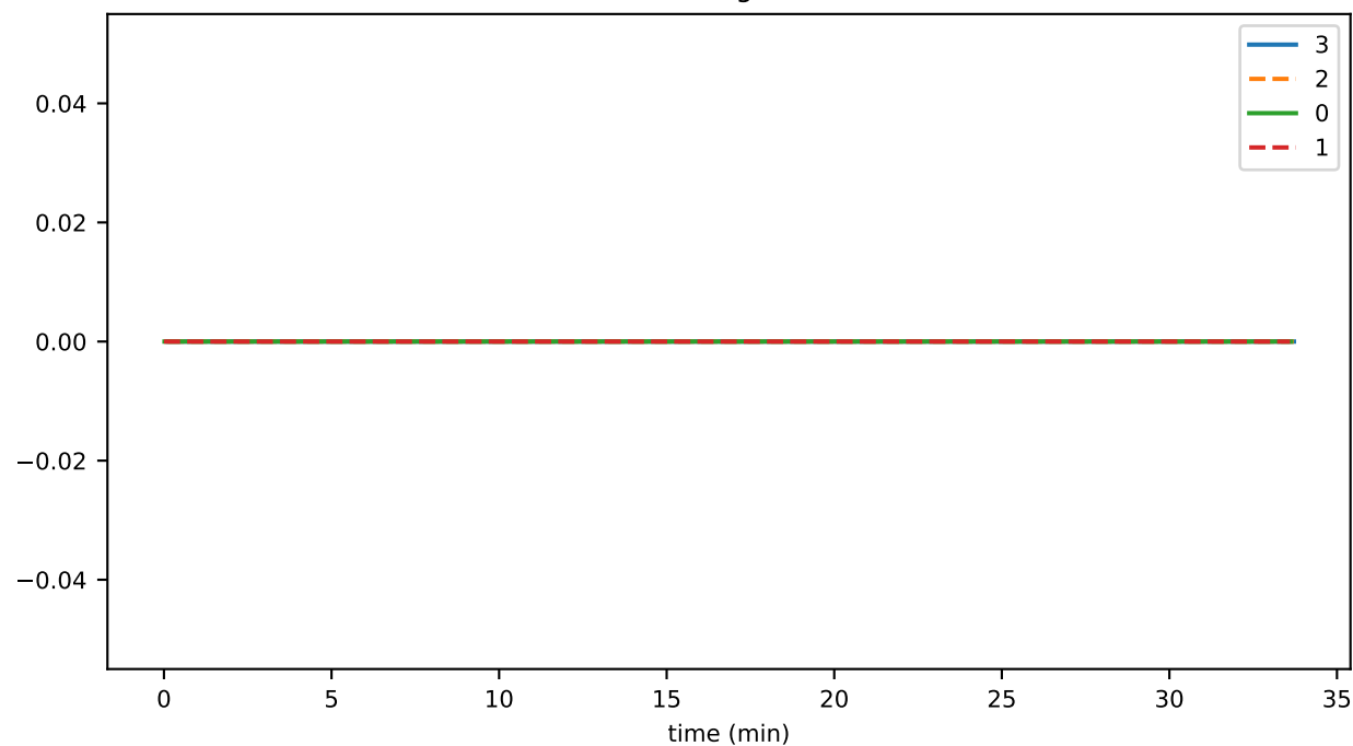
trans_per_event
