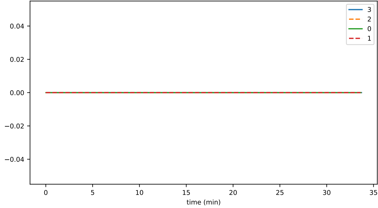
airdropsUsed
