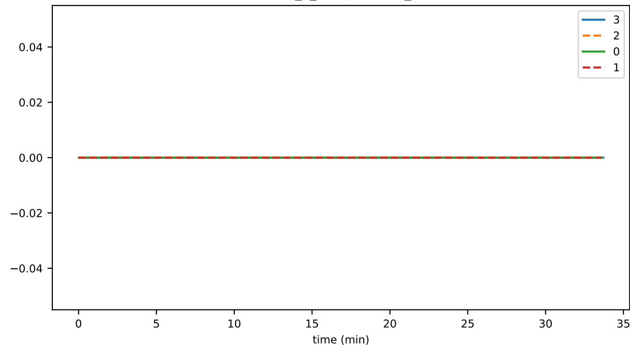
eventDelay_4_verification_gossip
