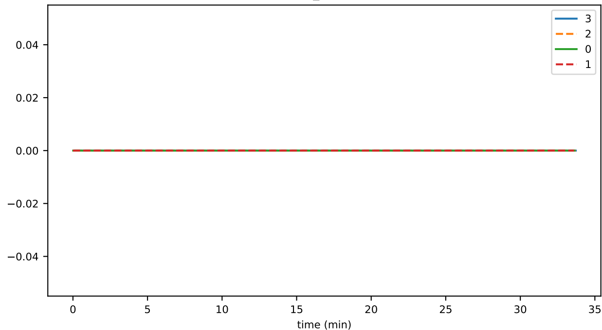
connRecv_resendBlock
