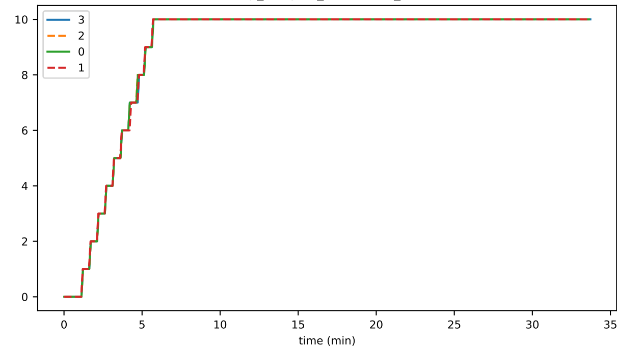
vmap_lifecycle_hashDurationMs_state
