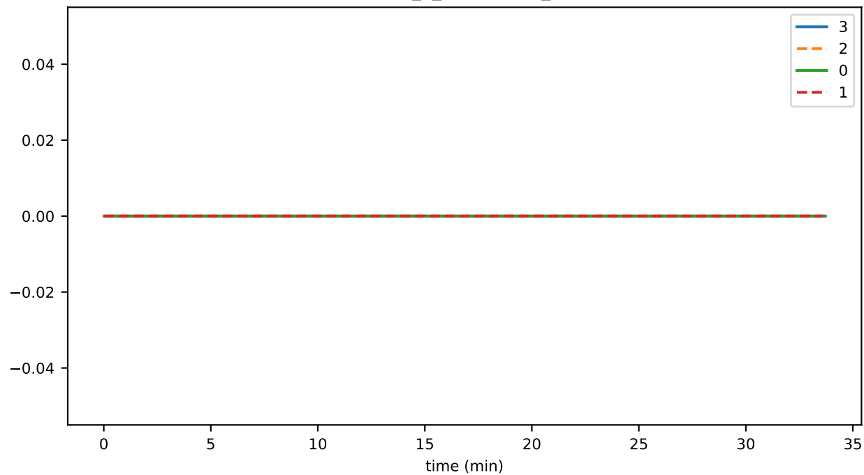
eventDelay_4_verification_storage
