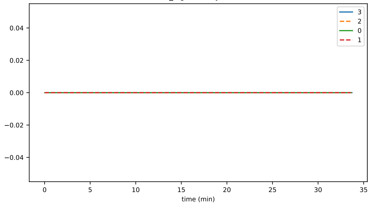
conn_highLatencyEvents
