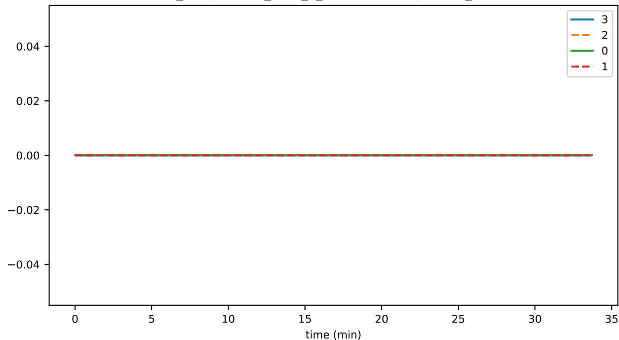
ds_compactions_level_9_leafKeysSavedSpaceMb_state
