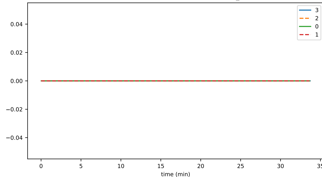
sstatesSigned_per_sec
