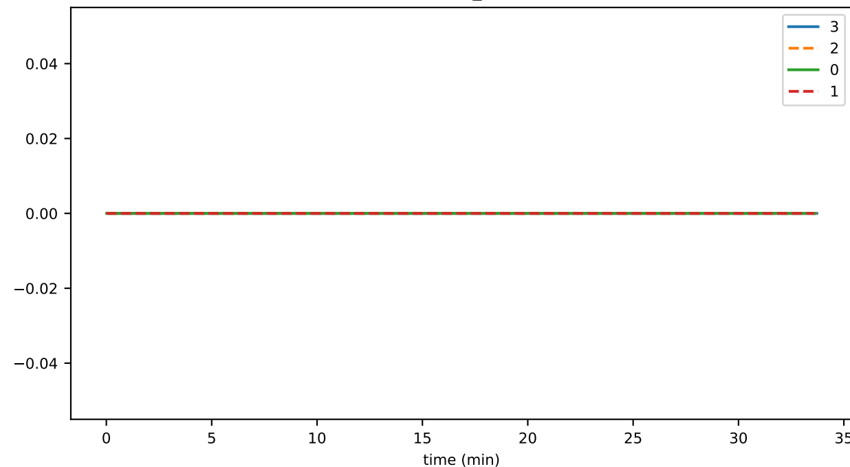
connSend_multitemRequestExceedsSoftLimit
