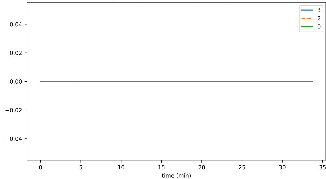
sync_phase_01_fraction_SELF_FALLEN_BEHIND
