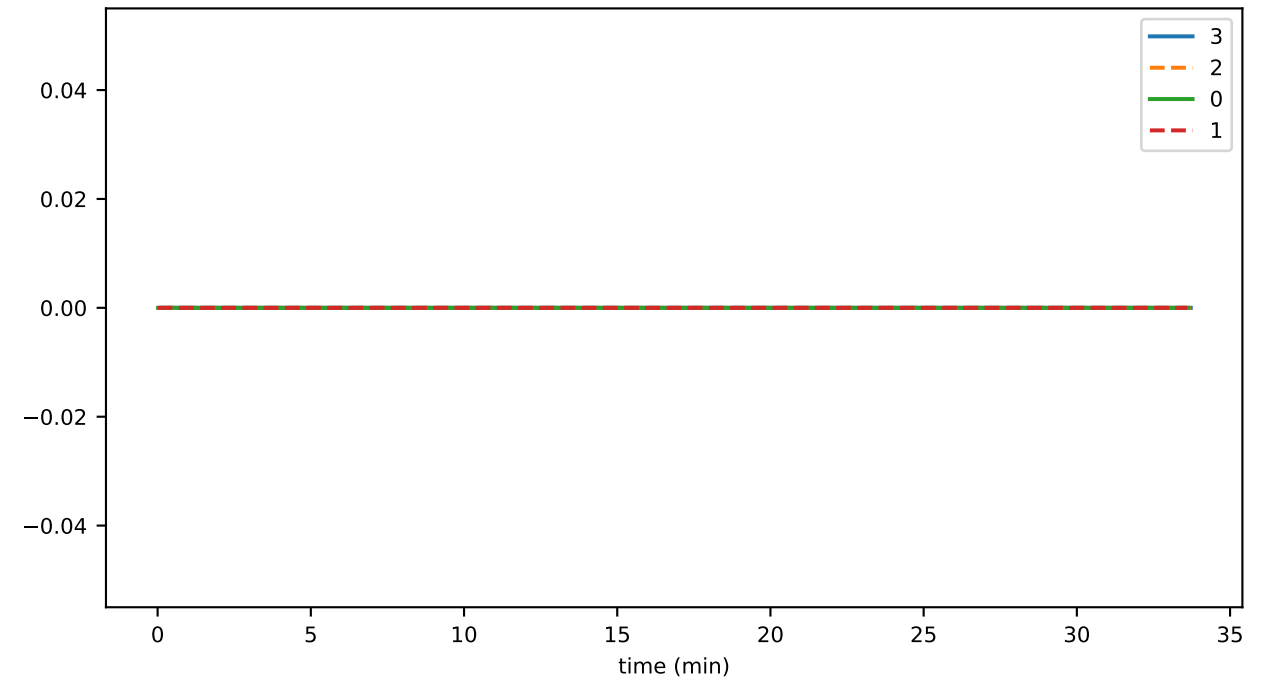
ds_compactions_level_4_leavesTimeMs_state
