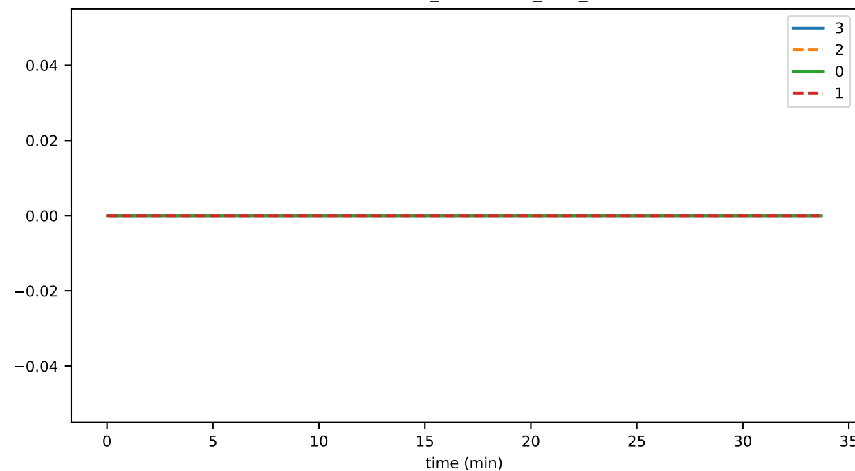
branchingNodeCount
