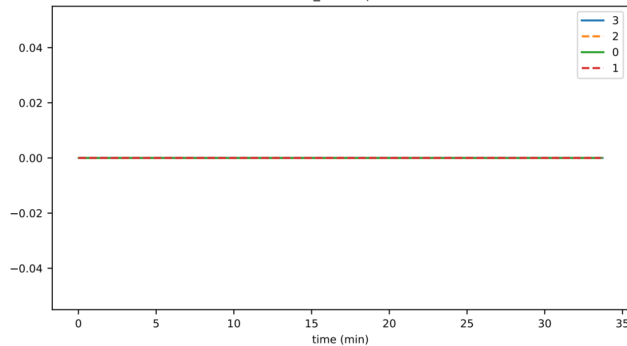
conn_onComplete
