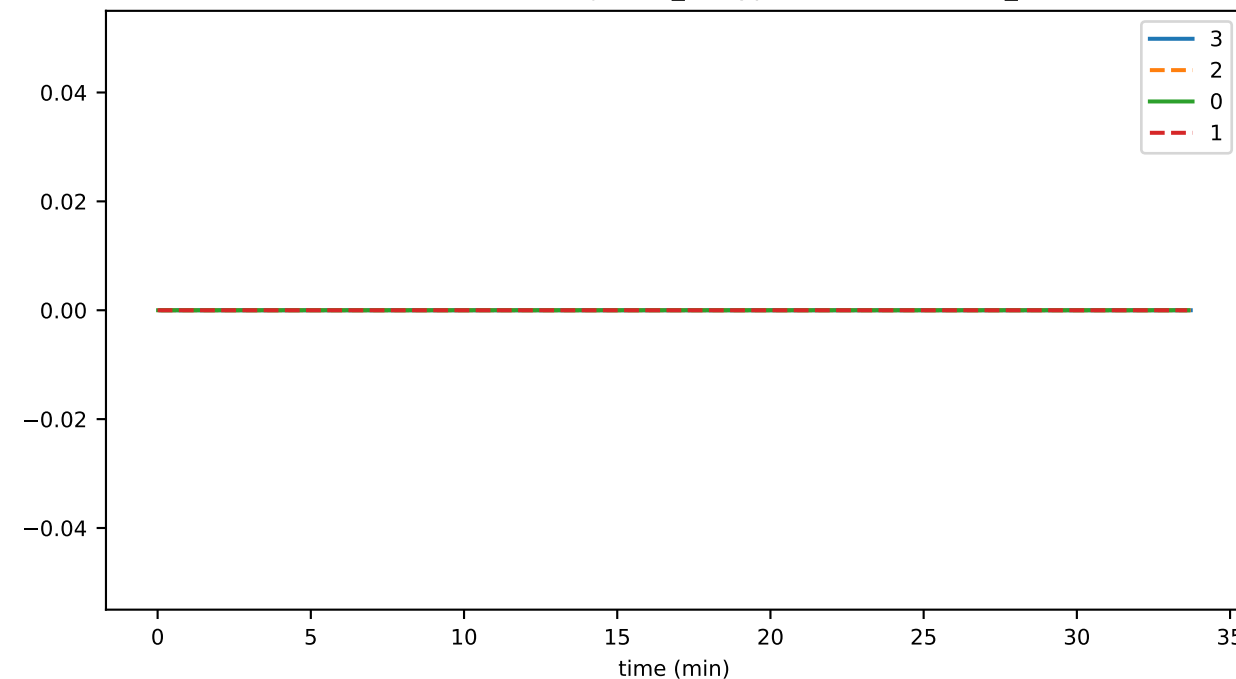
SmartContractService:SuccessfulTransactionDuration_count
