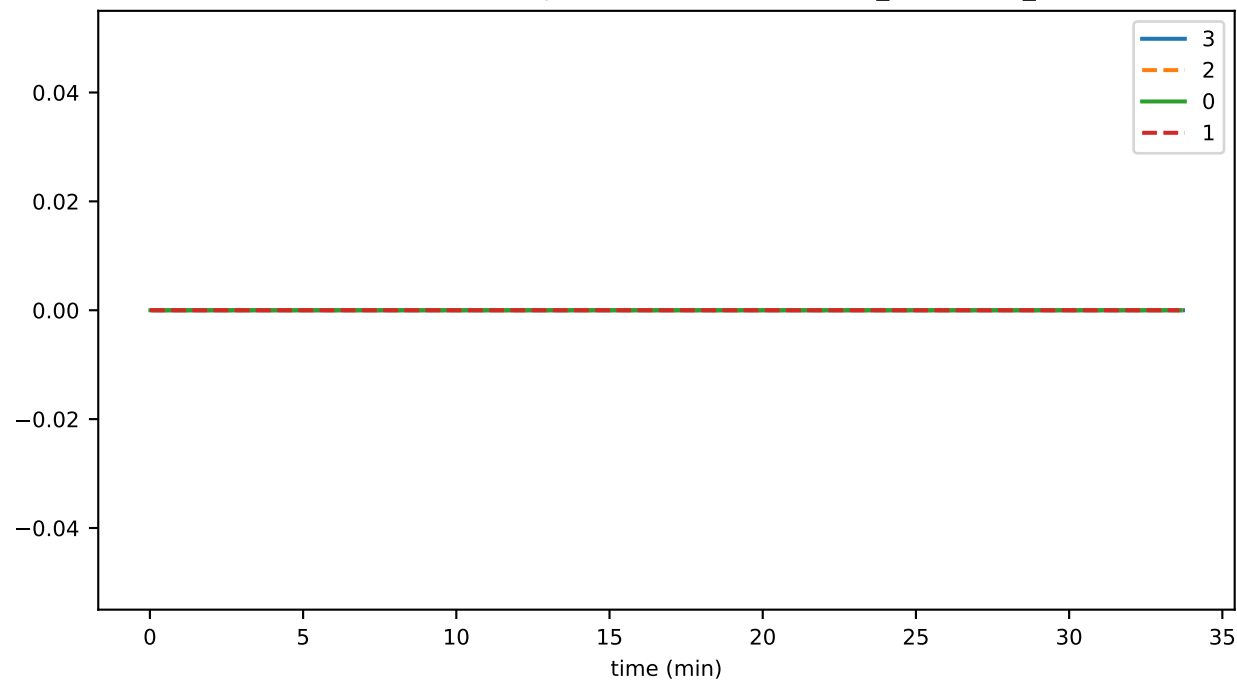
SmartContractService:SystemContractMethodCall_ASSOCIATION_total
