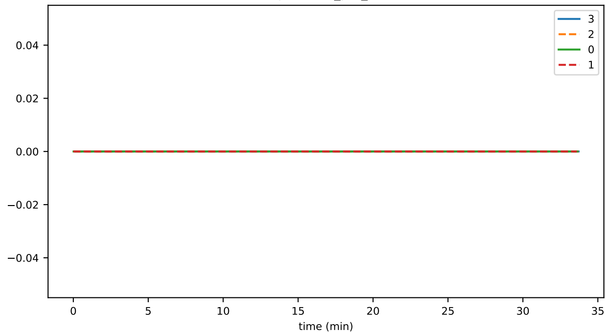
DigLockUp_per_sec
