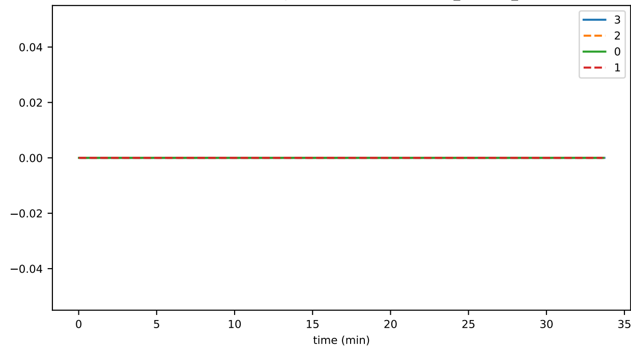
SmartContractService:SystemContractMethodCall_WIPE_failed
