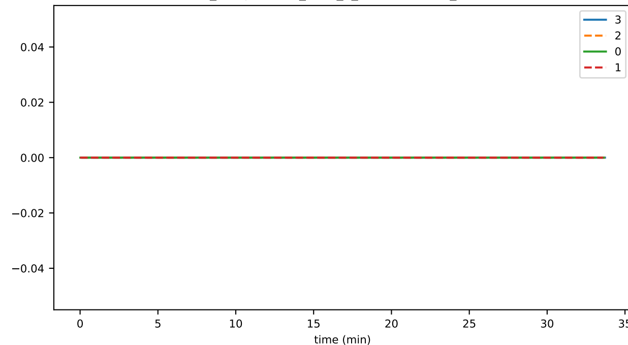
ds_compactions_level_8_hashesTimeMs_state
