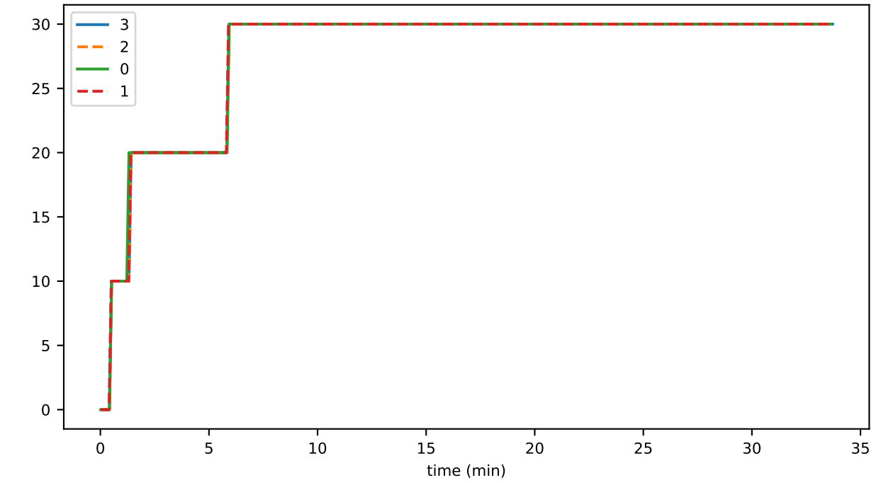
disconnects_per_sec_00
