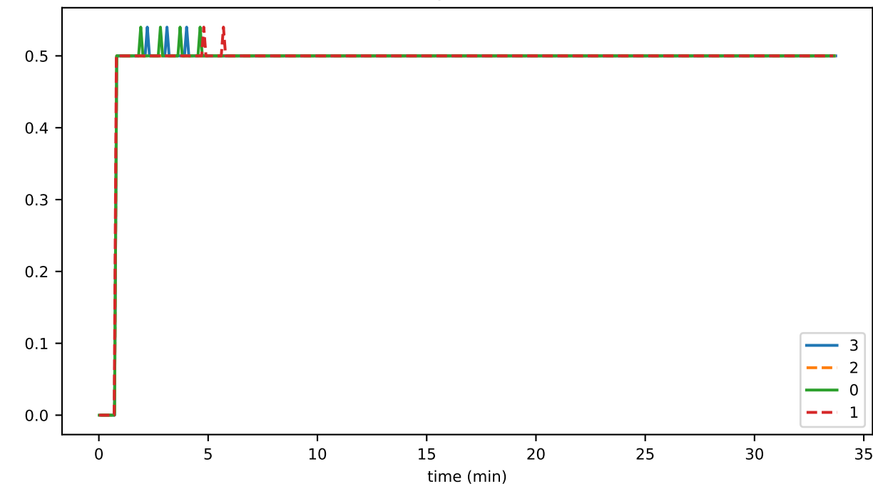
vmap_lifecycle_familySizeBackpressureMs_state
