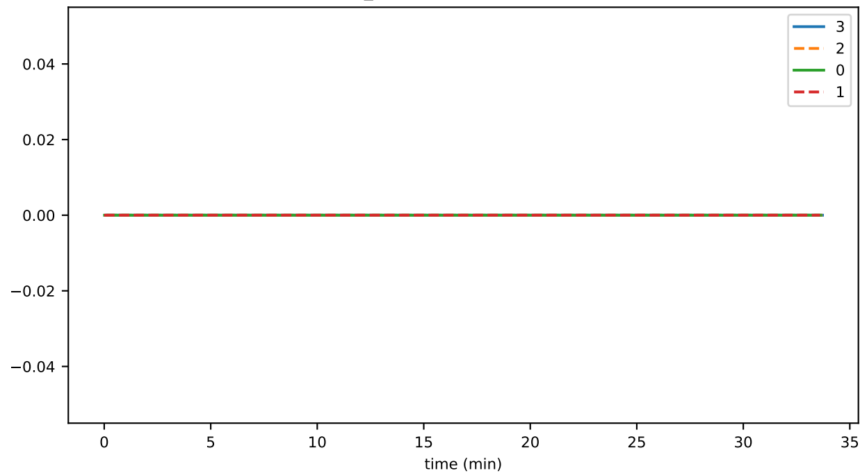
conn_pipelineOperationTimeout
