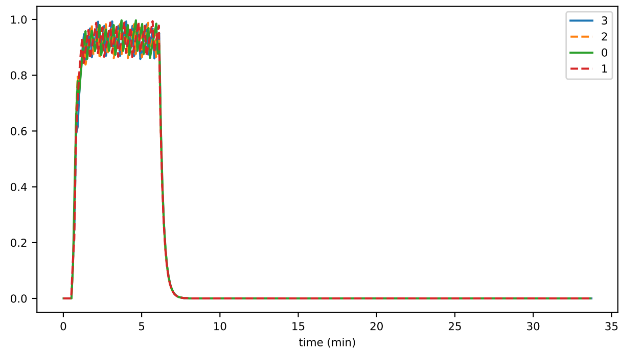
submittedPlatformTransactions
