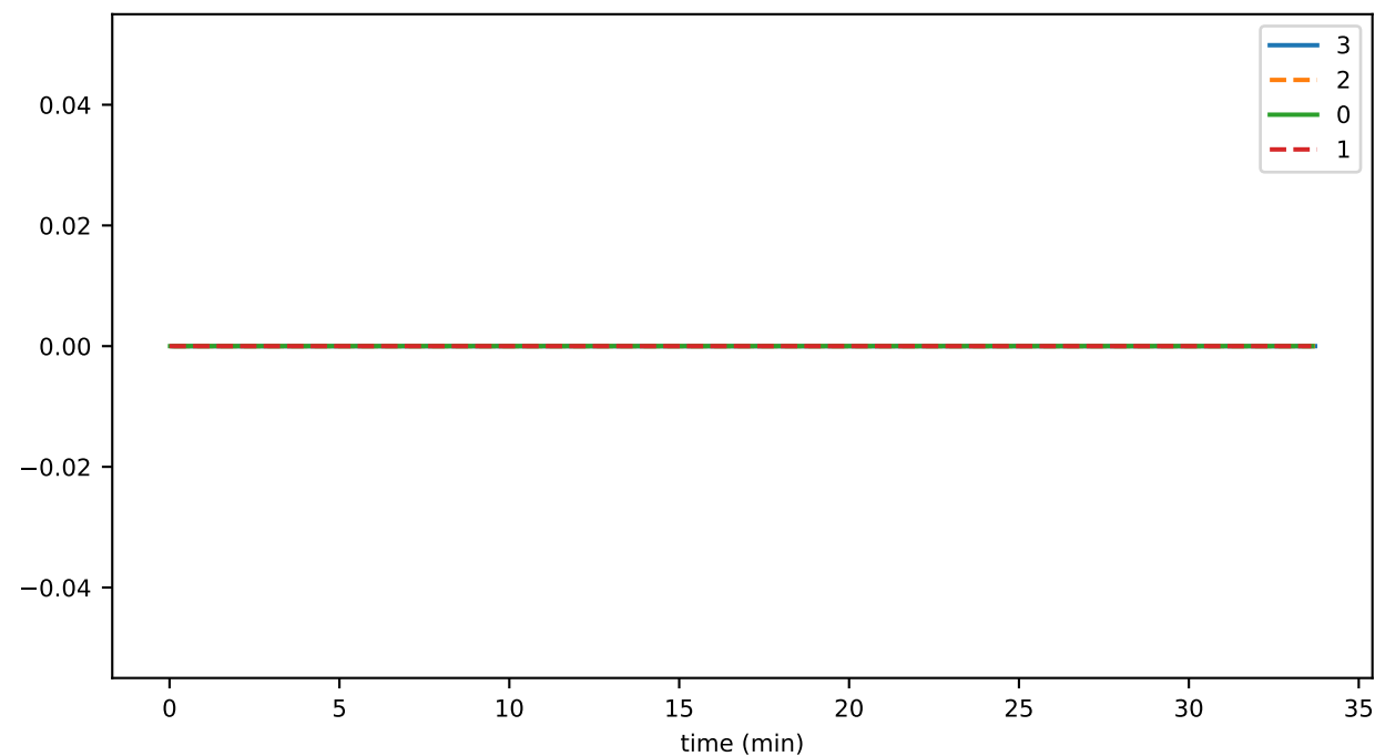
ev_per_syncRMAX
