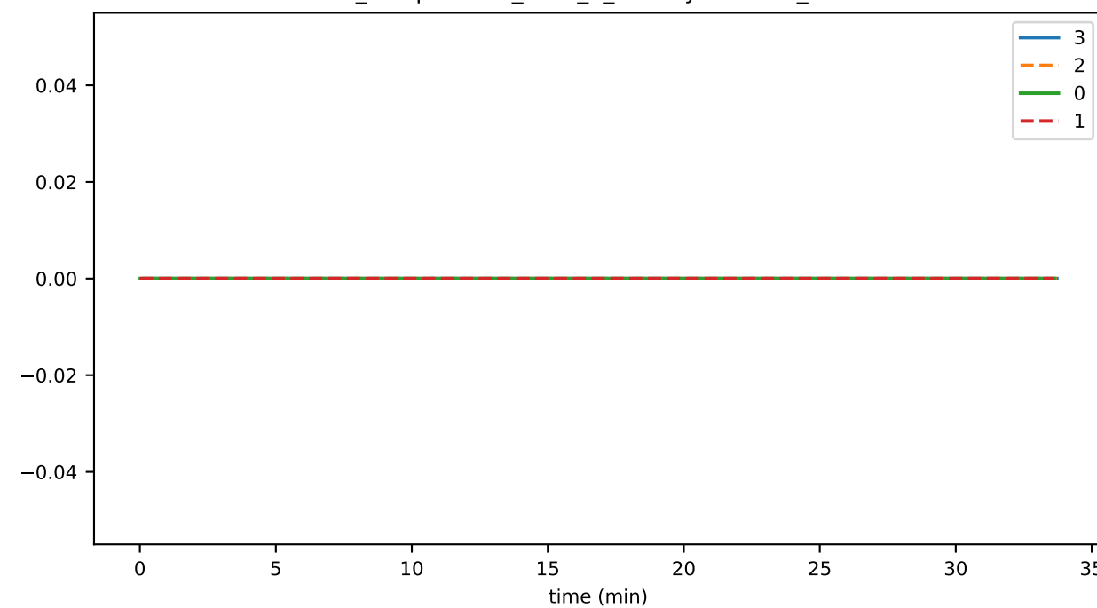
ds_compactions_level_5_leafKeysTimeMs_state
