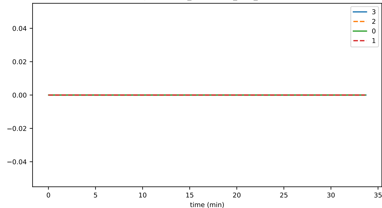
outgoingSyncRequests_per_sec
