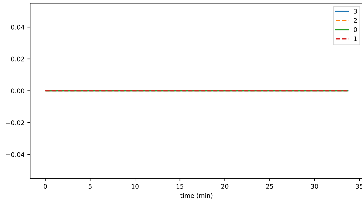
conn_connClose_newConnection
