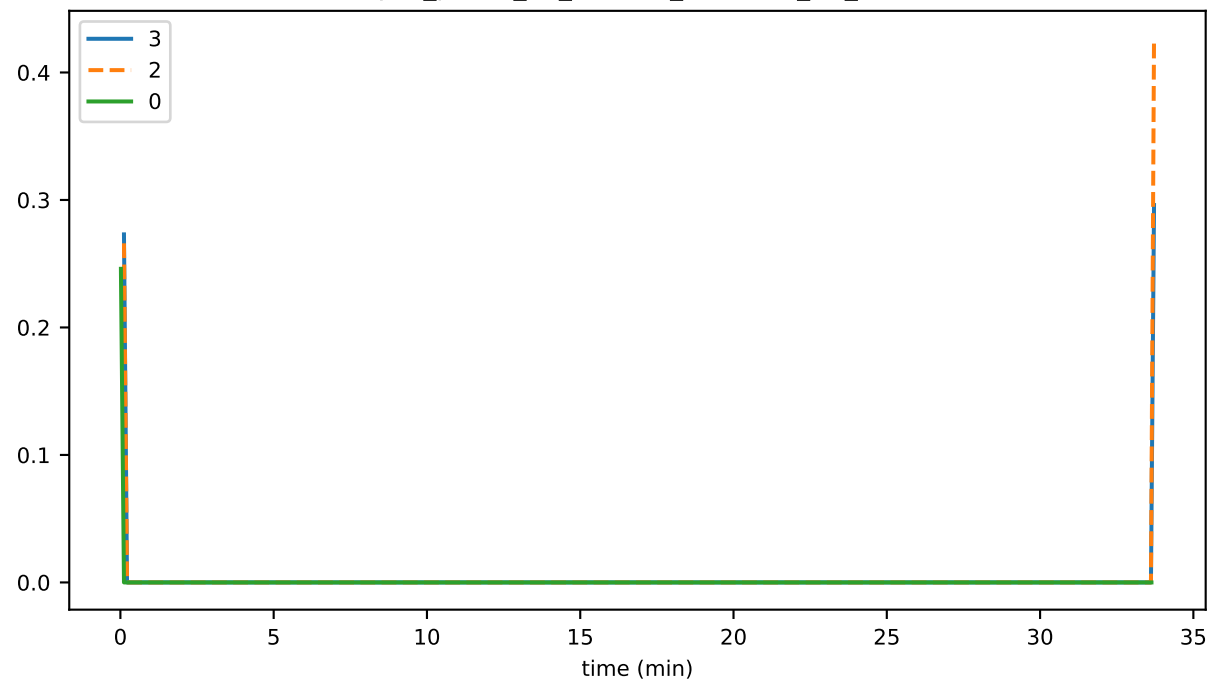
sync_phase_01_fraction_RECEIVING_EVENTS
