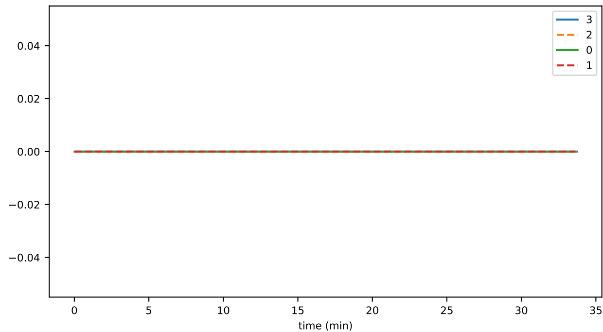
numIndirectProofs
