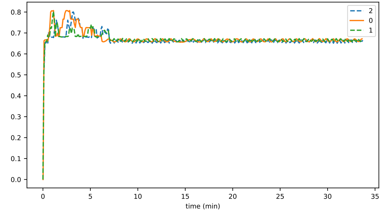
sync_phase_03_fraction_OTHER_FALLEN_BEHIND
