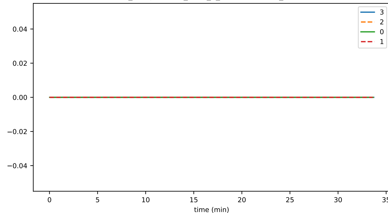
ds_compactions_level_0_leafKeysTimeMs_state
