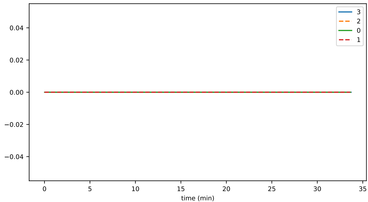
SmartContractService:LatestGasPrice
