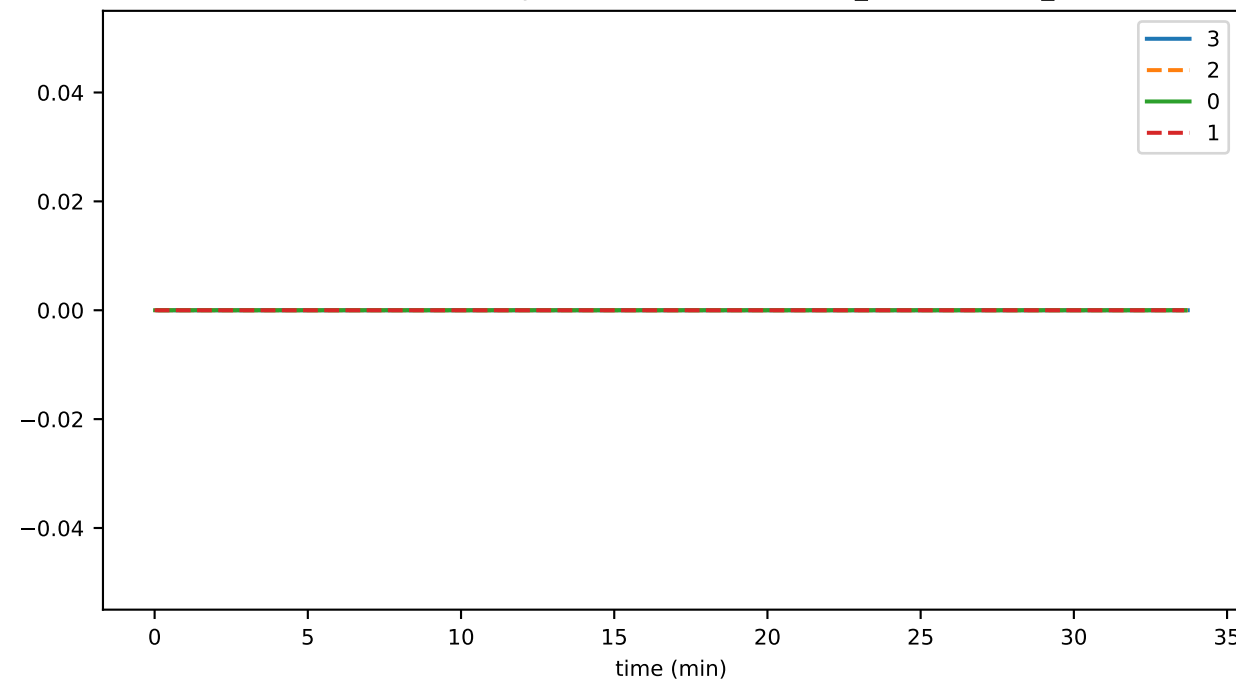
SmartContractService:SystemContractMethodCall_CREATE_DELETE_TOKEN_failed
