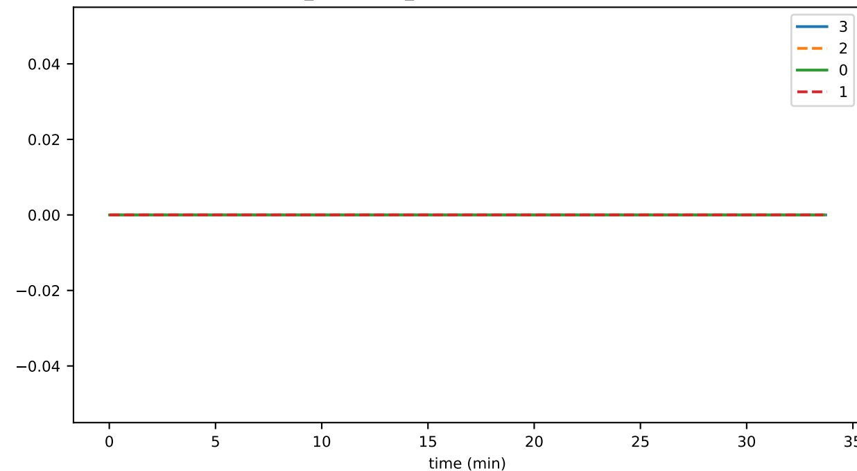
conn_connClose_transientEndStreamReceived
