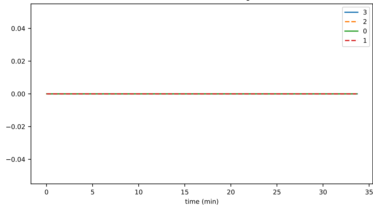
eventsWithNullFields
