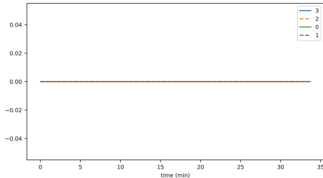
consensus_fraction_GETTING_STATE_TO_SIGN
