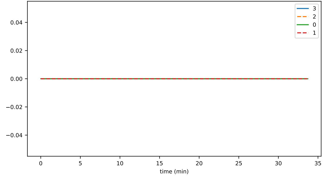
averageTimeToFullySignState
