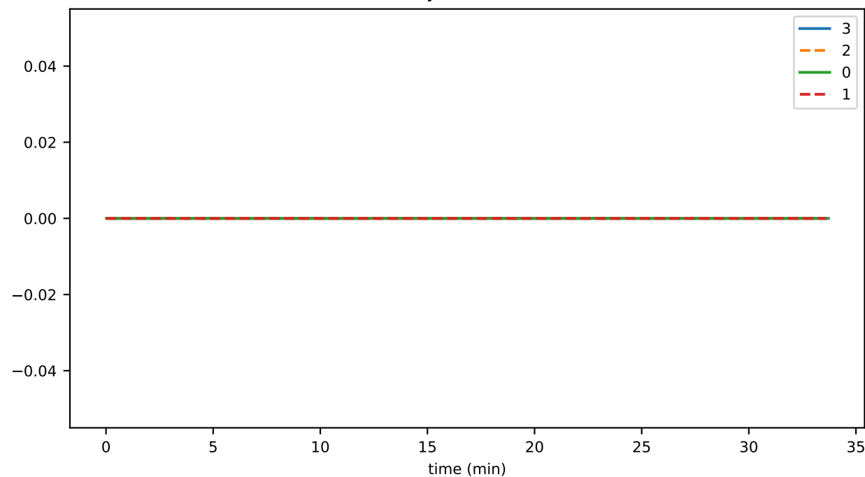
doNotSyncIntakeCounter
