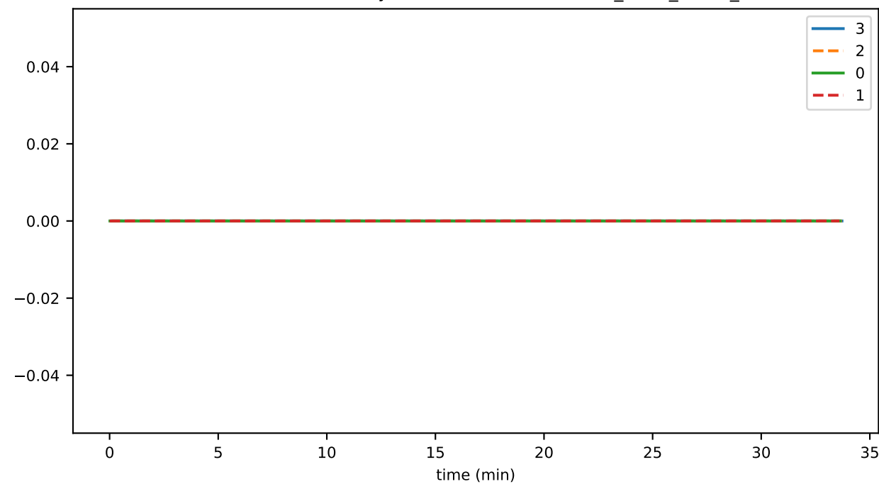
SmartContractService:SystemContractMethodCall_MINT_BURN_failed
