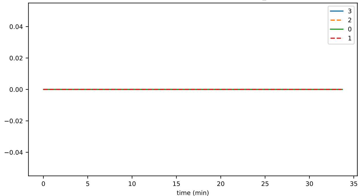
SmartContractService:TransactionGasUsed_sum
