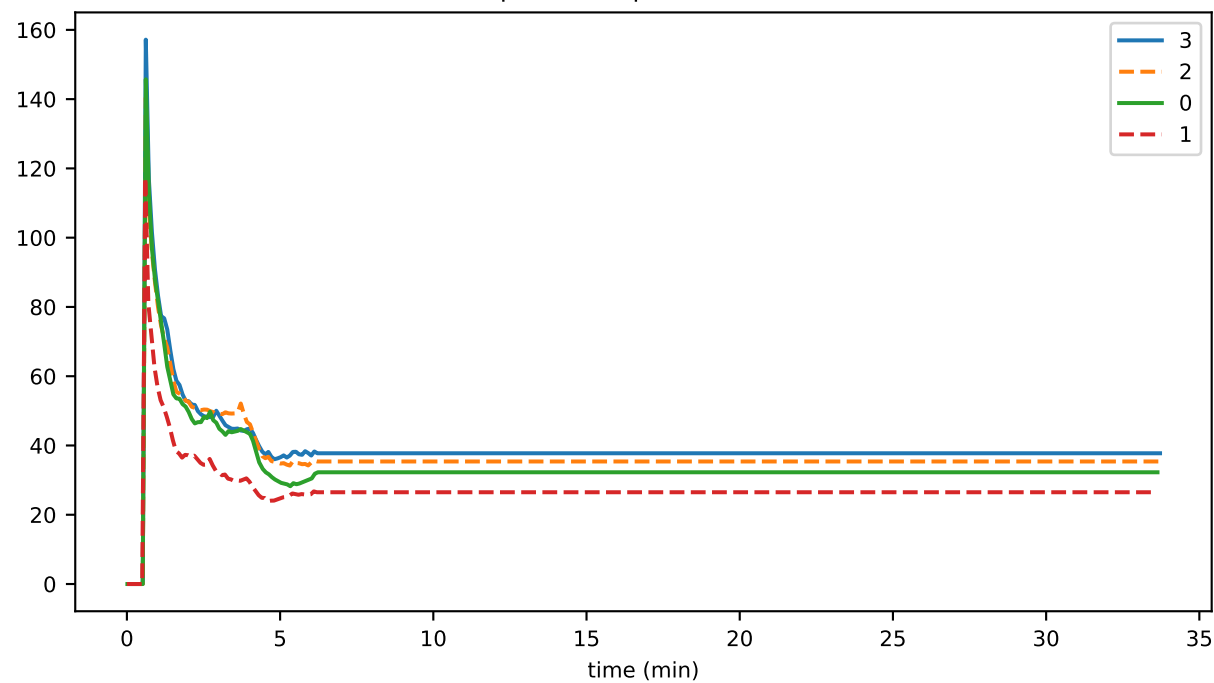
uptimeComputationTime
