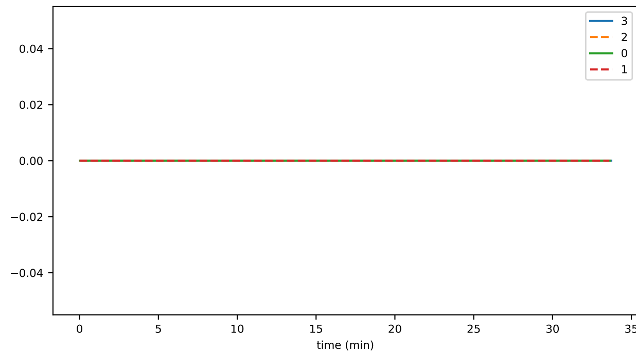
startsReconnectAsSender
