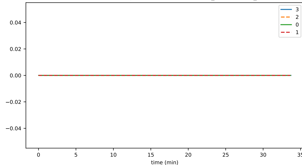
SmartContractService:SystemContractMethodCall_APPROVAL_failed
