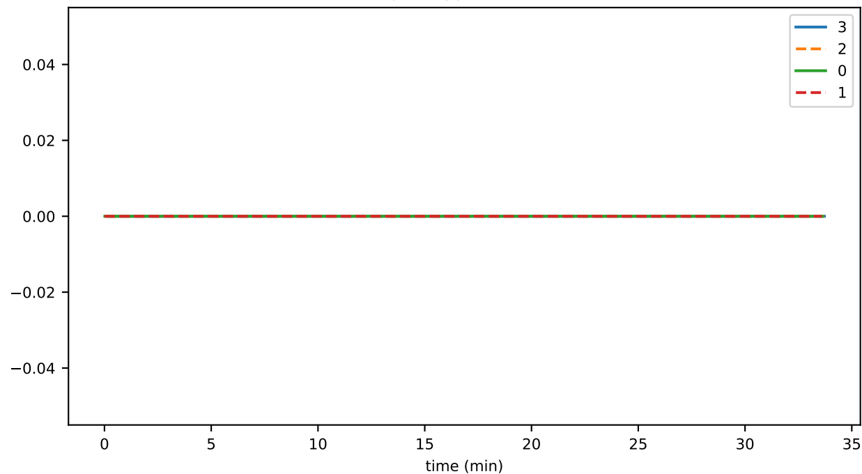
accountsMaxNumber
