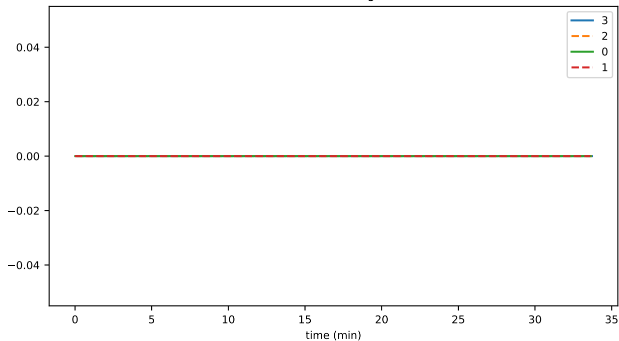
branchingEvents
