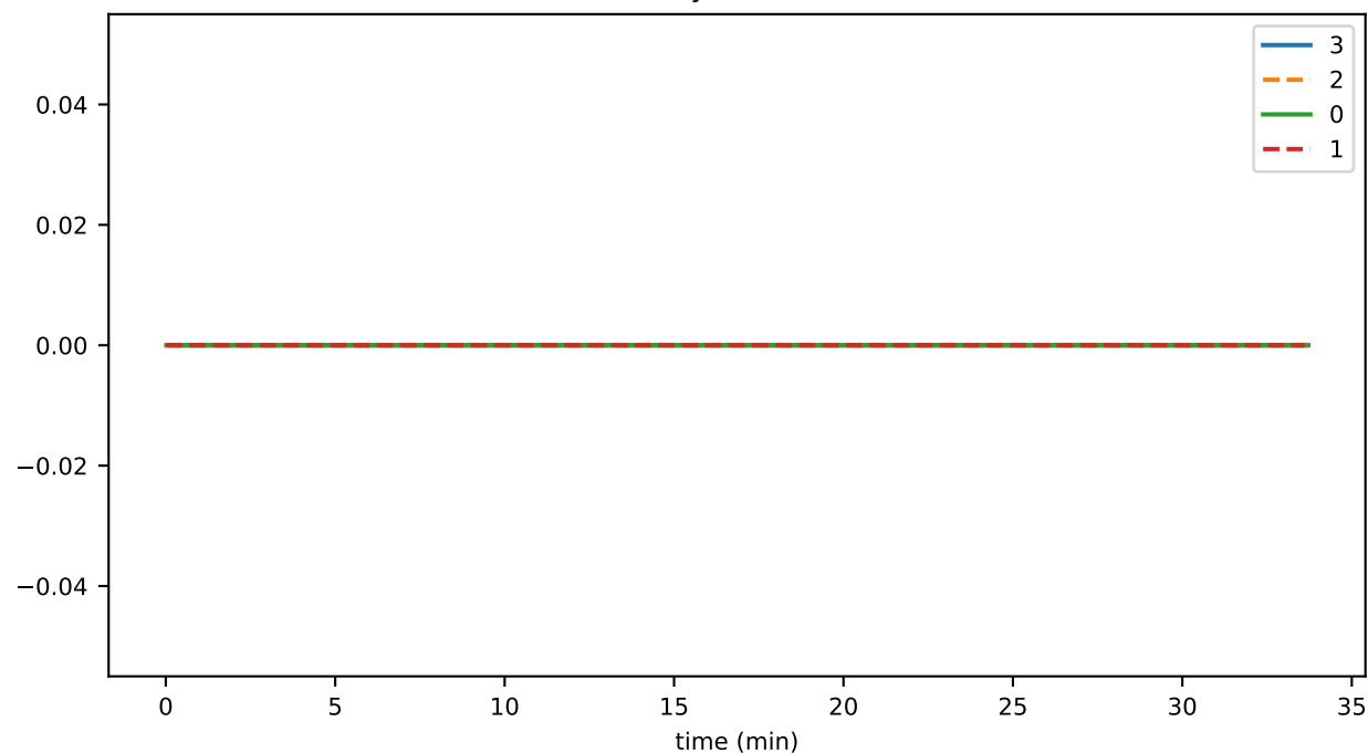
doNotSyncRemoteFallenBehind
