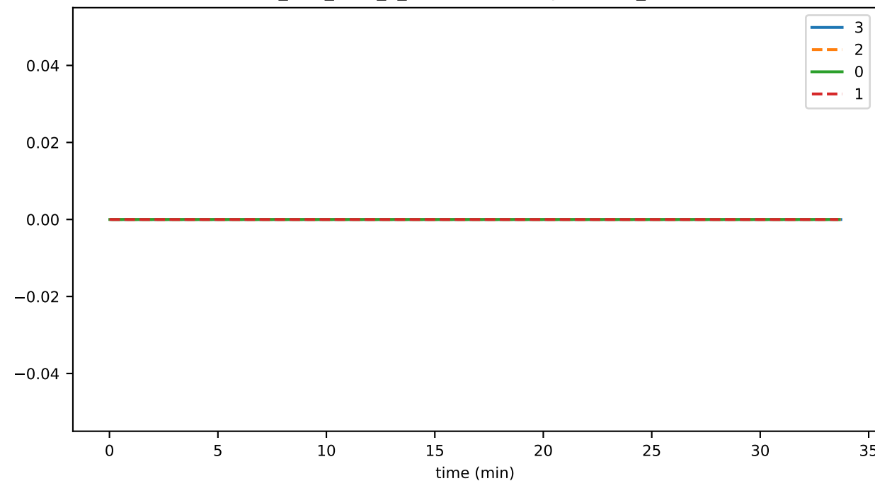
ds_files_level_6_leavesFileSizeByLevelMb_state
