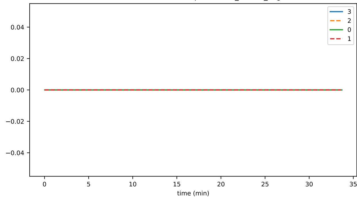
SmartContractService:OpsDuration_PerTxn_avg
