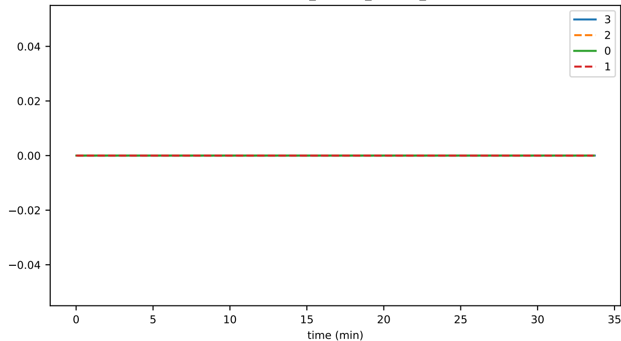
EventDeduplicator_busy_fraction
