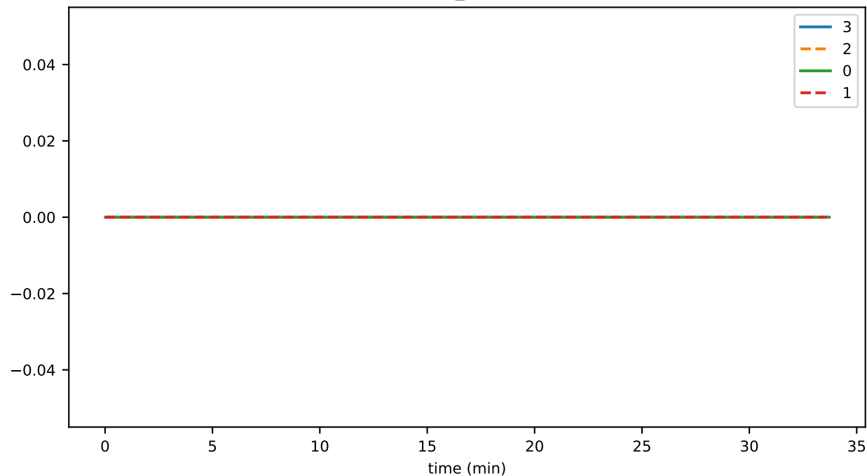
conn_closed
