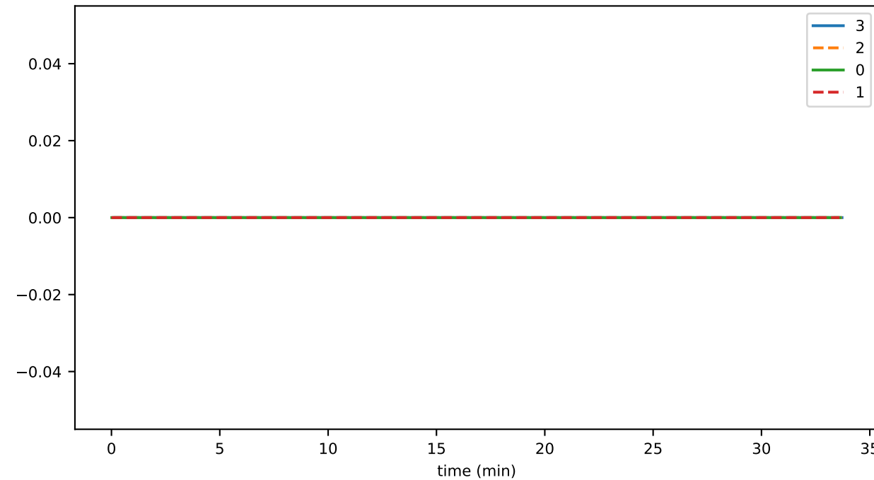
ds_compactions_level_4_hashesTimeMs_state
