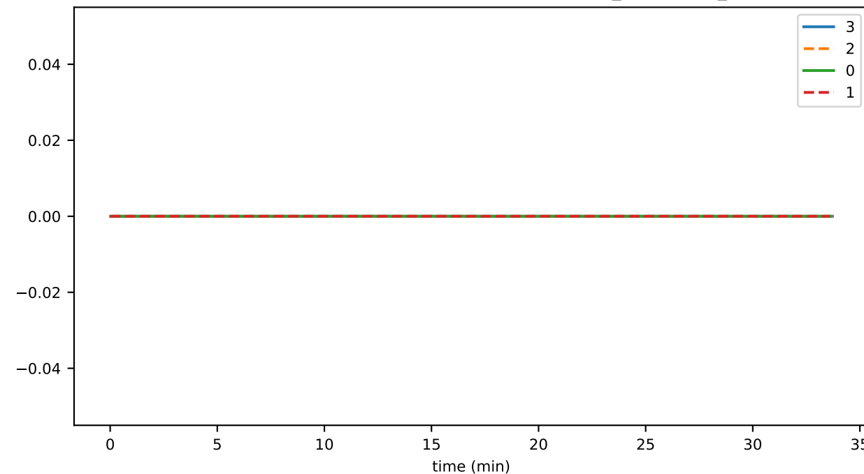
SmartContractService:SystemContractMethodCall_SCHEDULE_failed
