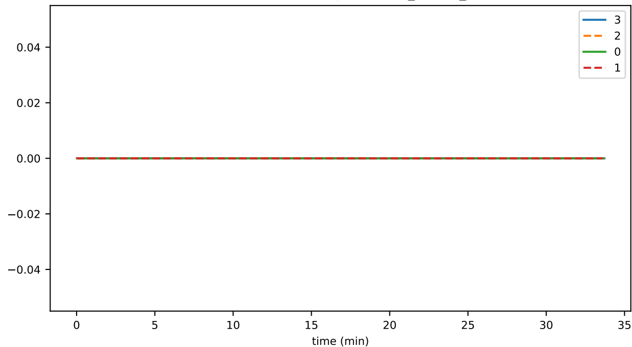
SmartContractService:OpsDuration_TxnsThrottled
