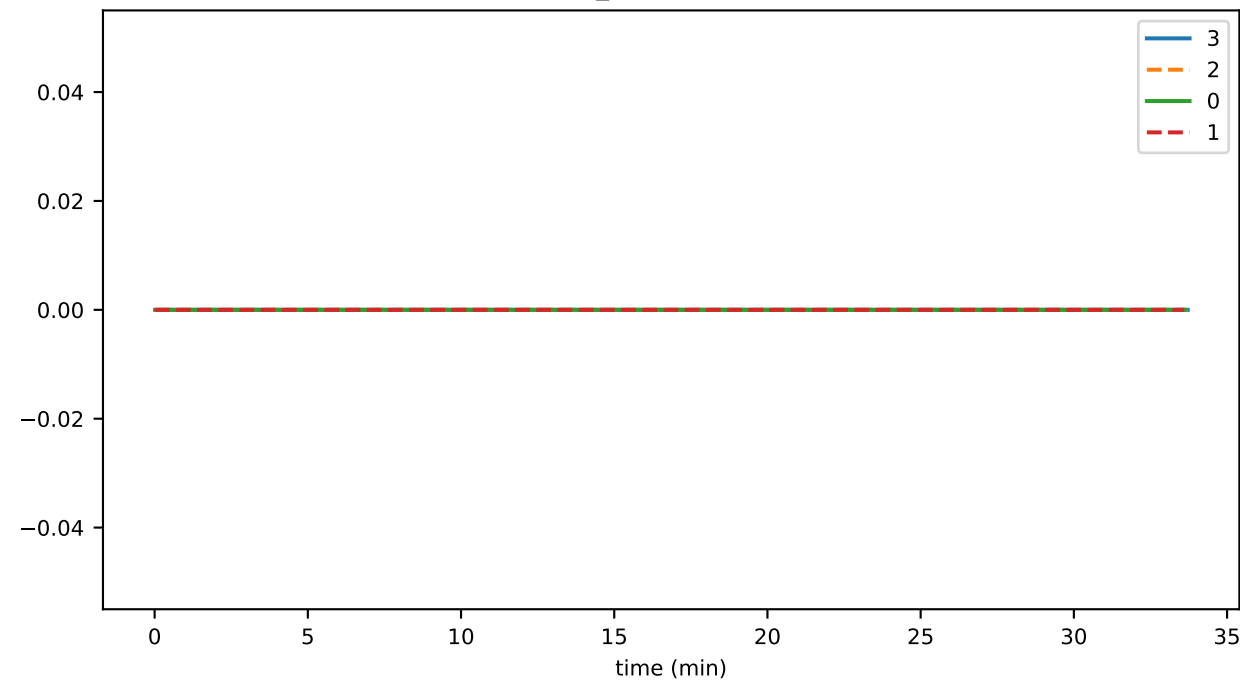
connSend_requestSendLatency
