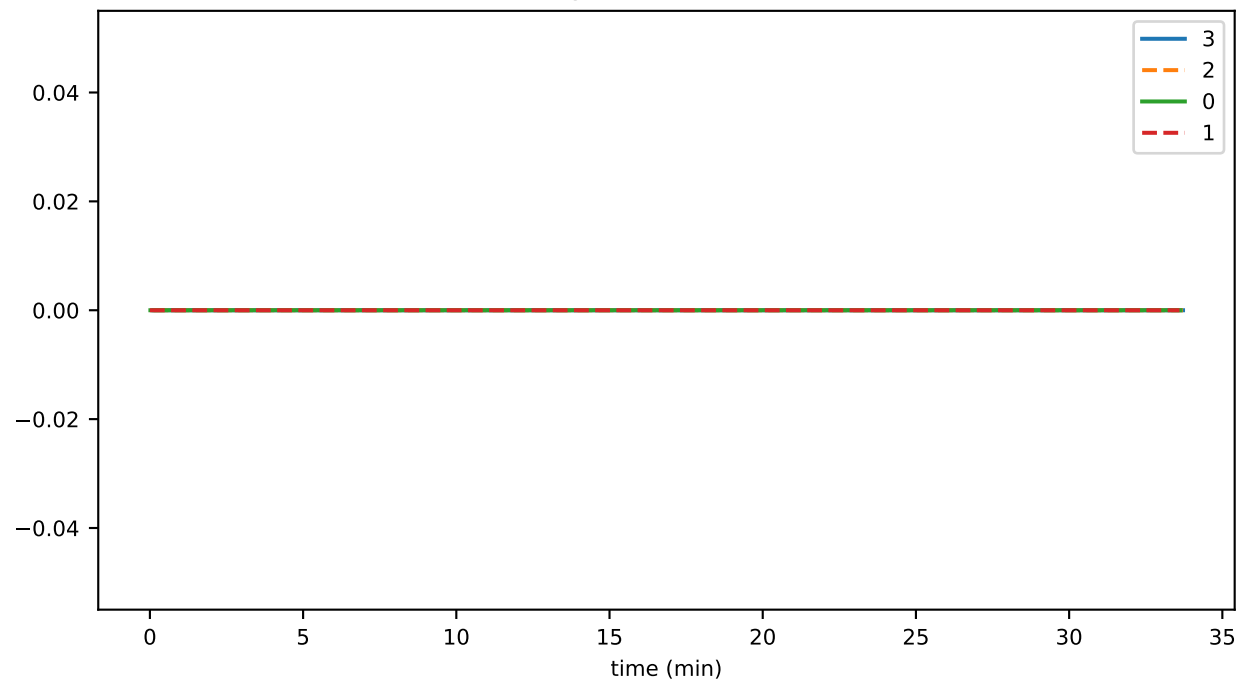
SigWrkTime
