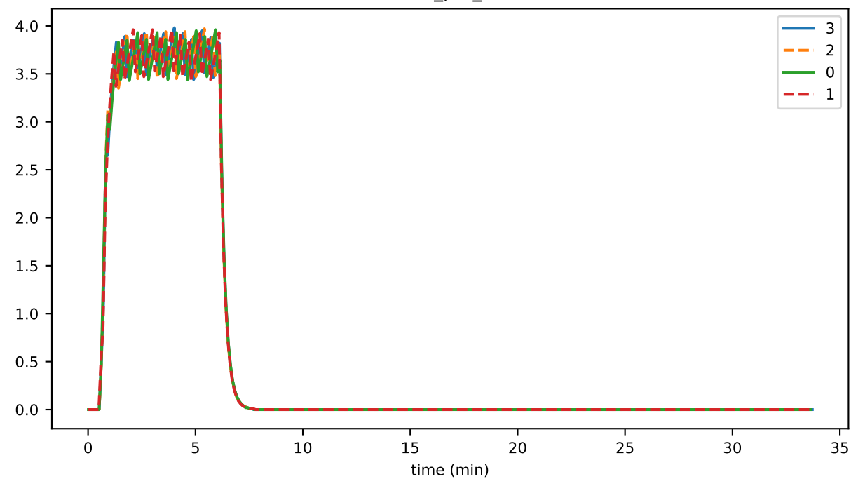
trans_per_sec
