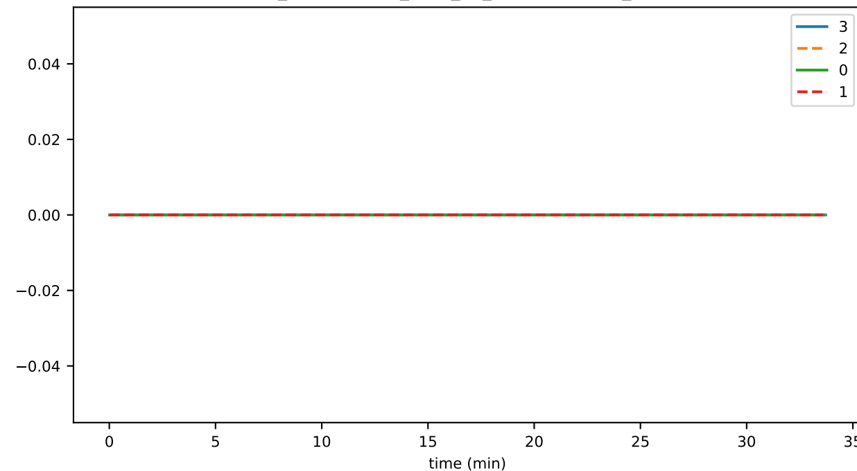
ds_compactions_level_10_hashesTimeMs_state
