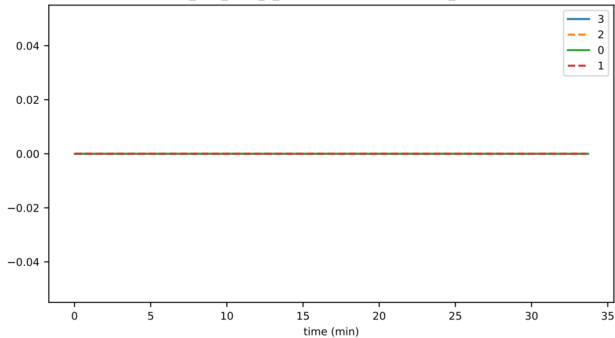
ds_files_level_6_leafKeysFileSizeByLevelMb_state
