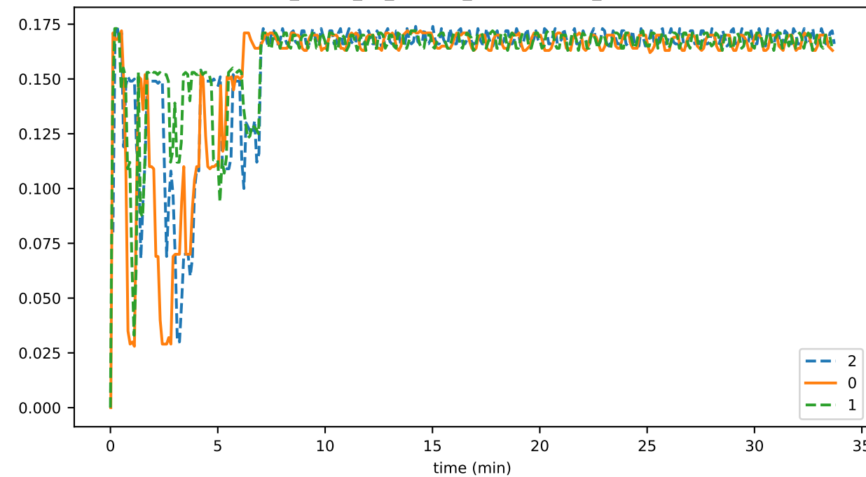
sync_phase_03_fraction_EXCHANGING_WINDOWS
