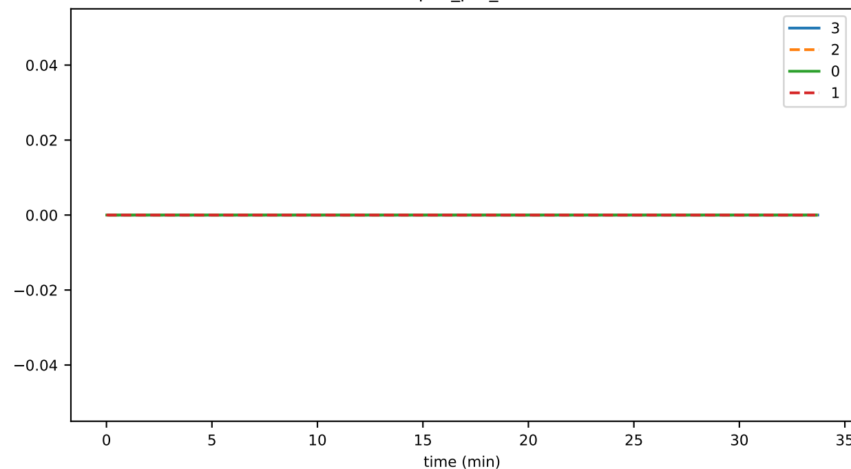
endsReconnectAsReceiver
