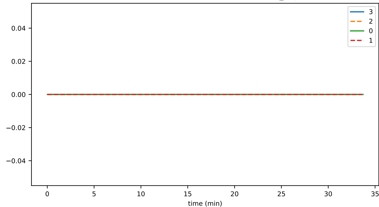
SmartContractService:TransactionDuration_sum
