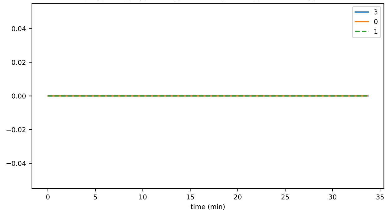
sync_phase_02_fraction_SELF_FALLEN_BEHIND
