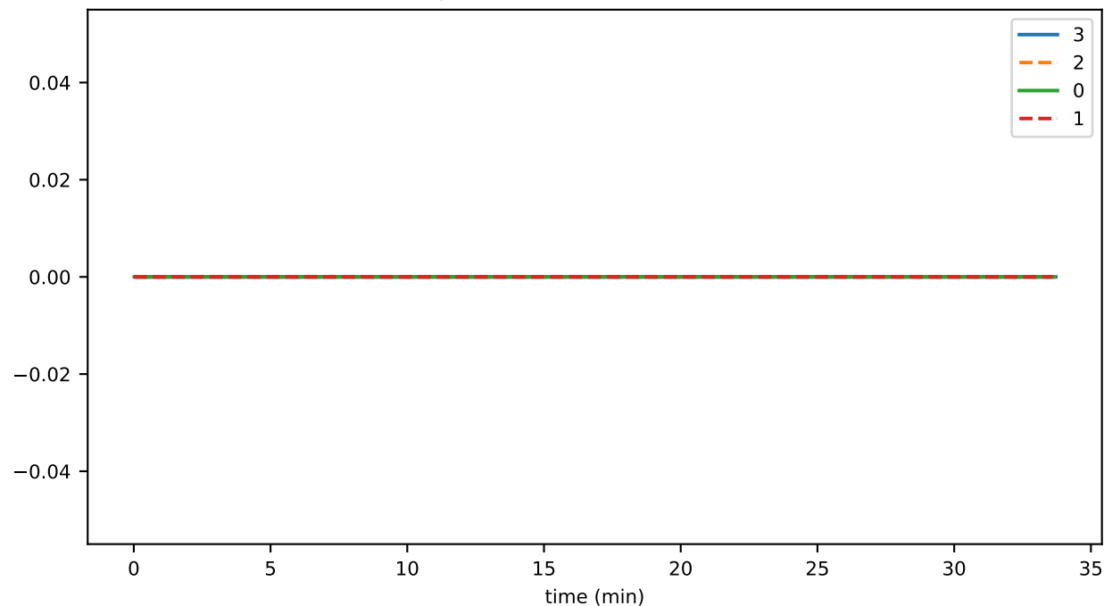
pcesAvgSyncDuration
