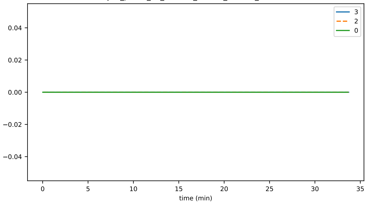
sync_phase_01_fraction_OTHER_FALLEN_BEHIND
