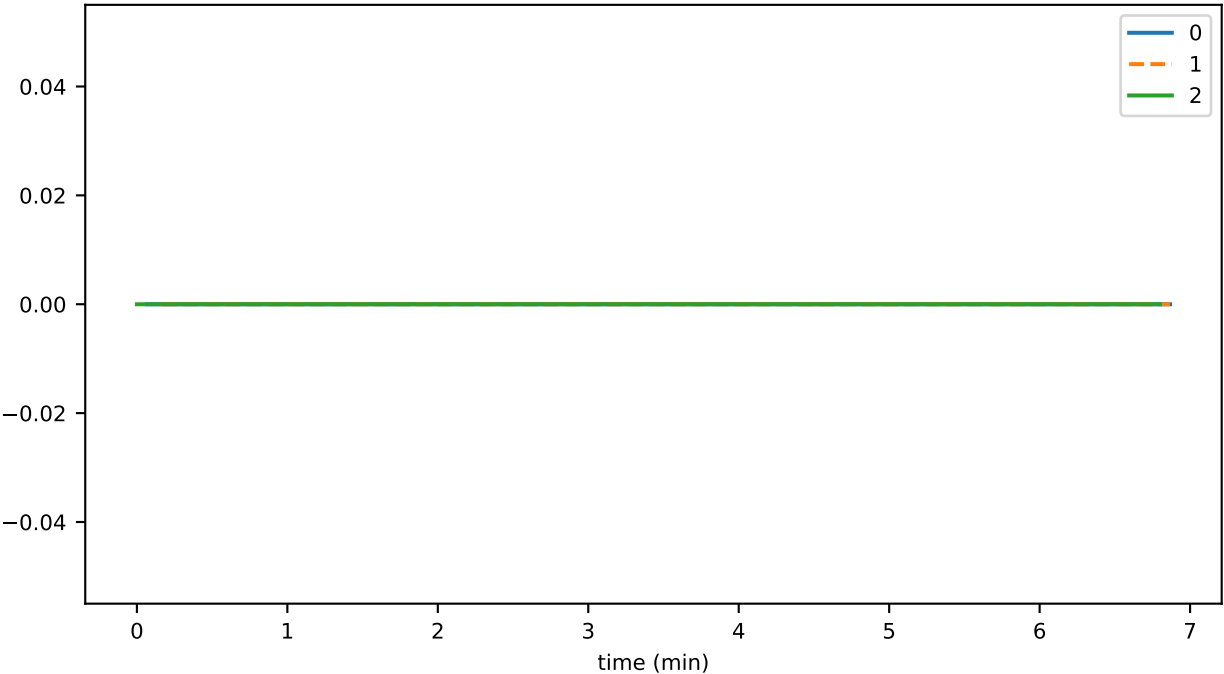
SmartContractService:SuccessfulTransactionDuration_avg
