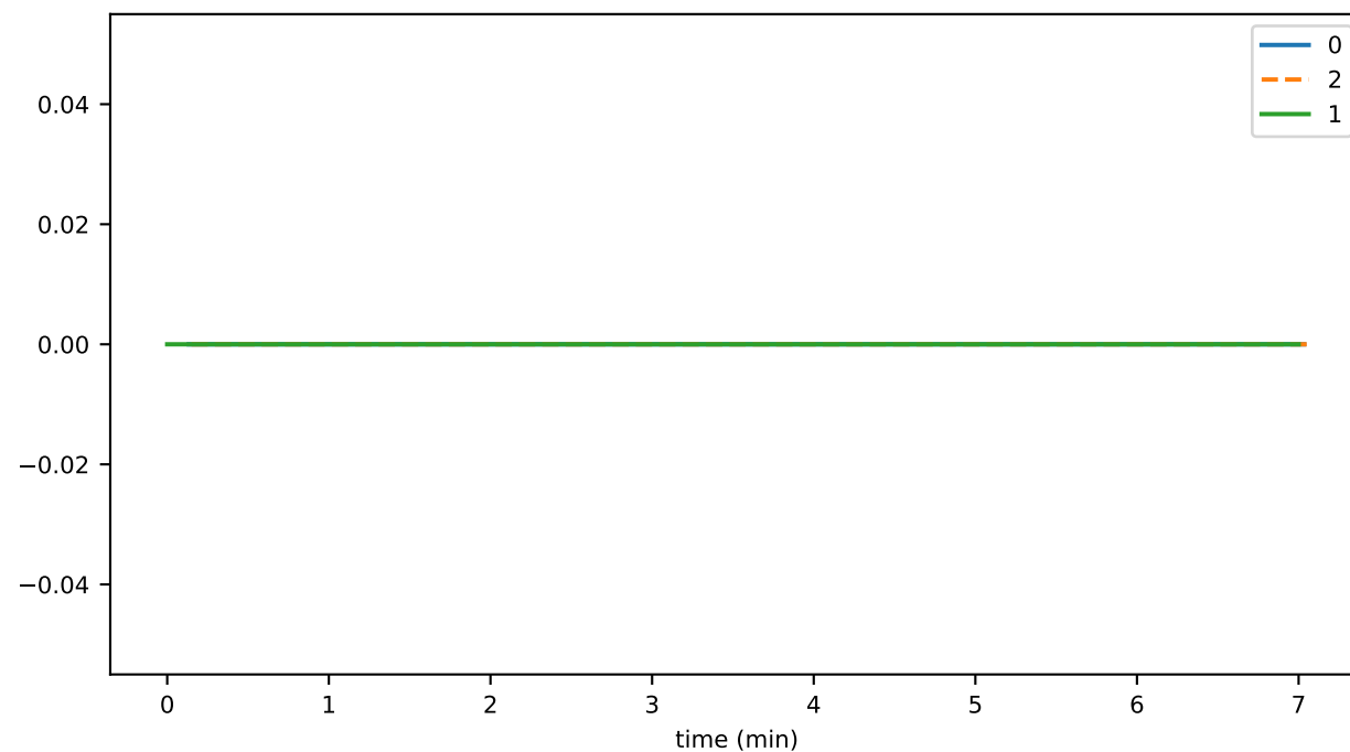
reconnectRejections_per_sec_01
