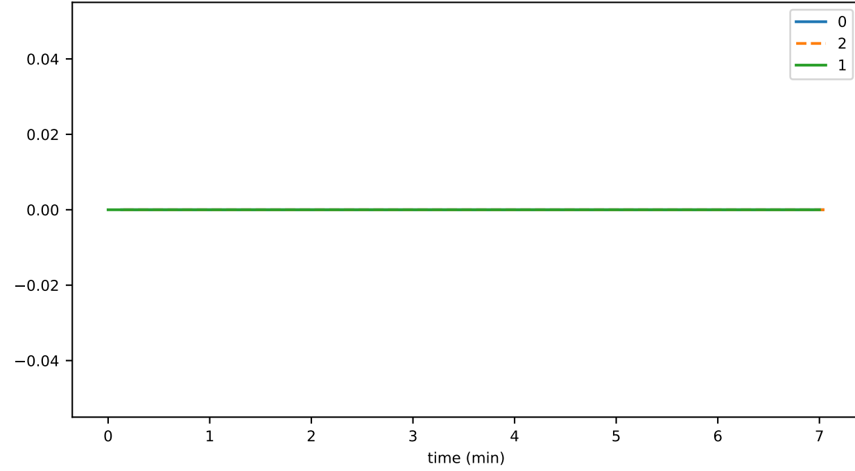
utilPrngThrottledTxns
