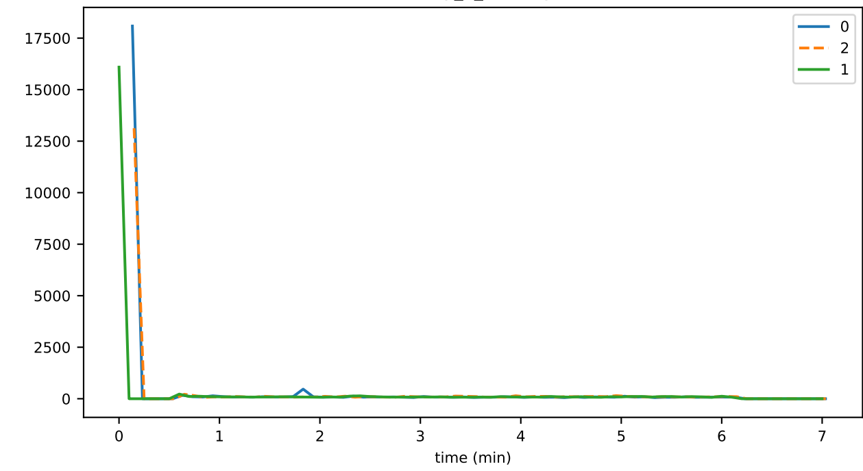
eventDelay_2_validationMAX
