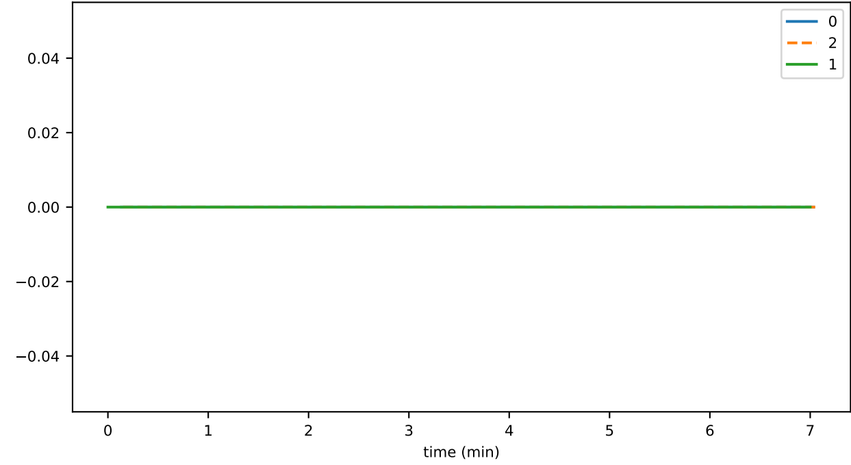
hintsPartialSignatureDurationMax
