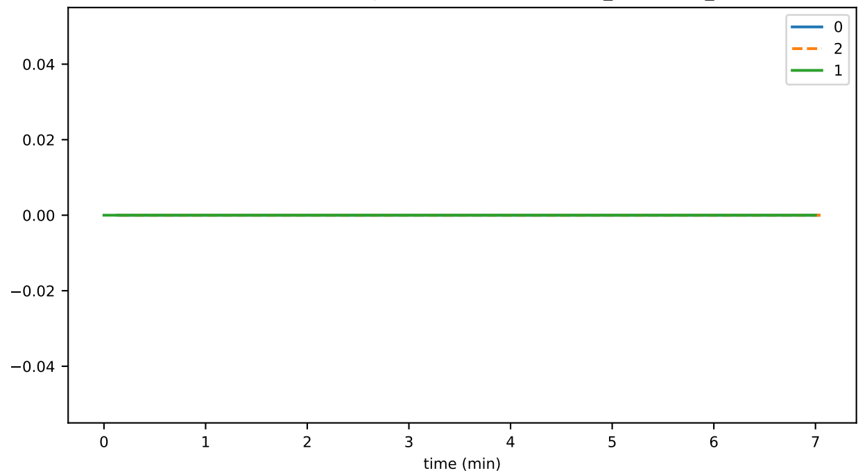
SmartContractService:SystemContractMethodCall_ASSOCIATION_failed
