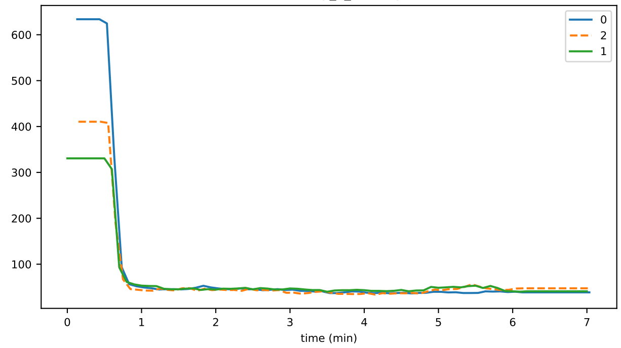
eventDelay_2_validation
