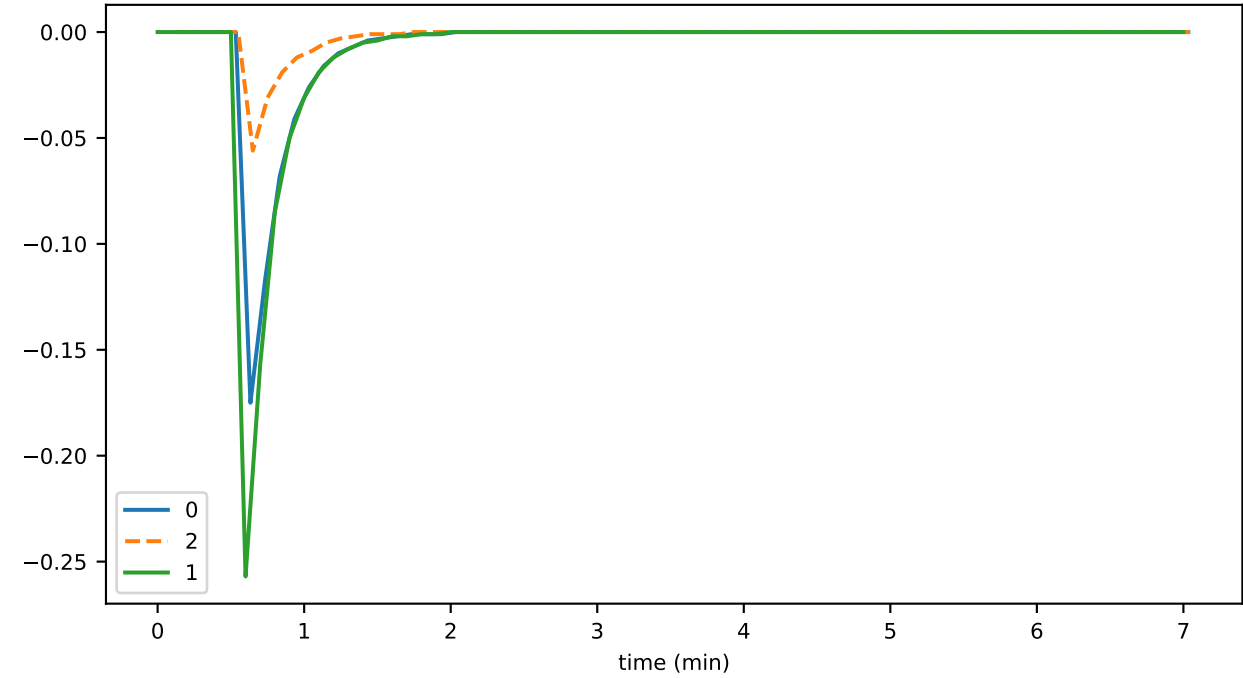
stateSignaturesGathered_per_sec
