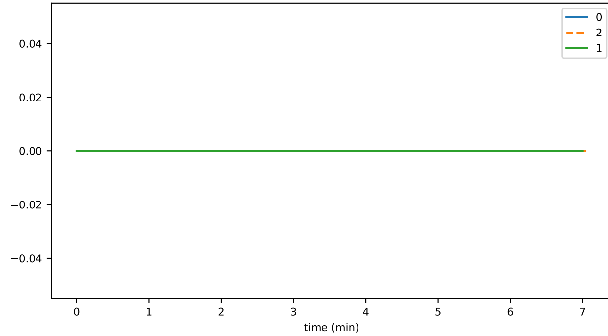
utilPrngThrottledTxns
