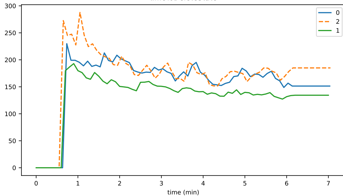
timeToDeleteState
