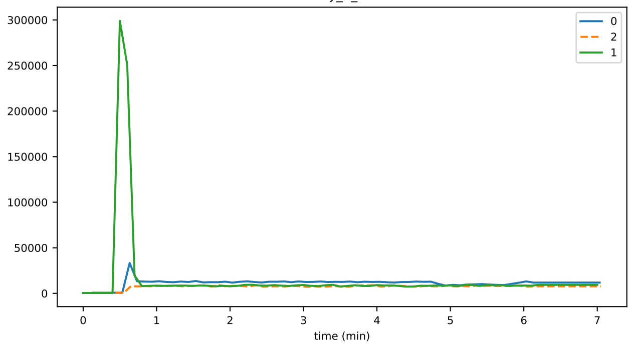
eventDelay_2_validation
