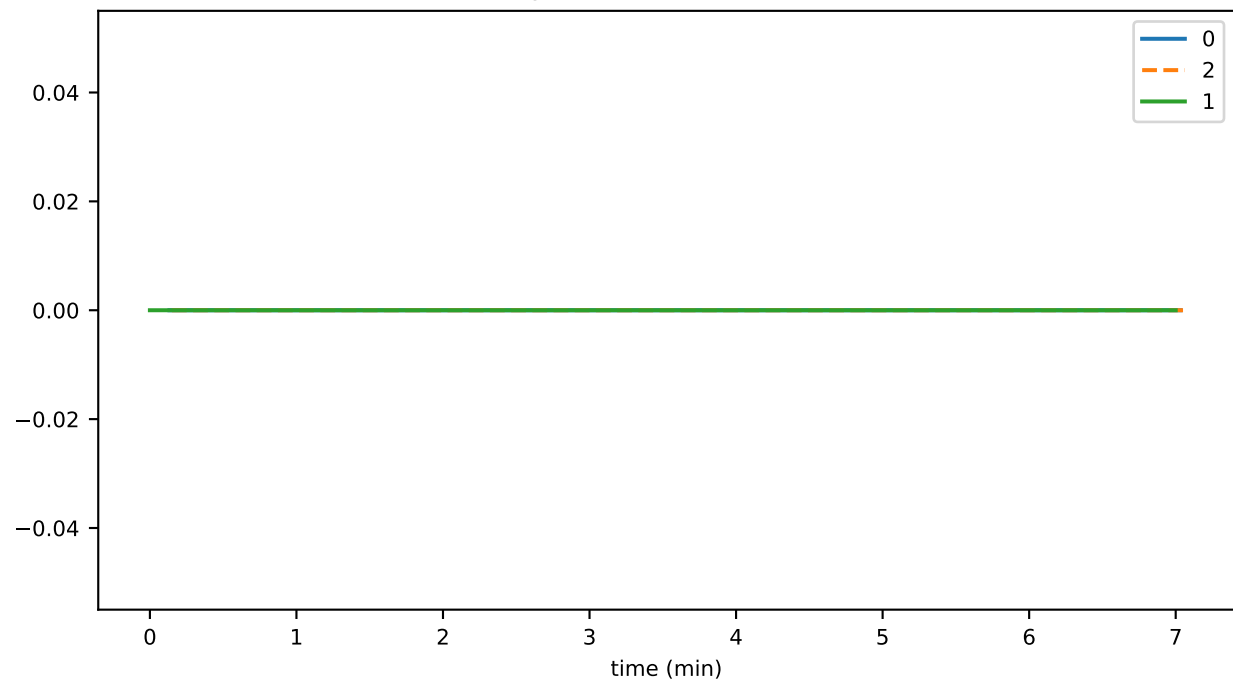
historyProofTransWasmToR1Cnt
