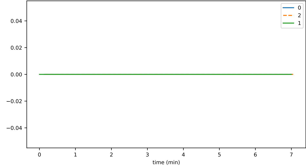
ethereumTransactionThrottledTxns
