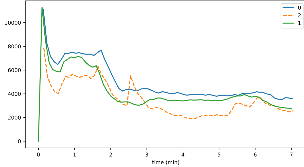
syncFilterTime
