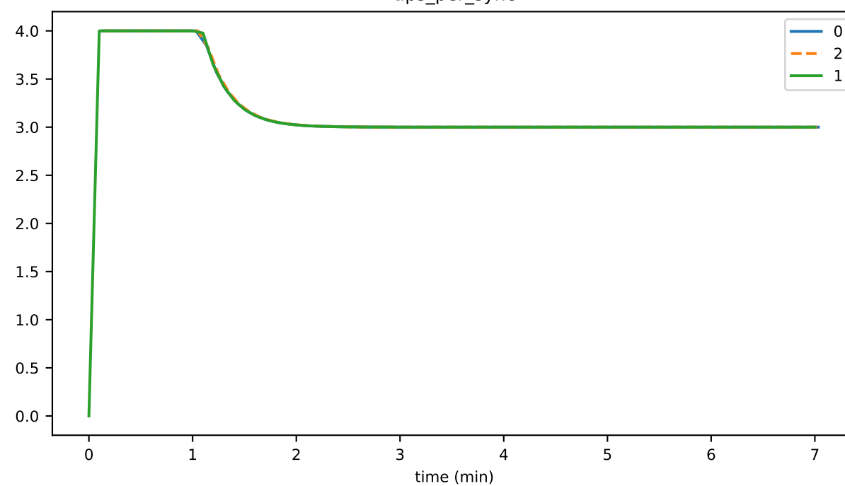
tips_per_sync
