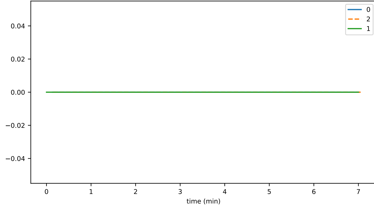
hintsPartialSignatureDurationAvg
