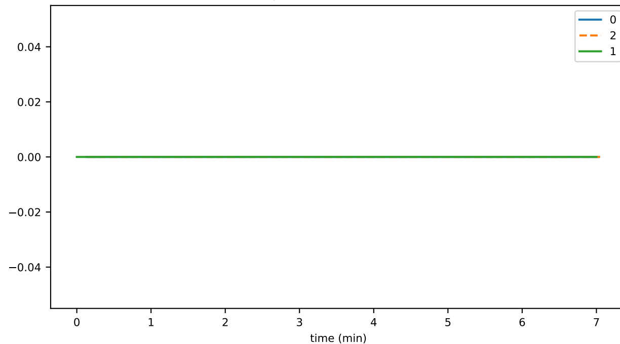
historyProofTransWasmToR1Ms
