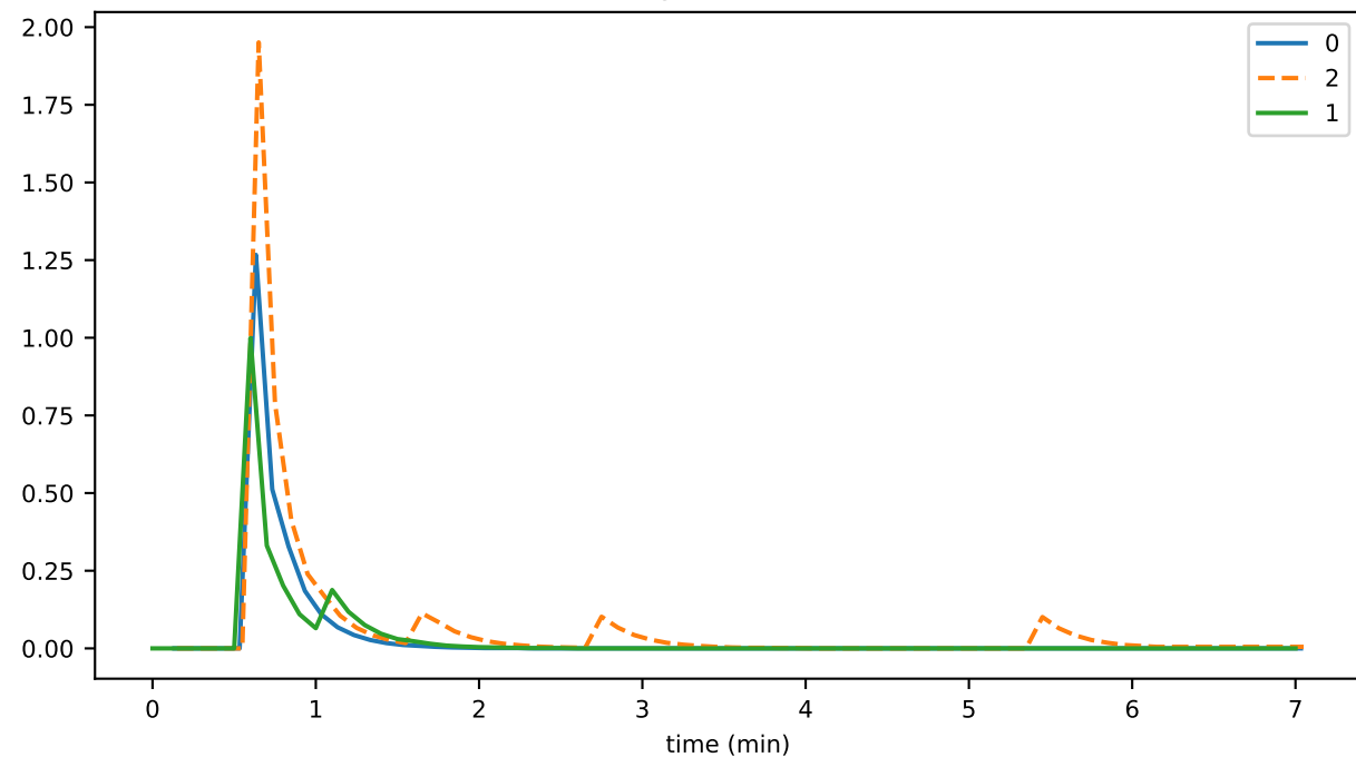
SigVal_per_sec
