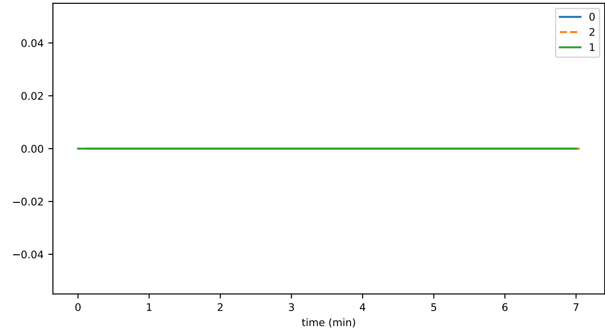
ethereumTransactionThrottledTxns
