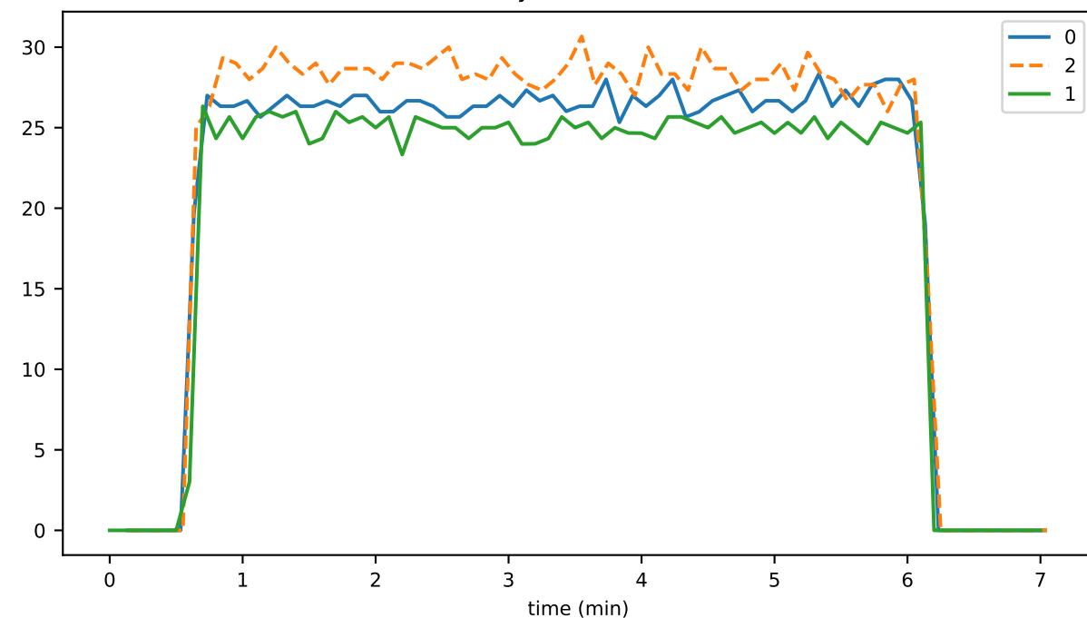
doNotSyncPlatformStatus
