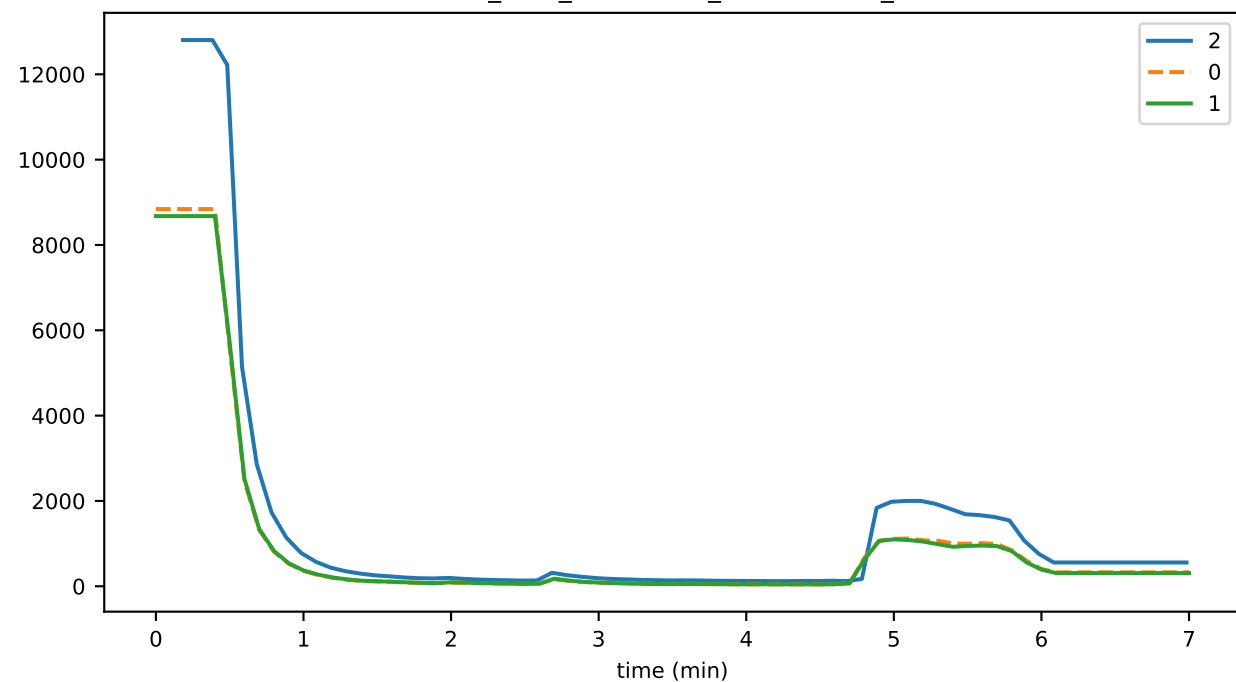
consensus_time_SETTING_EVENT_CONSENSUS_DATA
