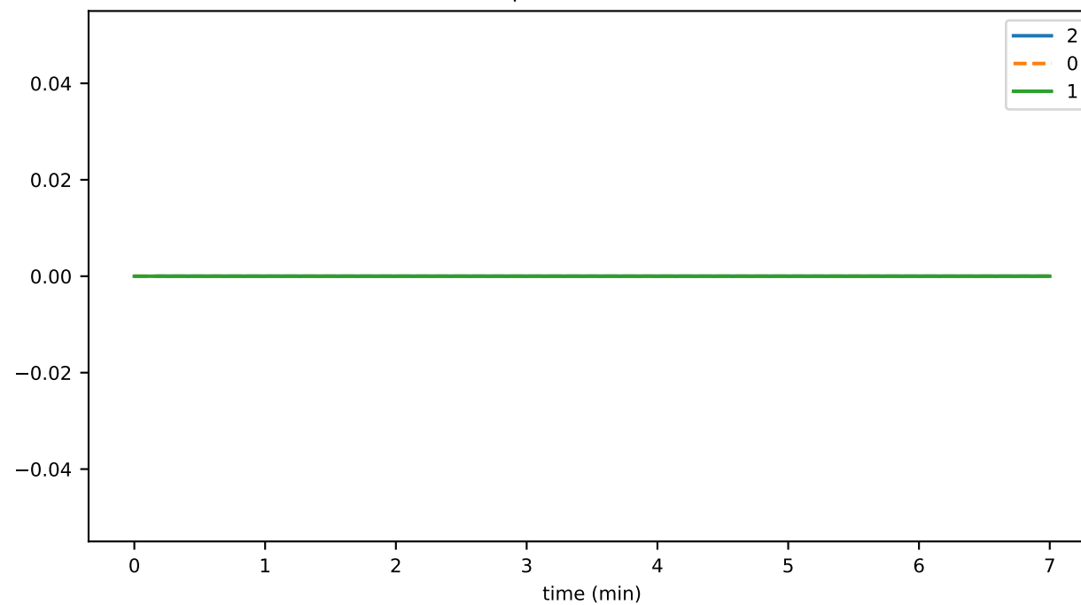
fileUpdateDurationMax
