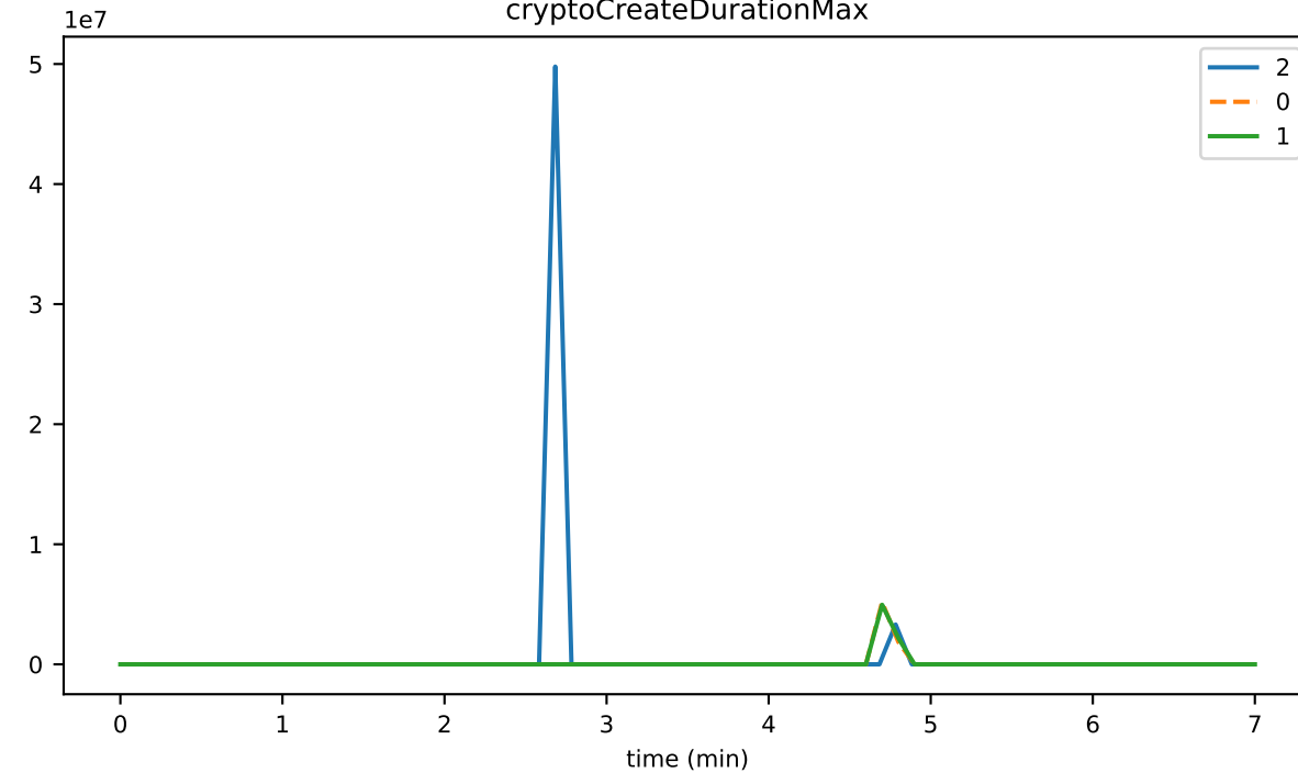
cryptoCreateDurationMax
