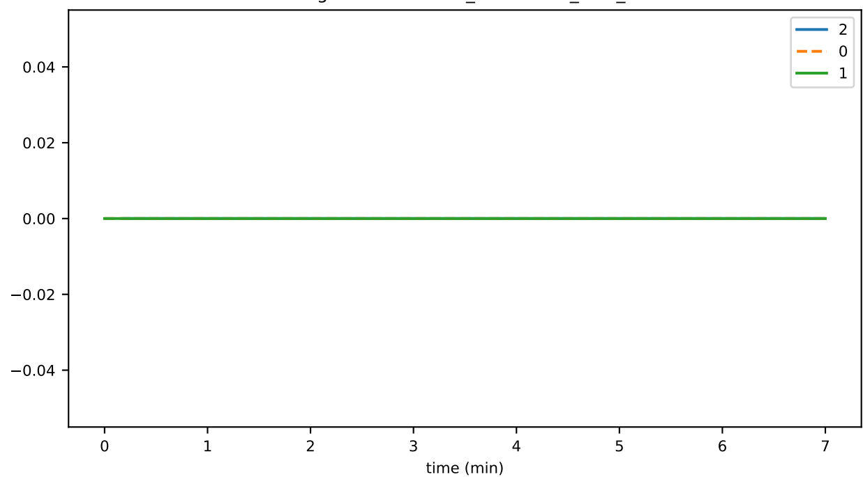
StateSignatureCollector_unhandled_task_count
