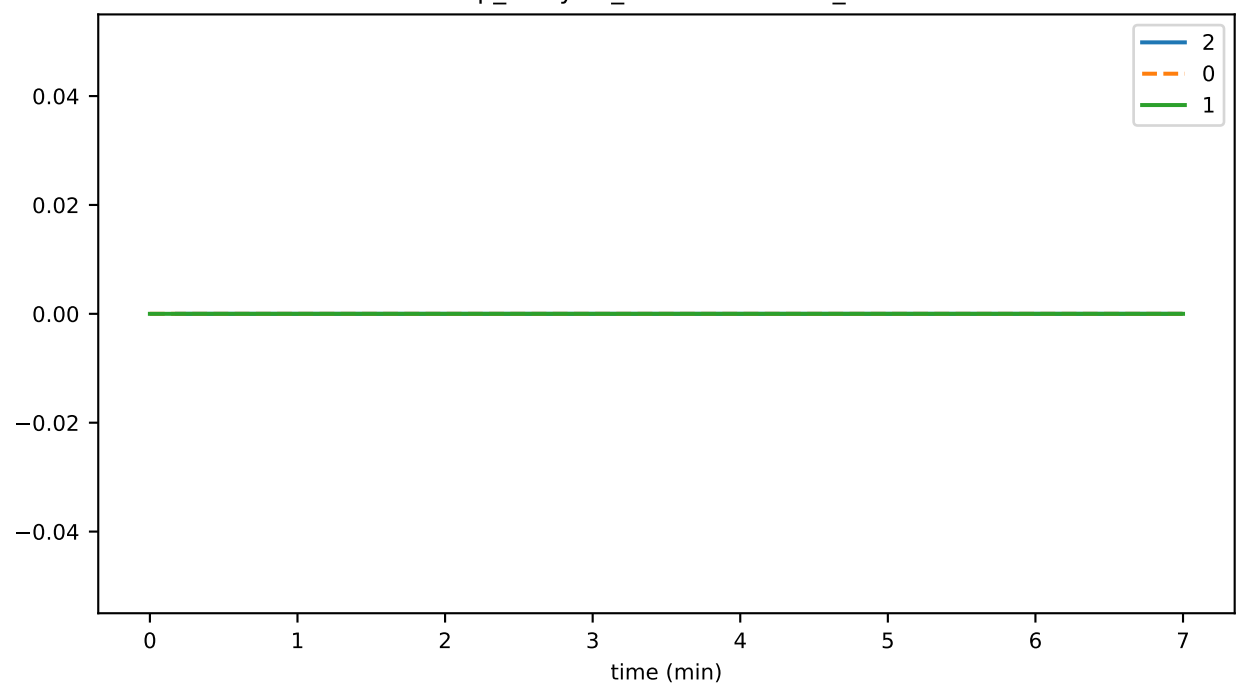
vmap_lifecycle_flushDurationMs_state
