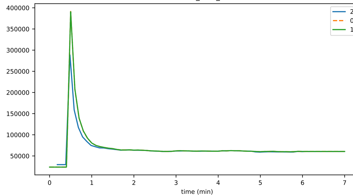
consensus_time_UPDATING_PLATFORM_STATE
