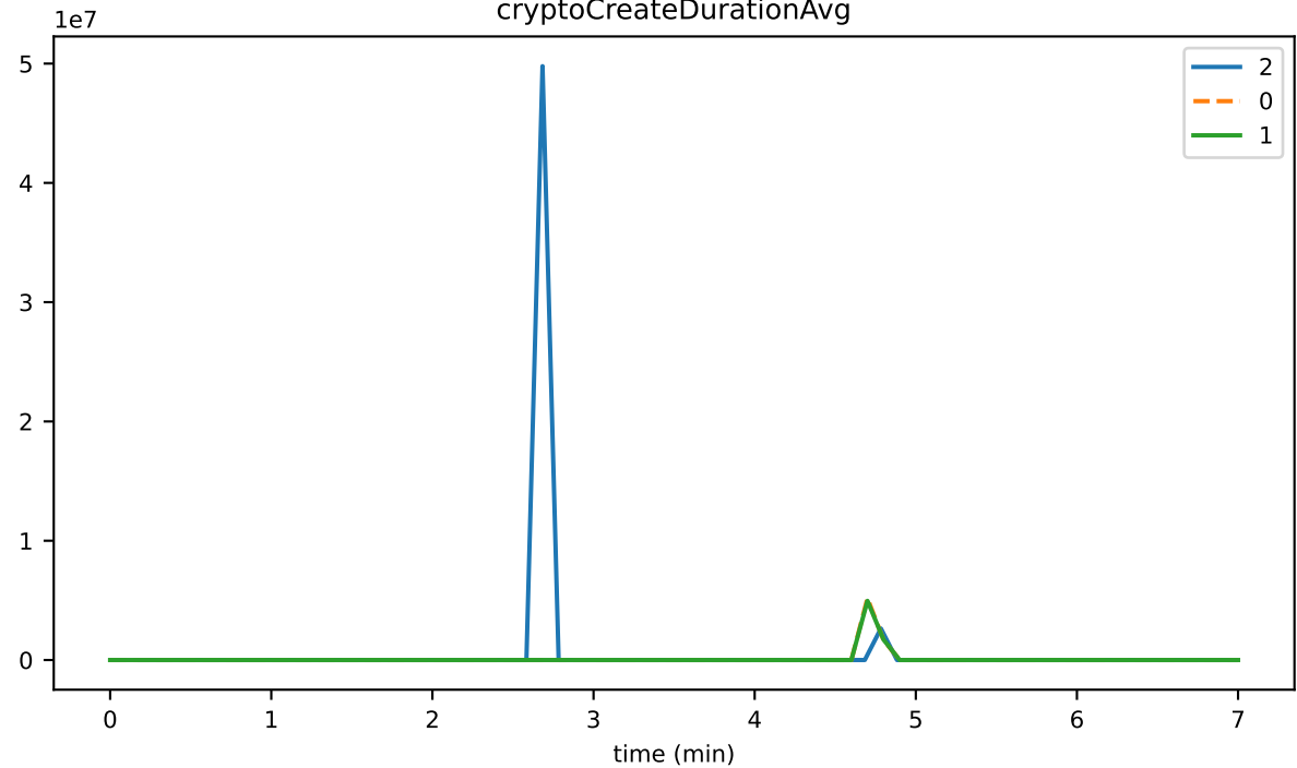
cryptoCreateDurationAvg
