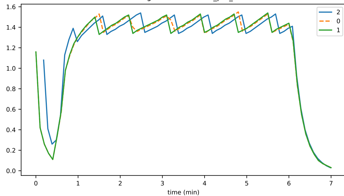
stateSignaturesGathered_per_sec
