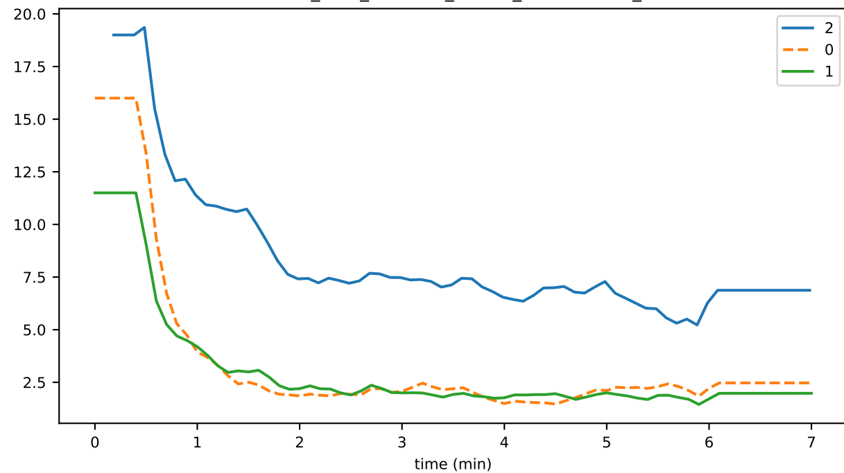
consensus_time_SETTING_EVENT_CONSENSUS_DATA
