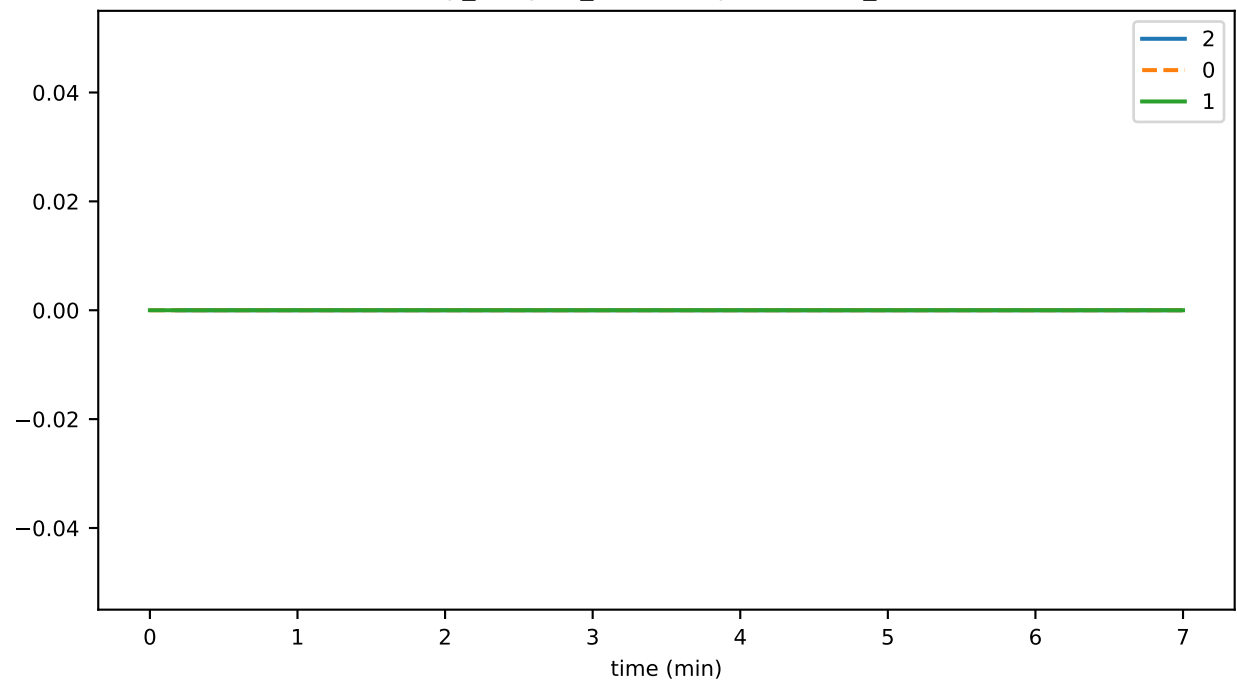
vmap_lifecycle_flushDurationMs_state
