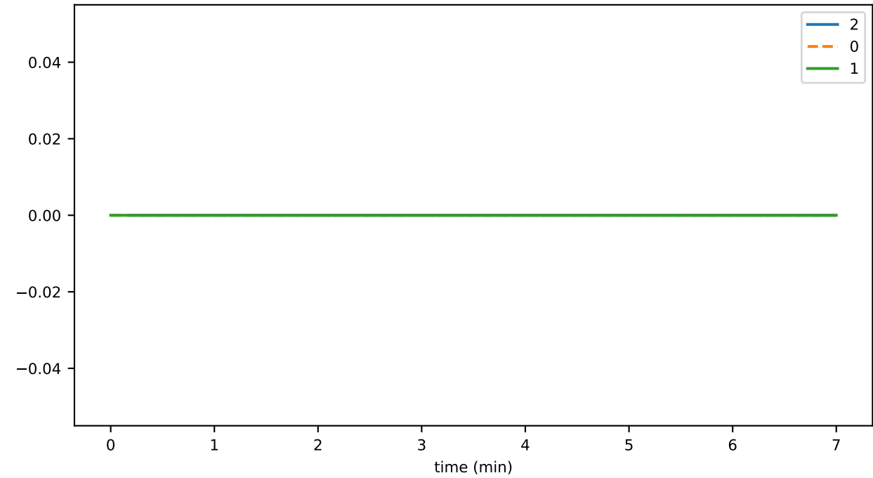
TransactionHandler_busy_fraction
