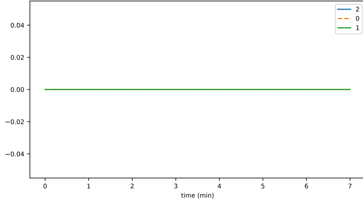
tokenPauseDurationAvg
