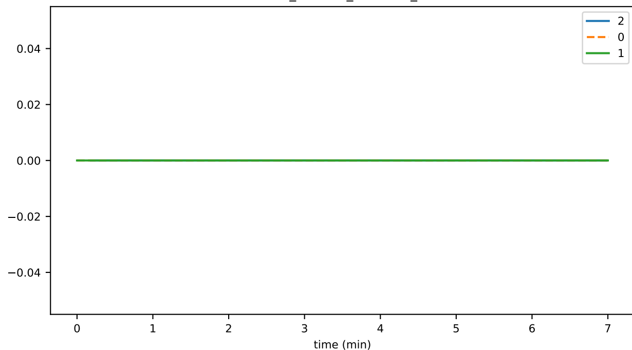
eventCreation_fraction_QUIESCENCE
