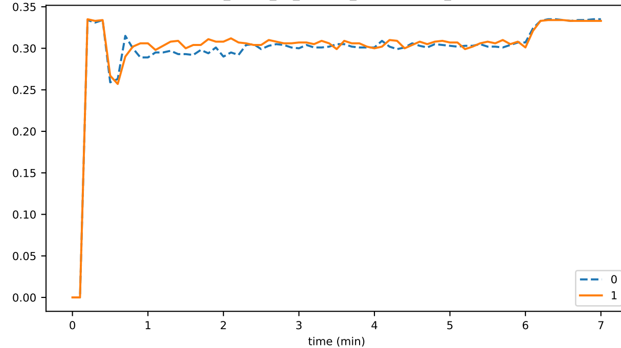
sync_phase_02_fraction_EXCHANGING_TIPS
