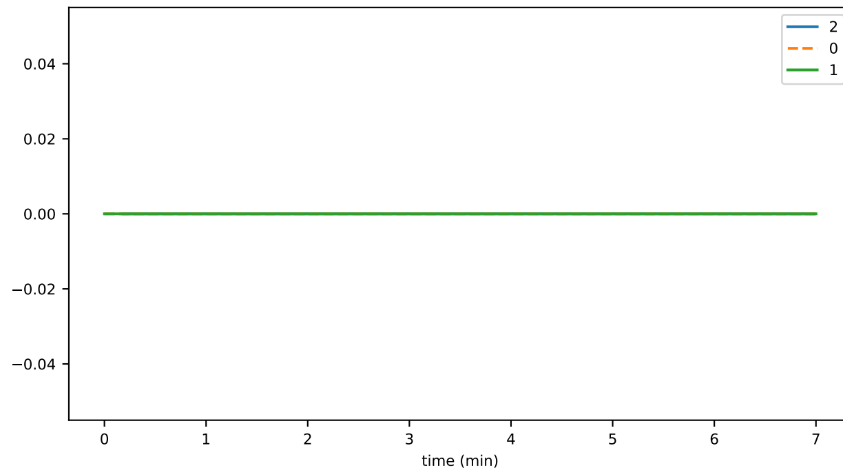
ledgerIdPublicationDurationAvg
