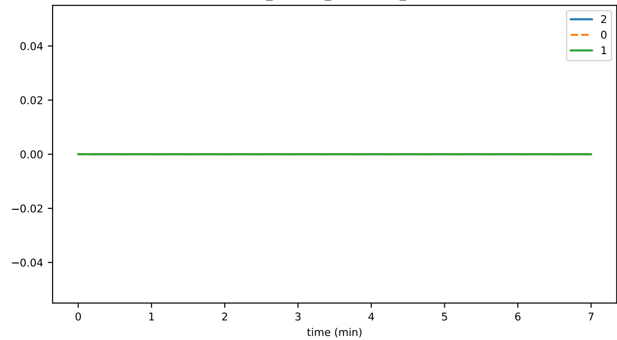
vmap_lifecycle_hashDurationMs_state
