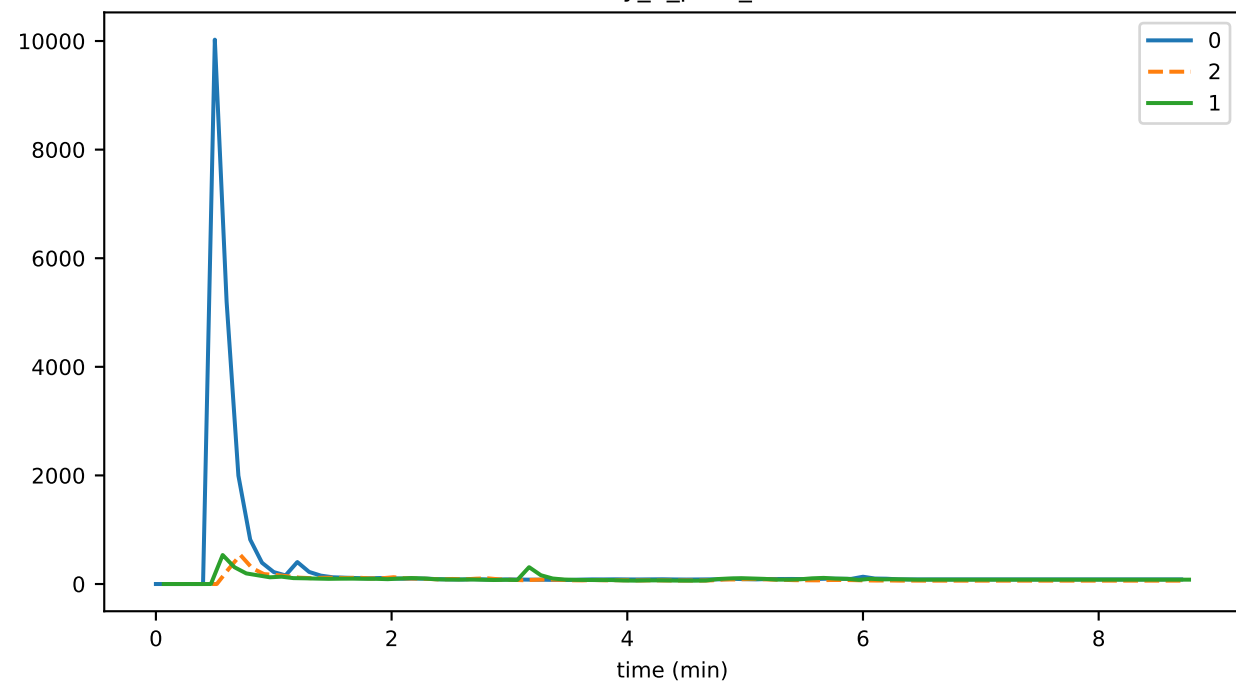
eventDelay_6_pces_runtime
