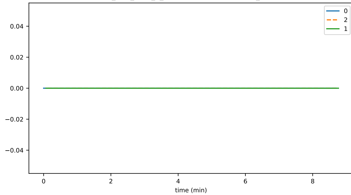
ds_files_level_3_hashesFileSizeByLevelMb_state
