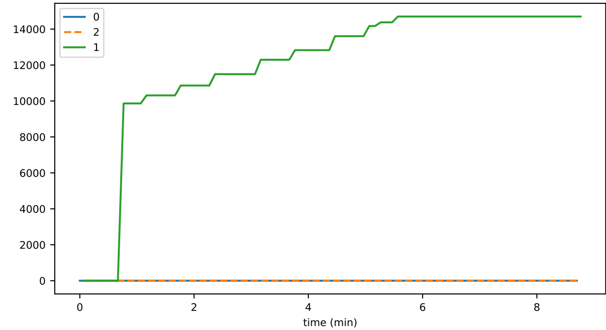
getAccountDetailsDurationAvg
