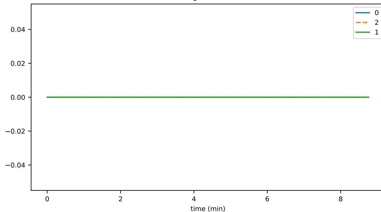
hintsPreprocessingVoteDurationAvg
