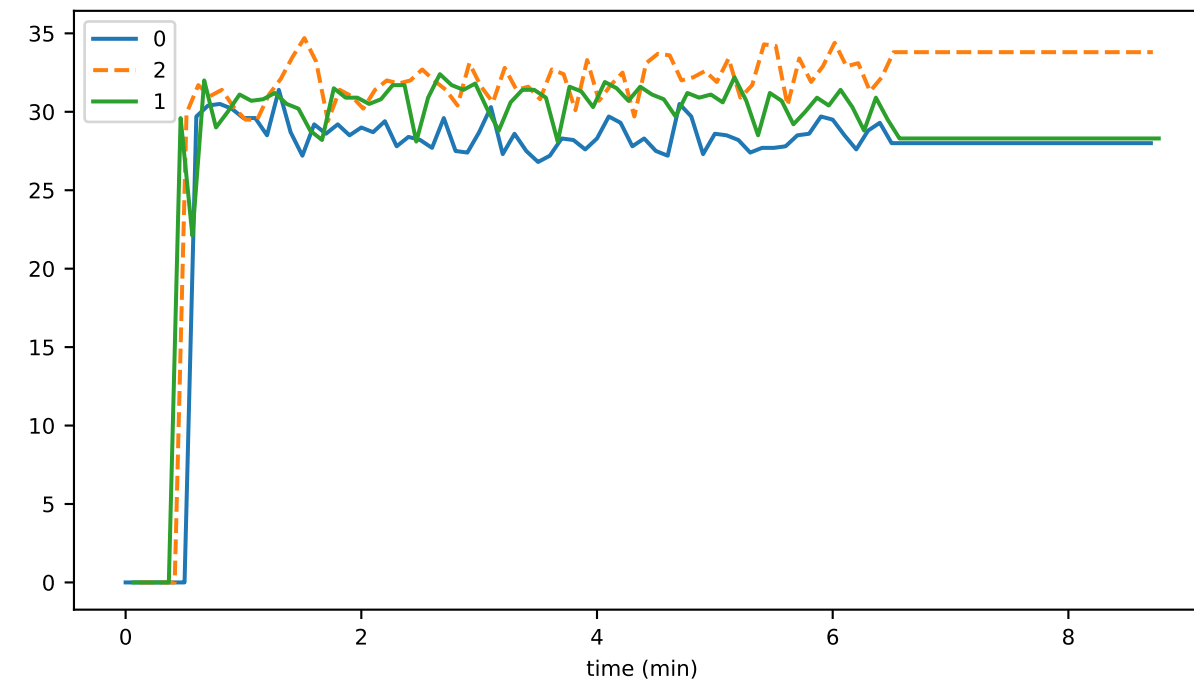
eventsFailedSignatureValidation
