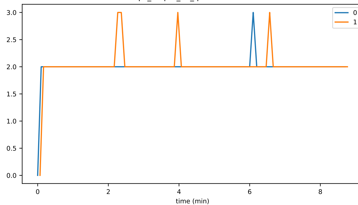
rpc_output_02_queueMaxSize
