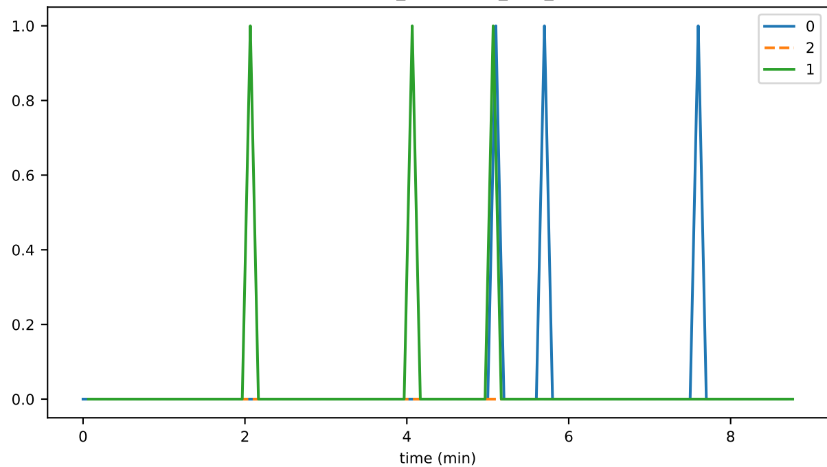
HealthMonitor_unhandled_task_count
