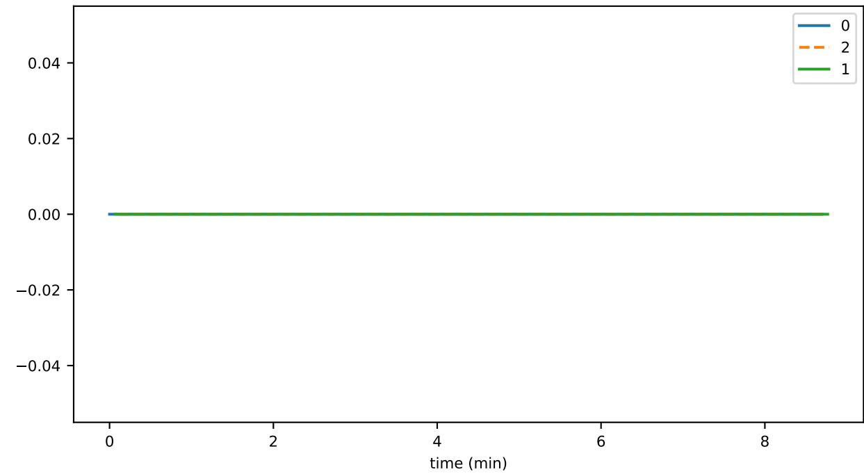
historyProofTransR3ToAggMs
