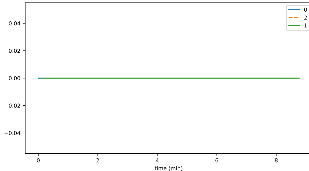
networkGetExecutionTimeThrottledTxns
