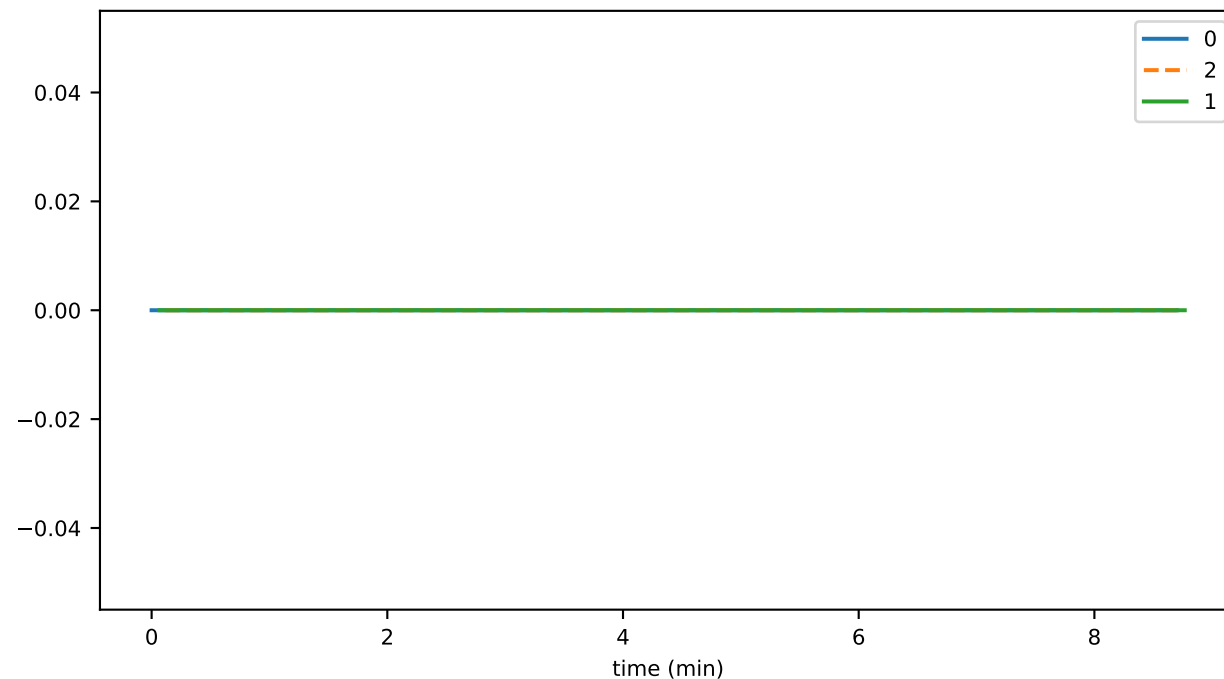
healthy
