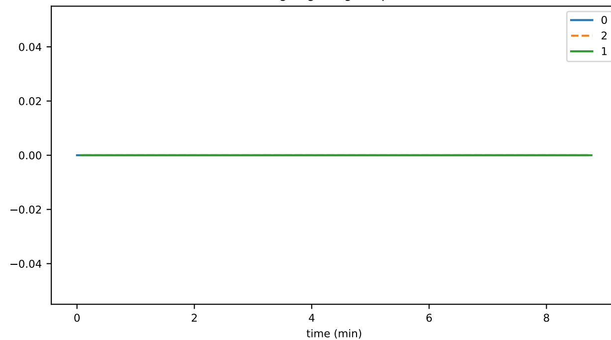
hintsSigningNoSigCompletions
