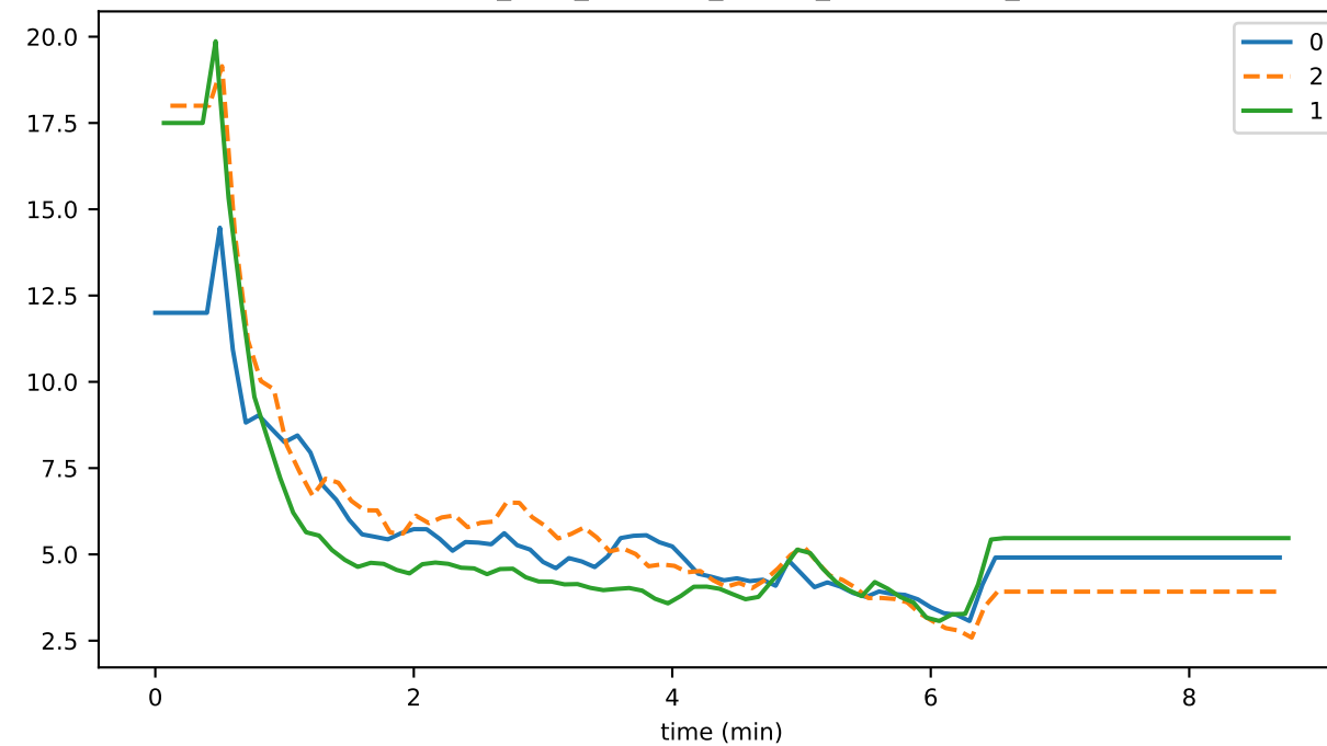
consensus_time_SETTING_EVENT_CONSENSUS_DATA
