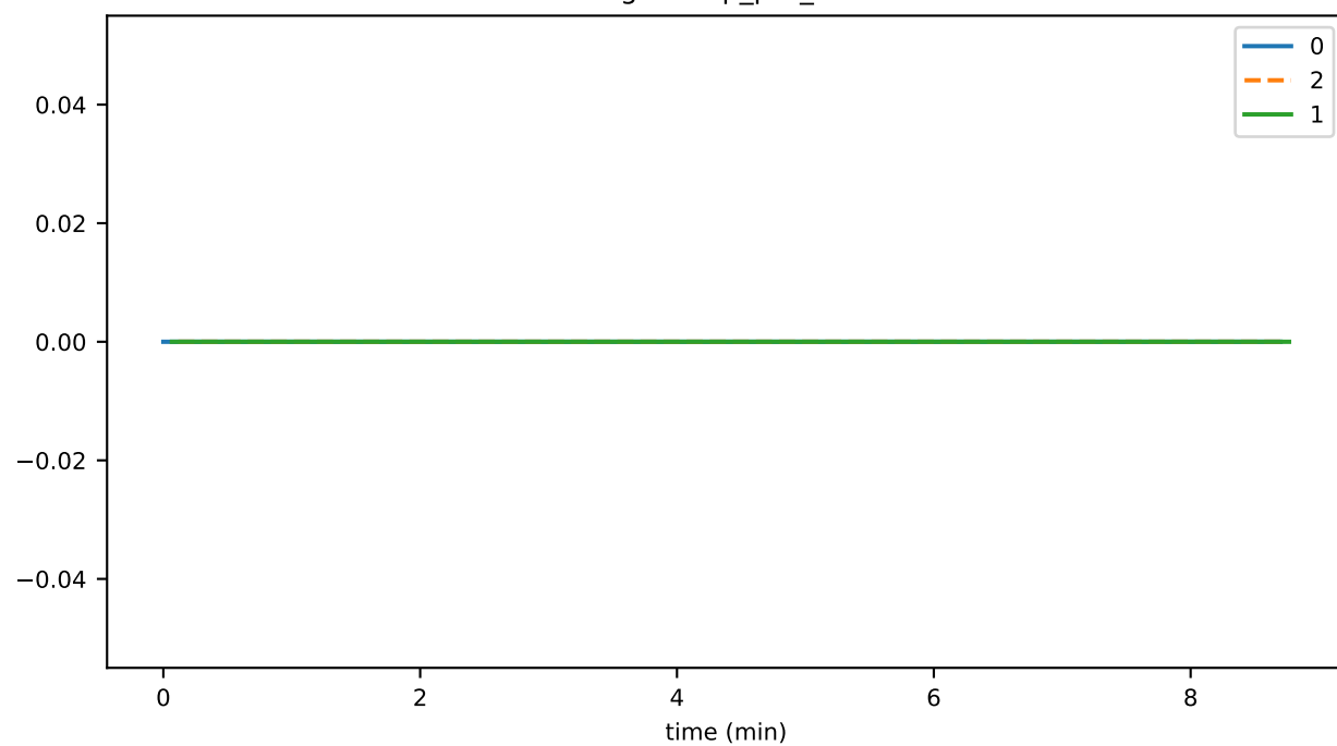
DigLockUp_per_sec
