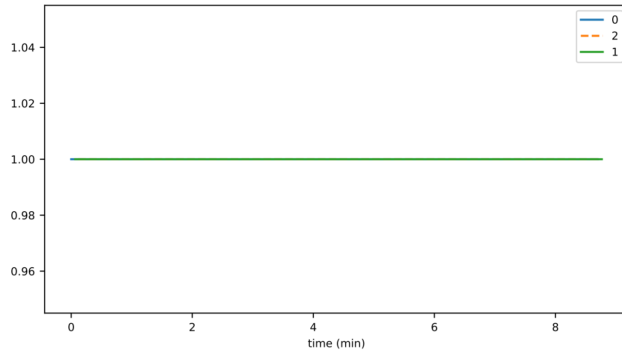
healthy
