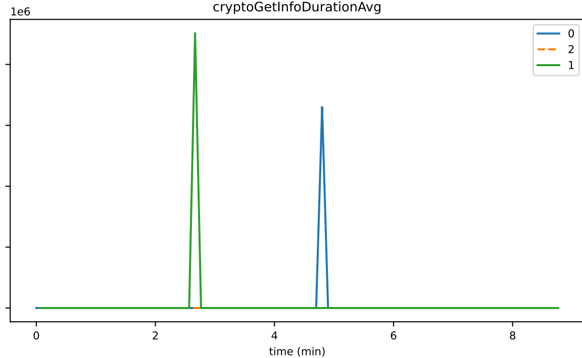
cryptoGetInfoDurationAvg
