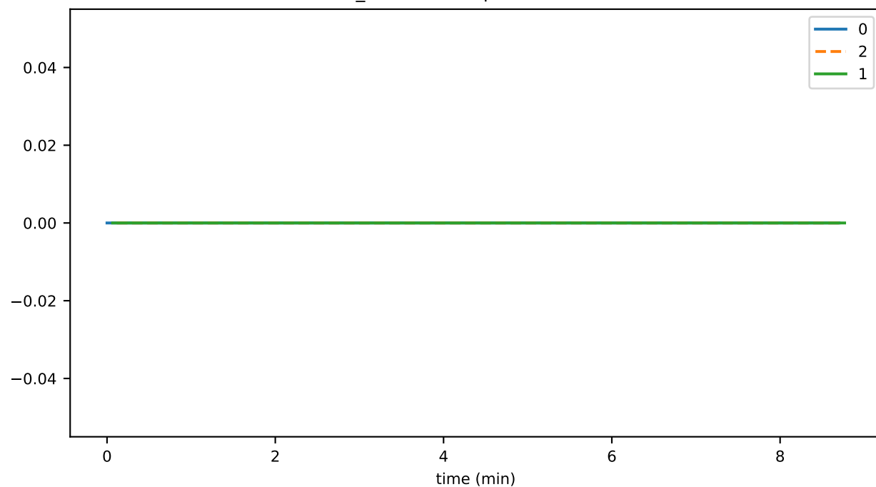
connSend_requestBytes
