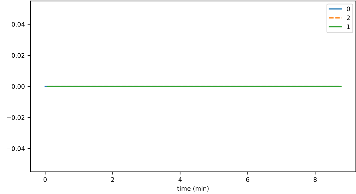
nodeUpdateDurationMax
