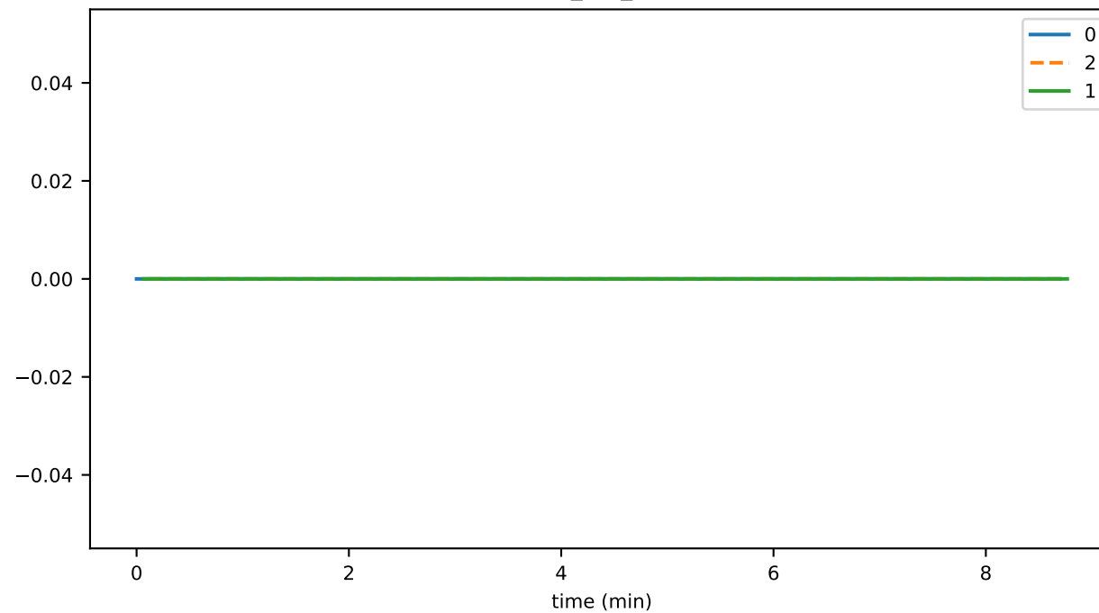
Dig_per_sec
