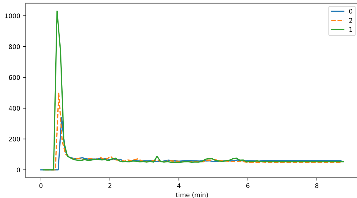
eventDelay_2_validation_runtime
