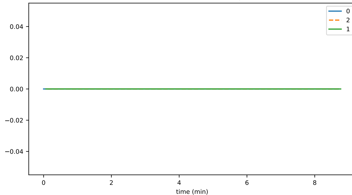
contractDeleteThrottledTxns
