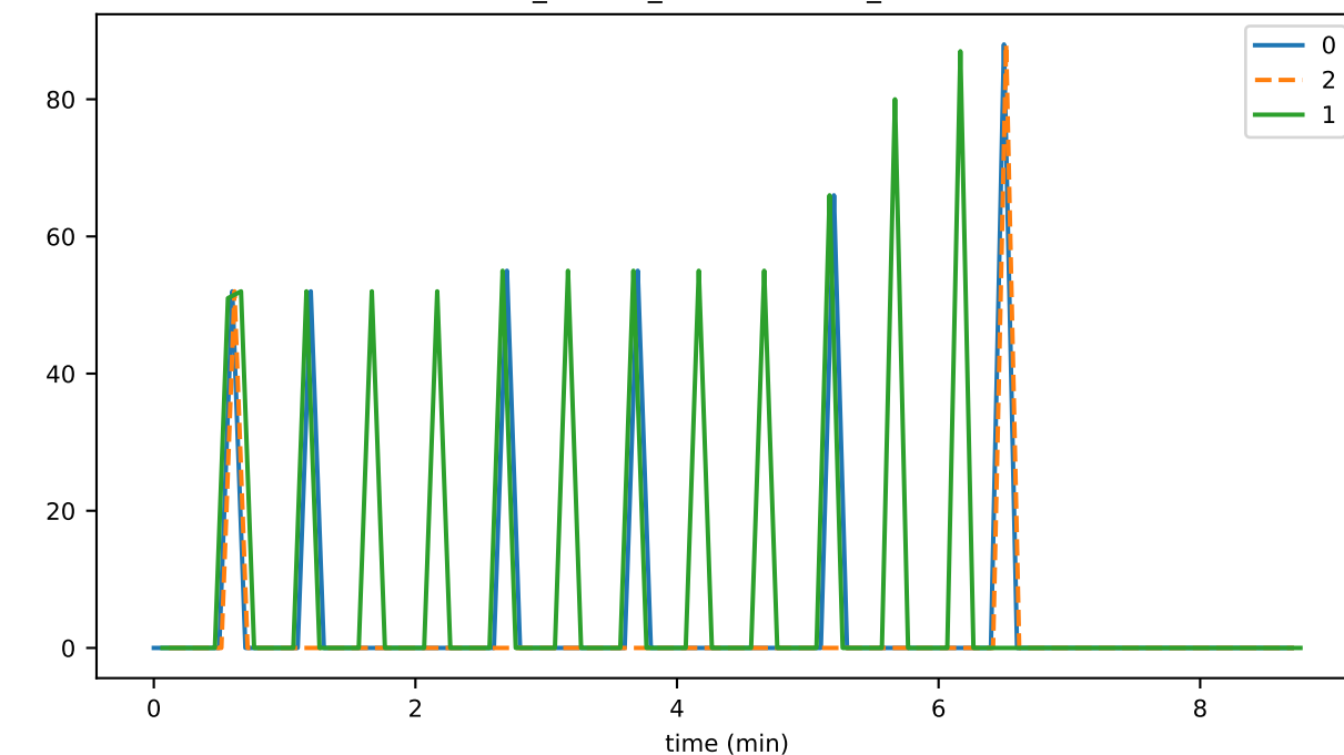
ds_flushes_leafKeysWritten_state
