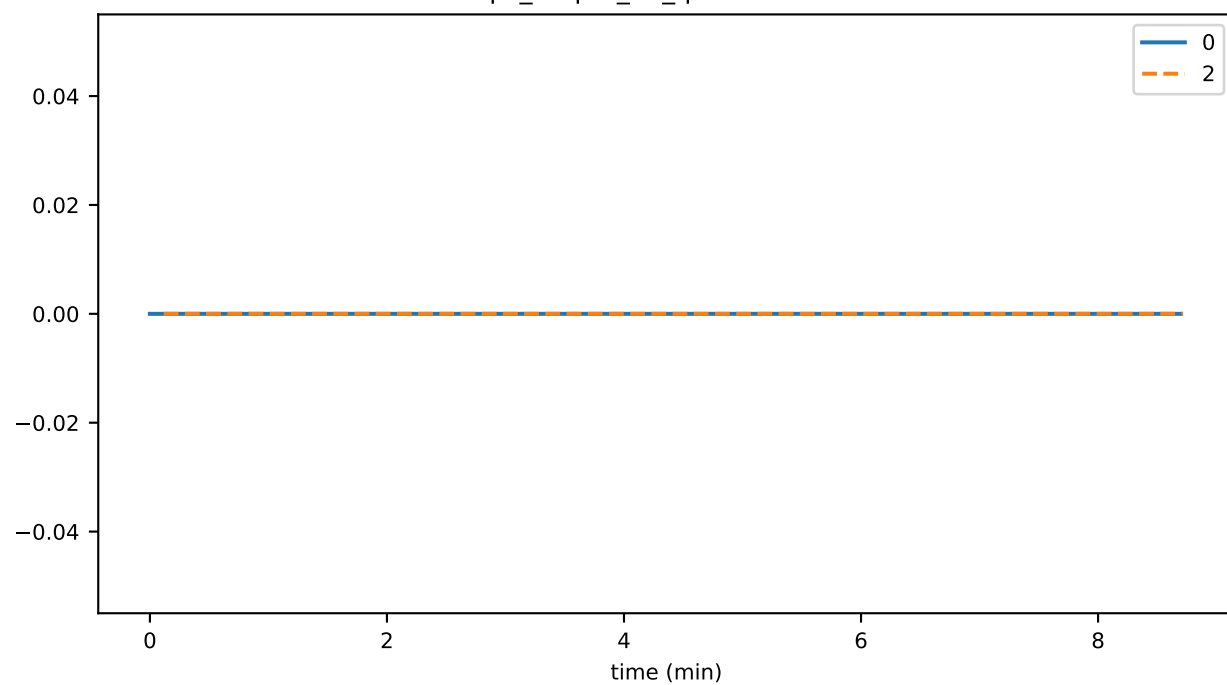
rpc_output_01_queueMinSize
