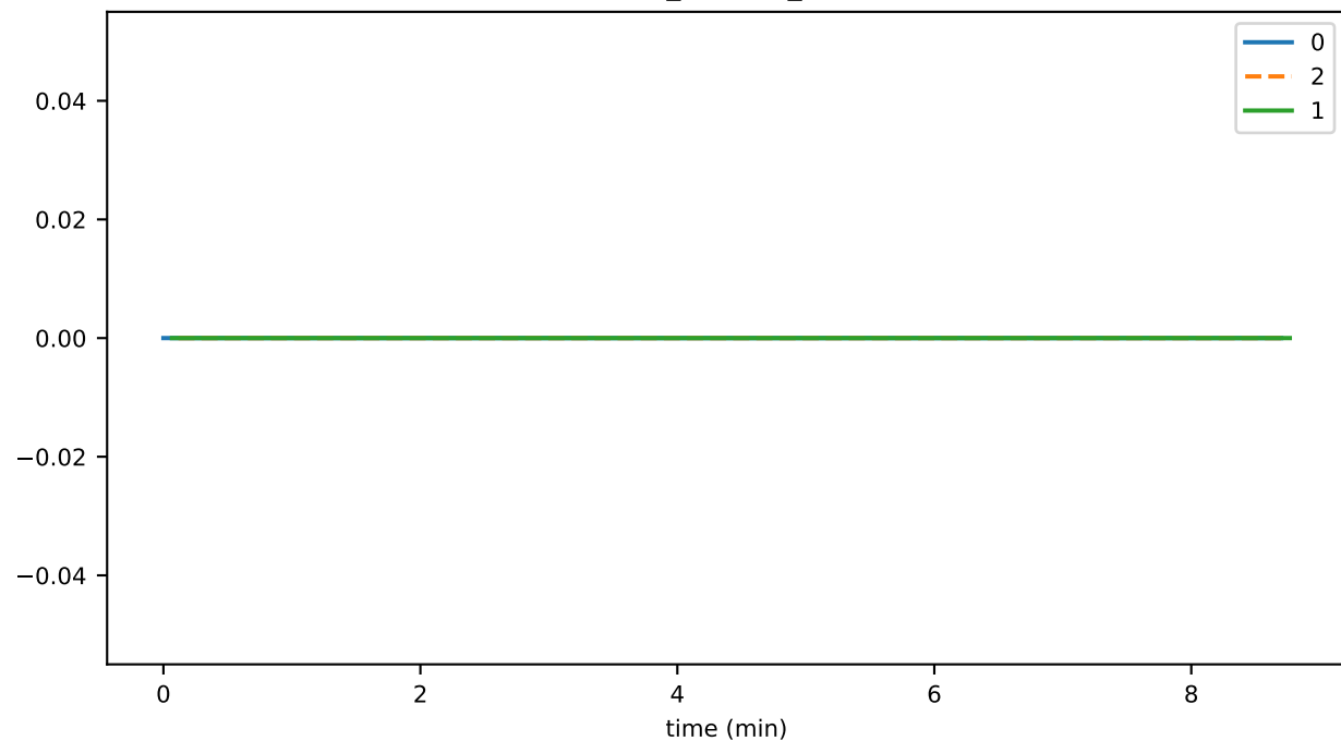
eventCreation_fraction ROUND_LAG
