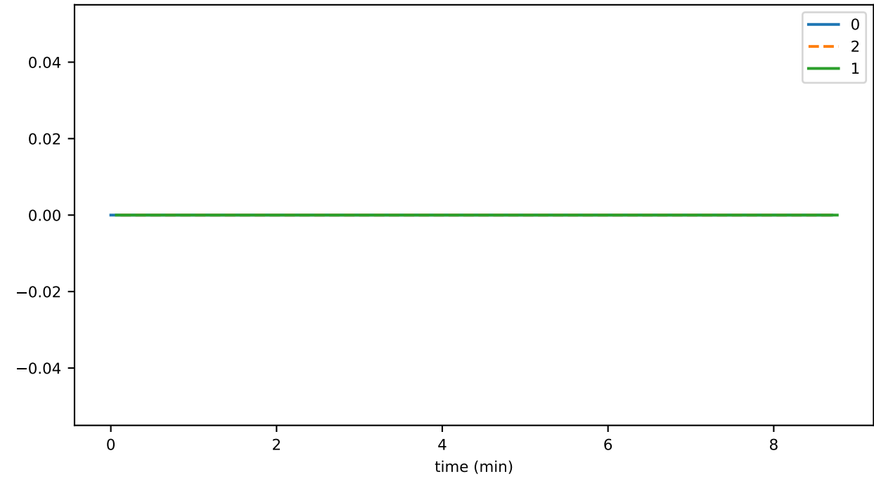
countInMemorySignedState
