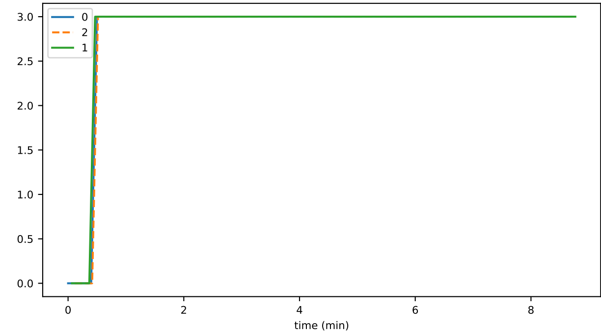
nodeUpdateDurationMax
