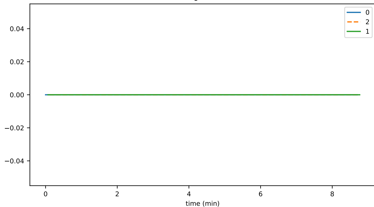
1e7 schedulesMaxNumber
