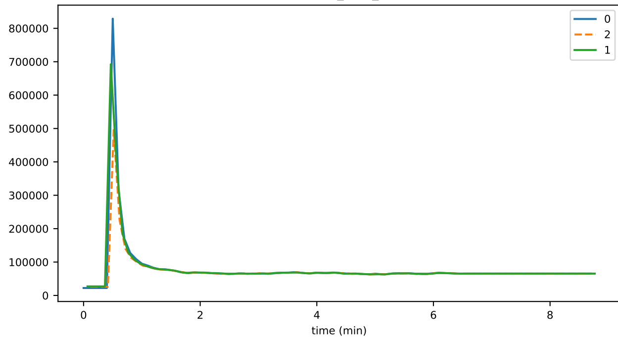
consensus_time_IDLE
