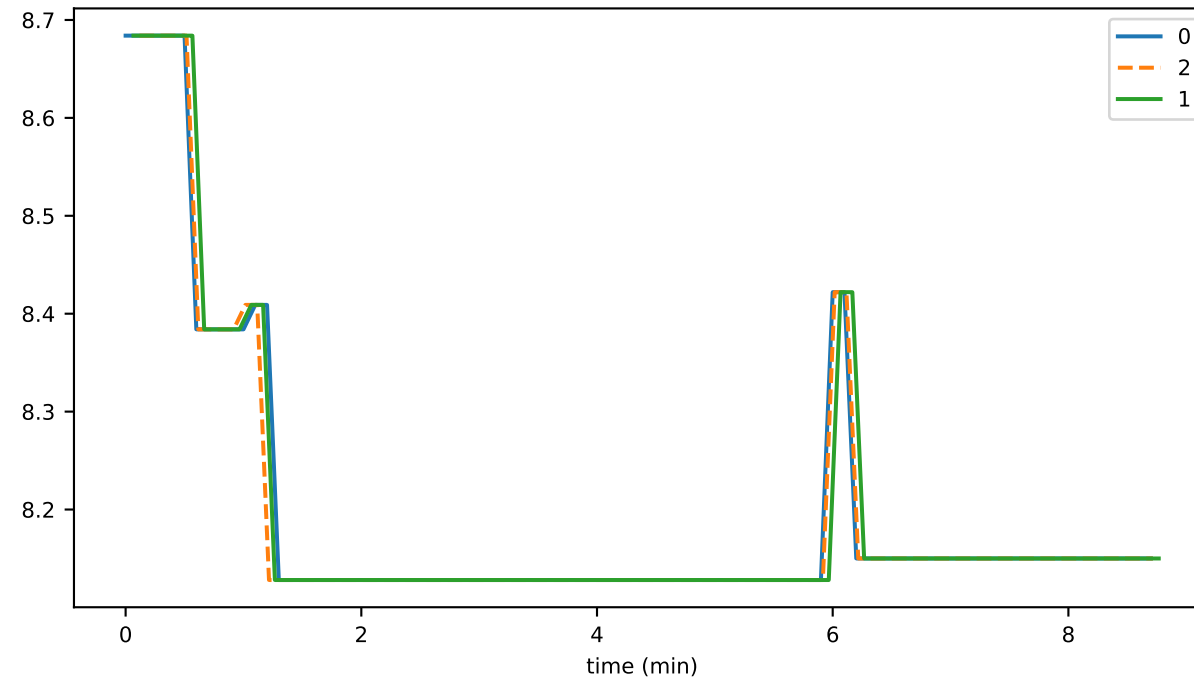
preconsensusEventFileAverageSizeMB
