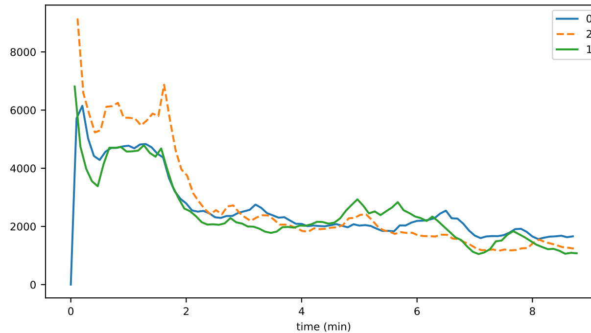
syncFilterTime
