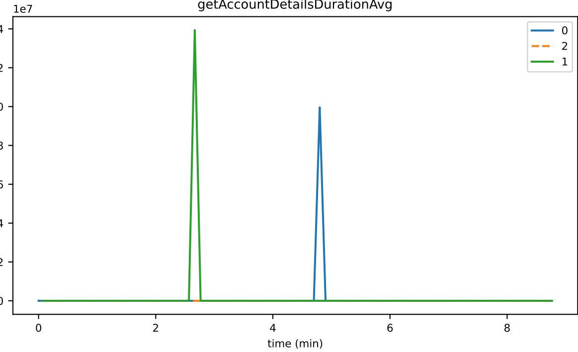
getAccountDetailsDurationAvg
