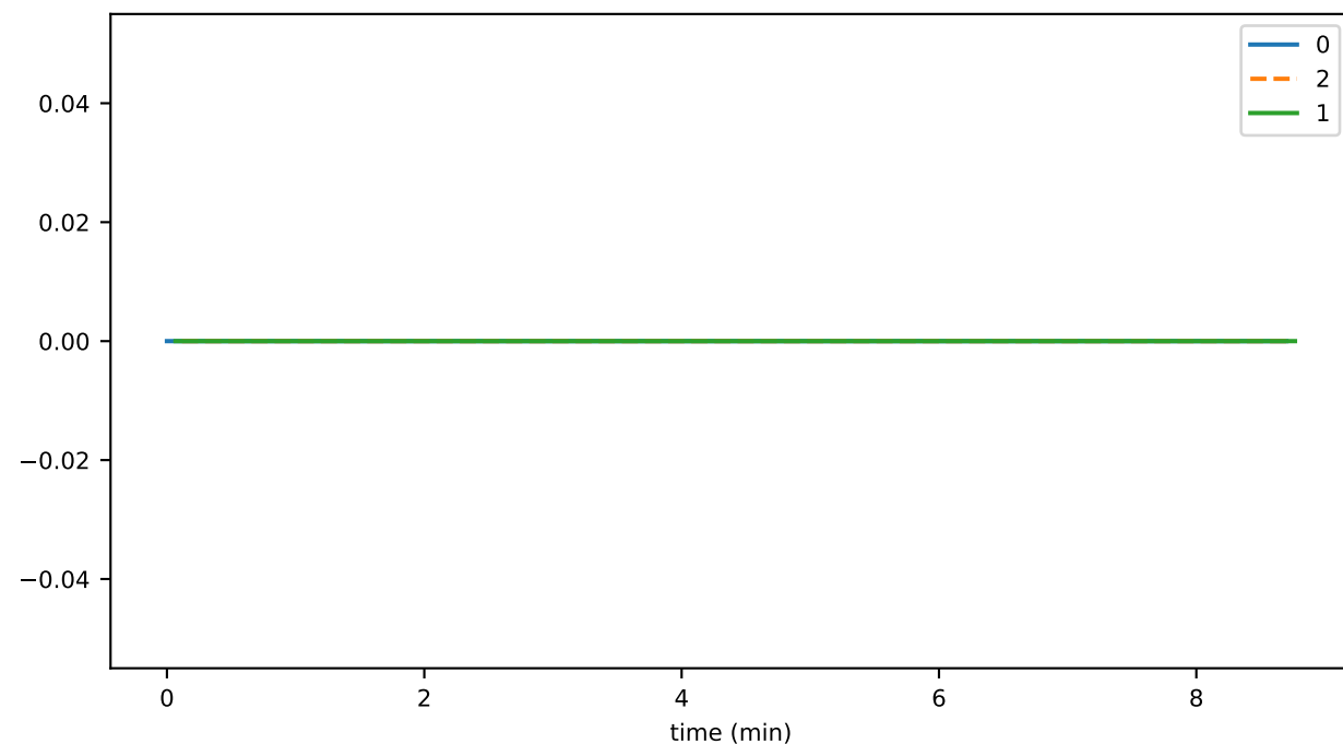
ledgerIdPublicationDurationMax
