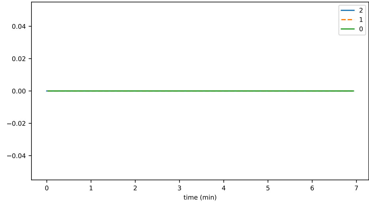
ds_compactions_level_3_leavesSavedSpaceMb_state
