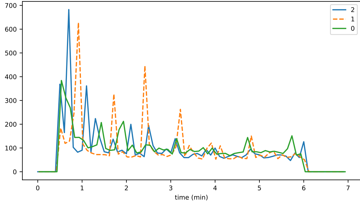
eventDelay_4_verification_storageMAX
