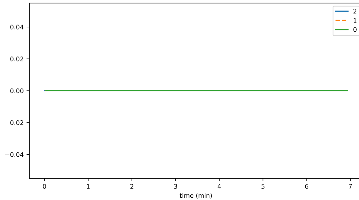
tokenClaimAirdropThrottledTxns
