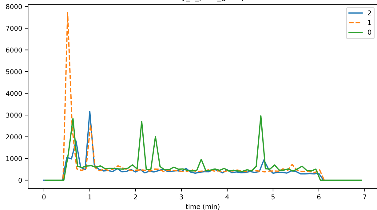
eventDelay_6_pces_gossipMAX
