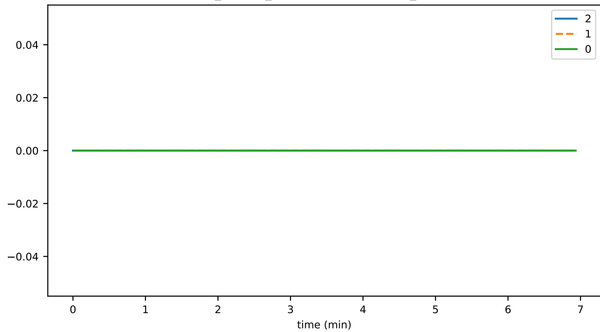
ds_flushes_leavesStoreFileSizeMb_state
