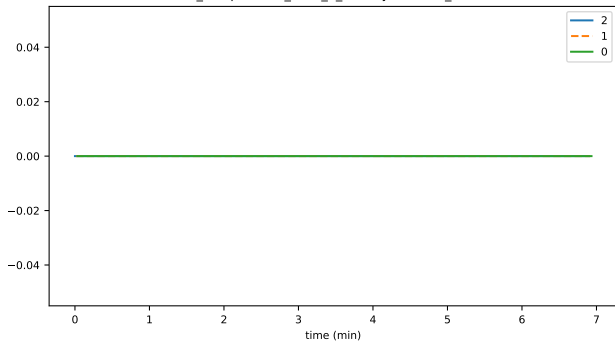
ds_compactions_level_2_leavesTimeMs_state
