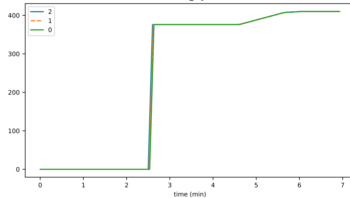
recordHashes_highestBlock
