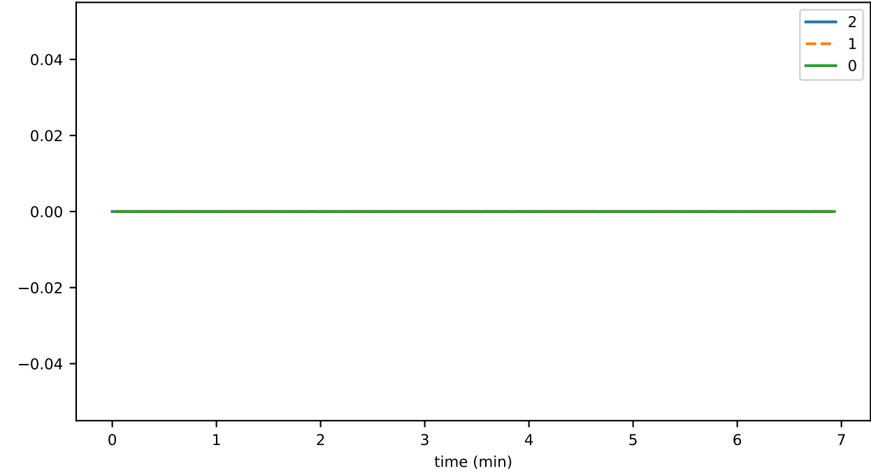
connSend_latestBlockEndOfBlock
