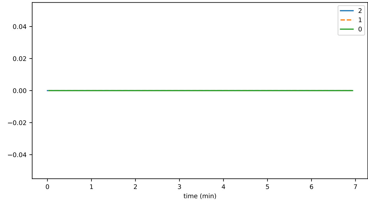
connRecv_endStream_error
