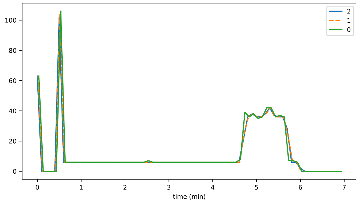
ds_reads_leafKeys_state
