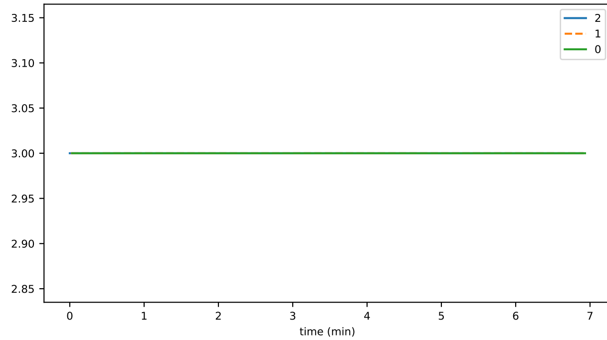
nodesPercentUsed
