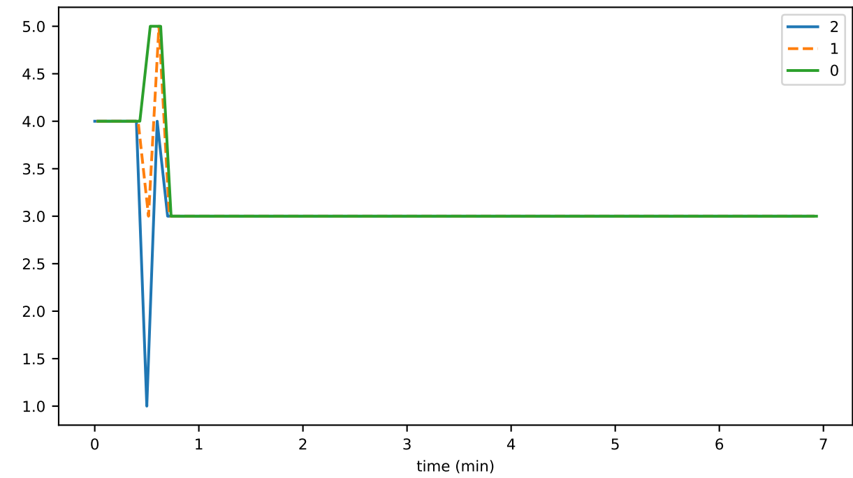
eventsPerRound
