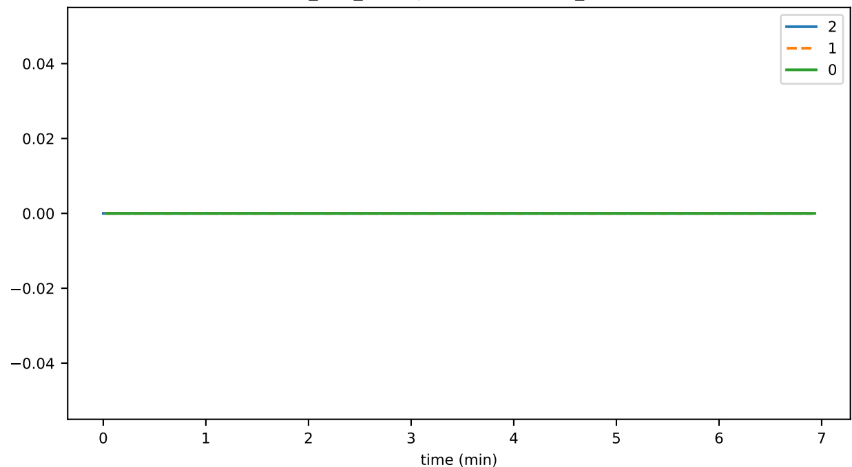
ds_files_leavesStoreFileSizeMb_state
