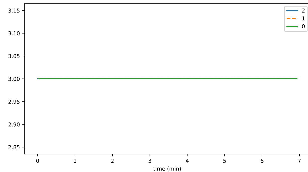
nodesUsed
