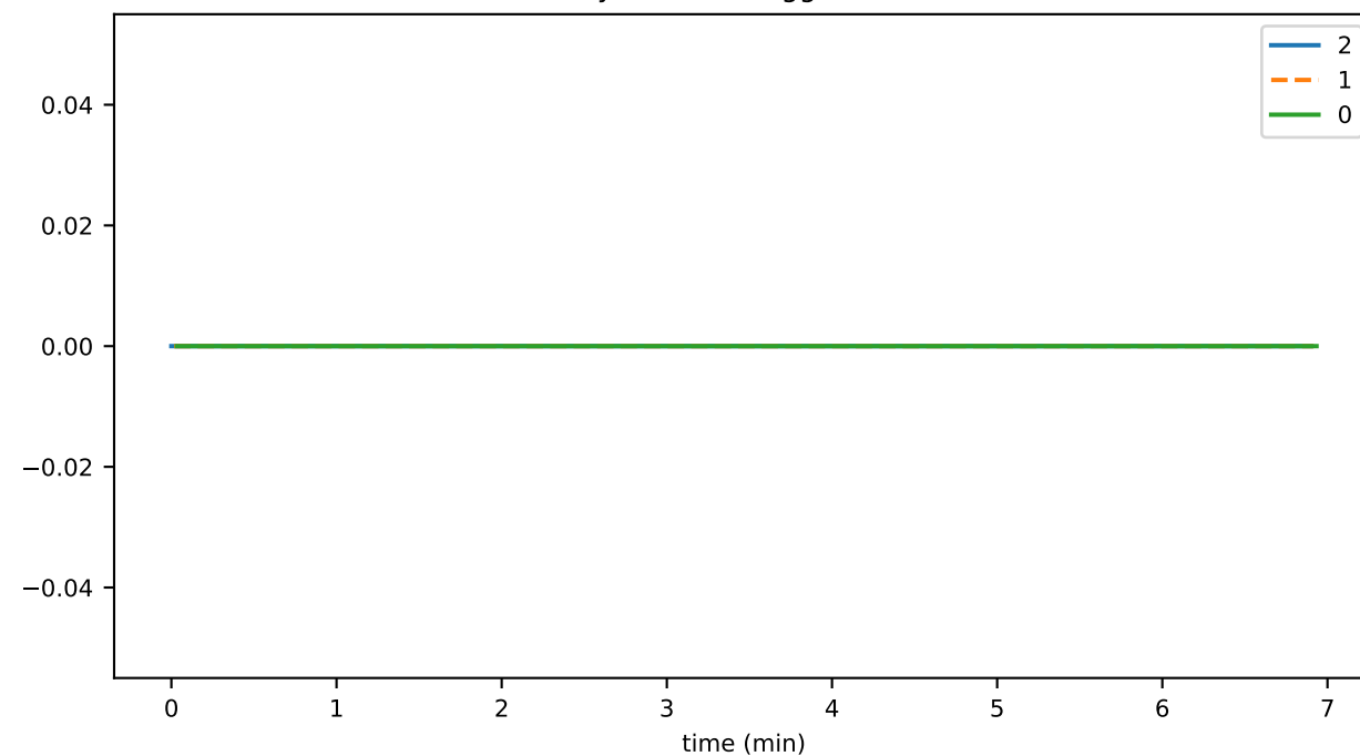
historyProofTransAggToFailCnt
