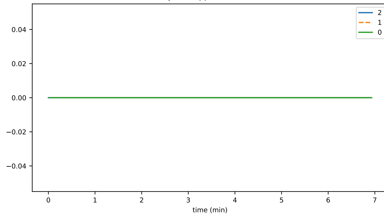
rejectedAppTransactions
