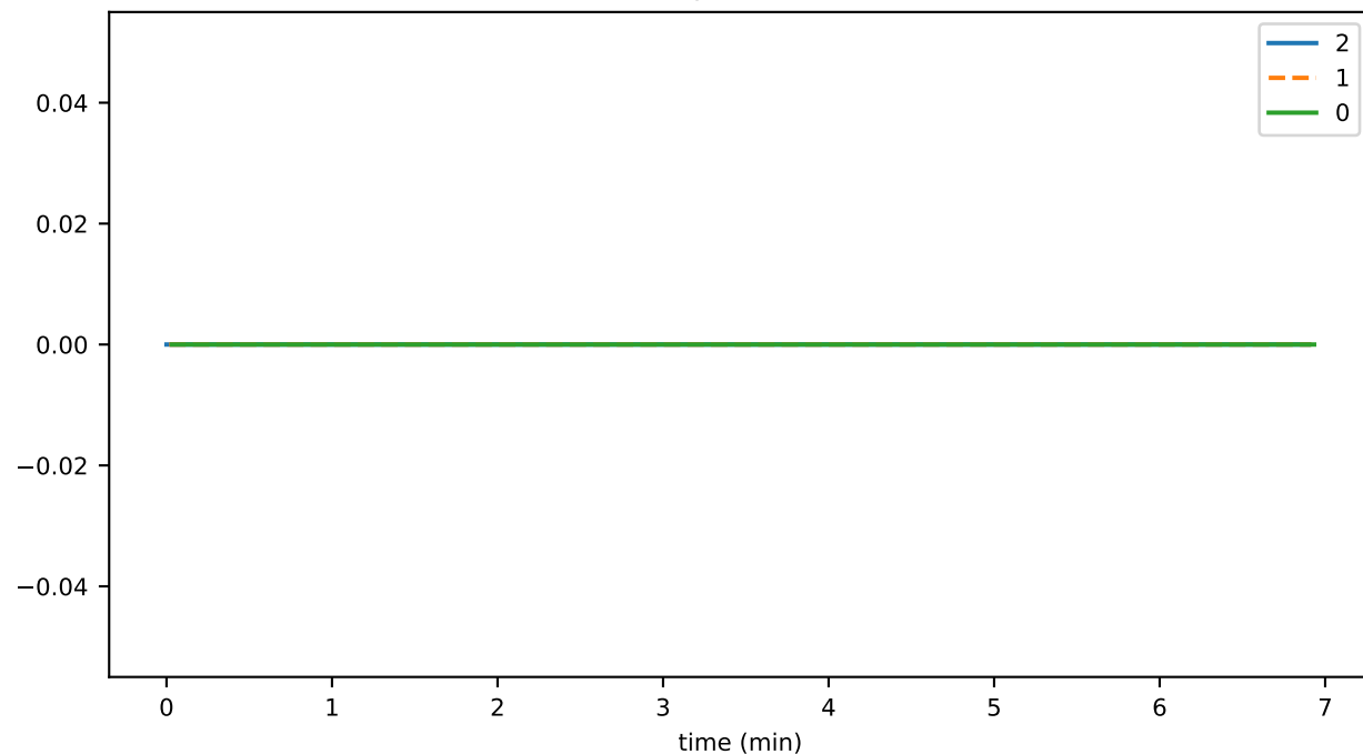
nodesUsed
