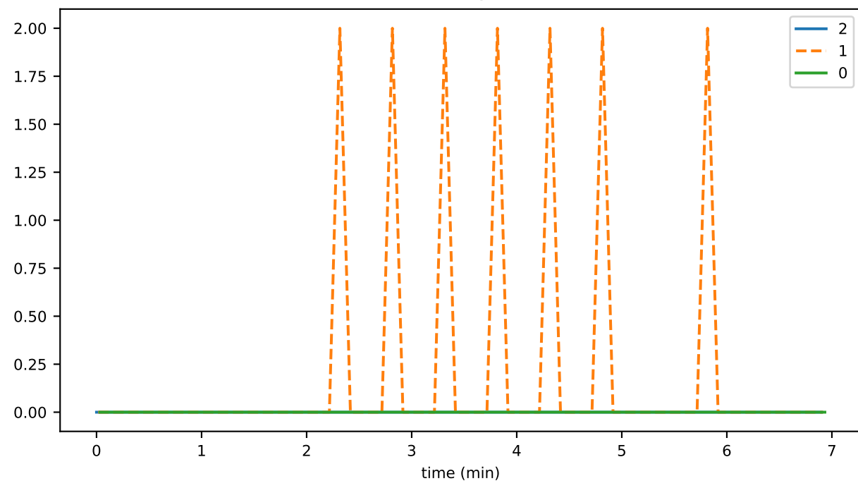
eventsWithInvalidBirthRound
