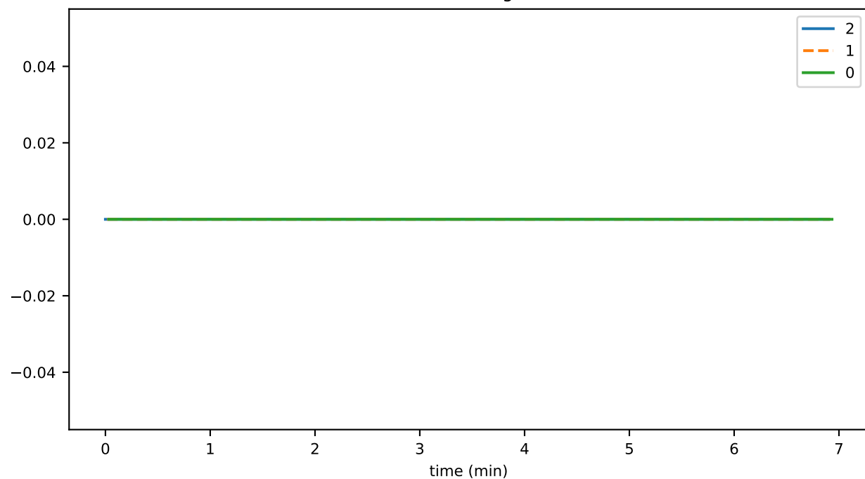
consensusTimeDeviation
