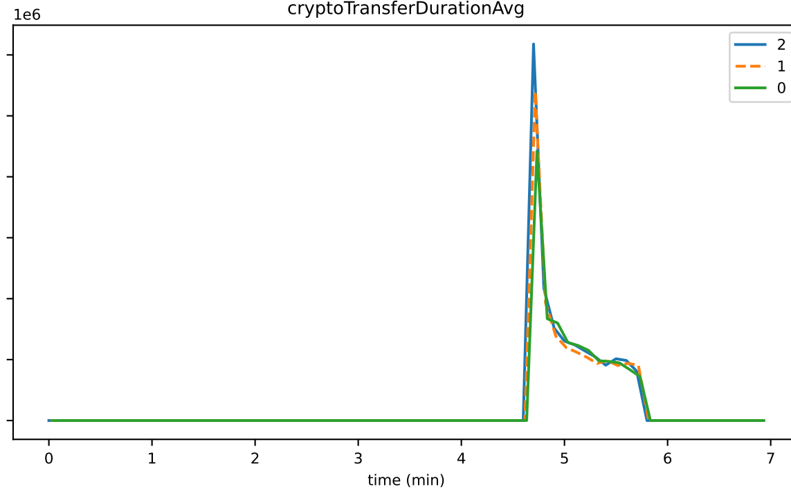
cryptoTransferDurationAvg
