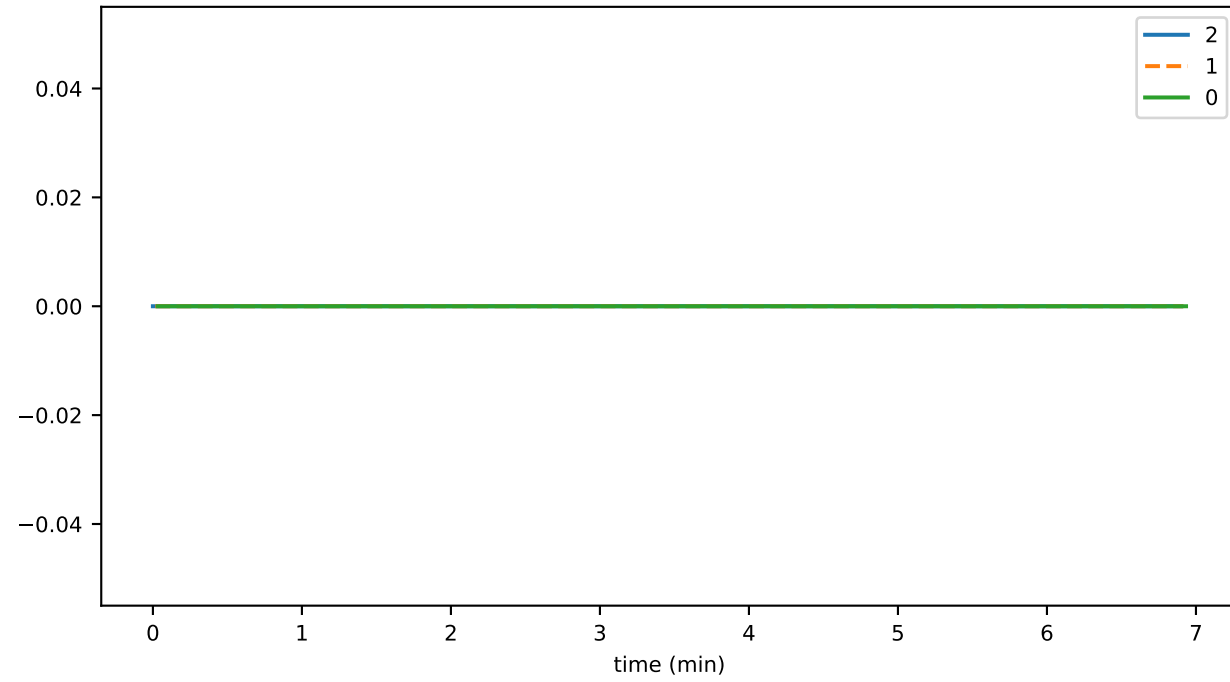
consensusSubmitMessageDurationAvg
