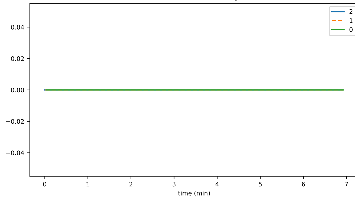
nodeDeleteDurationAvg
