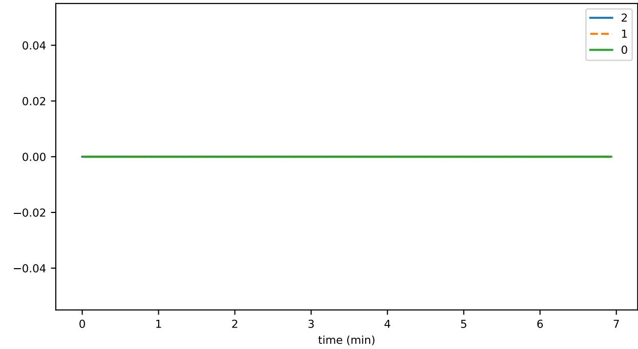
connSend_latestBlockEndOfBlock
