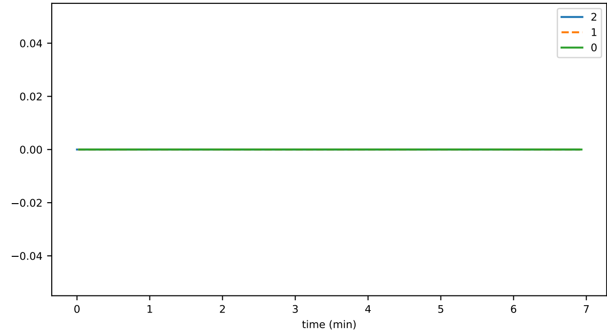
consensusSubmitMessageDurationMax
