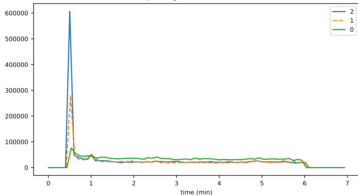
pcesAvgTotalWriteDuration
