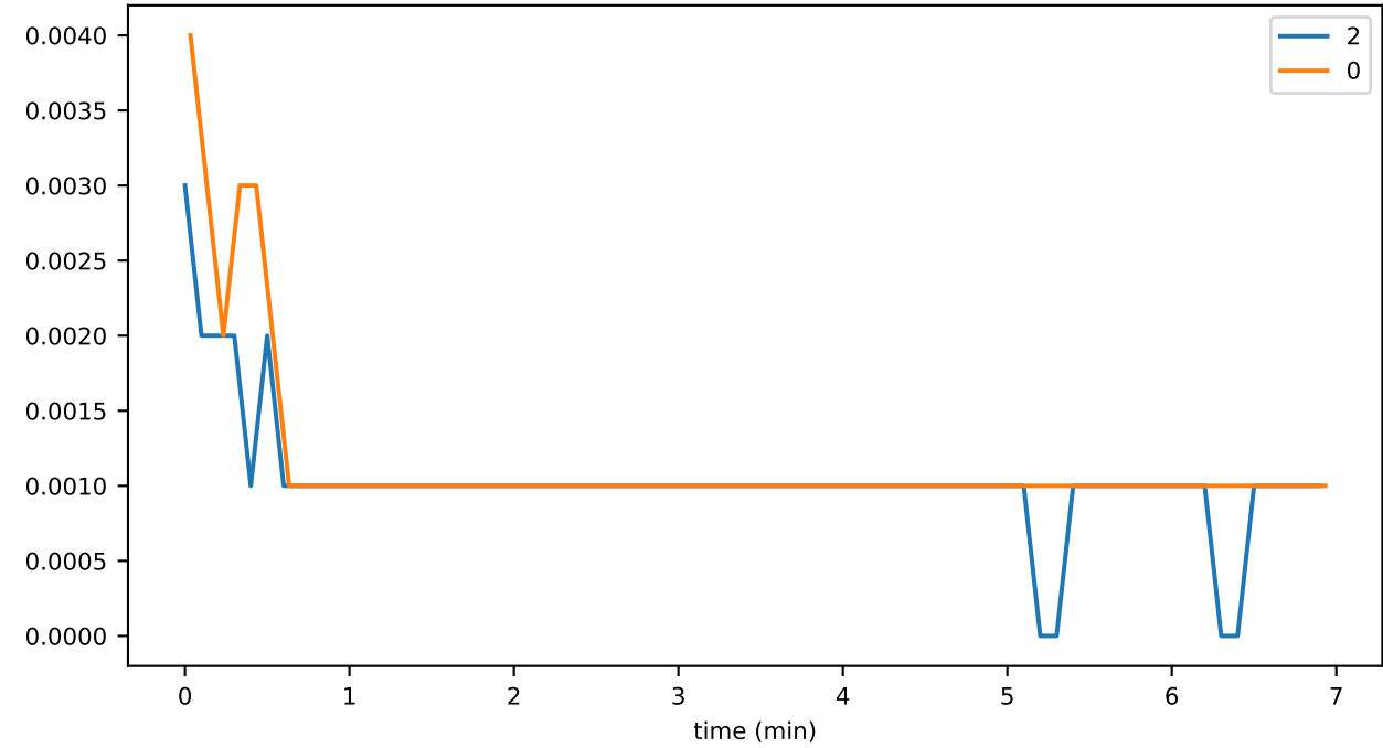
sync_phase_01_fraction_EXCHANGING_WINDOWS
