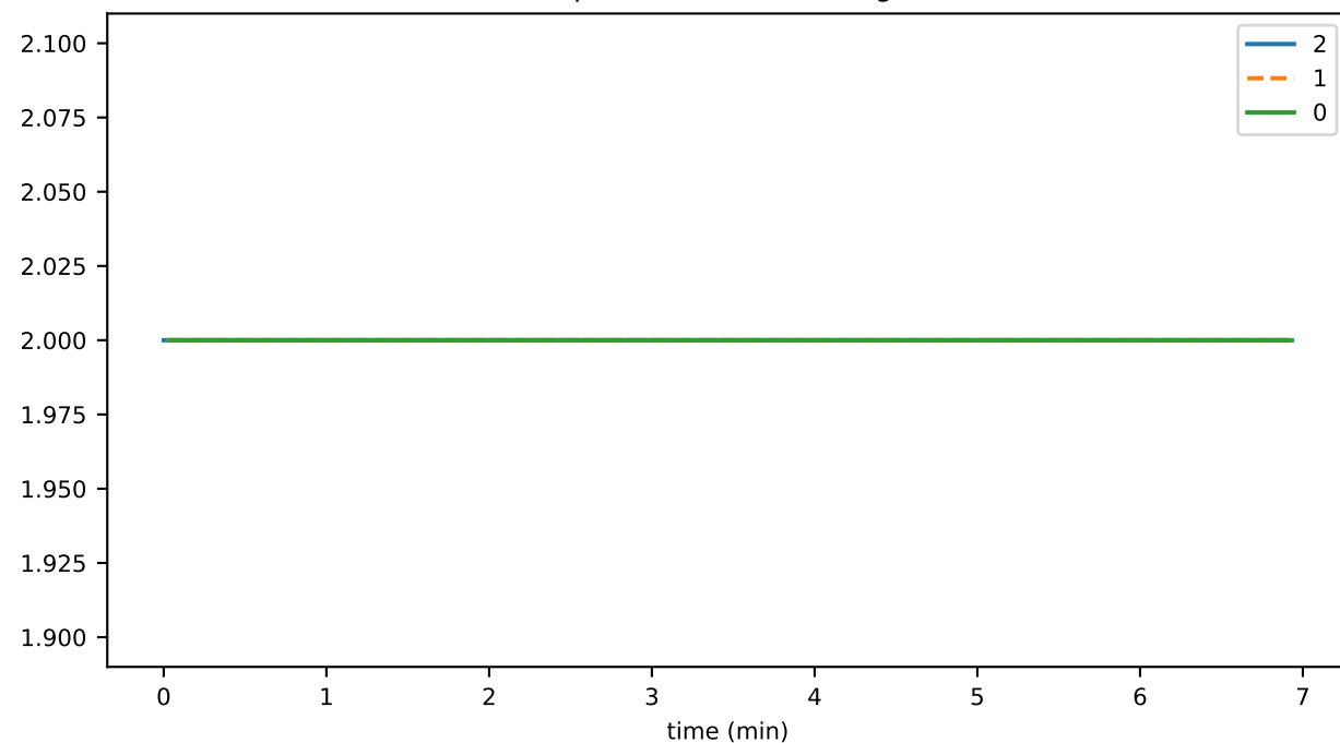
rpcWriteThreadRunning
