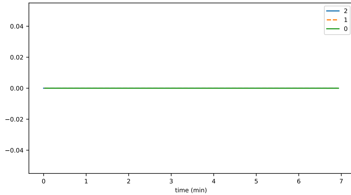
historyAssemblySignatureThrottledTxns
