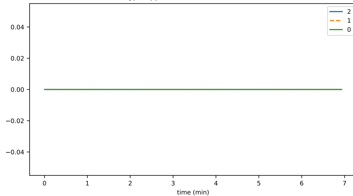
cryptoApproveAllowanceThrottledTxns
