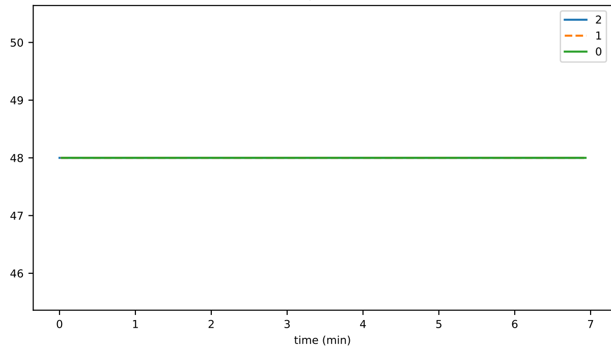
receiverReconnectDurationSeconds
