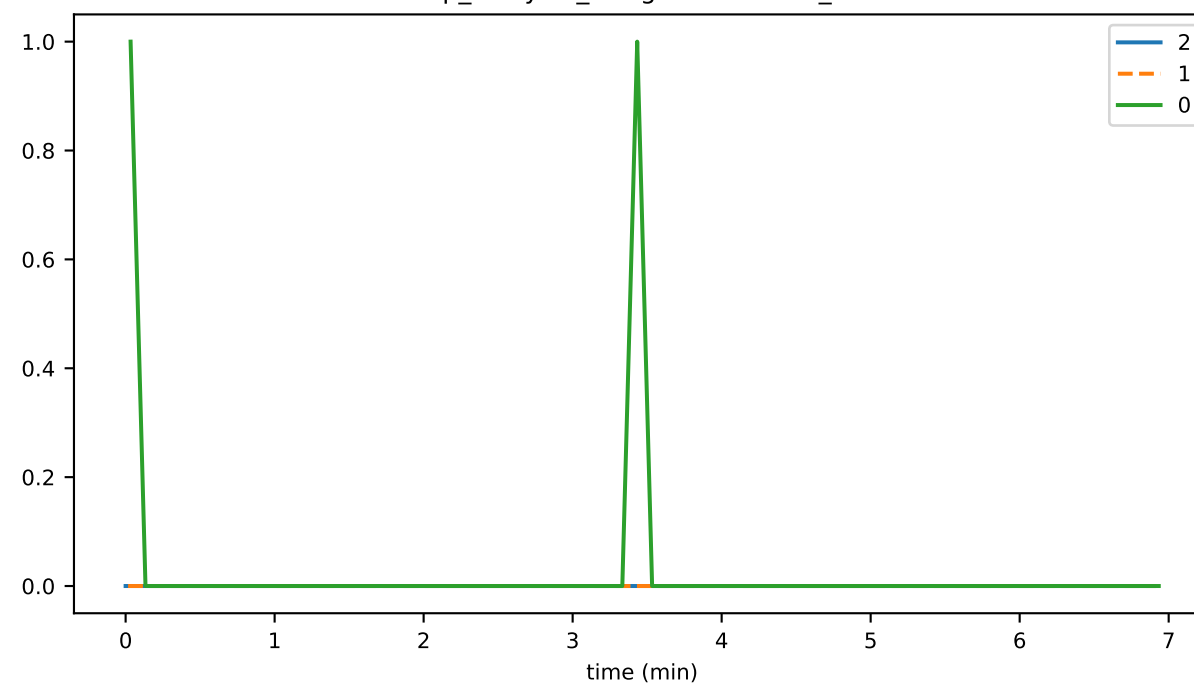
vmap_lifecycle_mergeDurationMs_state
