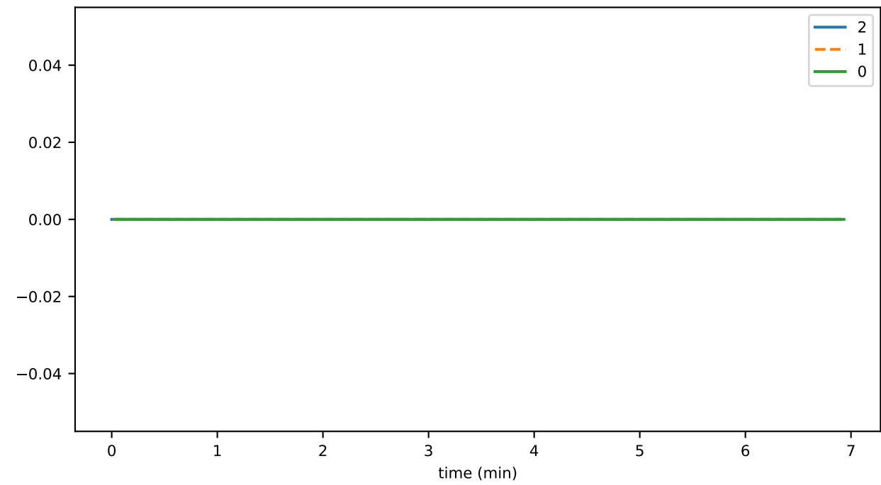
historyProofKeyPublicationDurationAvg
