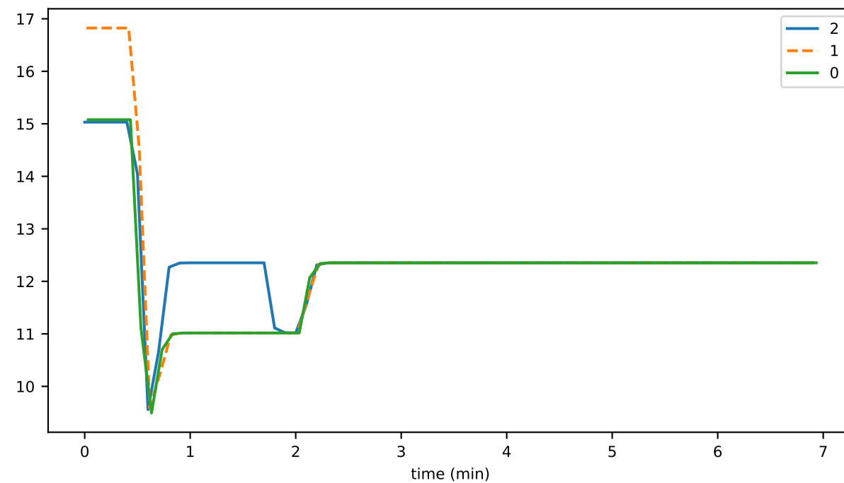
numEventsAddedUntilConsensus
