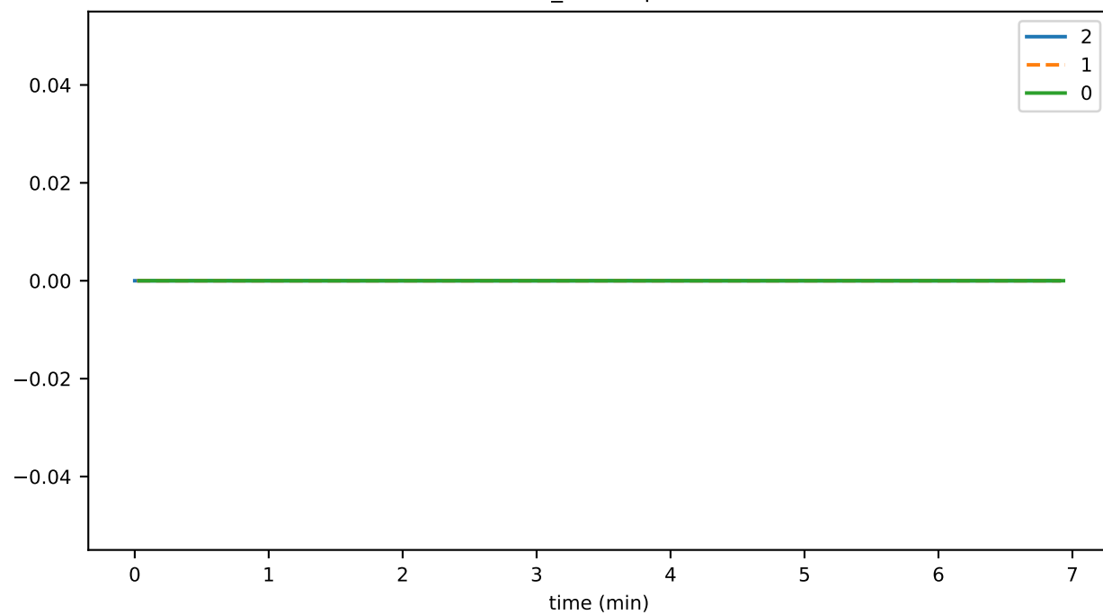
conn_opened
