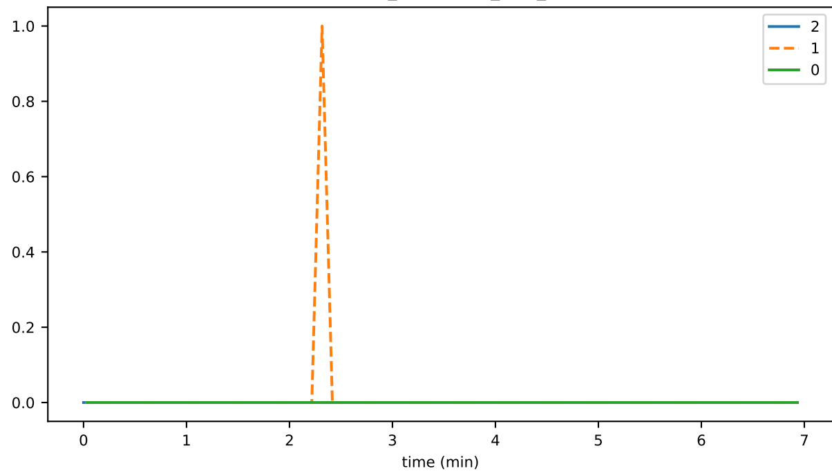
StateSigner_unhandled_task_count
