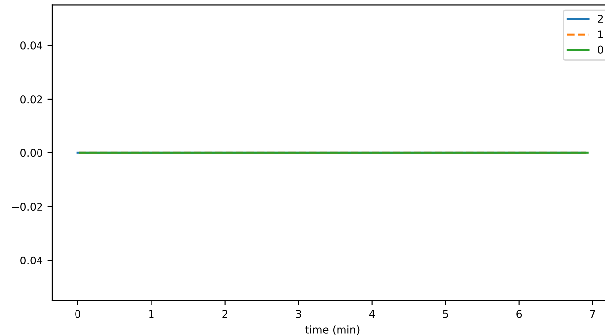
ds_compactions_level_7_leavesSavedSpaceMb_state
