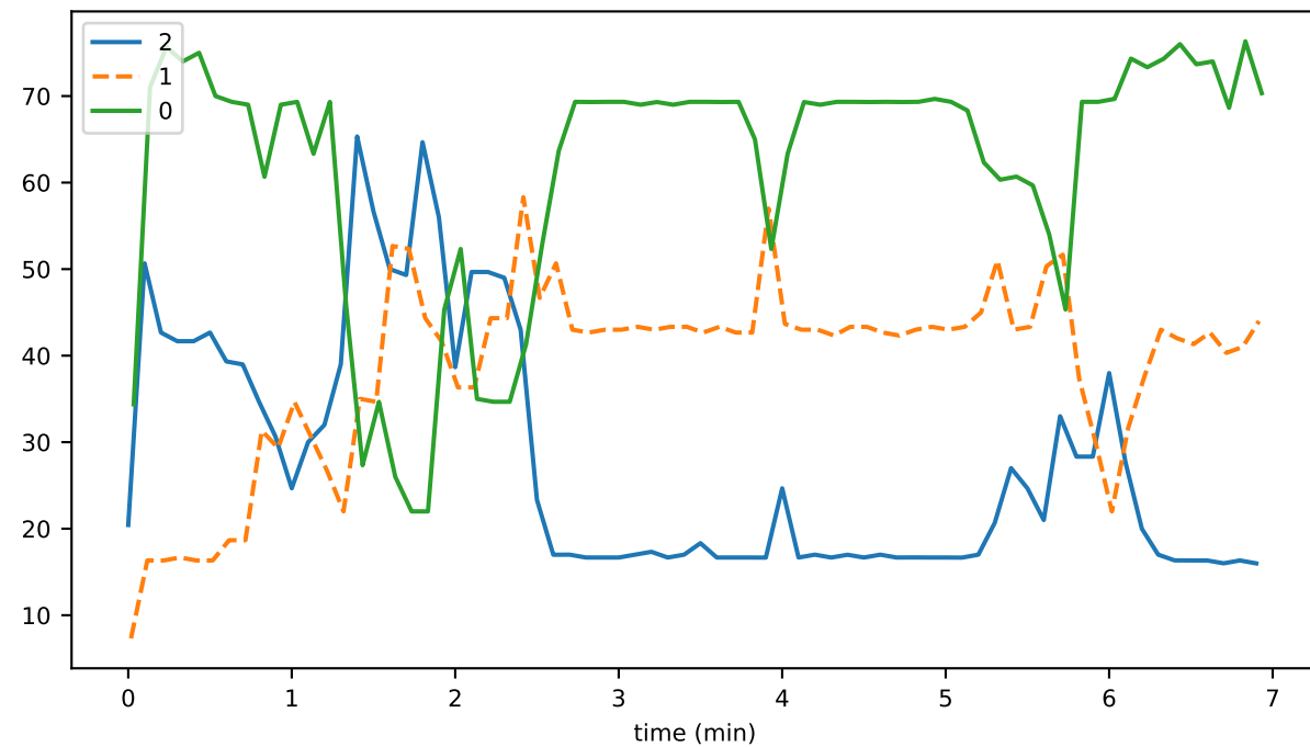
doNotSyncRemoteProcessingEvents
