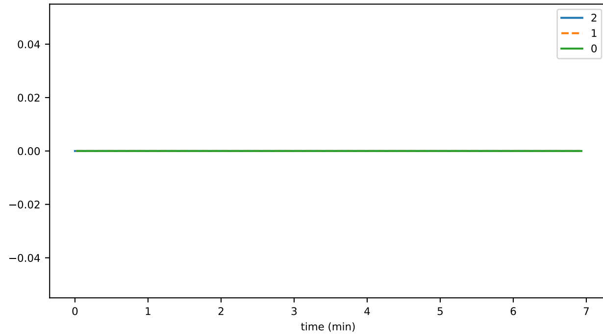
ds_compactions_level_3_leafKeysTimeMs_state
