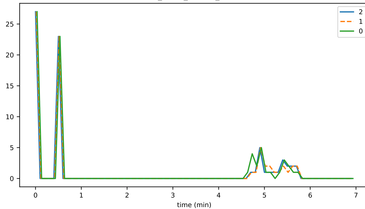
ds_reads_leaves_state
