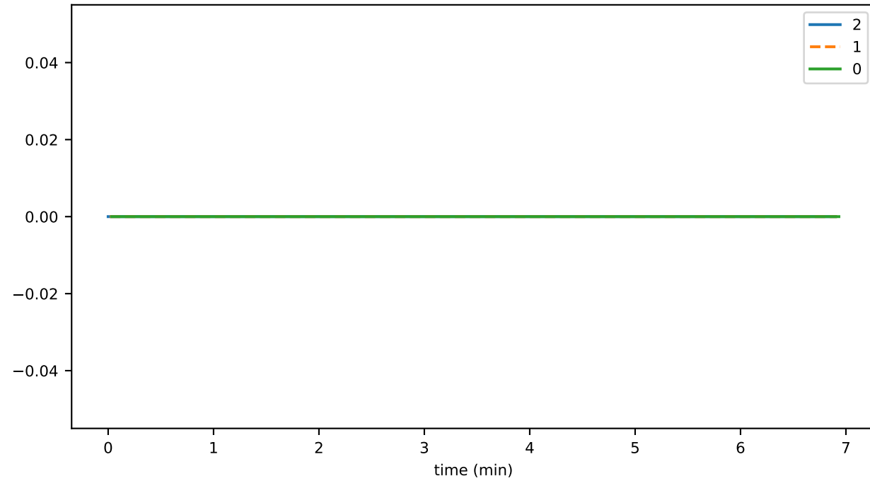
ds_compactions_level_3_leafKeysTimeMs_state
