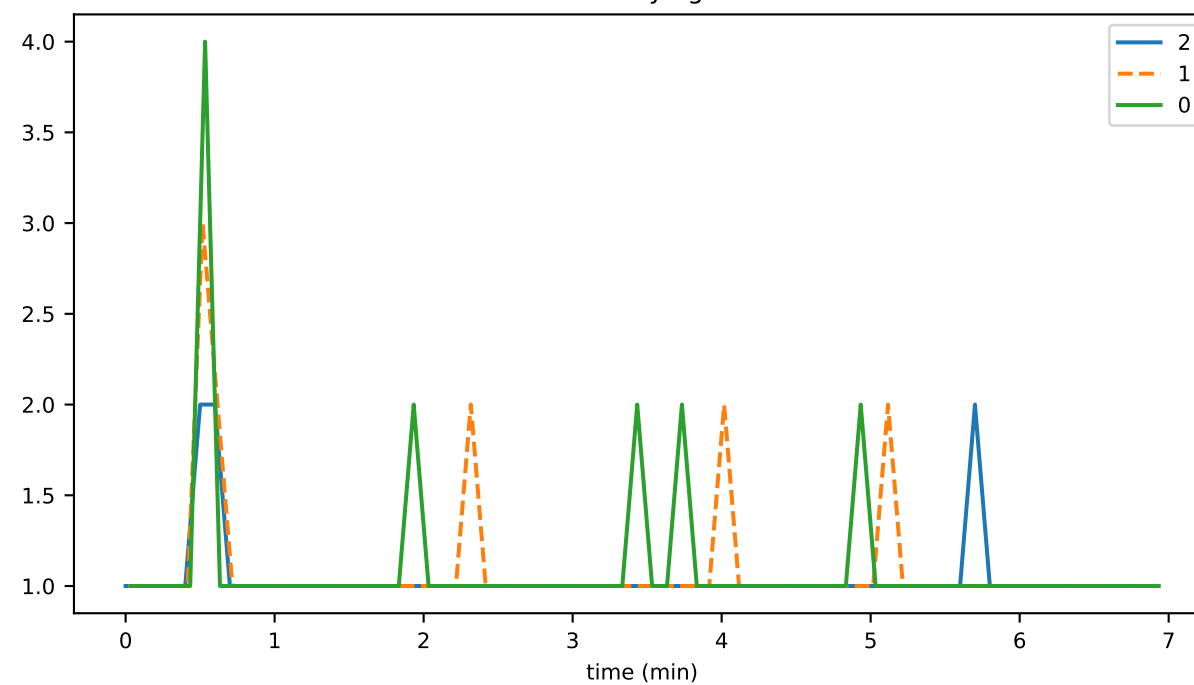
countInMemorySignedState
