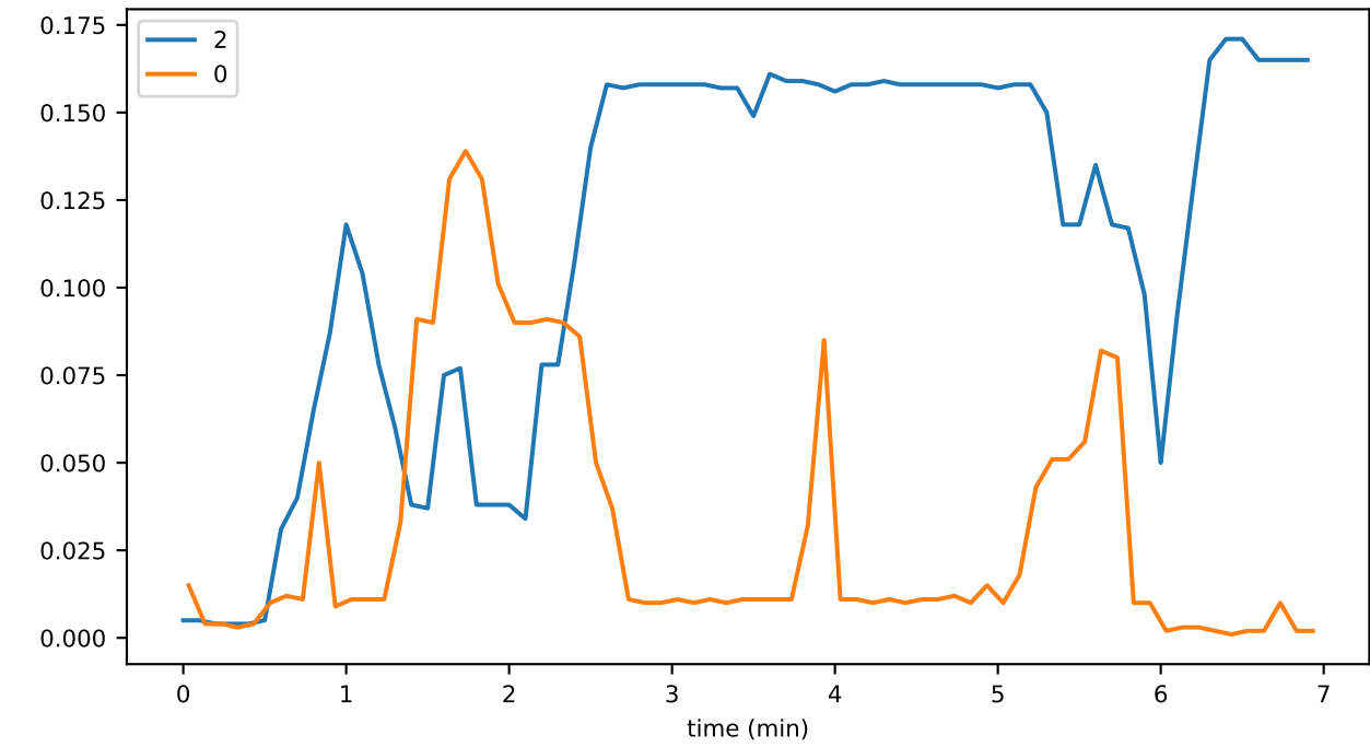
sync_phase_01_fraction_EXCHANGING_WINDOWS
