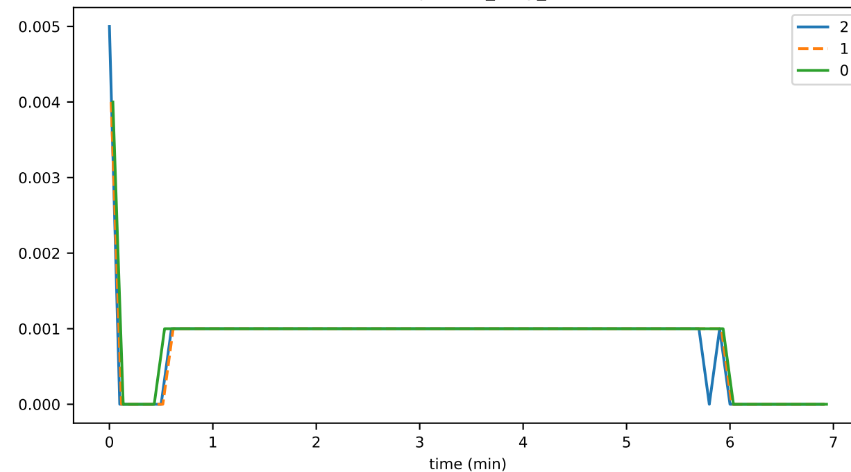
eventDelay_1_eventCreation_runtime
