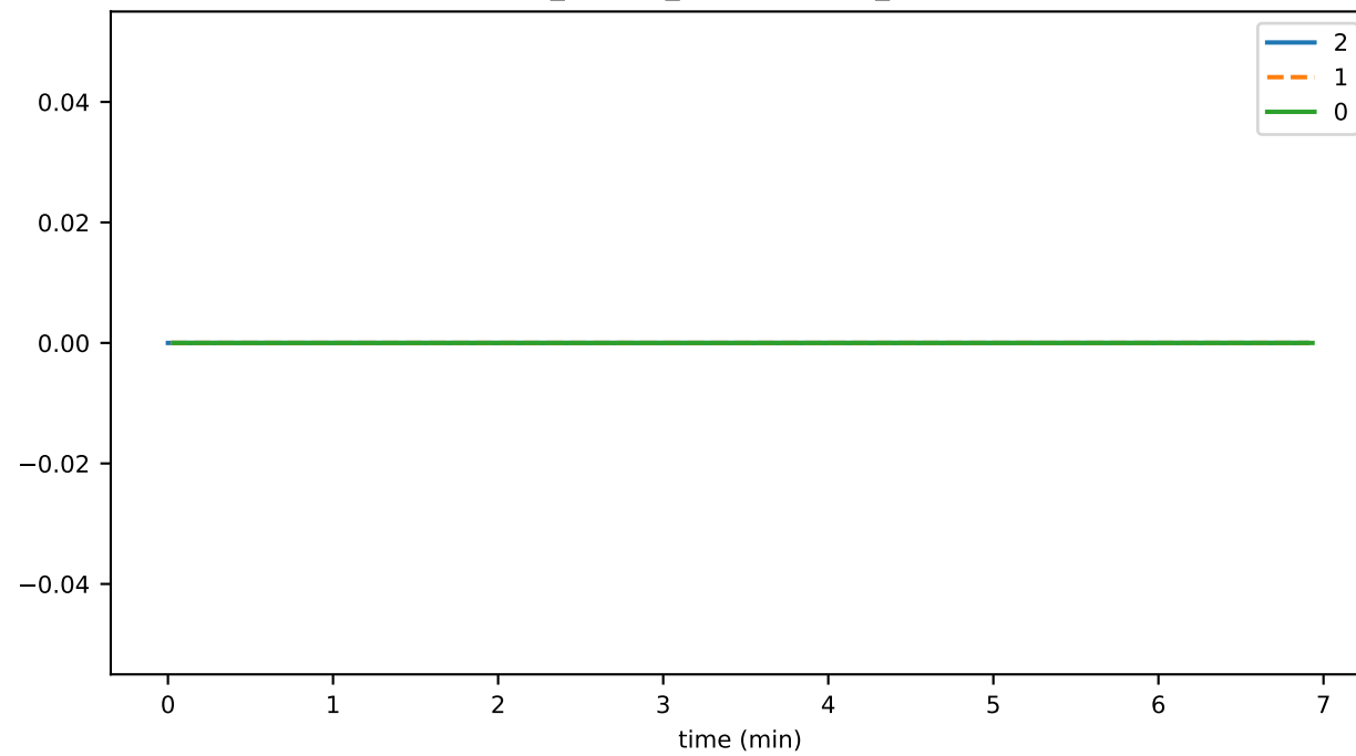
ds_flushes_leavesWritten_state
