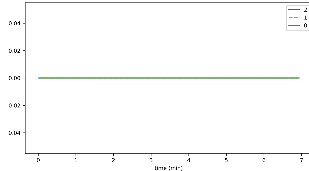
reconnectRejections_per_sec_00
