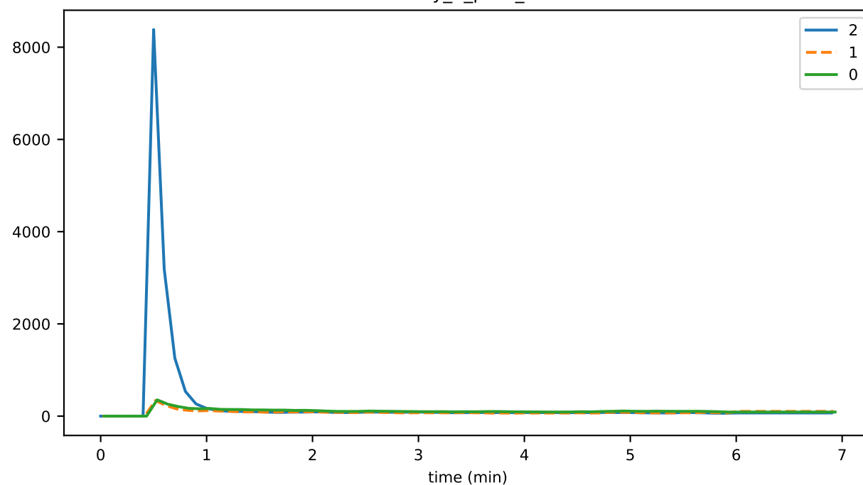
eventDelay_6_pces_runtime
