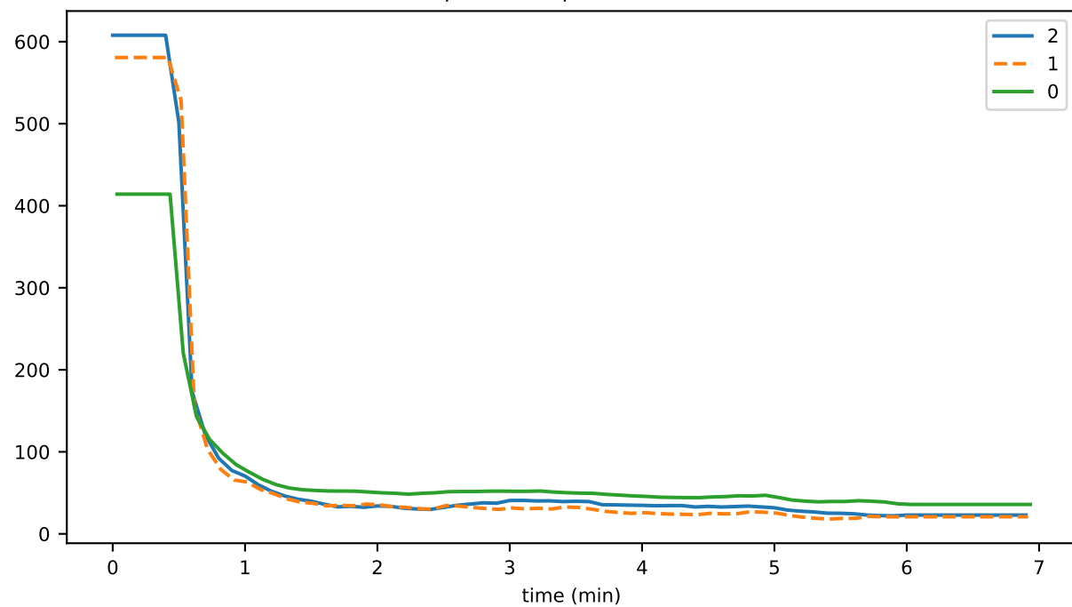
uptimeComputationTime
