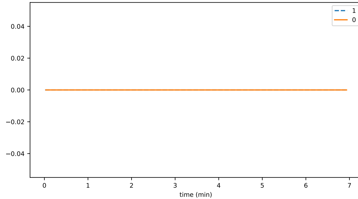
sync_phase_02_fraction_OTHER_FALLEN_BEHIND
