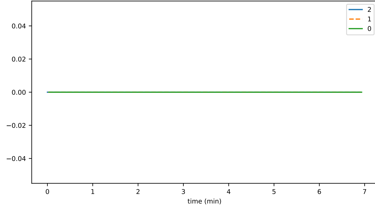
connSend_failure
