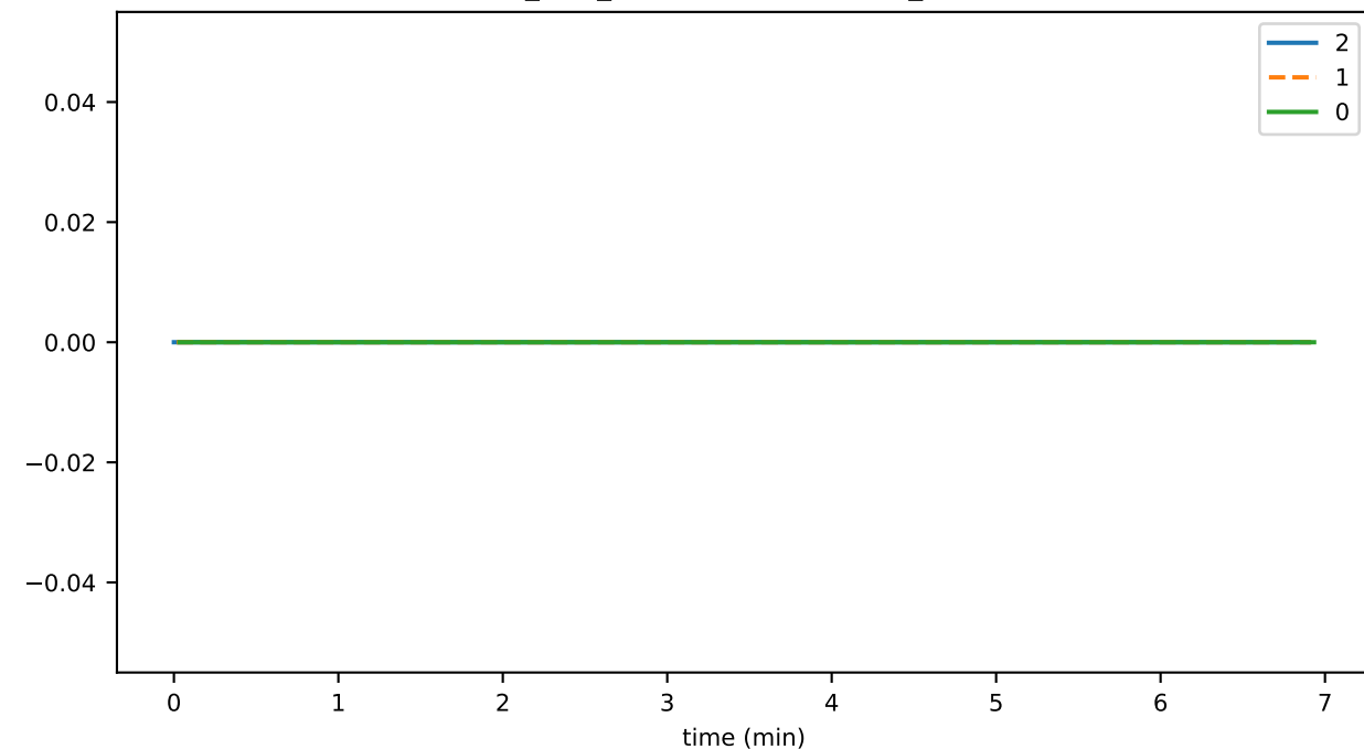
ds_files_level_0_hashesFileSizeByLevelMb_state
