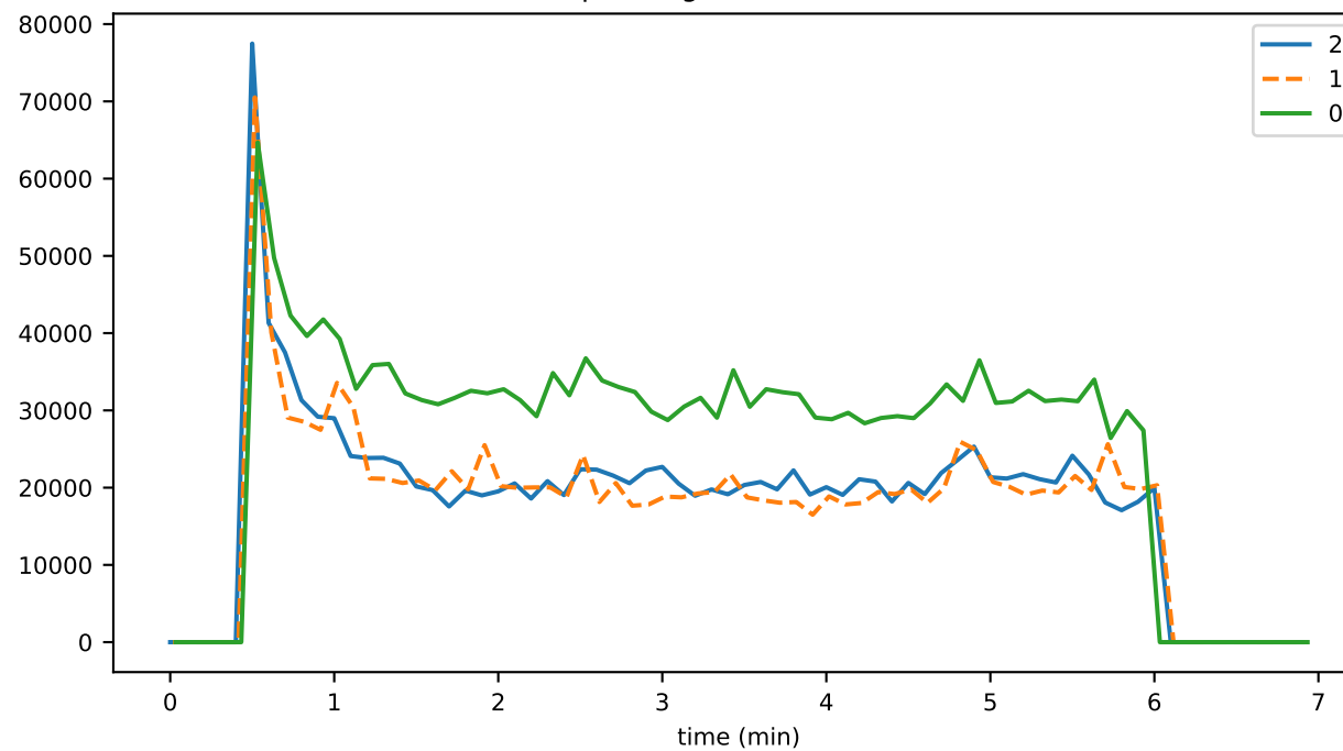
pcesAvgWriteDuration
