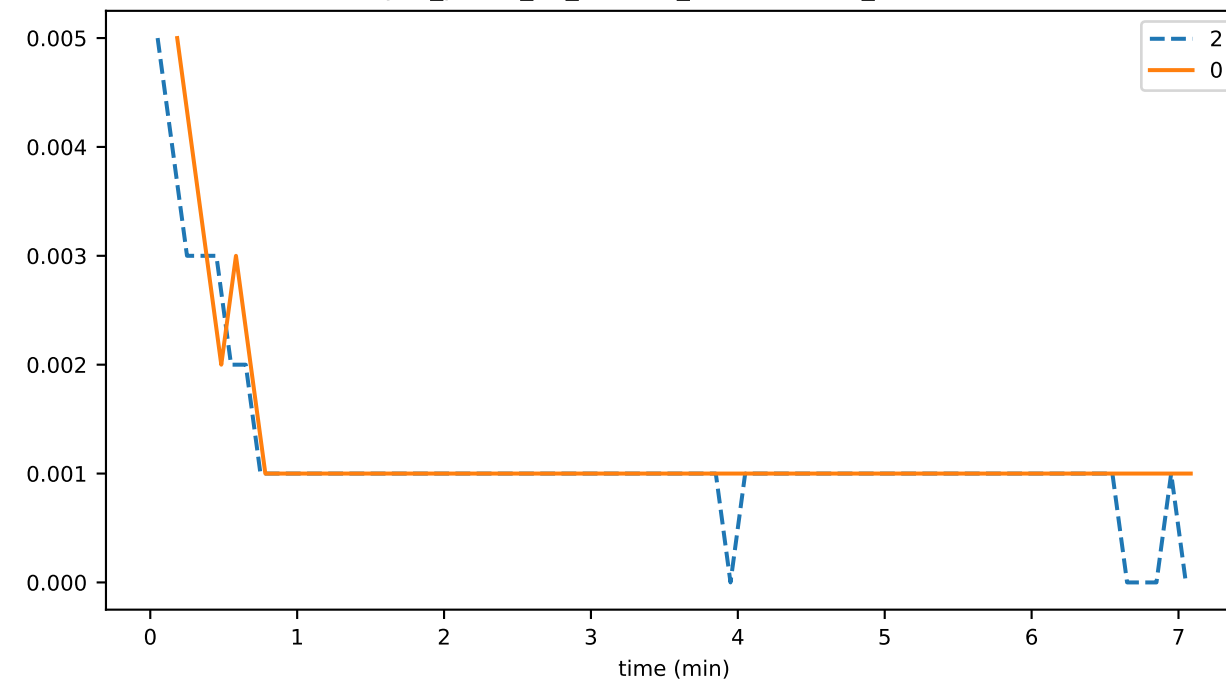
sync_phase_01_fraction_EXCHANGING_WINDOWS
