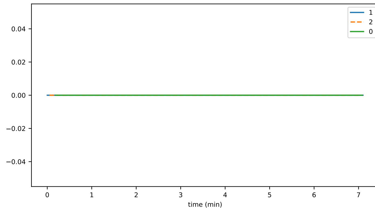
contractCallLocalDurationMax
