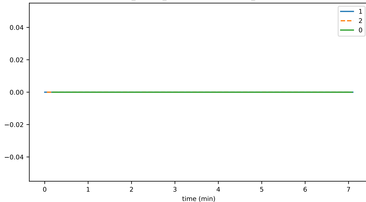
ds_flushes_leavesStoreFileSizeMb_state
