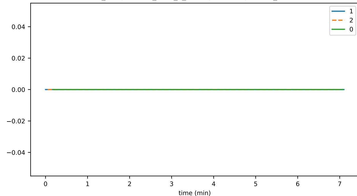
ds_compactions_level_1_leavesSavedSpaceMb_state
