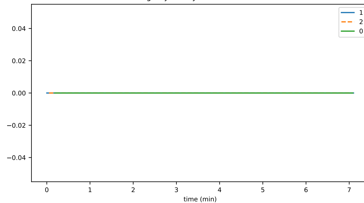
getBySolvencyIDDurationMax
