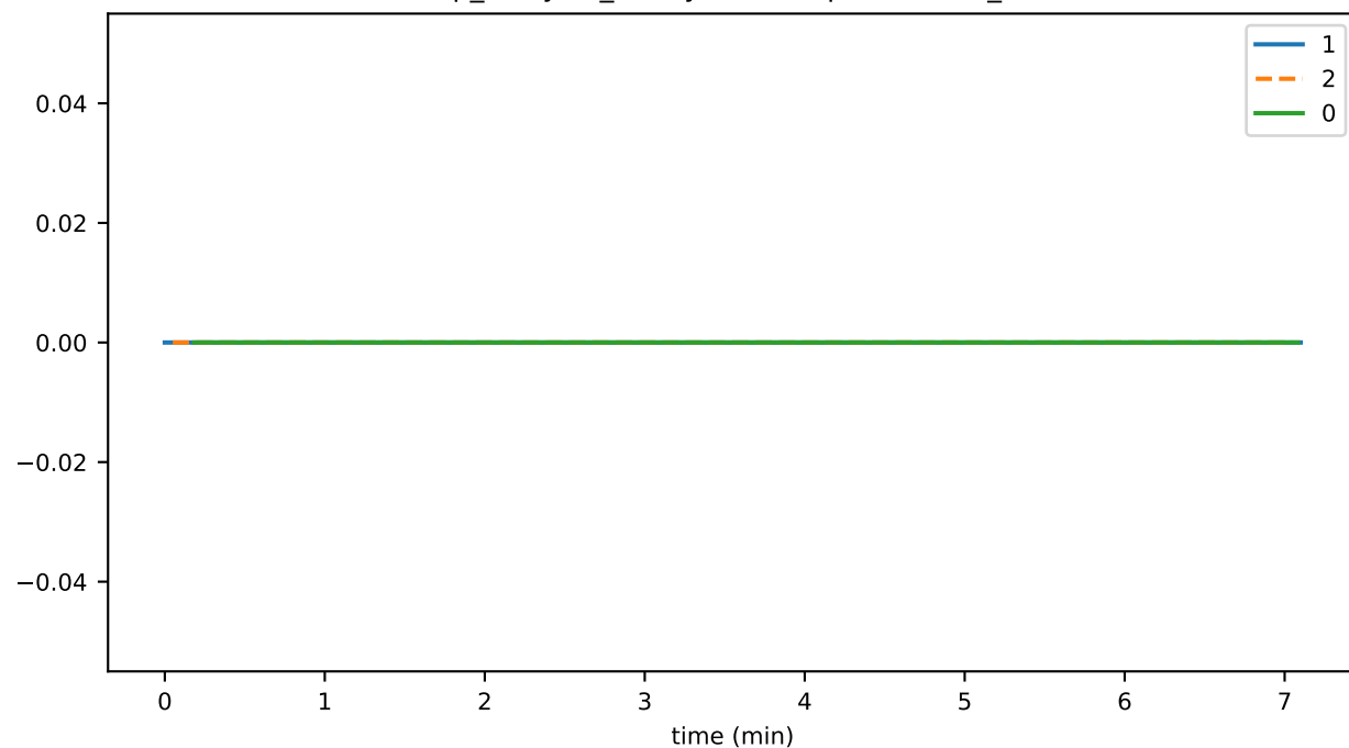
vmap_lifecycle_familySizeBackpressureMs_state
