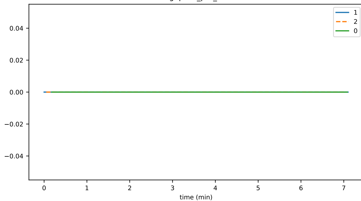
SigSpans_per_sec
