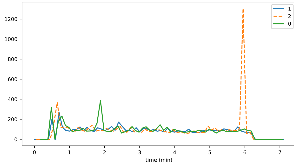
eventDelay_1_hashing_gossipMAX
