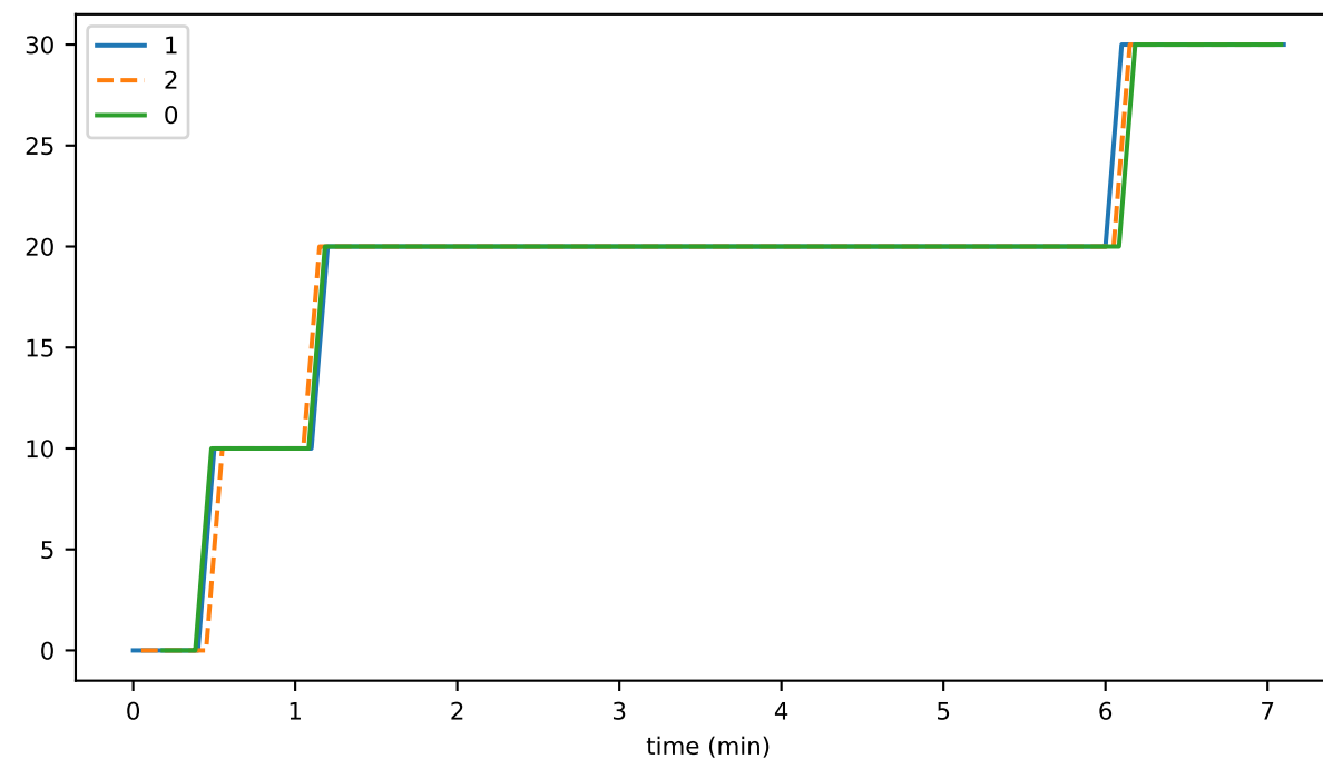
disconnects_per_sec_00
