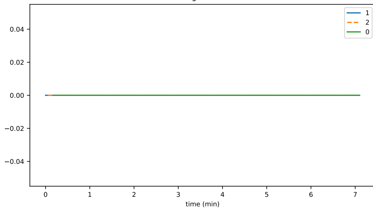
scheduleSignThrottledTxns
