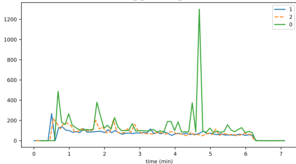
eventDelay_4_verification_storageMAX
