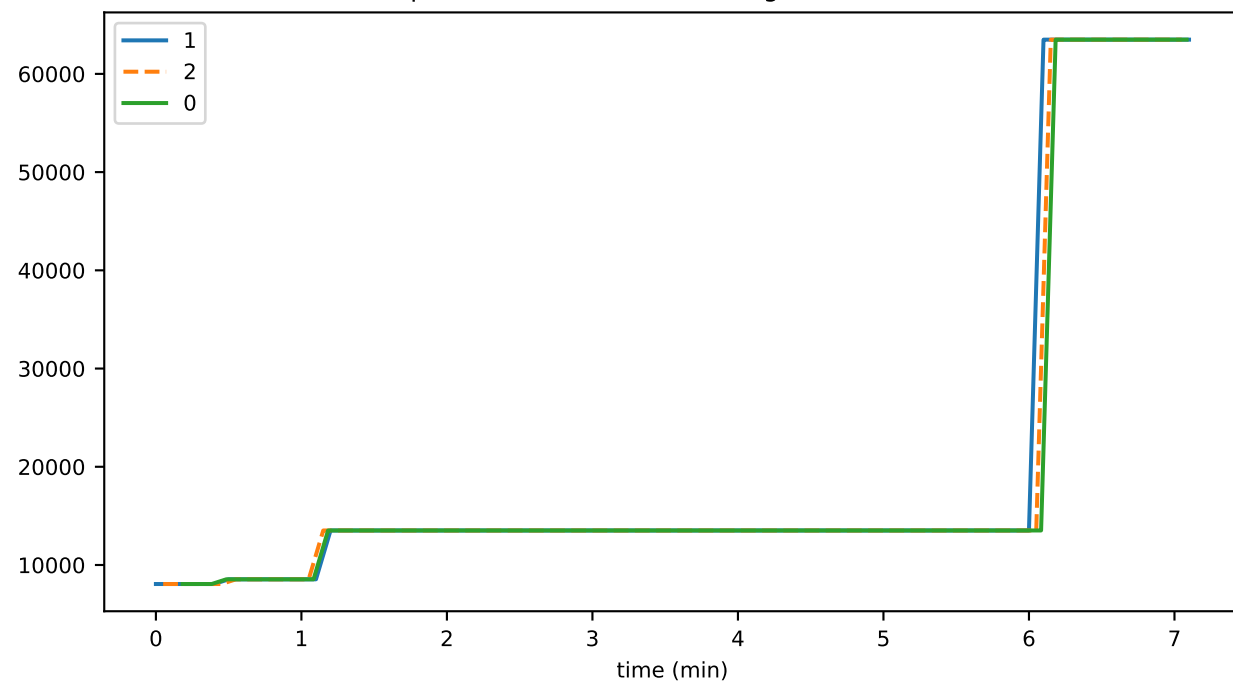
preconsensusEventFileYoungestIdentifier
