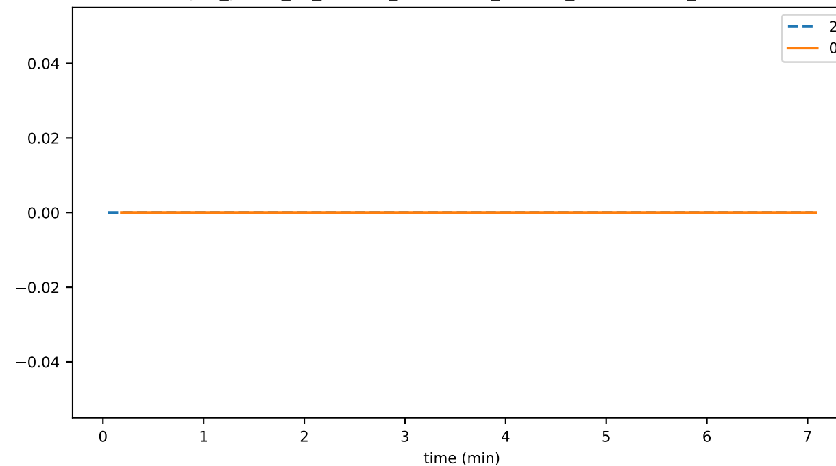
sync_phase_01_fraction_SELF_FALLEN_BEHIND
