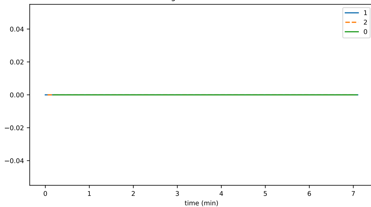
SigIntakePulseTime
