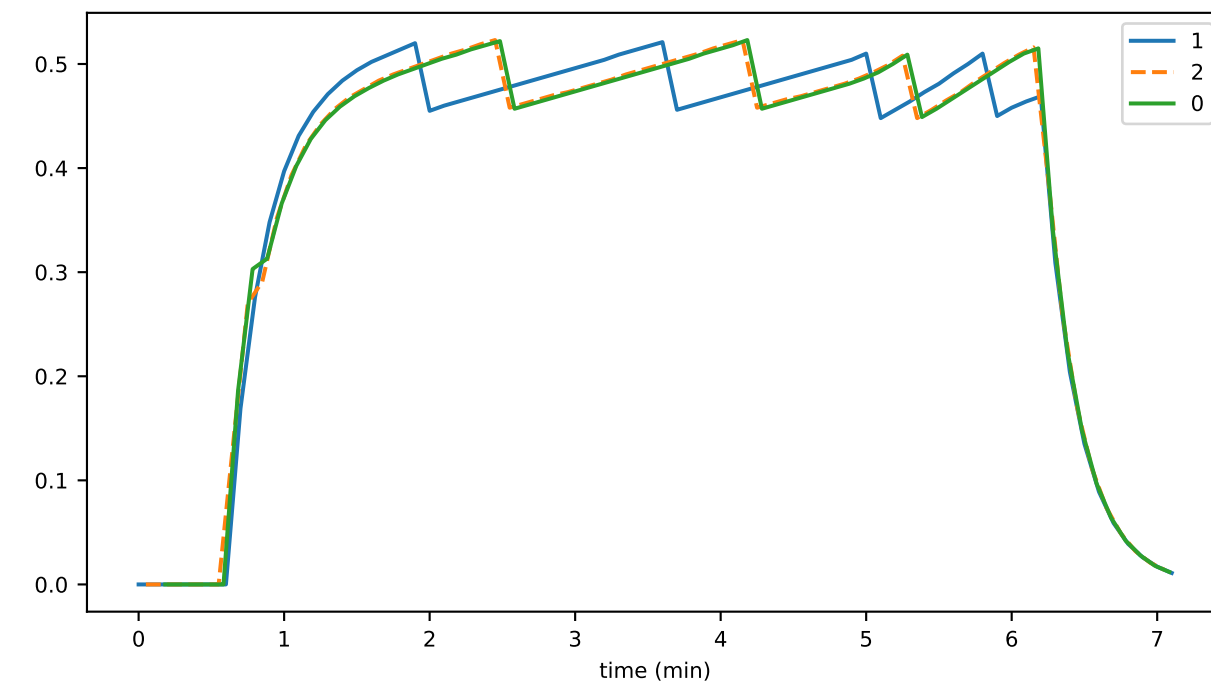
sync_per_secC
