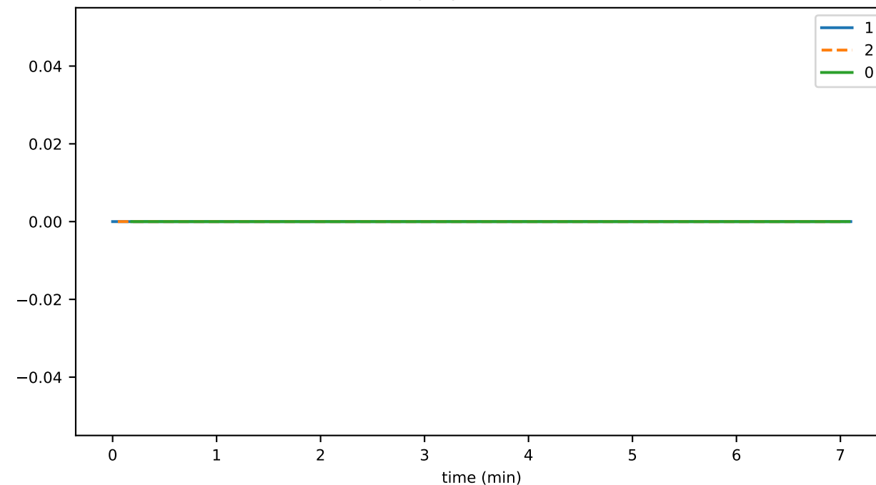
getBySolvencyIDDurationMax
