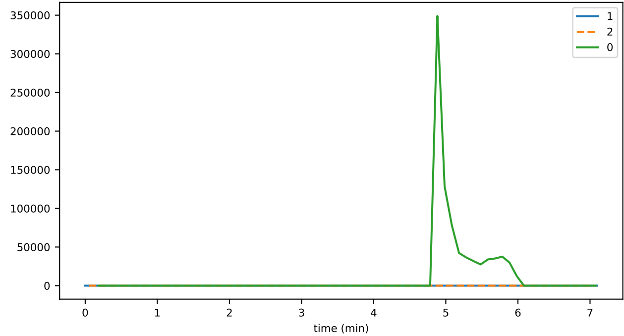
transactionGetReceiptThrottledTxns
