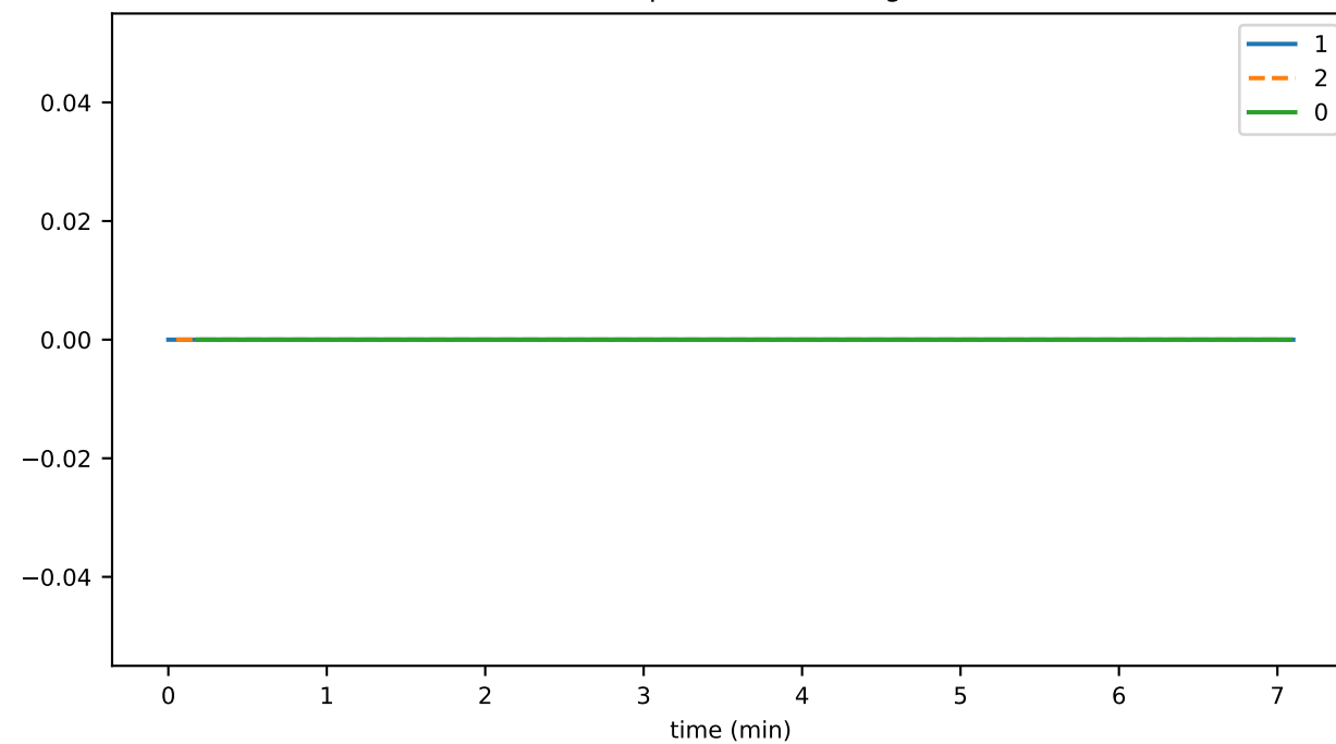
nodeUpdateDurationAvg
