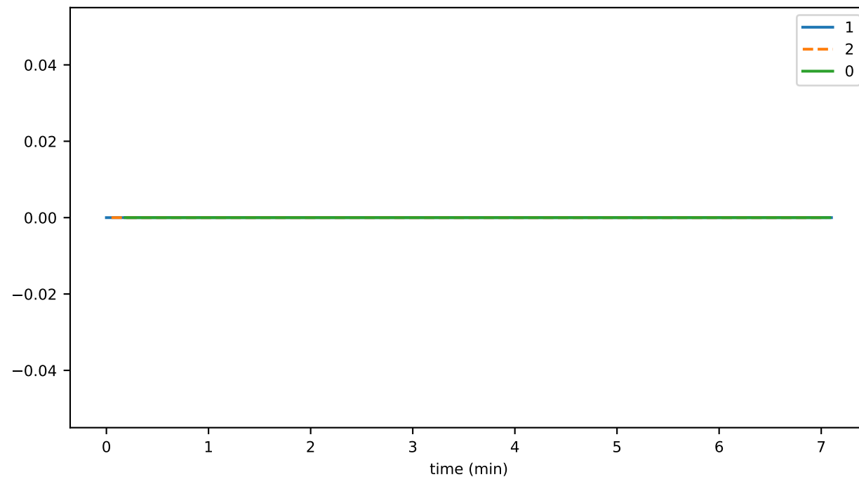
fileAppendDurationAvg
