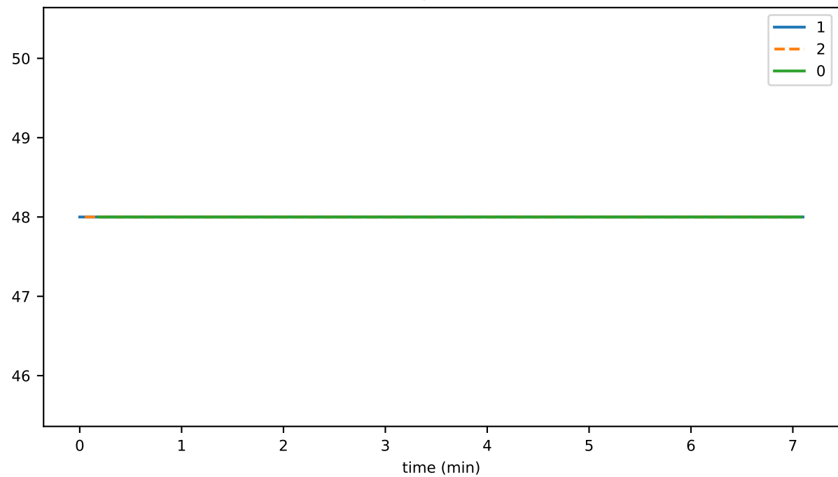
receiverReconnectDurationSeconds
