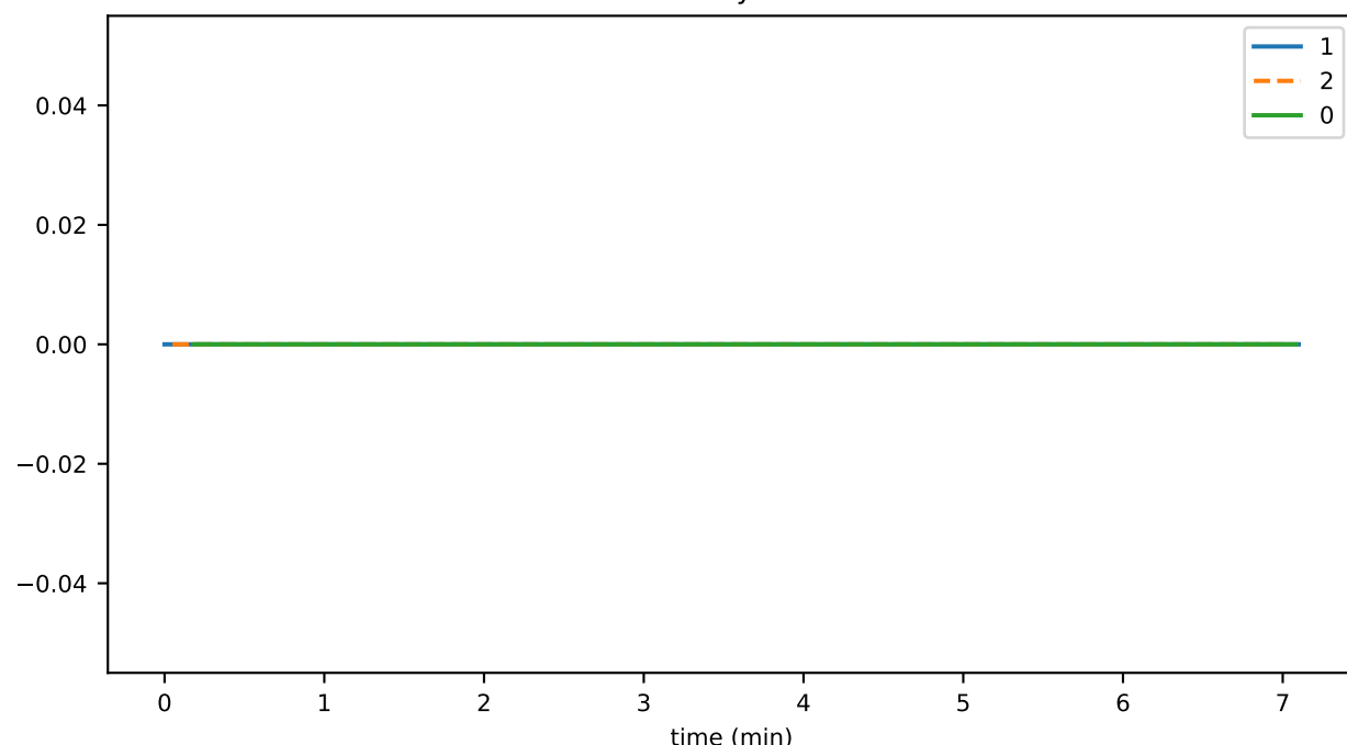
bufferedPriorityTransactions
