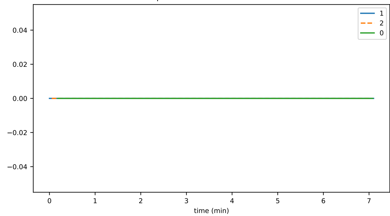
parentBirthRoundMismatch
