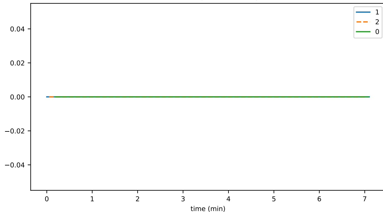
scheduleSignThrottledTxns
