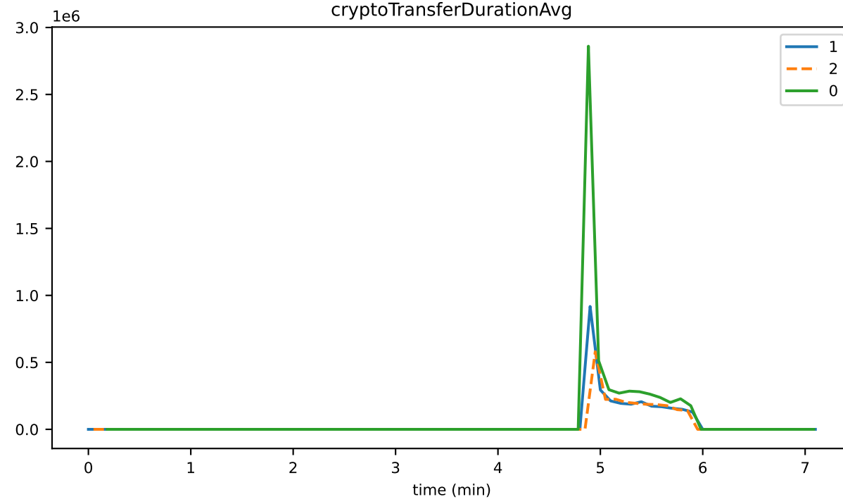
cryptoTransferDurationAvg
