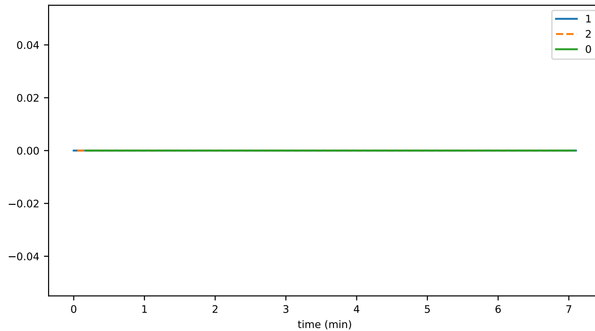
startsReconnectAsSender
