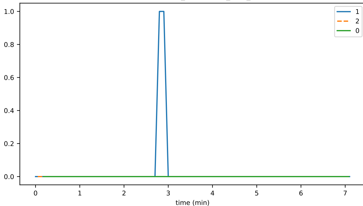
ConsensusEngine_unhandled_task_count
