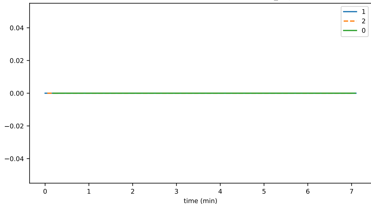
SmartContractService:TransactionGasUsed_sum
