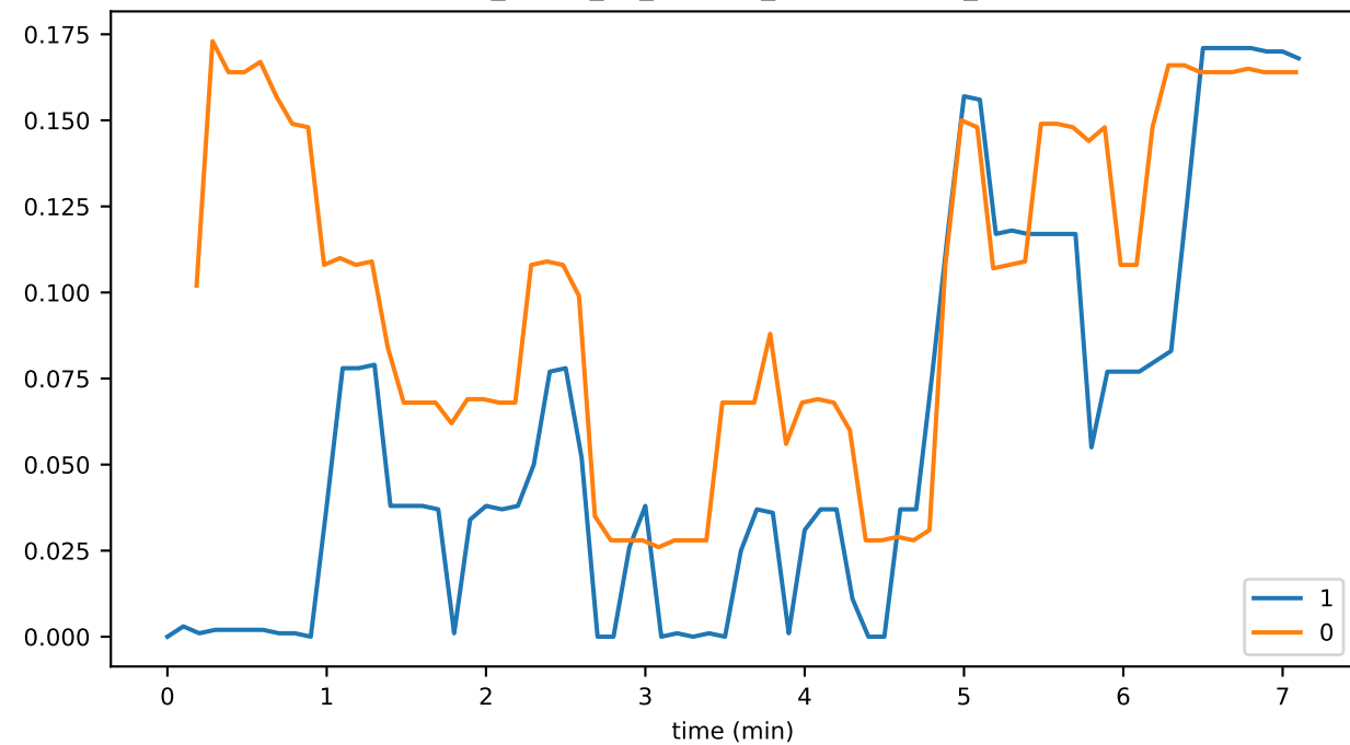
sync_phase_02_fraction_EXCHANGING_TIPS
