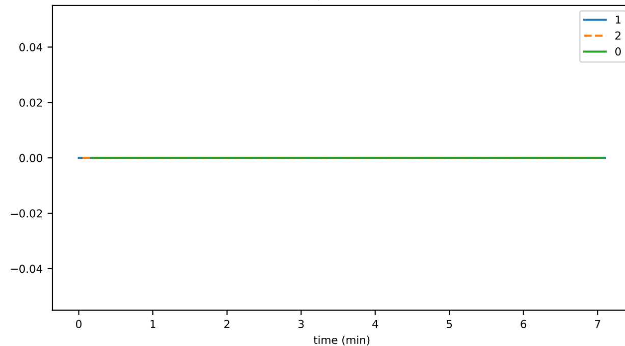
contractGetInfoDurationAvg
