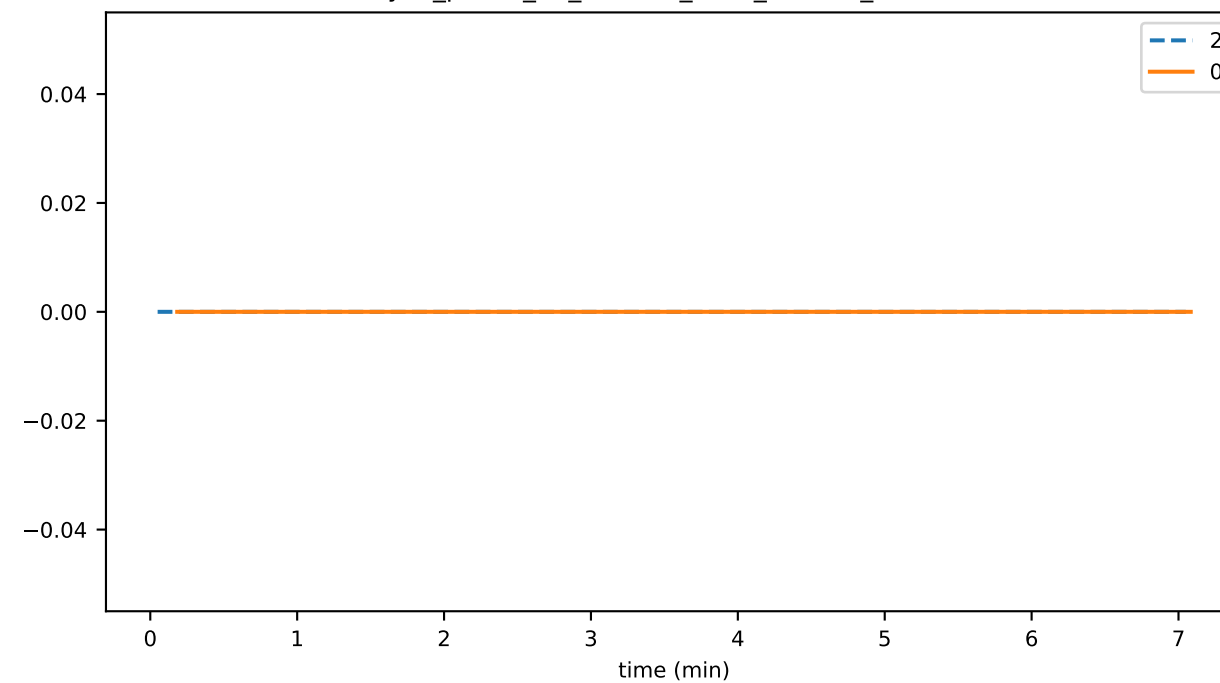
sync_phase_01_fraction_SELF_FALLEN_BEHIND
