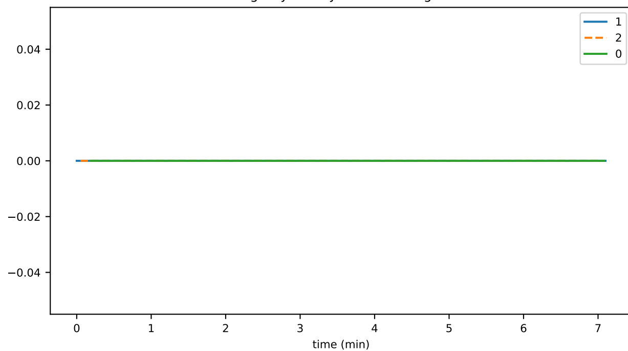
getBySolvencyIDDurationAvg
