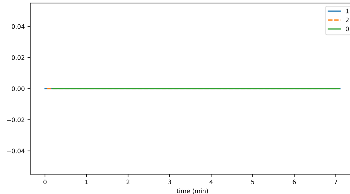
getByKeyDurationAvg
