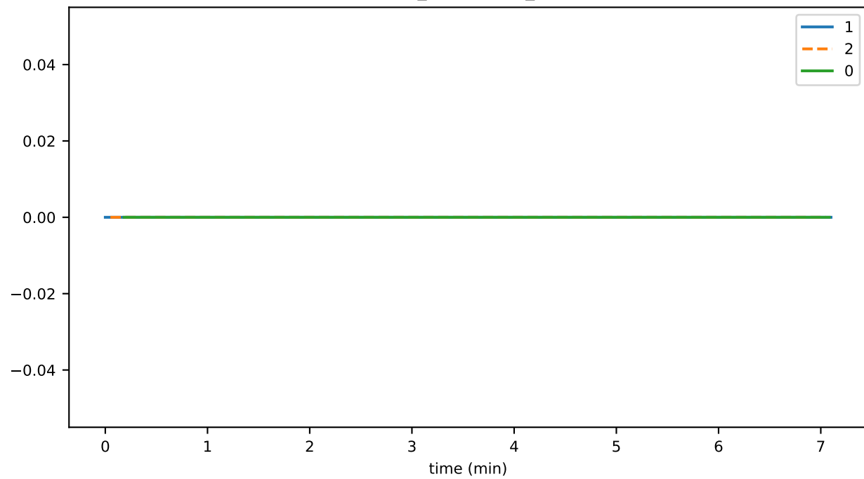
connRecv_endStream_success
