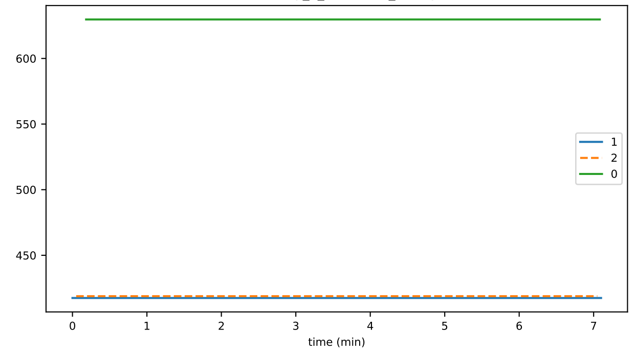
eventDelay_3_deduplication_gossip
