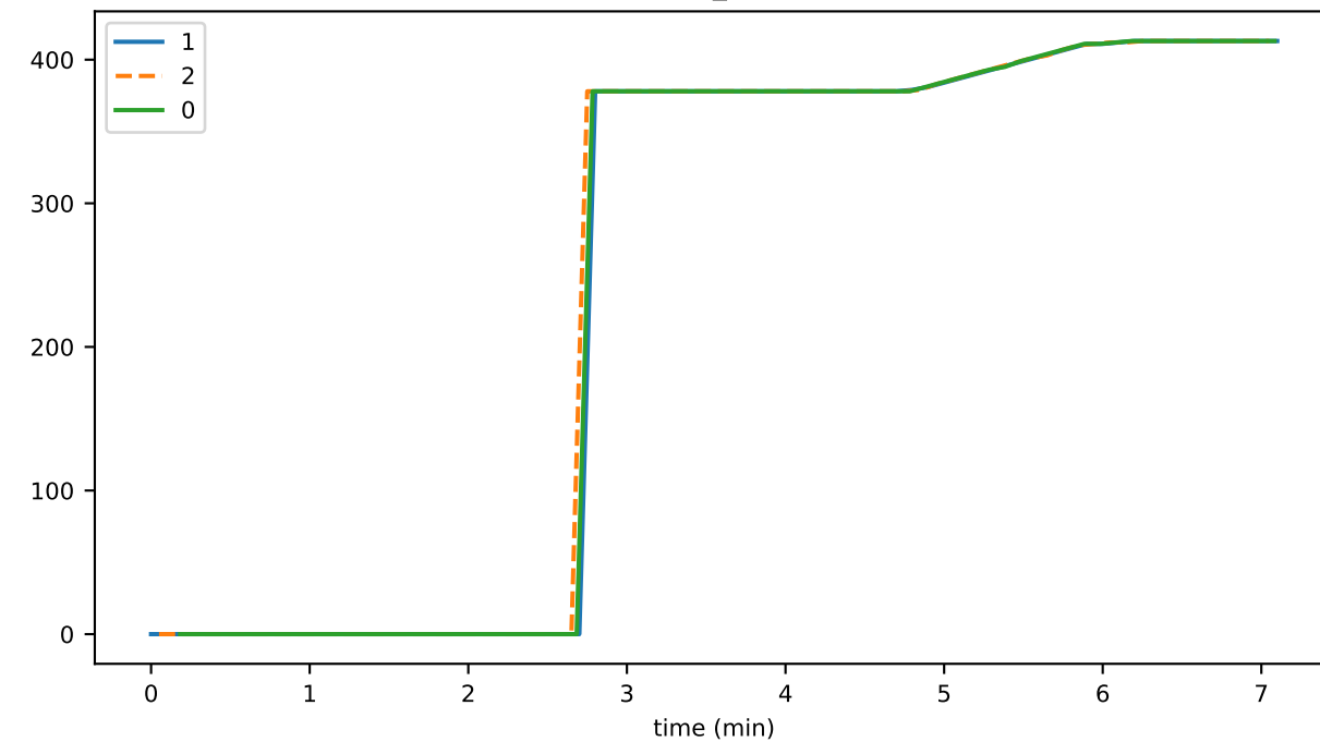
recordHashes_highestBlock
