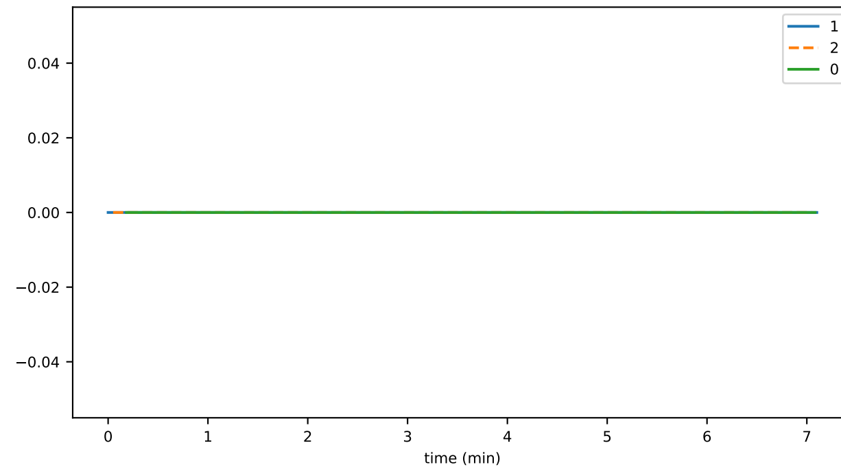
filesPercentUsed
