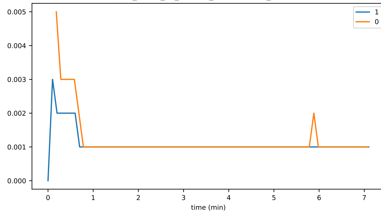
sync_phase_02_fraction_EXCHANGING_WINDOWS
