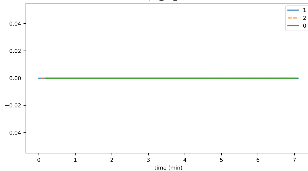
sync_per_secC
