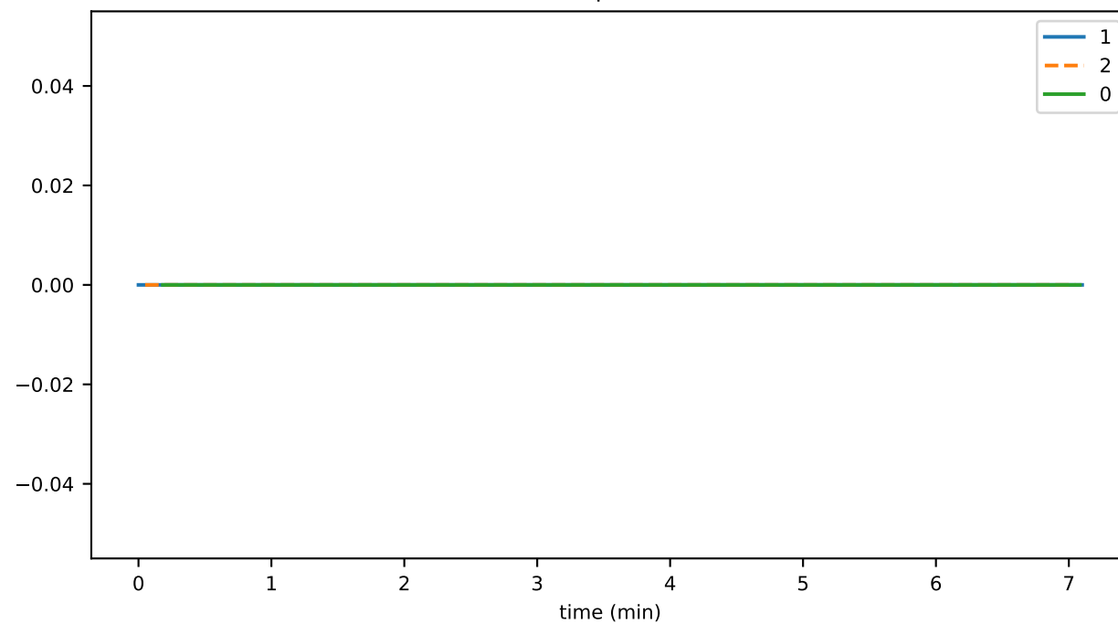
tokenAirdropDurationMax
