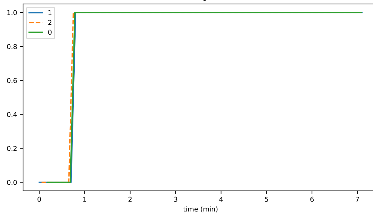
trans_per_event
