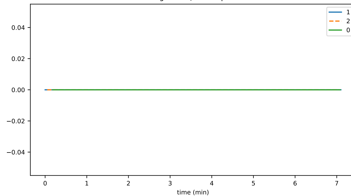
SigIntakeQueueDepth
