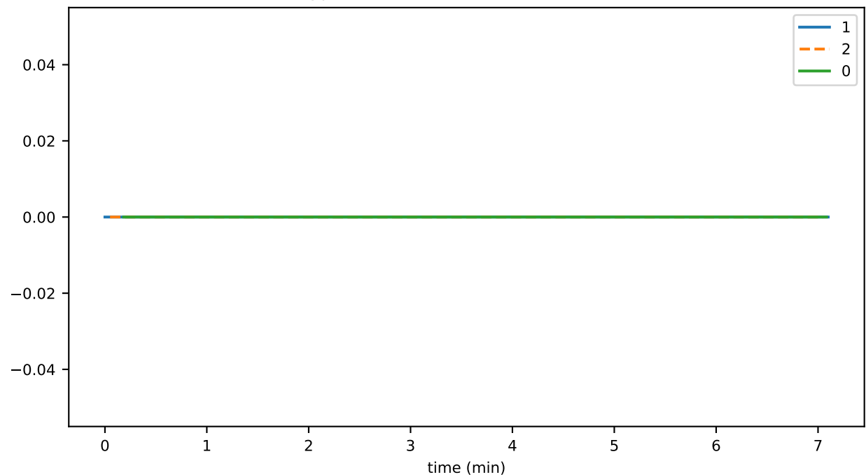
cryptoAddLiveHashDurationAvg
