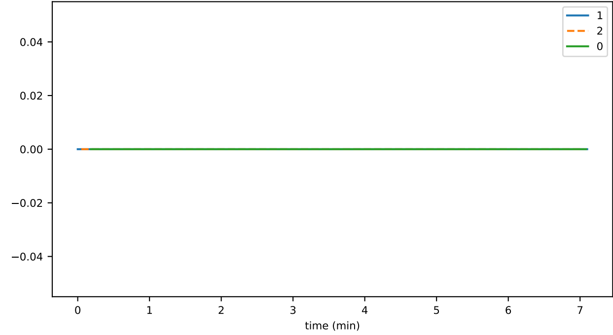
timeCreatedMismatch
