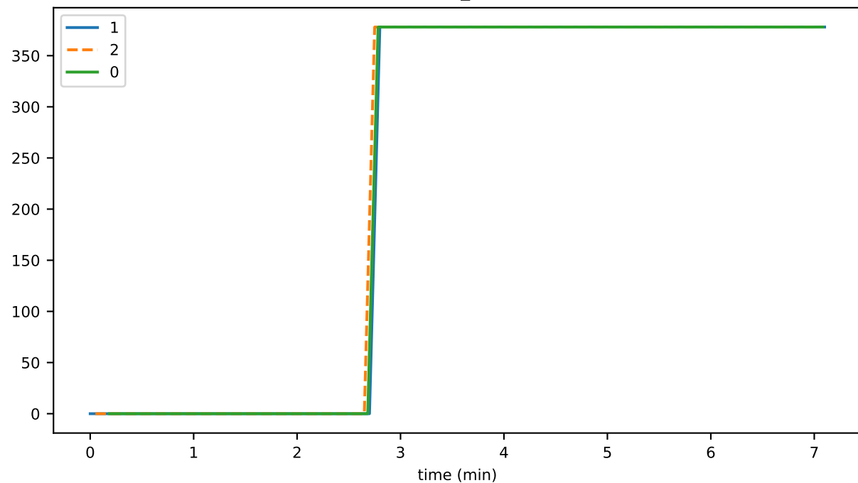
registeredNodeCreateDurationAvg
