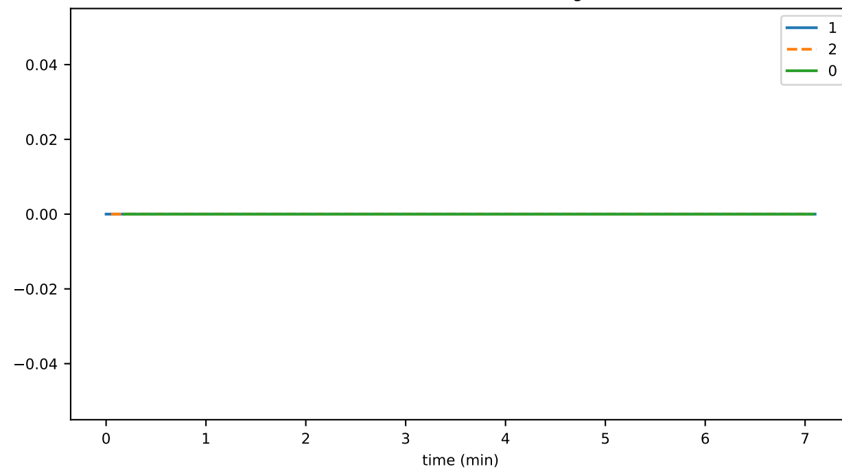
contractGetInfoDurationAvg
