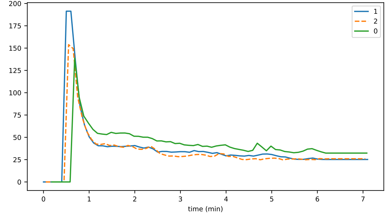
eventDelay_2_validation_runtime
