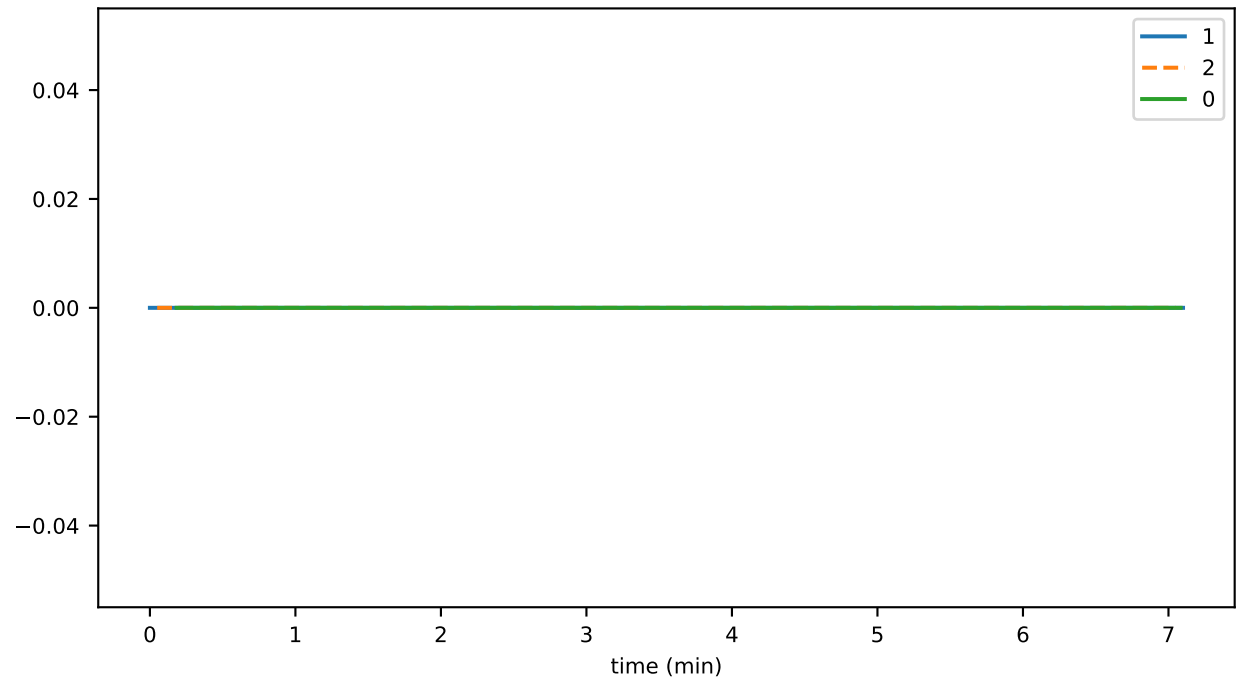
transactionGetReceiptThrottledTxns
