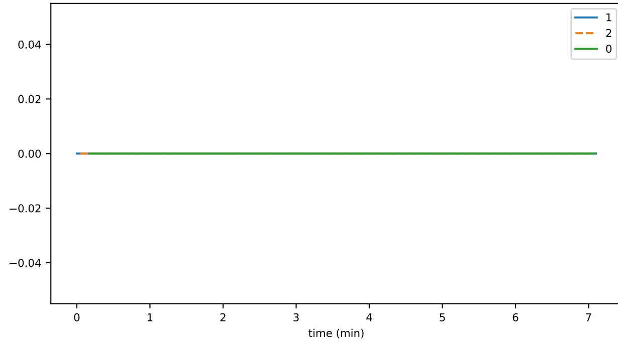
networkGetExecutionTimeThrottledTxns
