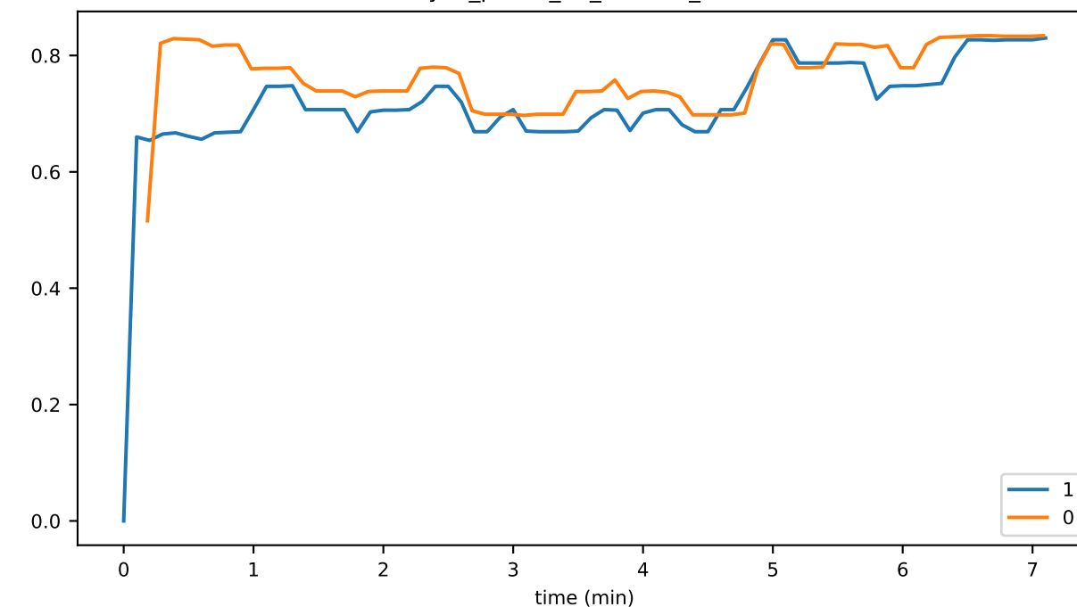
sync_phase_02_fraction_OTHER_FALLEN_BEHIND
