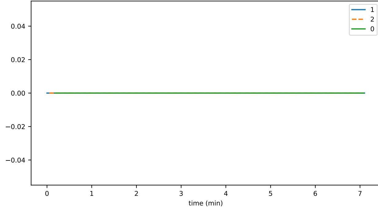
historyProofTransR2ToFailMs
