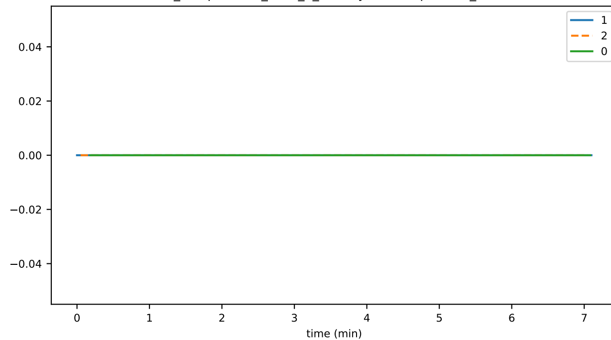
ds_compactions_level_8_leafKeysSavedSpaceMb_state
