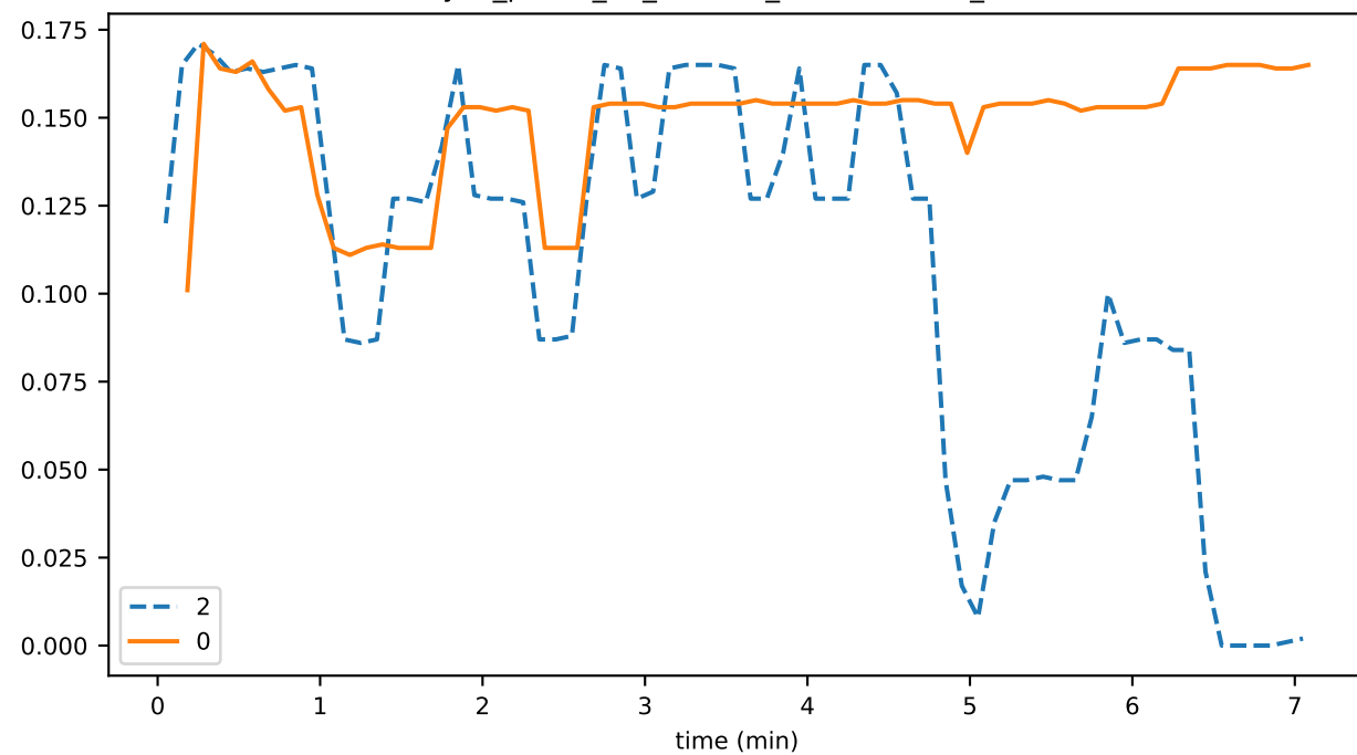
sync_phase_01_fraction_EXCHANGING_TIPS
