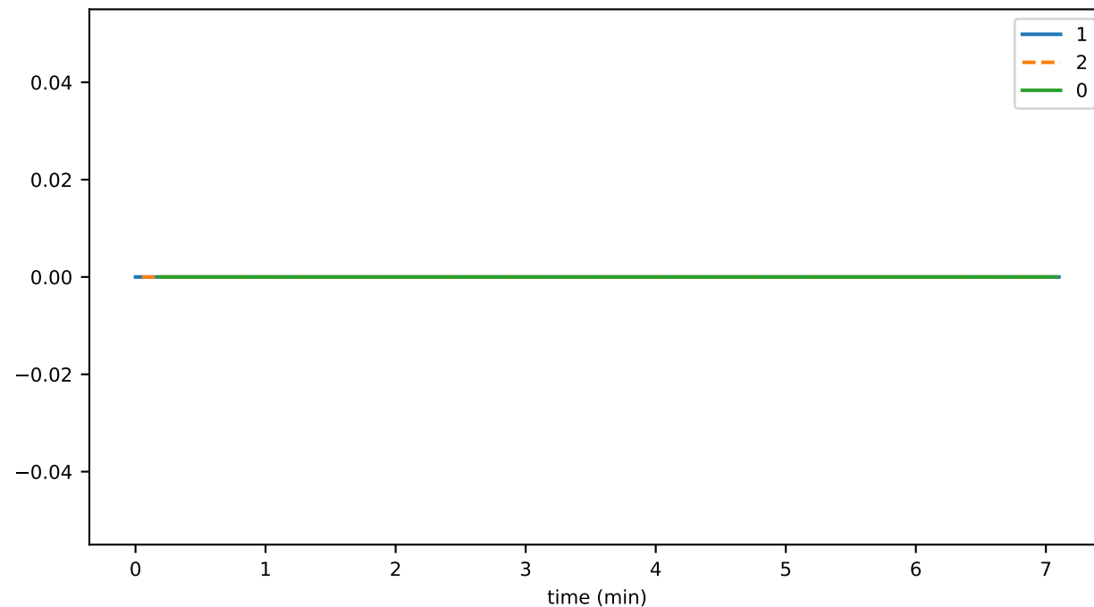
tokenRevokeKycFromAccountDurationAvg
