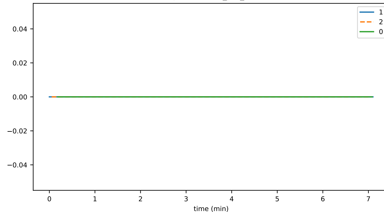
SigIntakeQueueDepth
