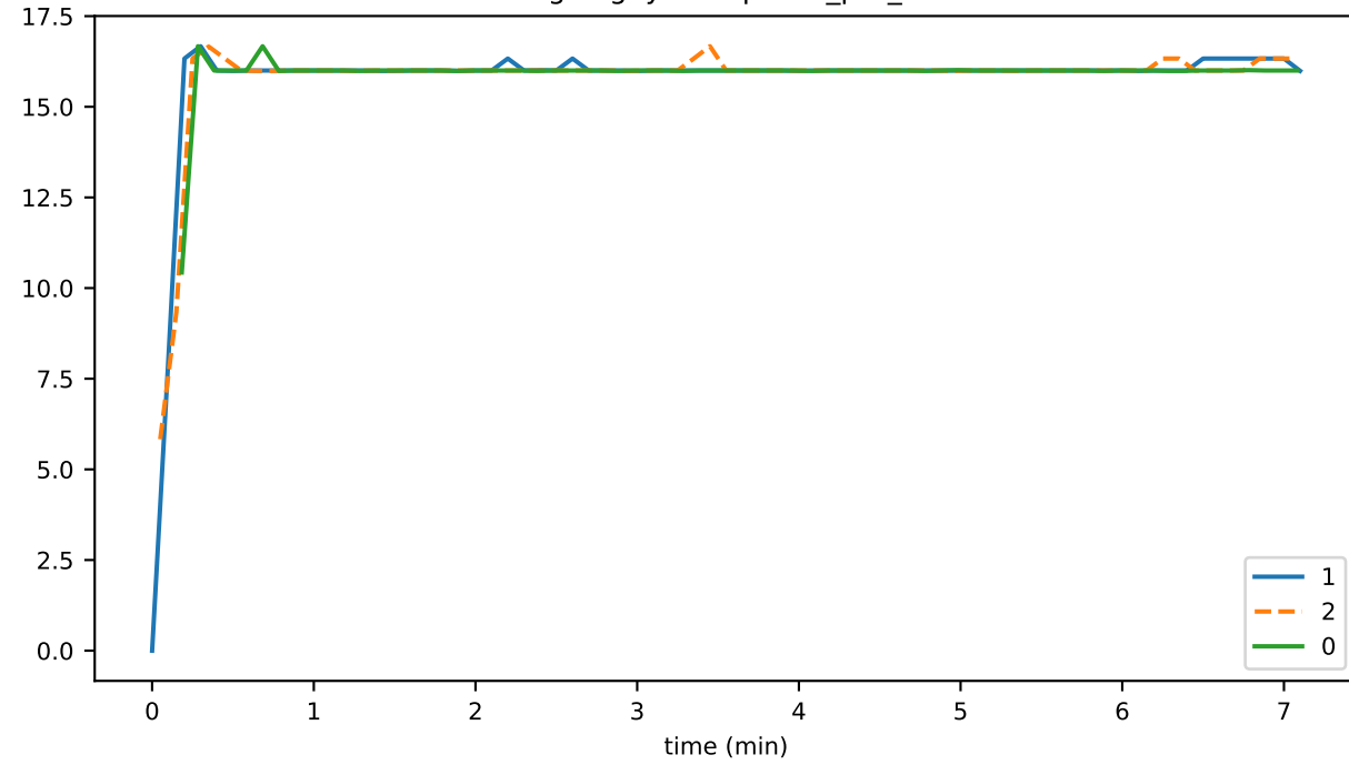
outgoingSyncRequests_per_sec
