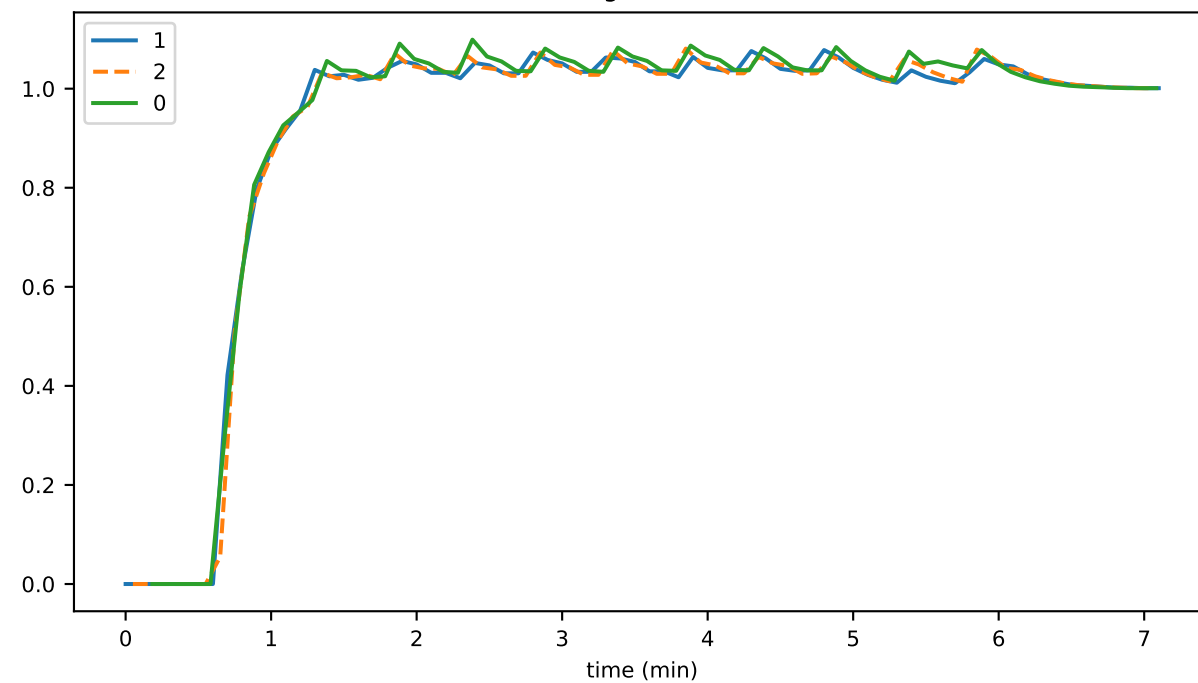
statesIneligibleForDeletion
