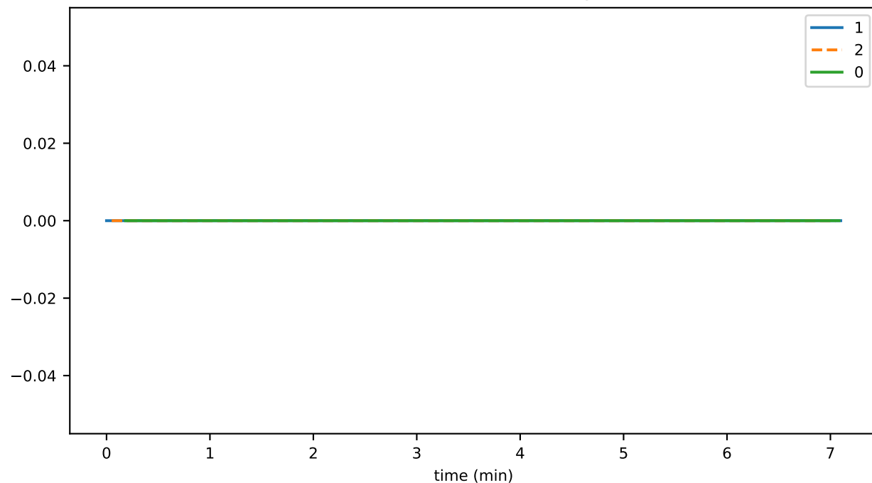
crsPublicationThrottledTxns
