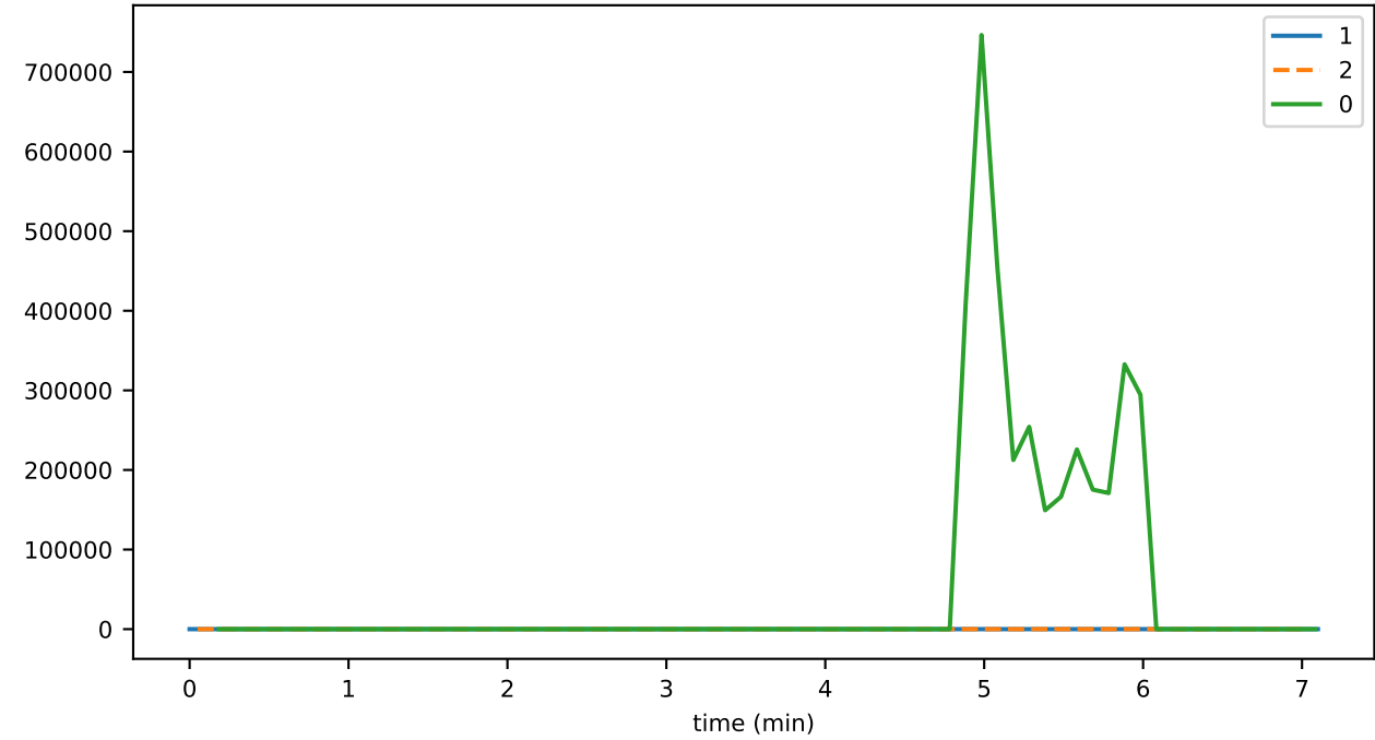
transactionGetRecordDurationAvg
