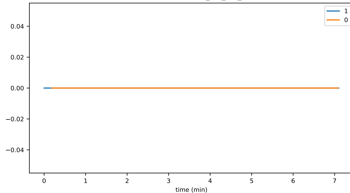
recordHashes_highestBlock
