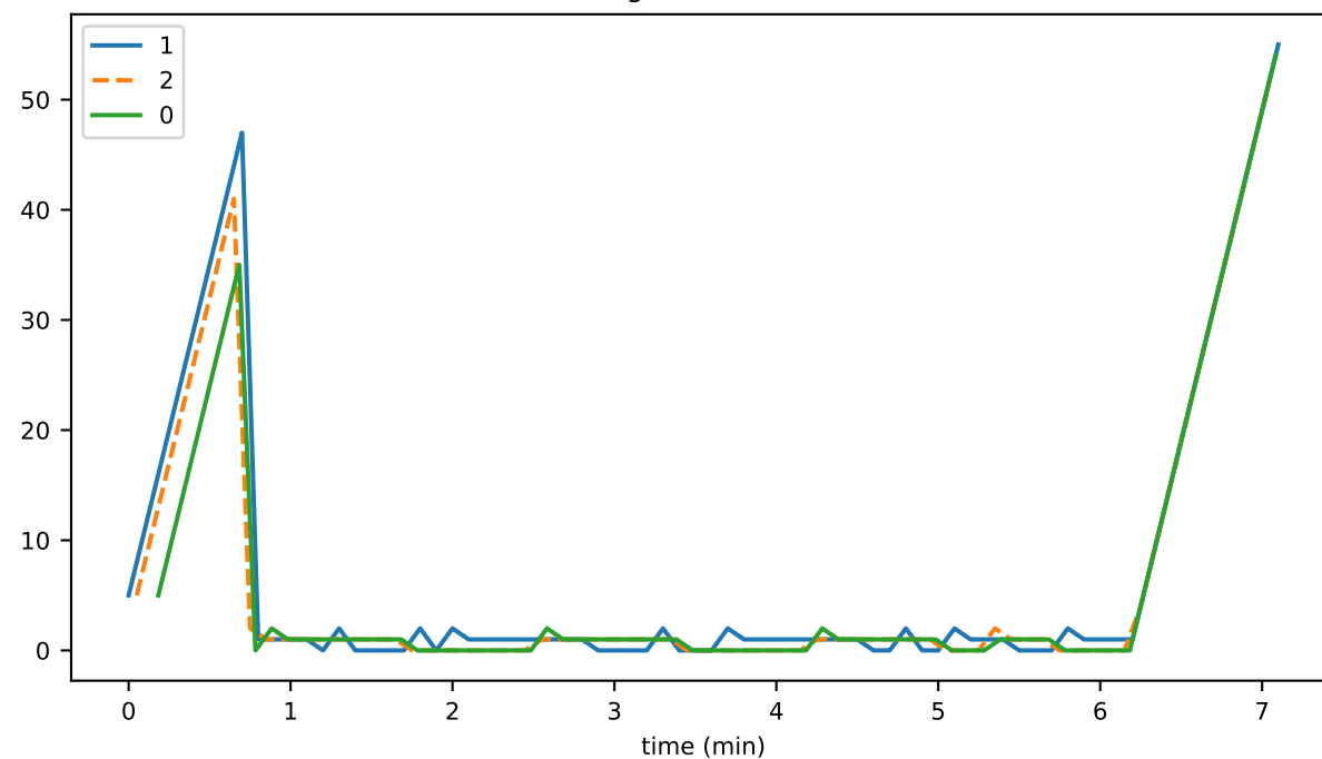
OrphanBuffer_busy_fraction
