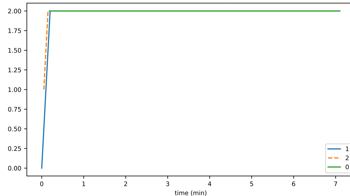
scheduleCreateDurationAvg
