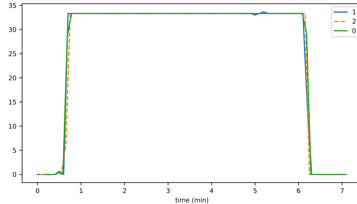
broadcastEventsReceived
