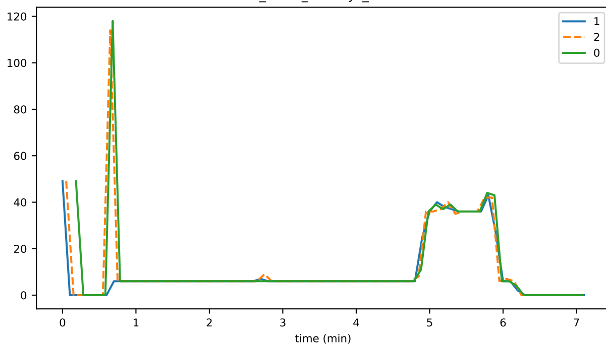
ds_reads_leafKeys_state
