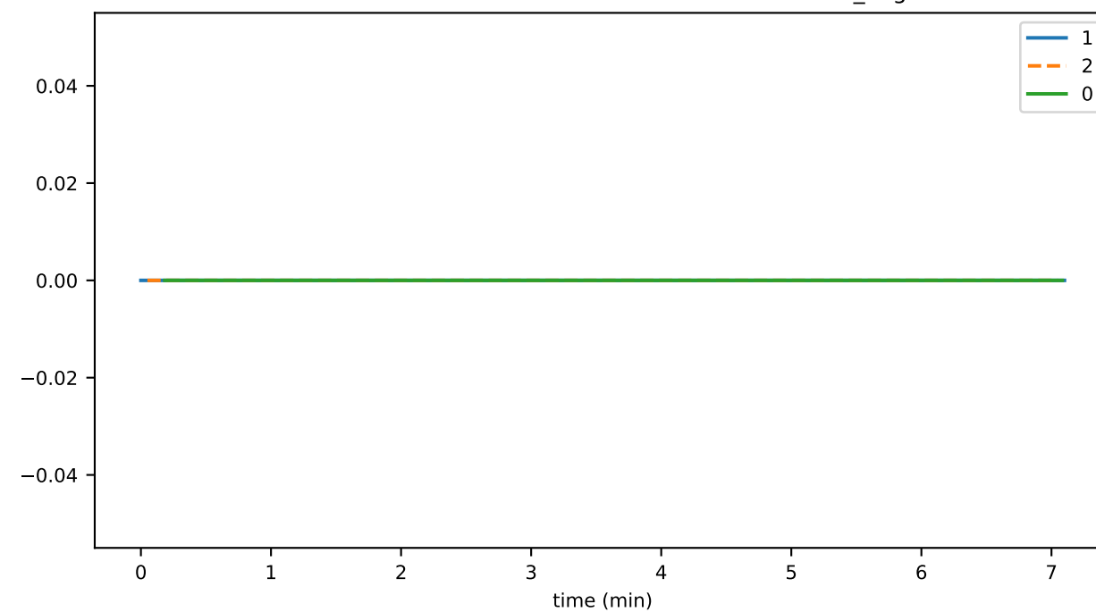
SmartContractService:FailedTransactionDuration_avg
