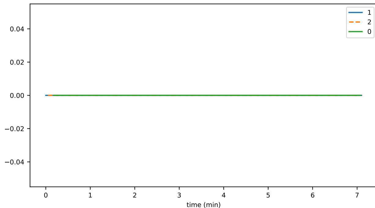
tokenGetInfoDurationAvg
