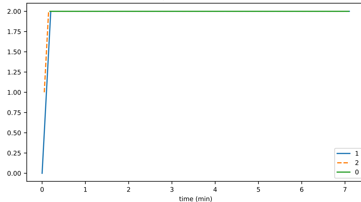
syncs_in_progress
