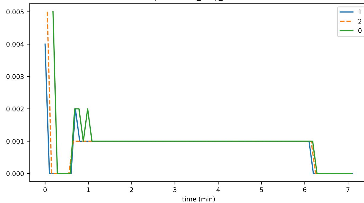
OrphanBuffer_busy_fraction
