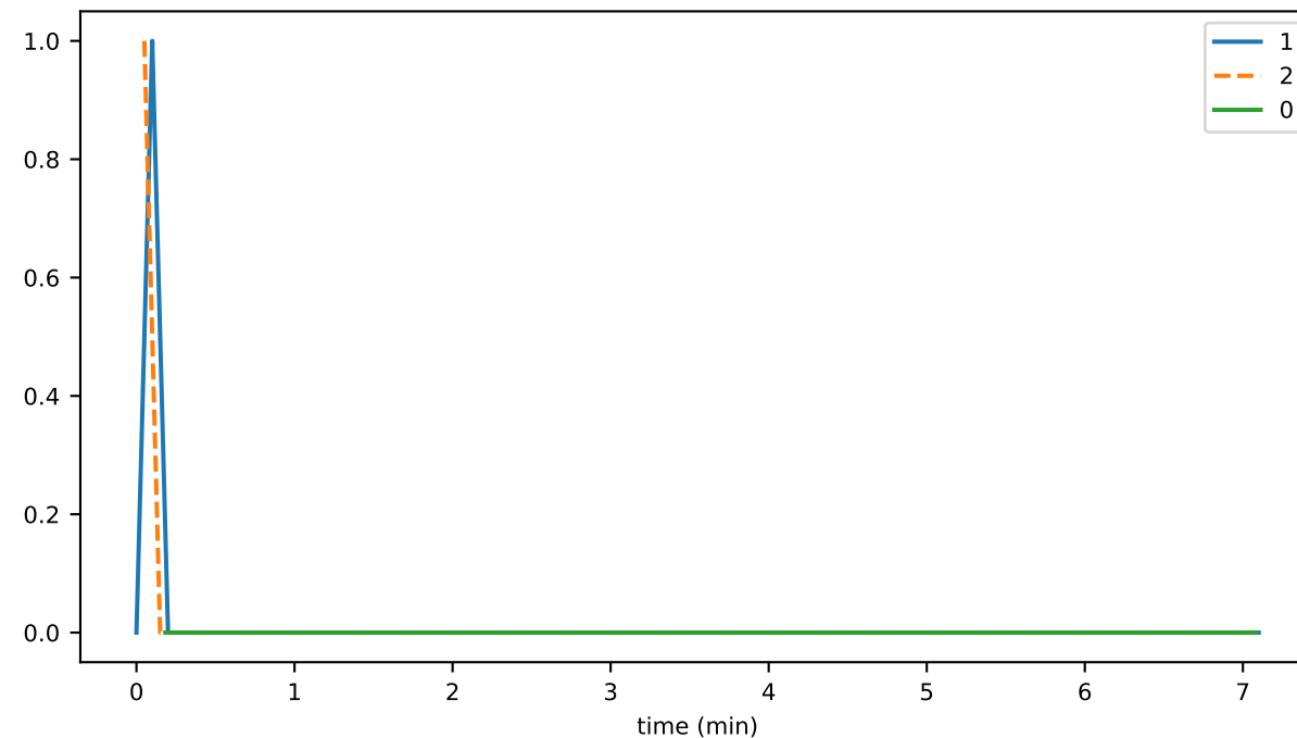
syncPermitsAvailable
