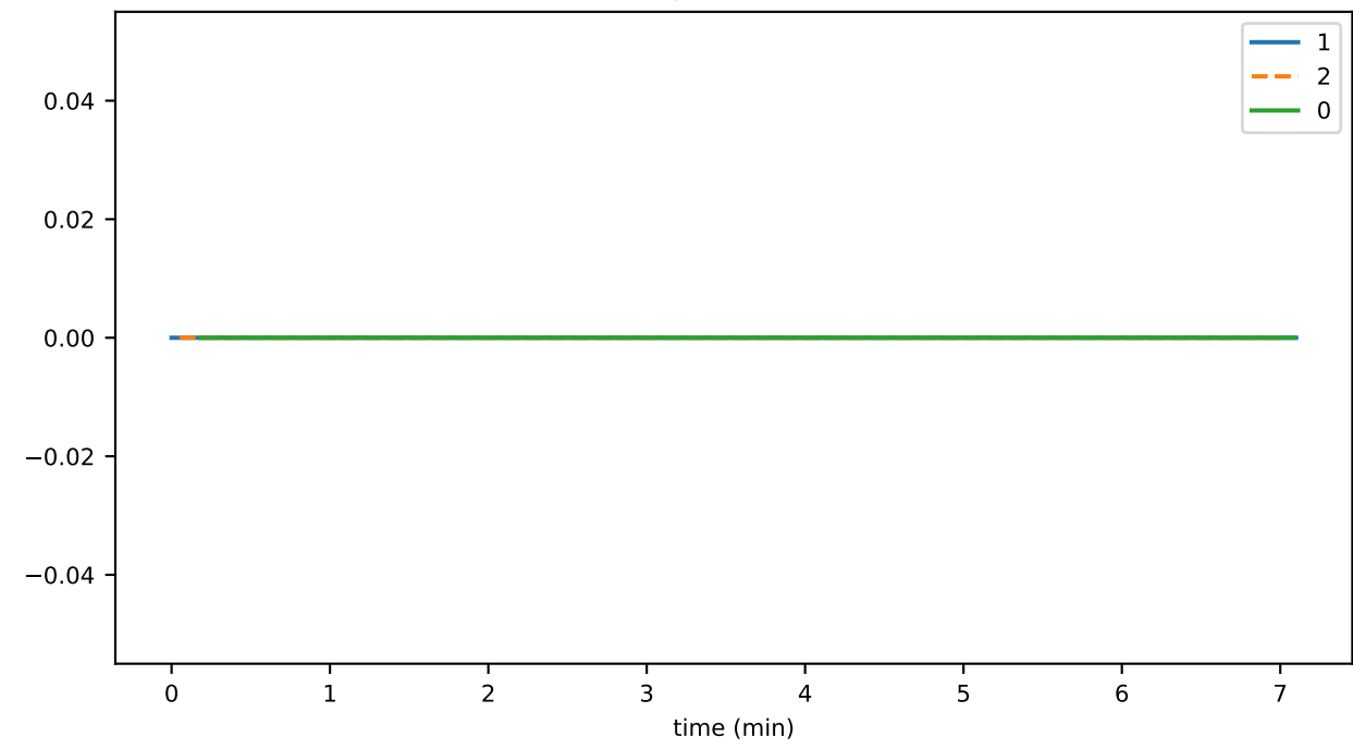
countInMemorySignedState
