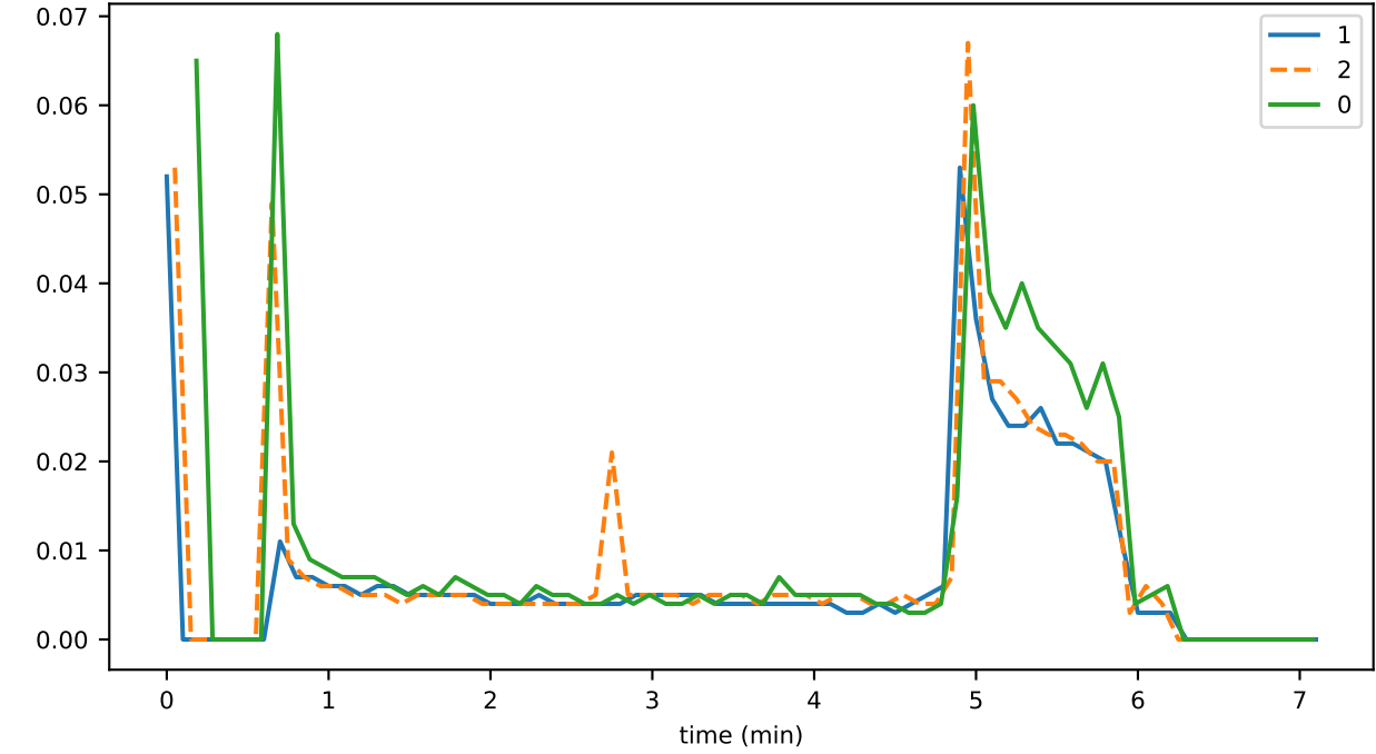
TransactionHandler_busy_fraction
