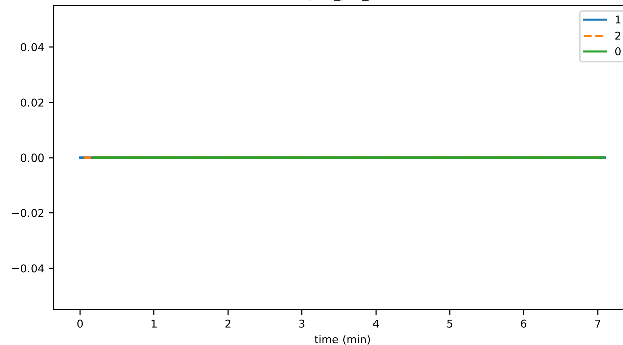
SmartContractService:FailedTransactionDuration_avg
