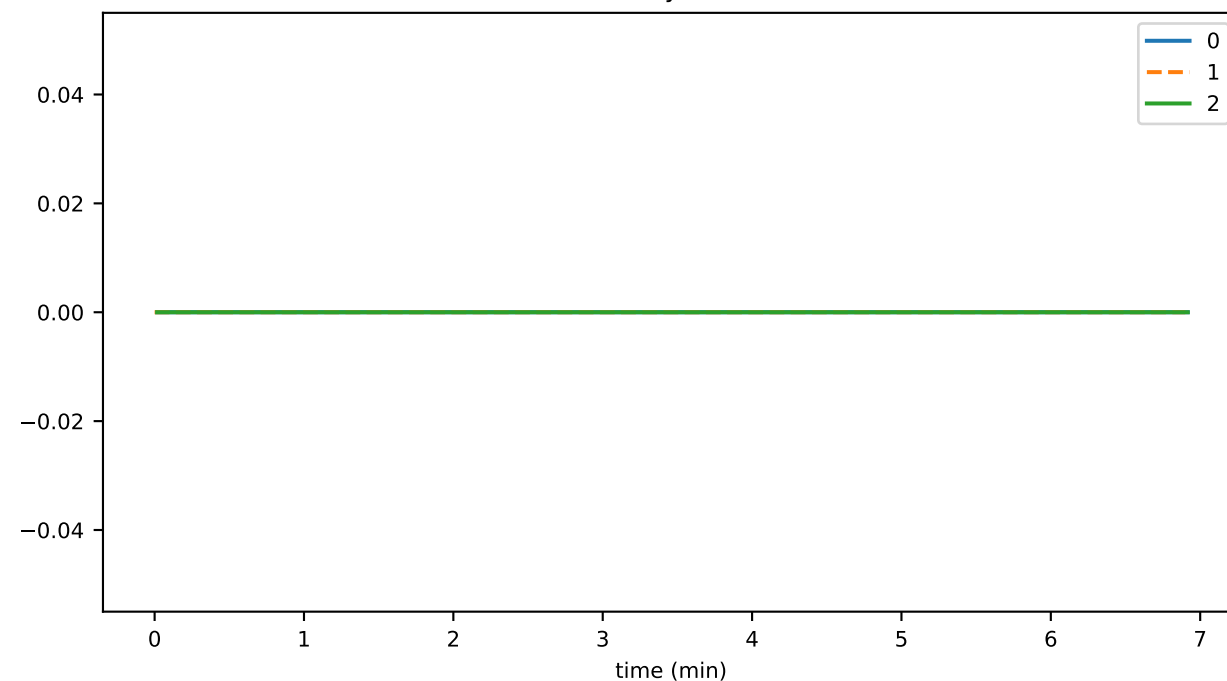
uNRECOGNIZEDDurationMax
