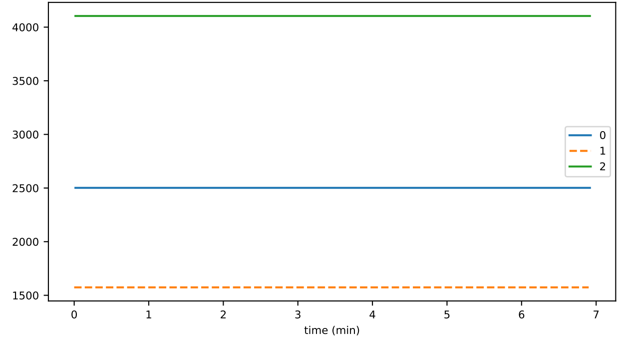
eventDelay_5_orphanBuffer_gossip
