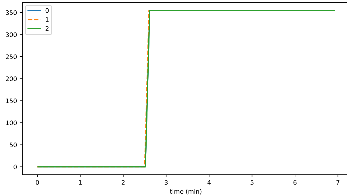
registeredNodeCreateDurationAvg
