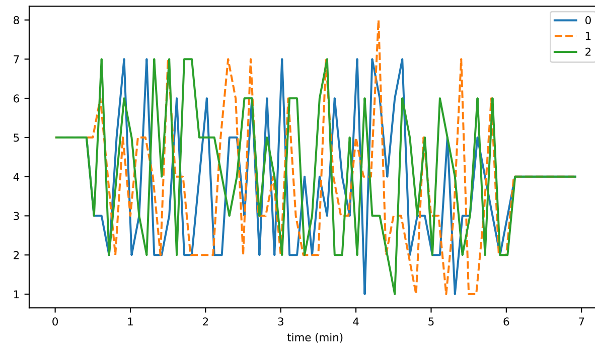
eventsPerRound
