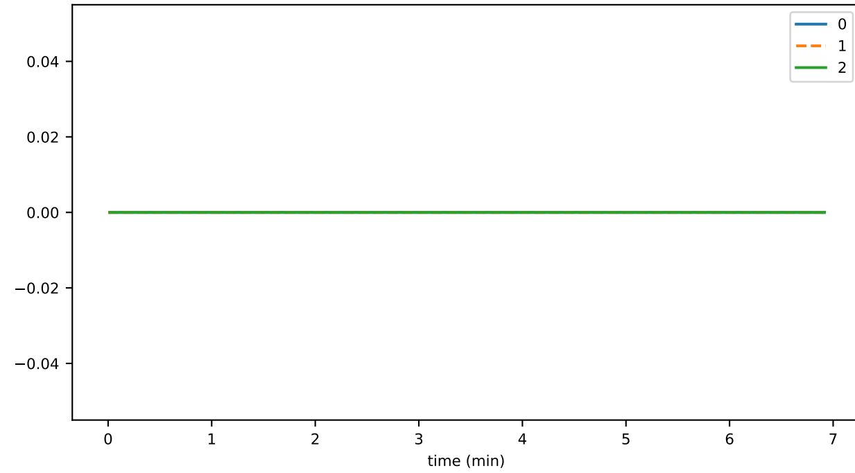
cryptoGetAccountBalanceThrottledTxns
