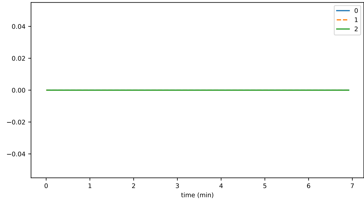
getBySolvencyIDDurationMax
