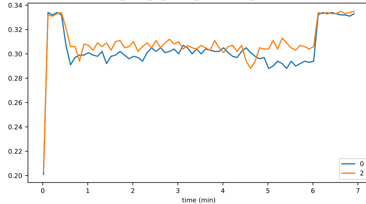
sync_phase_01_fraction_EXCHANGING_WINDOWS
