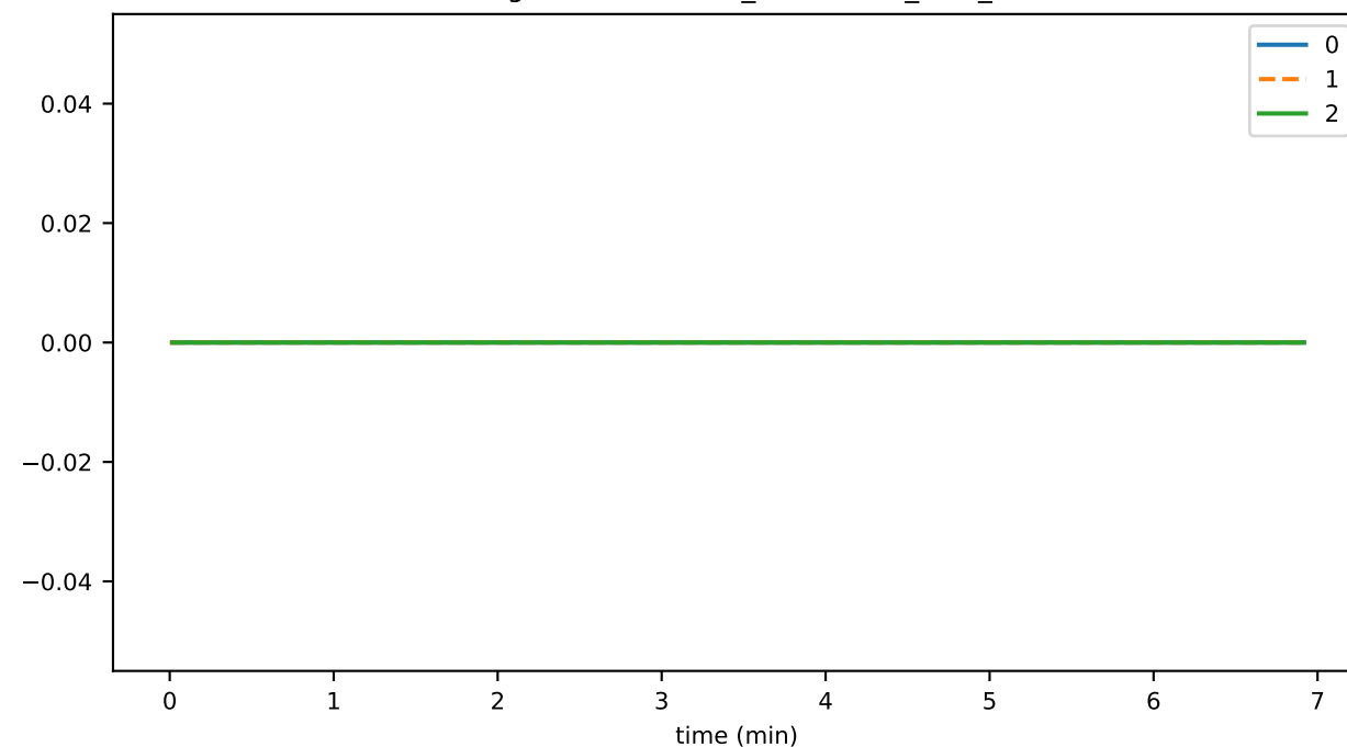
eventsPerRound
