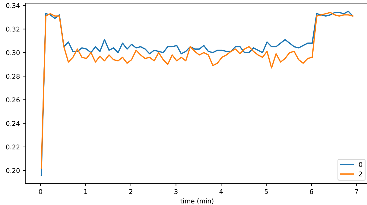
sync_phase_01_fraction_EXCHANGING_TIPS
