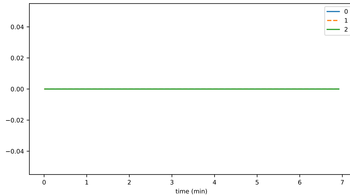
uNRECOGNIZEDDurationMax
