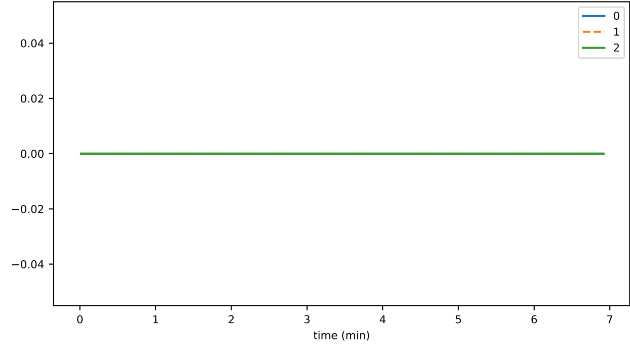
connRecv_resendBlock
