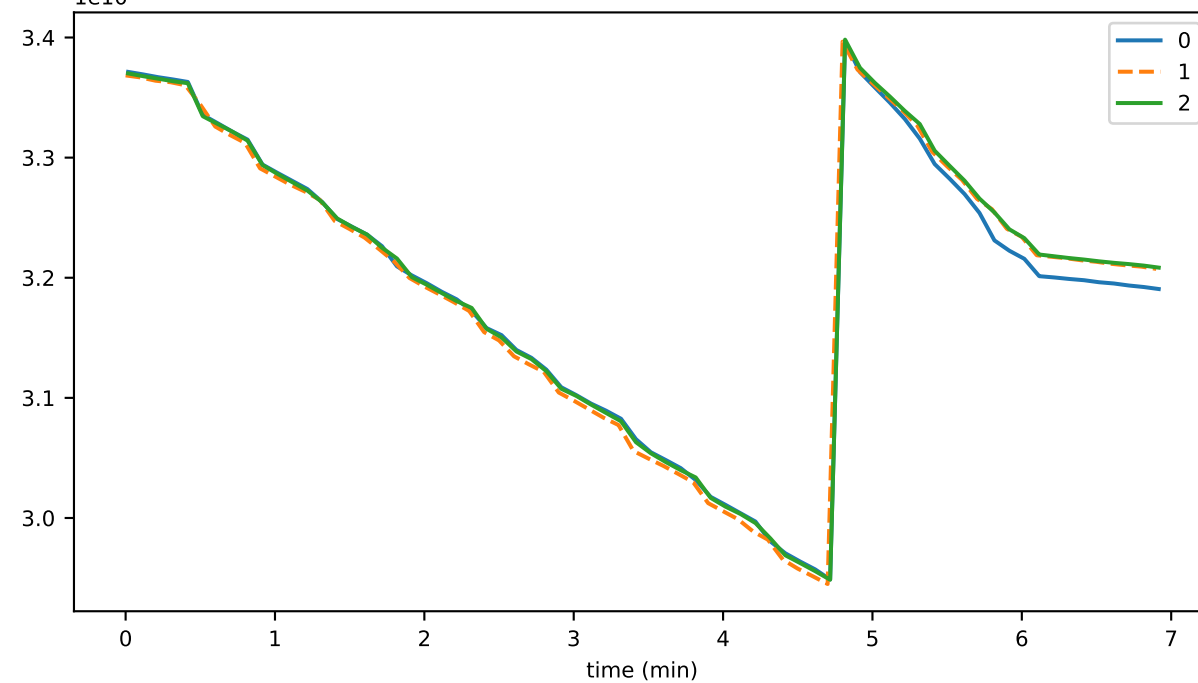
memFree
