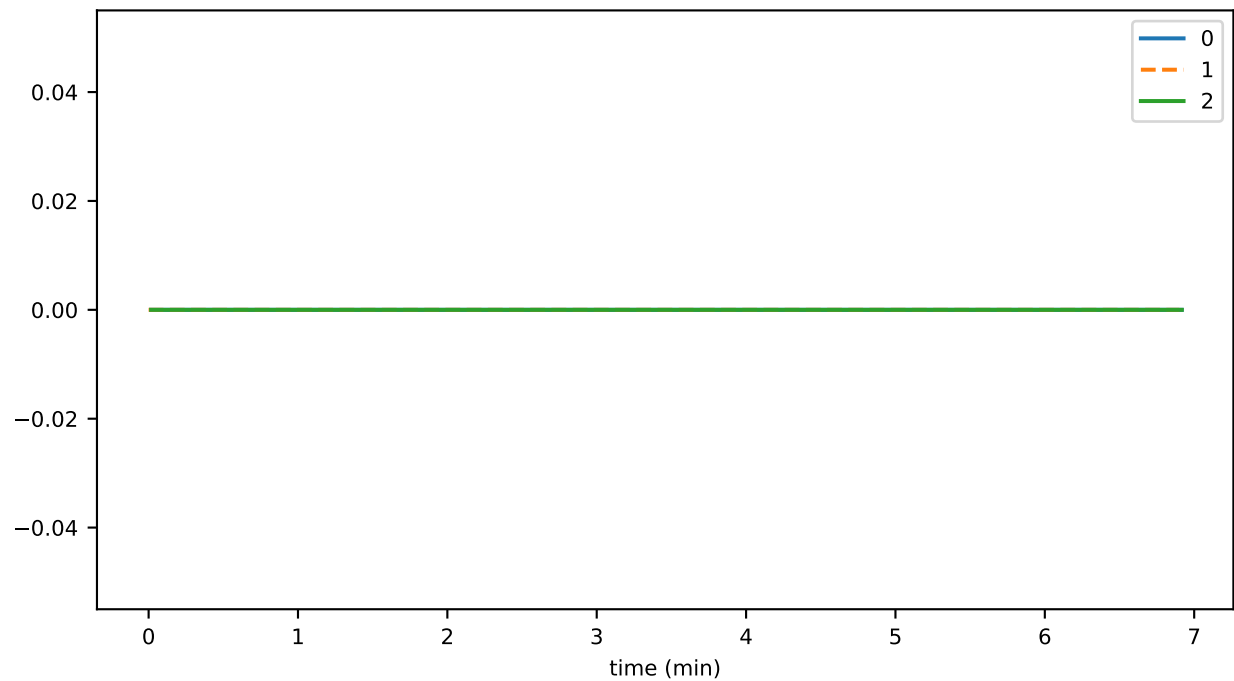
tokenRevokeKycFromAccountDurationAvg
