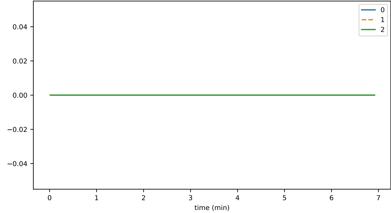
registeredNodeCreateDurationMax
