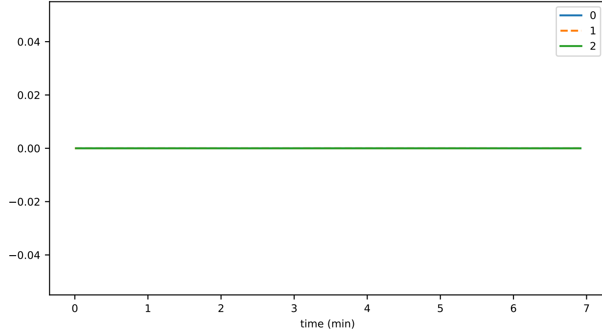
cryptoAddLiveHashDurationAvg
