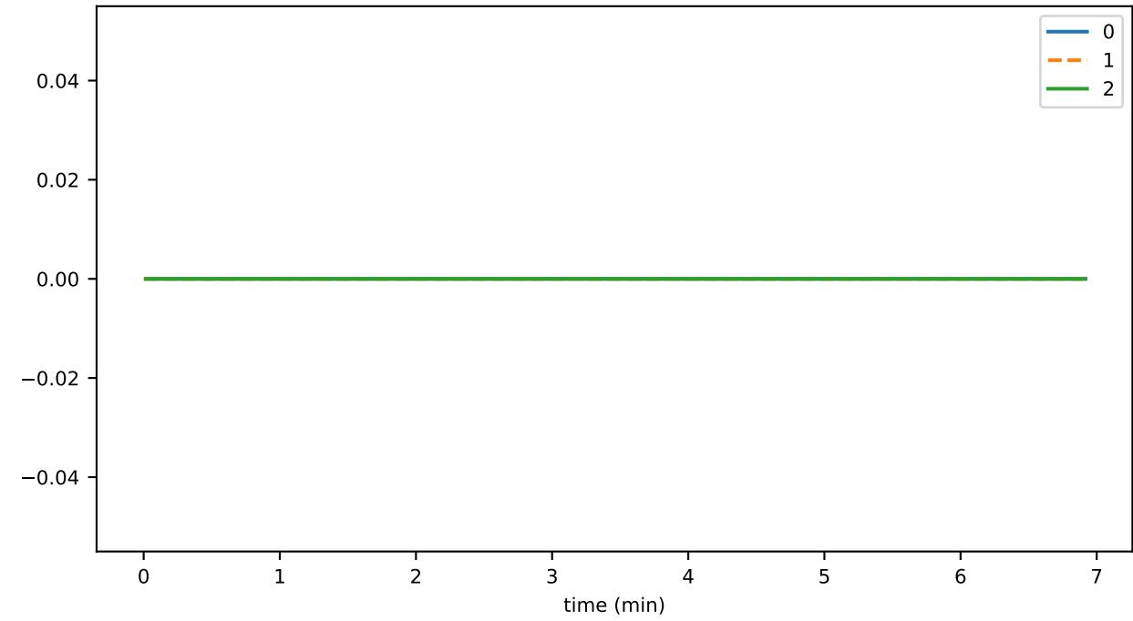
incomingSyncRequests_per_sec
