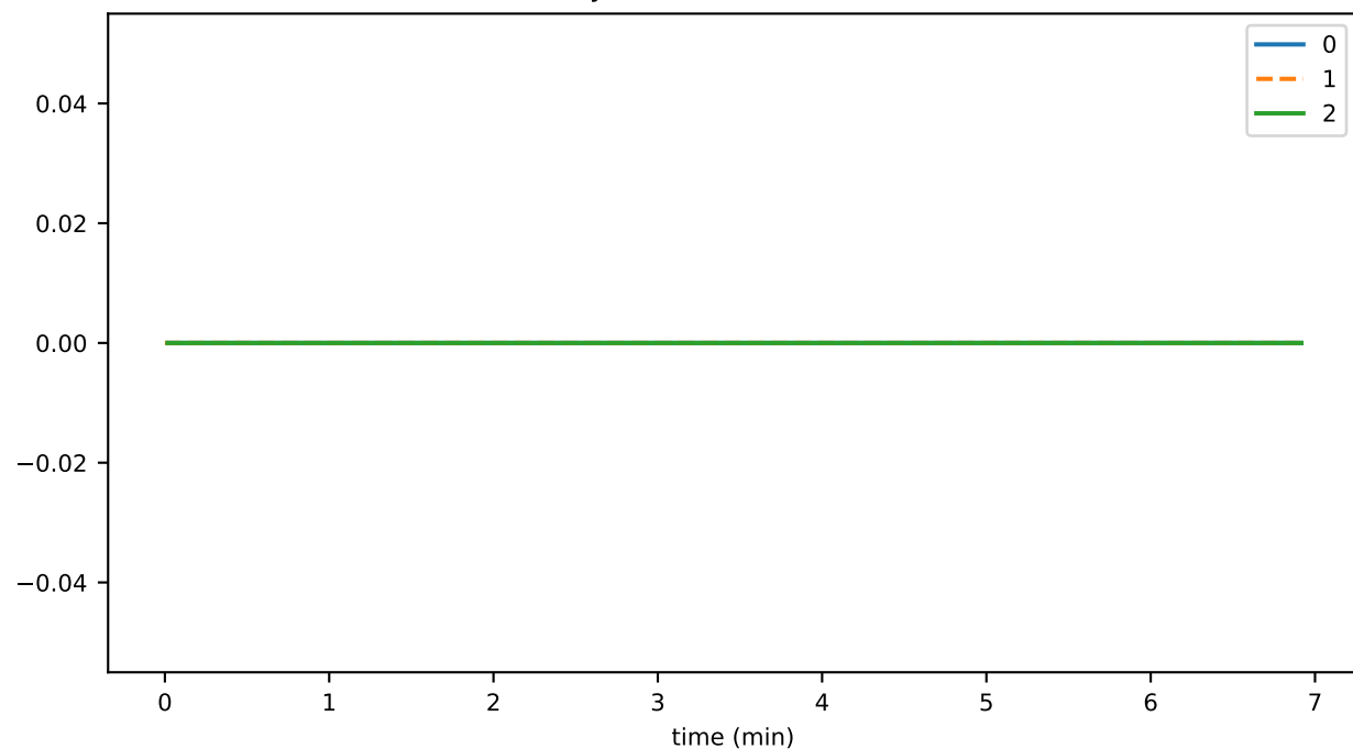
historyProofTransWAsmToFailMs
