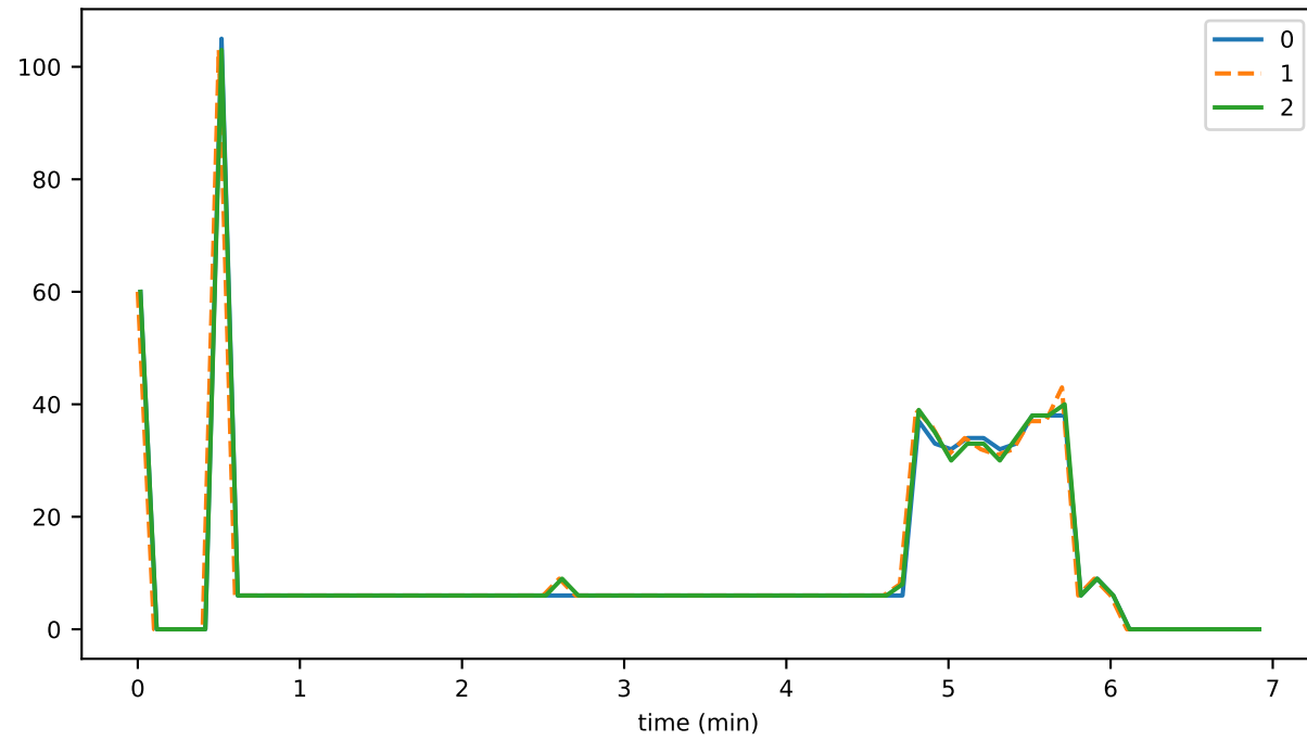
ds_reads_leafKeys_state
