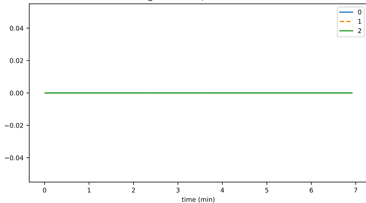
connSend_requestBytes
