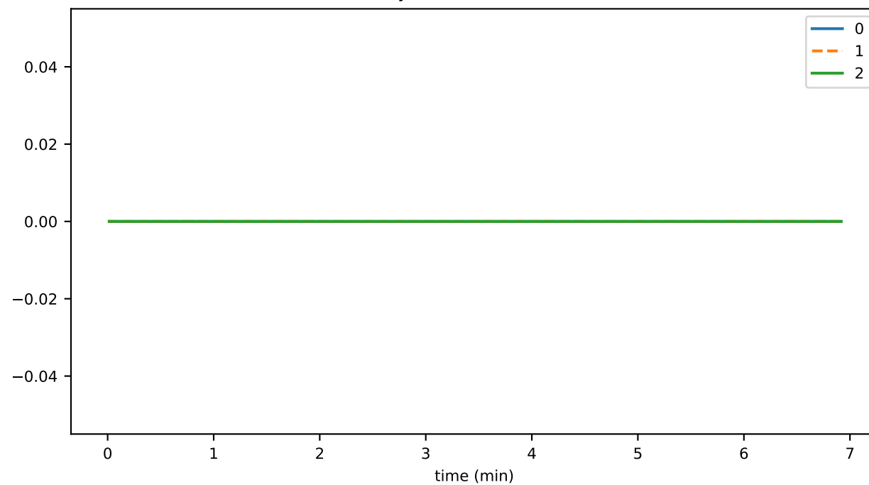
historyProofTransR1ToR2Cnt
