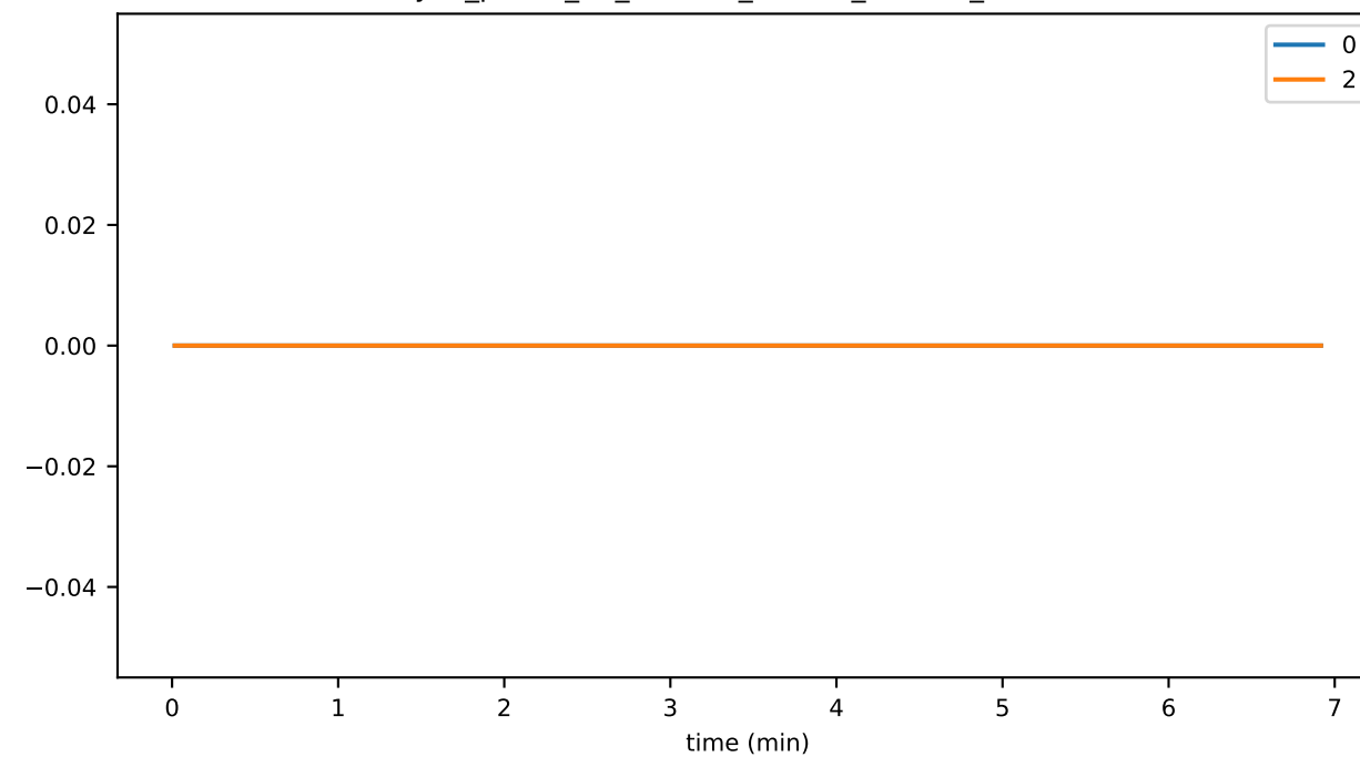
sync_phase_01_fraction_OTHER_FALLEN_BEHIND
