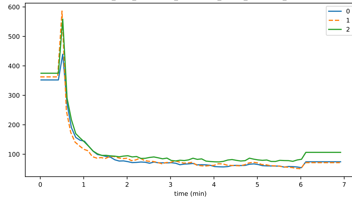
consensusCreateTopicDurationAvg
