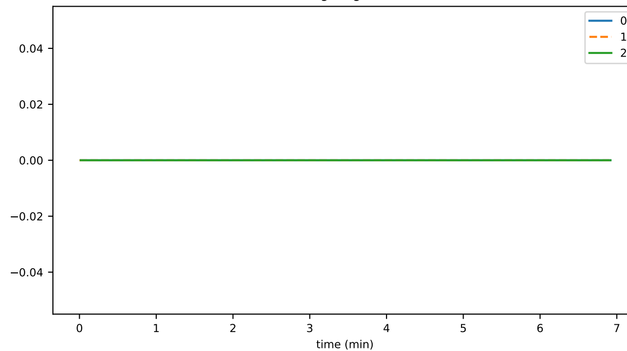
branchingWeightFraction
