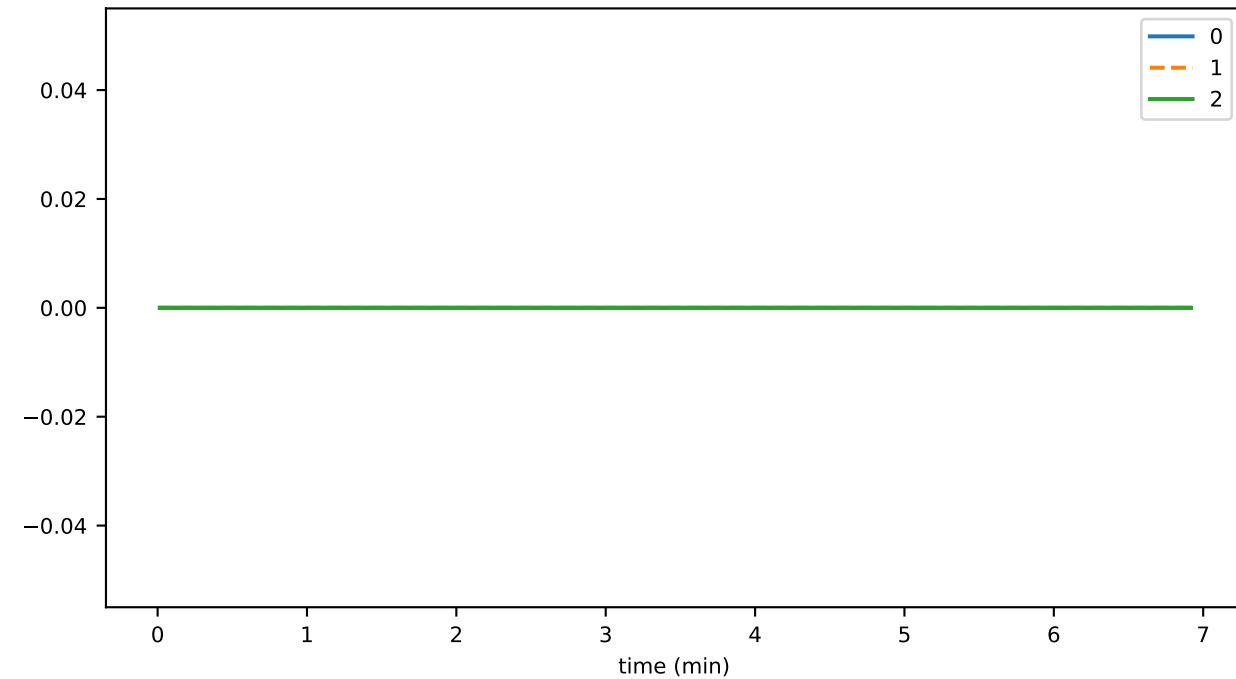
ds_compactions_level_0_leavesSavedSpaceMb_state
