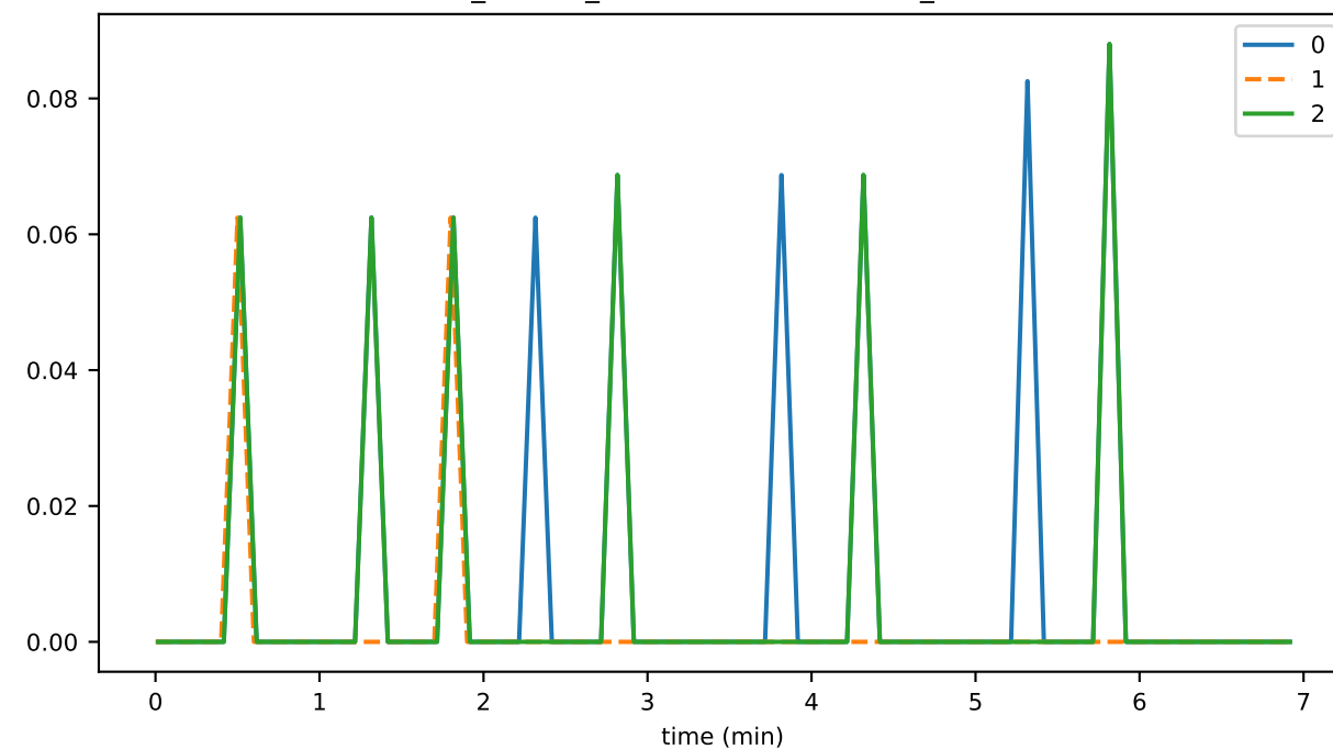
ds_flushes_leafKeysStoreFileSizeMb_state
