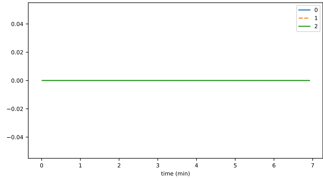
cryptoGetAccountRecordsDurationAvg
