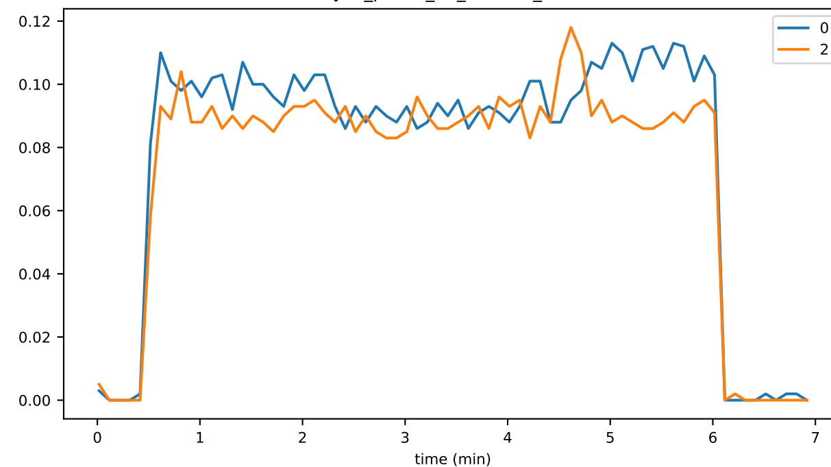
sync_phase_01_fraction_OTHER_FALLEN_BEHIND
