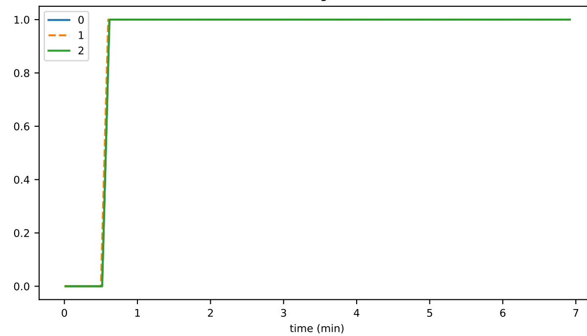
trans_per_event
