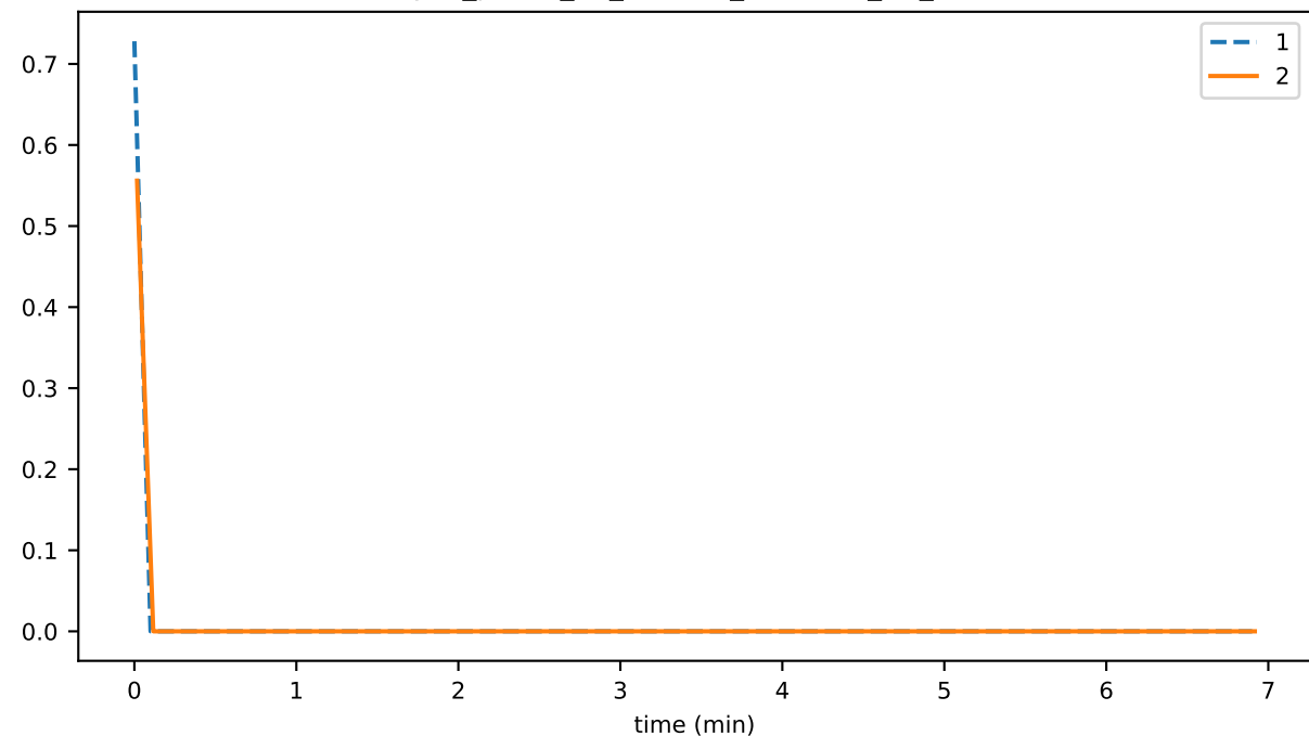
sync_phase_00_fraction_RECEIVING_EVENTS
