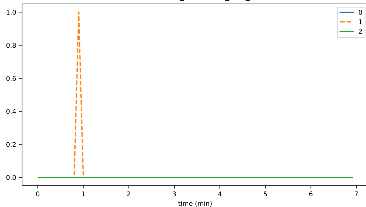
branchingNodeCount
