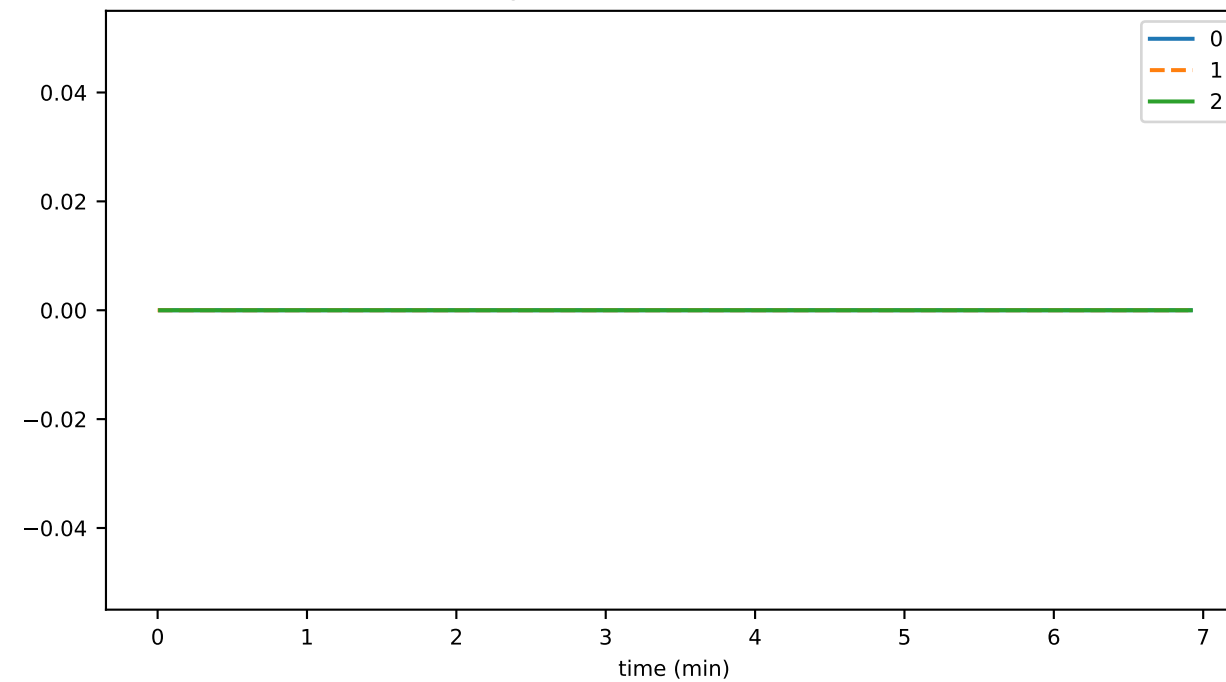
statesIneligibleForDeletion
