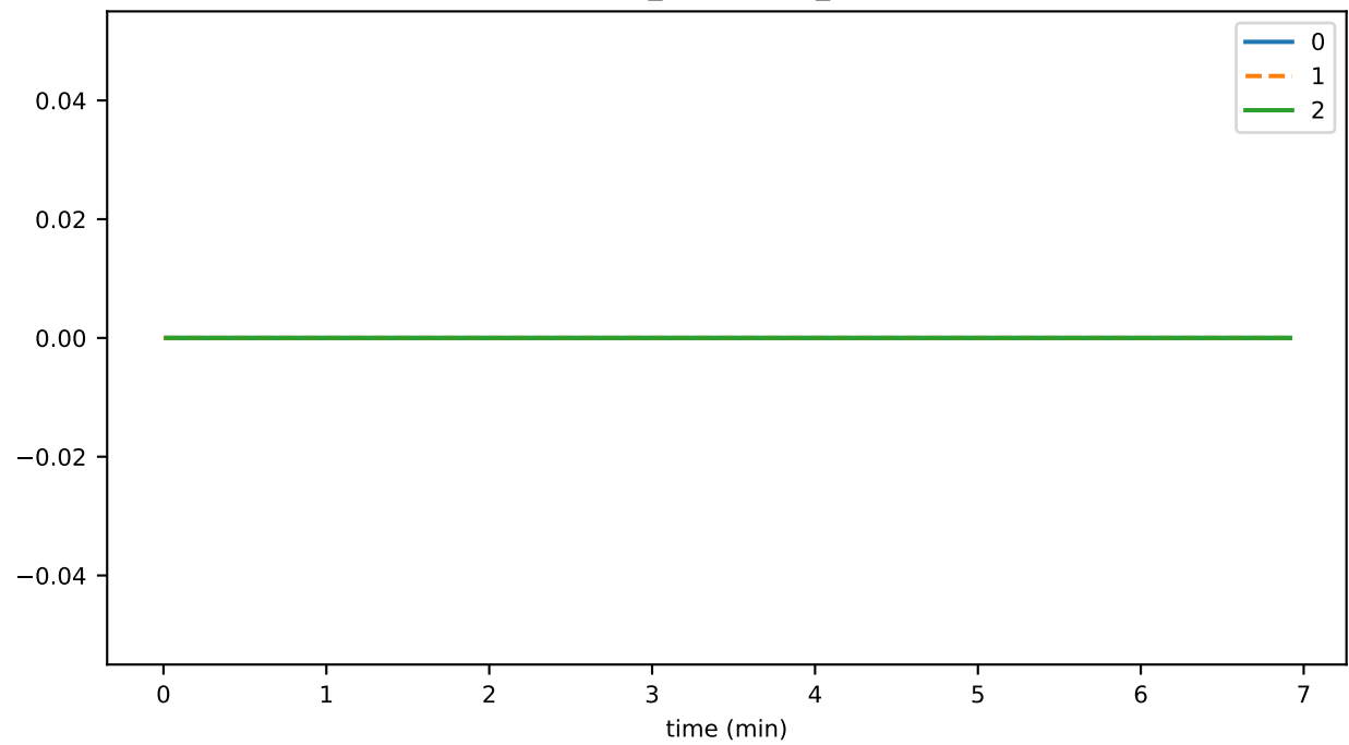
connRecv_endStream_success
