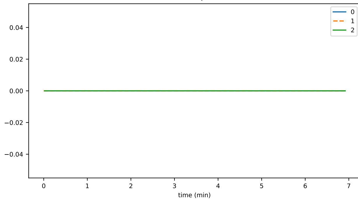
consensusDeleteTopicDurationAvg
