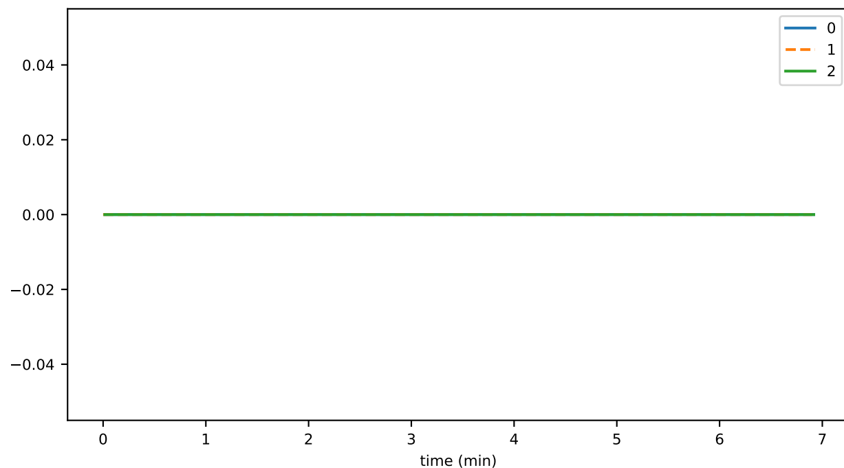
scheduleDeleteDurationAvg
