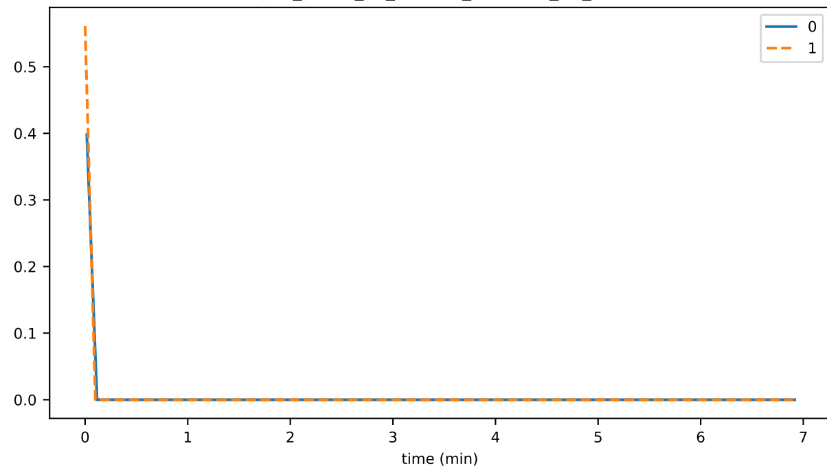
sync_phase_02_fraction_RECEIVING_EVENTS
