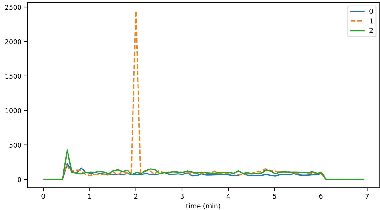
eventDelay_1_hashing_gossipMAX
