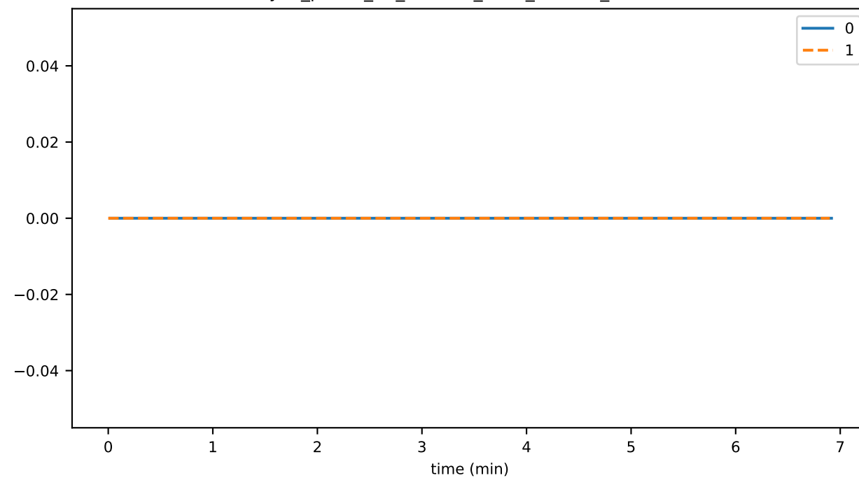
sync_phase_02_fraction_SELF_FALLEN_BEHIND
