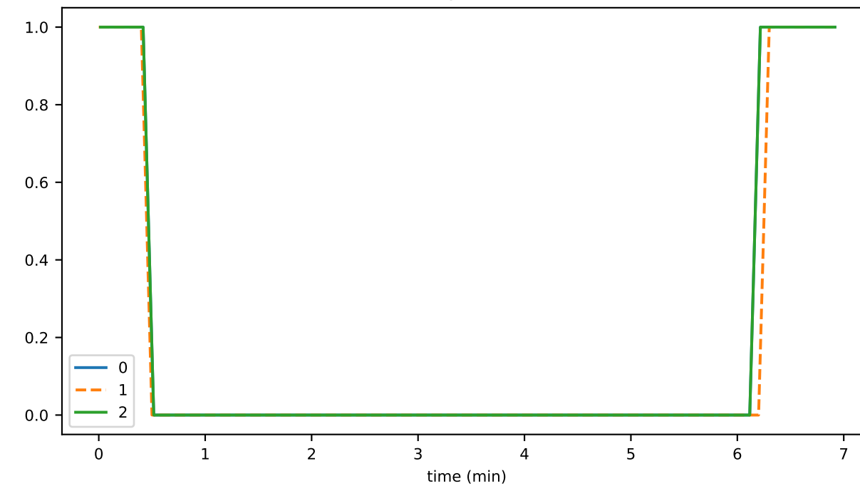
Dig_per_sec
