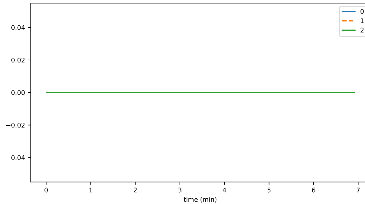
Dig_per_sec
