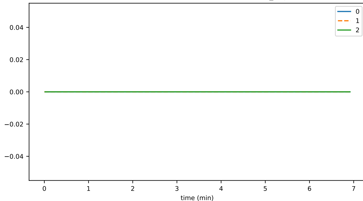
SmartContractService:TransactionGasUsed_sum
