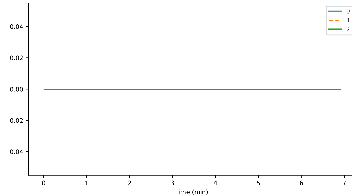
SmartContractService:SystemContractMethodCall_APPROVAL_failed
