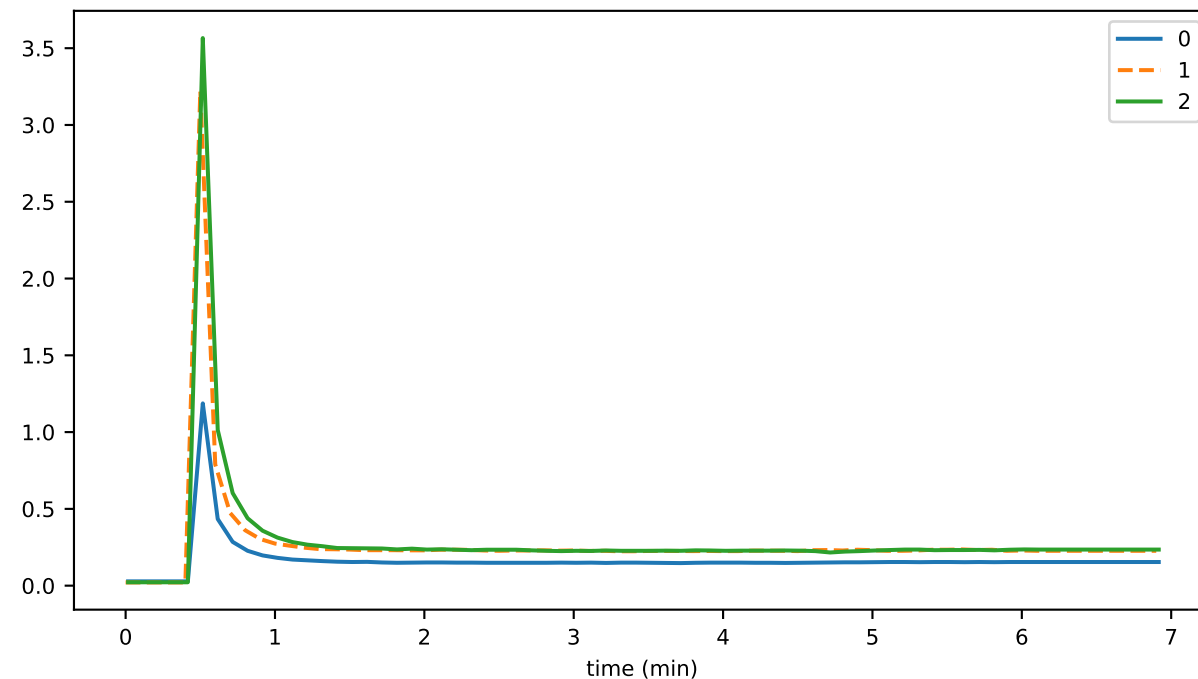
memFree
