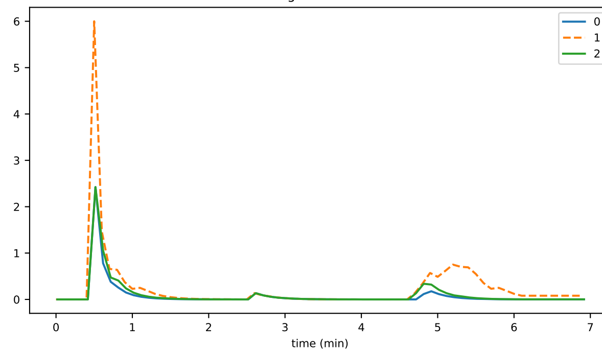
sigStateHash
