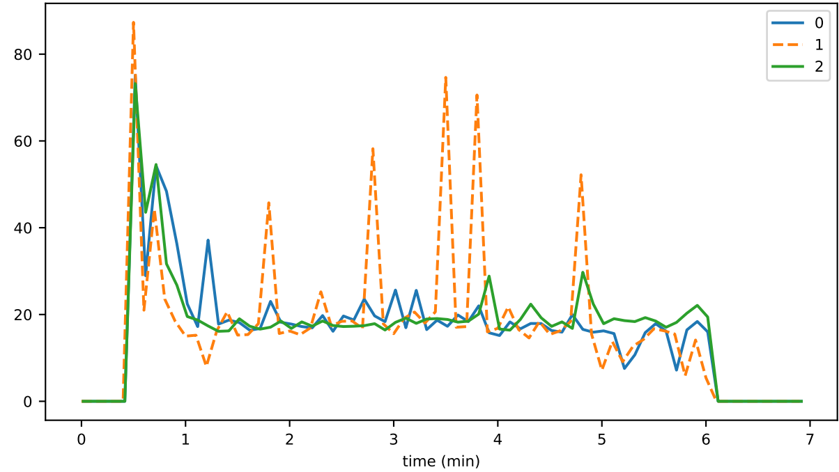
eventDelay_1_hashing_gossipMAX
