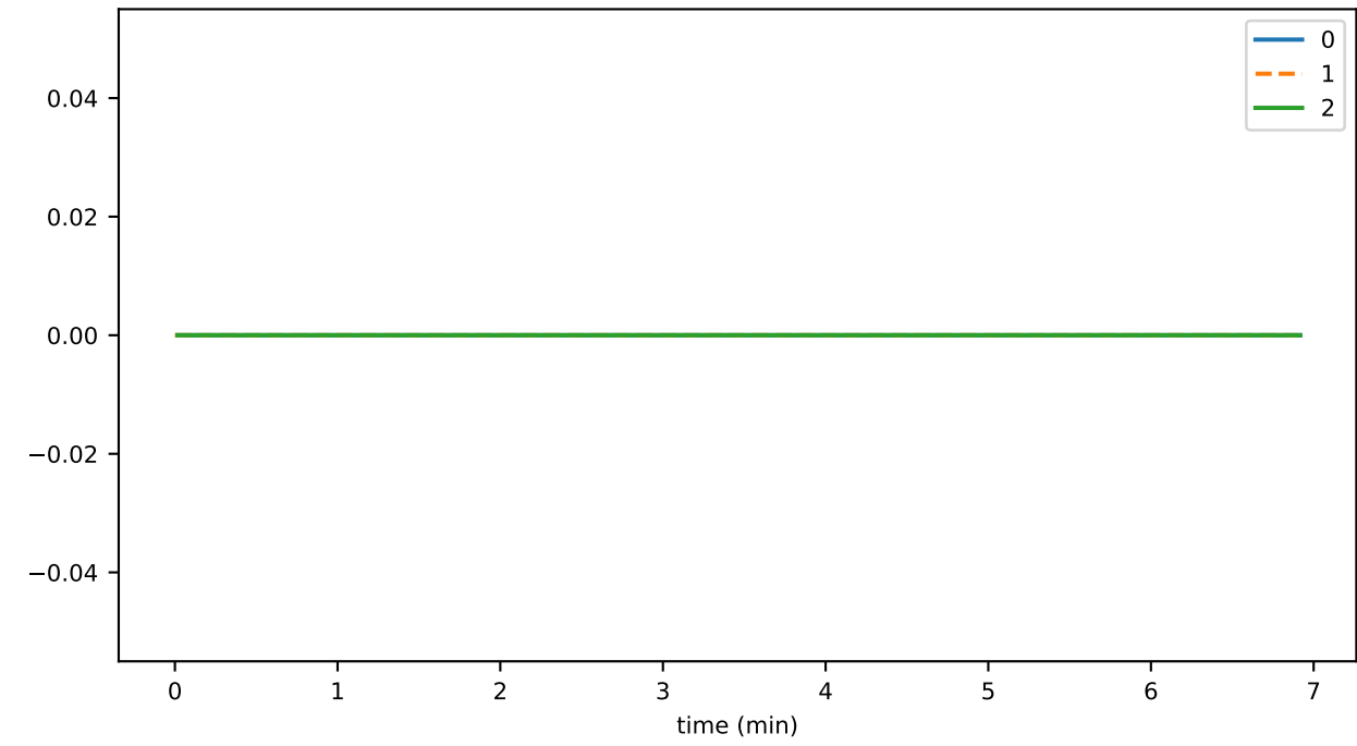
eventCreation_fraction_PIPELINE_INSERTION
