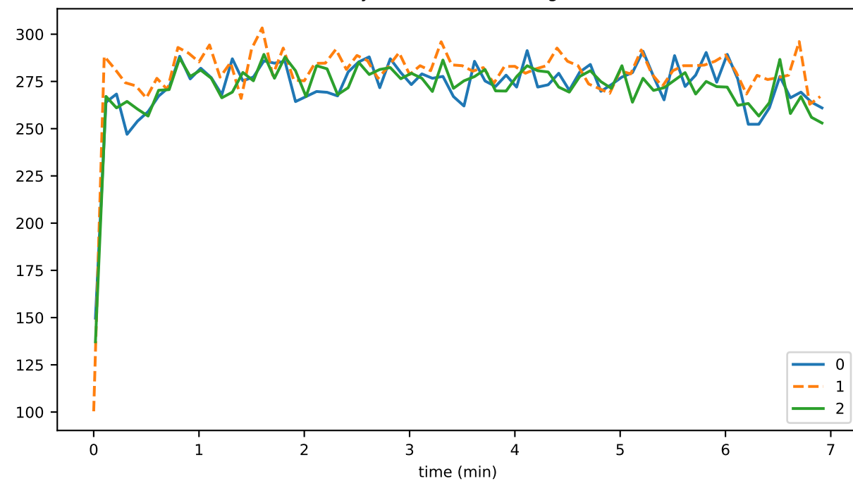
doNotSyncRemoteProcessingEvents
