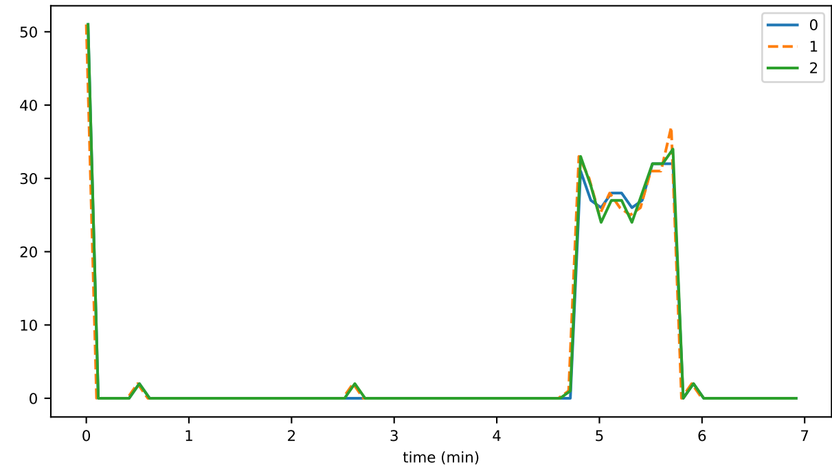
ds_reads_leaves_state
