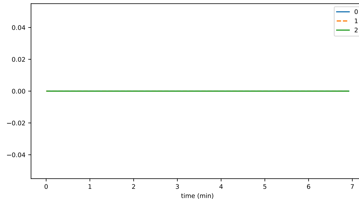
scheduleDeleteDurationMax
