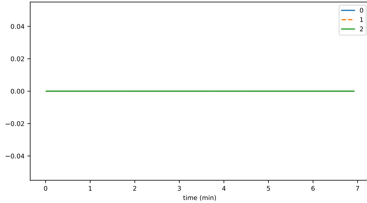
getBySolvencyIDDurationAvg
