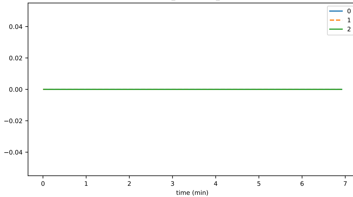
connRecv_endStream_timeout
