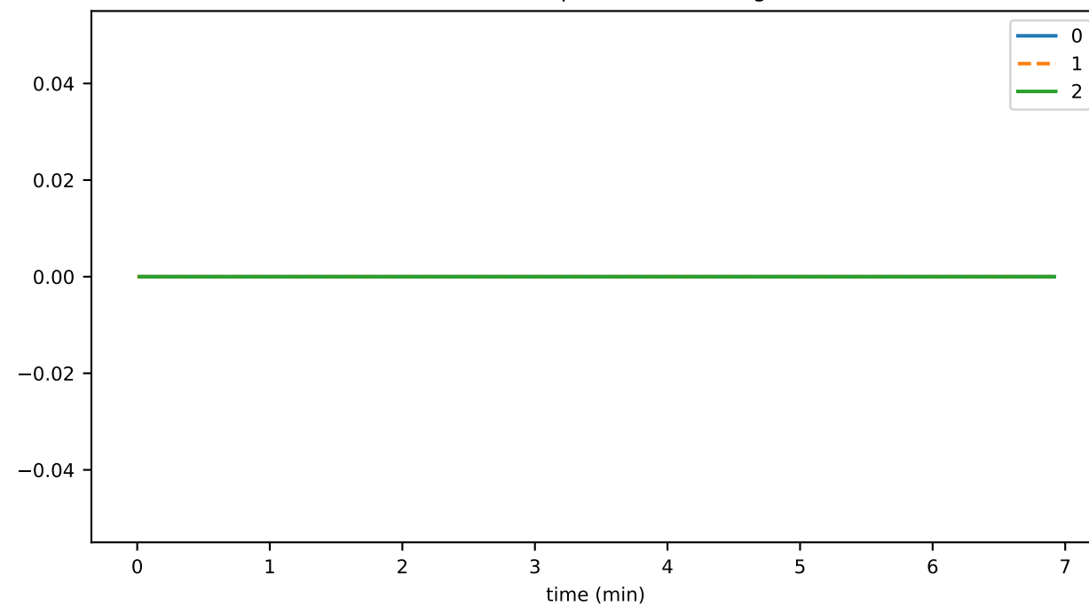
nodeStakeUpdateDurationAvg
