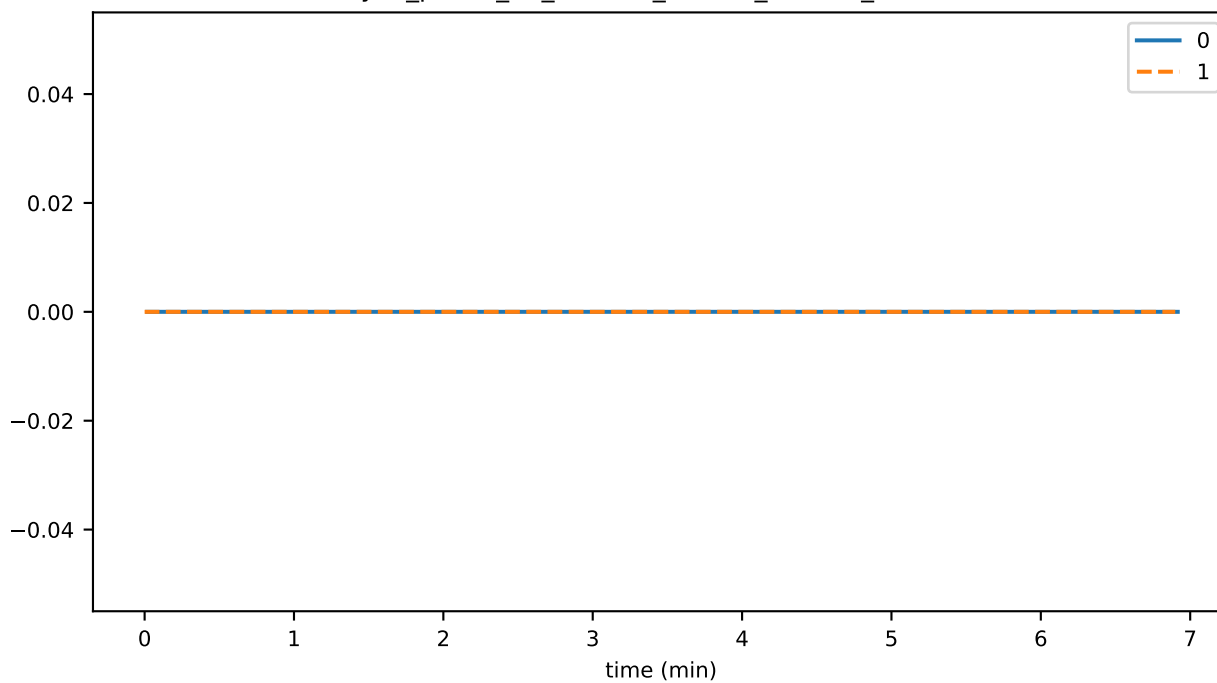
sync_phase_02_fraction_OTHER_FALLEN_BEHIND
