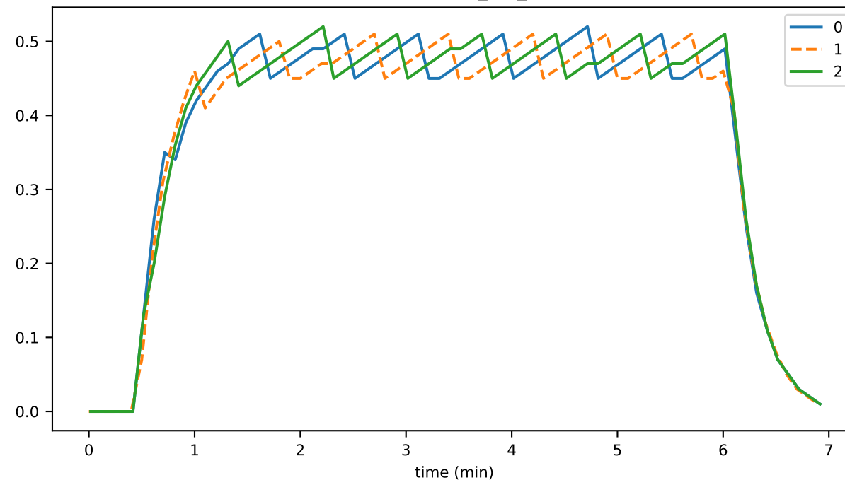
sstatesSigned_per_sec
