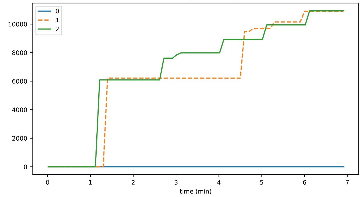
futureEventBuffer_eventCreator_maxBR
