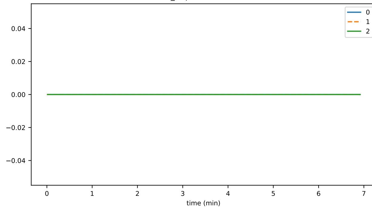
connSend_requestExceedsHardLimit
