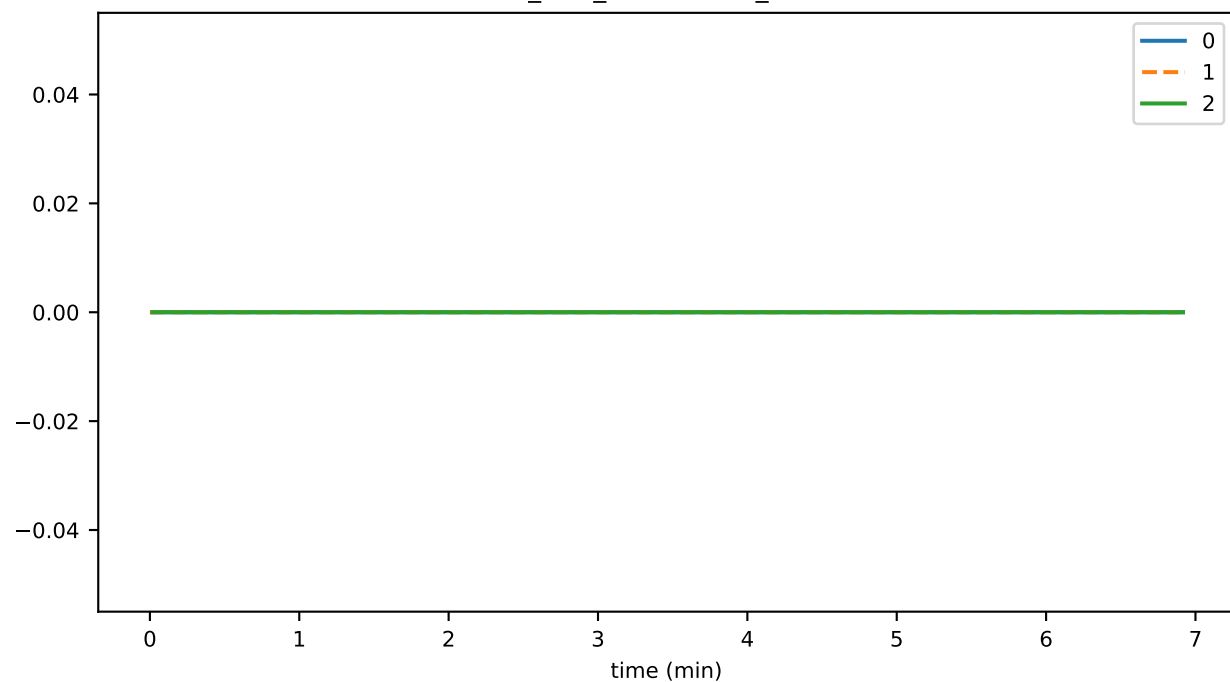
ds_flushes_hashesWritten_state
