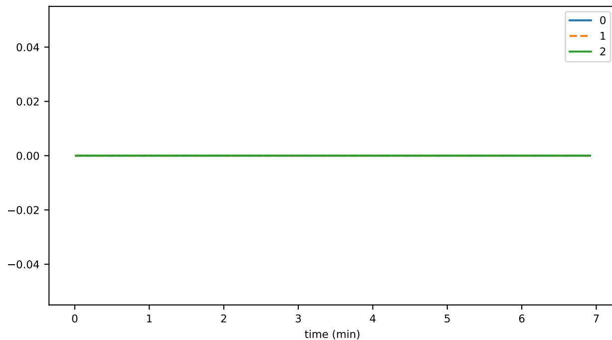
nodesPercentUsed
