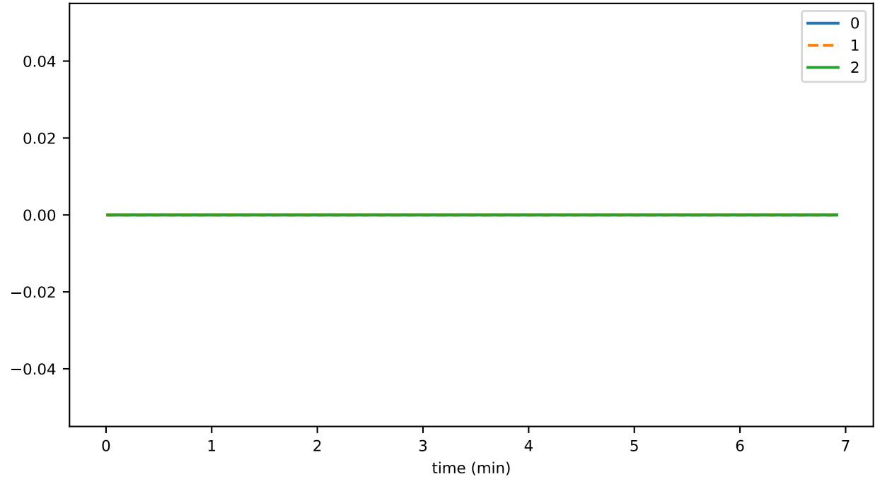
ConsensusEngine_unhandled_task_count
