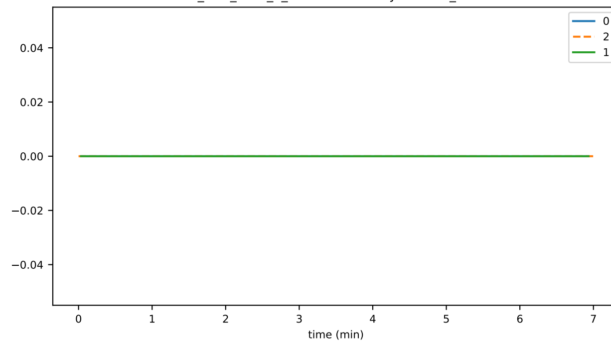
ds_files_level_6_hashesFileSizeByLevelMb_state
