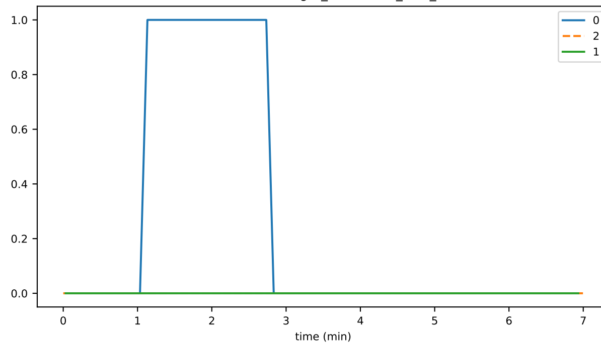
EventManager_unhandled_task_count
