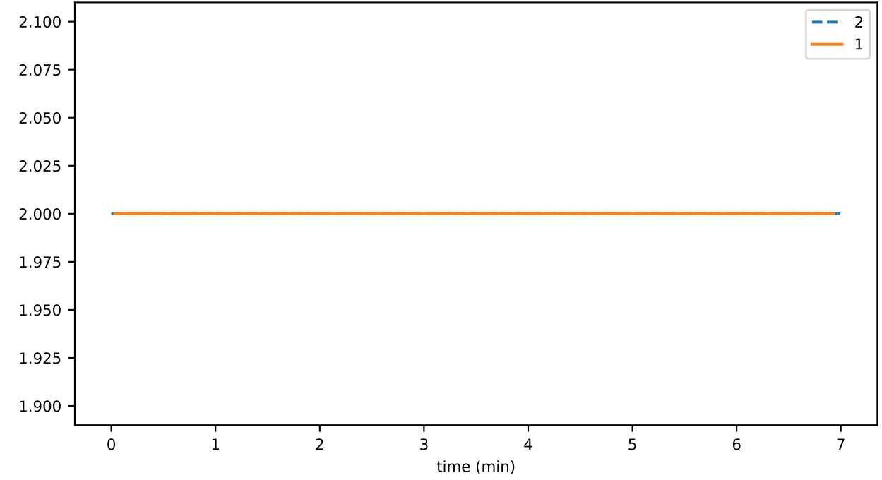
rpc_output_00_queueMaxSize
