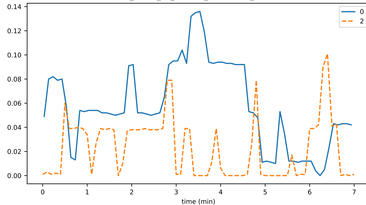
sync_phase_01_fraction_SENDING_EVENTS
