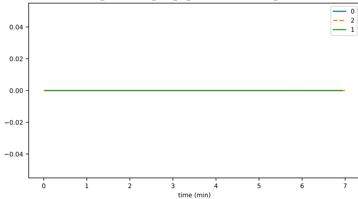
ds_compactions_level_10_leafKeysSavedSpaceMb_state
