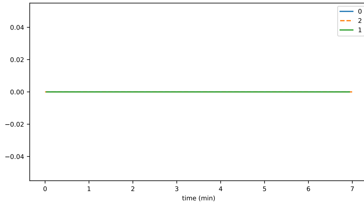
contractGetBytecodeDurationAvg
