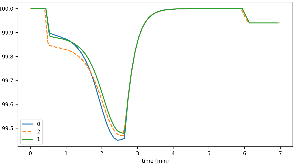
nodeActivePercent_node2
