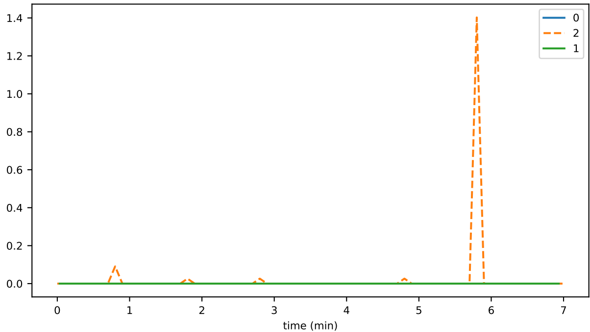
ds_compactions_level_1_leavesSavedSpaceMb_state
