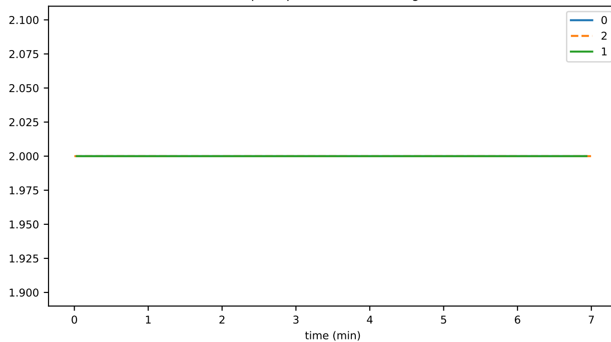
rpcDispatchThreadRunning
