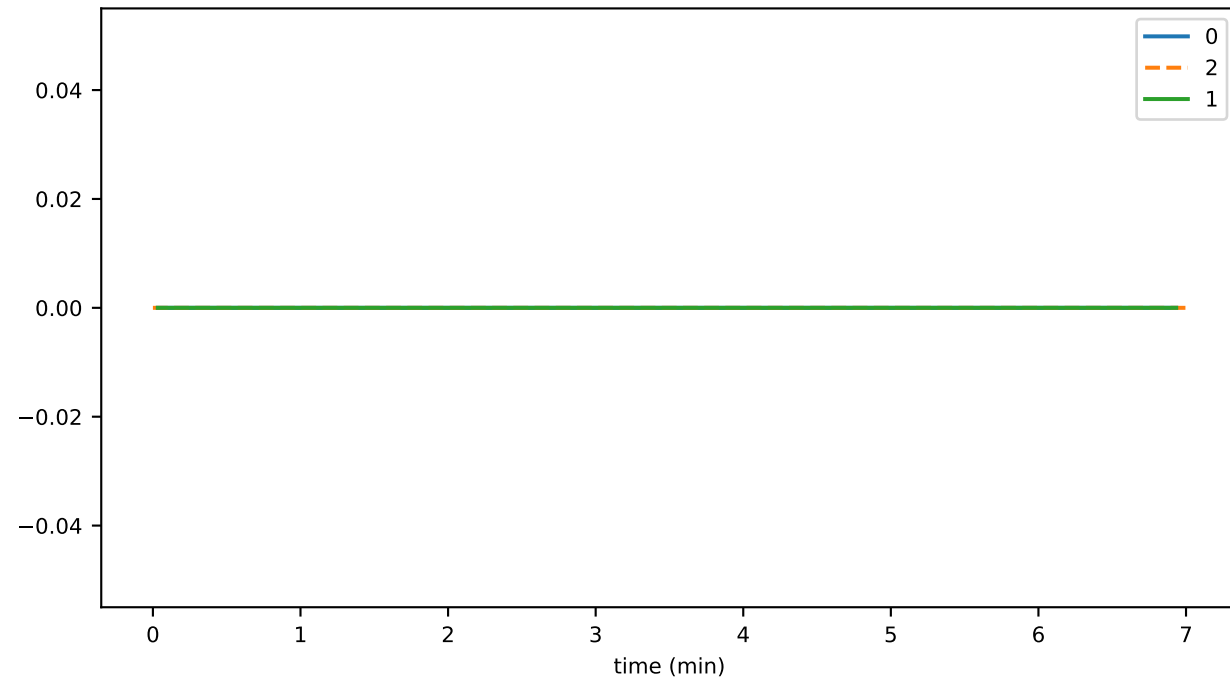
preconsensusEventAverageUnutilizedFileSpan
