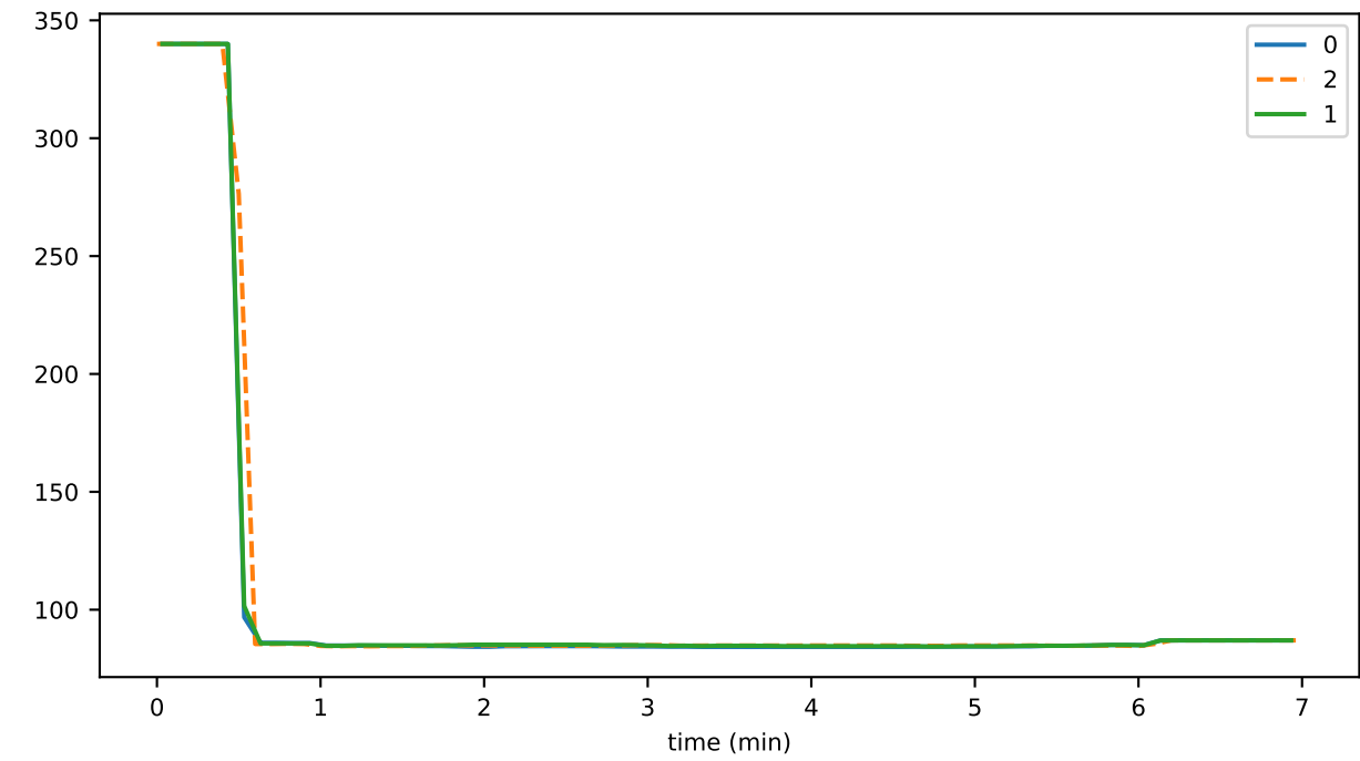
knownSetSize
