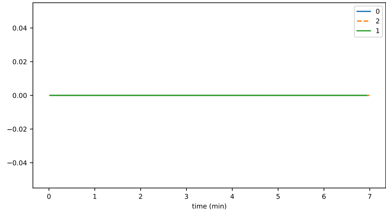
knownSetSize
