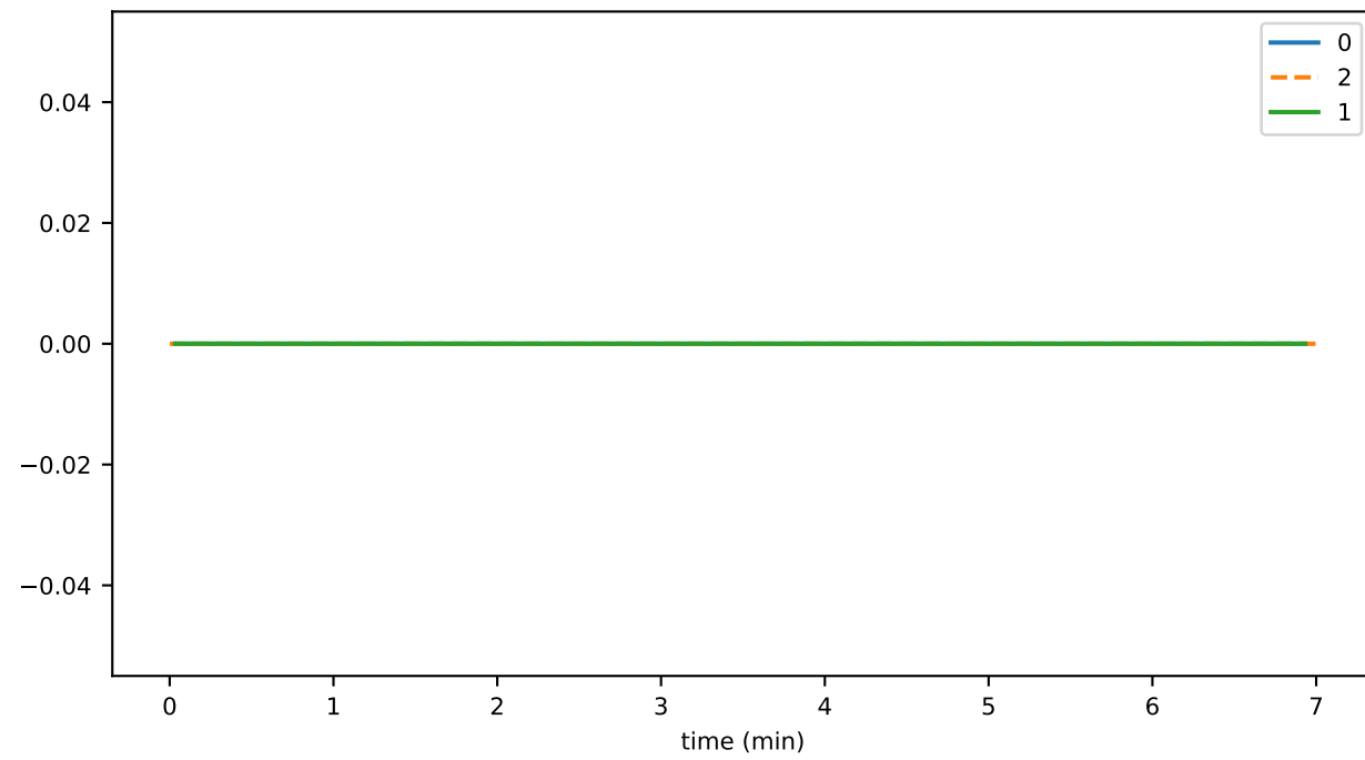
tokenBurnDurationAvg
