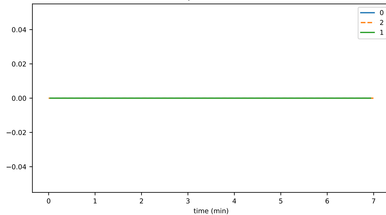
tokenUpdateDurationMax
