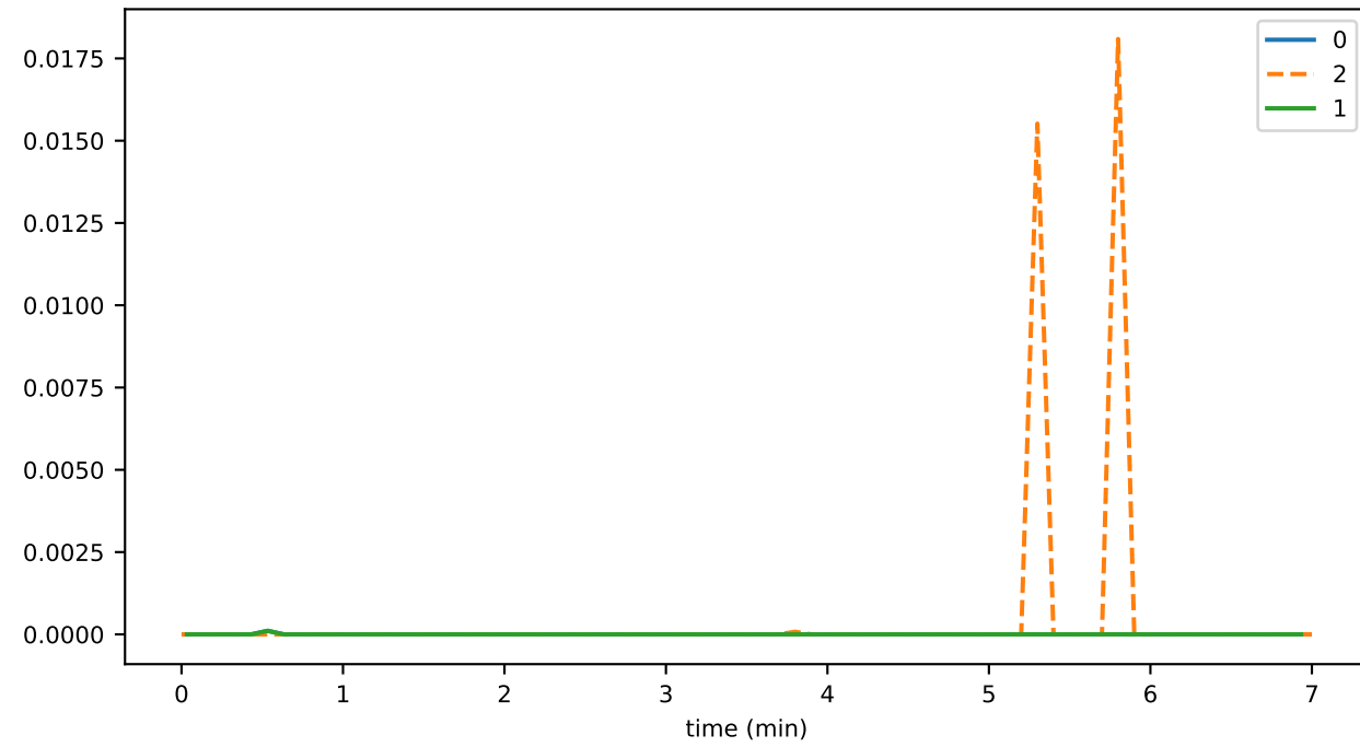
ds_flushes_leafKeysStoreFileSizeMb_state
