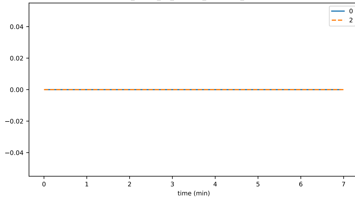
sync_phase_01_fraction_SENDING_EVENTS
