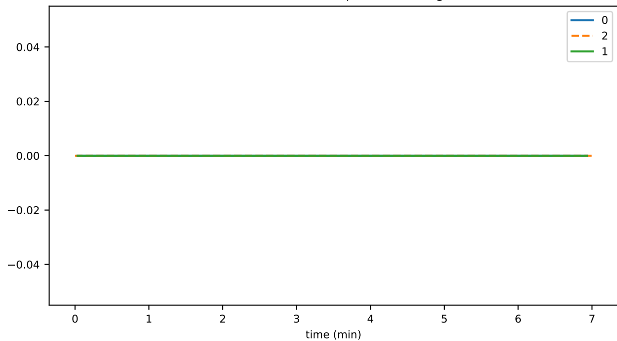
consensusCreateTopicDurationAvg
