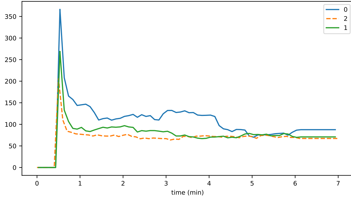
eventDelay_2_validation_runtime
