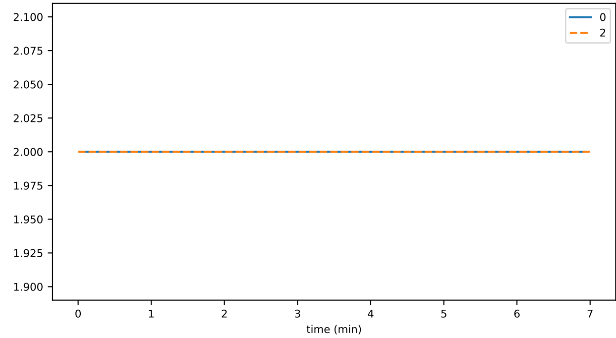
rpc_output_02_queueMaxSize
