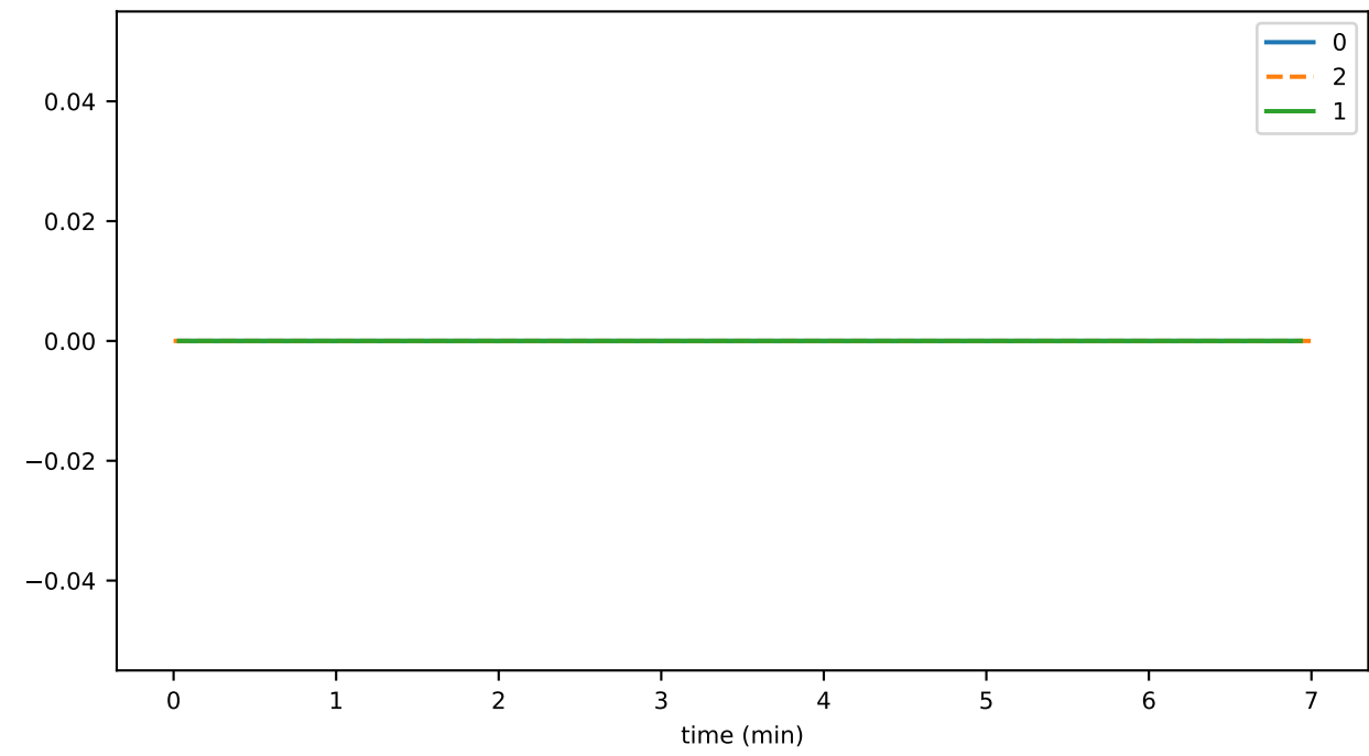
schedulesPercentUsed
