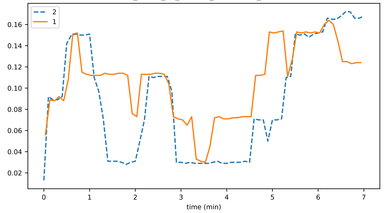
sync_phase_00_fraction_SENDING_EVENTS
