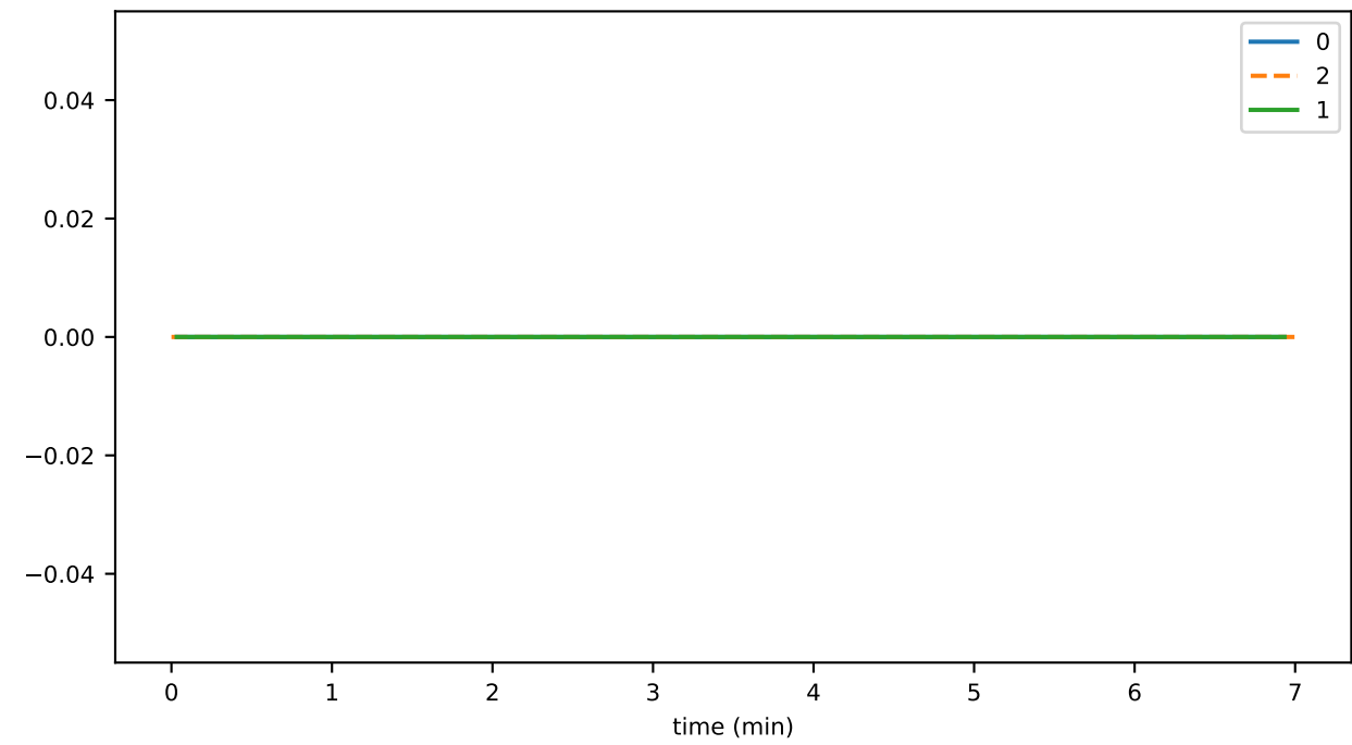
tokenFreezeAccountDurationAvg
