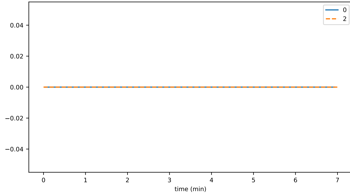
rpc_input_02_queueMinSize
