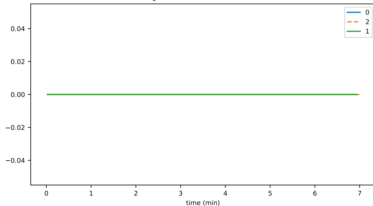
statesIneligibleForDeletion
