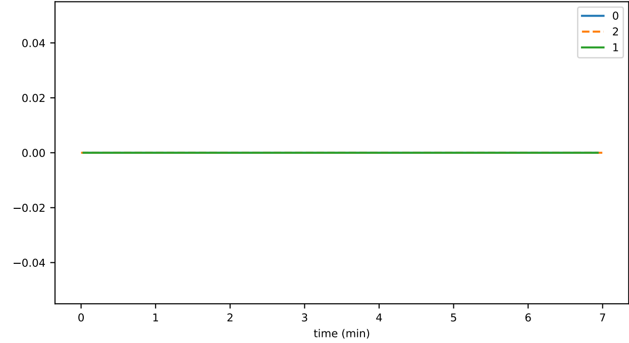
connRecv_latestBlockResendBlock
