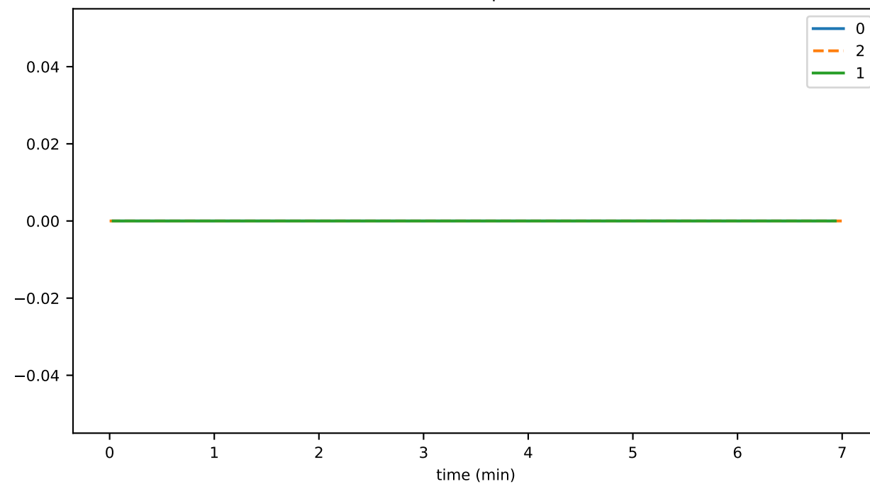
consensusCreateTopicDurationMax
