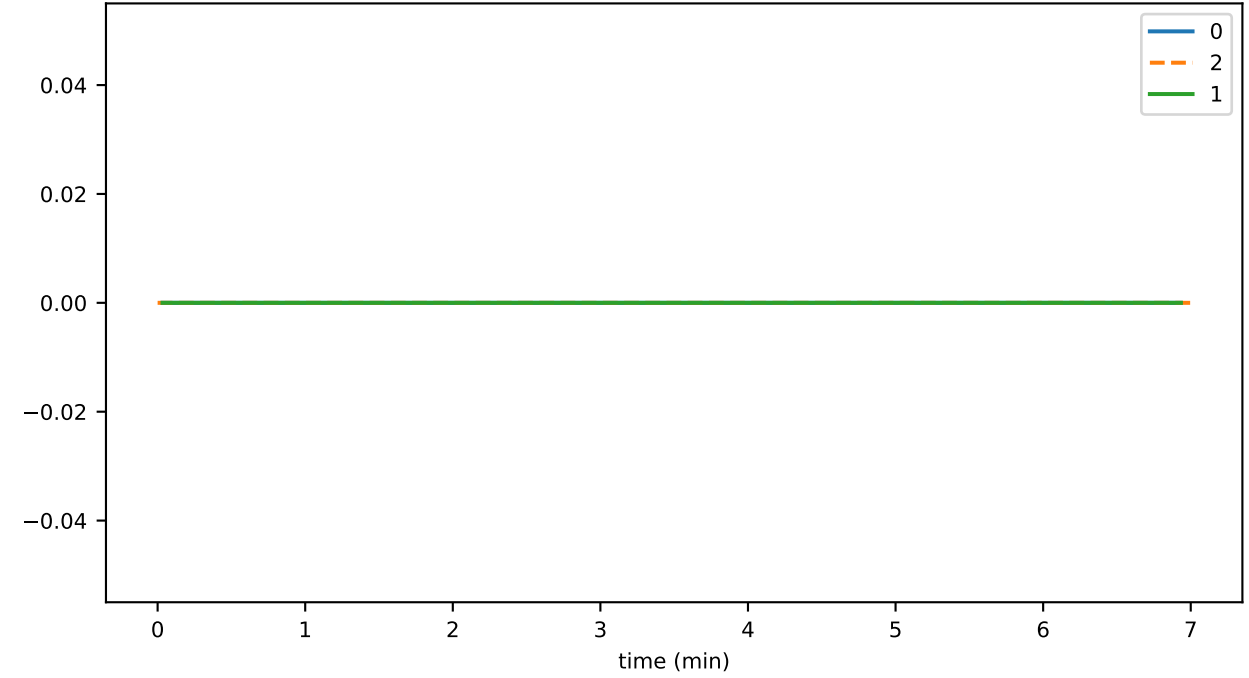
consensusGetTopicInfoDurationMax
