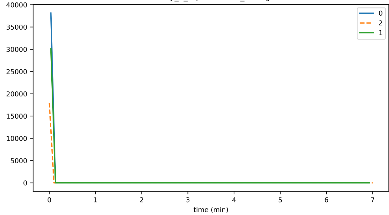
eventDelay_5_orphanBuffer_storageMAX
