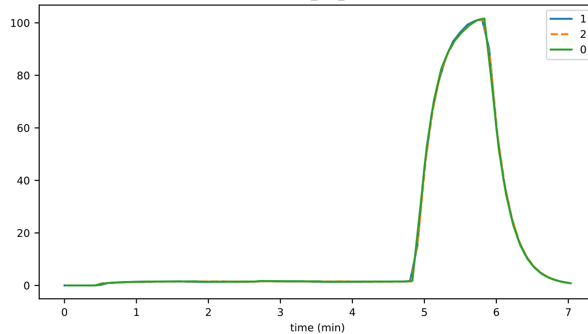
transH_per_sec
