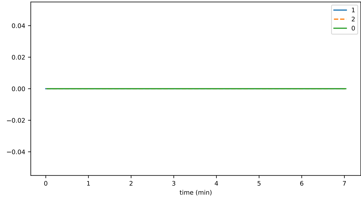
SmartContractService:SystemContractMethodCall_REJECT_failed
