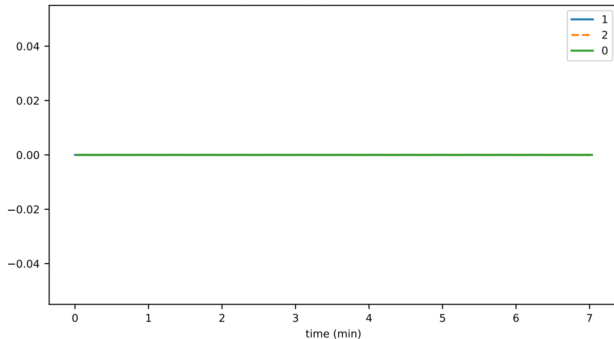
historyProofKeyPublicationDurationMax
