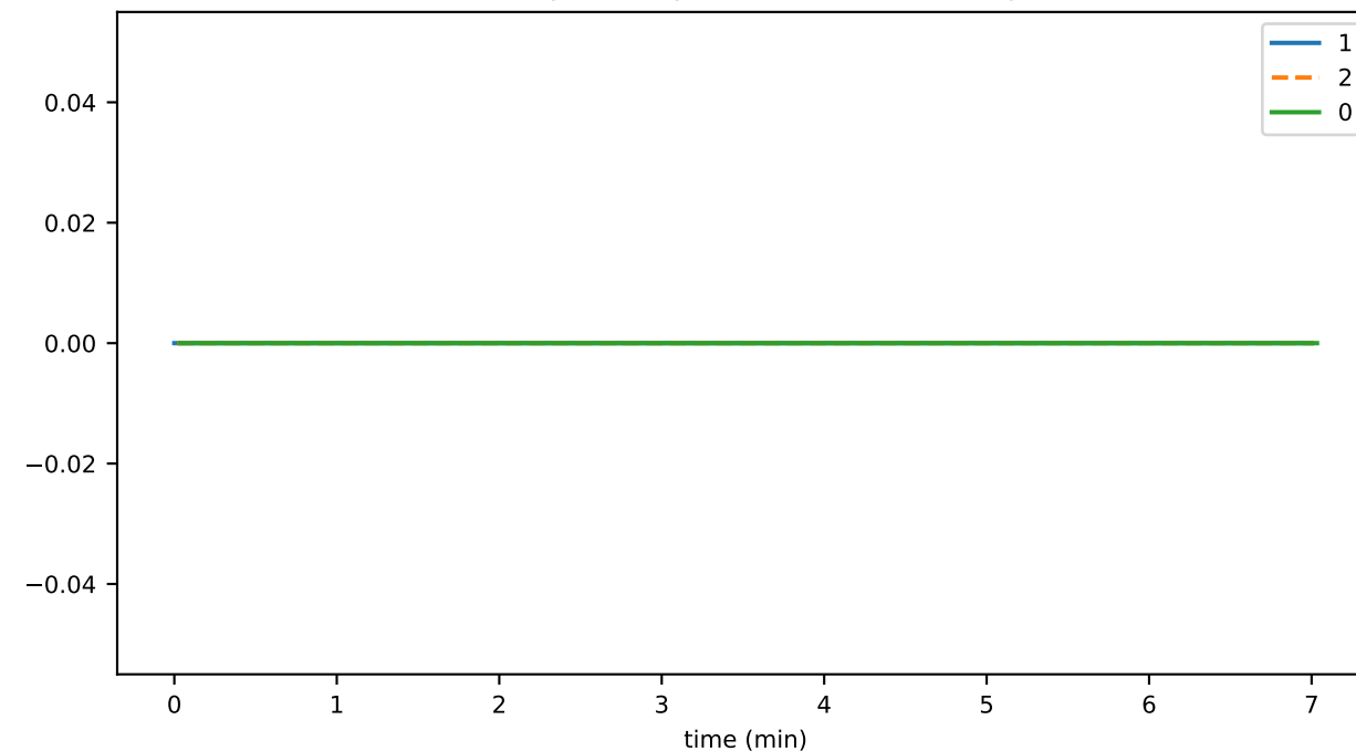
historyProofKeyPublicationThrottledTxns
