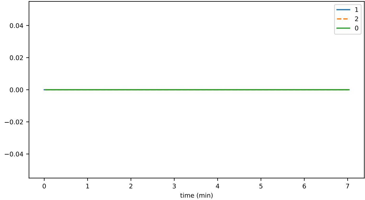
stateCopyMicros
