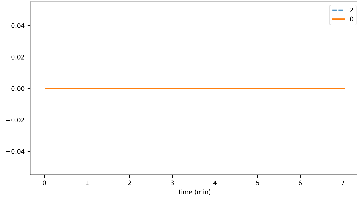
sync_phase_01_fraction_OUTSIDE_OF_RPC
