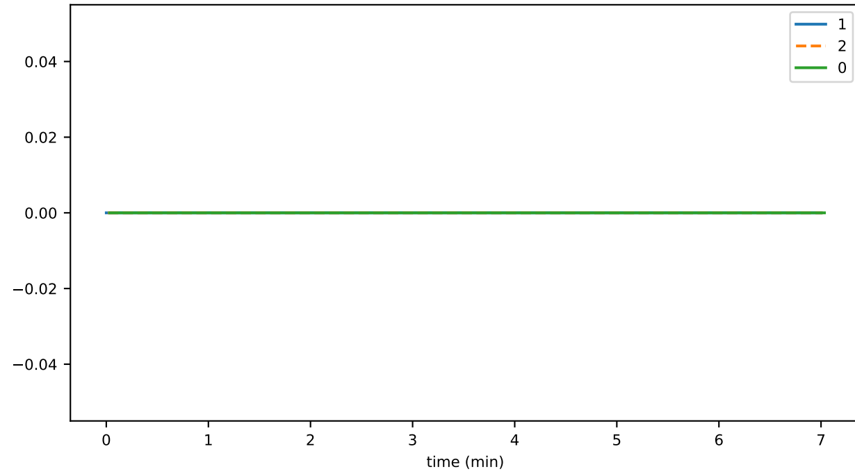
scheduleSignDurationAvg
