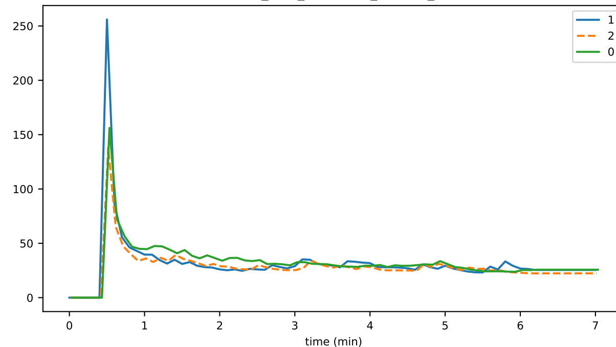
consensus_time_HANDLING_CONSENSUS_ROUND
