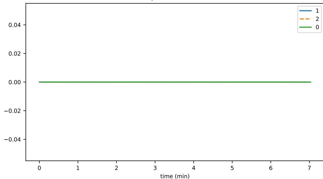
freezeDurationAvg
