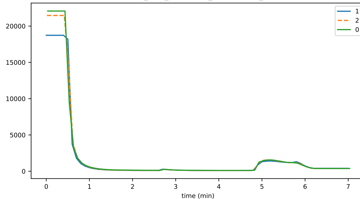
consensus_time_HANDLING_CONSENSUS_ROUND
