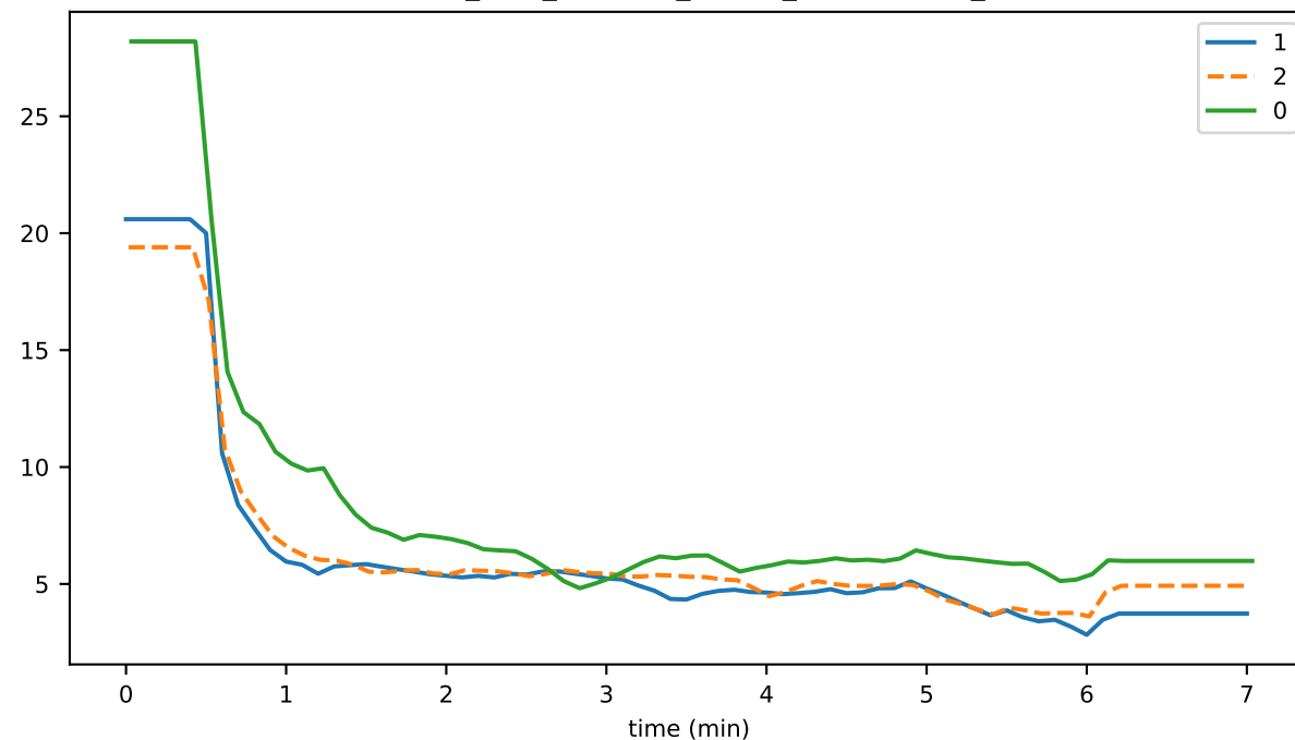
consensus_time_UPDATING_PLATFORM_STATE_RUNNING_HASH
