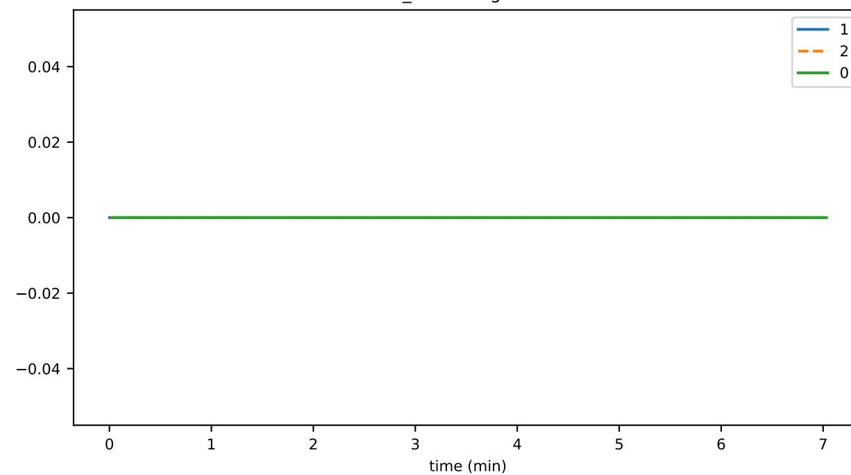
connSend_streamingBlockNumber
