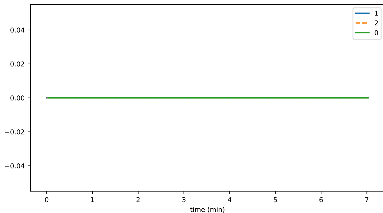
uNRECOGNIZEDThrottledTxns
