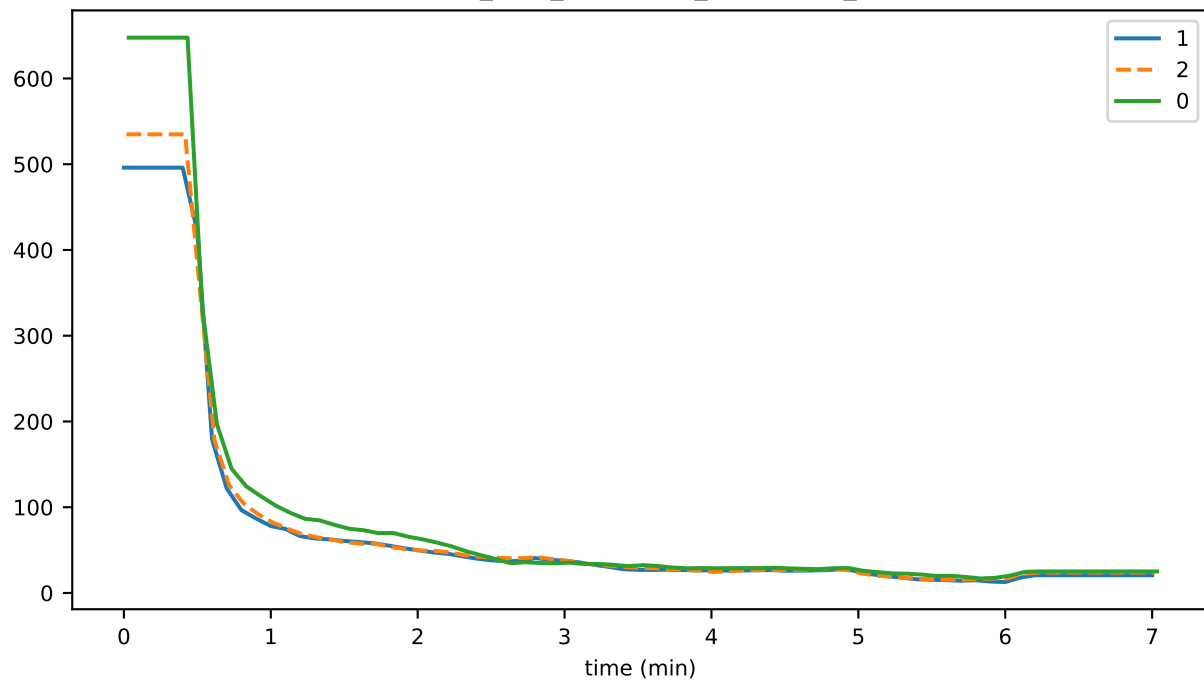
consensus_time_UPDATING_PLATFORM_STATE
