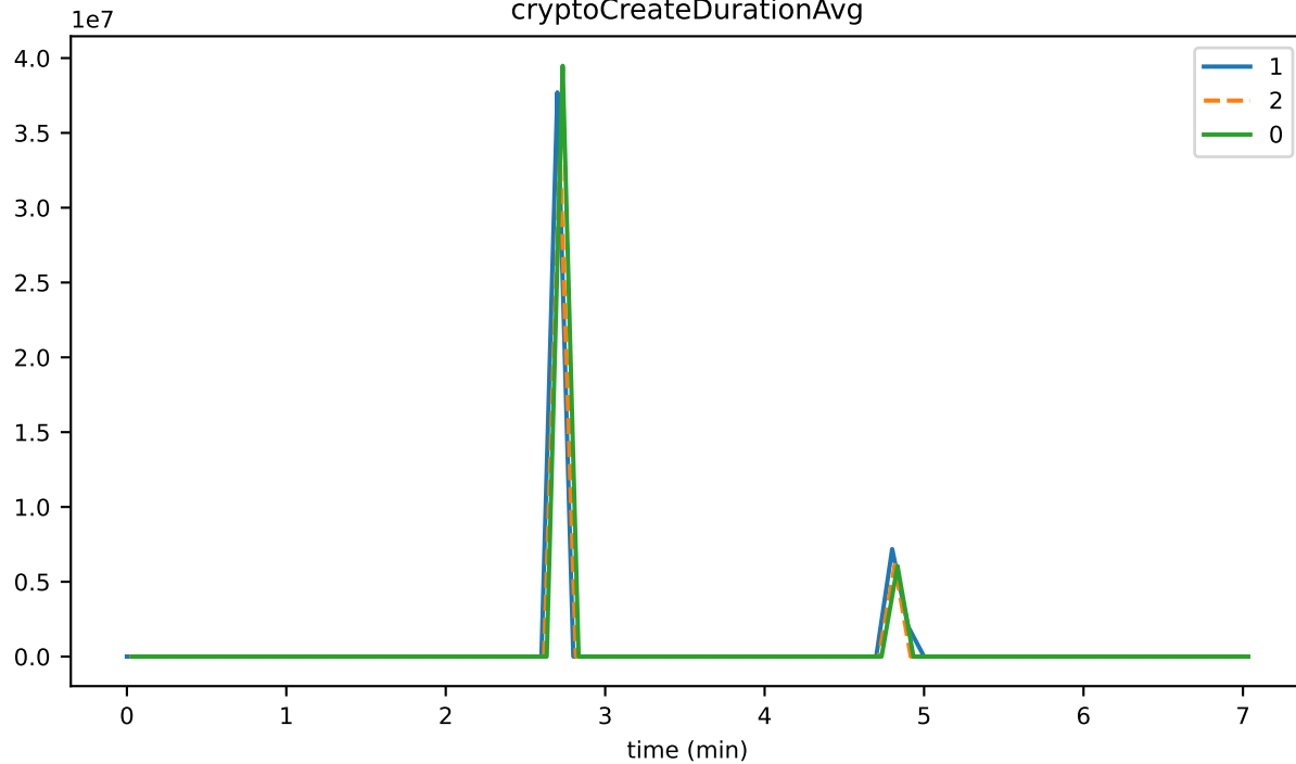
cryptoCreateDurationAvg
