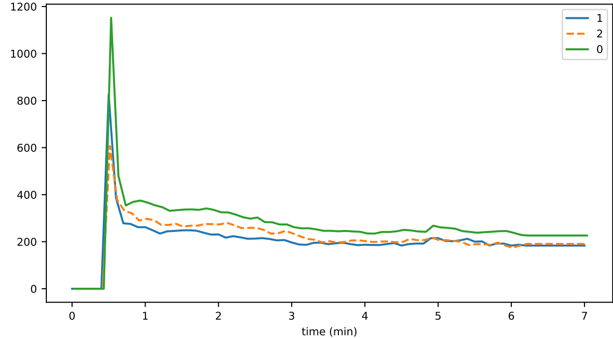
eventDelay_4_verification_gossip
