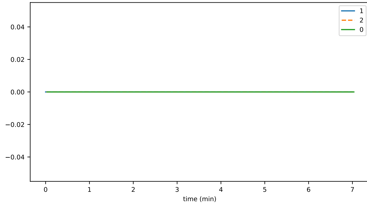
conn_activeConnIp
