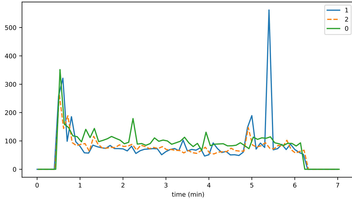
eventDelay_1_hashing_storageMAX
