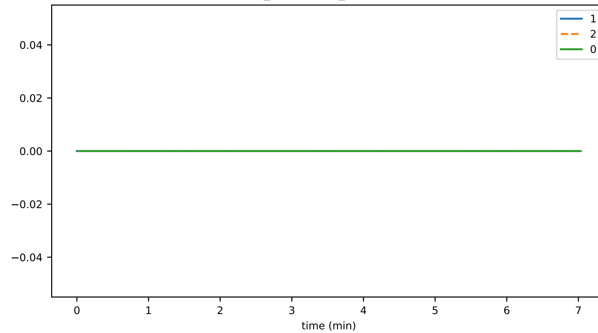
connRecv_endStream_persistenceFailed
