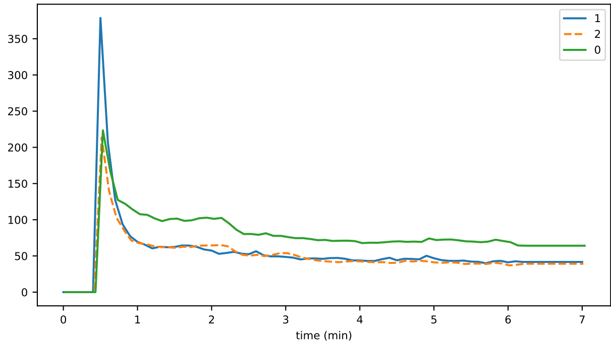
eventDelay_5_orphanBuffer_runtime
