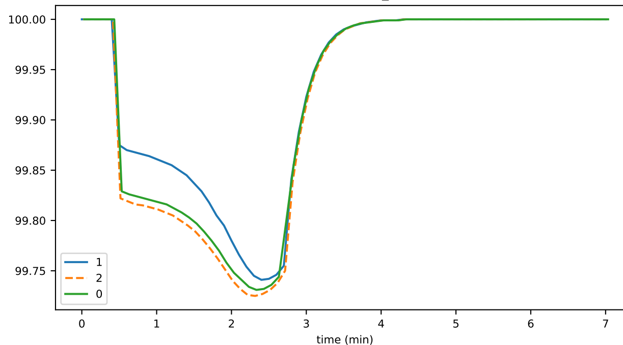
nodeActivePercentSnapshot_node0
