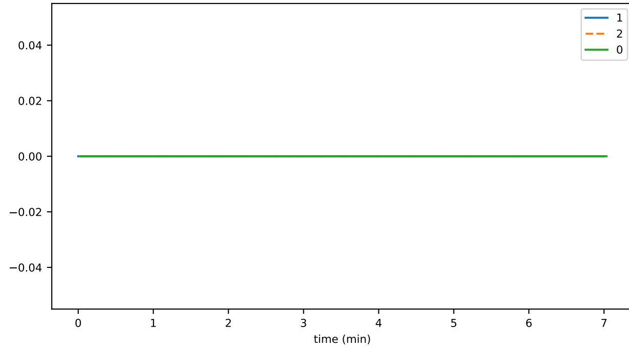
ds_offheap_objectKeyBucketsIndexMb_state
