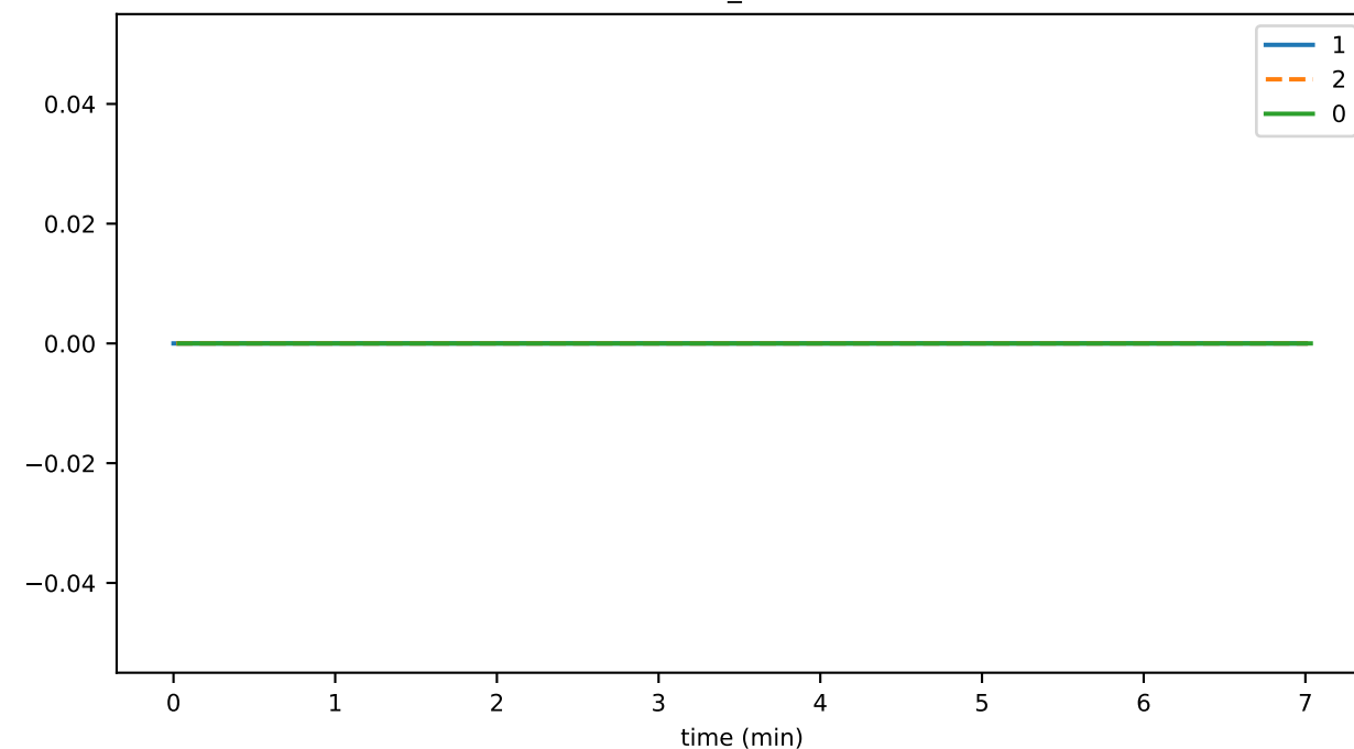
connSend_endStream_error
