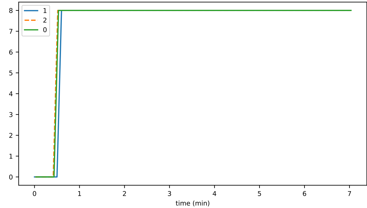
ds_reads_hashes_state
