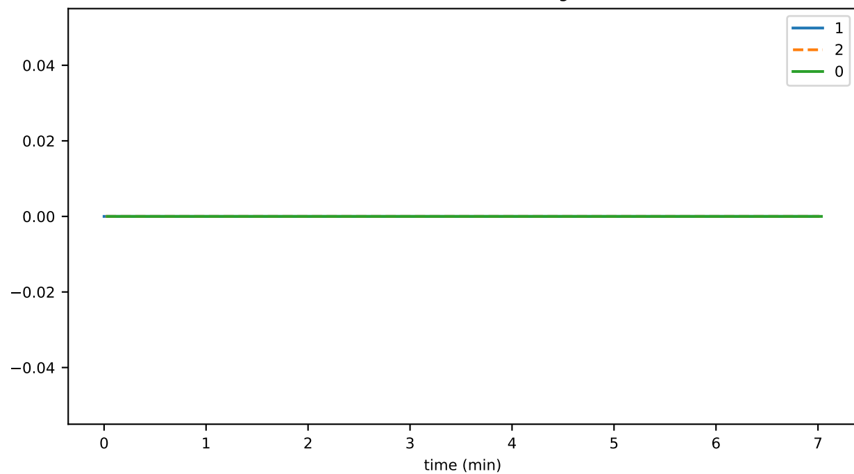
nodeCreateDurationAvg
