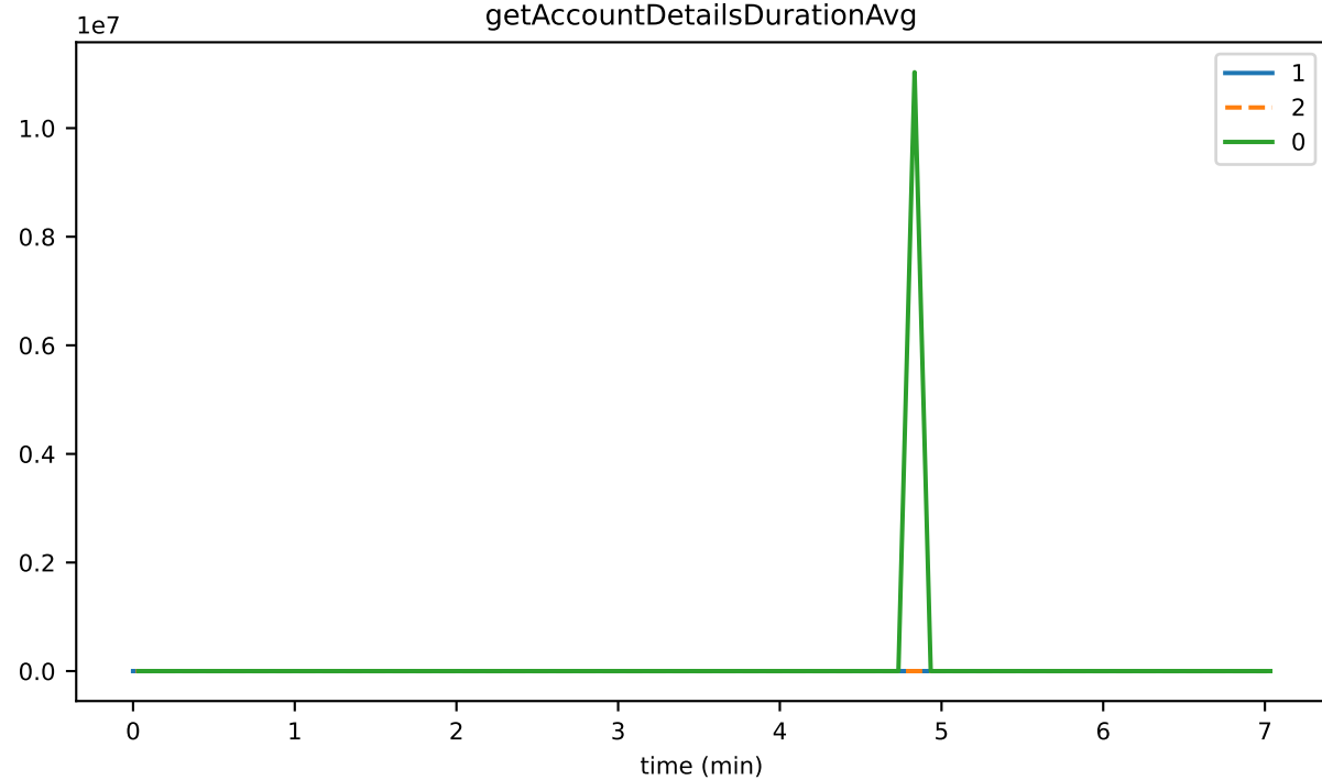
getAccountDetailsDurationAvg
