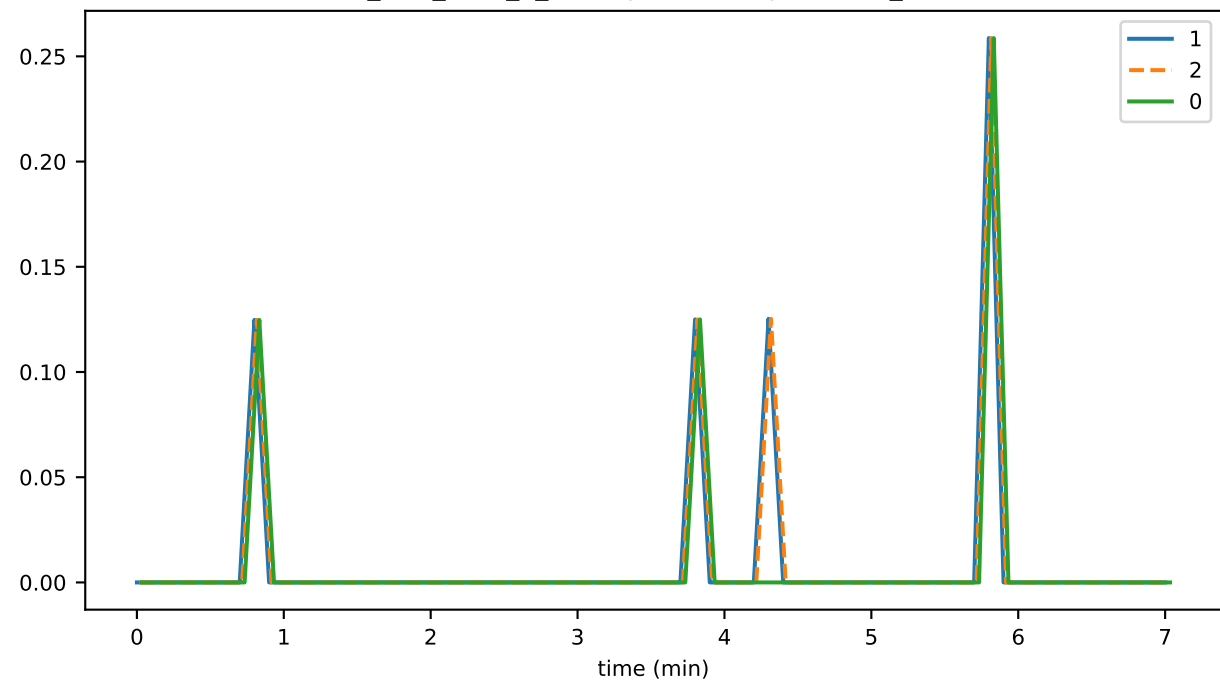
ds_files_level_2_hashesFileSizeByLevelMb_state
