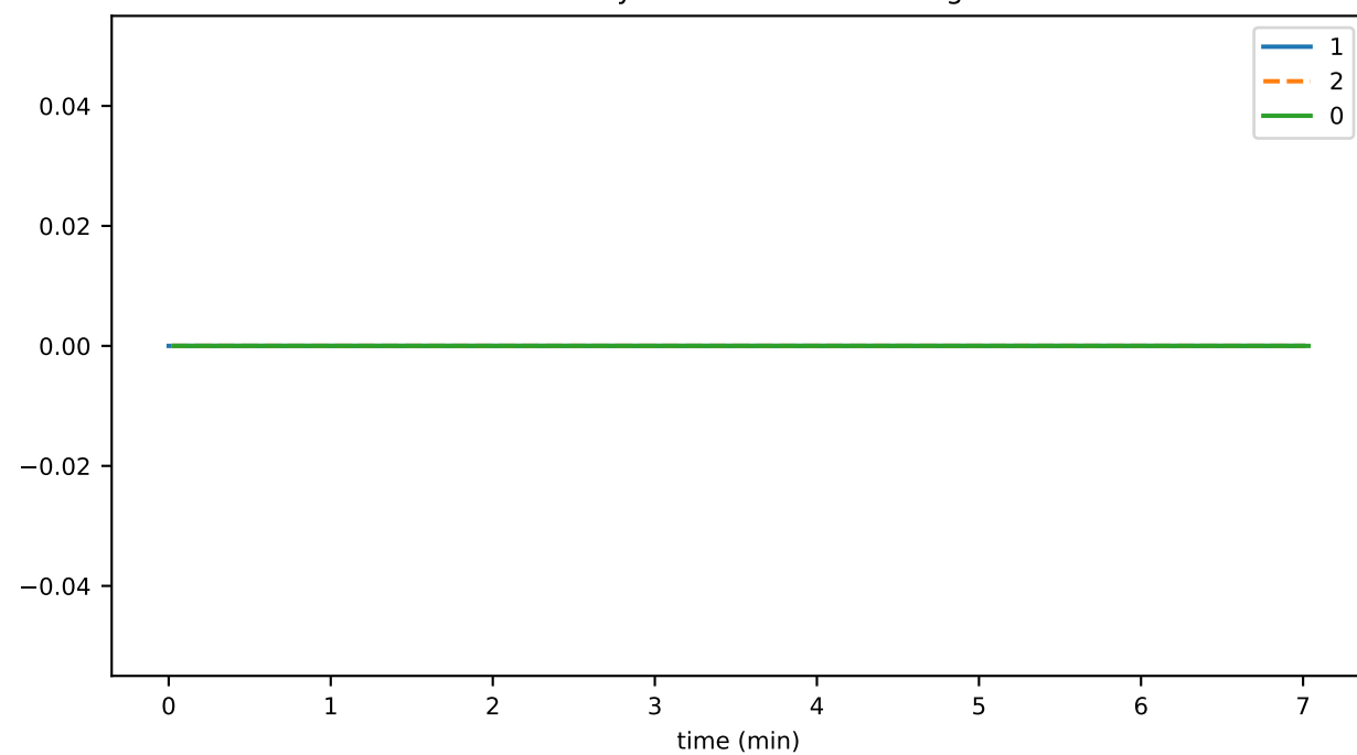
hintsKeyPublicationDurationAvg
