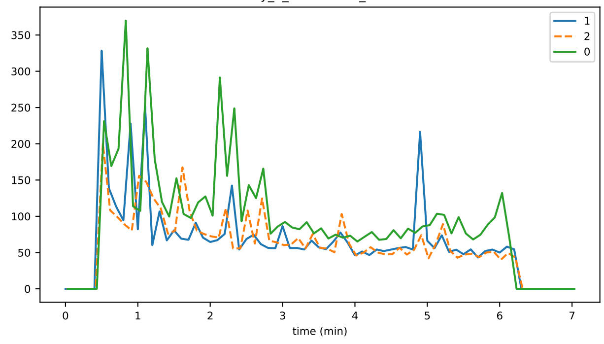
eventDelay_4_verification_runtimeMAX
