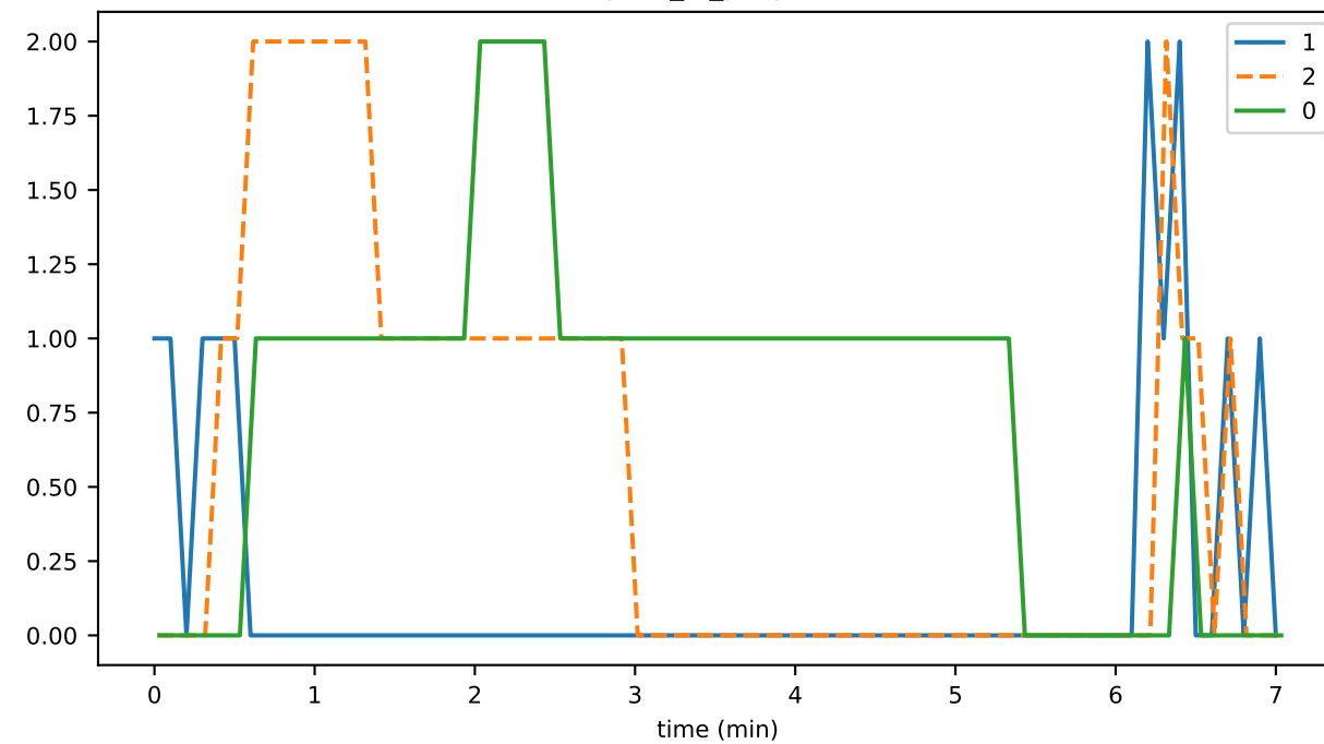
systemDeleteDurationAvg
