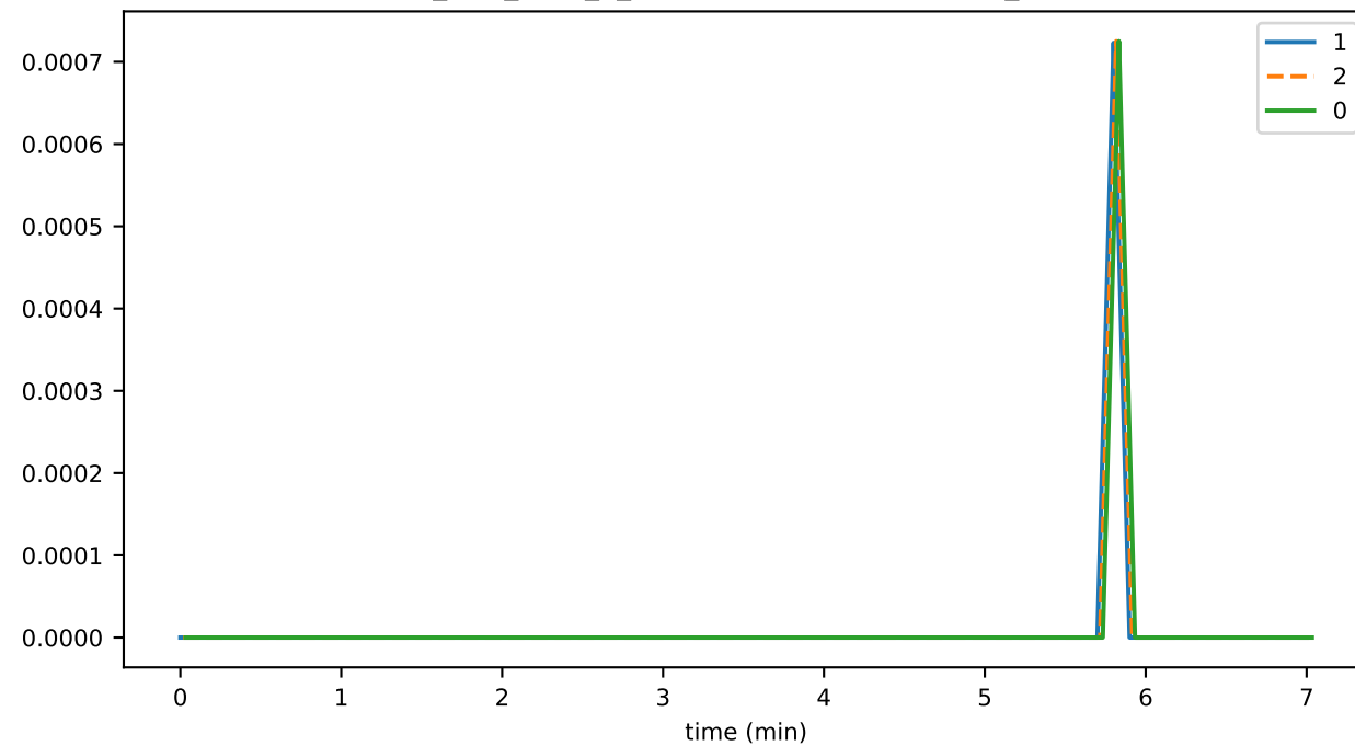
ds_files_level_2_leafKeysFileSizeByLevelMb_state
