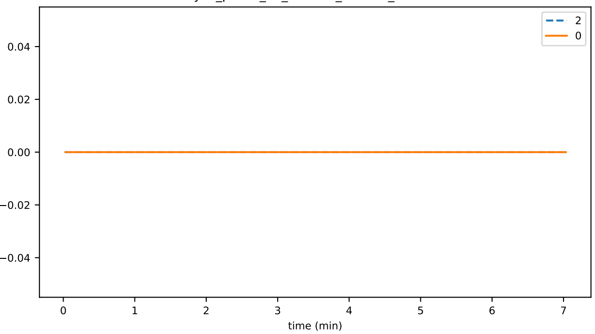
sync_phase_01_fraction_GOSSIP_HALTED
