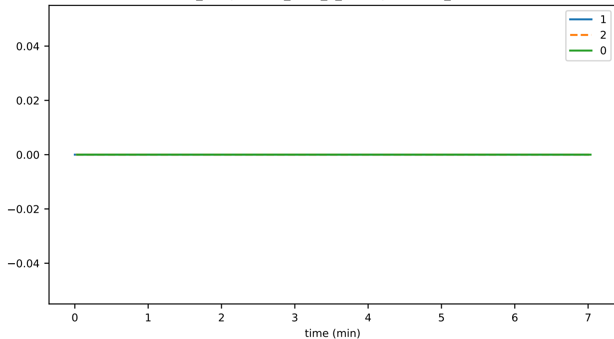
ds_compactions_level_3_leavesTimeMs_state
