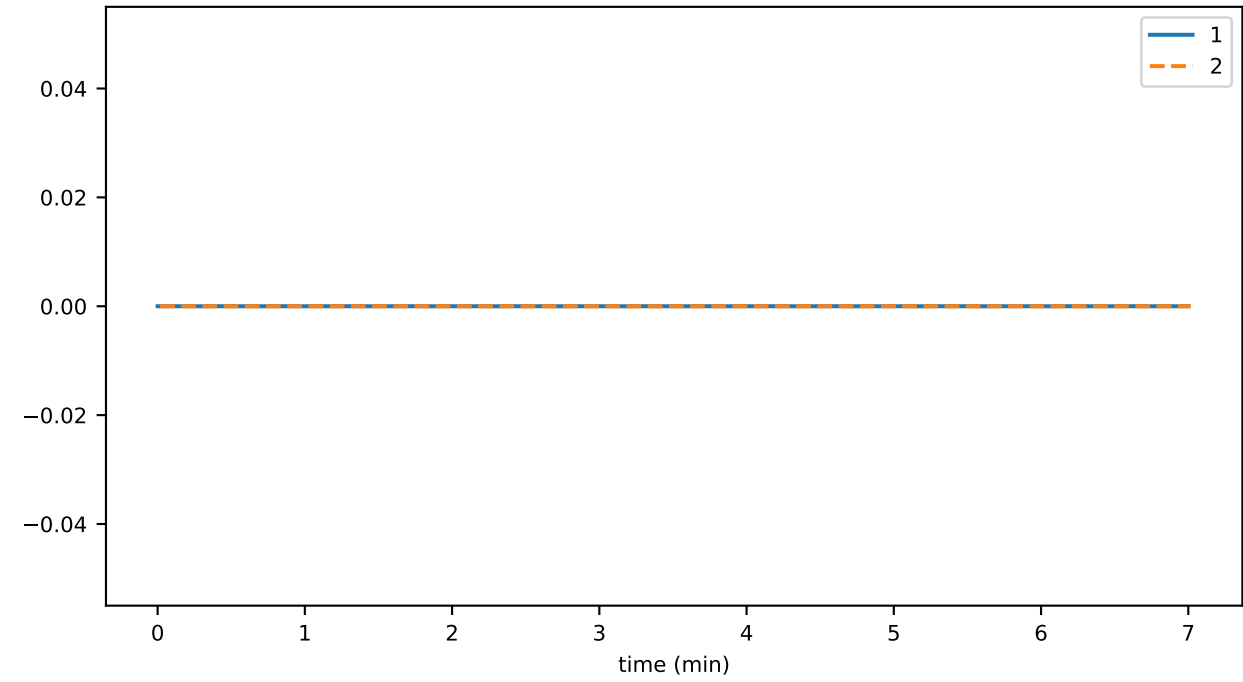
reconnectRejections_per_sec_02
