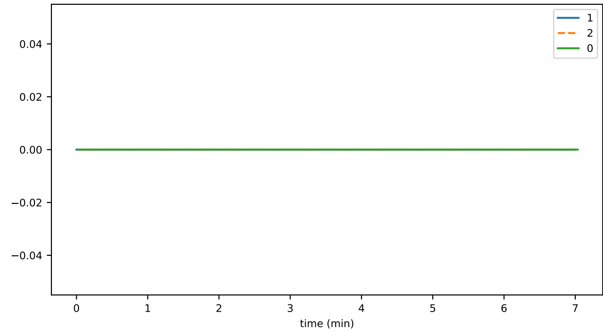
connRecv_unknown
