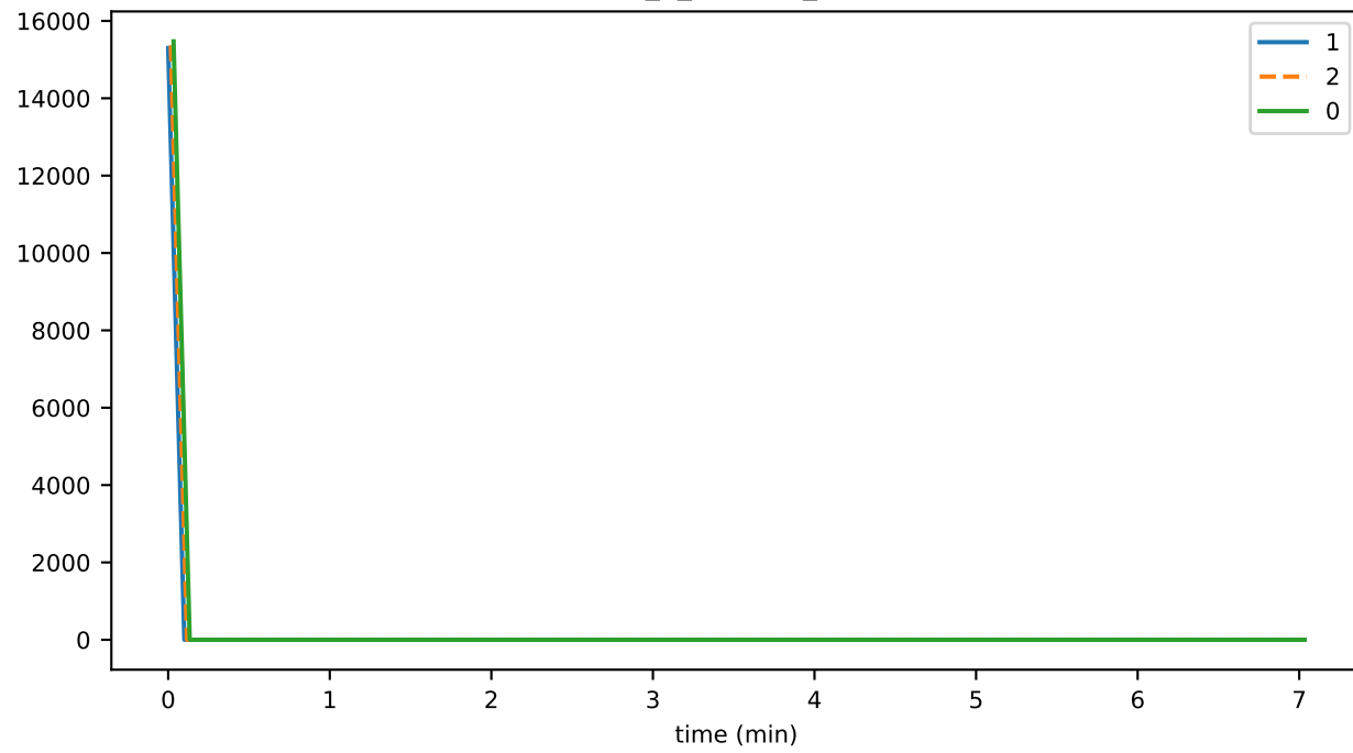
eventDelay_1_hashing_storageMAX
