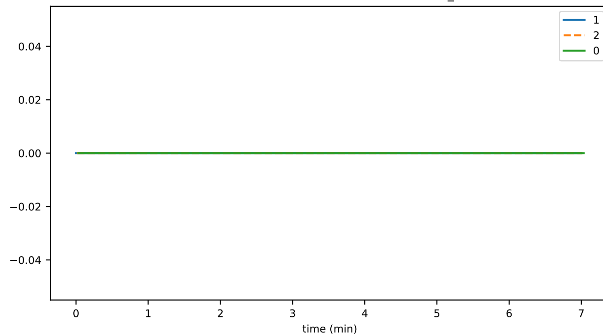
SmartContractService:TransactionGasUsed_count
