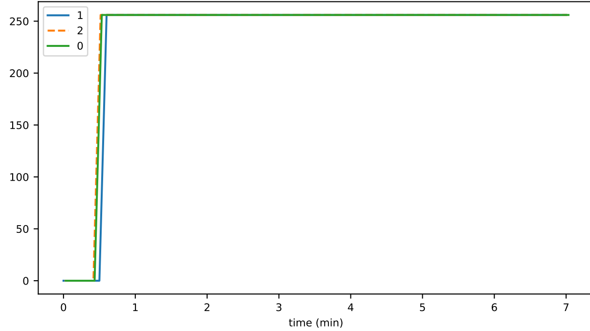
ds_offheap_objectKeyBucketsIndexMb_state
