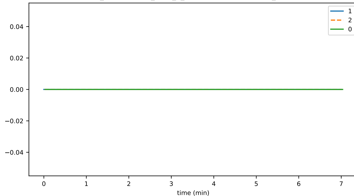
ds_compactions_level_3_leafKeysSavedSpaceMb_state
