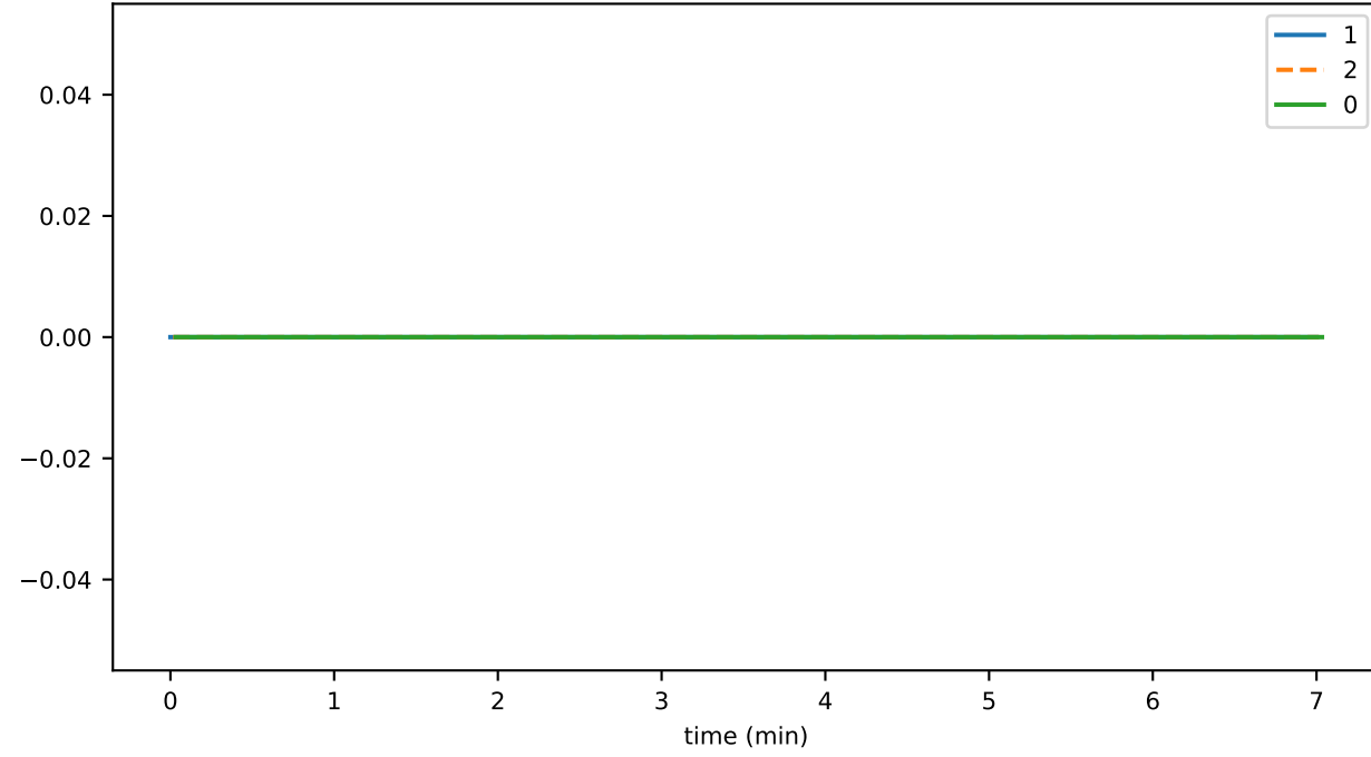
nodeStakeUpdateDurationMax
