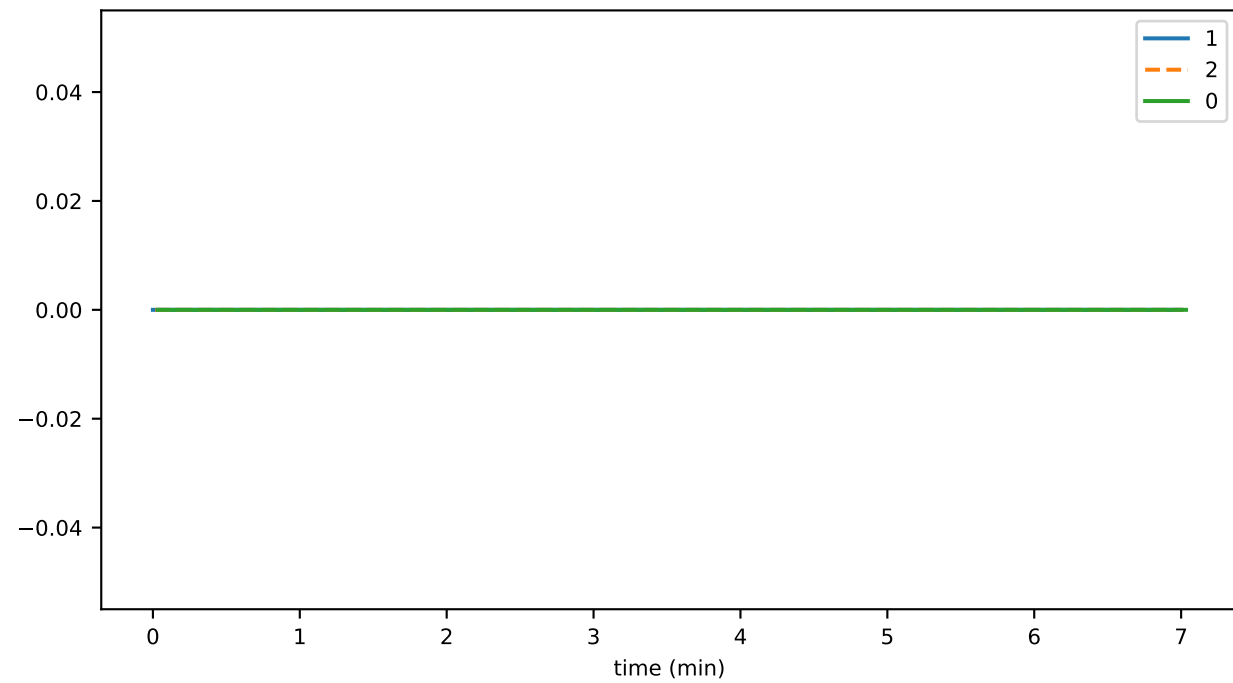
stateSignatureAge
