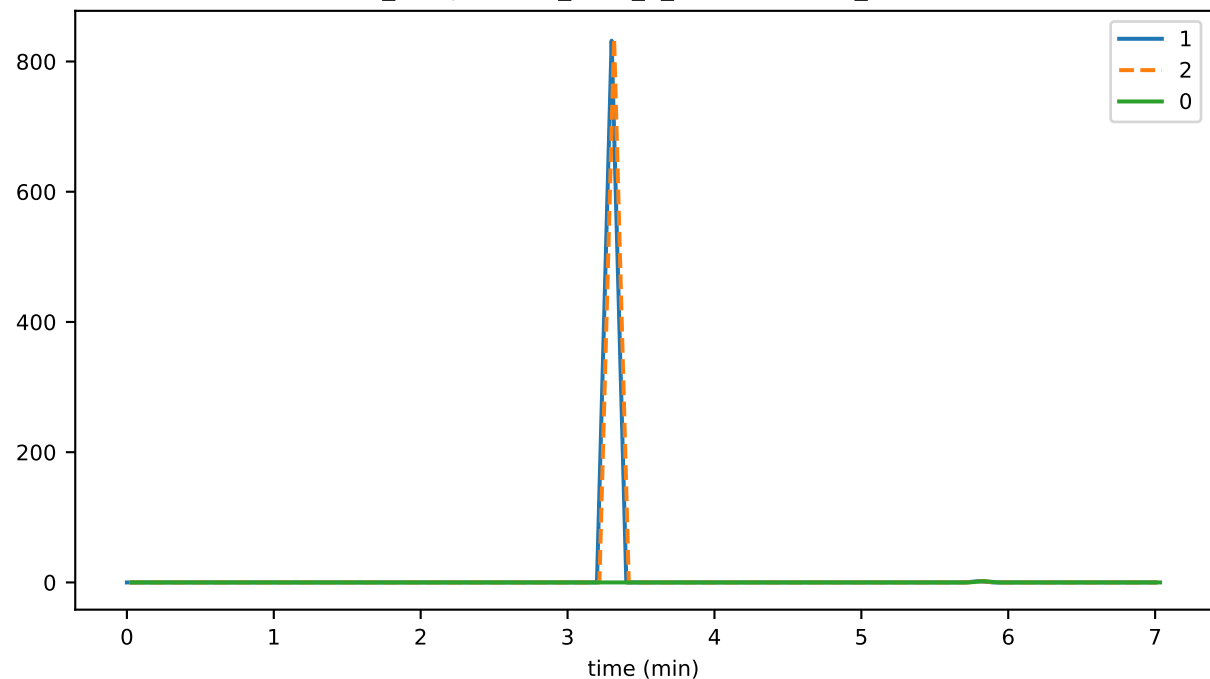
ds_compactions_level_3_hashesTimeMs_state
