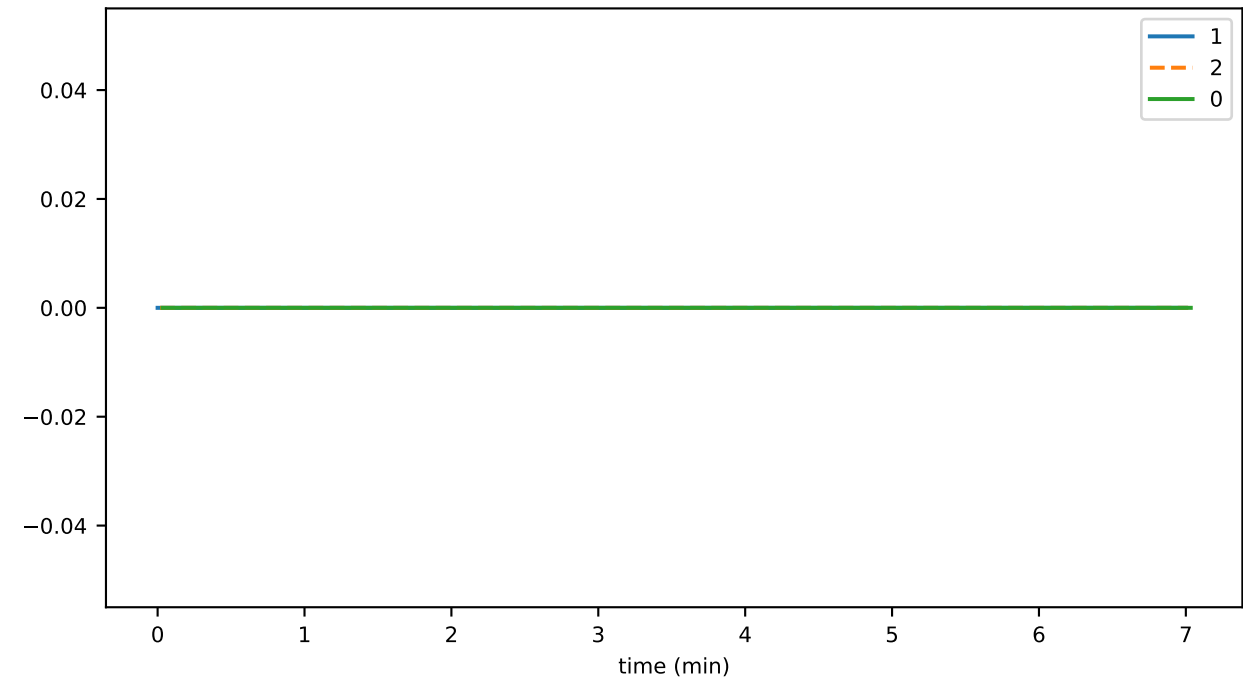
SmartContractService:SystemContractMethodCall_REJECT_failed
