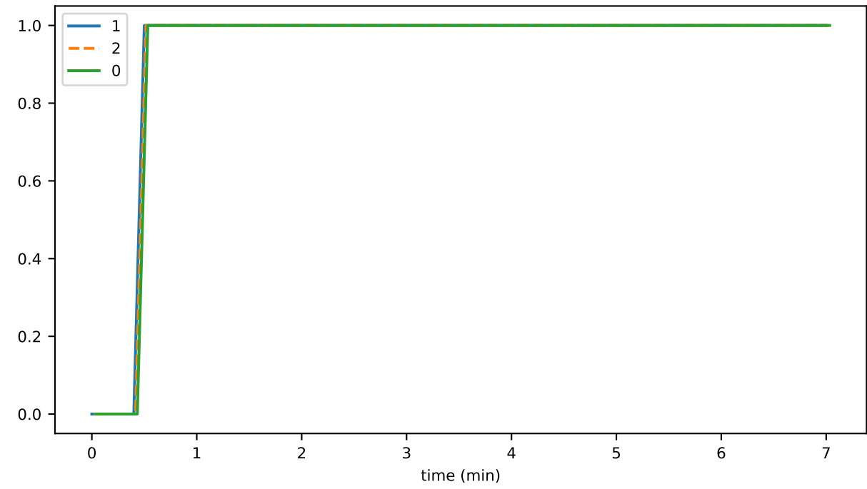
totalNeverSignedStates
