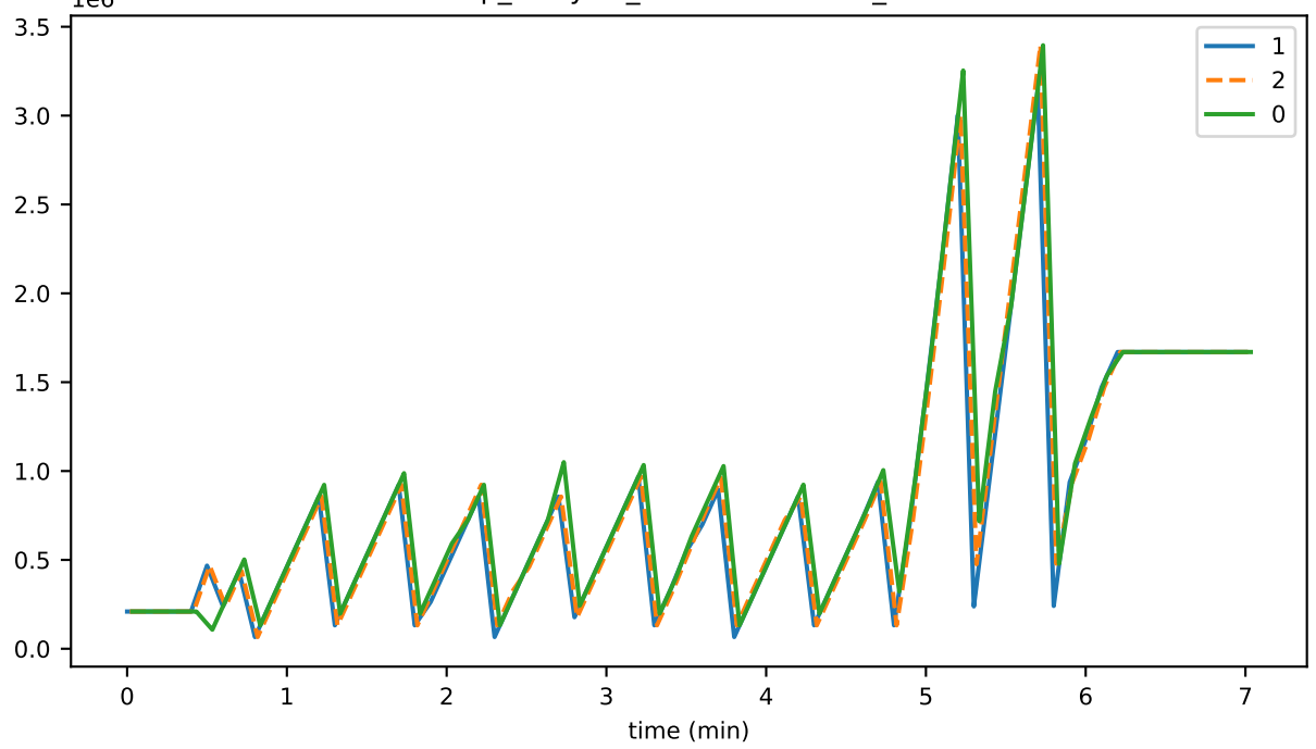
vmap_lifecycle_nodeCacheSizeB_state
