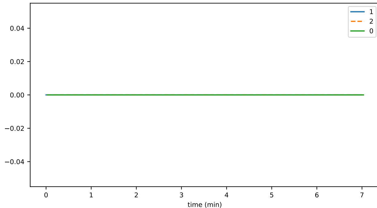
uncheckedSubmitThrottledTxns
