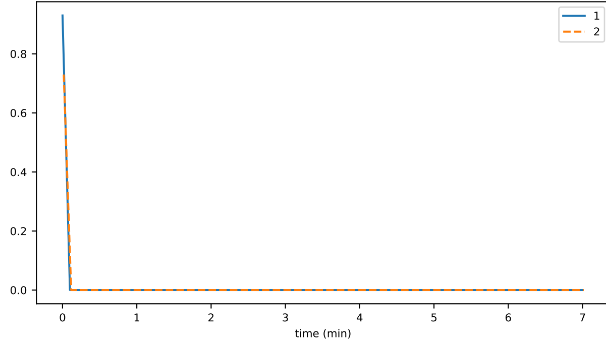
sync_phase_00_fraction_OUTSIDE_OF_RPC
