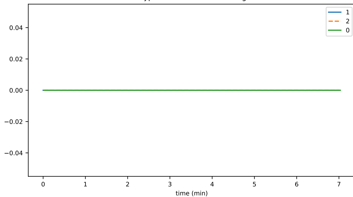
cryptoGetStakersDurationAvg
