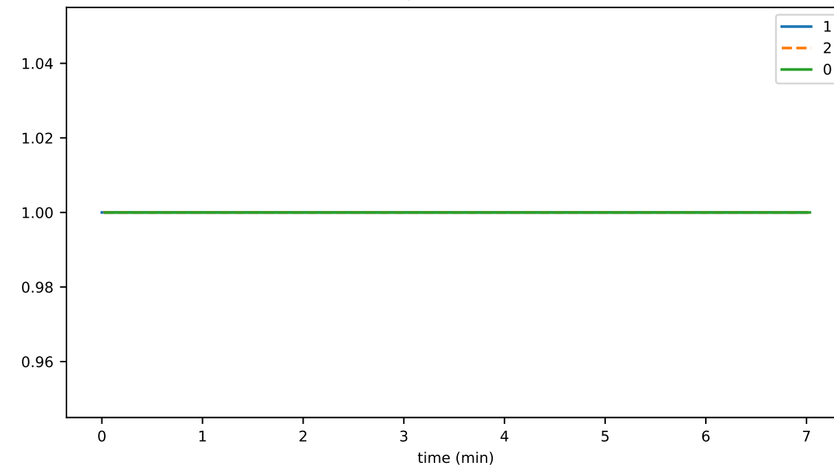
hintsKeyPublicationDurationMax
