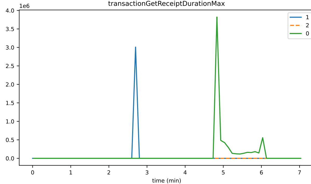
transactionGetReceiptDurationMax
