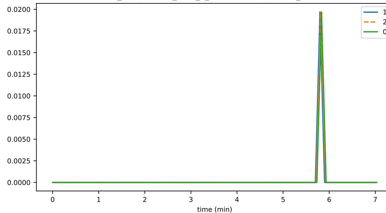
ds_compactions_level_4_hashesSavedSpaceMb_state
