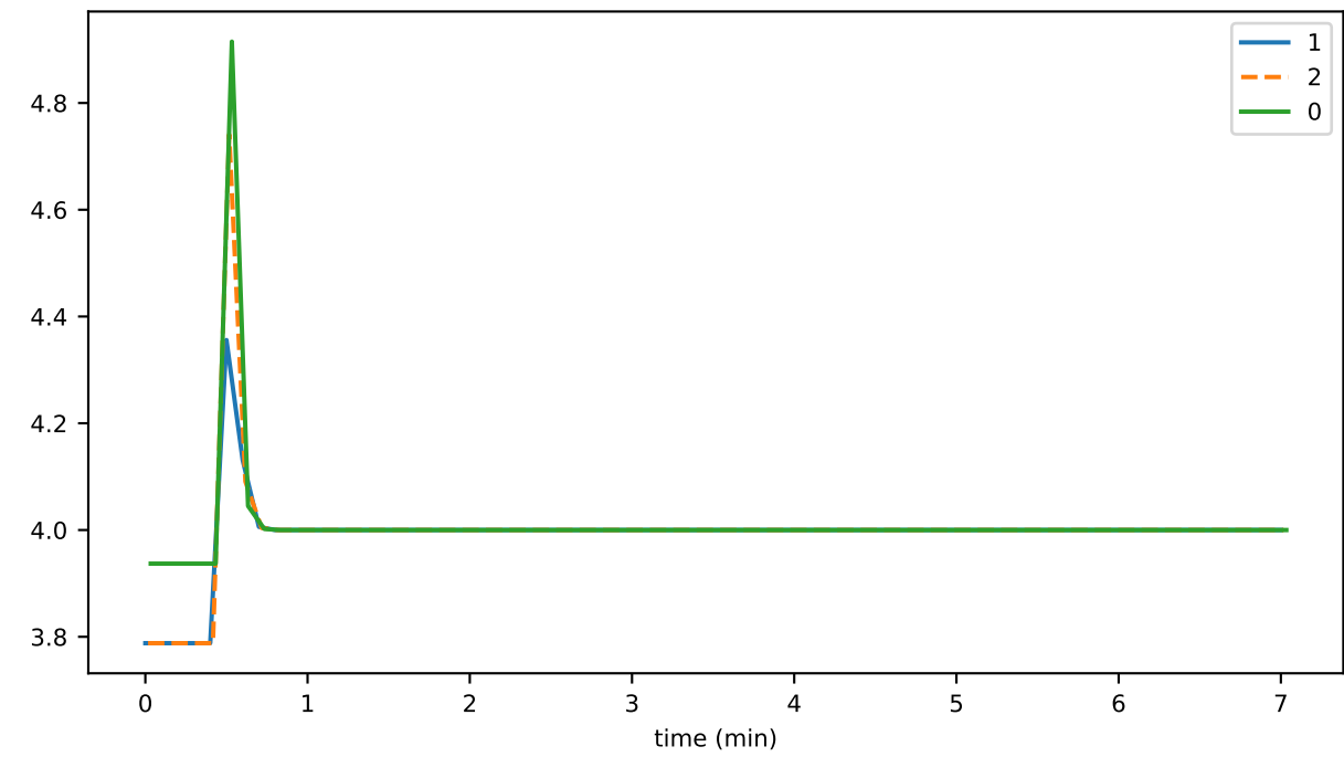
graphDepthUntilConsensus
