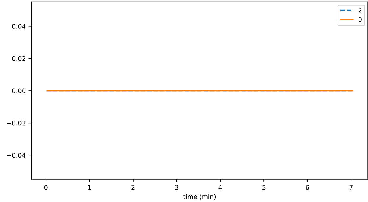
sync_phase_01_fraction_PLATFORM_STATUS_PREVENTING_SYNC
