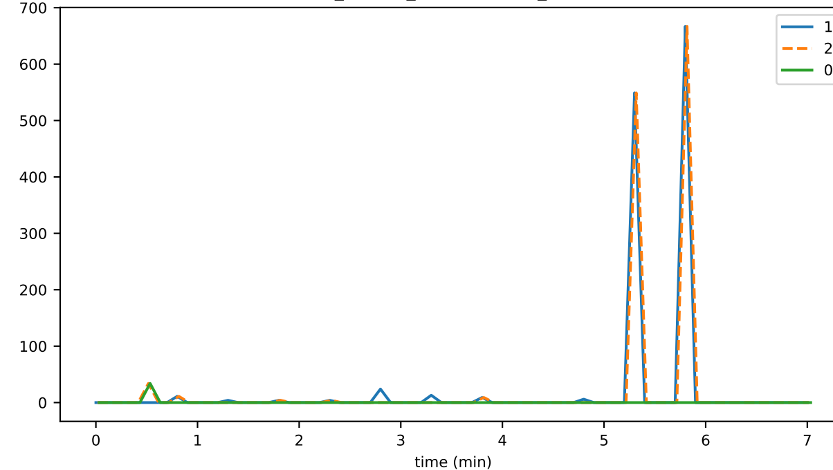
ds_offheap_hashesIndexMb_state
