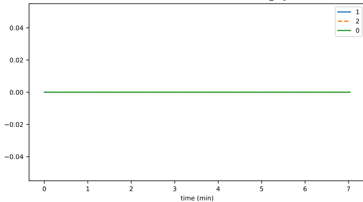
SmartContractService:TransactionGasUsed_avg
