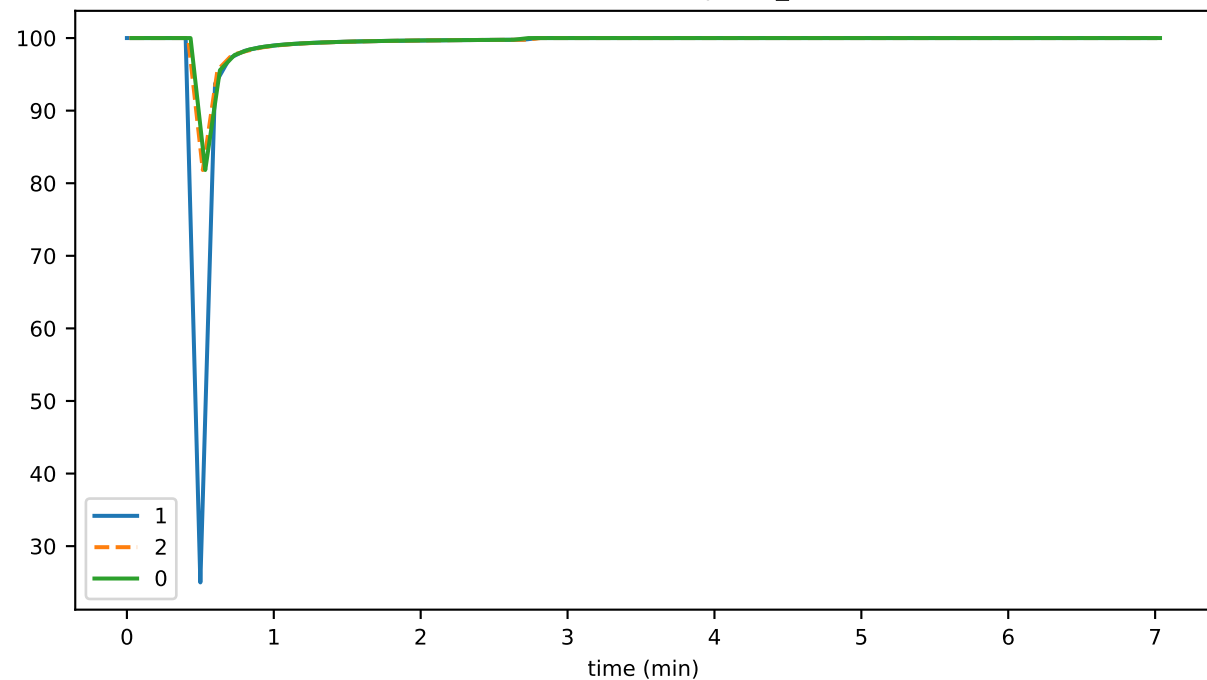
nodeCreateDurationAvg
