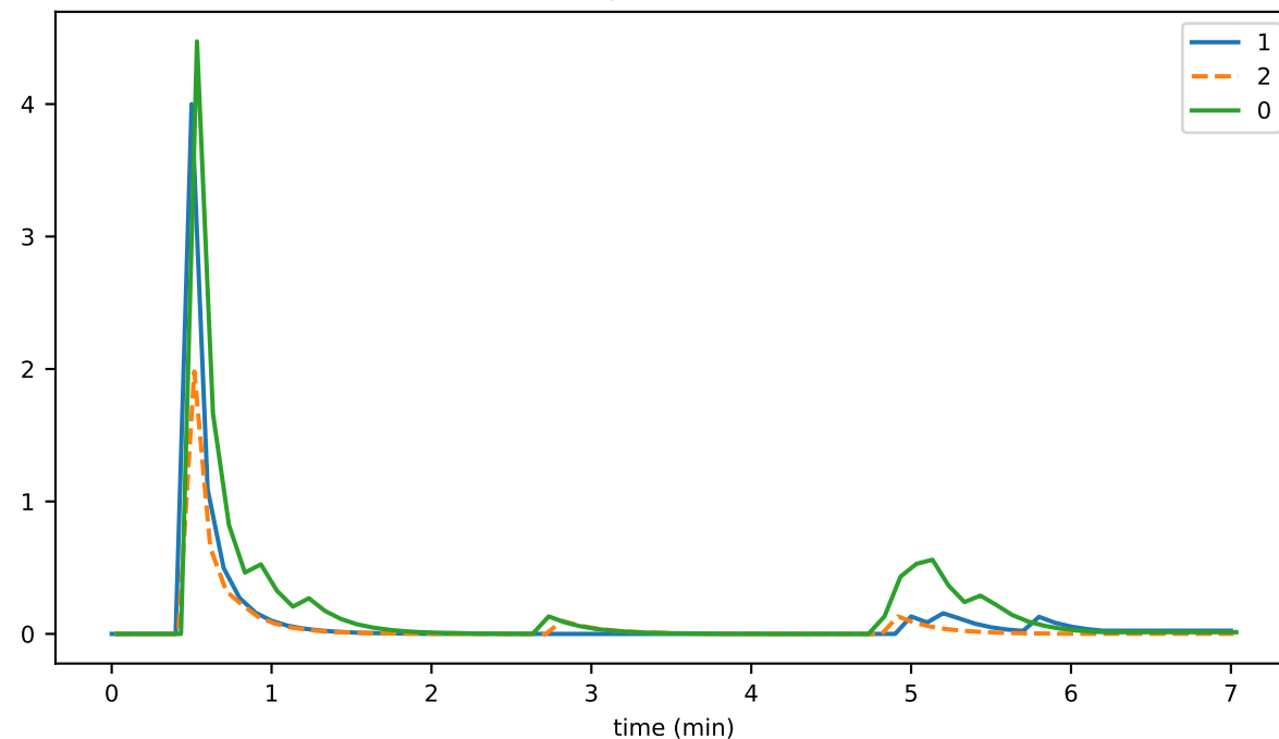
SigVal_per_sec
