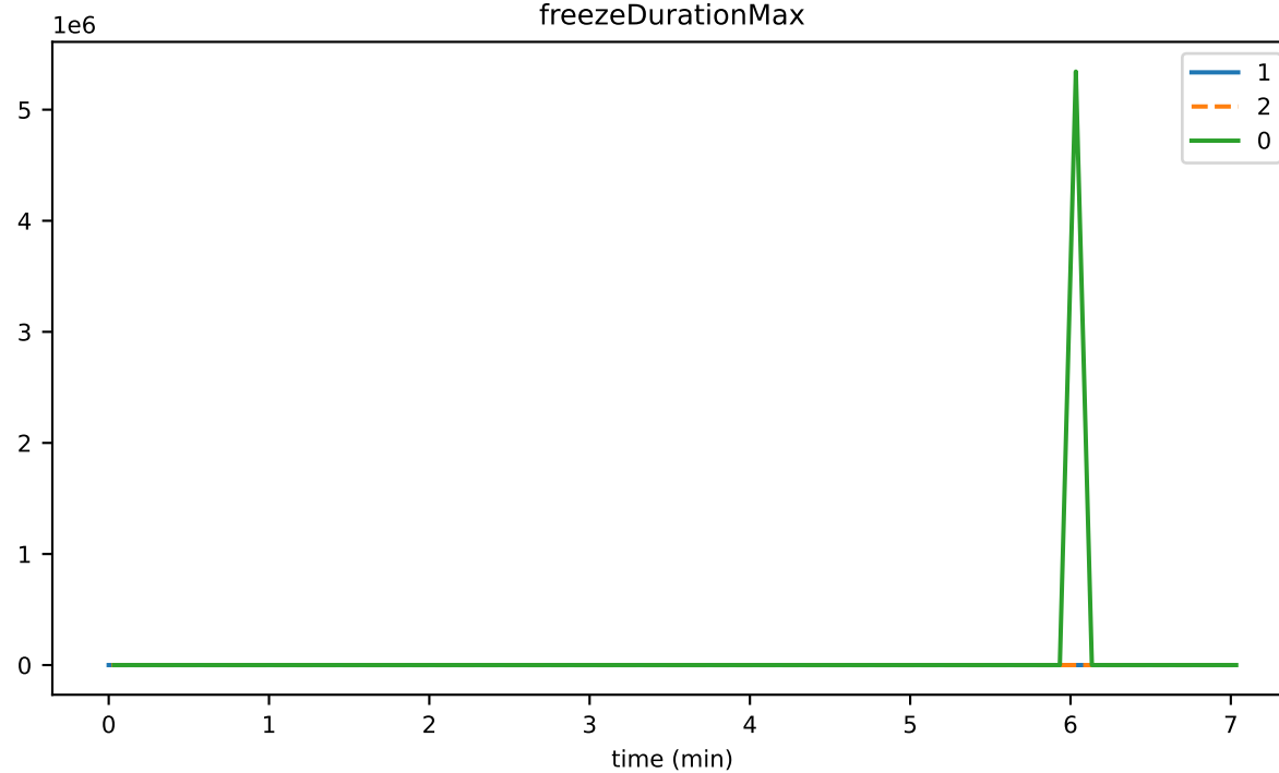
freezeDurationMax
