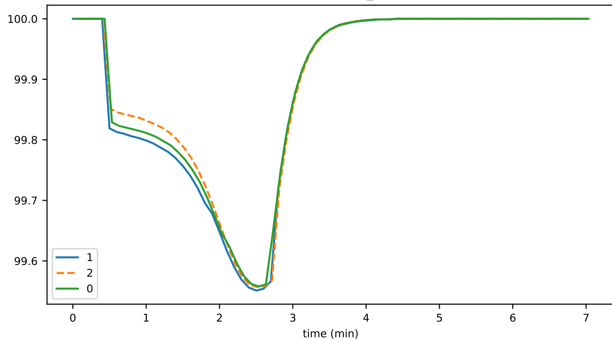
nodeActivePercent_node2
