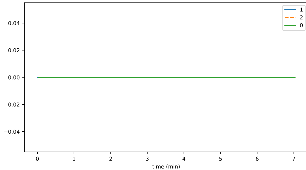
connRecv_endStream_invalidRequest
