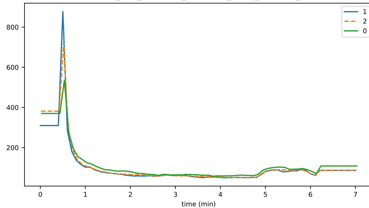
consensus_time_UPDATING_PLATFORM_STATE_RUNNING_HASH
