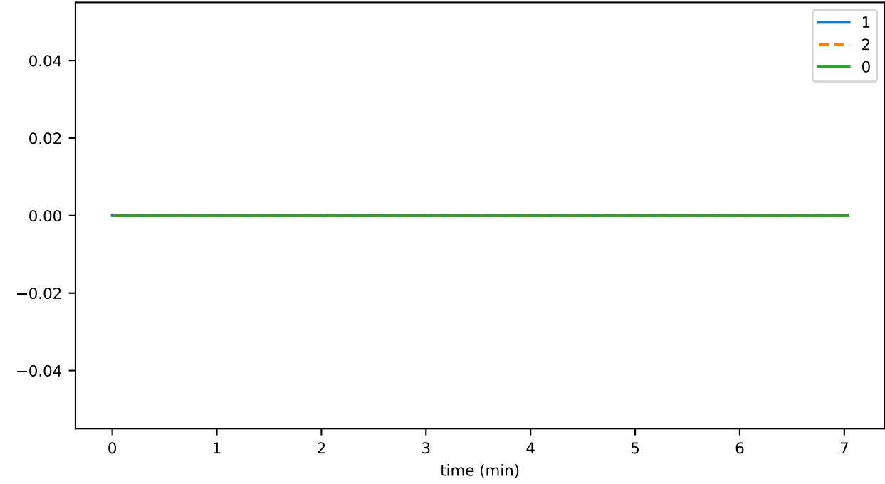
scheduleSignDurationMax
