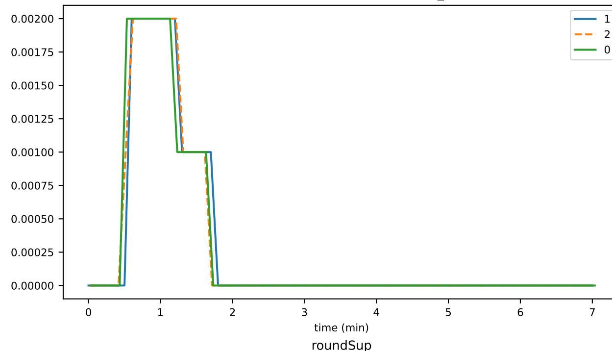
roundsSinceLastConsensusEvent_1
