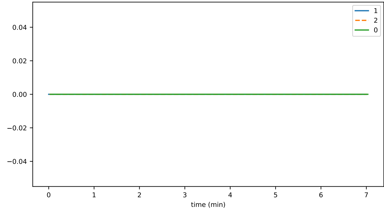
scheduleSignDurationMax
