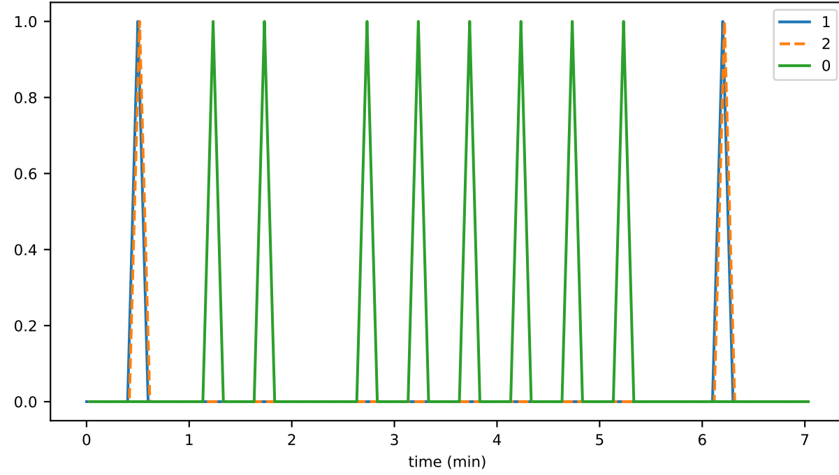
StateSnapshotManager_unhandled_task_count
