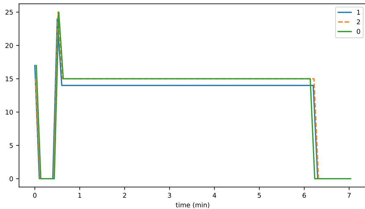
numEventsAddedUntilConsensusMAX
