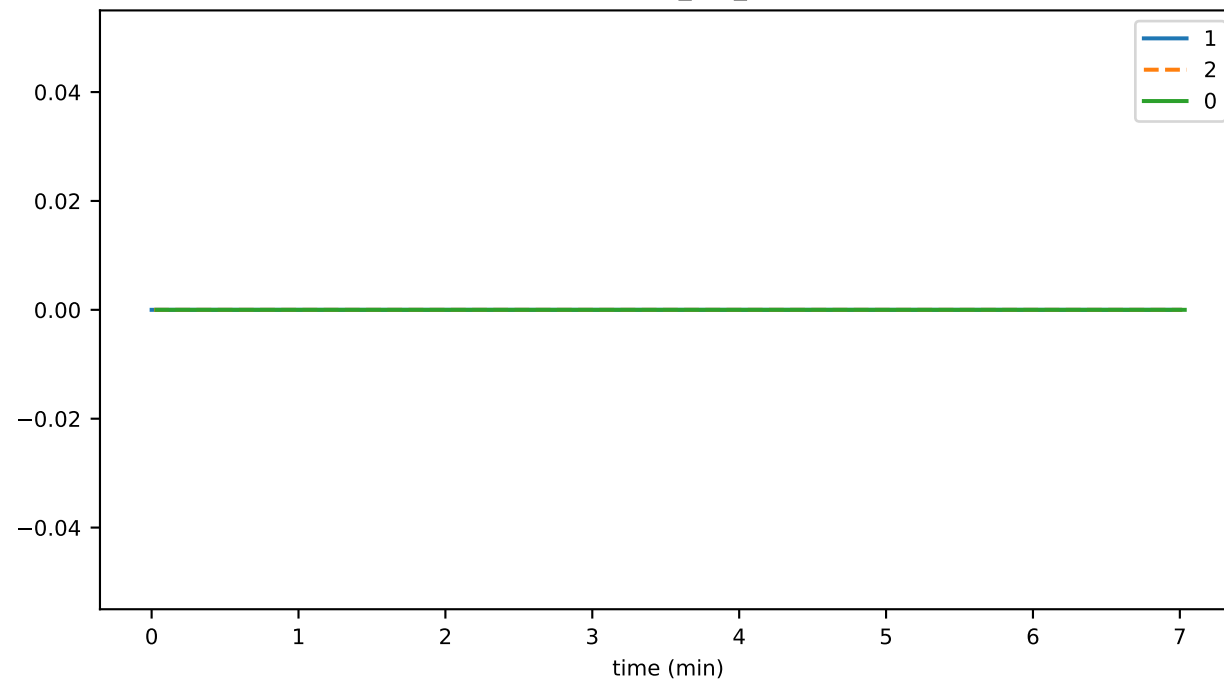
SigLockUp_per_sec
