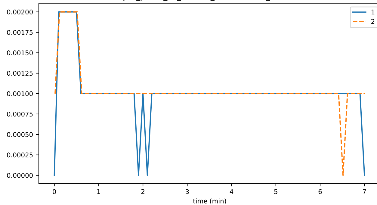
sync_phase_00_fraction_EXCHANGING_EVENTS
