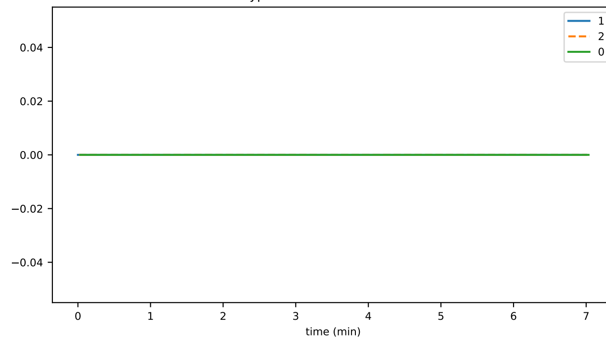
cryptoGetStakersDurationMax
