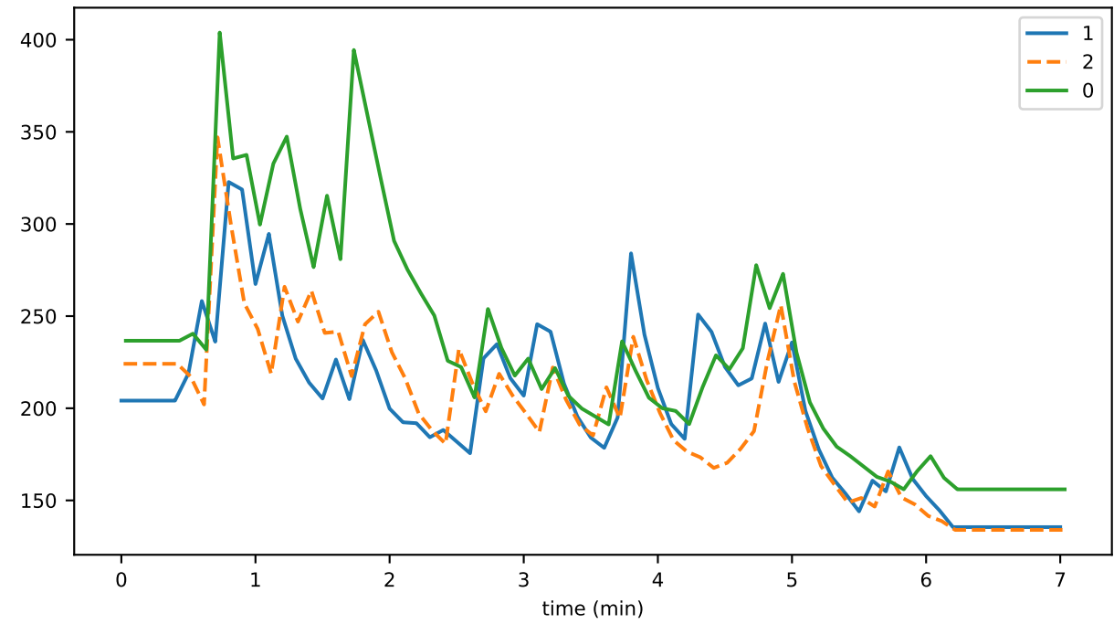
stateCopyMicros
