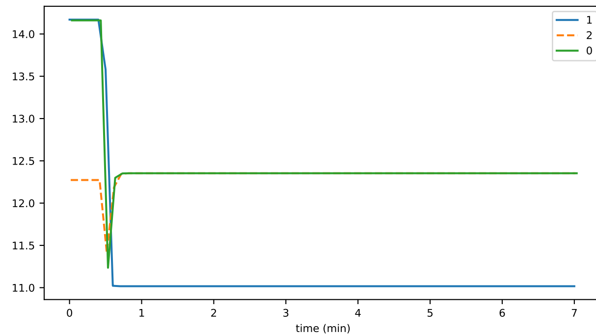
numIndirectProofs
