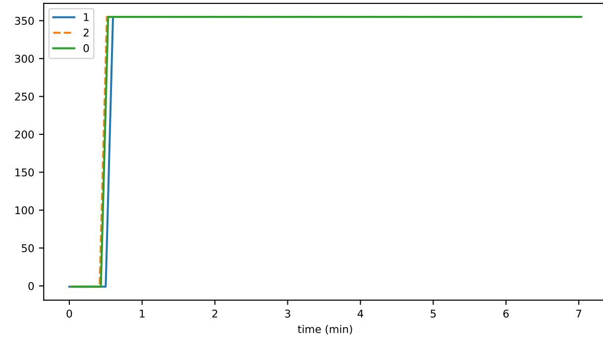
bufferedPriorityTransactions
