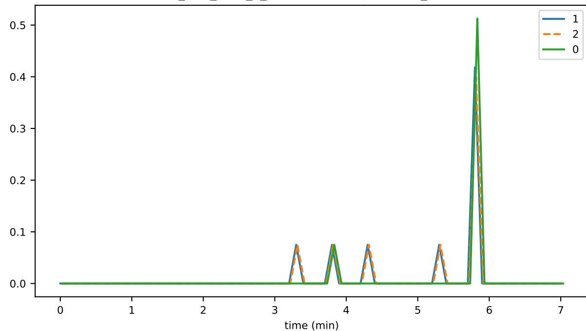
ds_files_level_3_leafKeysFileSizeByLevelMb_state
