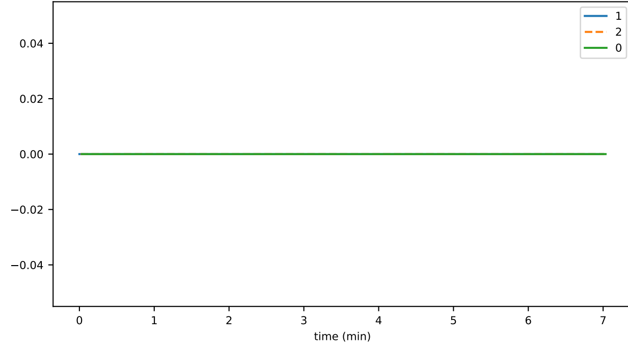
bufferedPriorityTransactions
