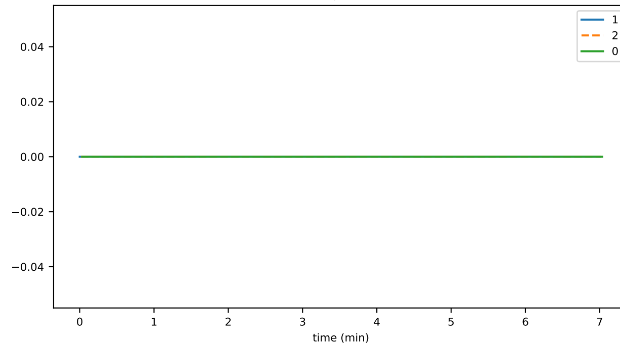
tokenAssociateToAccountDurationAvg
