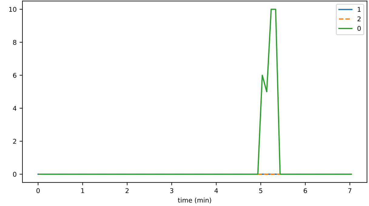
bufferedTransactions
