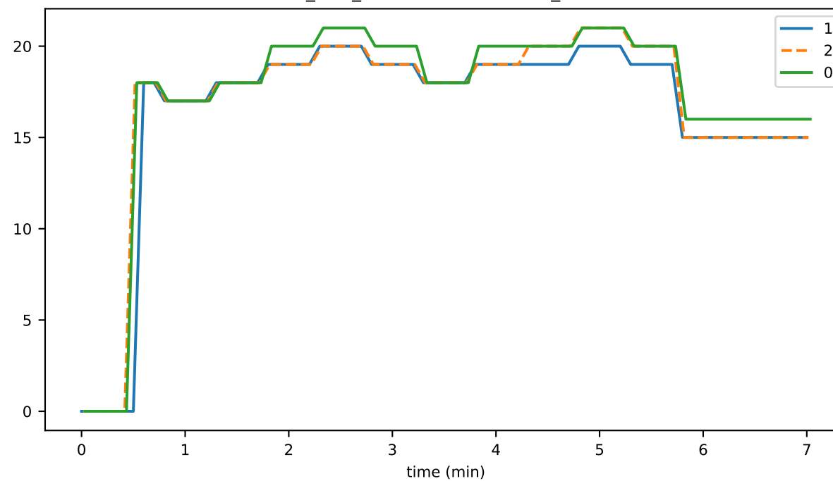
ds_files_leavesStoreFileCount_state
