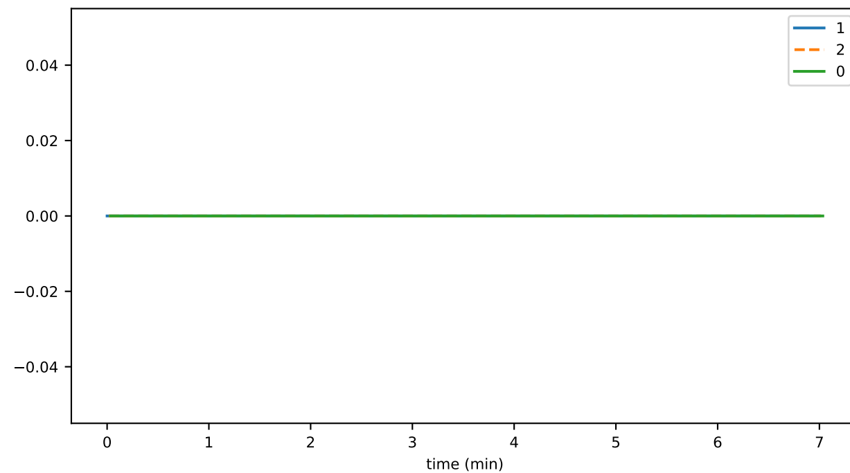
nodeCreateDurationMax
