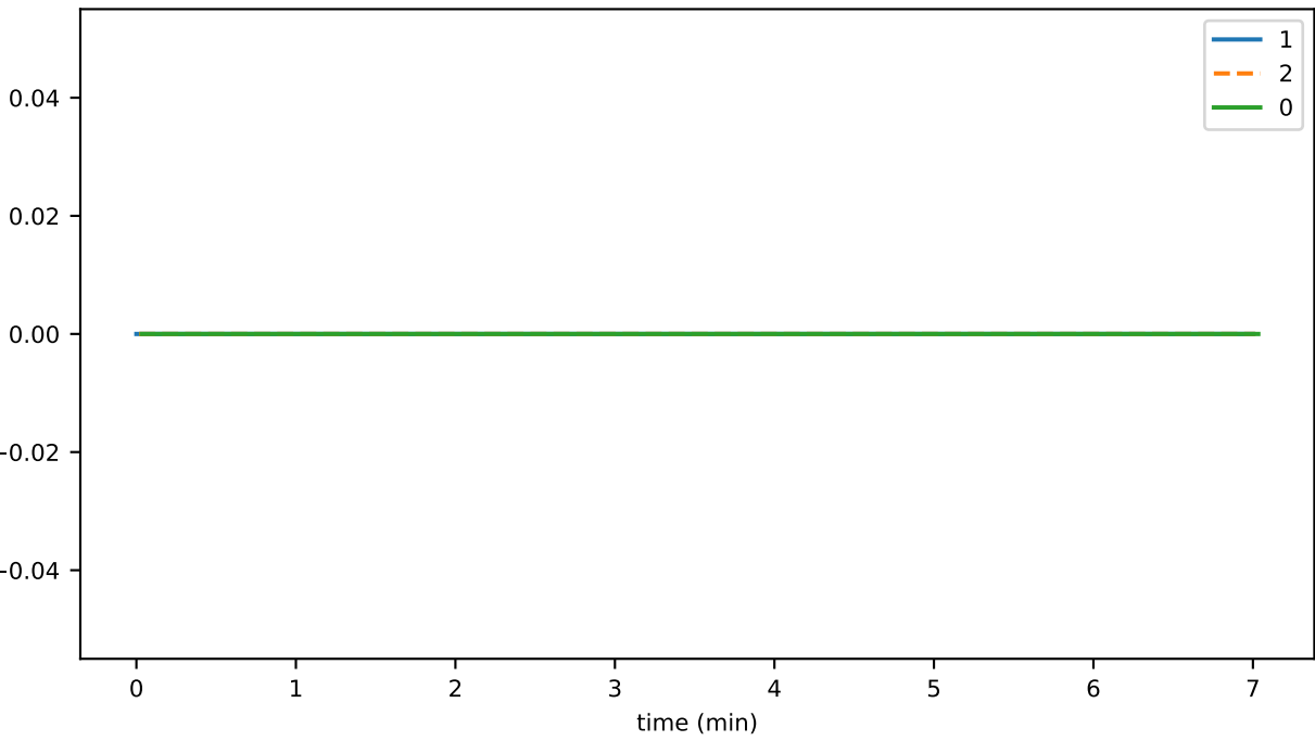
staleTransactions
