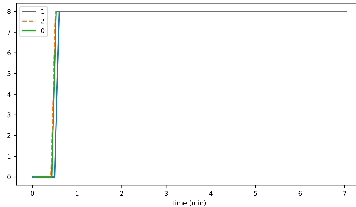
ds_offheap_hashesIndexMb_state
