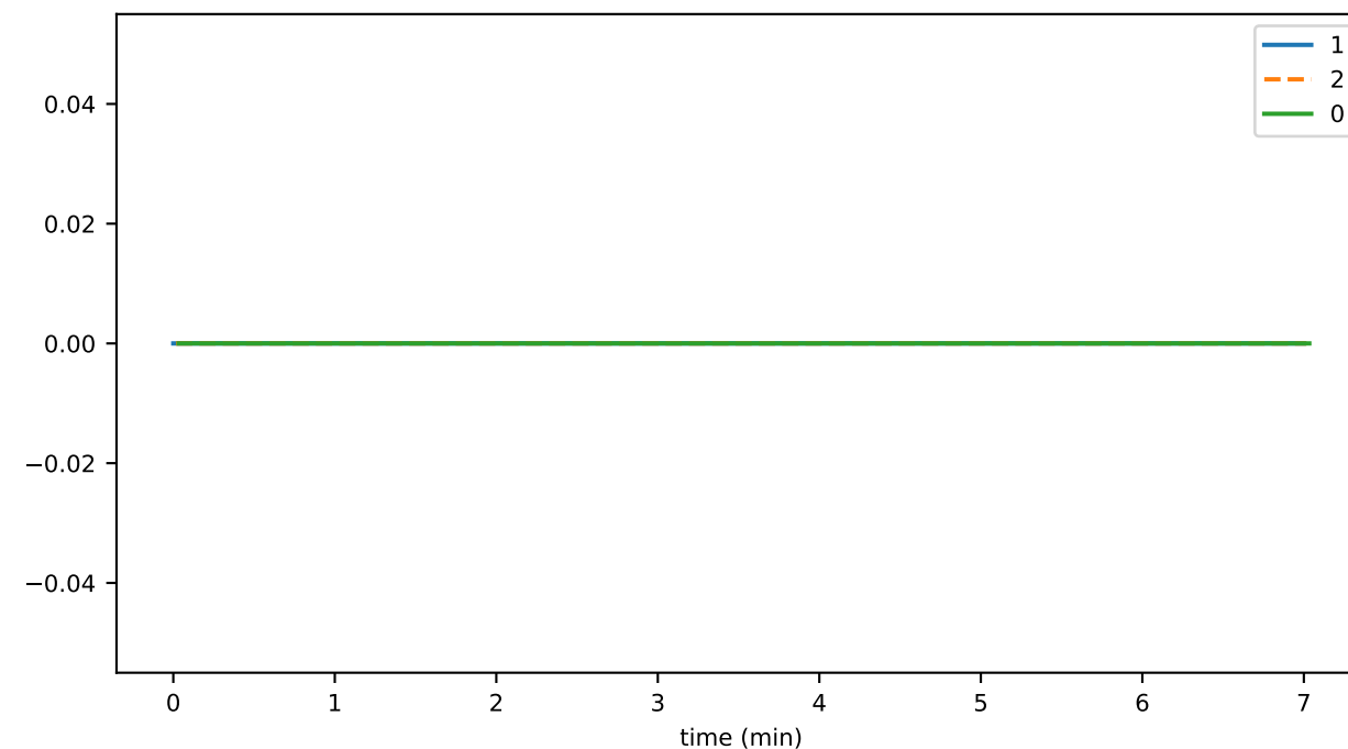
scheduleGetInfoDurationAvg
