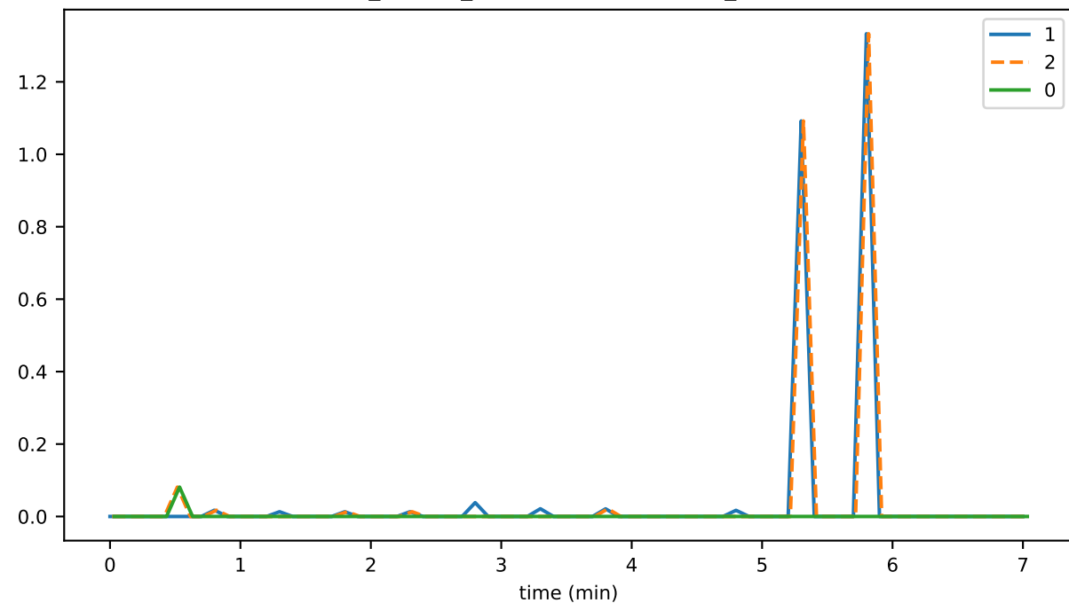
ds_offheap_dataSourceMb_state
