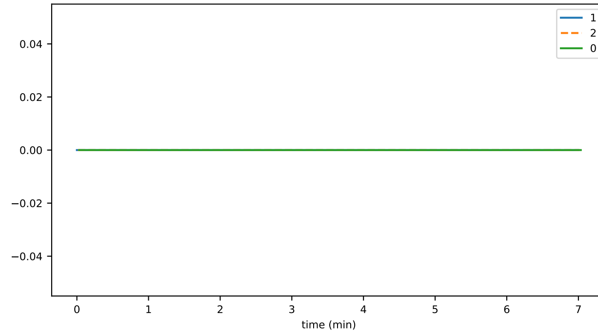
connRecv_endStream_badBlockProof
