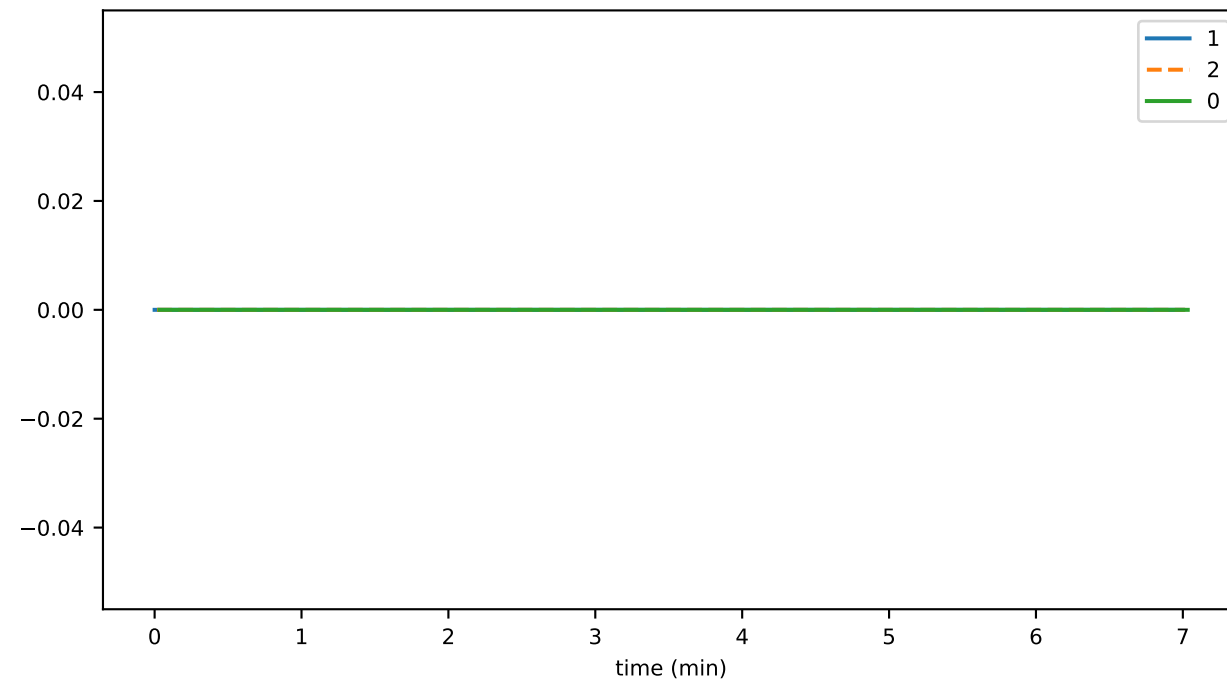
hintsSignaturesProduced
