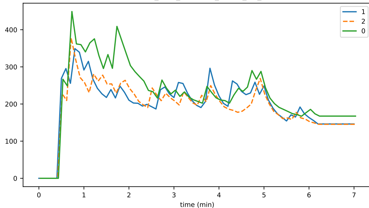
consensus_time_GETTING_STATE_TO_SIGN
