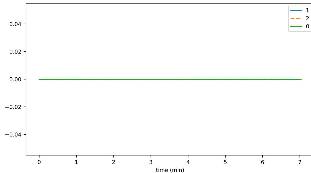
transactionGetReceiptDurationMax
