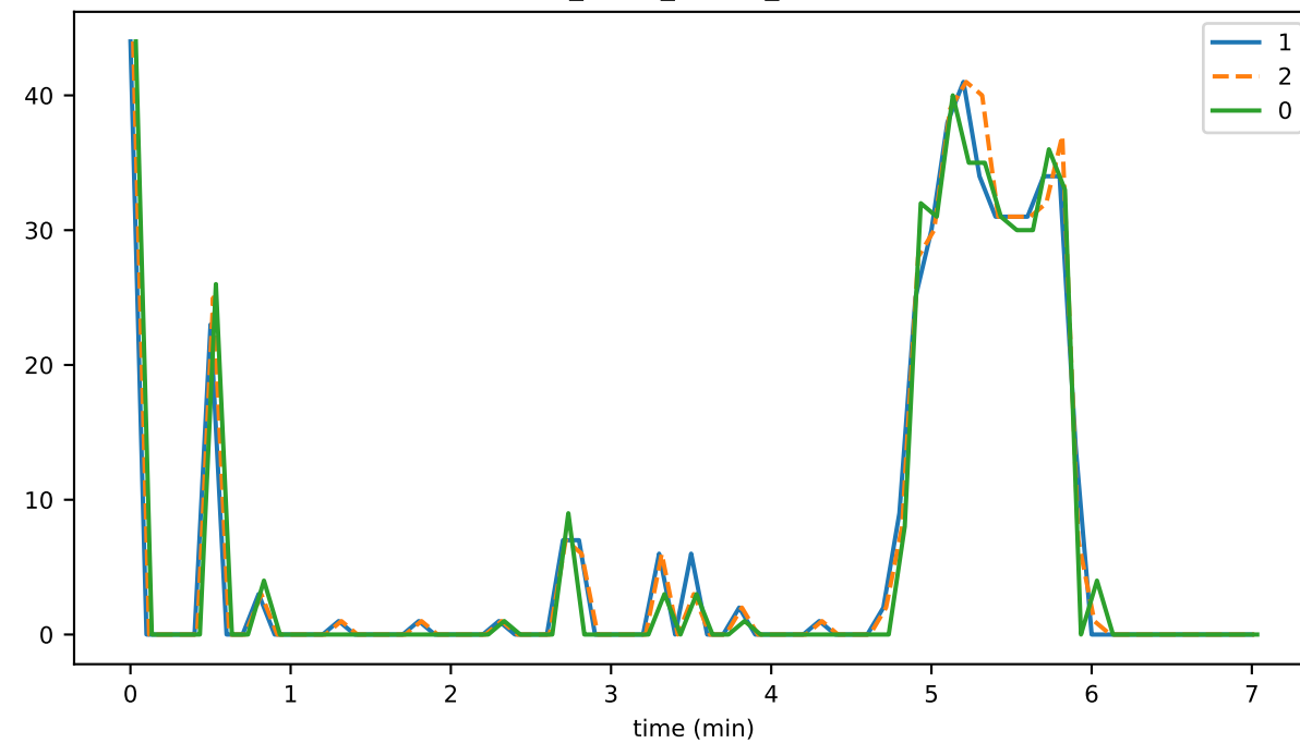
dupEvPercent
