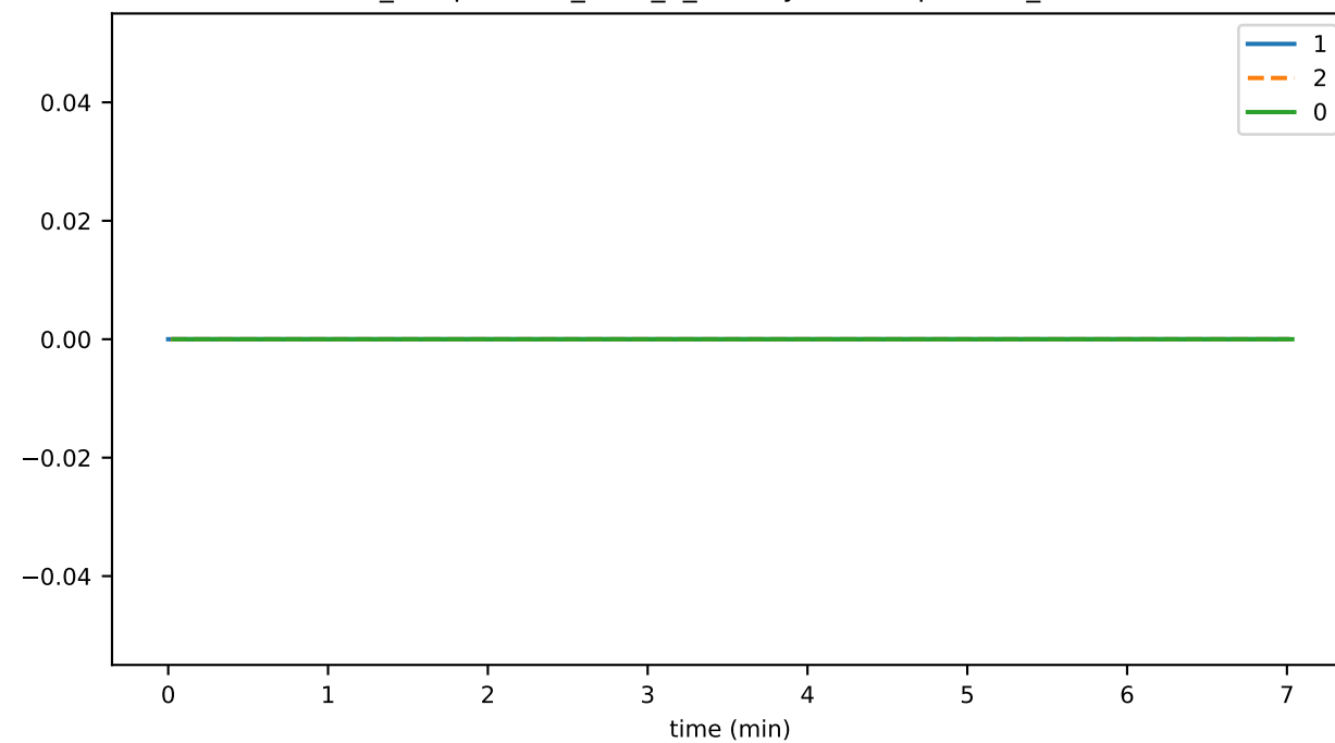
ds_compactions_level_7_leafKeysSavedSpaceMb_state
