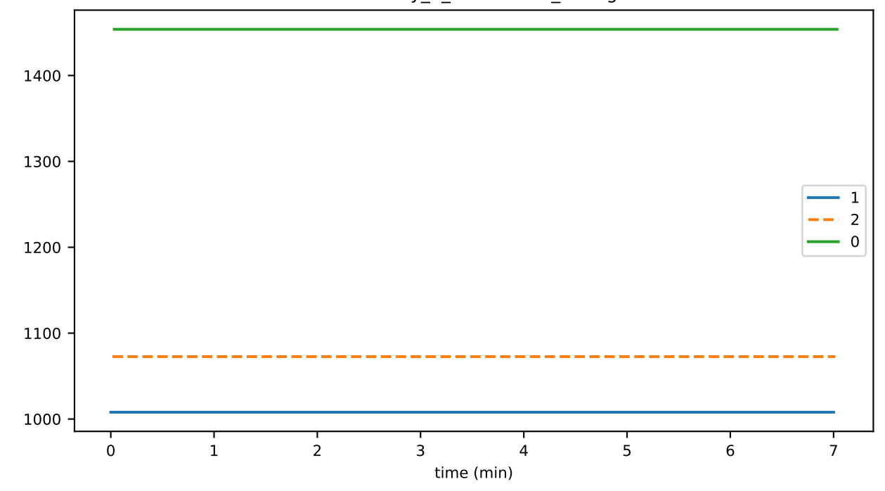
eventDelay_4_verification_storage
