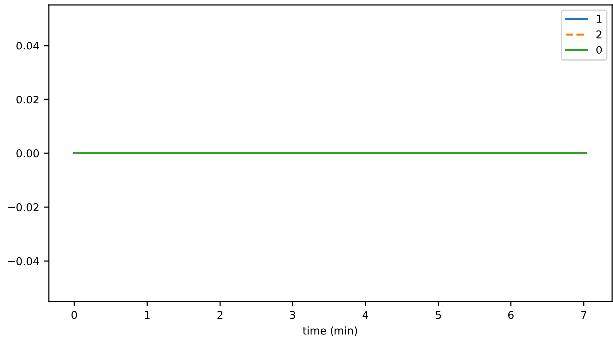
SigInval_per_sec
