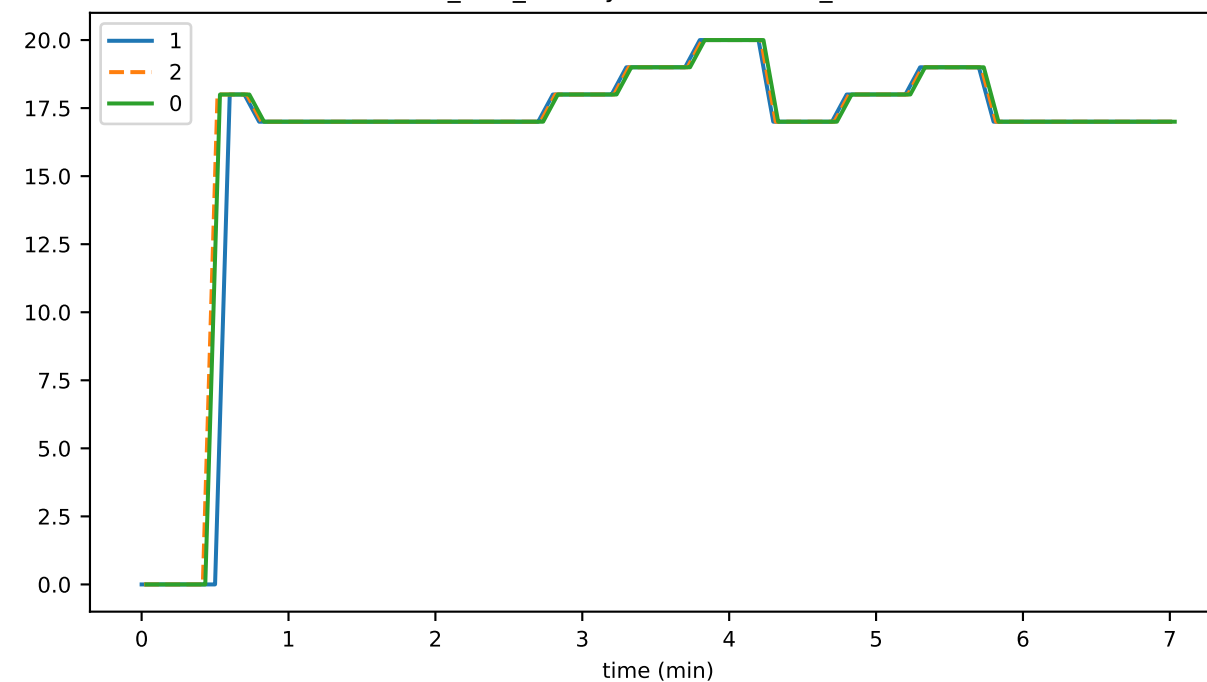
ds_files_leavesStoreFileCount_state
