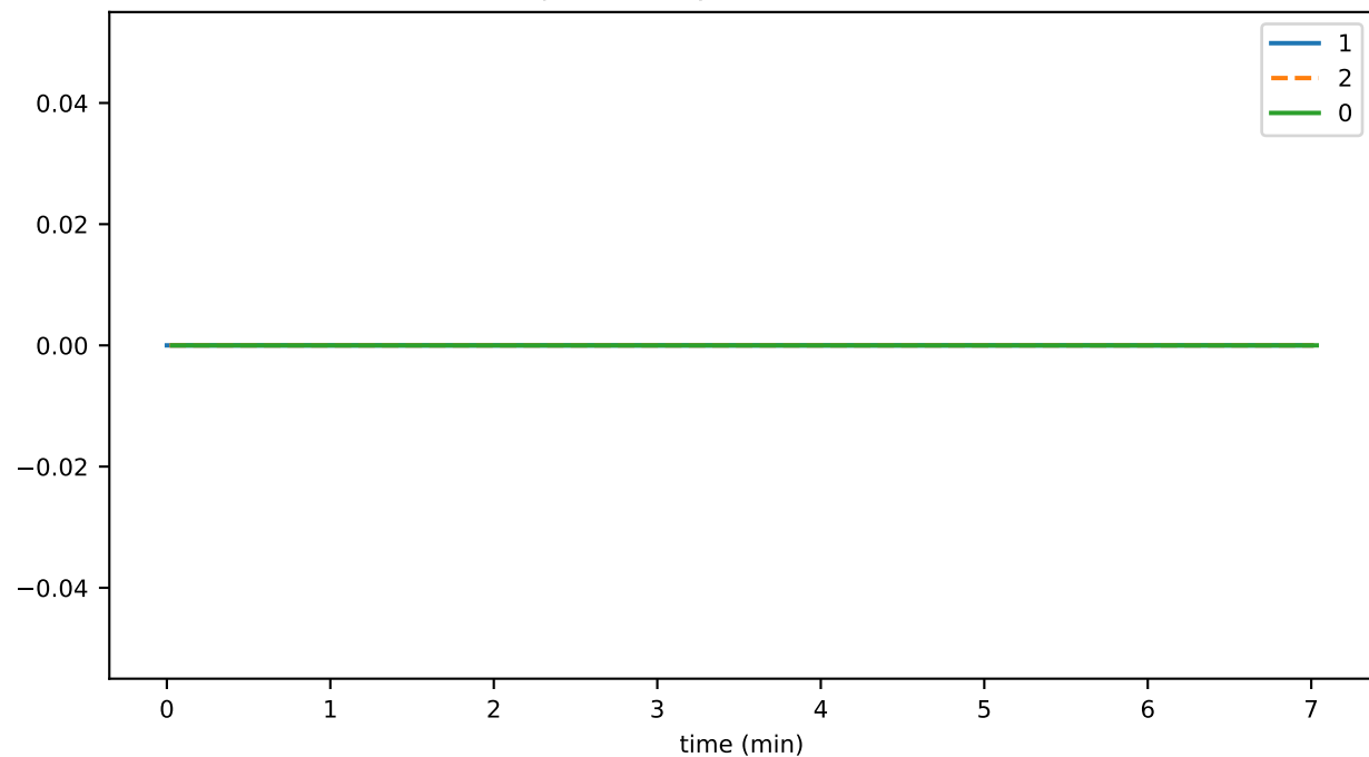
hapiOffHeapQueryLimitsPercentUsed
