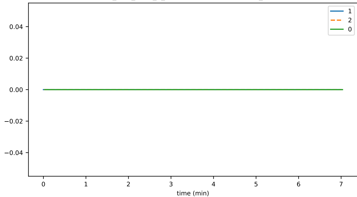
ds_files_level_2_hashesFileSizeByLevelMb_state
