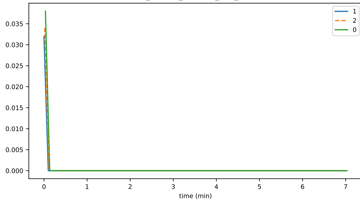
consensus_time_GETTING_STATE_TO_SIGN
