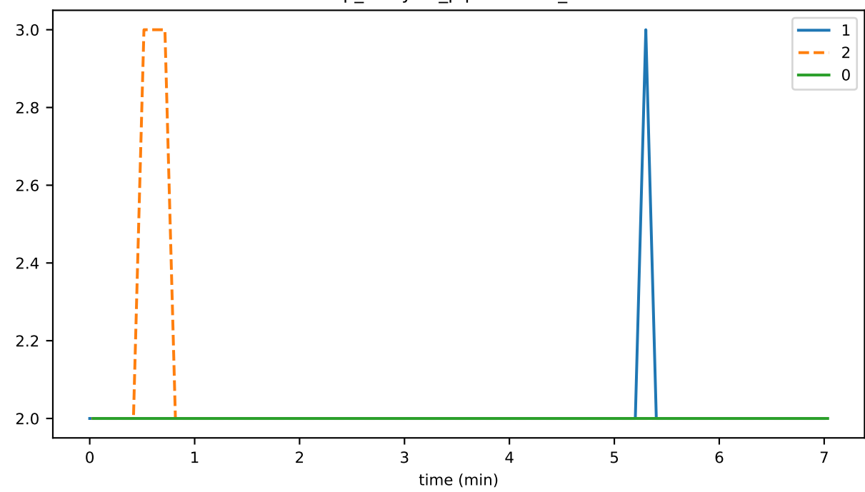
vmap_lifecycle_pipelineSize_state
