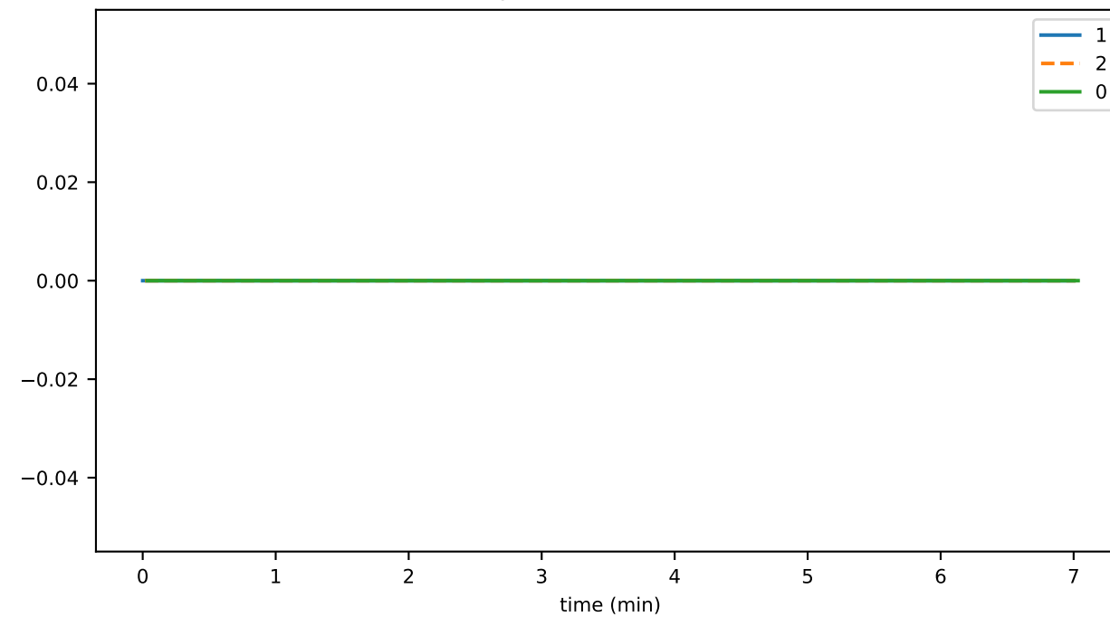
syncPermitsUtilized
