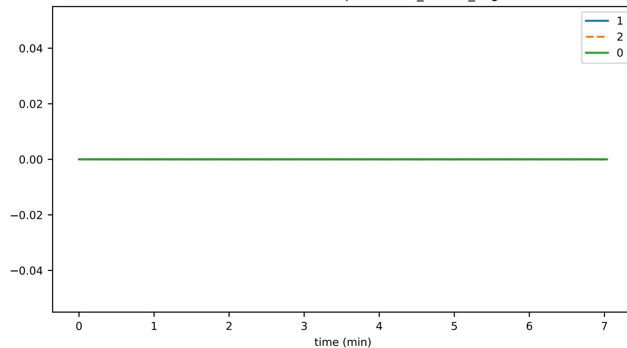
SmartContractService:OpsDuration_PerTxn_sum
