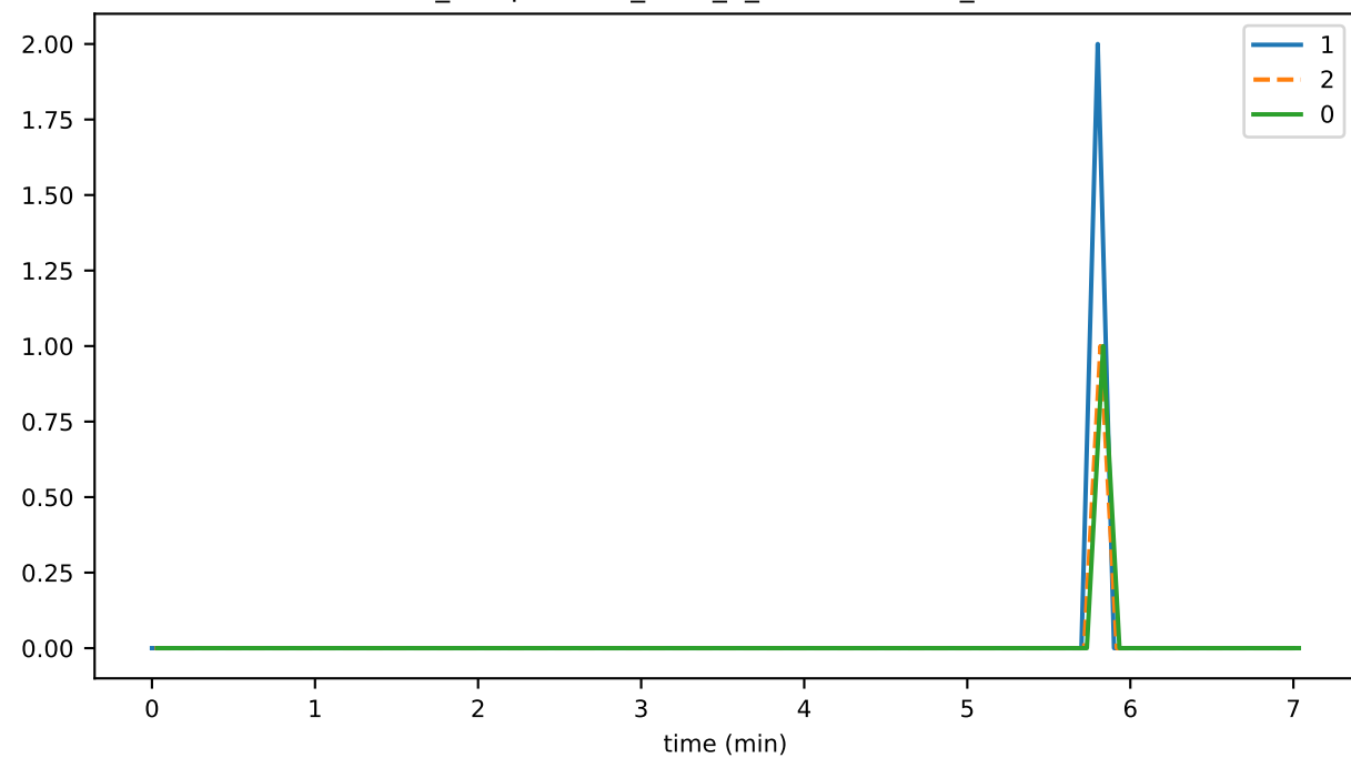
ds_compactions_level_3_leavesTimeMs_state
