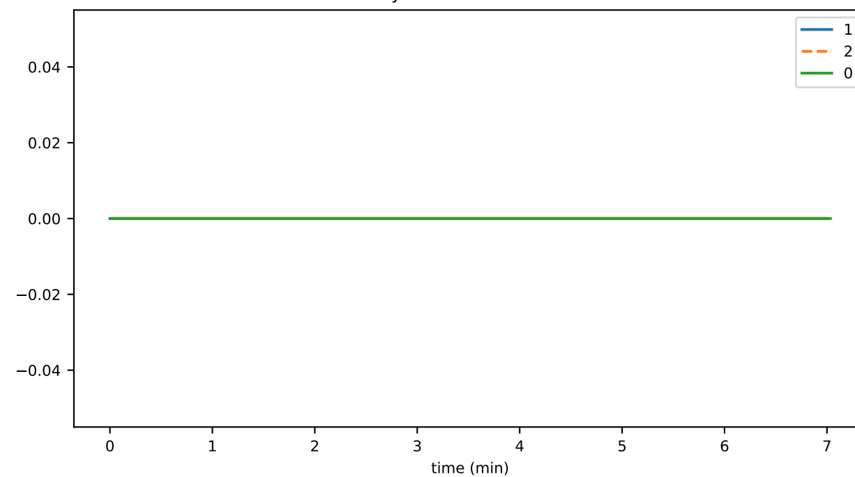
hintsKeyPublicationDurationMax
