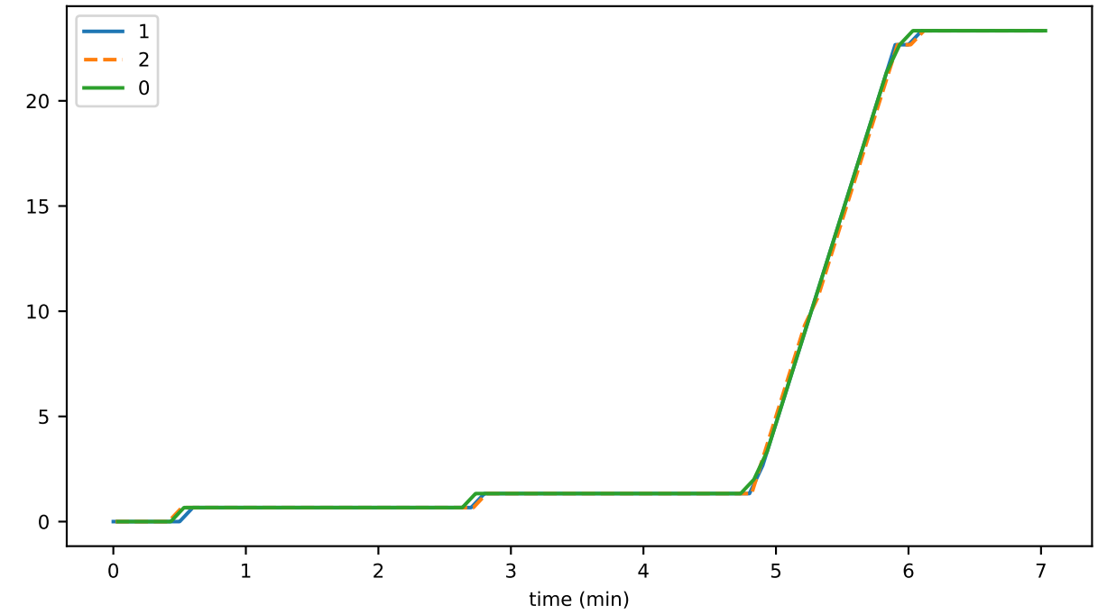
bufferedTransactions
