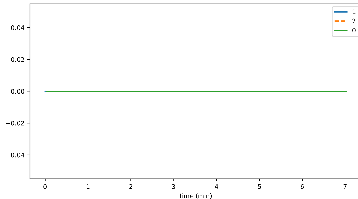
tokenPauseDurationAvg
