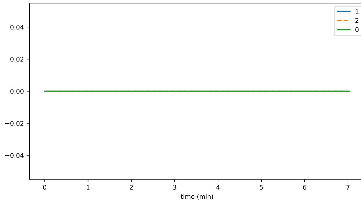
systemDeleteDurationAvg
