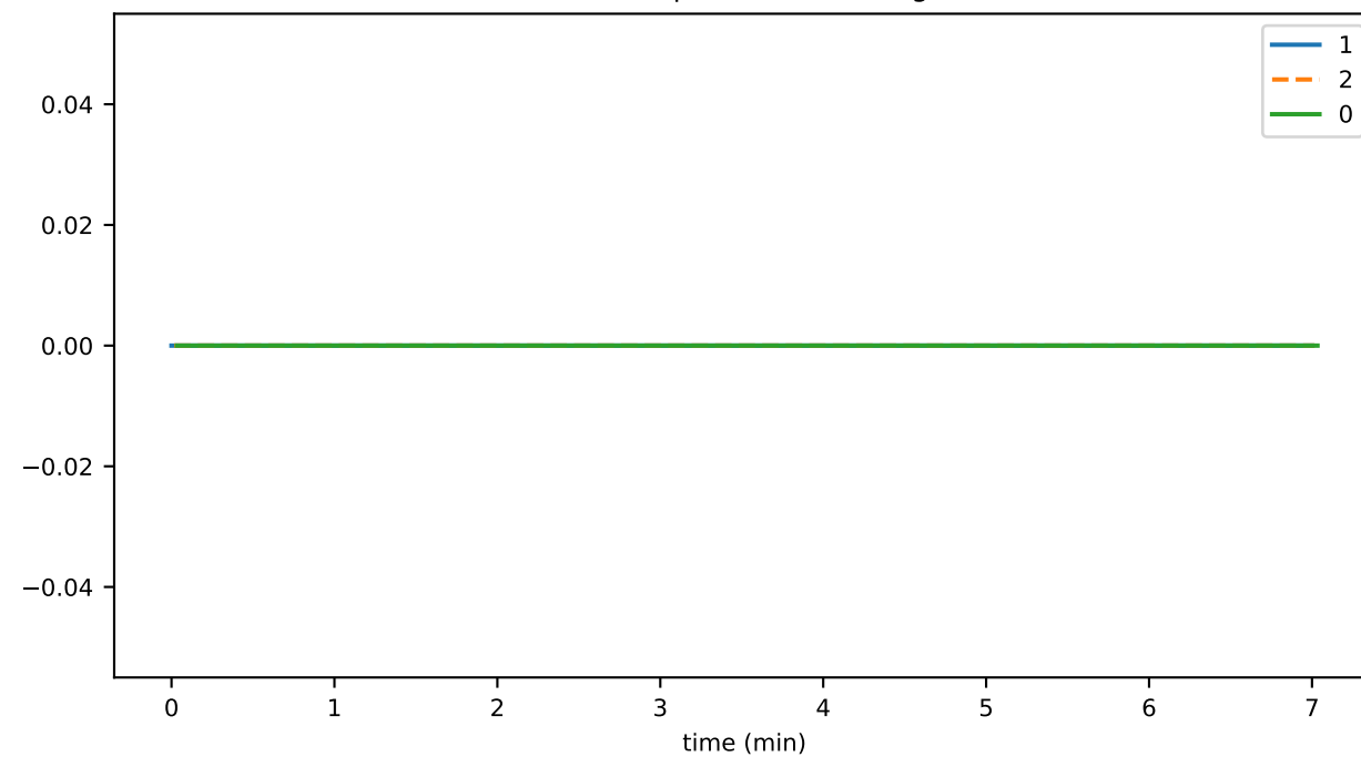
hookDispatchDurationAvg
