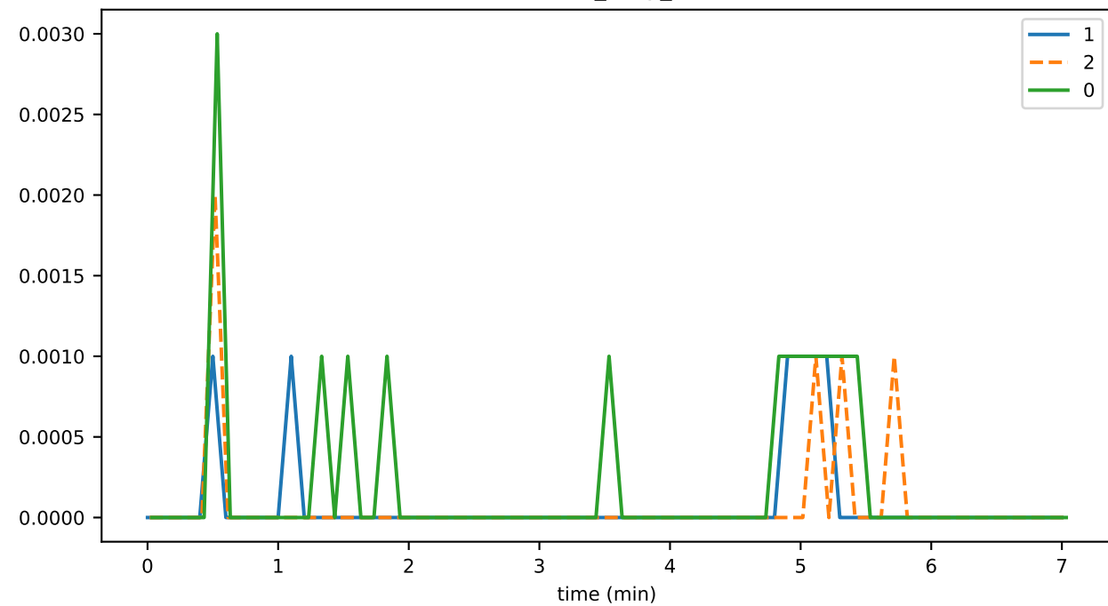
stateSignatureAge
