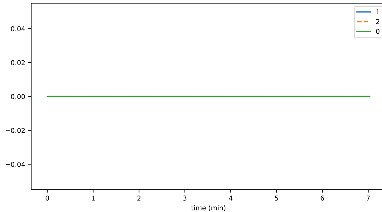
SigVal_per_sec
