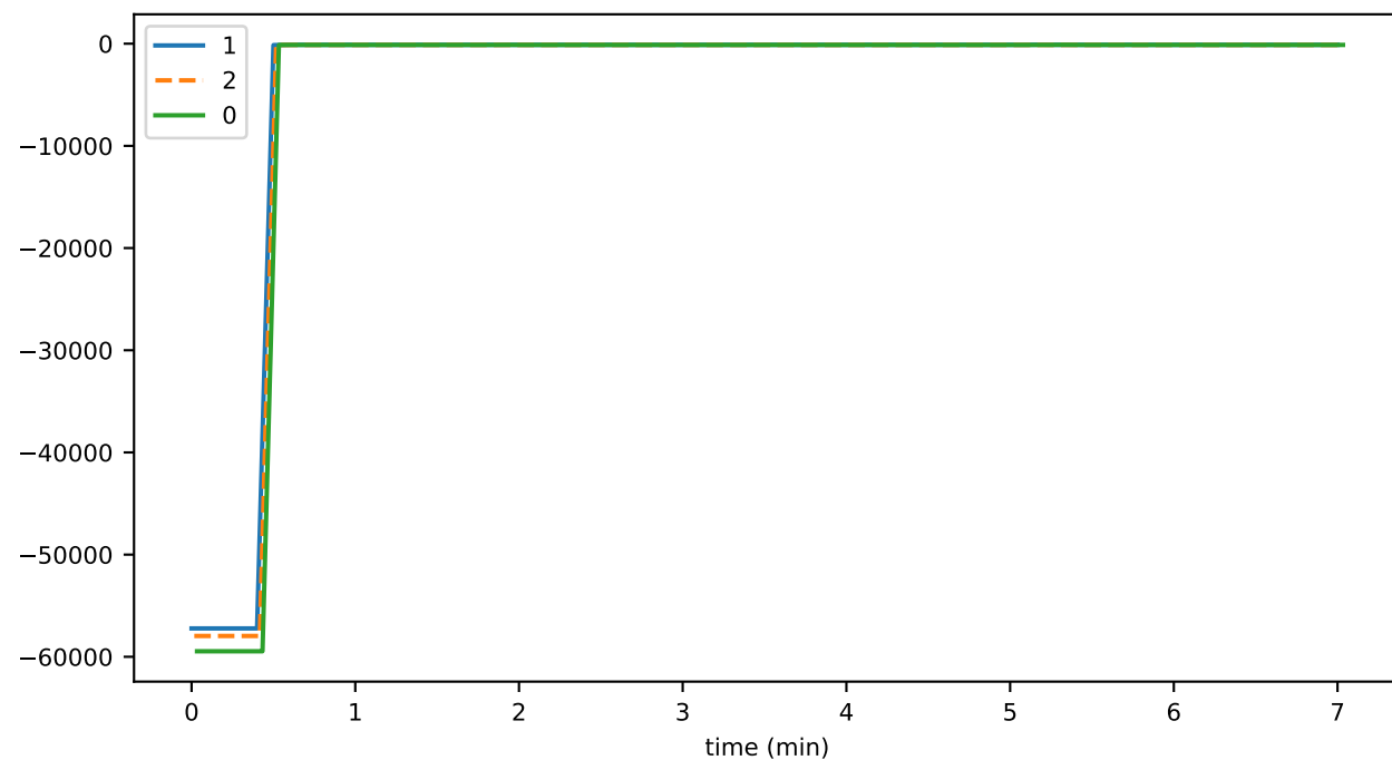
consensusUpdateTopicDurationMax
