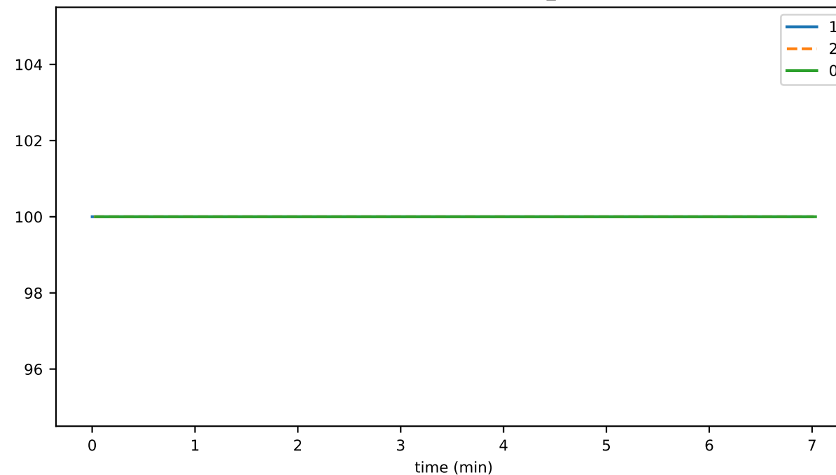
nodeActivePercentSnapshot_node0
