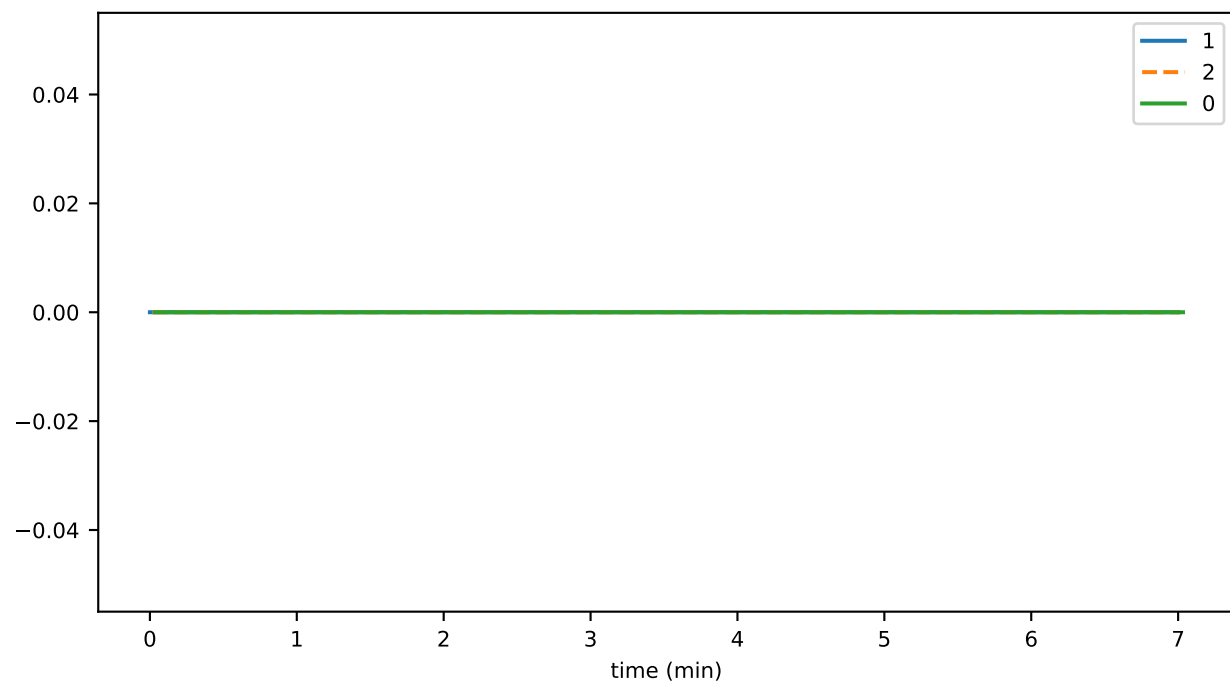
transactionGetReceiptDurationAvg
