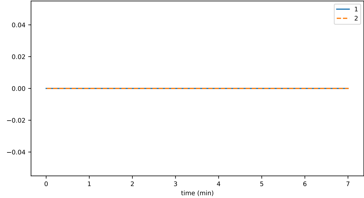
sync_phase_00_fraction_PLATFORM_STATUS_PREVENTING_SYNC
