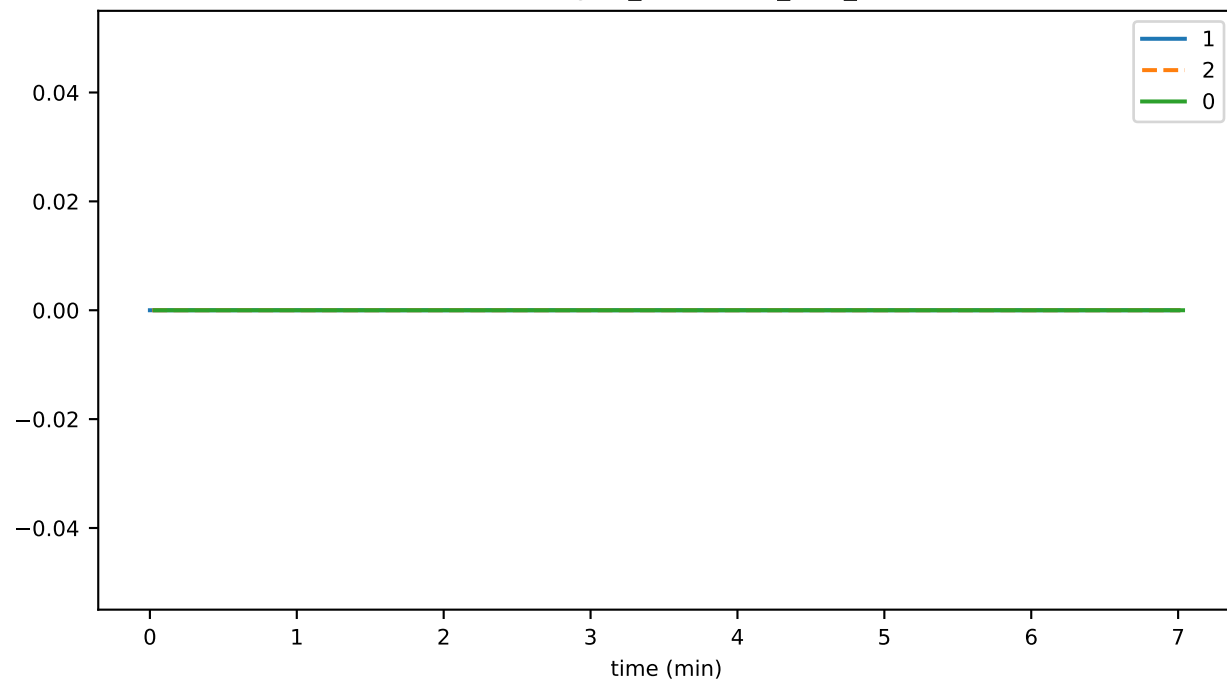
consensusGetTopicInfoDurationMax
