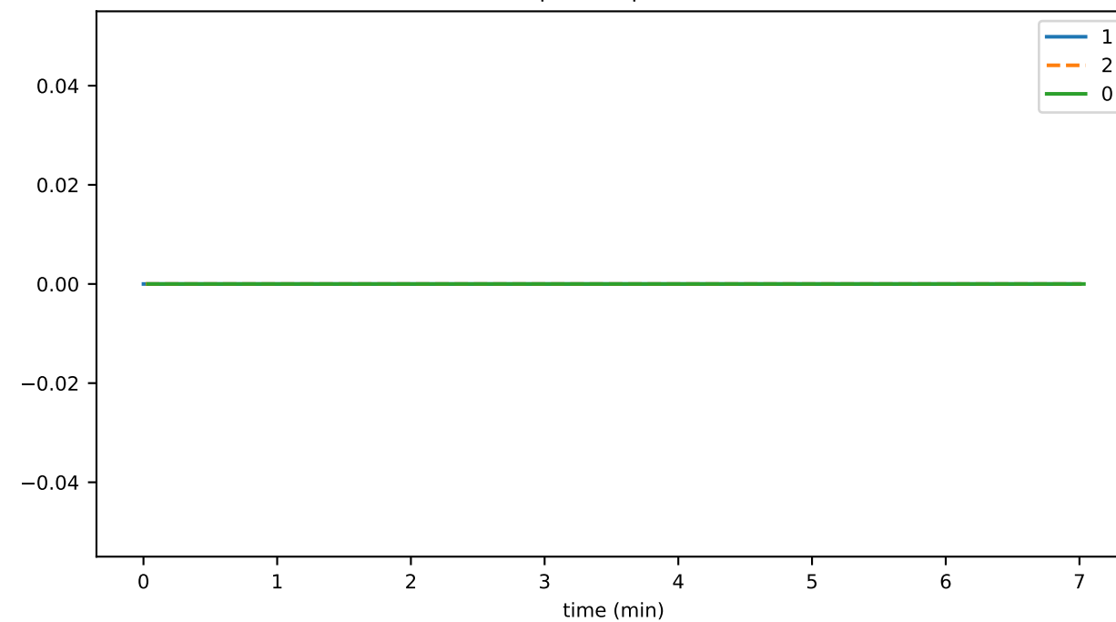
consensusUpdateTopicThrottledTxns
