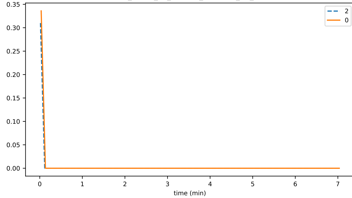
sync_phase_01_fraction_OUTSIDE_OF_RPC
