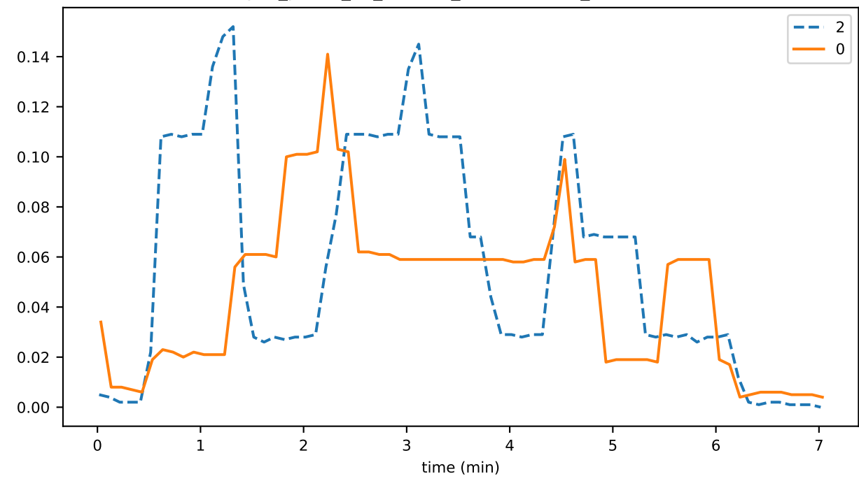
sync_phase_01_fraction_IDLE
