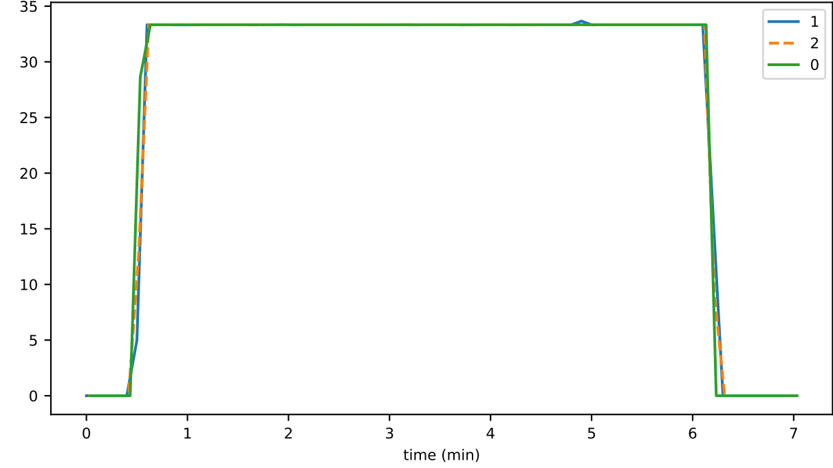
broadcastEventsReceived
