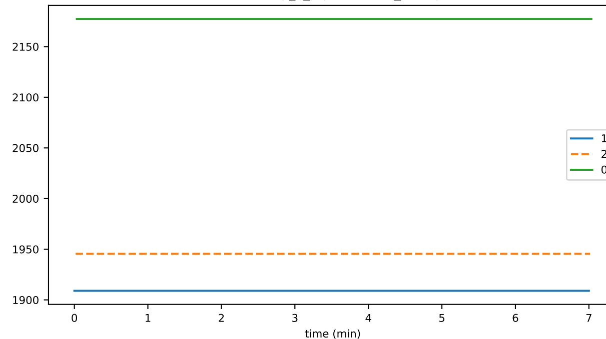
eventDelay_6_pces_gossip
