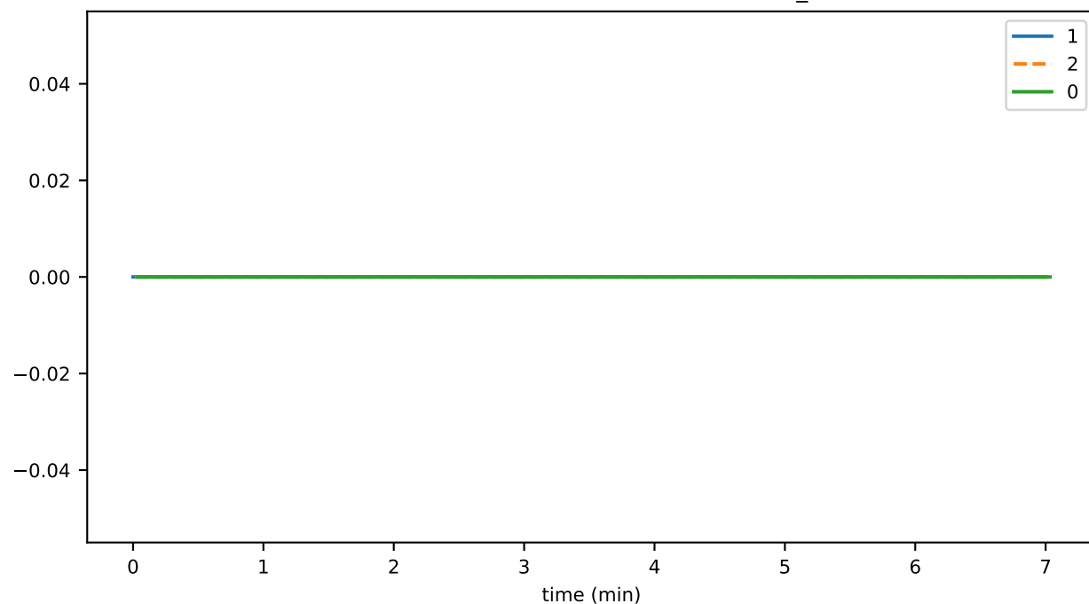
SmartContractService:TransactionGasUsed_avg
