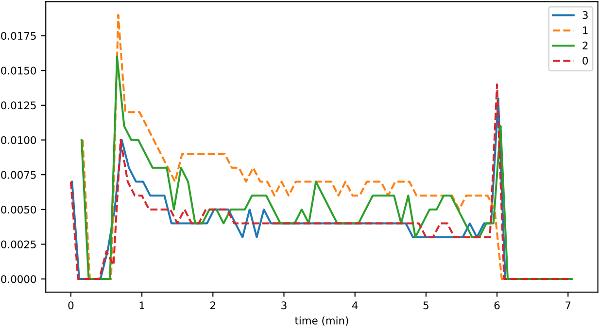
ConsensusEngine_busy_fraction
