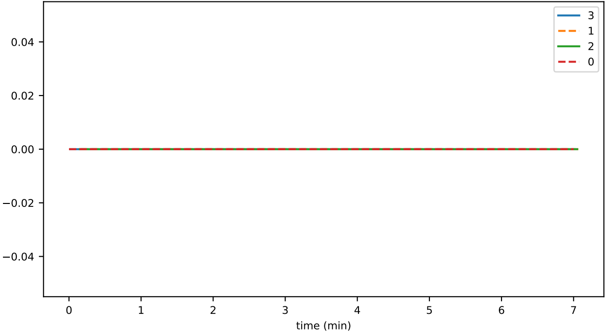
SmartContractService:SystemContractMethodCall_WIPE_failed
