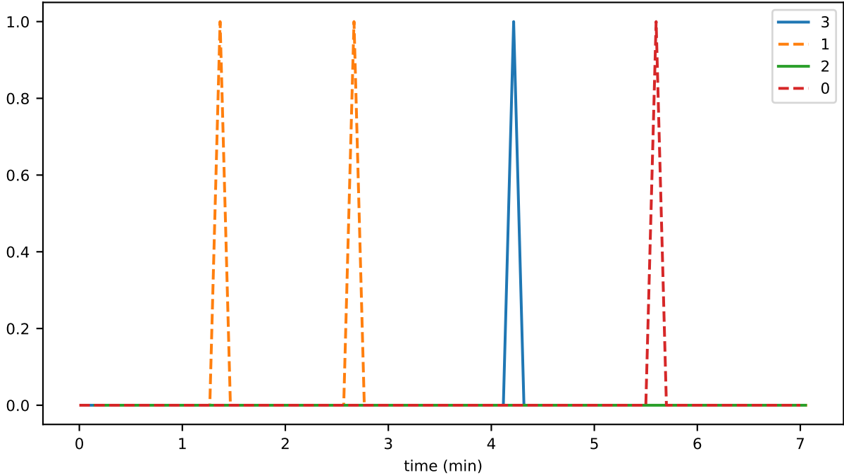
ConsensusEngine_unhandled_task_count
