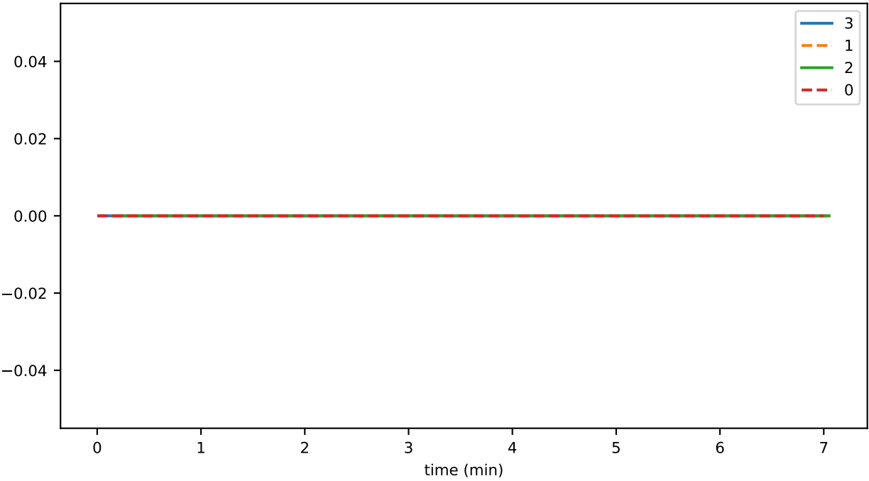
SmartContractService:SystemContractMethodCall_ERC20_failed
