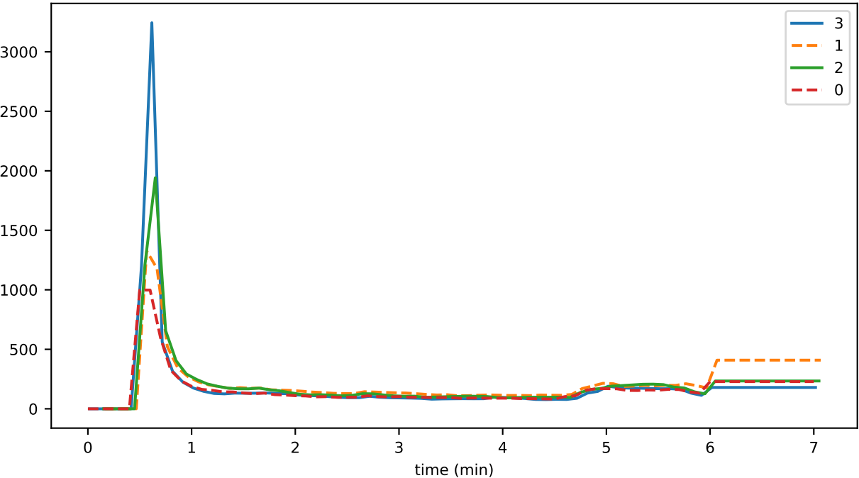
ConsensusEngine_busy_fraction
