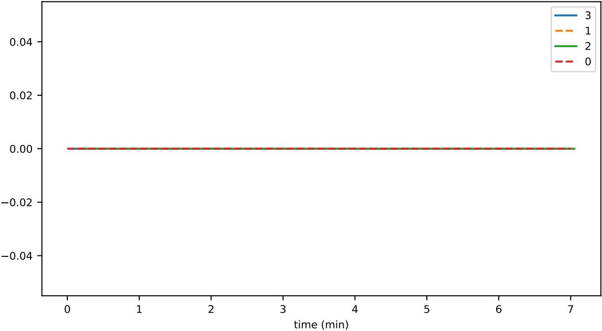
SmartContractService:SystemContractMethodCall_ALIASES_failed
