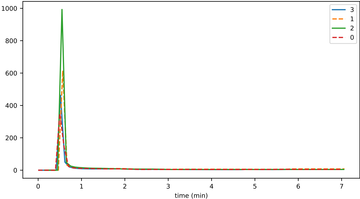
ConsensusEngine_unhandled_task_count
