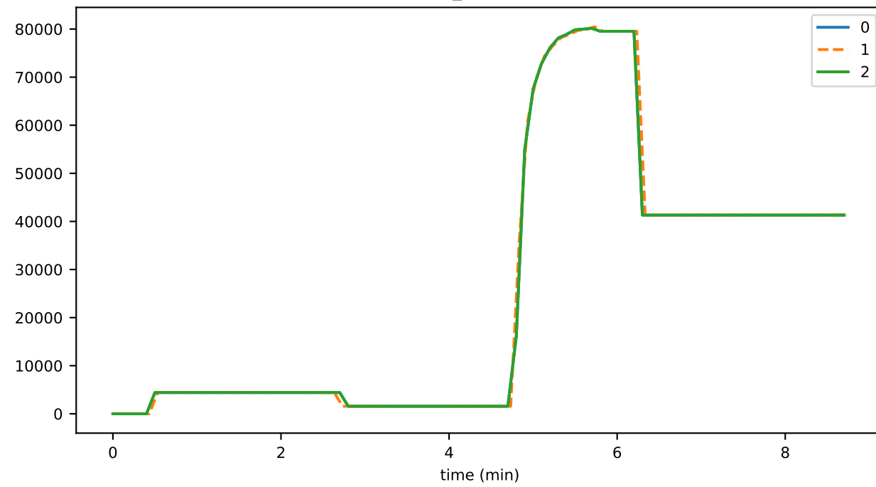
buffer_blockBytes
