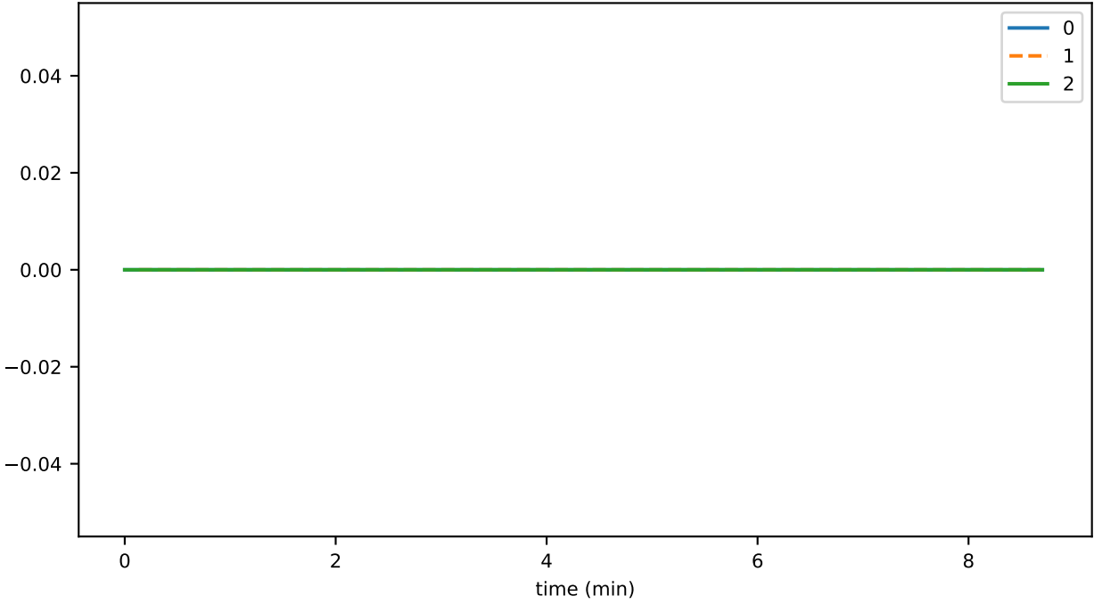
SmartContractService:SystemContractMethodCall_HSS_total
