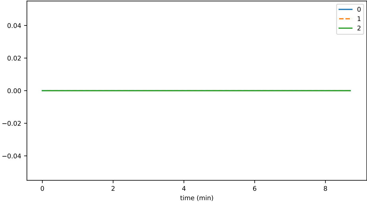
SmartContractService:SystemContractMethodCall_HTS_failed
