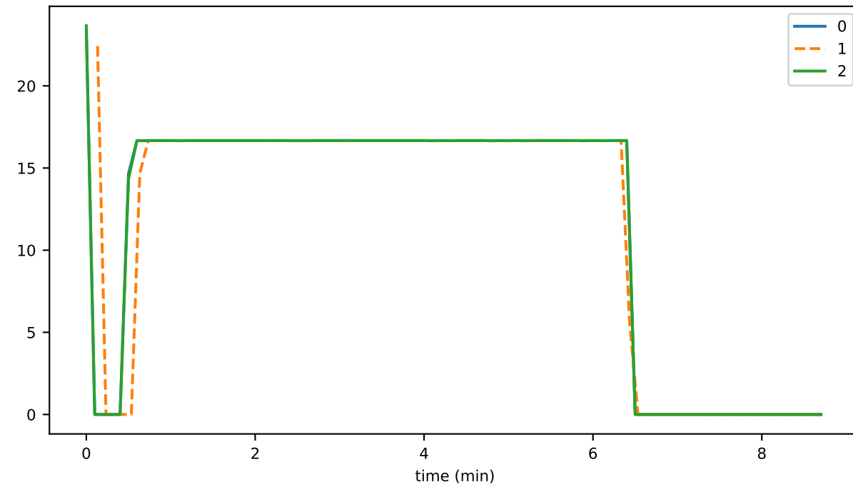
buffer_blockBytes
