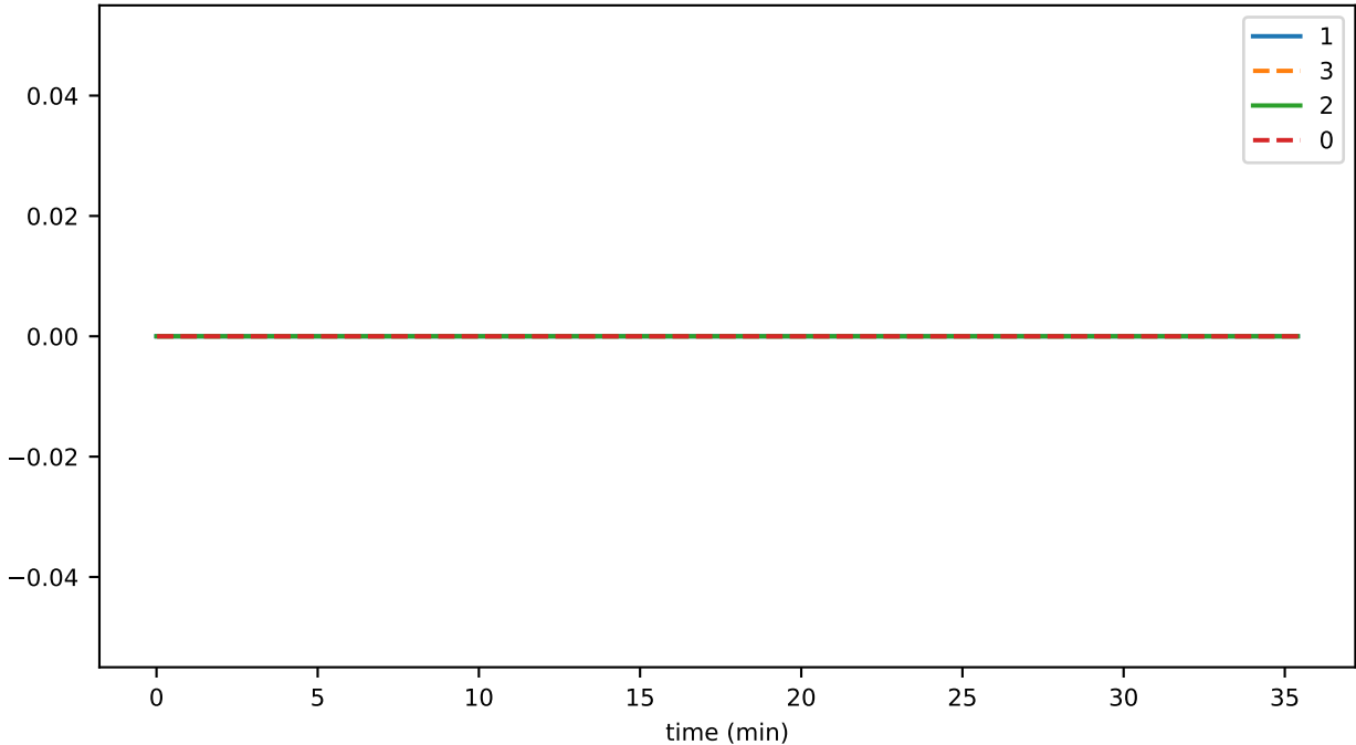
SmartContractService:SystemContractMethodCall_ERC20_failed
