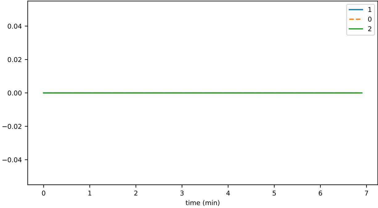
SmartContractService:SystemContractMethodCall_ERC721_failed
