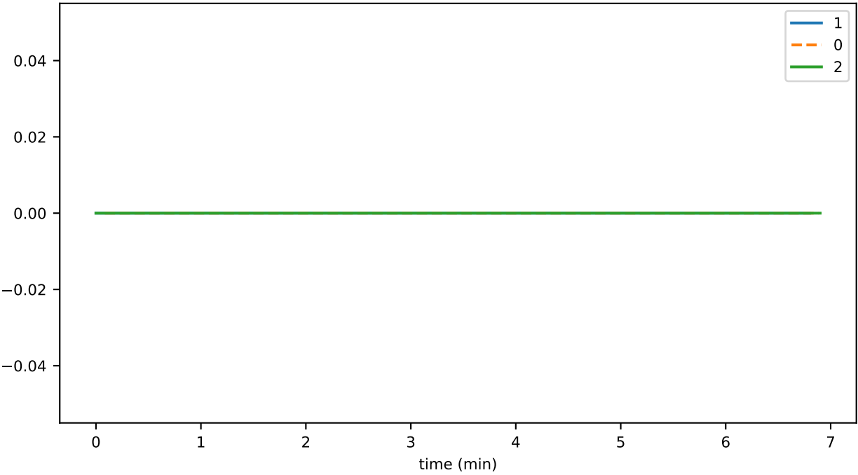
SmartContractService:Rejected_ethereumTxDueToIntrinsicGas_total
