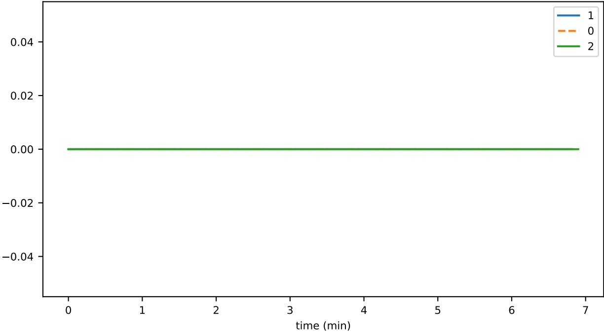
SmartContractService:Rejected_ethType3BlobTransaction_total
