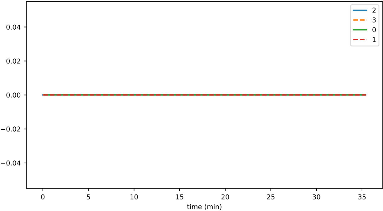
ds_compactions_level_5_hashesSavedSpaceMb_state
