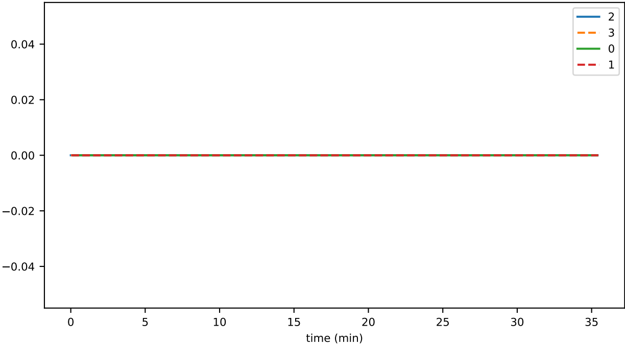
ds_compactions_level_5_hashesTimeMs_state
