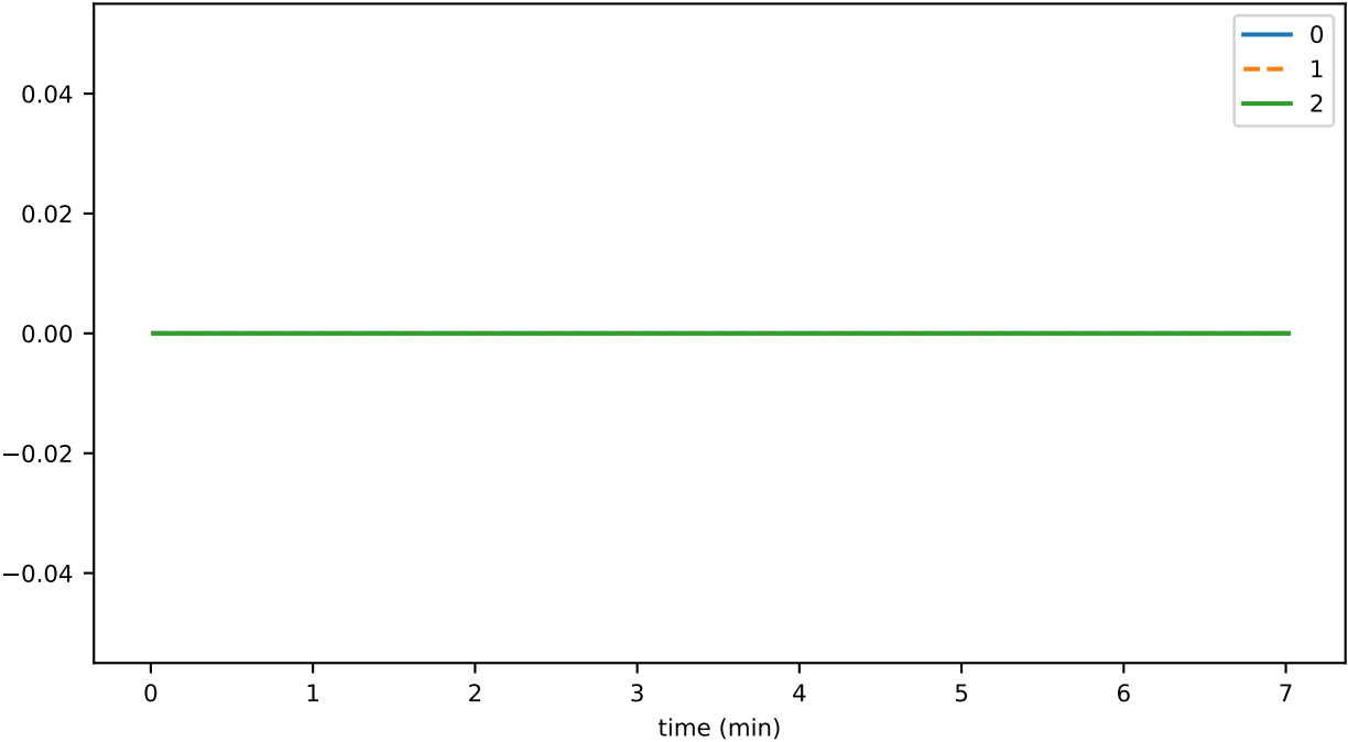
SmartContractService:OpsDuration_PerTxn_avg
