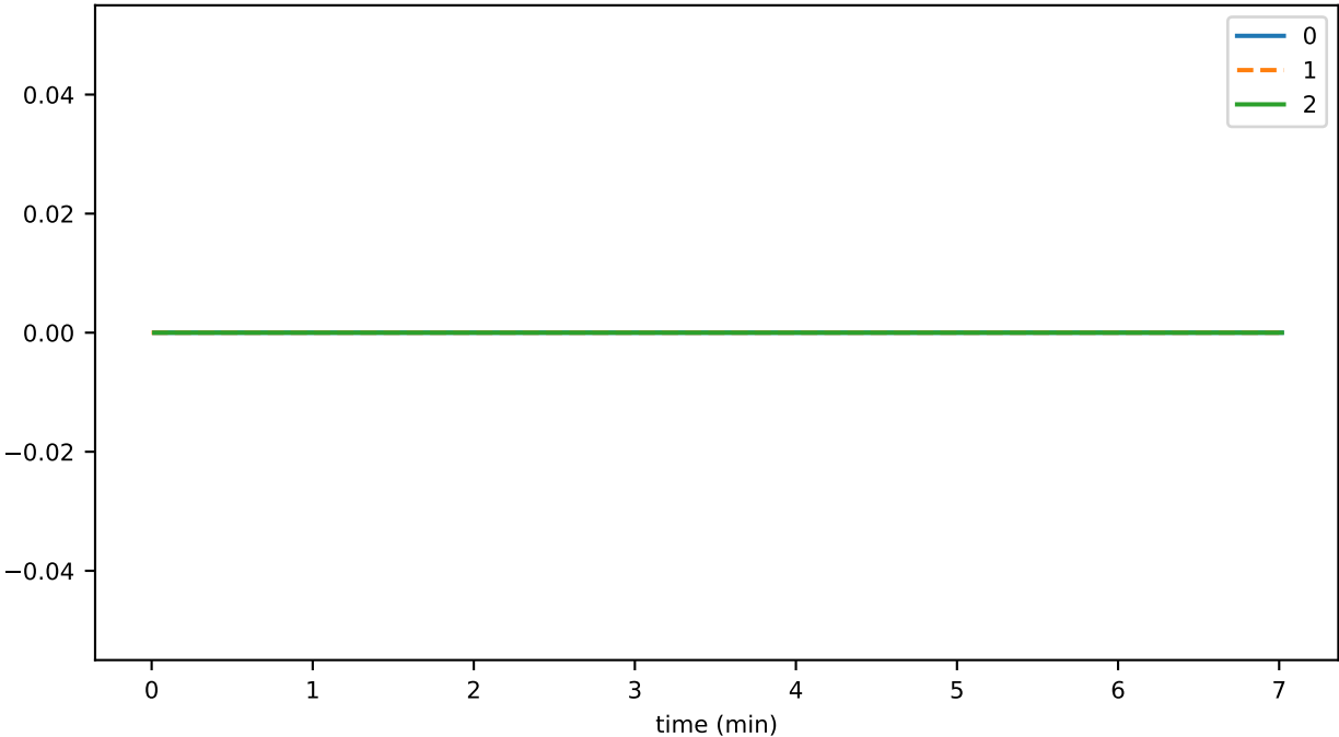
SmartContractService:OpsDuration_PerTxn_count
