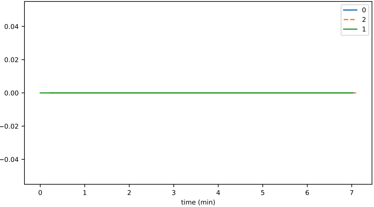
SmartContractService:SystemContractMethodCall_ASSOCIATION_failed
