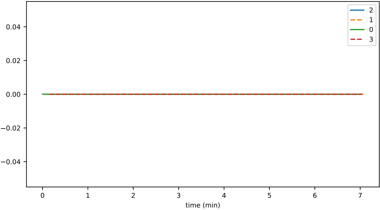
SmartContractService:SystemContractMethodCall_WIPE_failed
