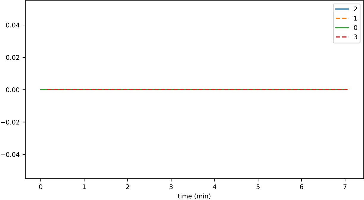
SmartContractService:SuccessfulTransactionDuration_count
