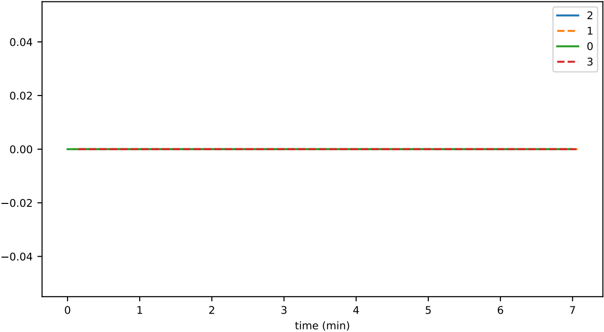
SmartContractService:SystemContractMethodCall_ERC20_failed
