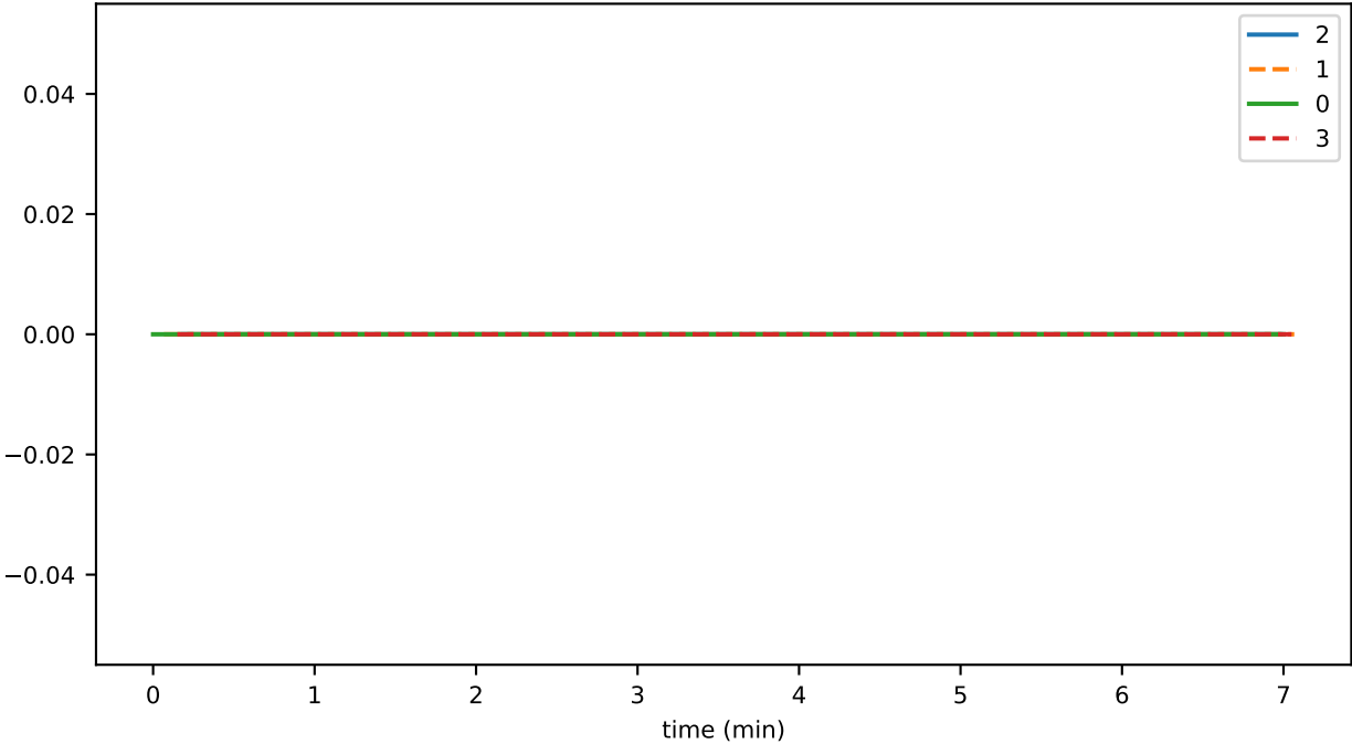
SmartContractService:SystemContractMethodCall_HSS_total
