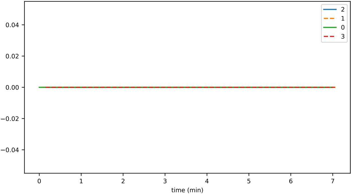
SmartContractService:SystemContractMethodCall_MINT_BURN_failed
