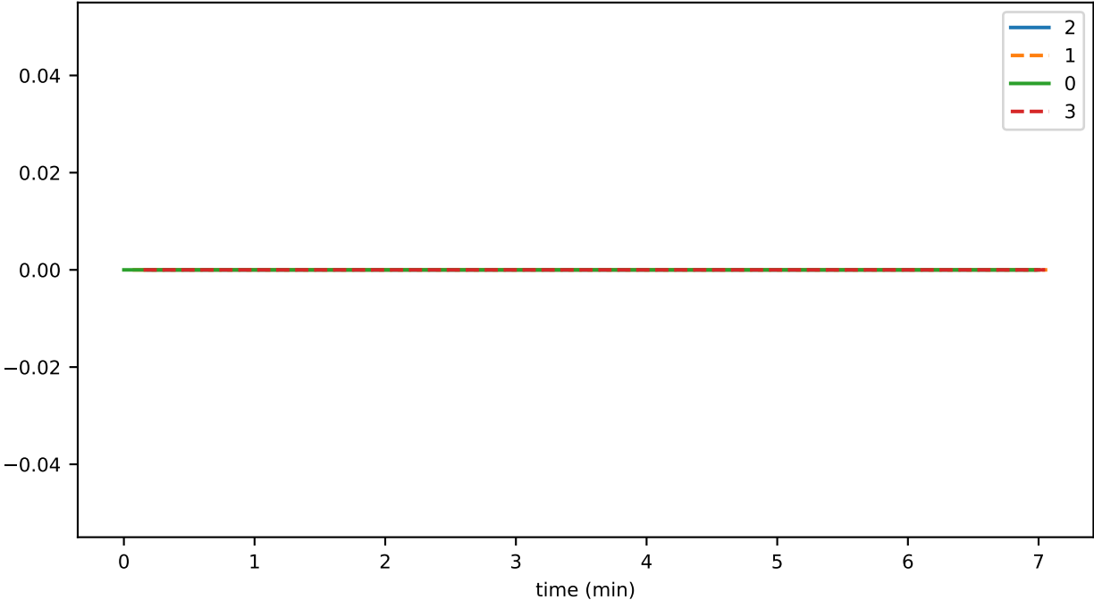
SmartContractService:SuccessfulTransactionDuration_sum
