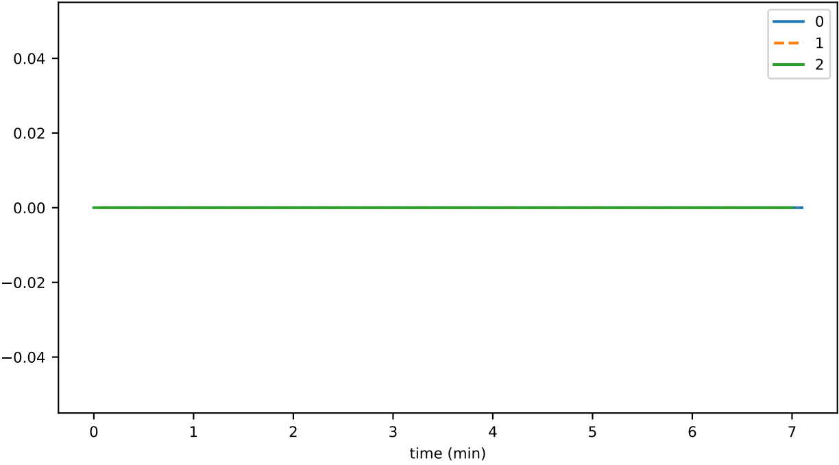
SmartContractService:SuccessfulTransactionDuration_sum
