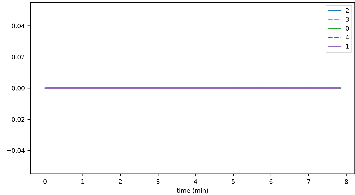
eventDelay_1_hashingMAX
