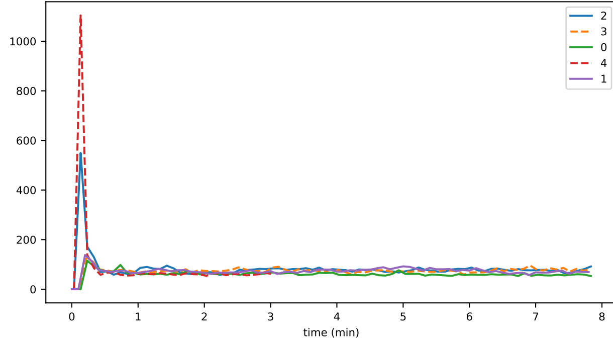
eventDelay_1_hashing
