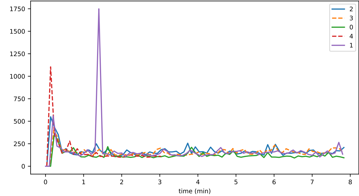
eventDelay_1_hashingMAX
