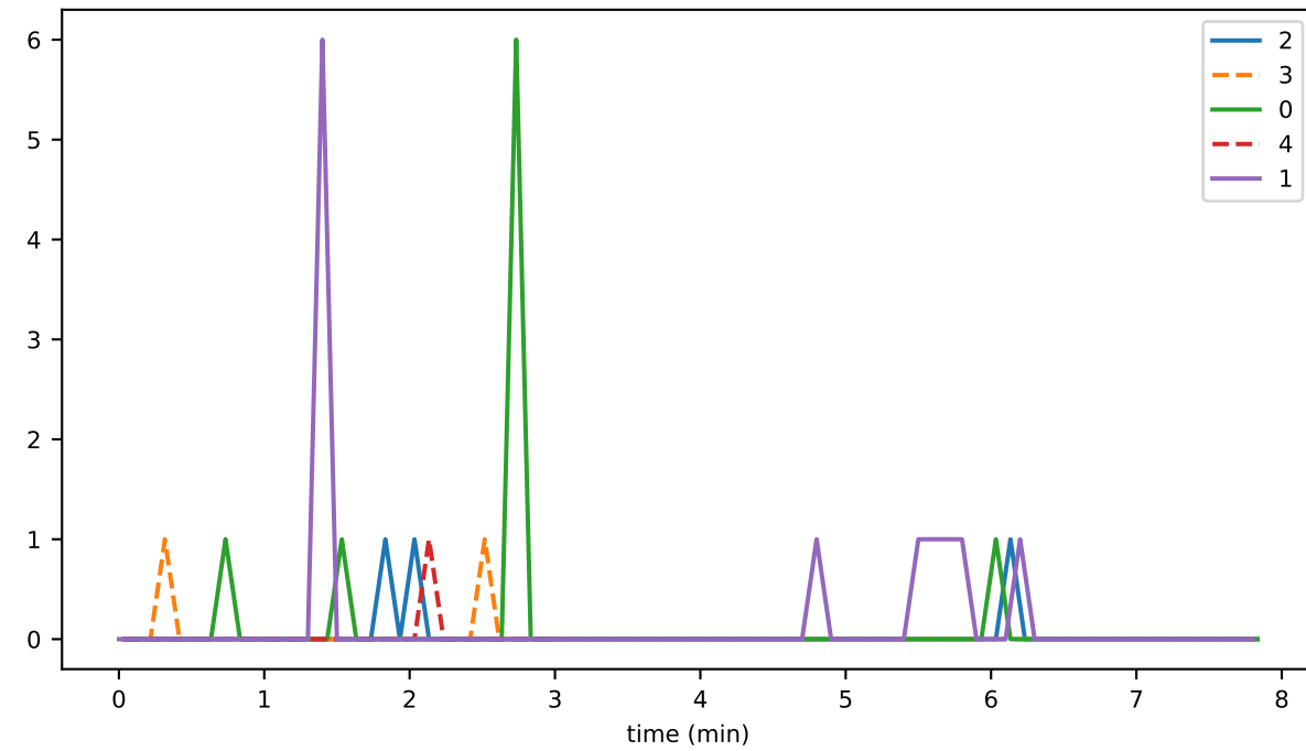
eventDelay_1_hashing
