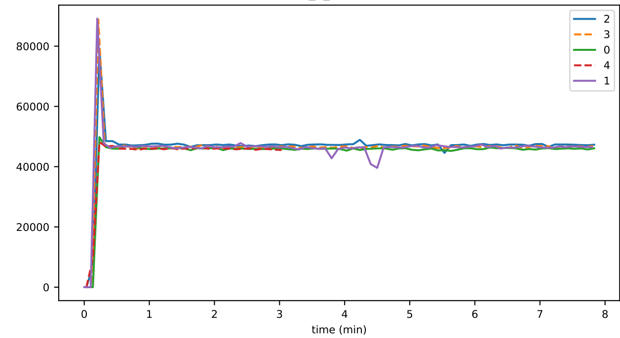
eventDelay_5_orphanBufferMAX
