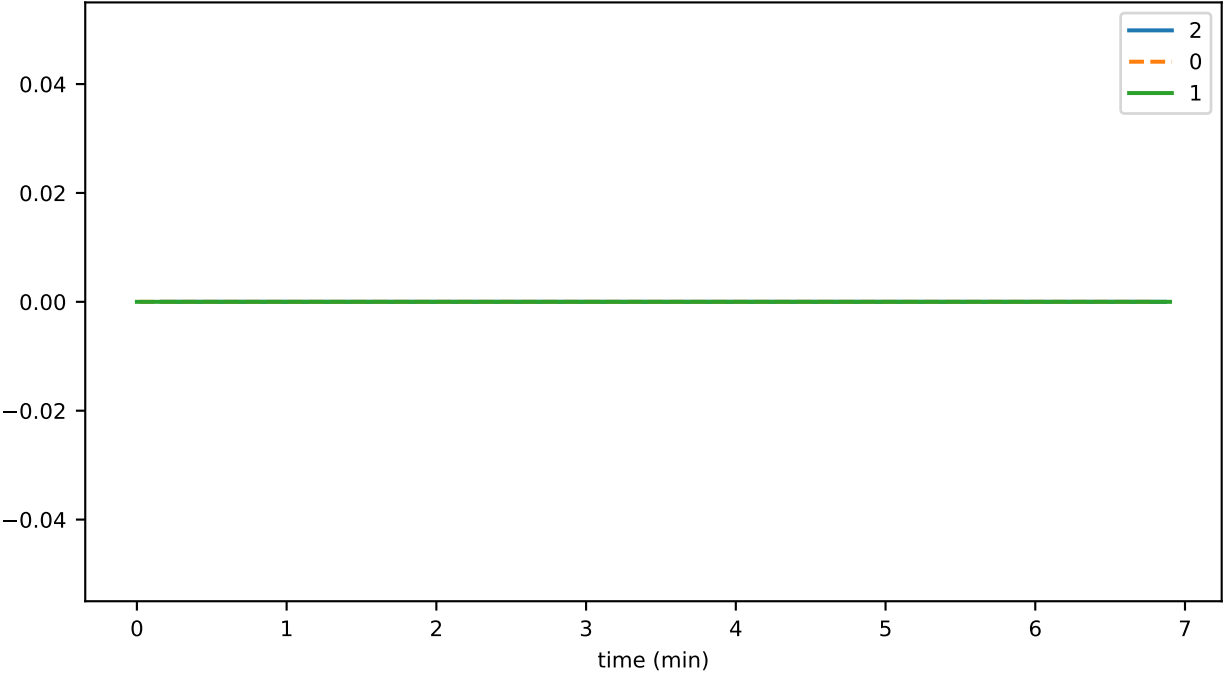
SmartContractService:SuccessfulTransactionDuration_avg
