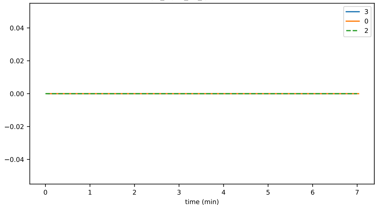
rpc_input_02_queueMinSize
