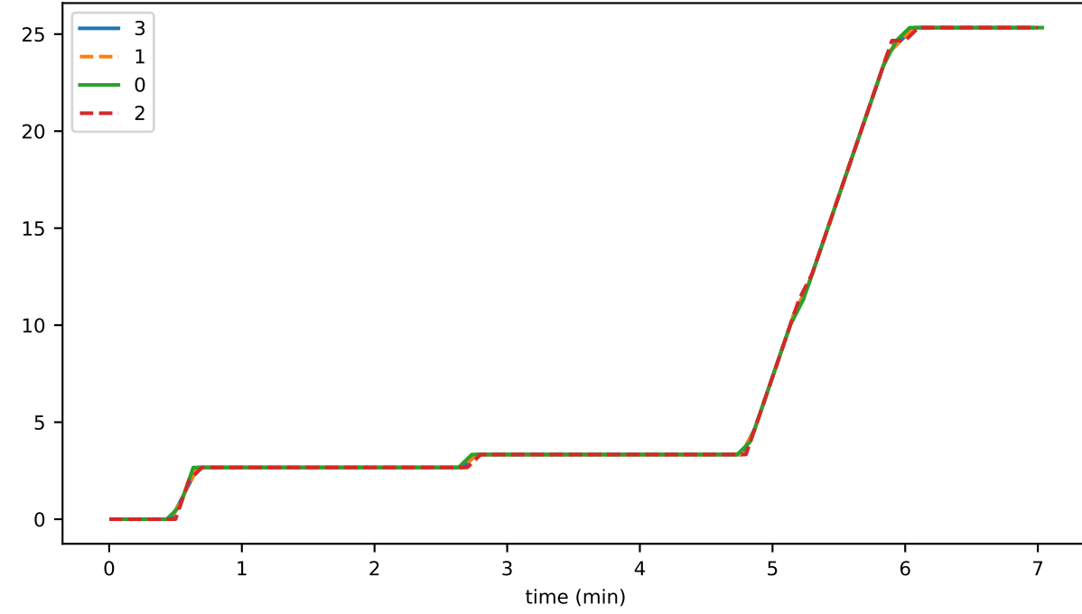
buffer_saturation
