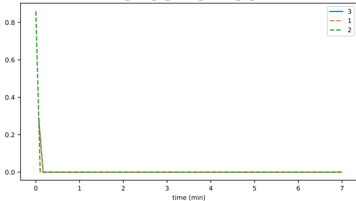
sync_phase_00_fraction_RECEIVING_EVENTS
