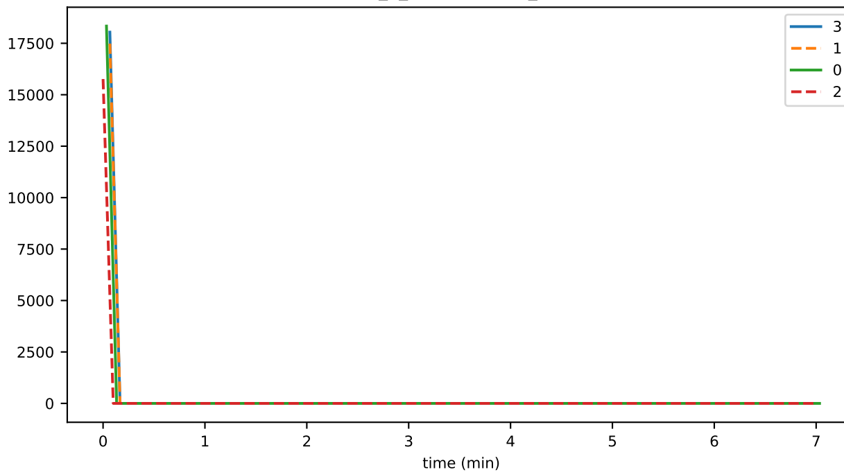
eventDelay_3_deduplication_storageMAX
