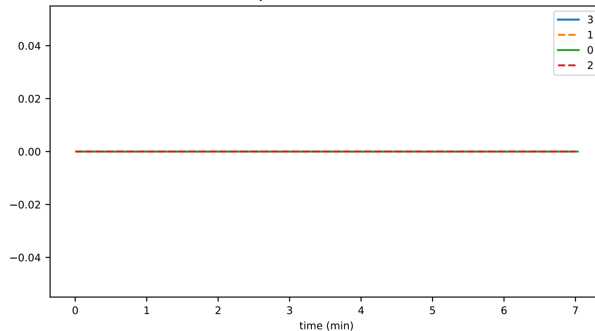
historyProofTransWMetaToFailCnt
