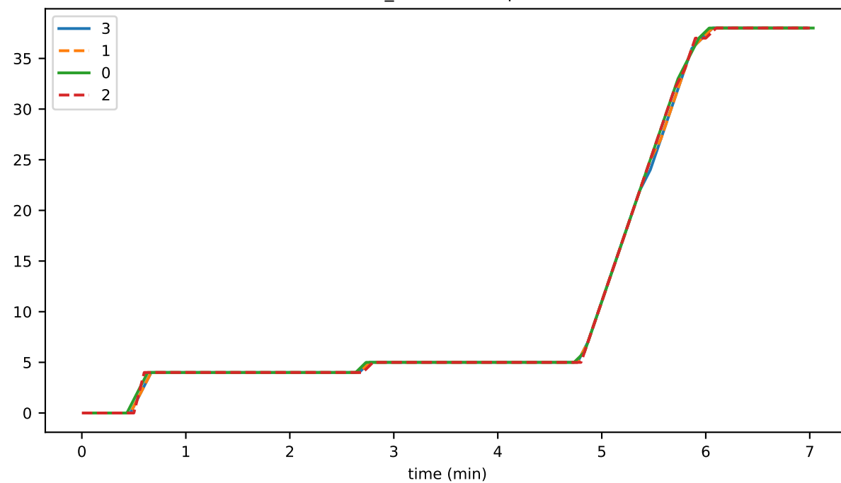
buffer_numBlocksOpened
