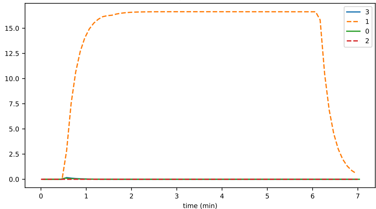
tokenAssociationsMaxNumber
