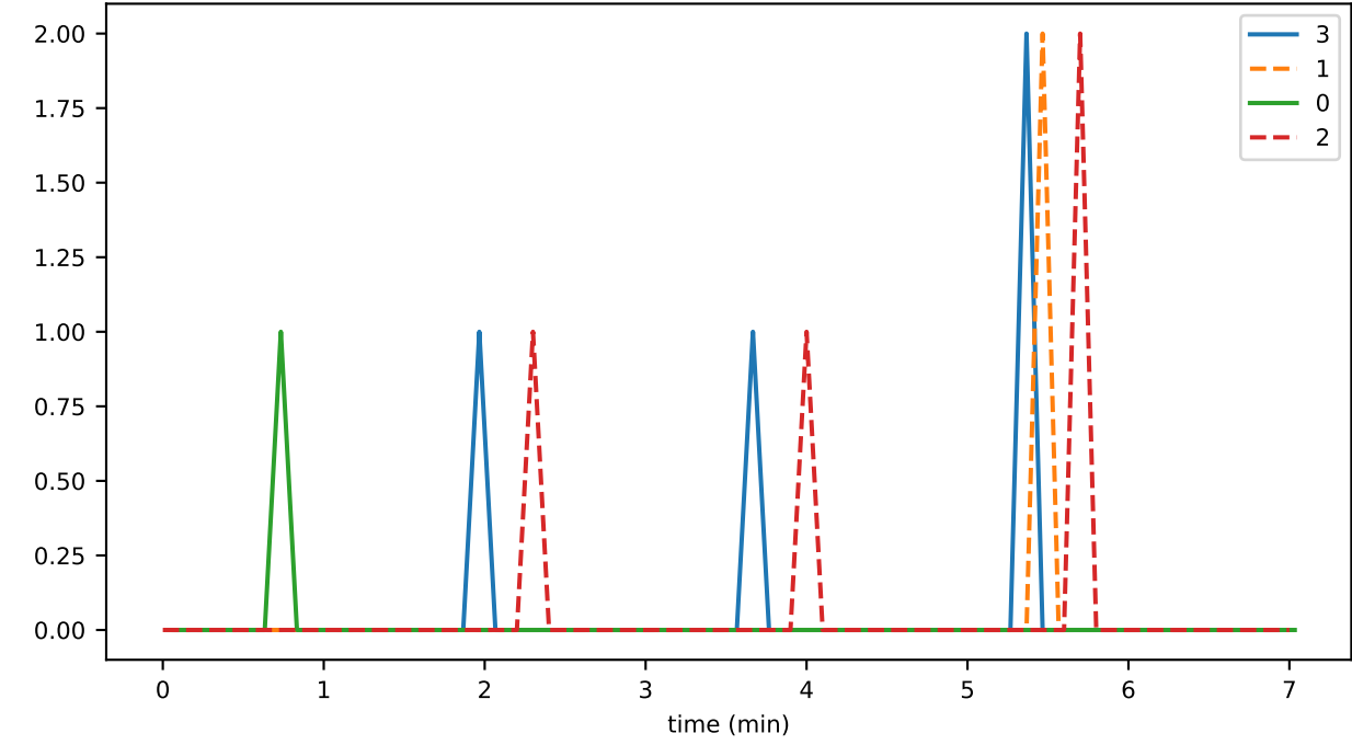
bufferedPriorityTransactions
