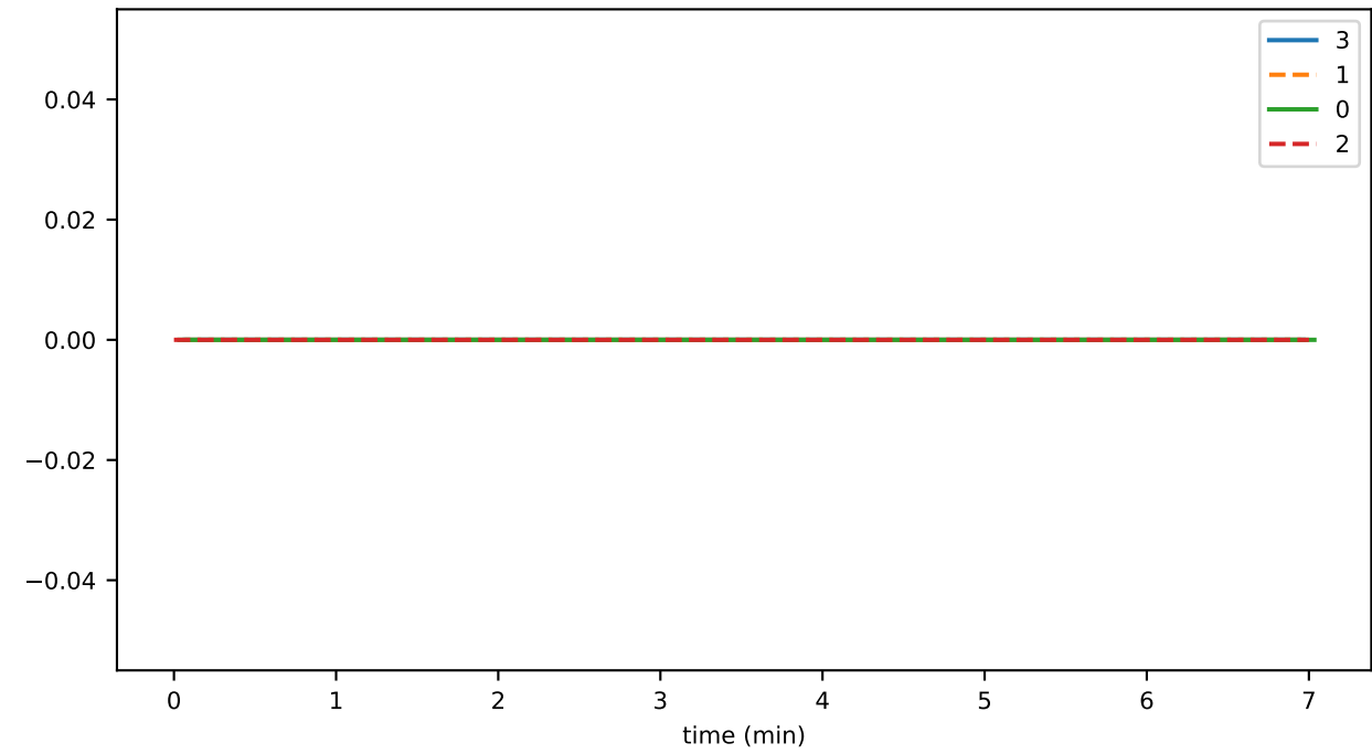
ds_files_level_5_hashesFileSizeByLevelMb_state
