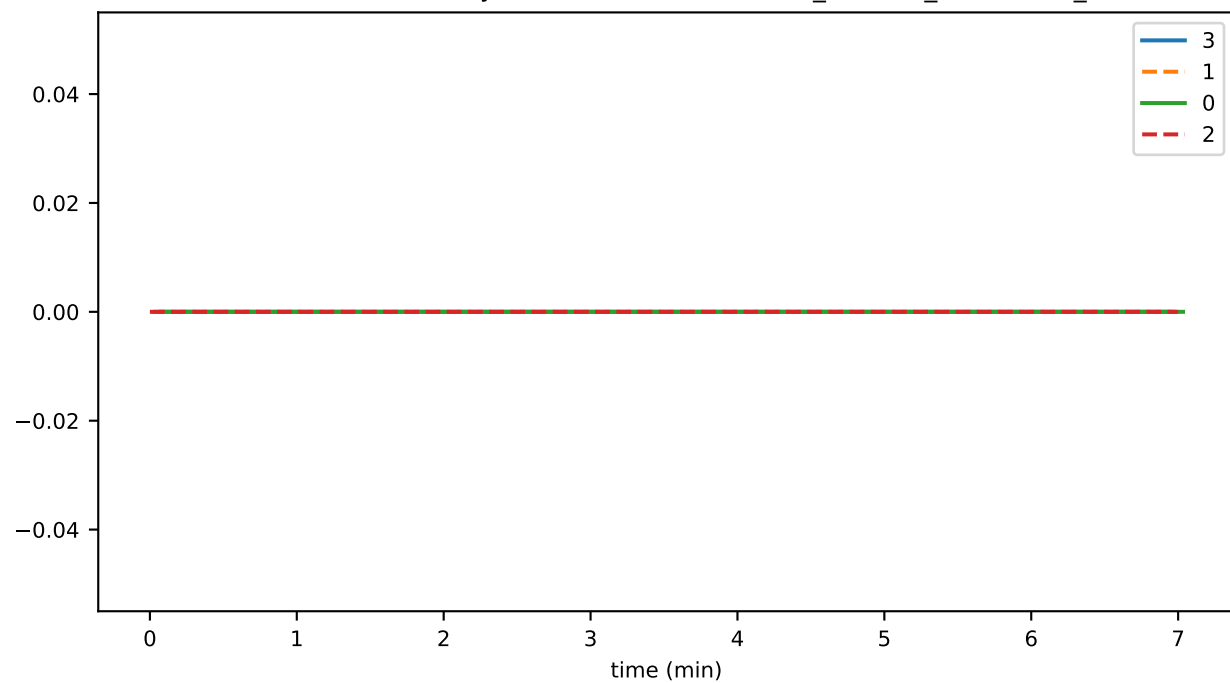
SmartContractService:SystemContractMethodCall_FREEZE_UNFREEZE_failed
