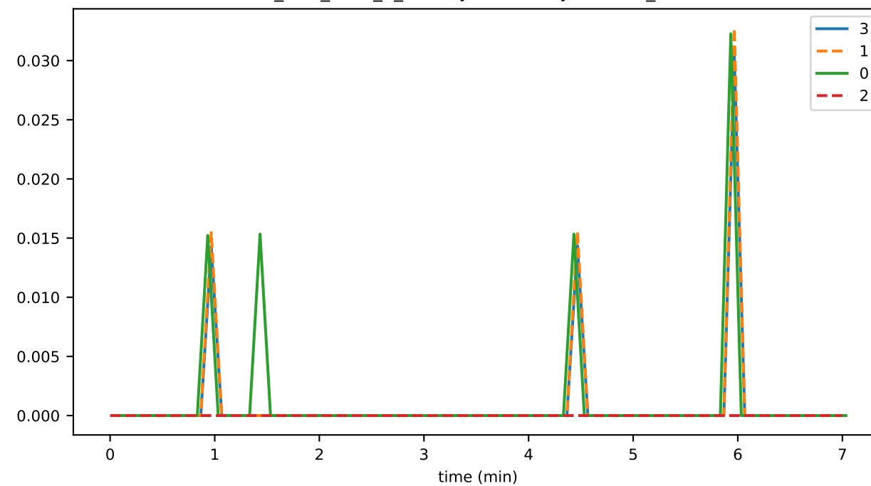
ds_files_level_2_leafKeysFileSizeByLevelMb_state
