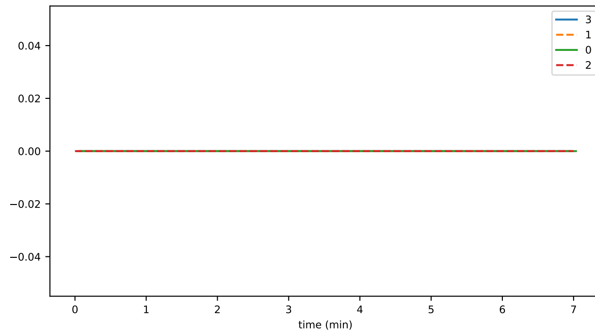
eventsWithInvalidParents
