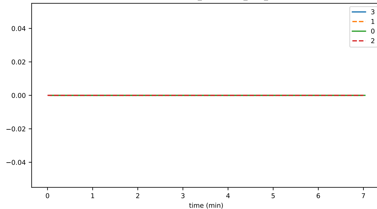
transH_per_sec
