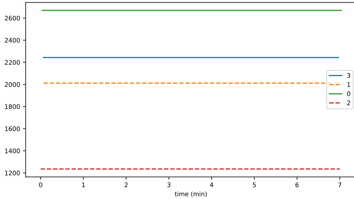
eventDelay_5_orphanBuffer_storage
