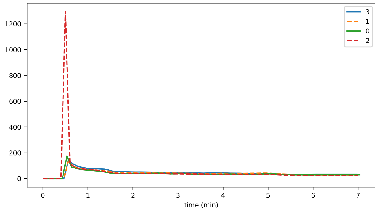
uptimeComputationTime
