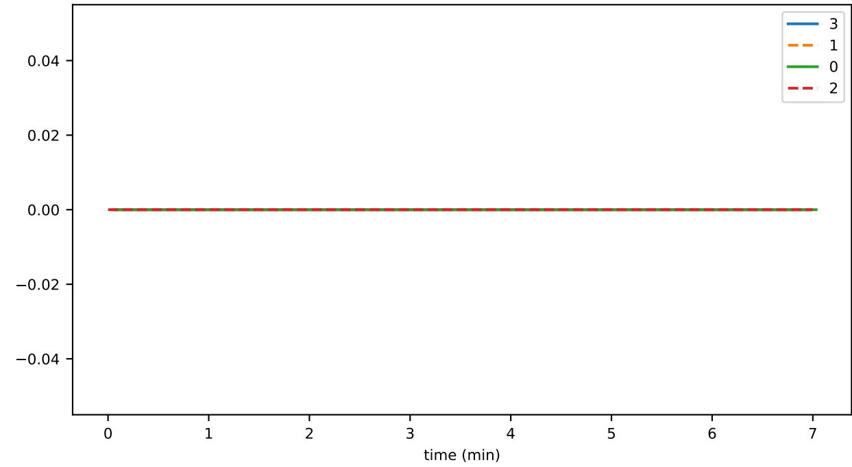
SmartContractService:OpsDuration_PerTxn_count
