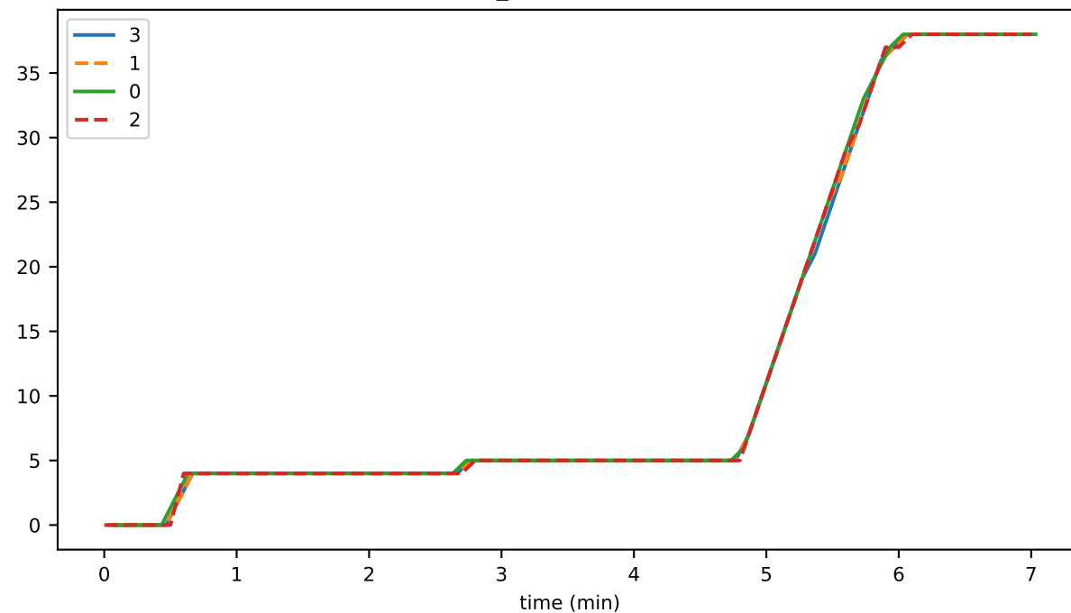
buffer_numBlocksOpened
