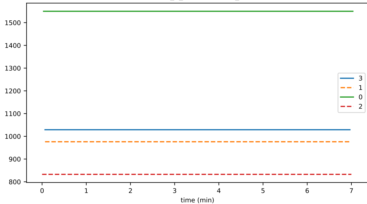
eventDelay_3_deduplication_storage
