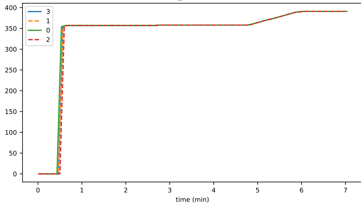
buffer_numBlocksMissing
