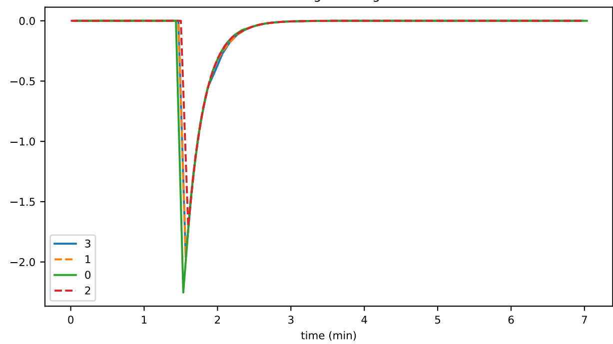
stateSignatureAge
