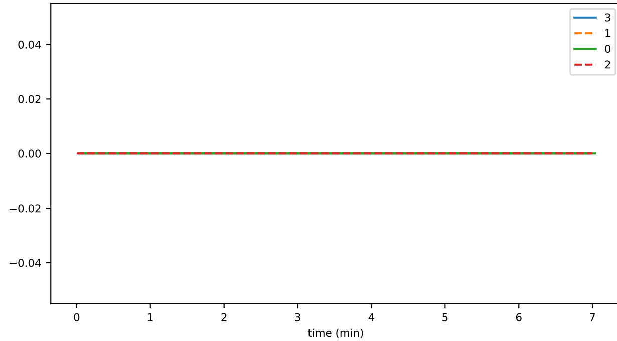
ds_files_level_4_leavesFileSizeByLevelMb_state
