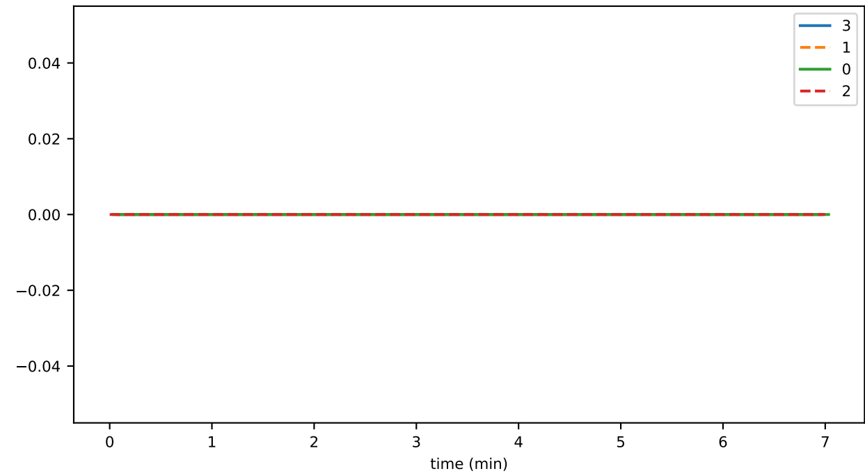
recordHashes_lowestBlock
