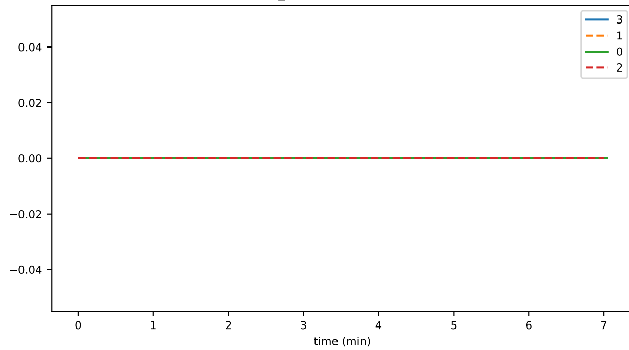
conn_activeConnectionCount
