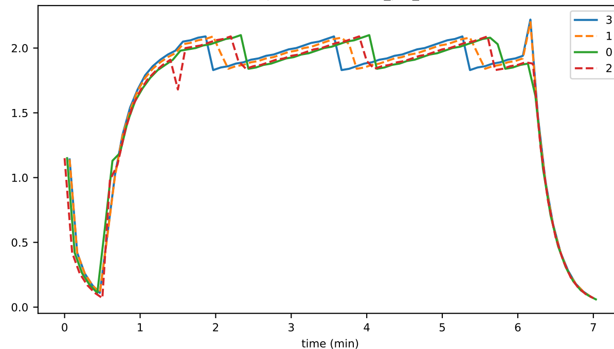
statesIneligibleForDeletion
