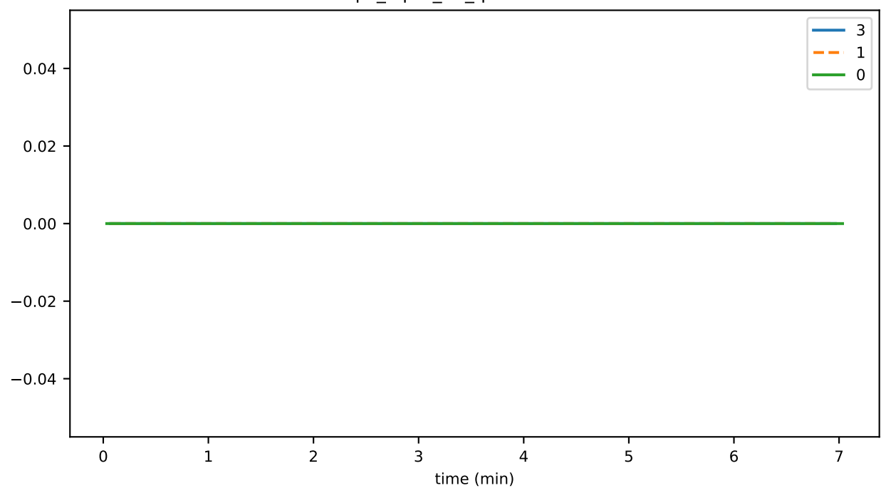
rpc_input_02_queueMinSize
