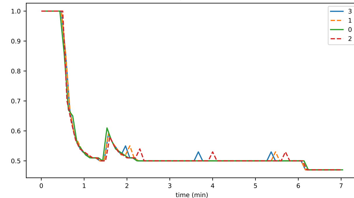
vmap_lifecycle_familySizeBackpressureMs_state
