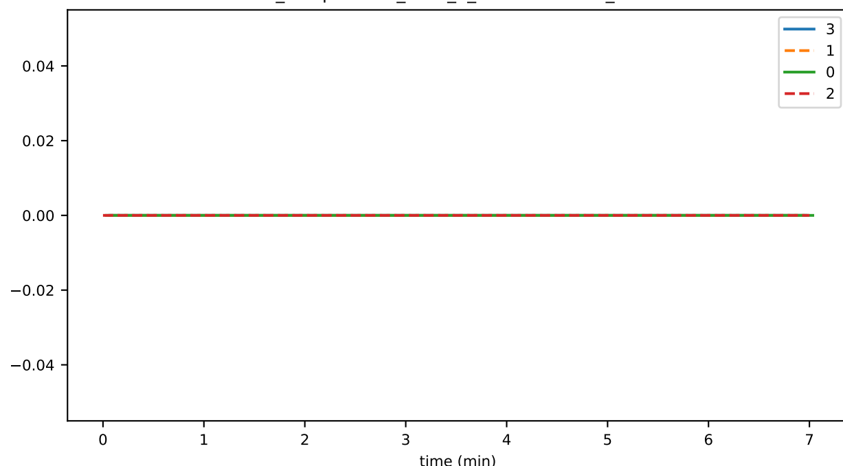
ds_compactions_level_0_hashesTimeMs_state
