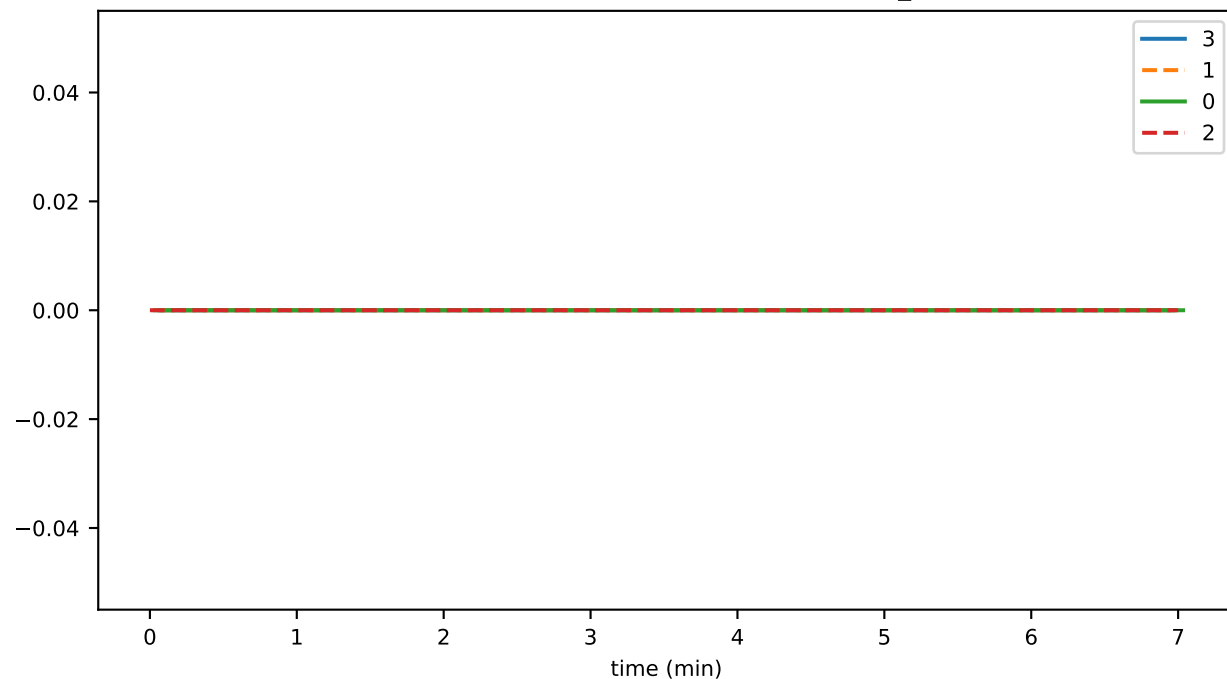
sstatesSigned_per_sec
