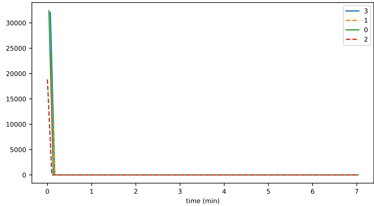
eventDelay_5_orphanBuffer_storageMAX
