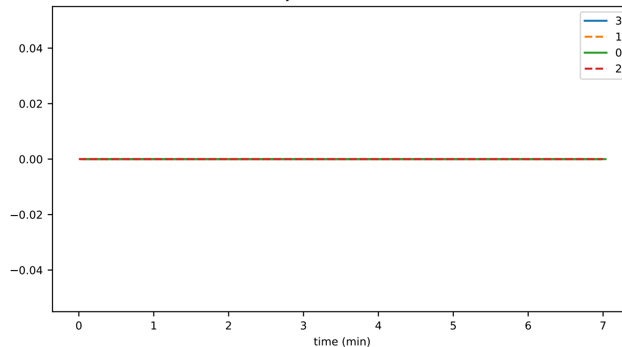
historyProofTransWasmToFailCnt
