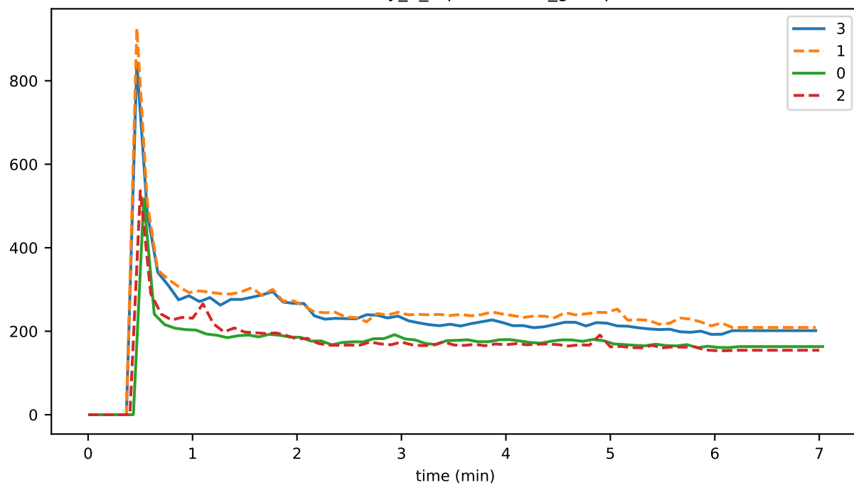
eventDelay_5_orphanBuffer_gossip
