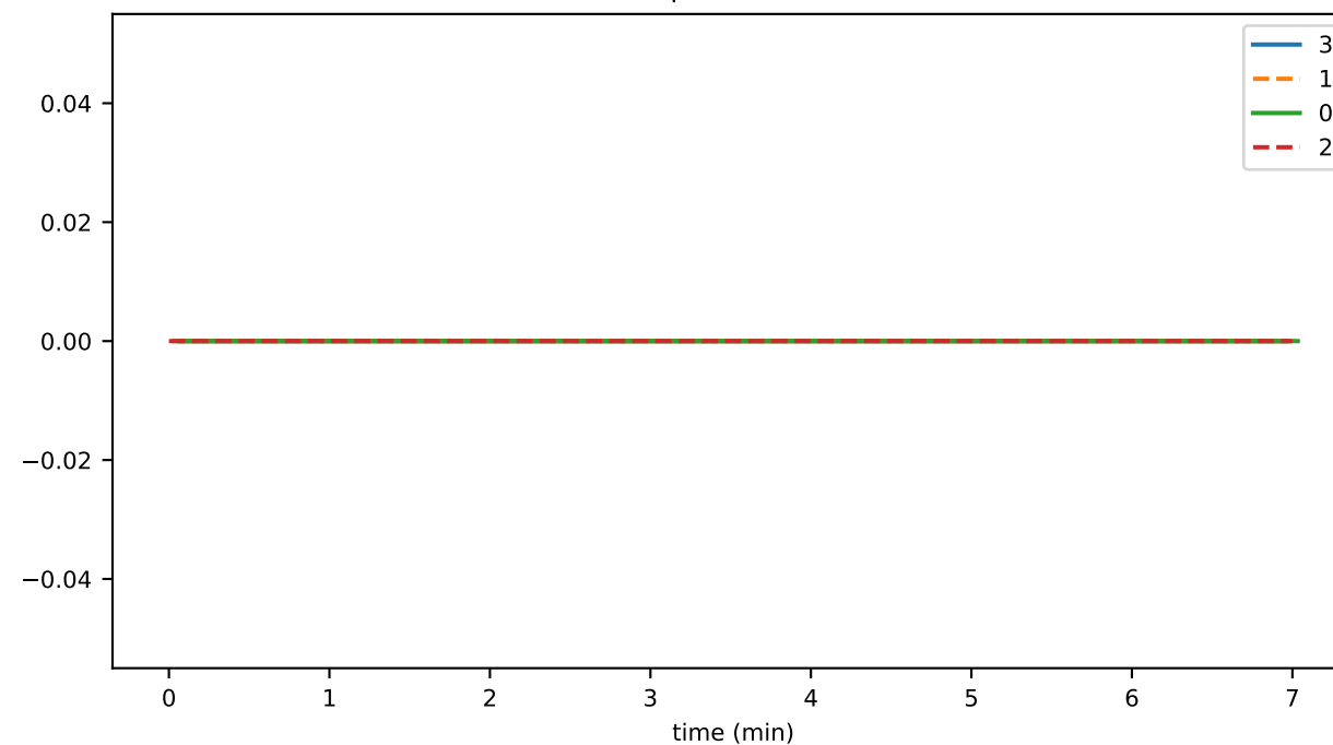
averageTimeToFullySignState
