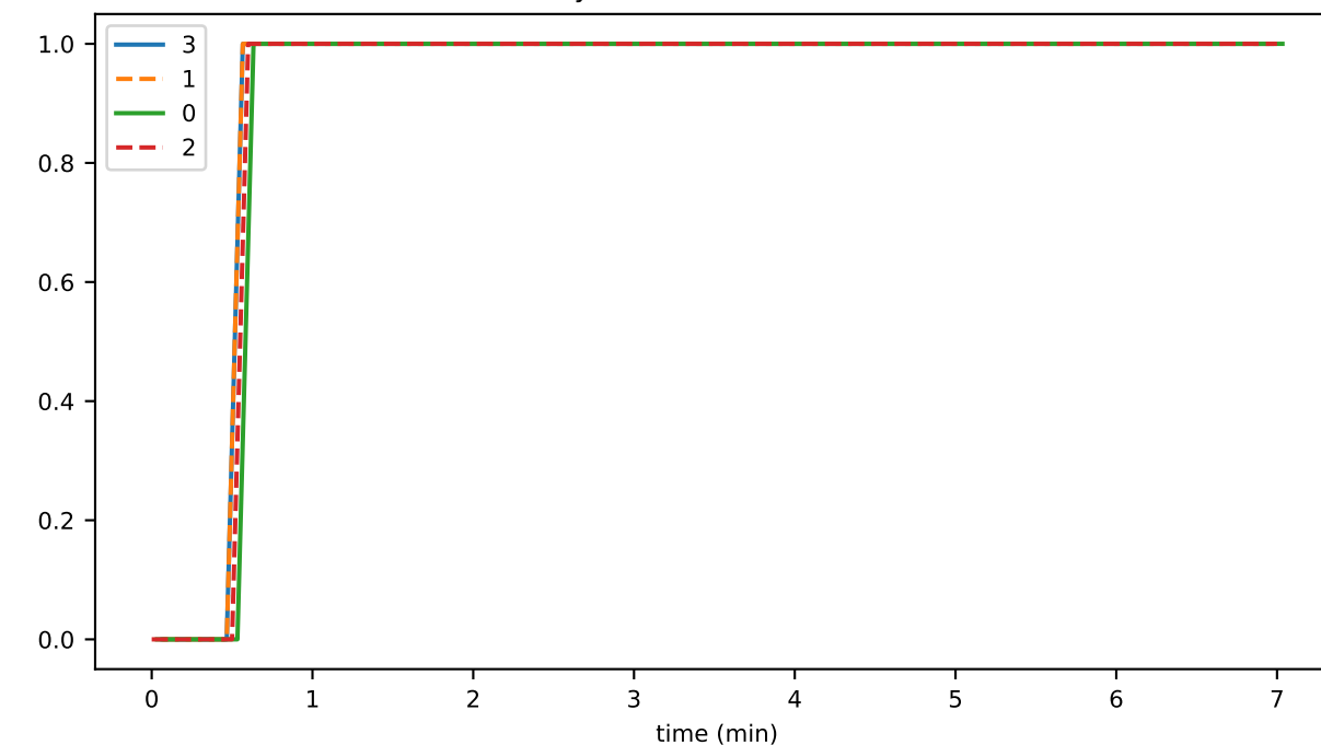
historyProofTransWMetaToFailCnt
