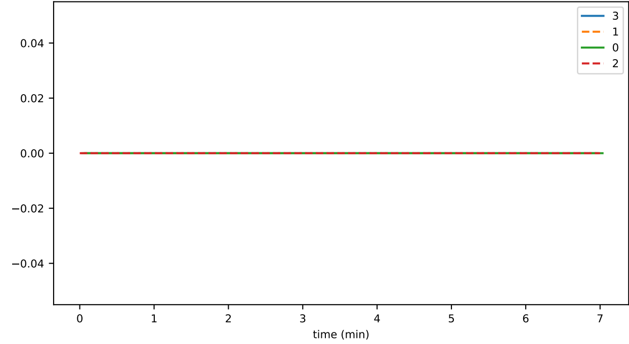
hasFallenBehind
