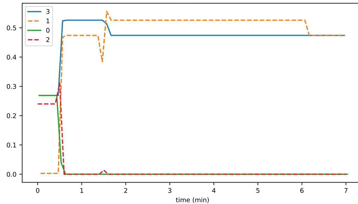
OrphanBuffer_unhandled_task_count
