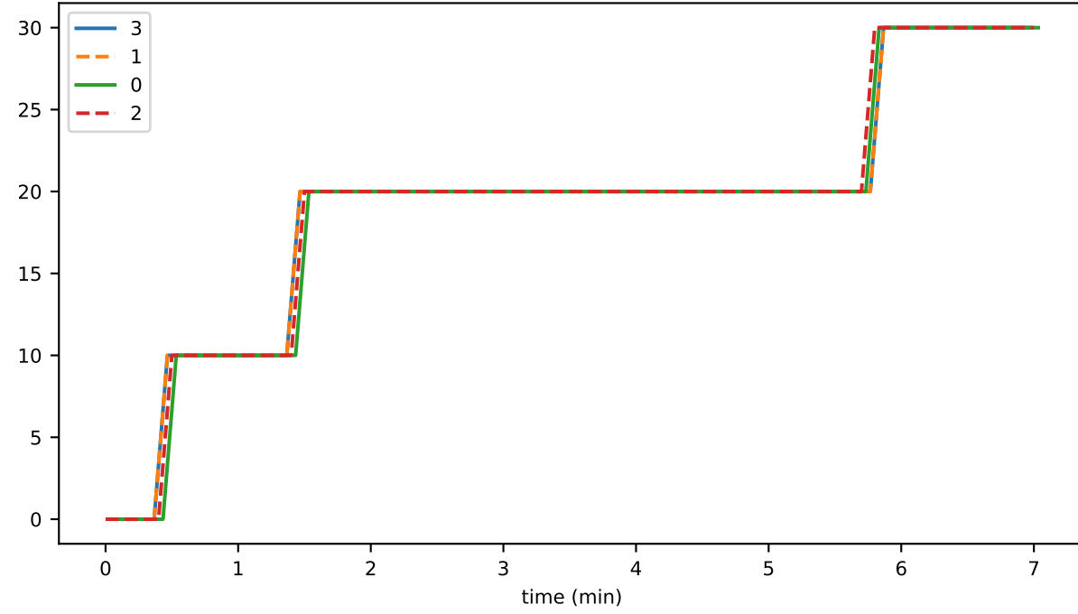
directMemInMB
