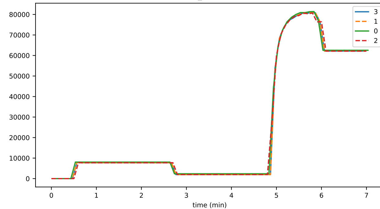
buffer_blockBytes
