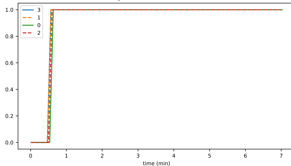
historyProofWrapsRetriesStarted
