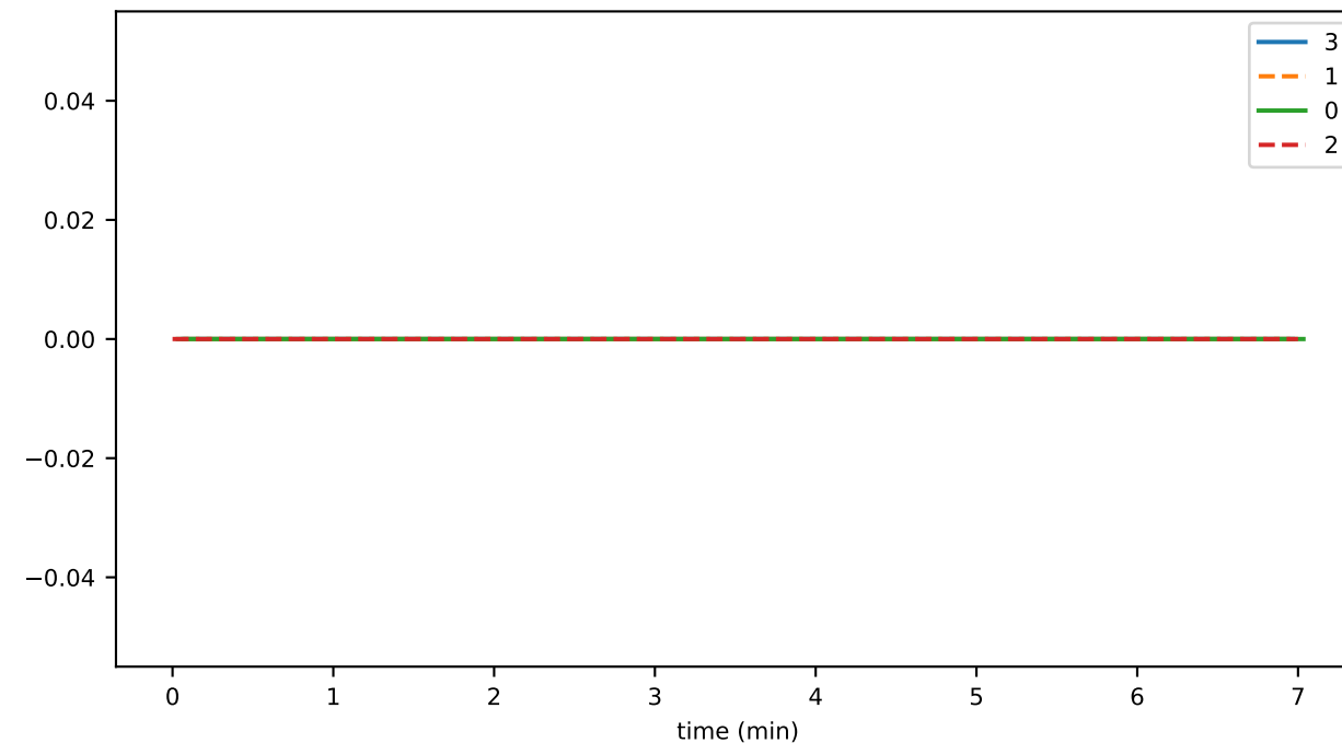
hapiFreeQueryLimitsPercentUsed
