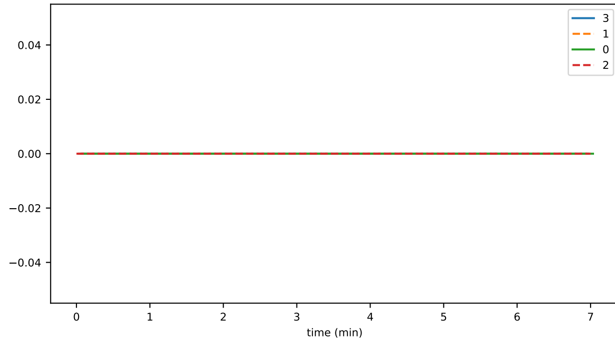
ds_files_level_4_leavesFileSizeByLevelMb_state
