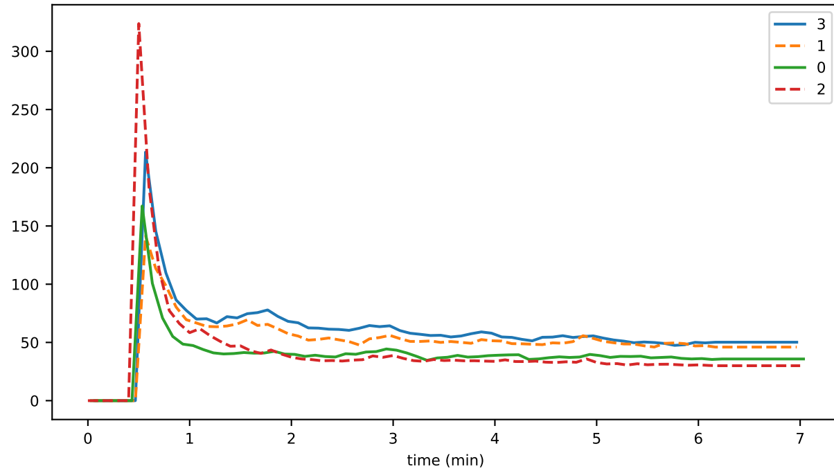
eventDelay_5_orphanBuffer_storage
