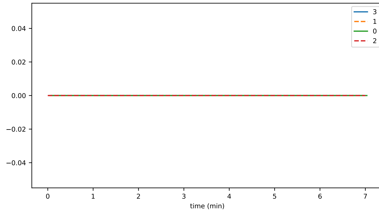
dupEvPercent
