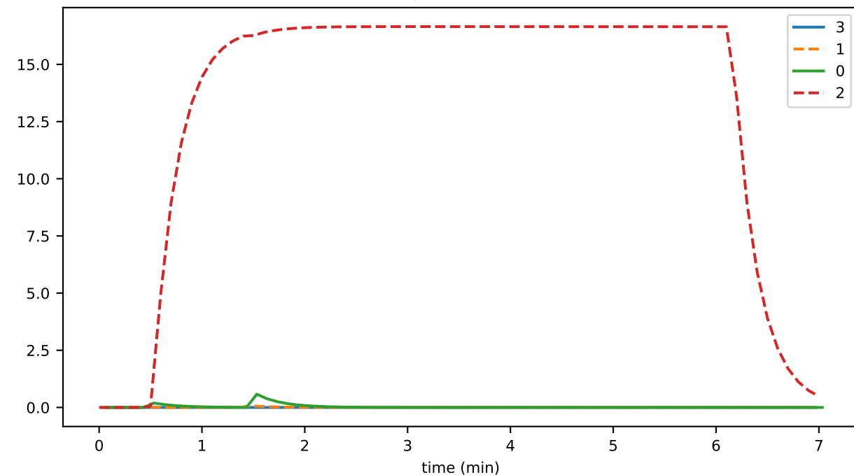
tokenAssociationsPercentUsed
