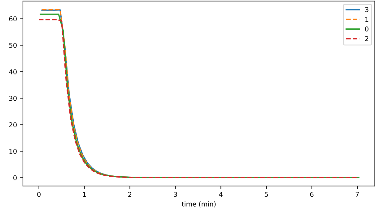
secGossipRoundtrip
