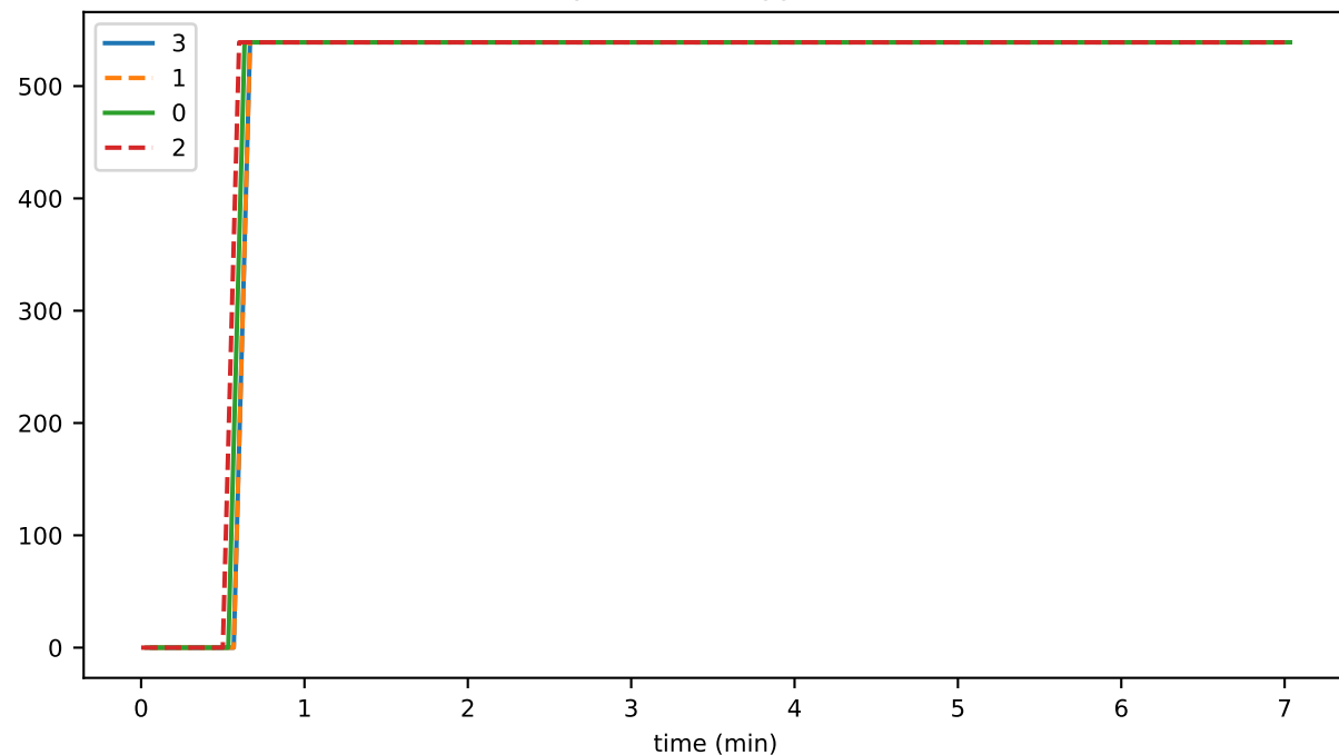
historyProofTransAggToFailMs
