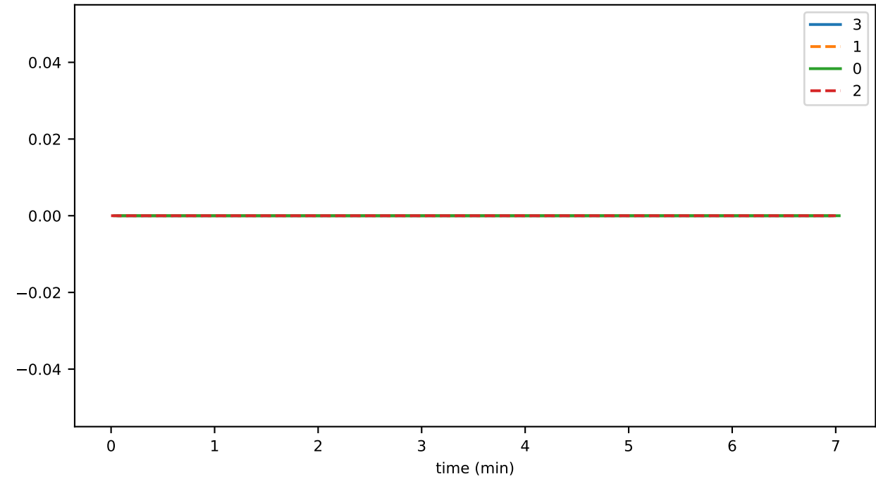
ds_files_level_5_hashesFileSizeByLevelMb_state
