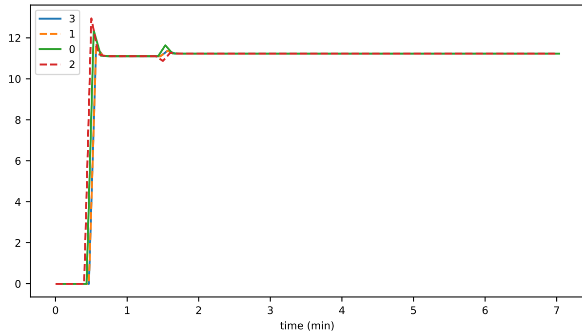
graphDepthUntilConsensus
