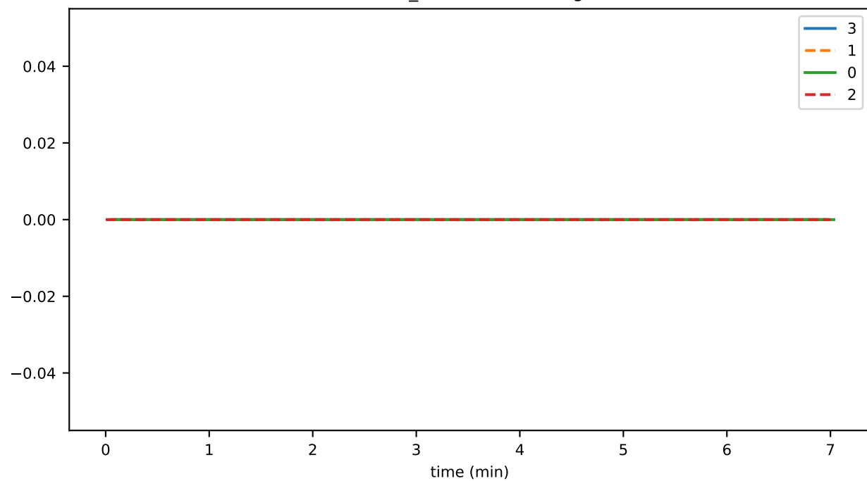
buffer_numBlocksMissing
