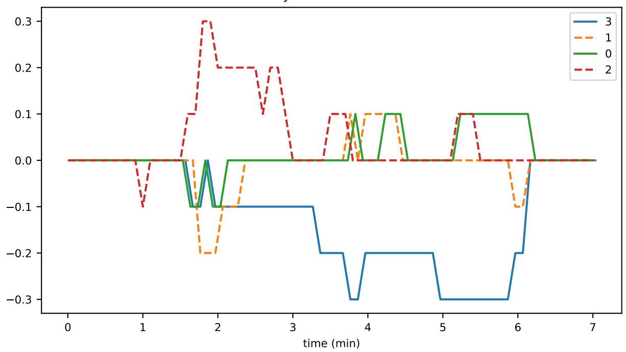
syncIndicatorDiff
