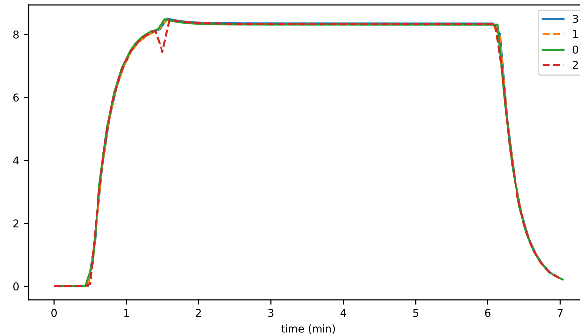
rounds_per_sec
