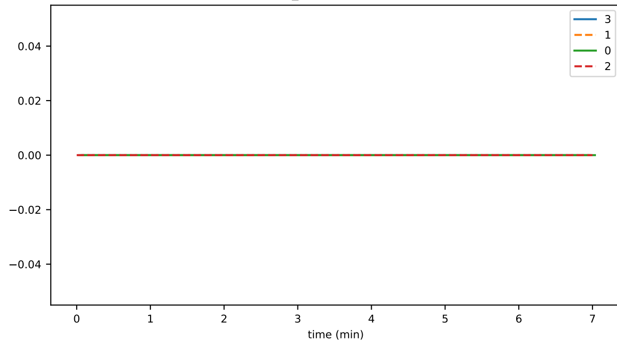
buffer_backPressureState
