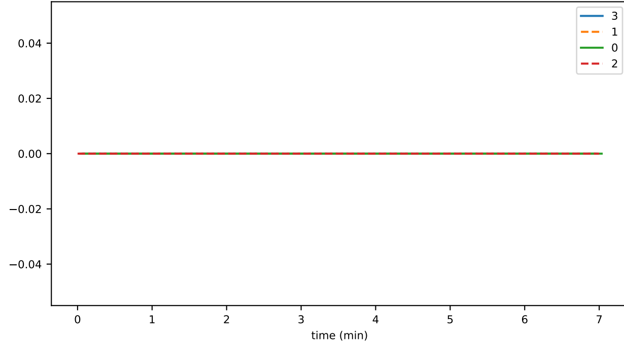
hapiThroughputLimitsPercentUsed
