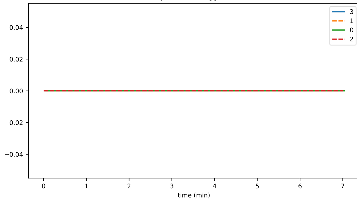
historyProofTransAggToFailMs
