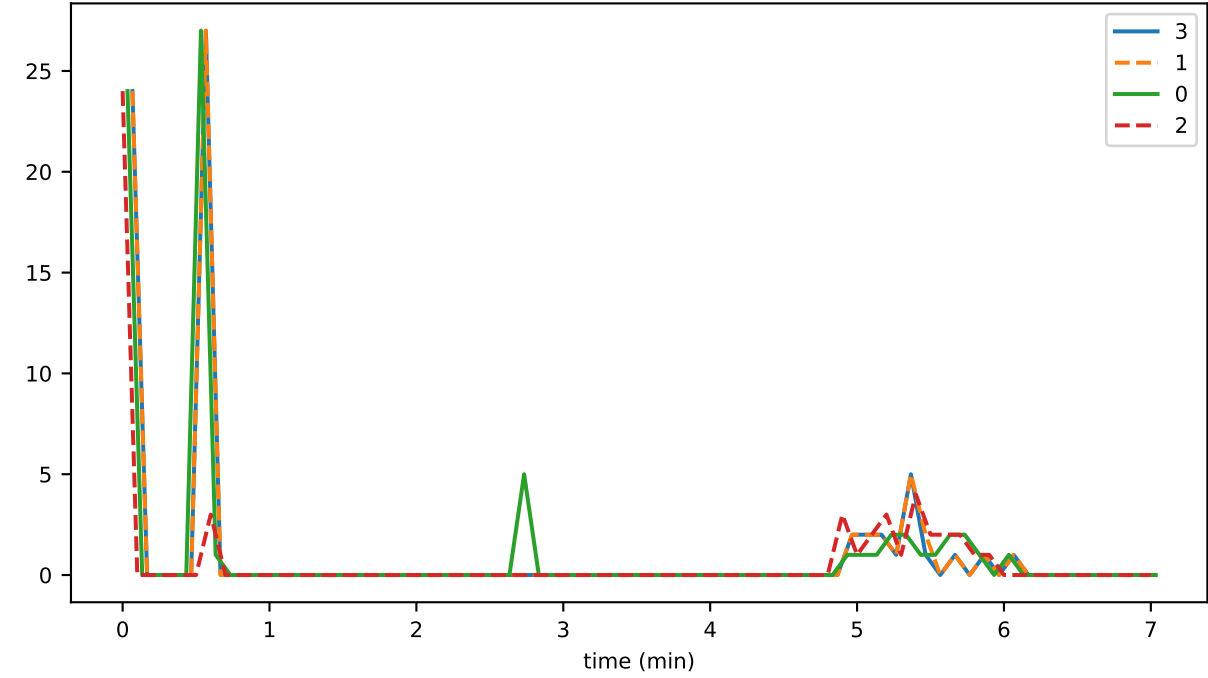
ds_reads_hashes_state
