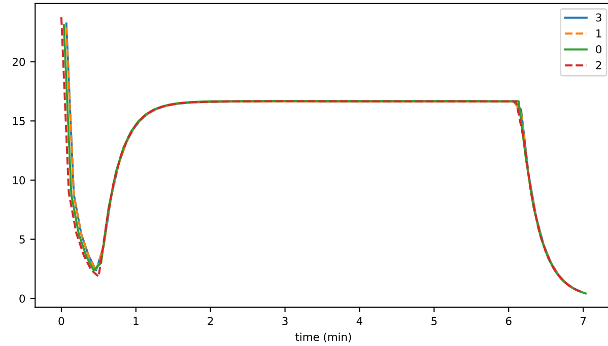
conn_activeConnectionCount
