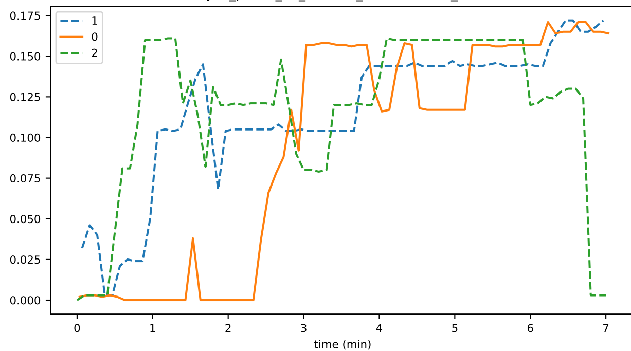
sync_phase_03_fraction_EXCHANGING_TIPS
