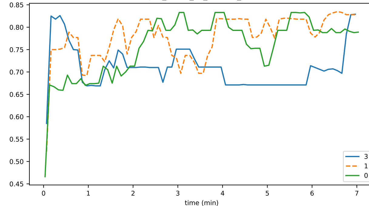
sync_phase_02_fraction_OTHER_FALLEN_BEHIND
