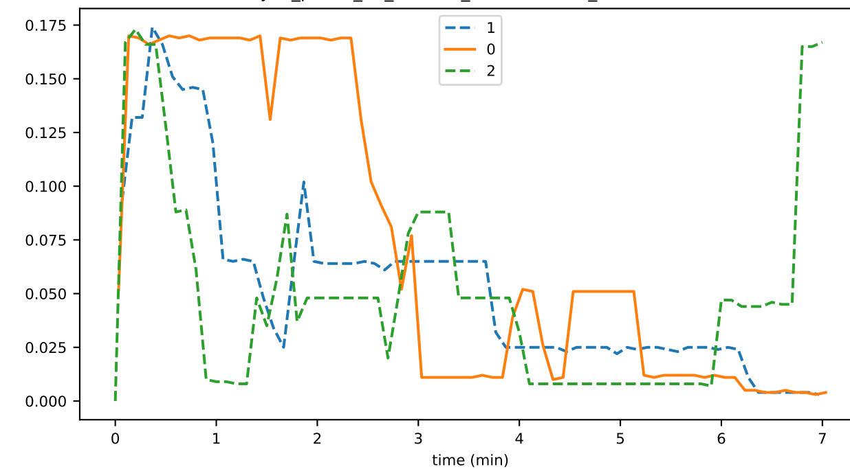
sync_phase_03_fraction_EXCHANGING_WINDOWS
