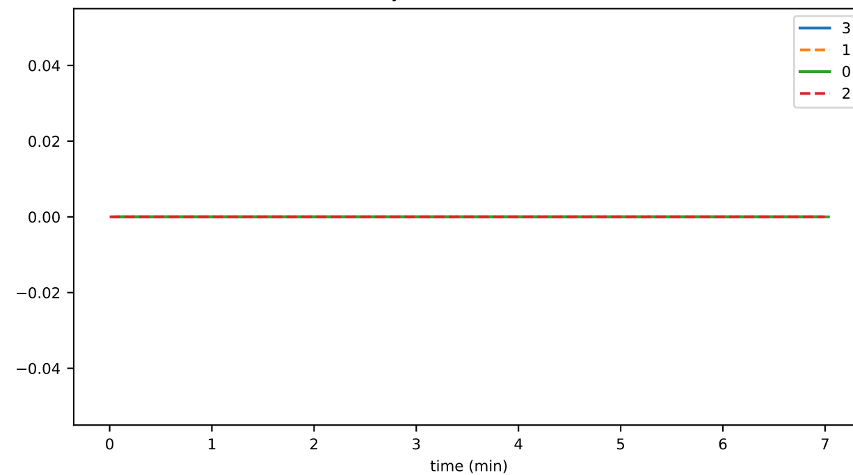
historyProofTransR1ToFailCnt
