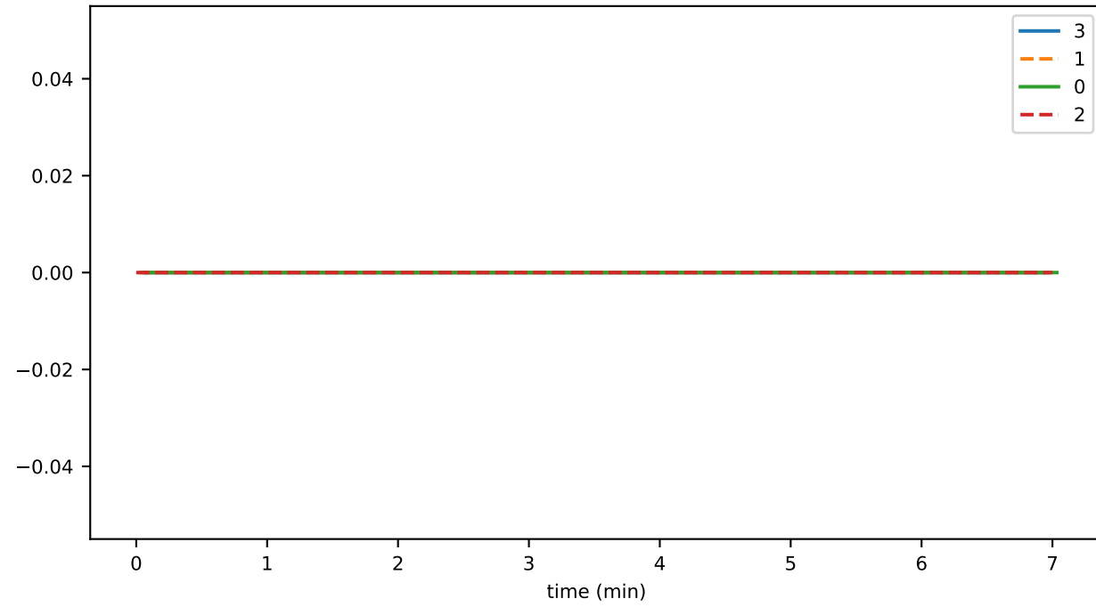
directMemInMB
