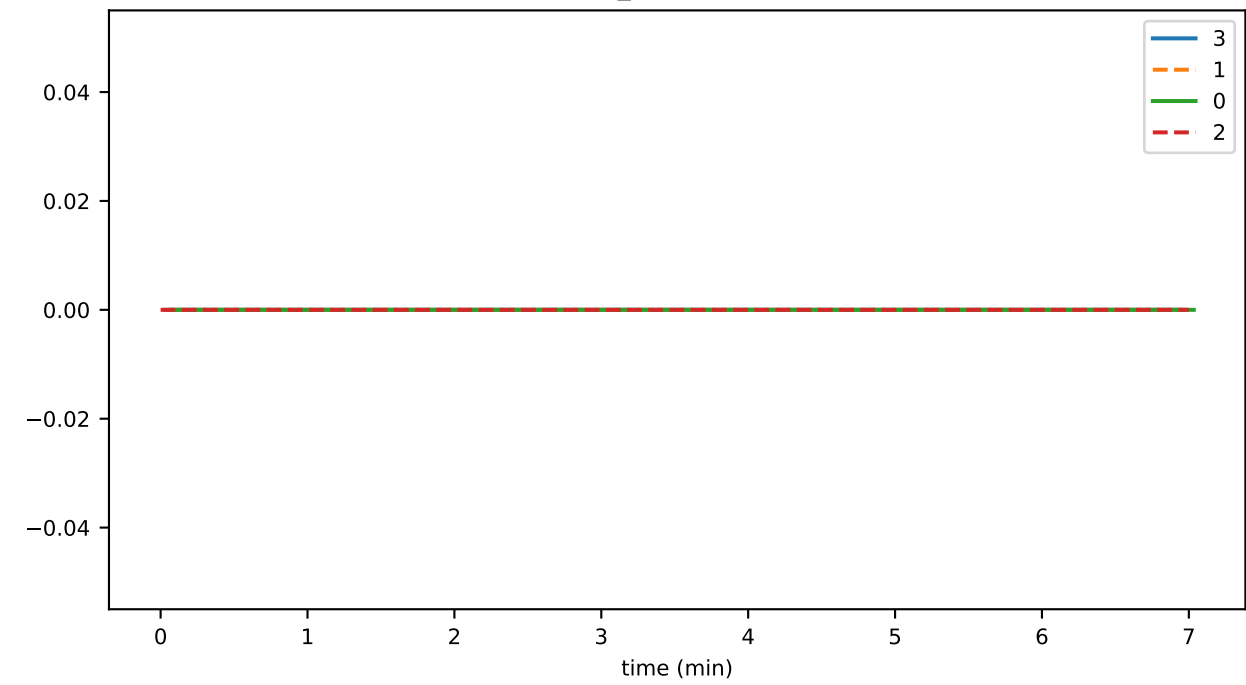
conn_activeConnIp
