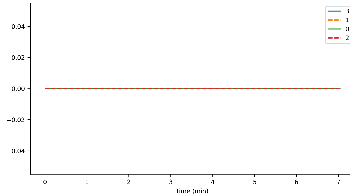
SmartContractService:FailedTransactionDuration_count
