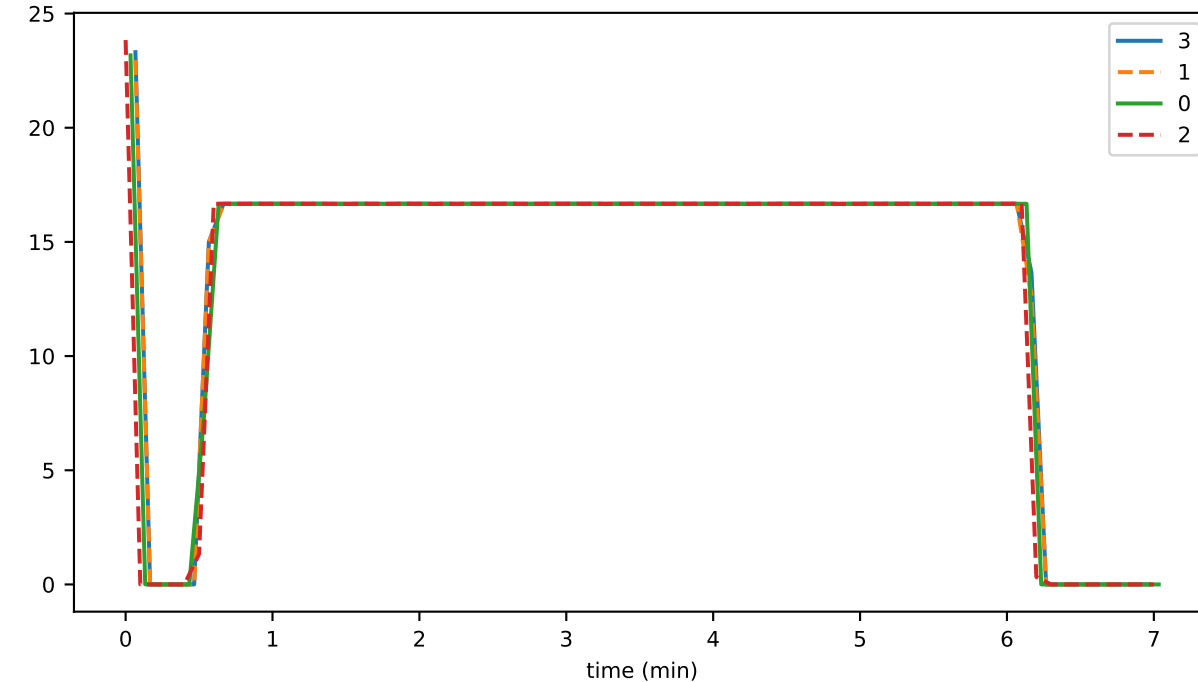
buffer_blockBytes
