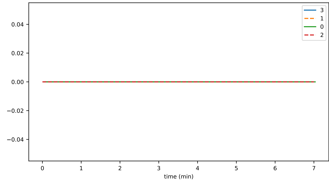
filesPercentUsed
