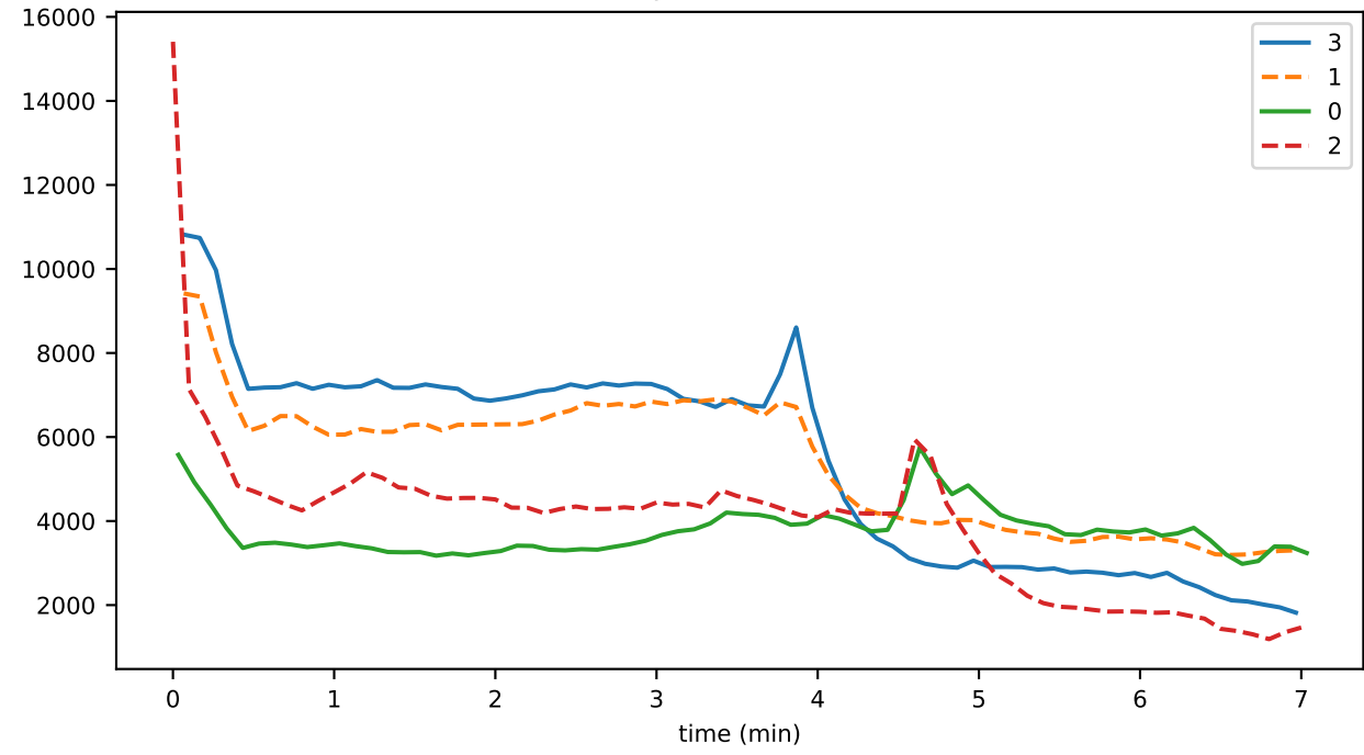
syncPermitsAvailable
