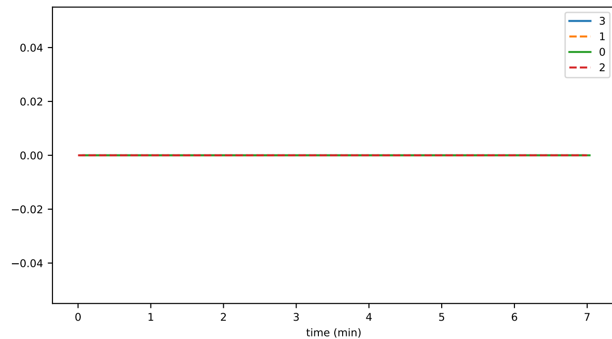
tokenAssociationsPercentUsed
