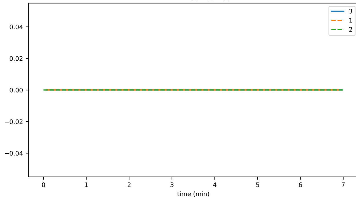
disconnects_per_sec_02
