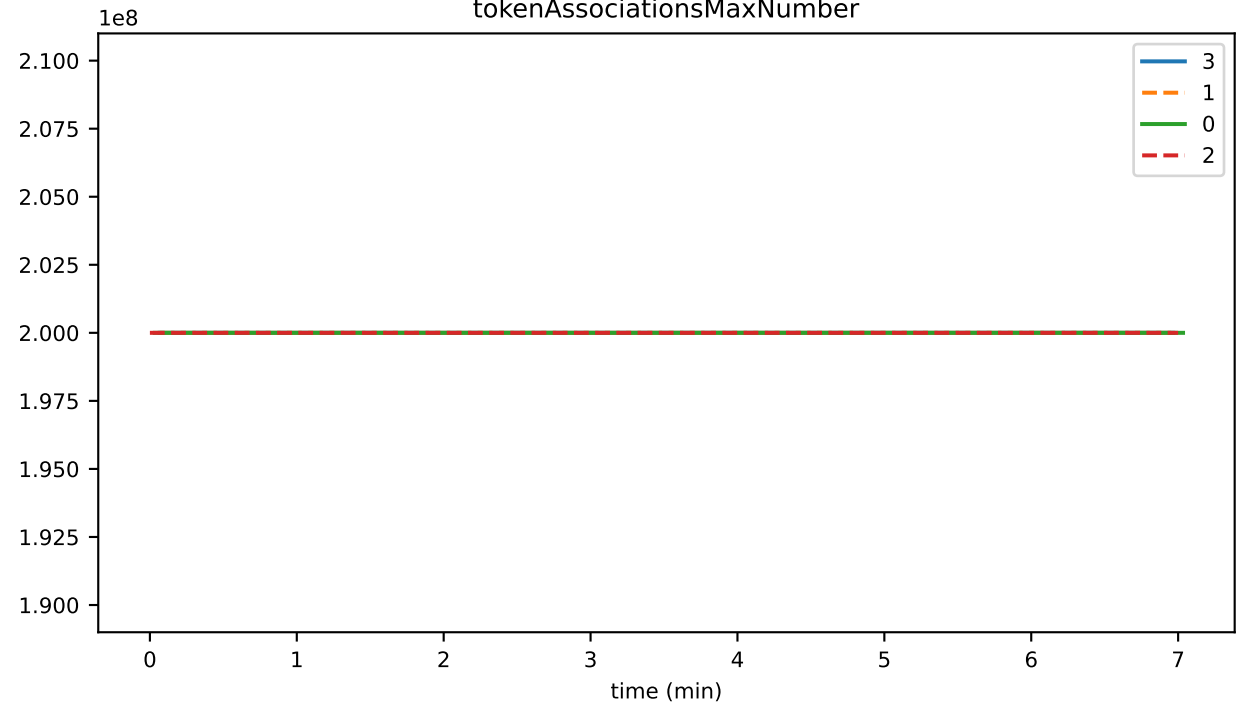
tokenAssociationsMaxNumber
