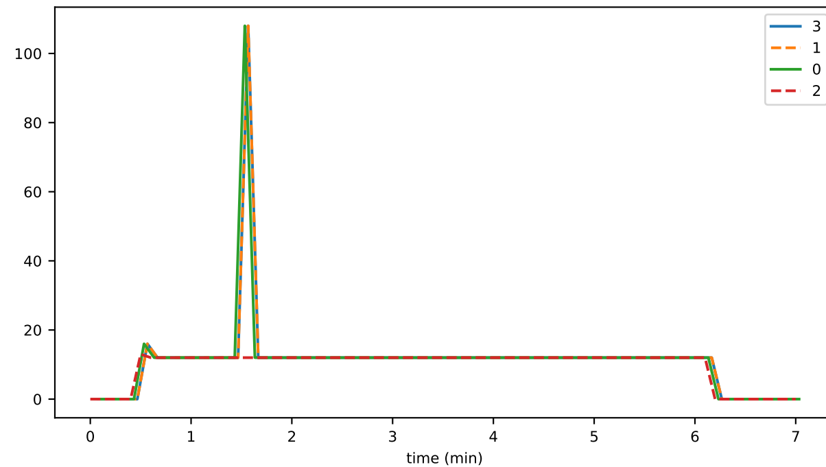
graphDepthUntilConsensusMAX
