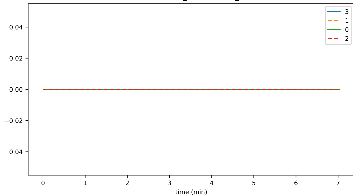
graphDepthUntilConsensus
