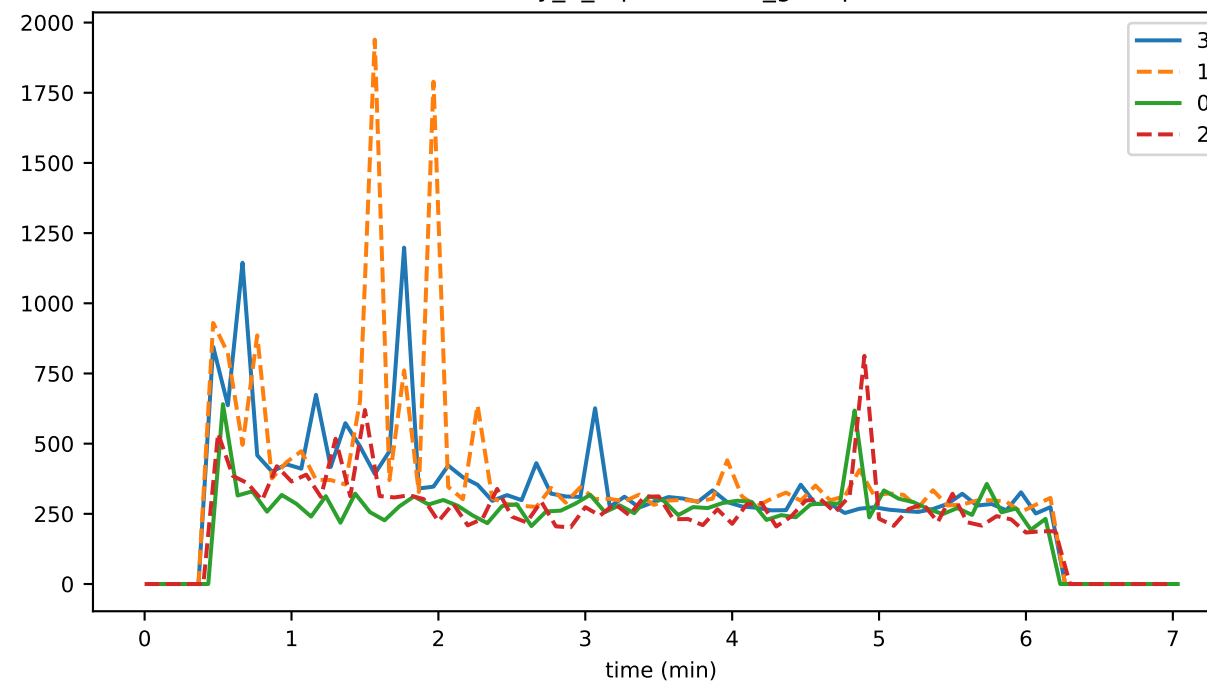
eventDelay_5_orphanBuffer_gossipMAX
