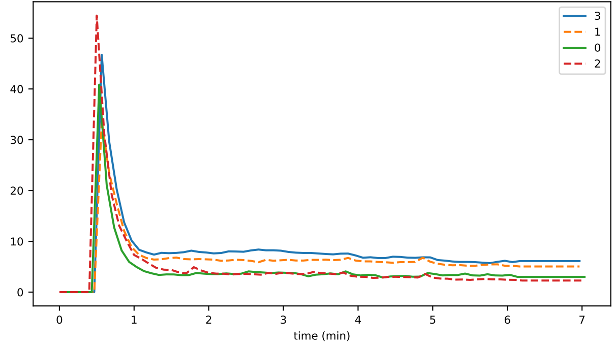
eventDelay_1_eventCreation_runtime
