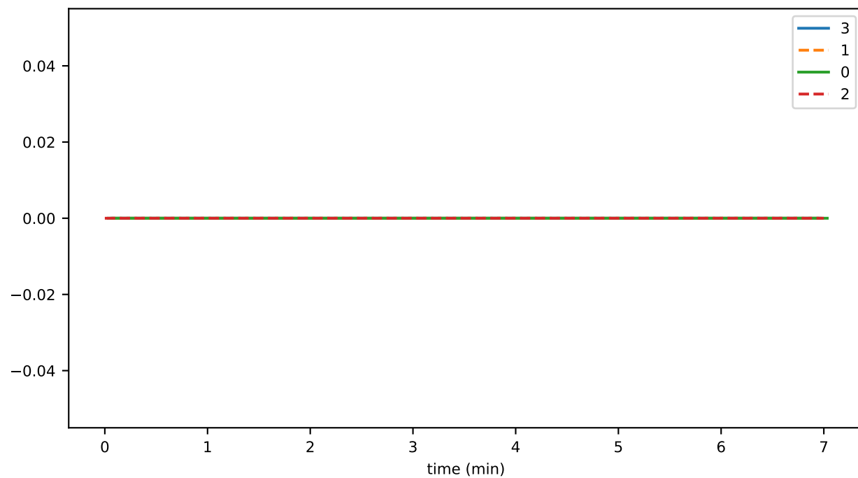
ParseErrUnknownFieldRcv
