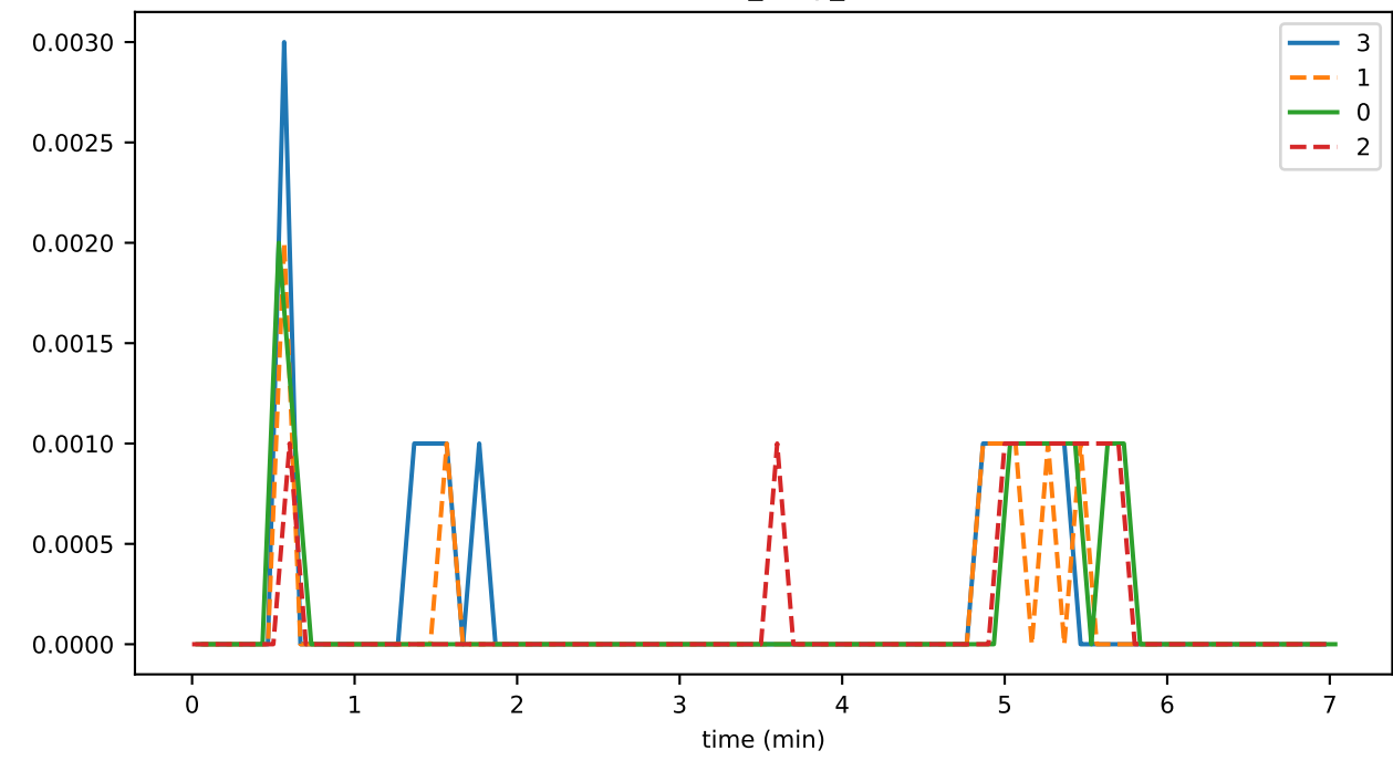
stateSignatureAge
