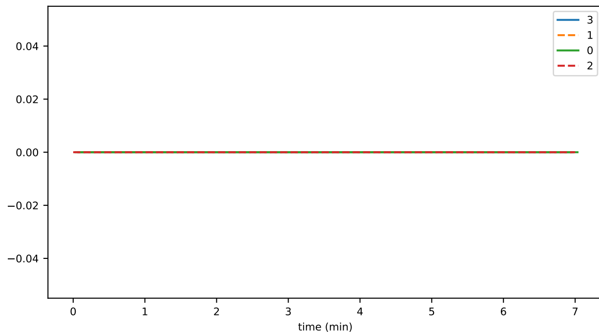
ParseErrUnknownFieldRcv
