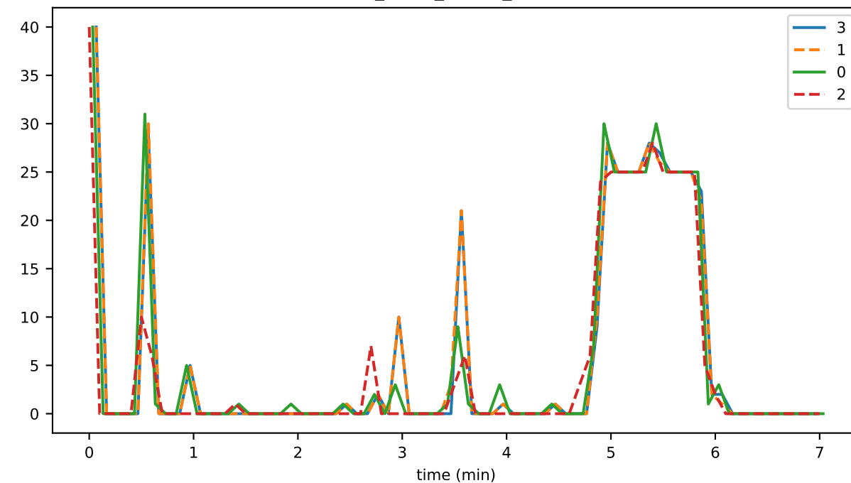
dupEvPercent
