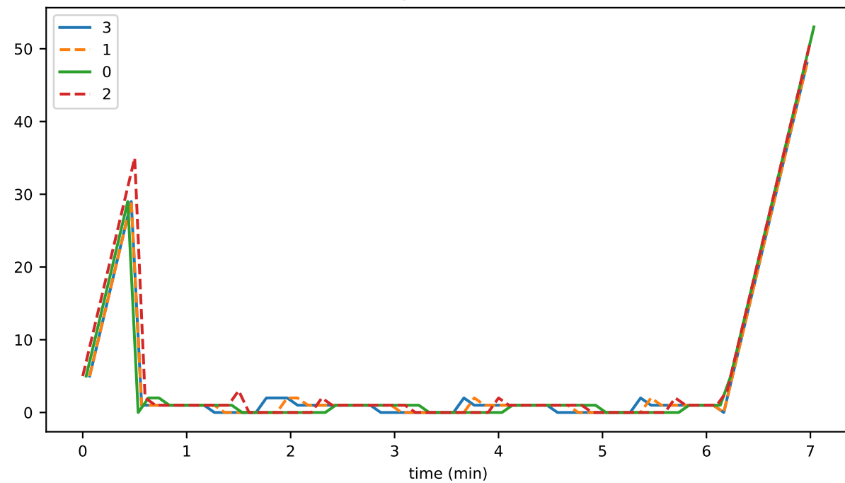
OrphanBuffer_busy_fraction
