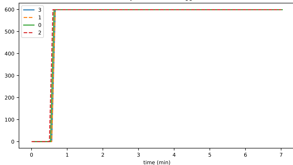
historyProofTransR3ToFailMs
