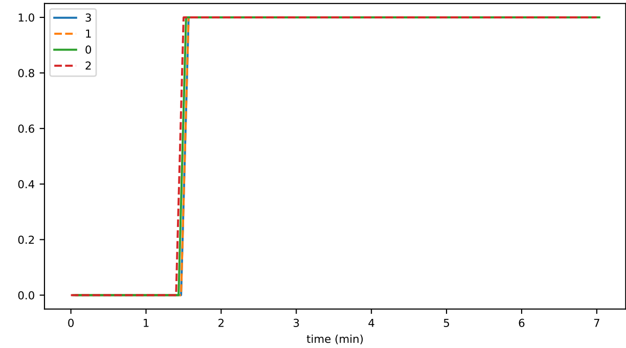
conn_activeConnIp
