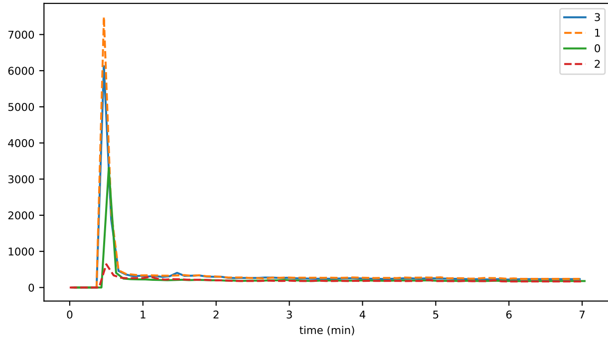
eventDelay_6_pces_runtime
