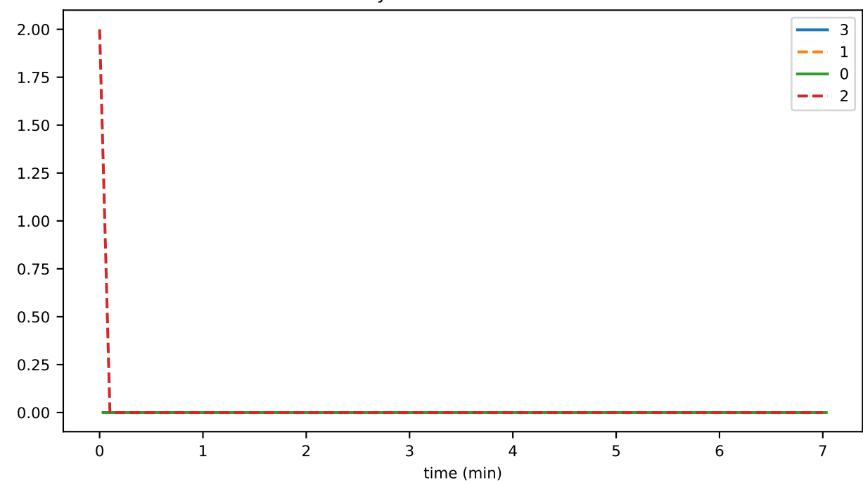
syncPermitsAvailable
