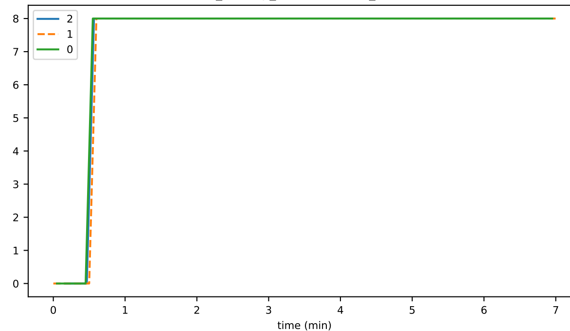
ds_reads_hashes_state
