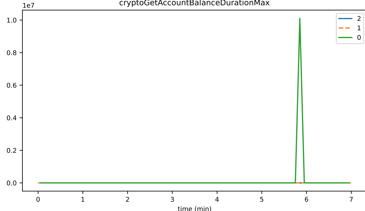
cryptoGetAccountBalanceDurationMax
