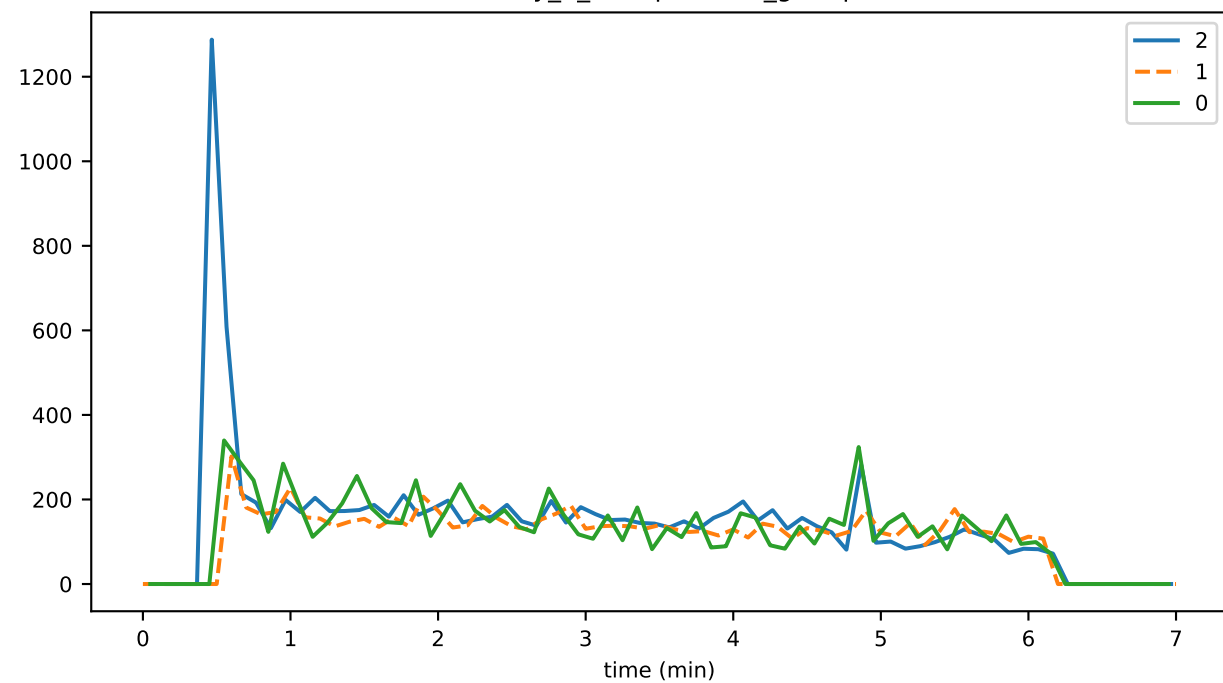
eventDelay_3_deduplication_gossipMAX
