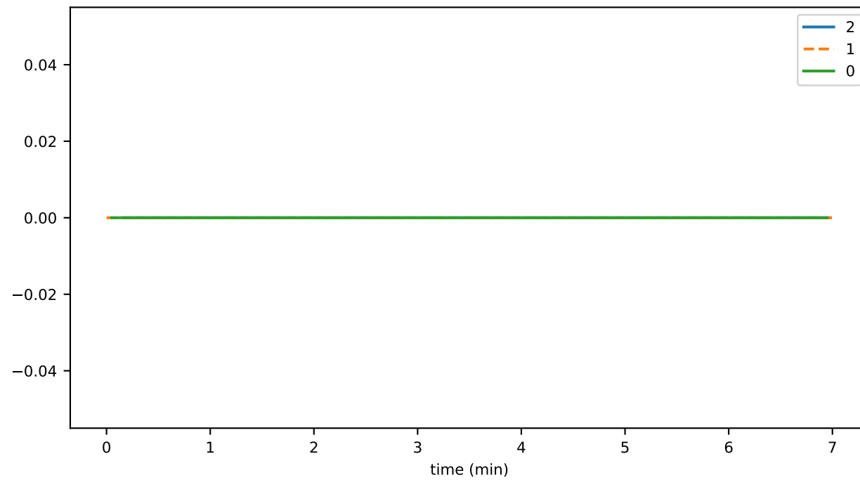
registeredNodeDeleteDurationAvg
