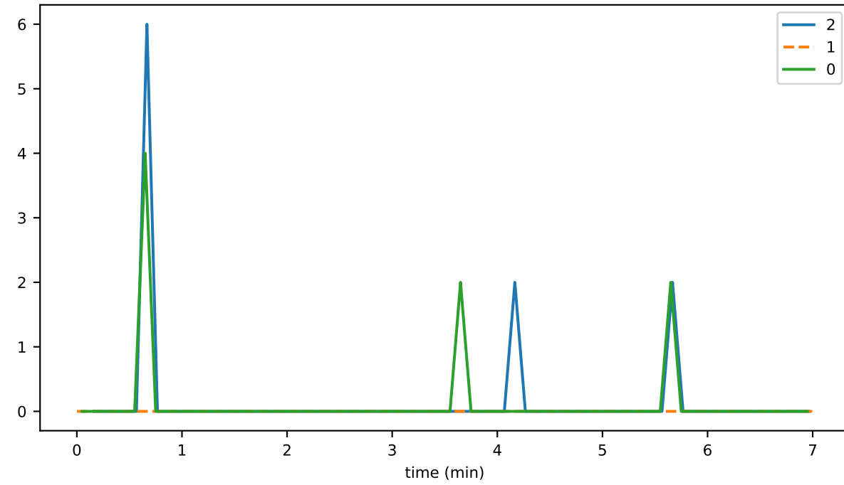
ds_compactions_level_3_hashesTimeMs_state
