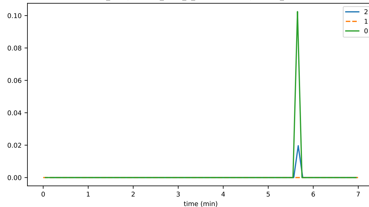
ds_compactions_level_4_hashesSavedSpaceMb_state
