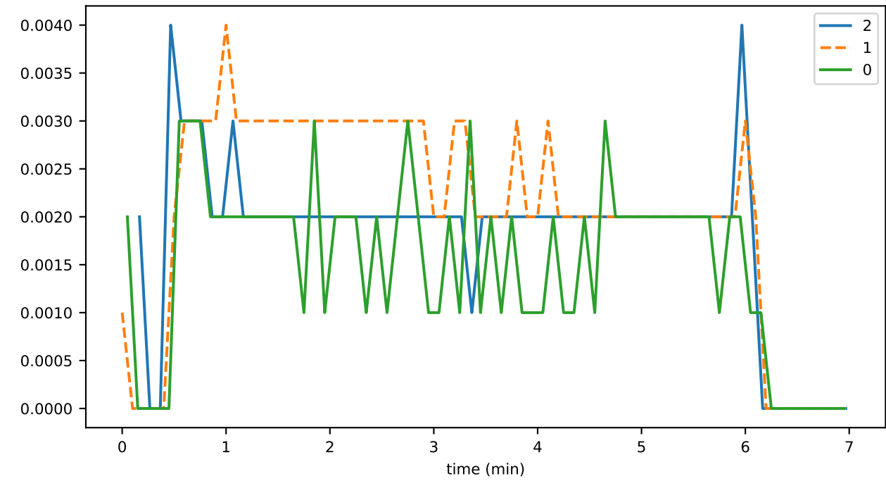
InlinePcesWriter_busy_fraction
