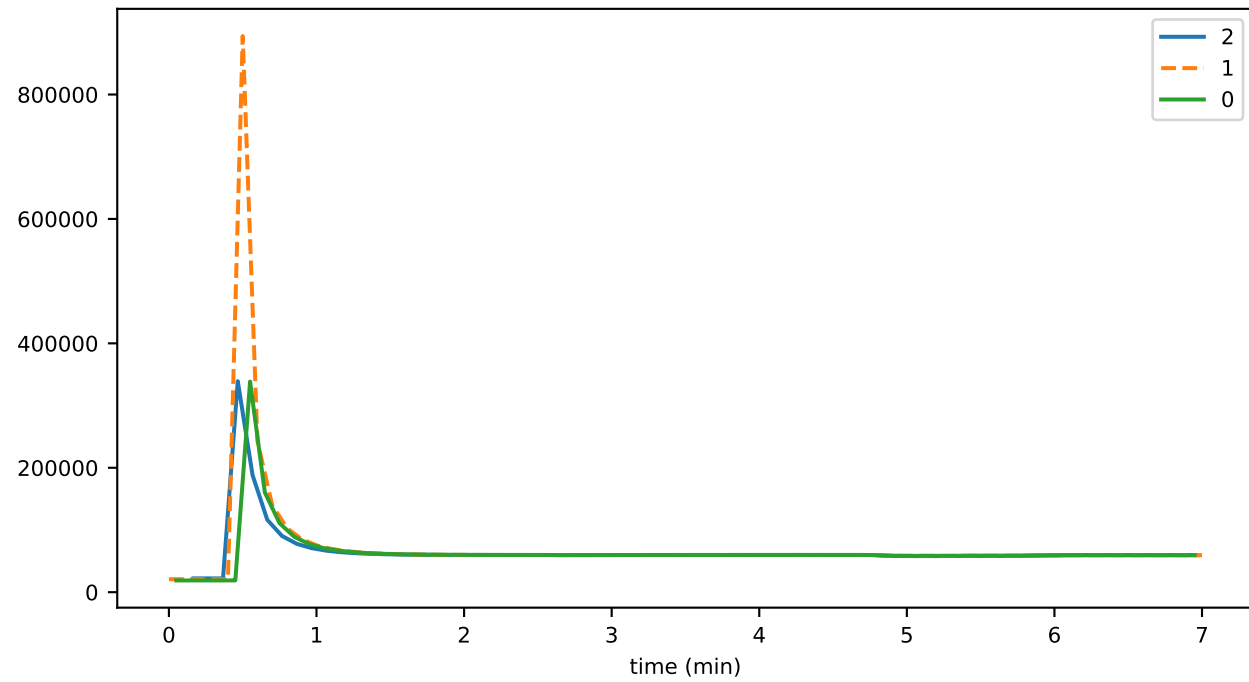
consensus_time_UPDATING_PLATFORM_STATE
