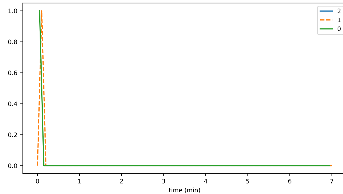
syncPermitsUtilized
