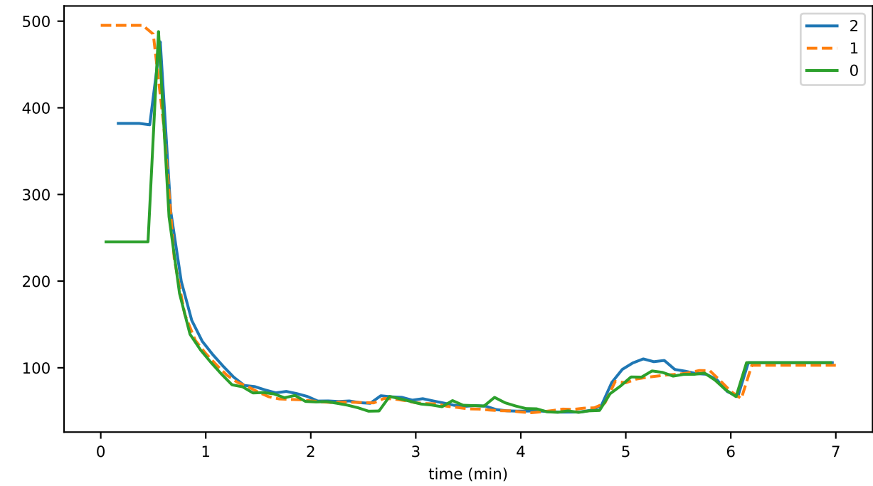
consensus_time_UPDATING_PLATFORM_STATE_RUNNING_HASH
