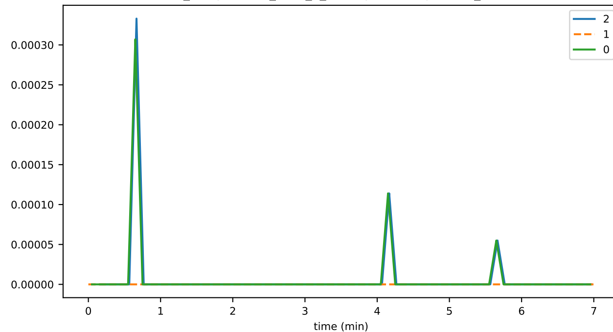
ds_compactions_level_2_leavesSavedSpaceMb_state
