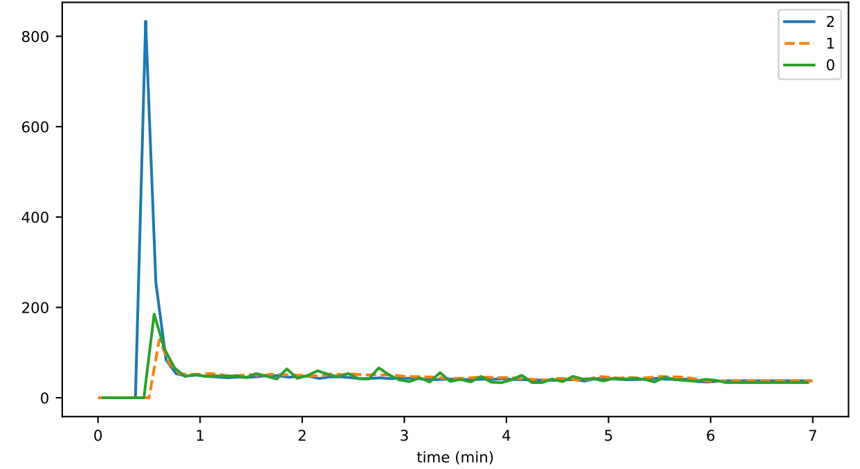
eventDelay_1_hashing_gossip
