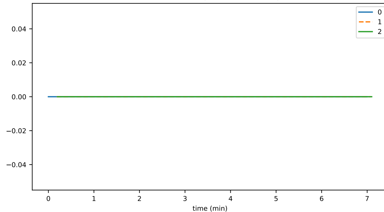
consensusGetTopicInfoThrottledTxns
