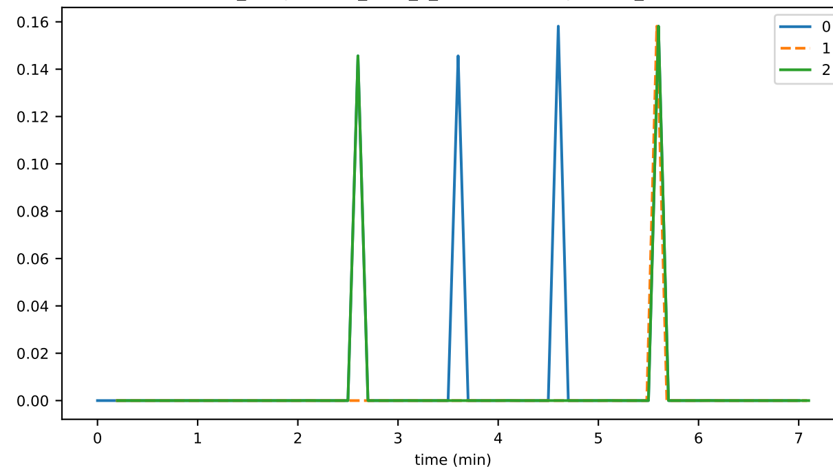
ds_compactions_level_1_leafKeysSavedSpaceMb_state
