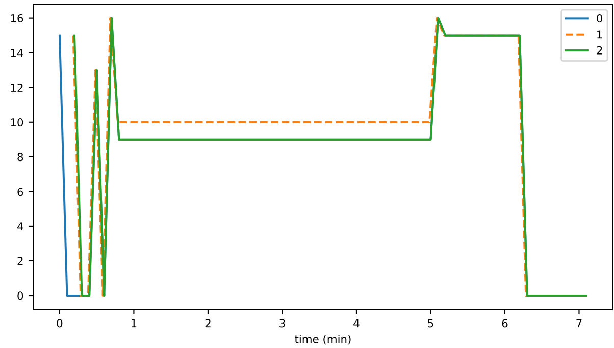
numEventsAddedUntilConsensusMAX
