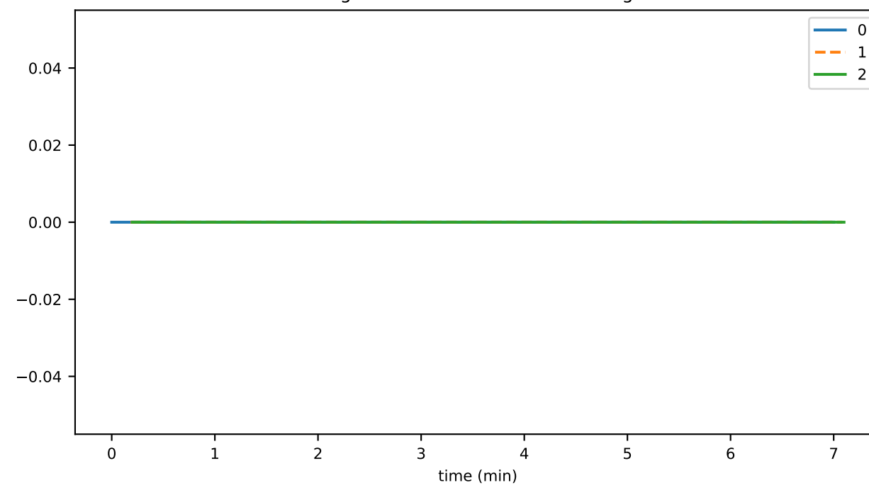
registeredNodeDeleteDurationAvg
