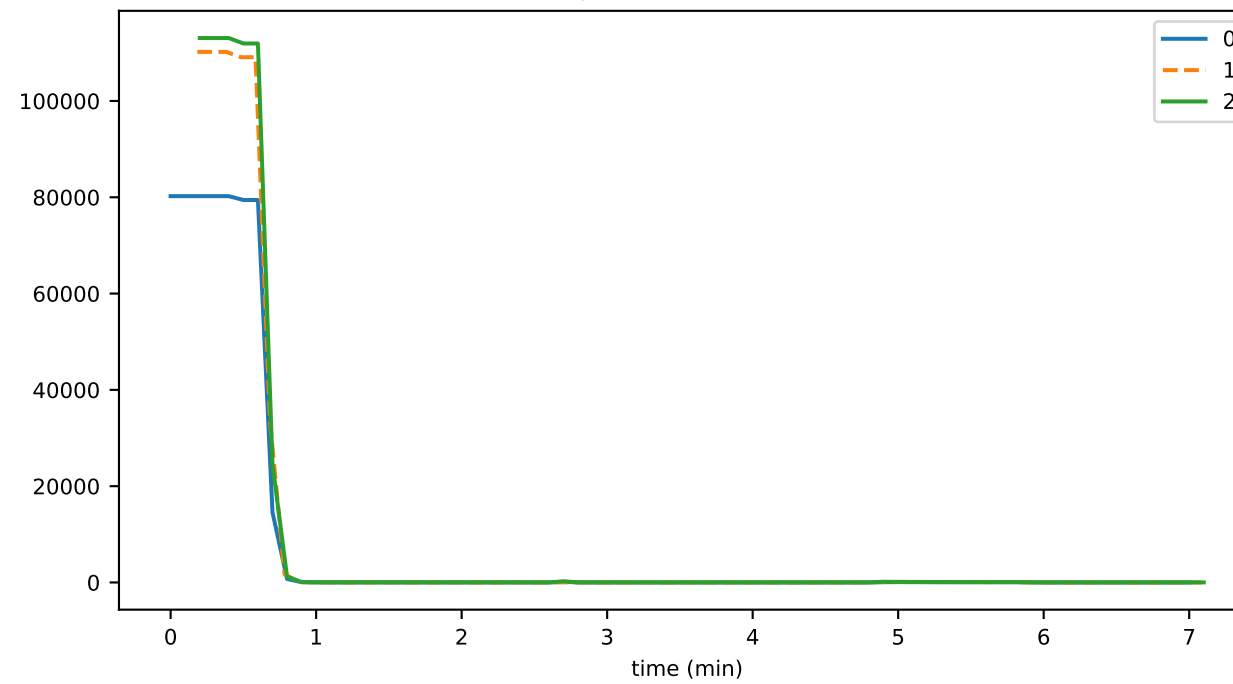
queriedAccountBalances
