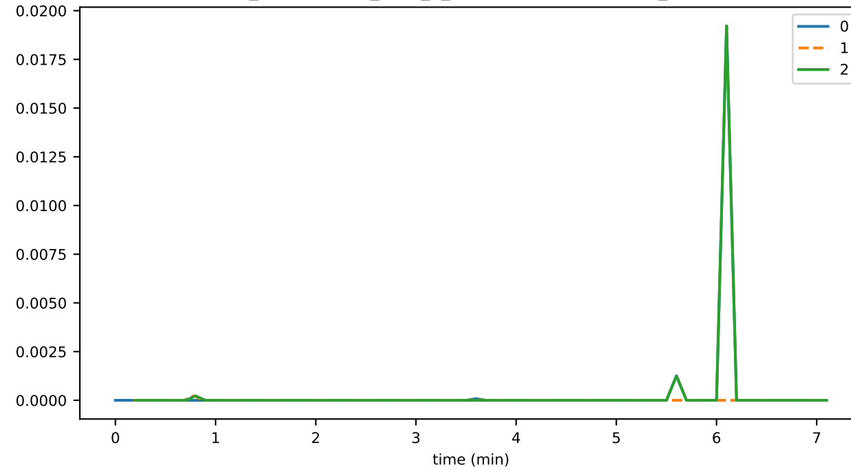
ds_compactions_level_1_leafKeysSavedSpaceMb_state
