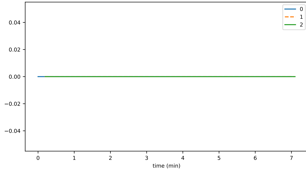
SmartContractService:Rejected_ethereumTxDueToIntrinsicGas_total
