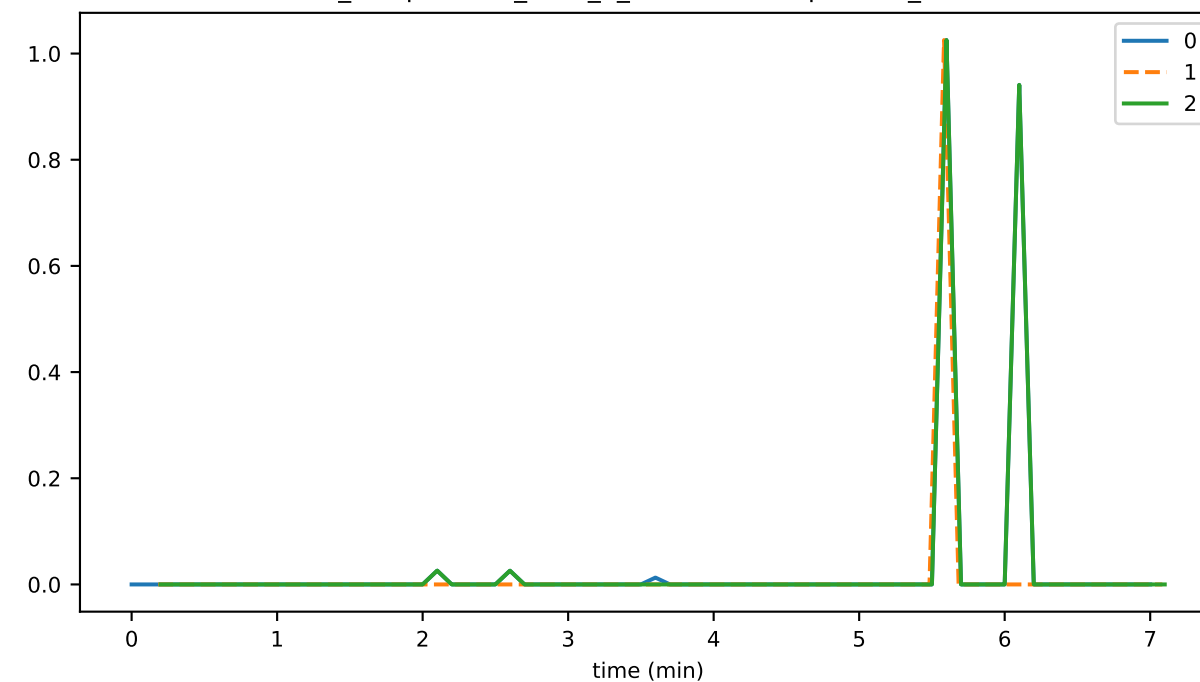
ds_compactions_level_2_hashesSavedSpaceMb_state
