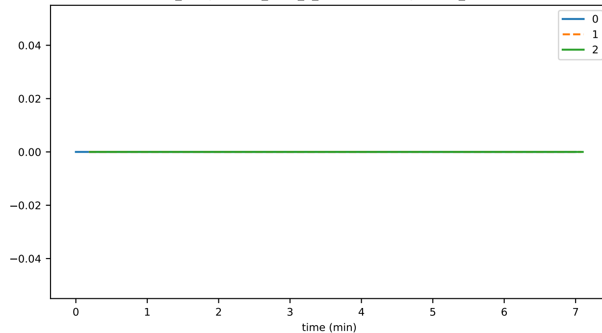
ds_compactions_level_7_leafKeysSavedSpaceMb_state
