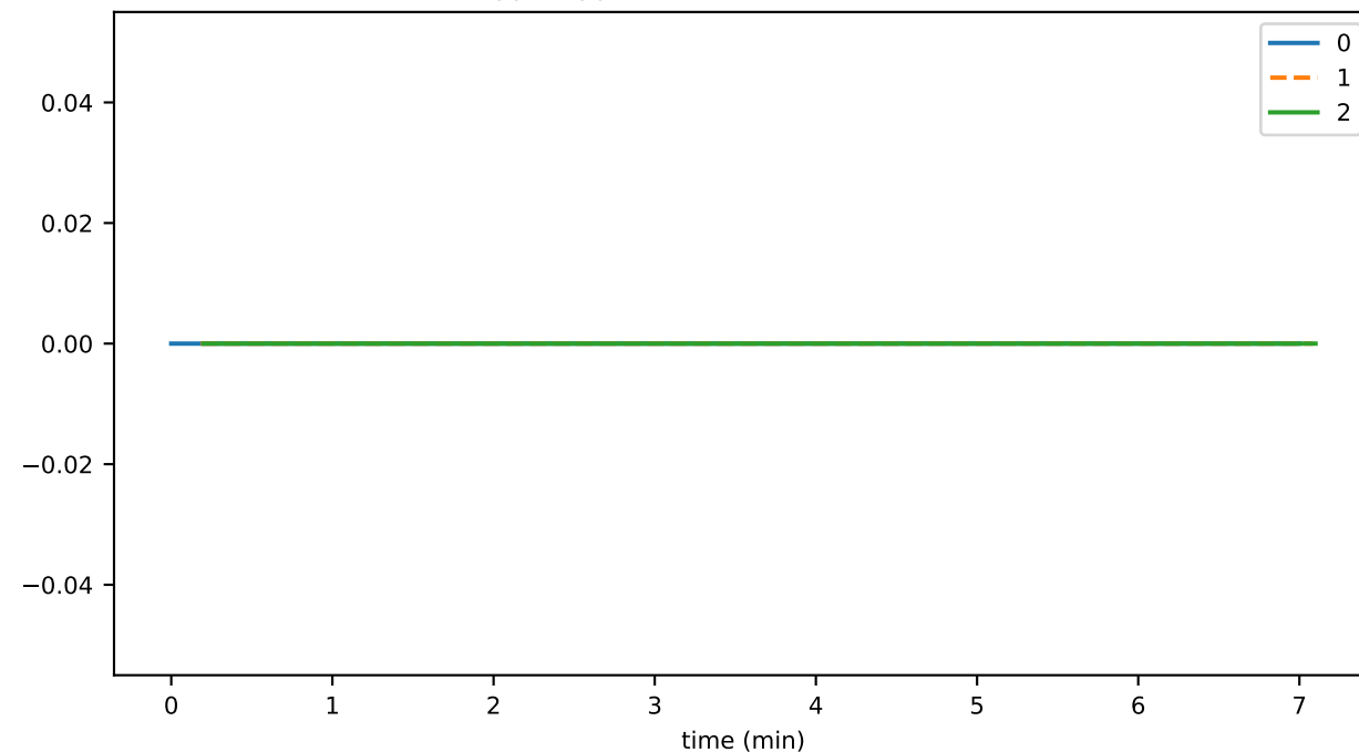
cryptoCreateDurationMax
