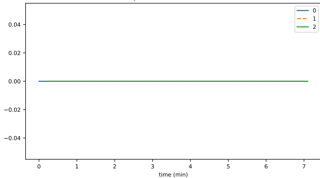
historyProofTransWMetaToWasmMs
