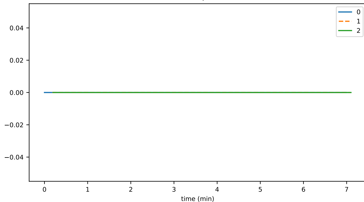
consensusDeleteTopicThrottledTxns
