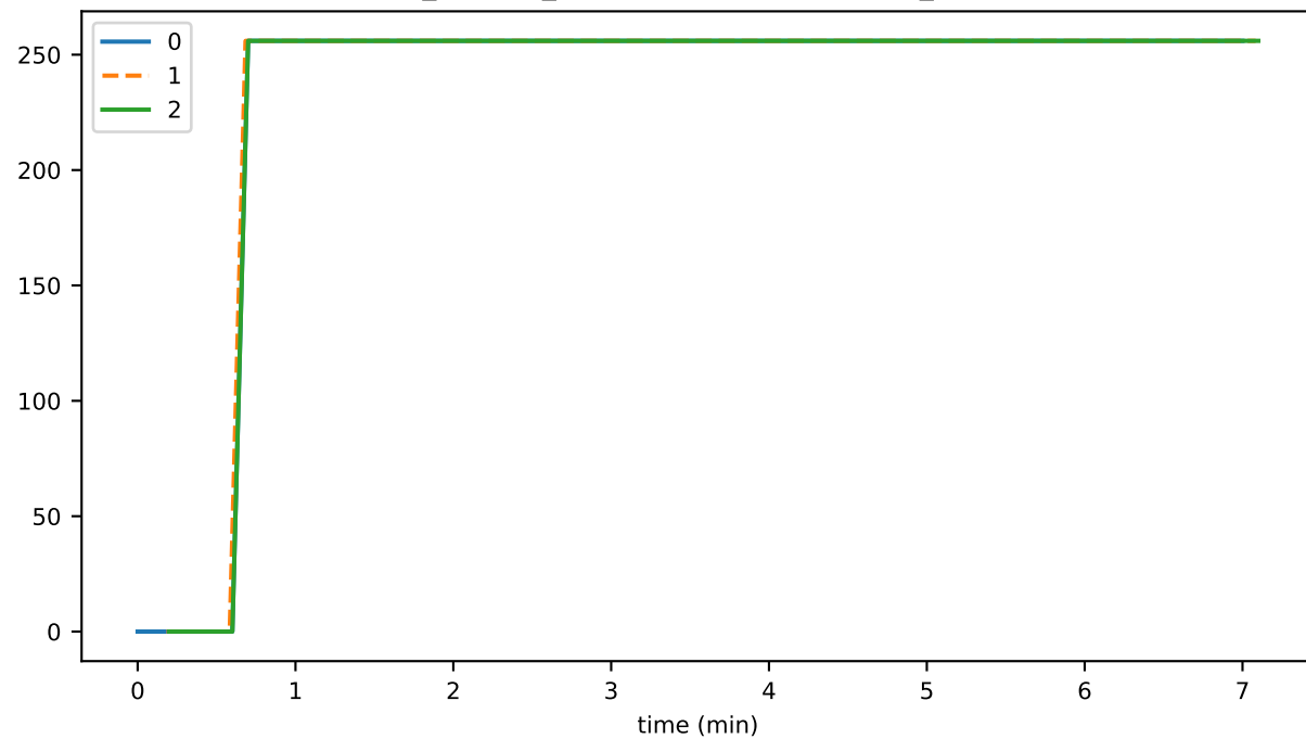
ds_offheap_objectKeyBucketsIndexMb_state
