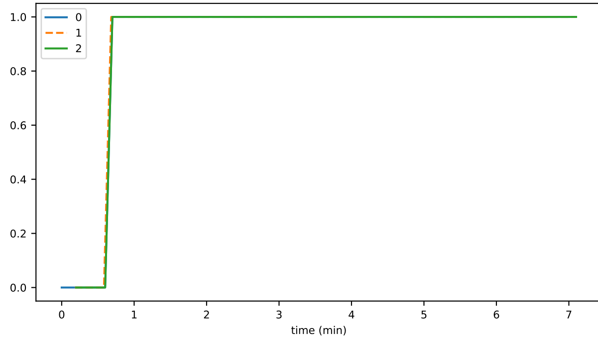
conn_activeConnIp
