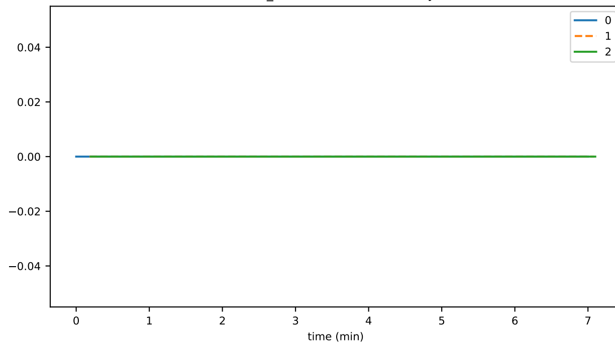
conn_headerSentToAckLatency
