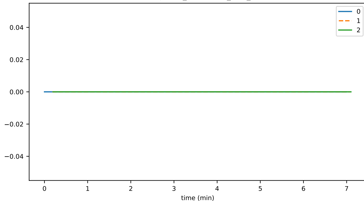
broadcastDisabledDueToOverload
