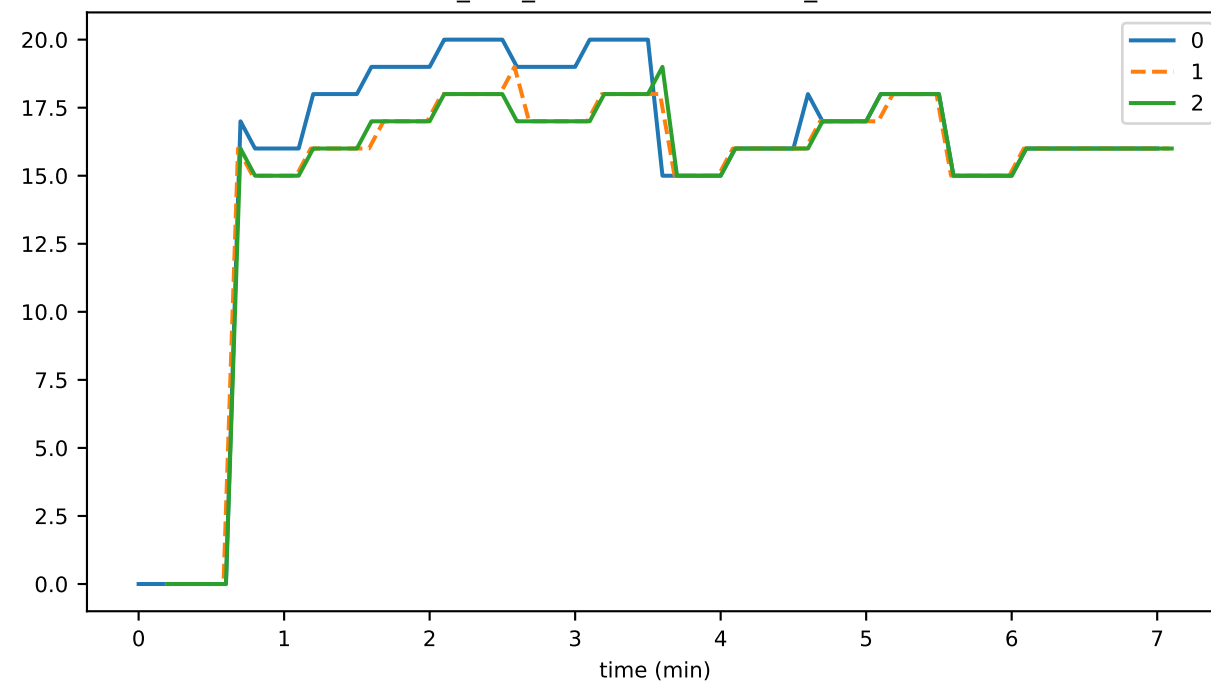
ds_files_leavesStoreFileCount_state
