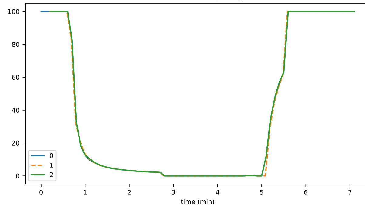
nodeCreateDurationMax
