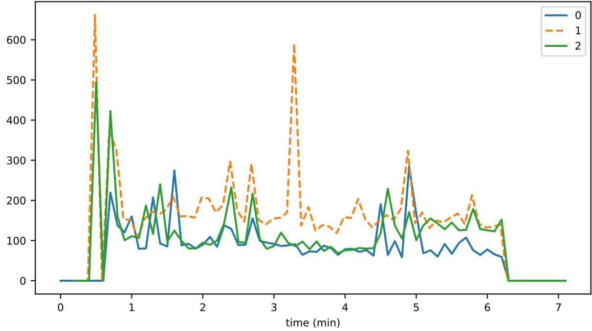
eventDelay_3_deduplication_gossipMAX
