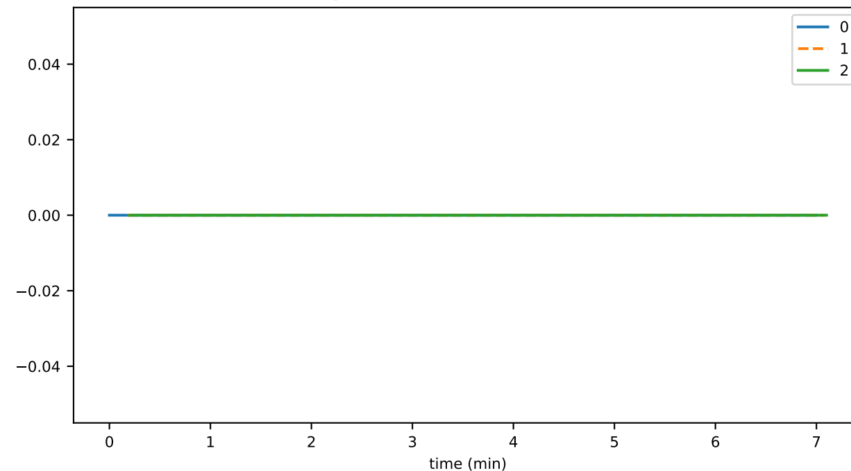
registeredNodeDeleteDurationAvg
