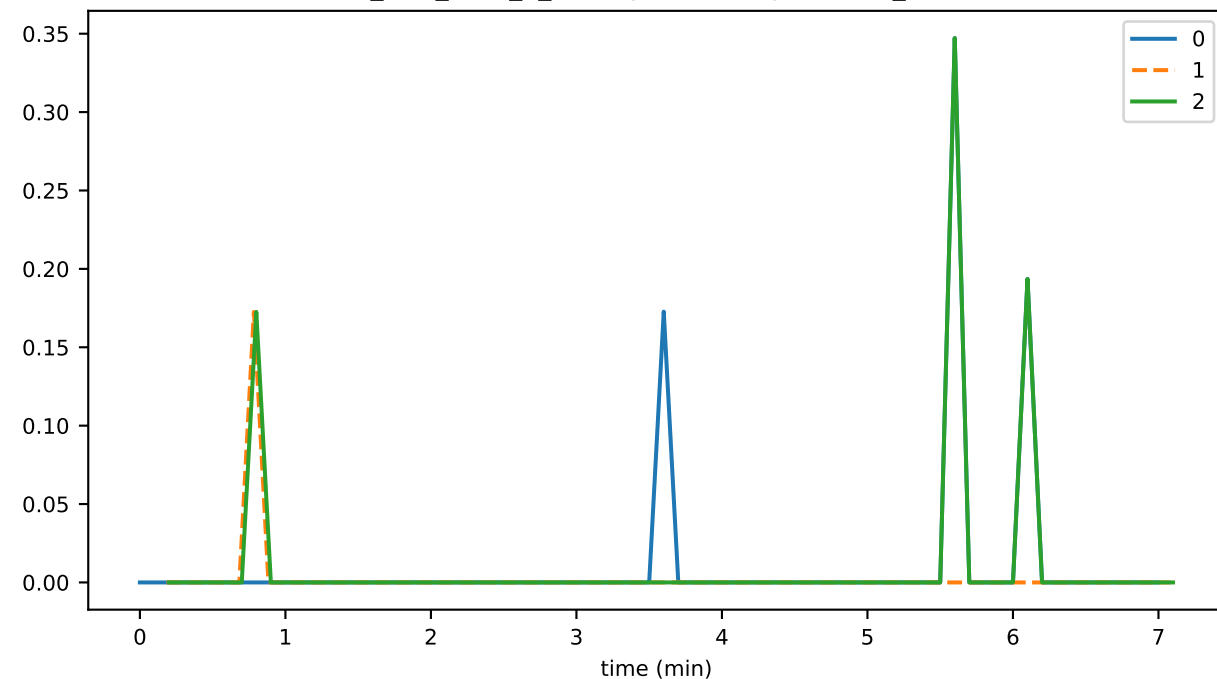
ds_files_level_2_hashesFileSizeByLevelMb_state
