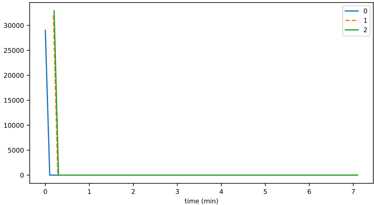
eventDelay_5_orphanBuffer_storageMAX
