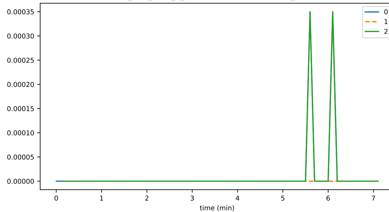
ds_files_level_2_leafKeysFileSizeByLevelMb_state
