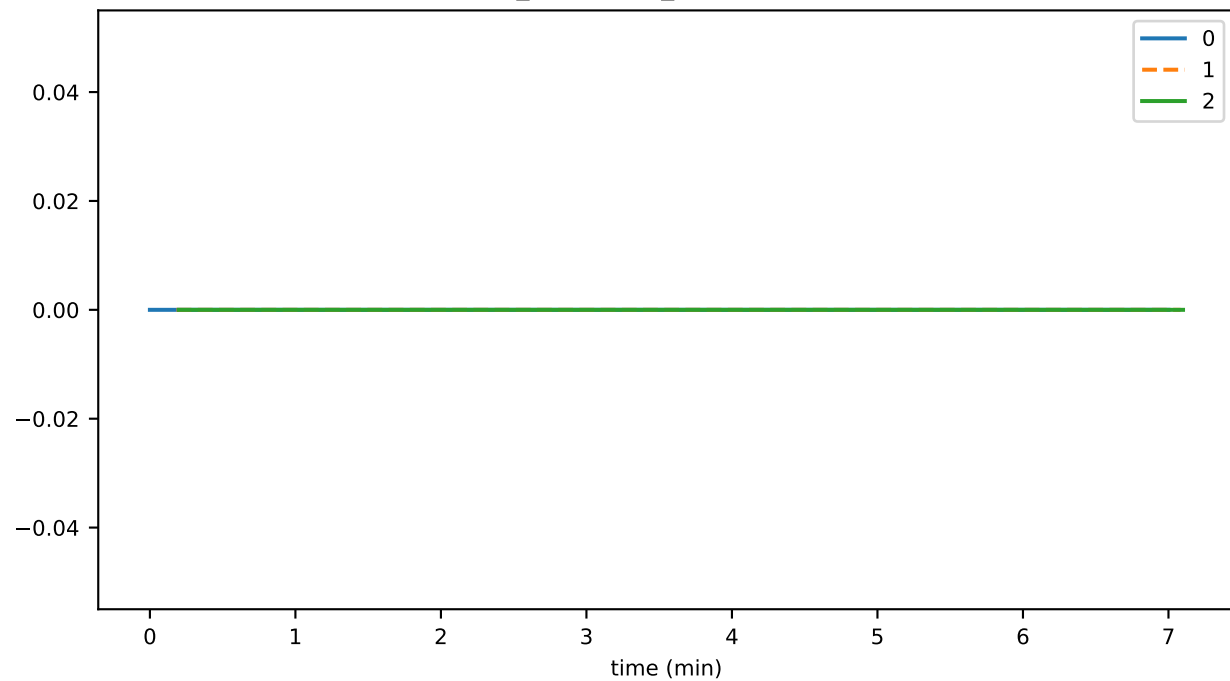
conn_connClose_connectionError
