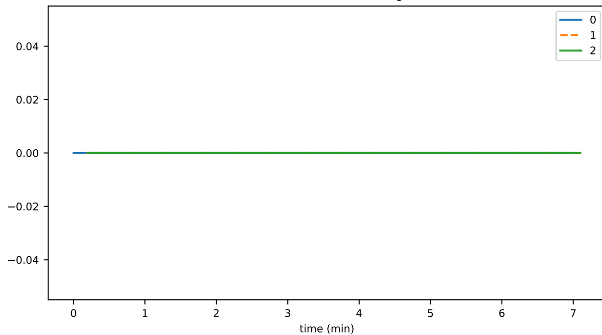
contractCallDurationAvg
