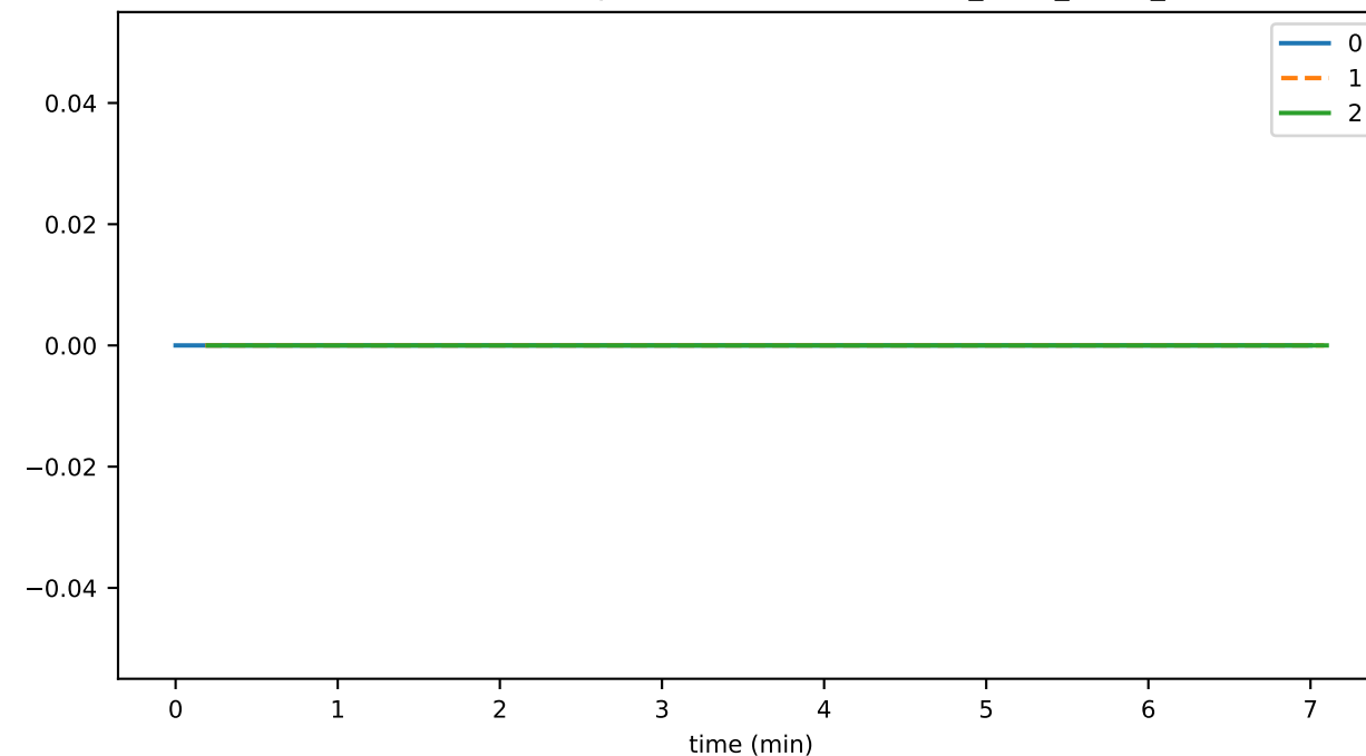
SmartContractService:SystemContractMethodCall_PAUSE_UNPAUSE_failed
