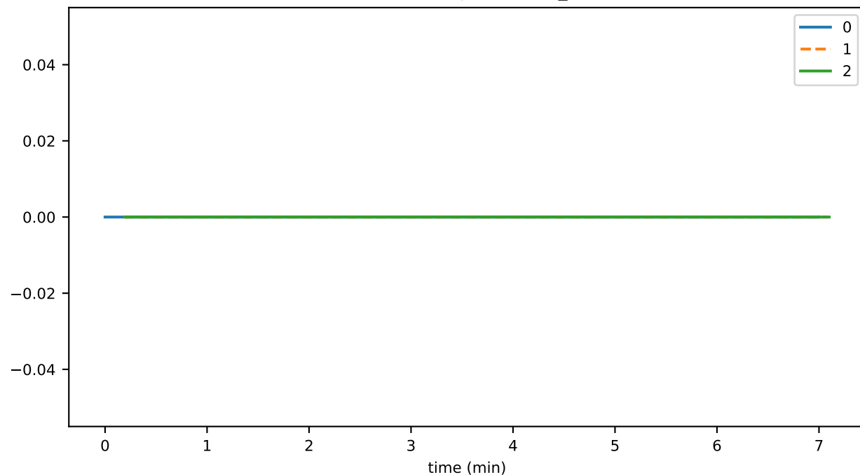
SmartContractService:Rejected_contractCallTxDueToIntrinsicGas_total
