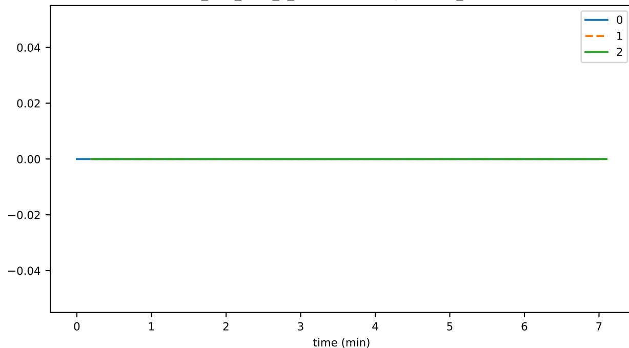
ds_files_level_7_leafKeysFileSizeByLevelMb_state
