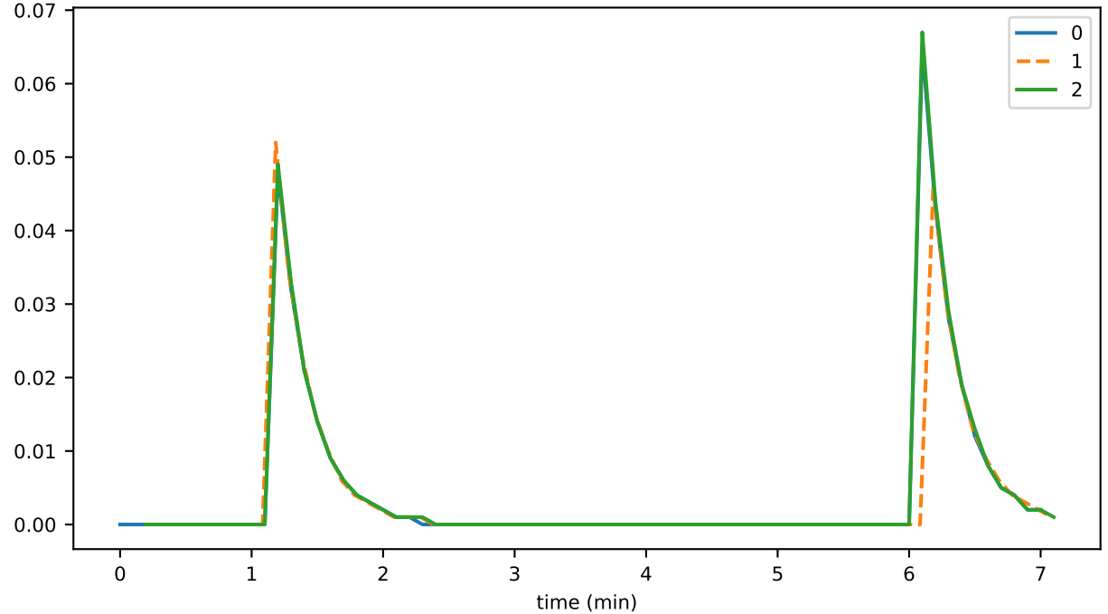
preconsensusEventFileRate
