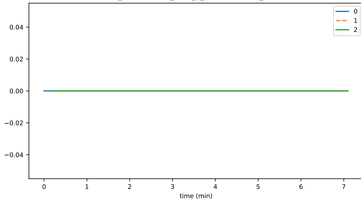
ds_compactions_level_4_leafKeysTimeMs_state
