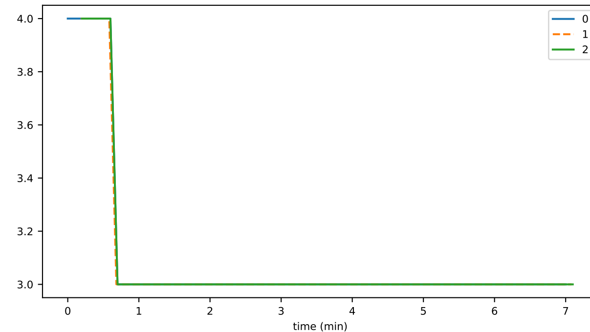
eventsWithDisparateSignature
