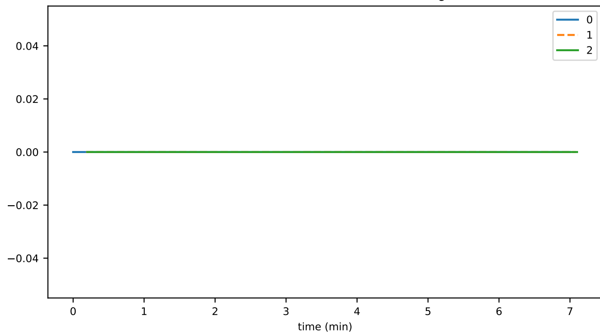
networkGetExecutionTimeDurationAvg
