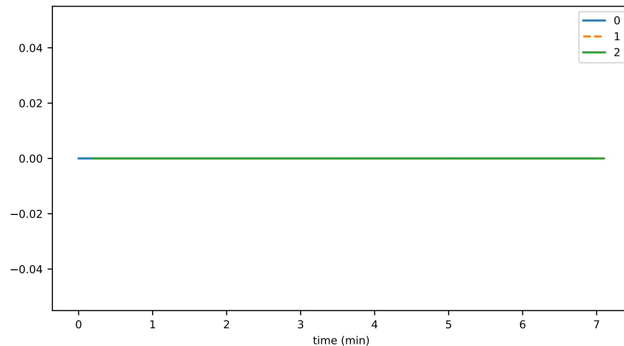
networkGetExecutionTimeDurationMax
