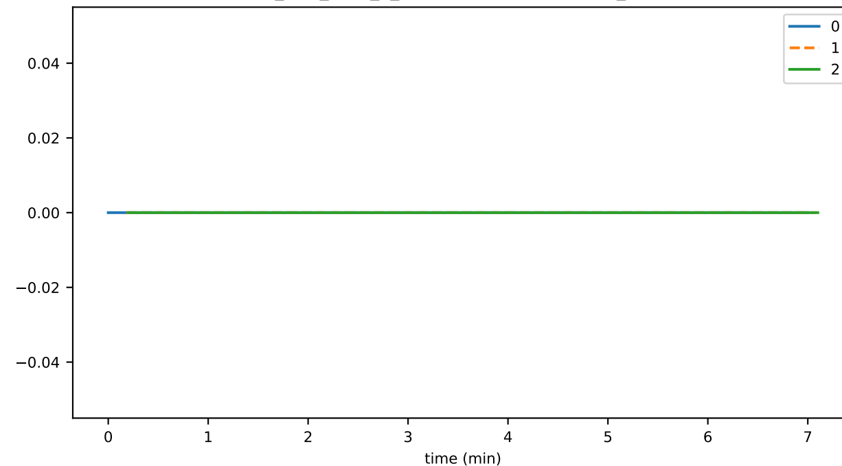
ds_files_level_7_leavesFileSizeByLevelMb_state
