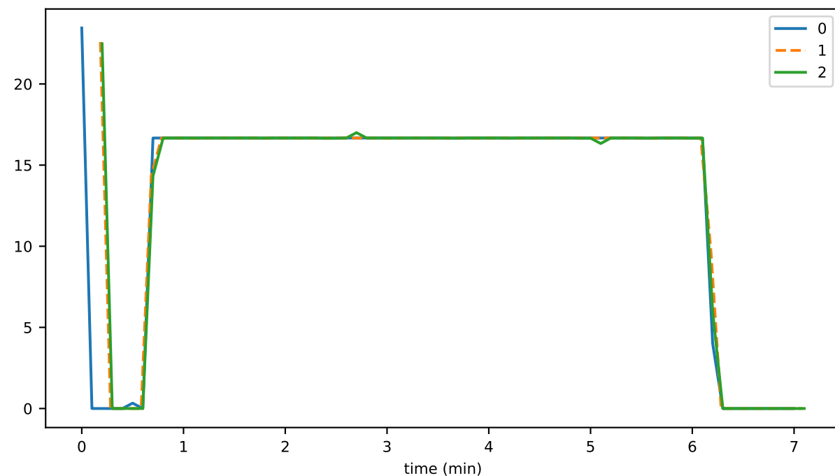
buffer_blockBytes
