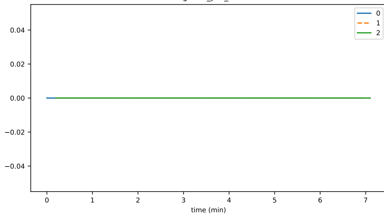
SigInval_per_sec
