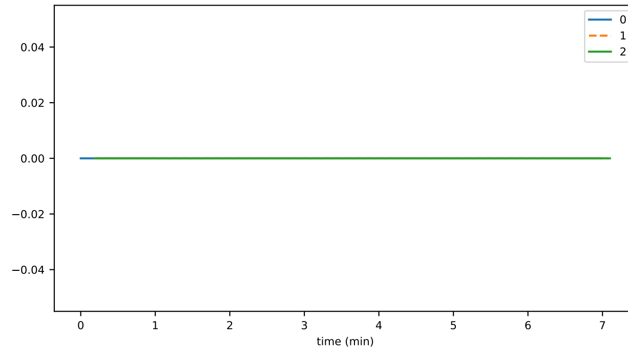
cryptoDeleteAllowanceThrottledTxns
