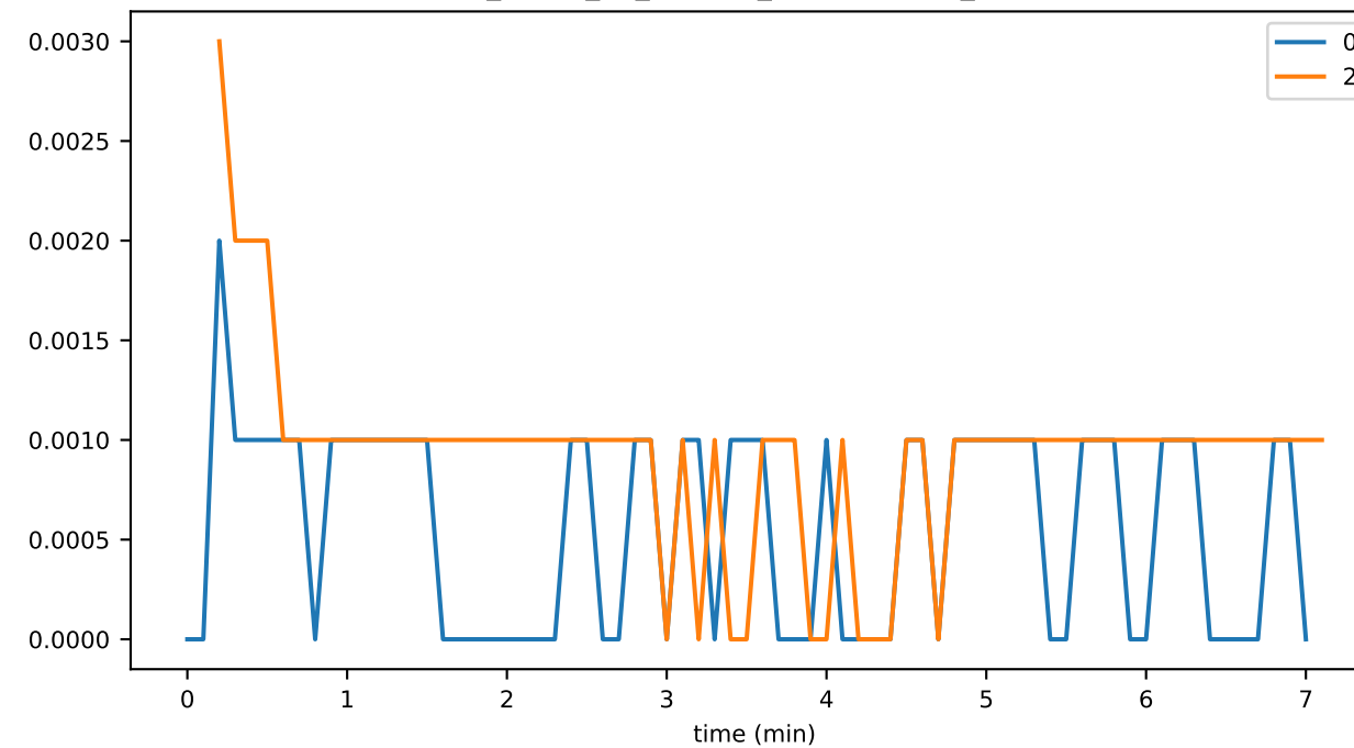
sync_phase_01_fraction_EXCHANGING_EVENTS
