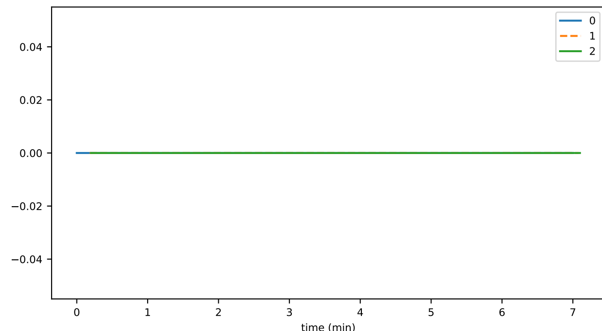
tokenFreezeAccountDurationMax
