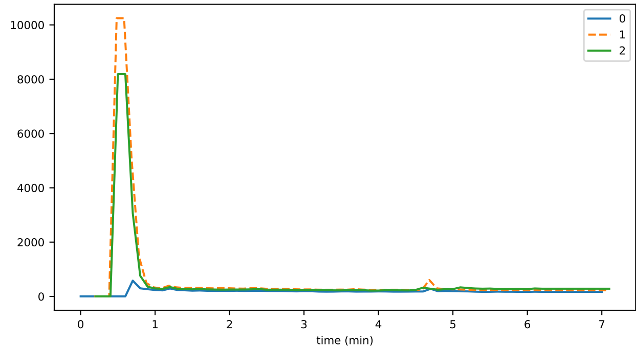
eventDelay_6_pces_gossip
