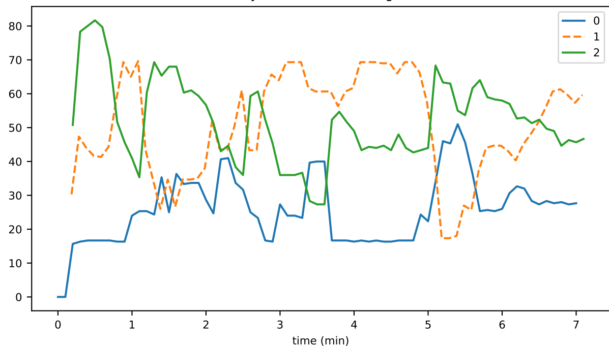
ds_compactions_level_0_hashesTimeMs_state
