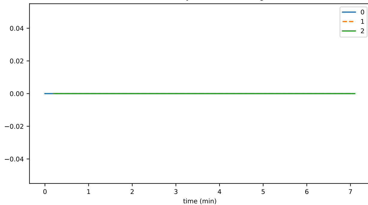
contractGetBytecodeDurationAvg
