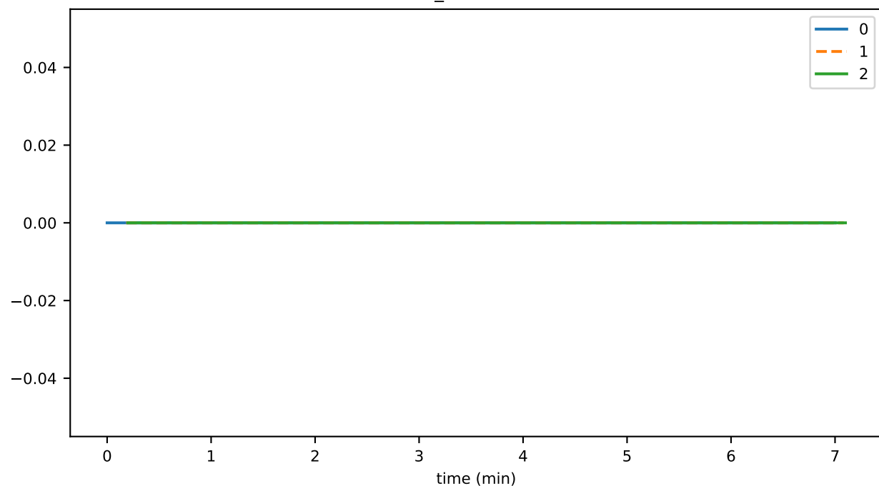
conn_headerProducedToAckLatency
