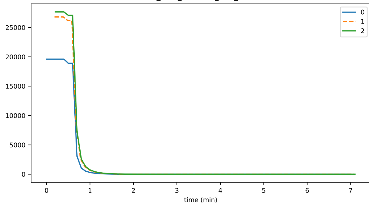
consensusCreateTopicDurationMax
