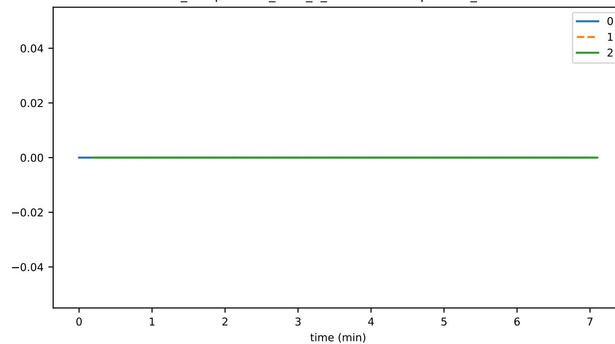
ds_compactions_level_8_hashesSavedSpaceMb_state
