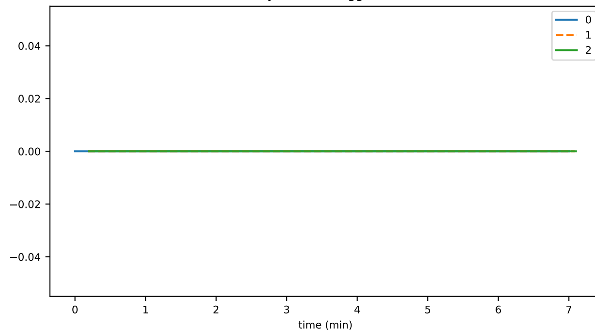
historyProofTransR1ToFailCnt
