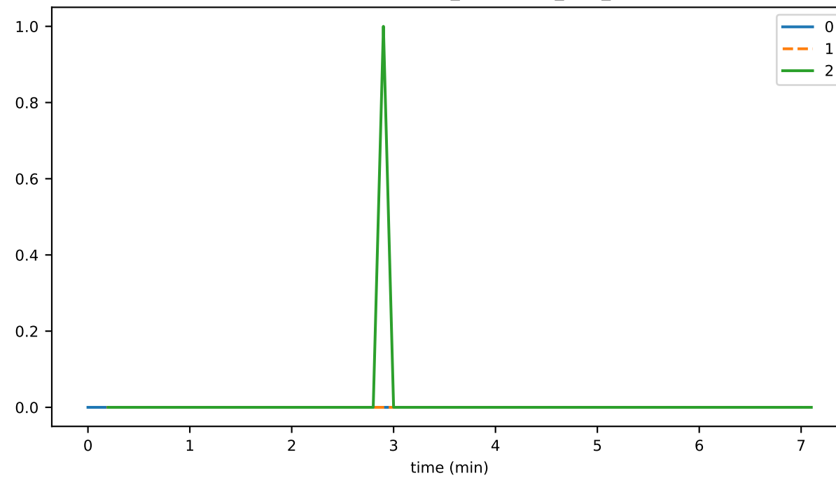
StateSignatureCollector_unhandled_task_count
