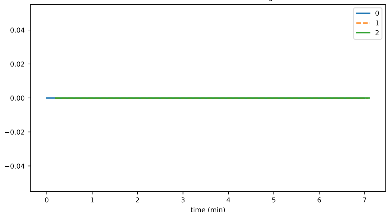
tokenFreezeAccountDurationAvg
