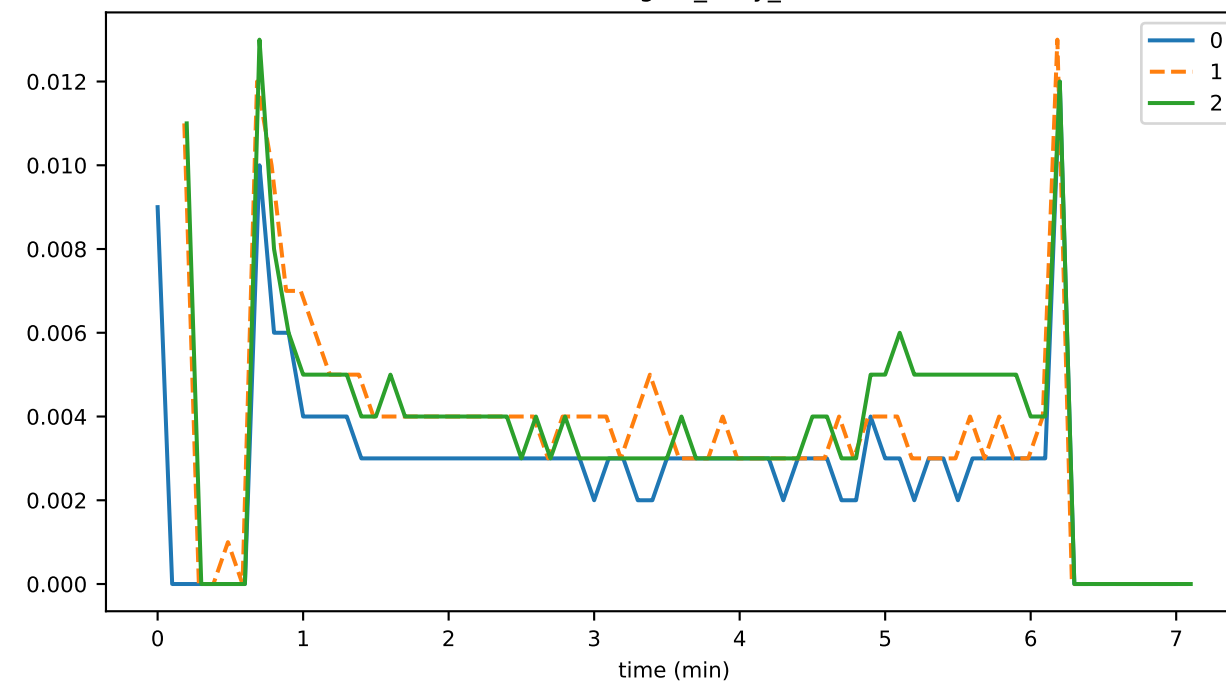
ConsensusEngine_busy_fraction
