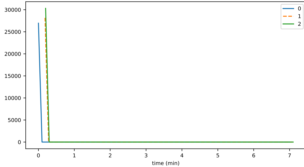
eventDelay_5_orphanBuffer_gossipMAX
