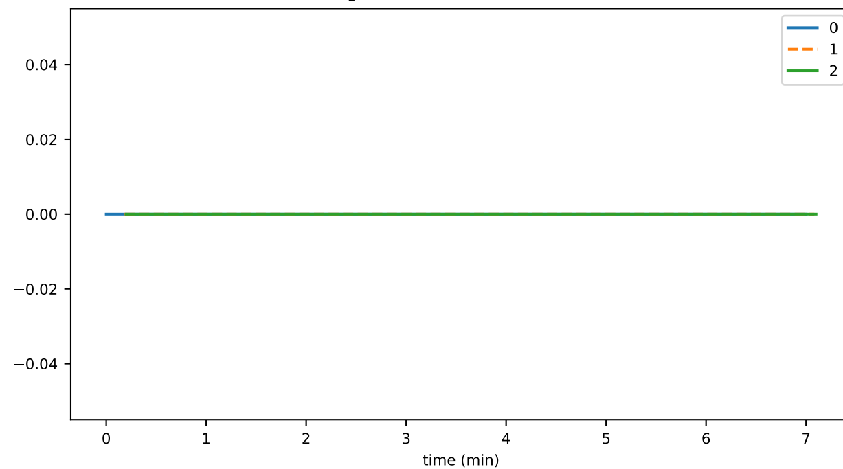
ledgerIdPublicationDurationMax
