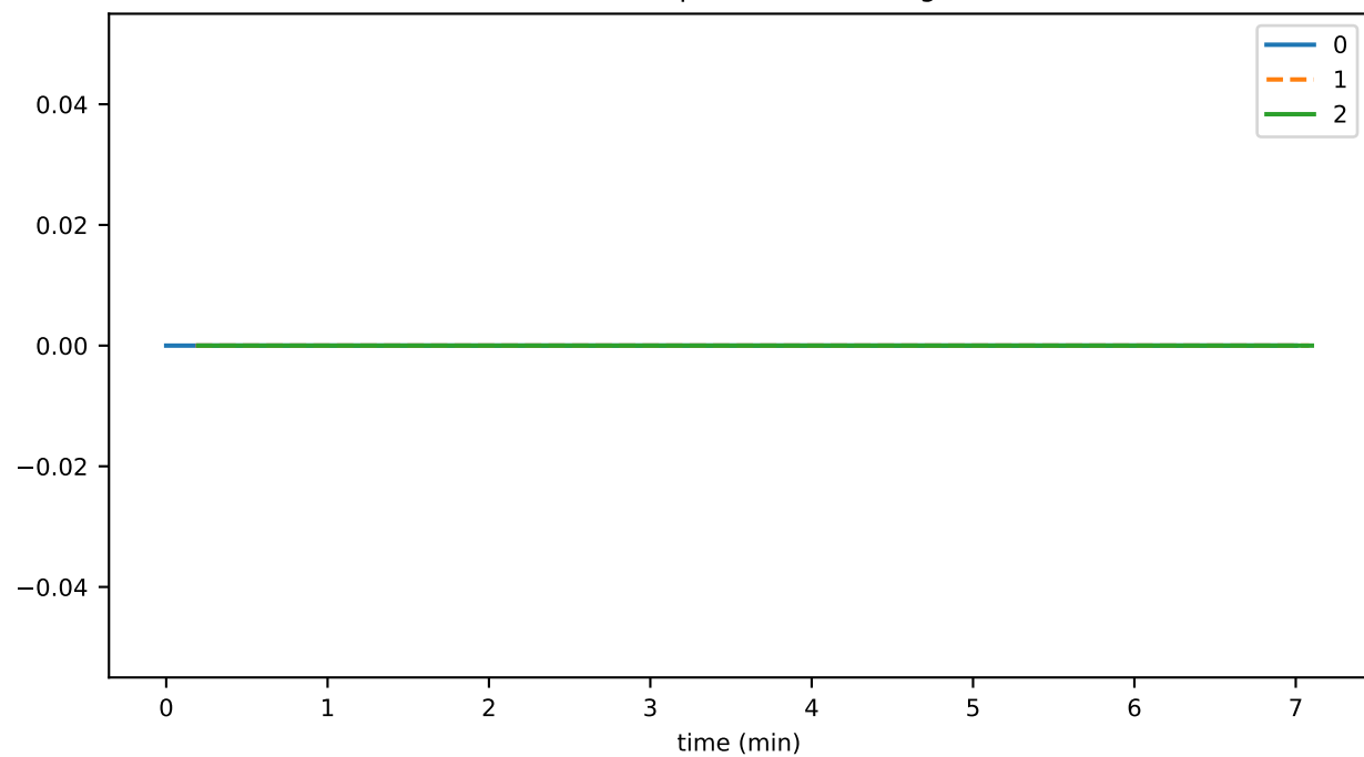
contractUpdateDurationAvg
