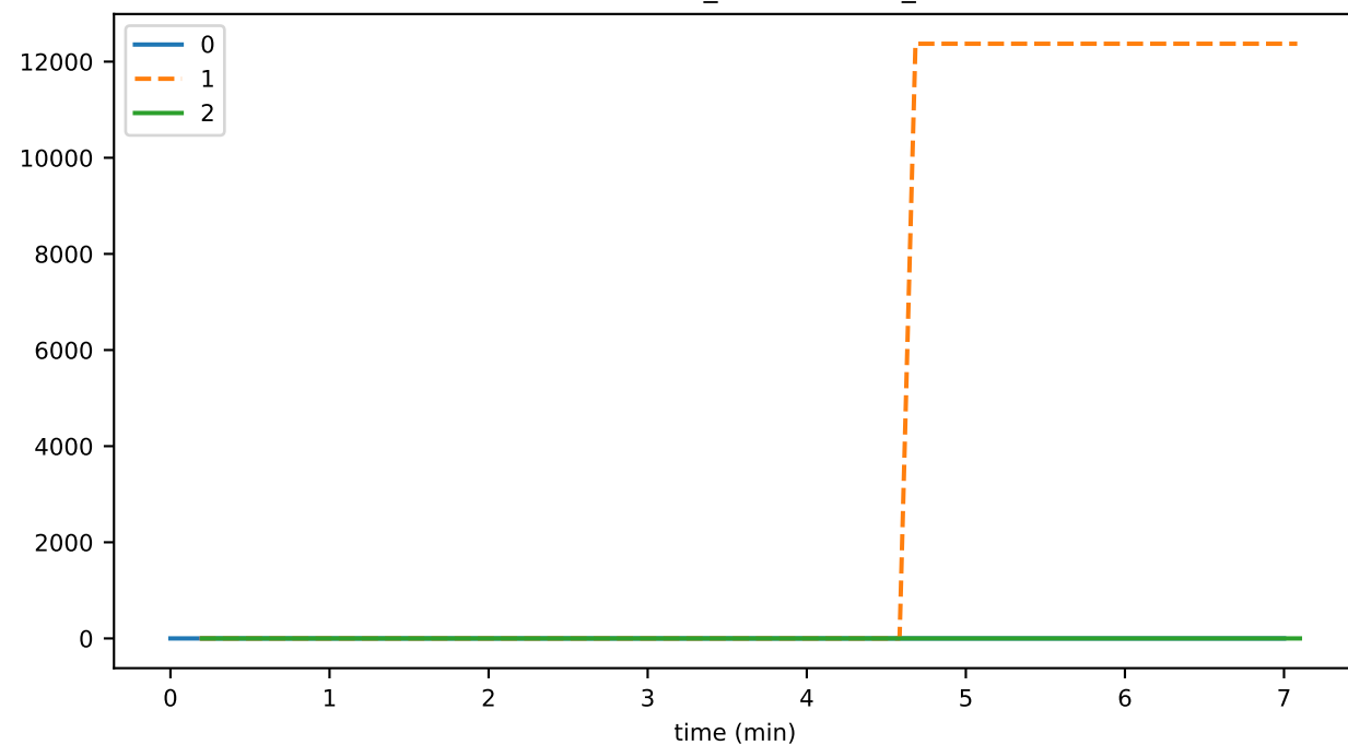
getAccountDetailsDurationAvg
