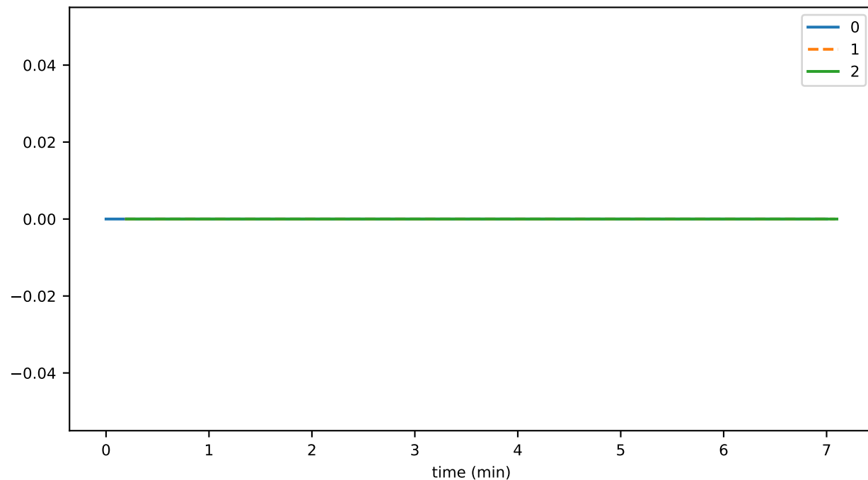
branchingNodeCount
