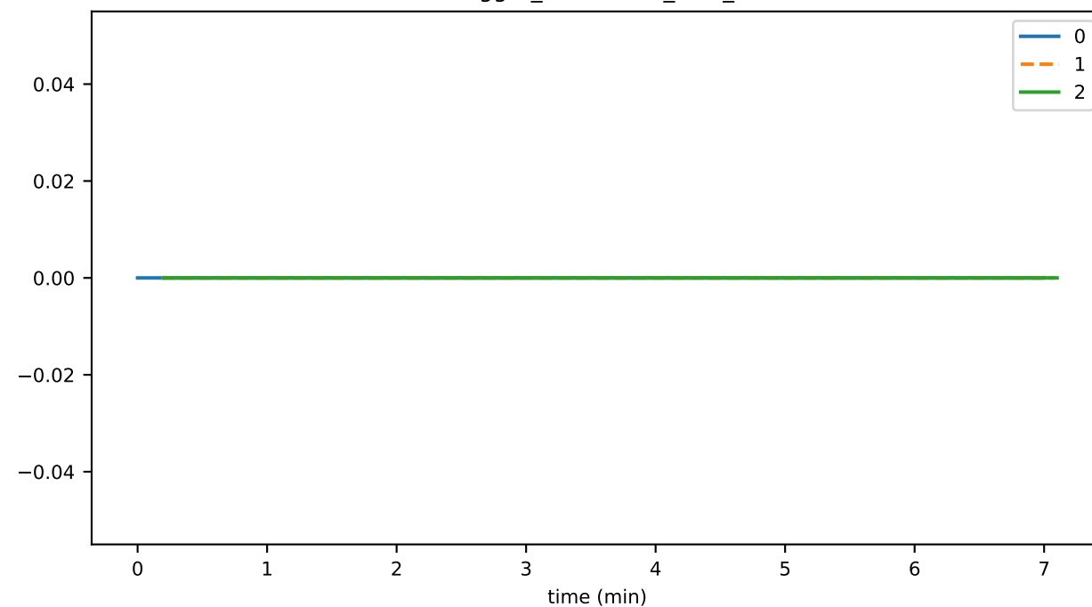
HealthMonitor_unhandled_task_count
