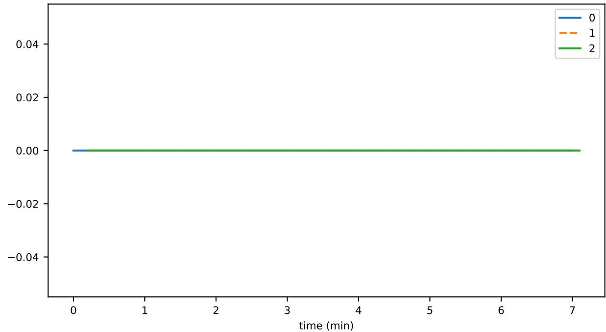
ds_compactions_level_6_leafKeysTimeMs_state
