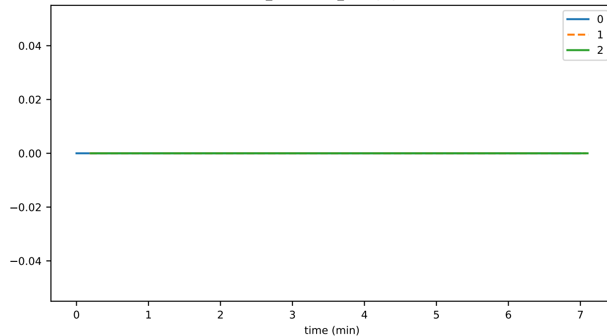
conn_connClose_endStreamReceived
