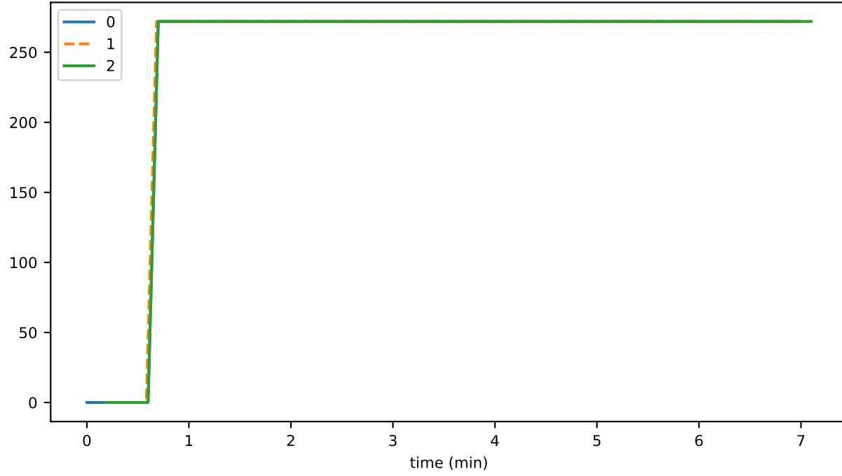
ds_offheap_dataSourceMb_state
