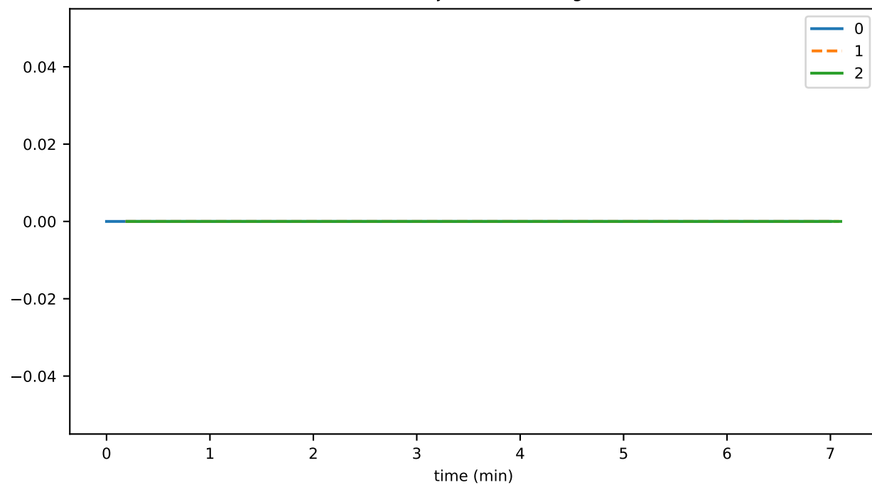
tokenRejectDurationAvg
