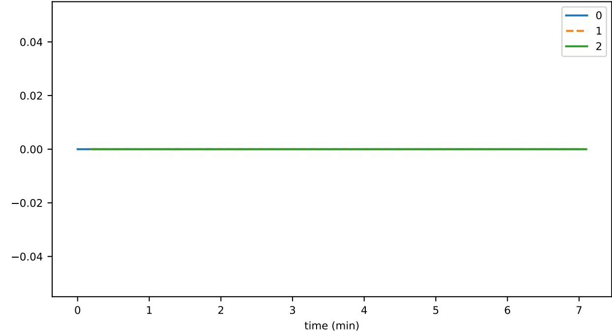
cryptoDeleteLiveHashDurationMax
