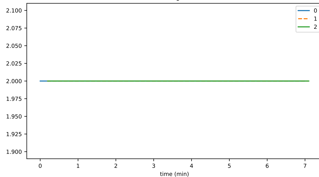
oldestSignedStateSeconds
