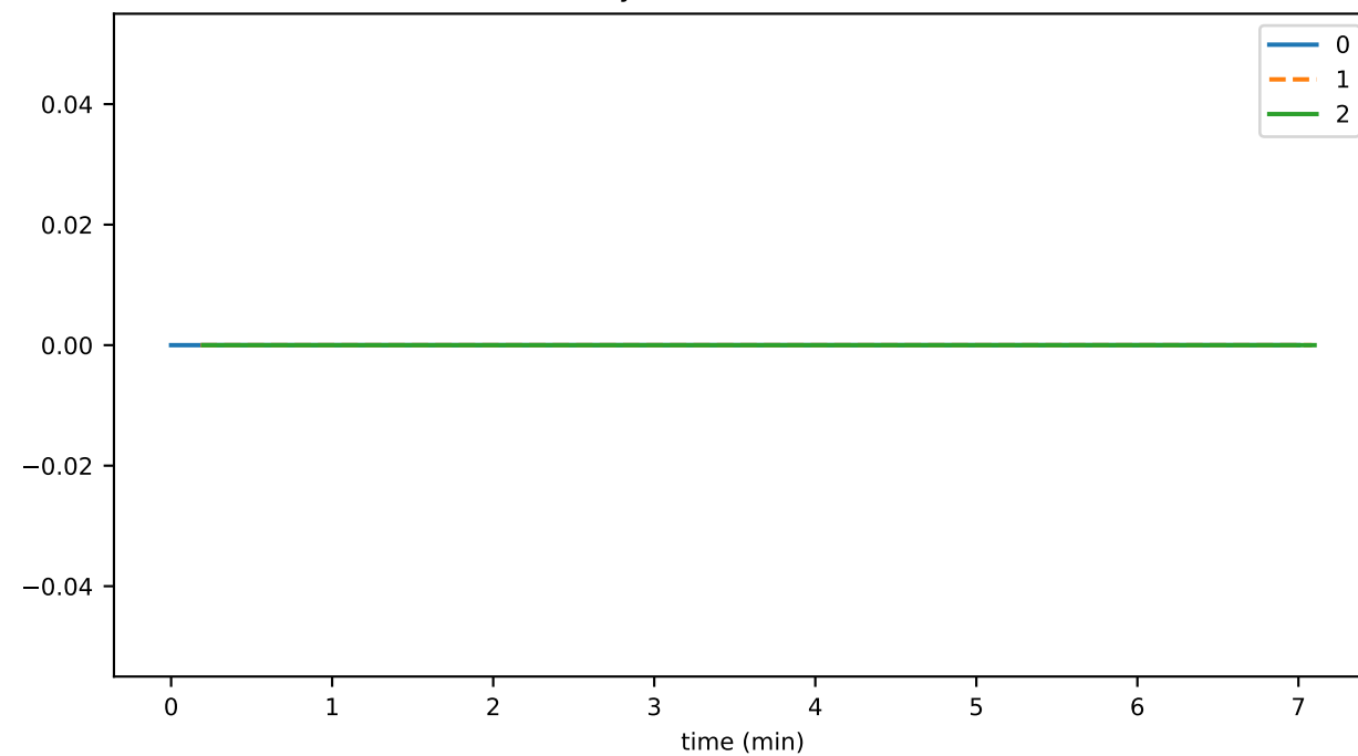
historyProofTransR2ToFailCnt
