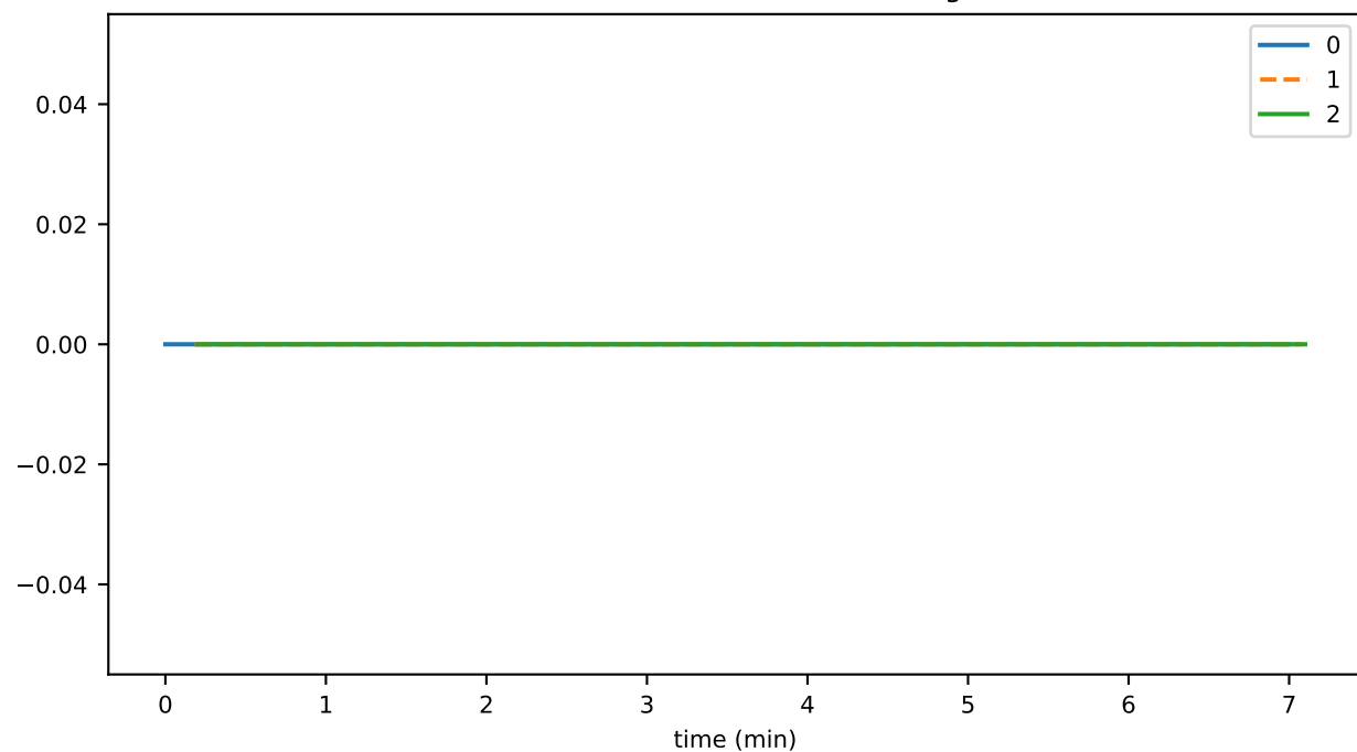
contractGetRecordsThrottledTxns
