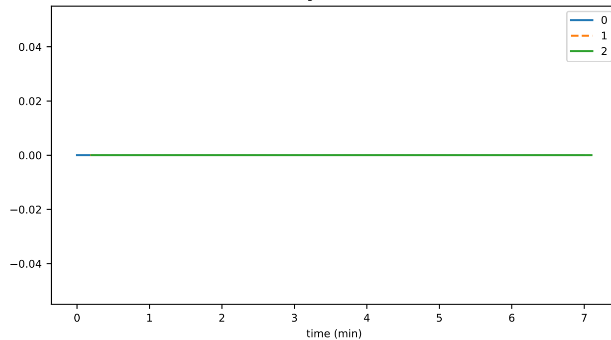
utilPrngThrottledTxns
