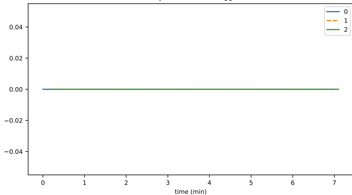
historyProofTransR3ToFailMs
