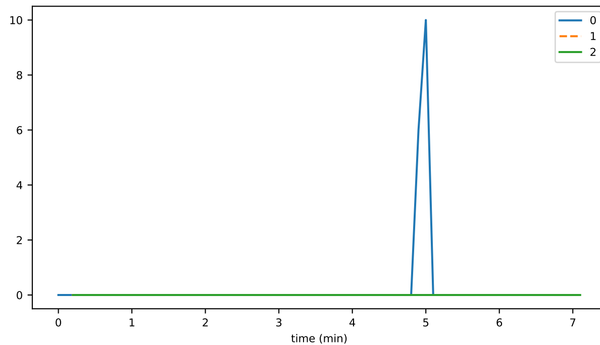
bufferedTransactions
