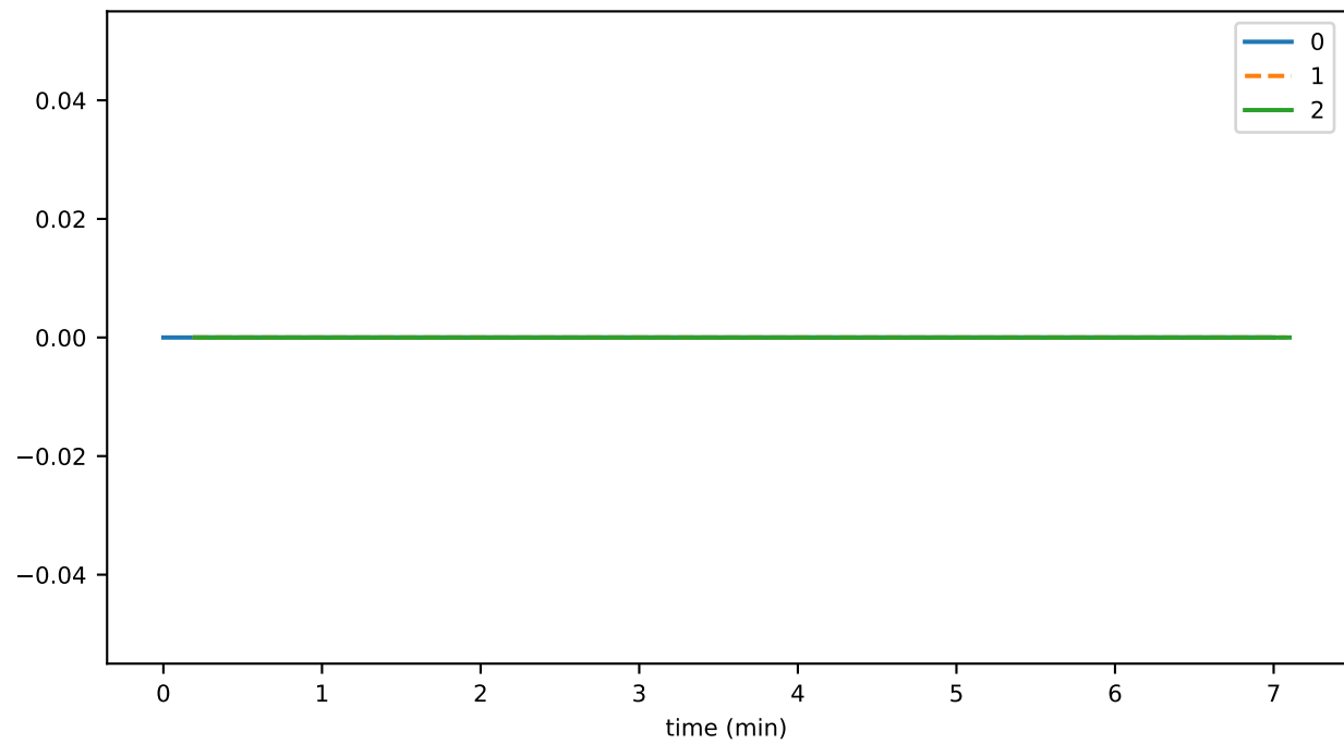
historyProofsProduced
