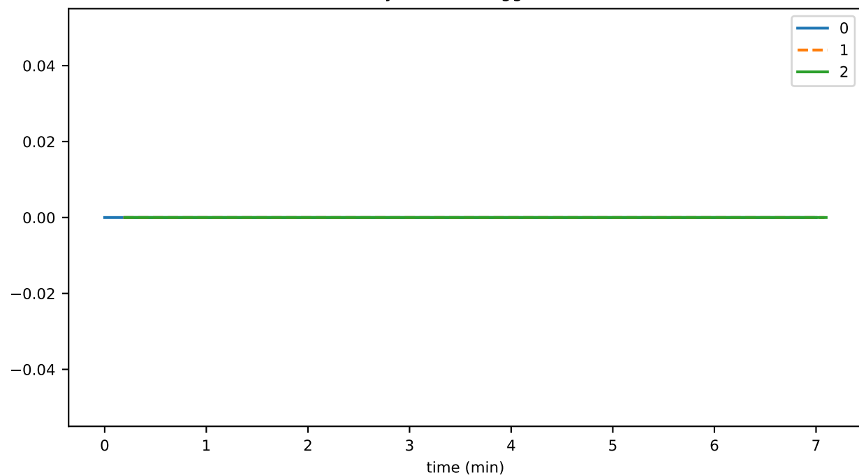
historyProofTransAggToFailMs
