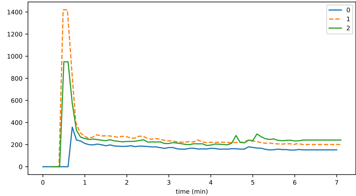
eventDelay_5_orphanBuffer_runtime
