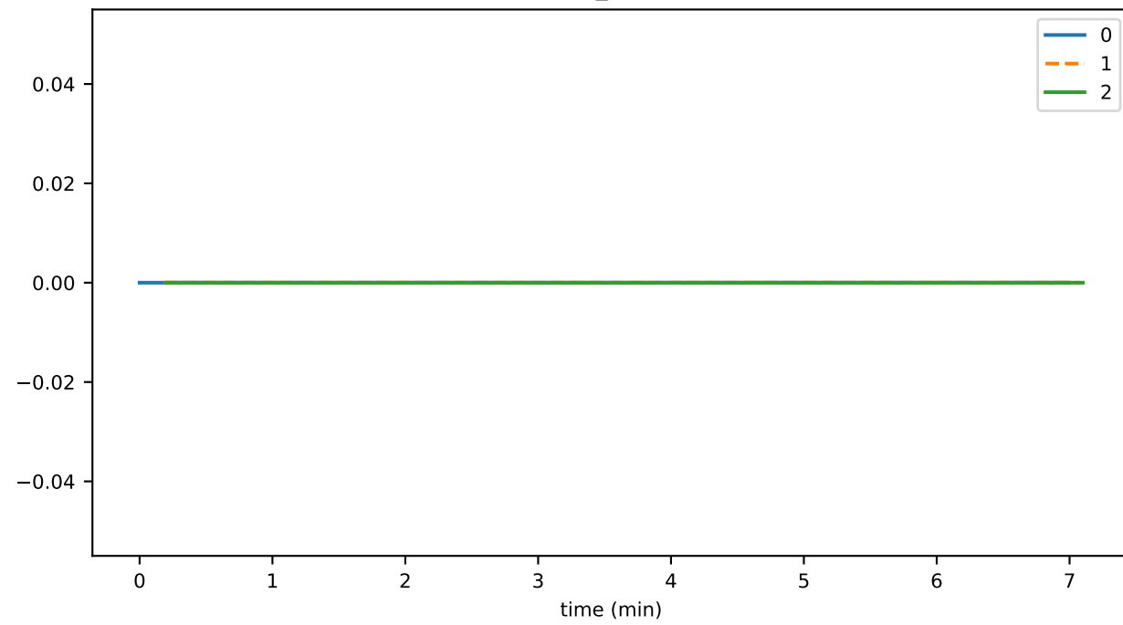
connSend_endOfBlock
