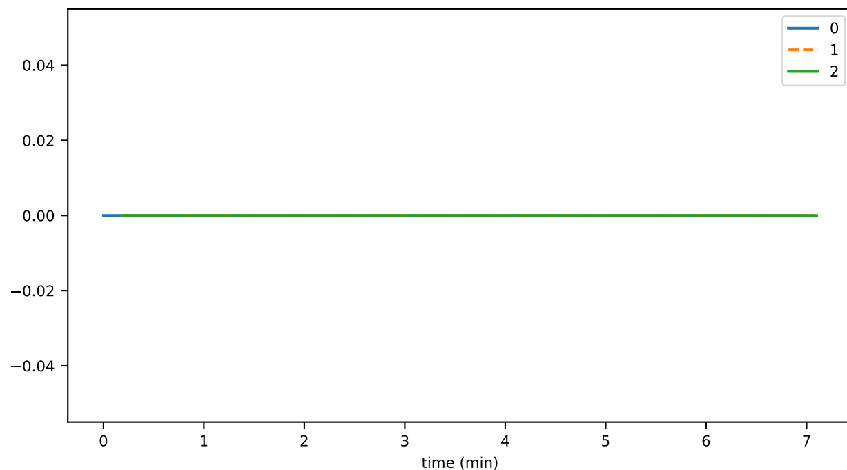
transactionGetReceiptDurationAvg
