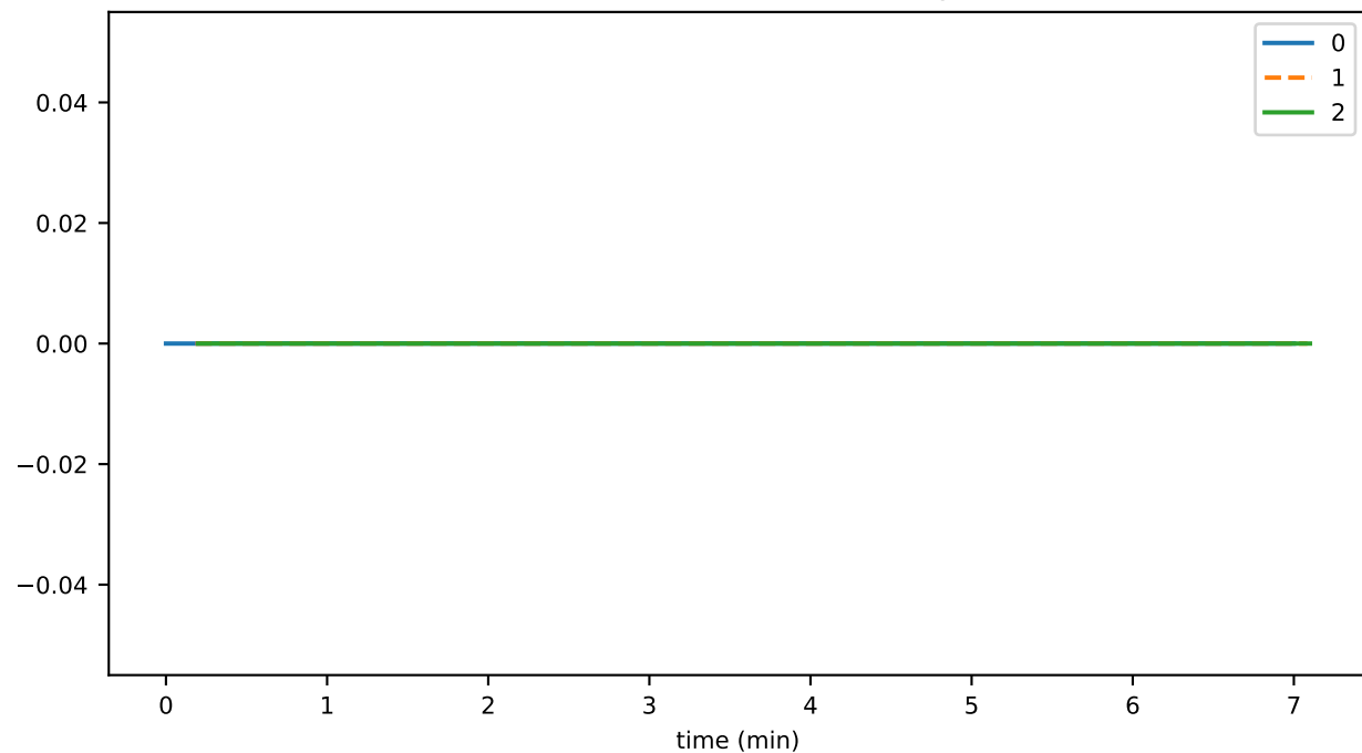
uncheckedSubmitThrottledTxns
