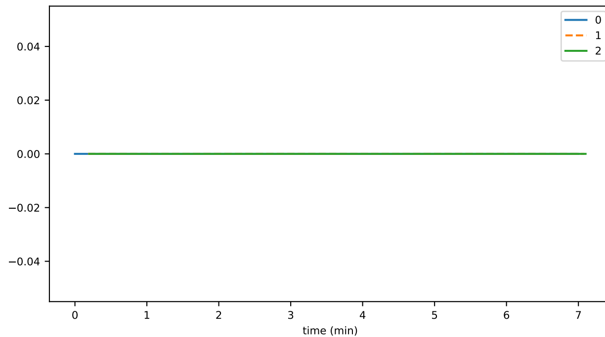
schedulesUsed
