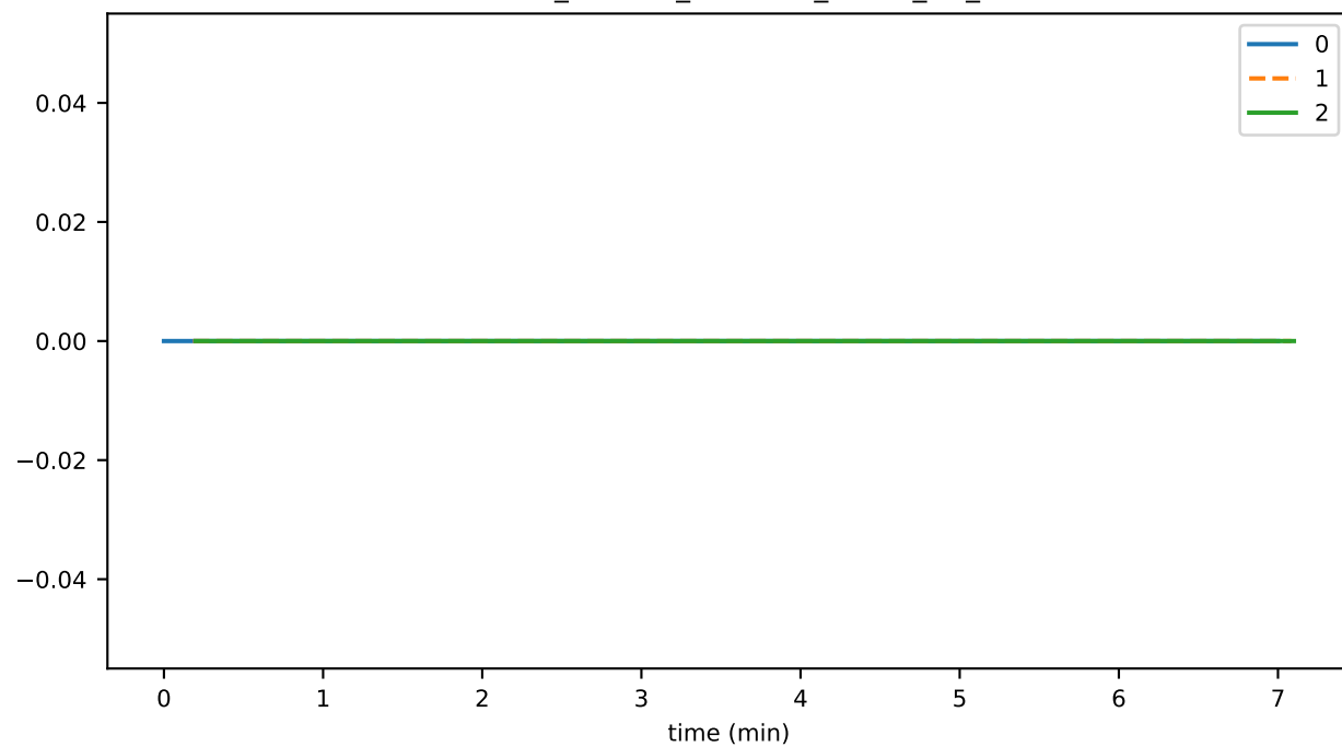
consensus_fraction_GETTING_STATE_TO_SIGN
