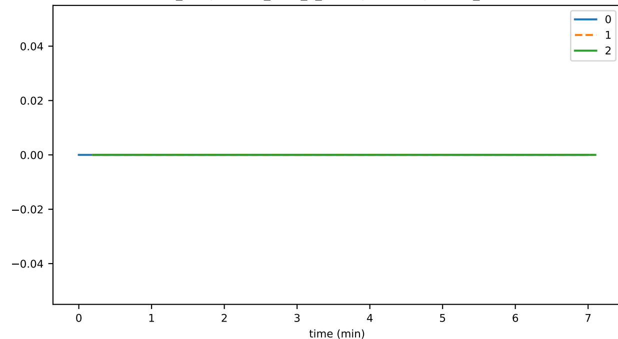
ds_compactions_level_6_leavesSavedSpaceMb_state
