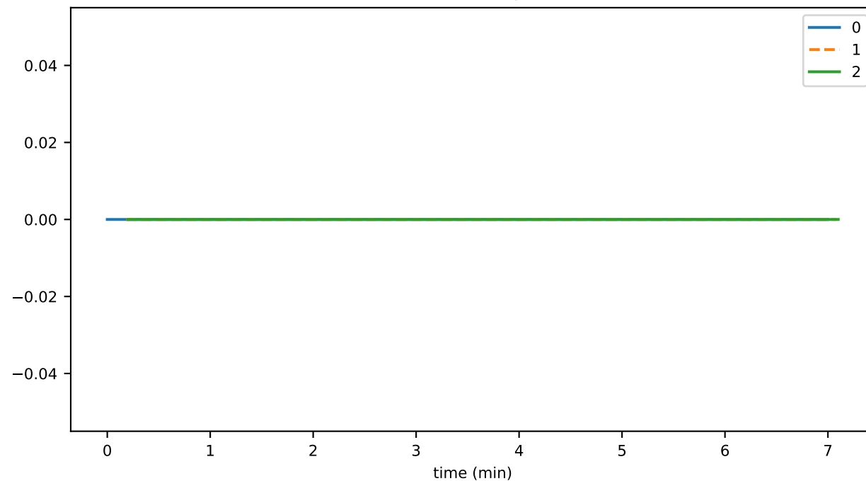
consensusTime
