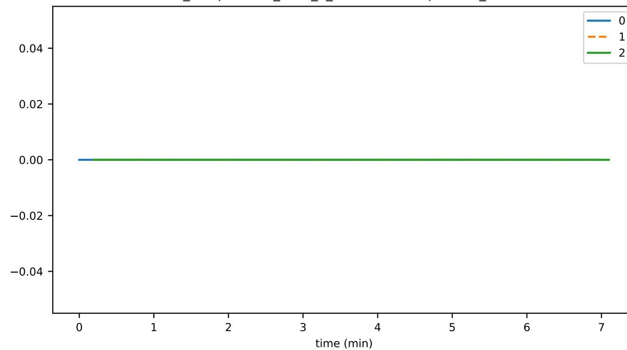
ds_compactions_level_2_hashesSavedSpaceMb_state
