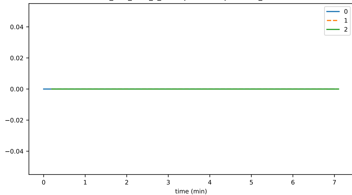
ds_files_level_3_leafKeysFileSizeByLevelMb_state
