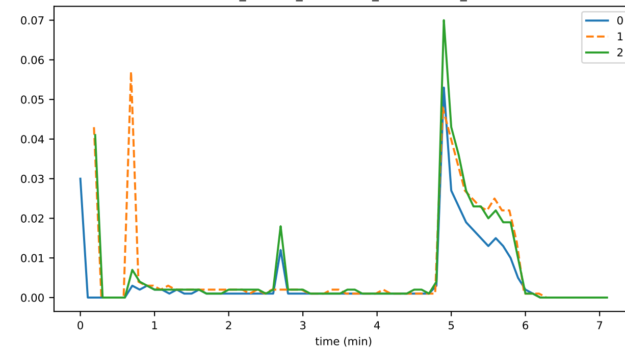
consensus_fraction_HANDLING_CONSENSUS_ROUND
