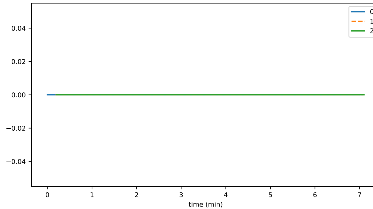
queriedAccountBalances
