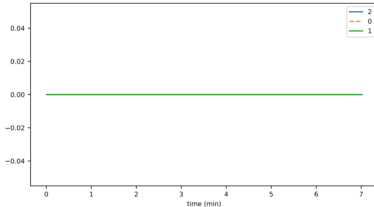
transactionGetReceiptDurationMax
