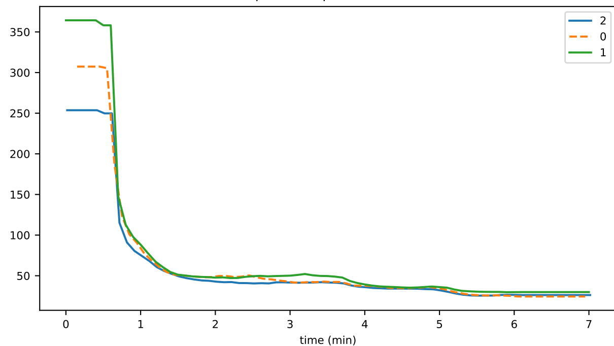
utilPngDurationMax
