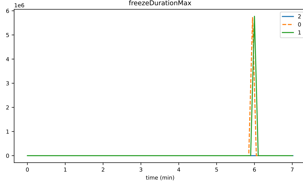
freezeDurationMax
