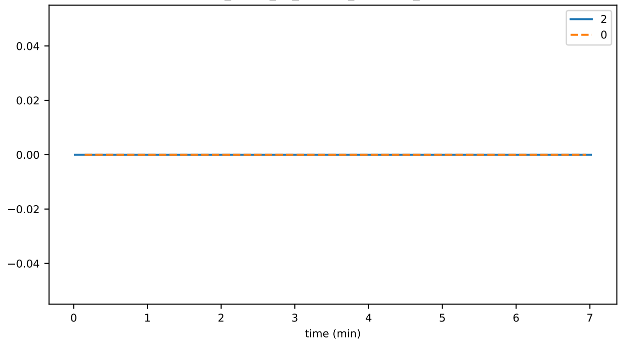
sync_phase_01_fraction_SENDING_EVENTS
