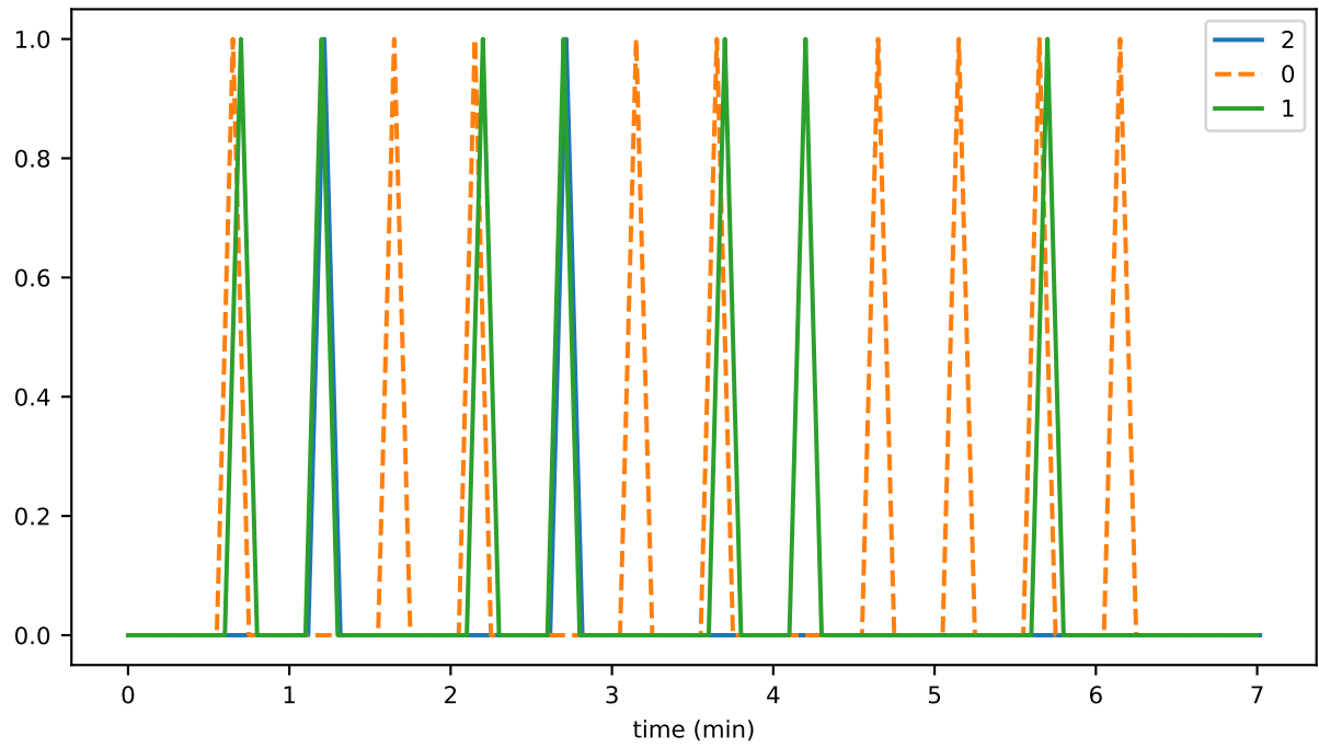
StateSnapshotManager_unhandled_task_count
