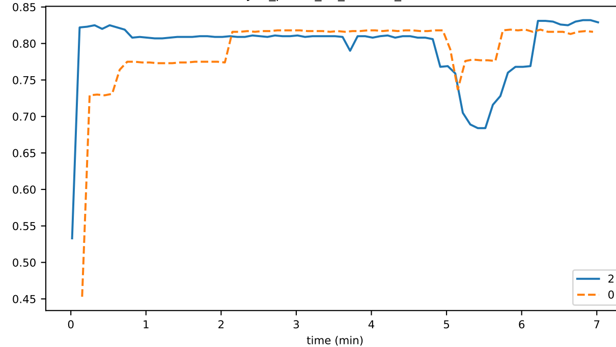
sync_phase_01_fraction_IDLE
