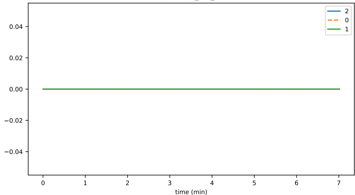
DigQuDepth
