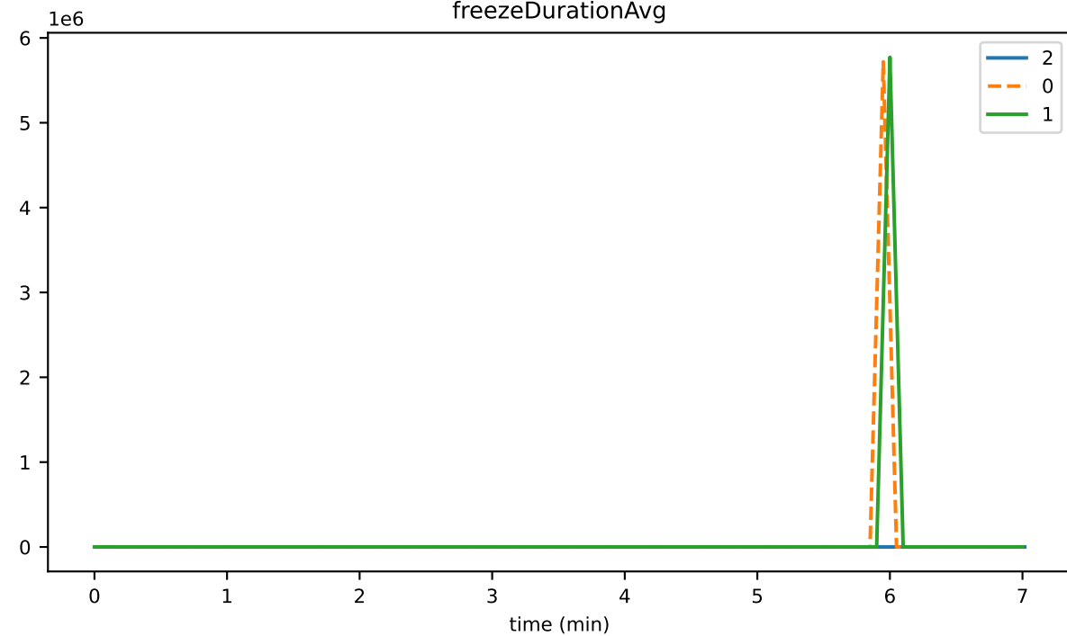
freezeDurationAvg
