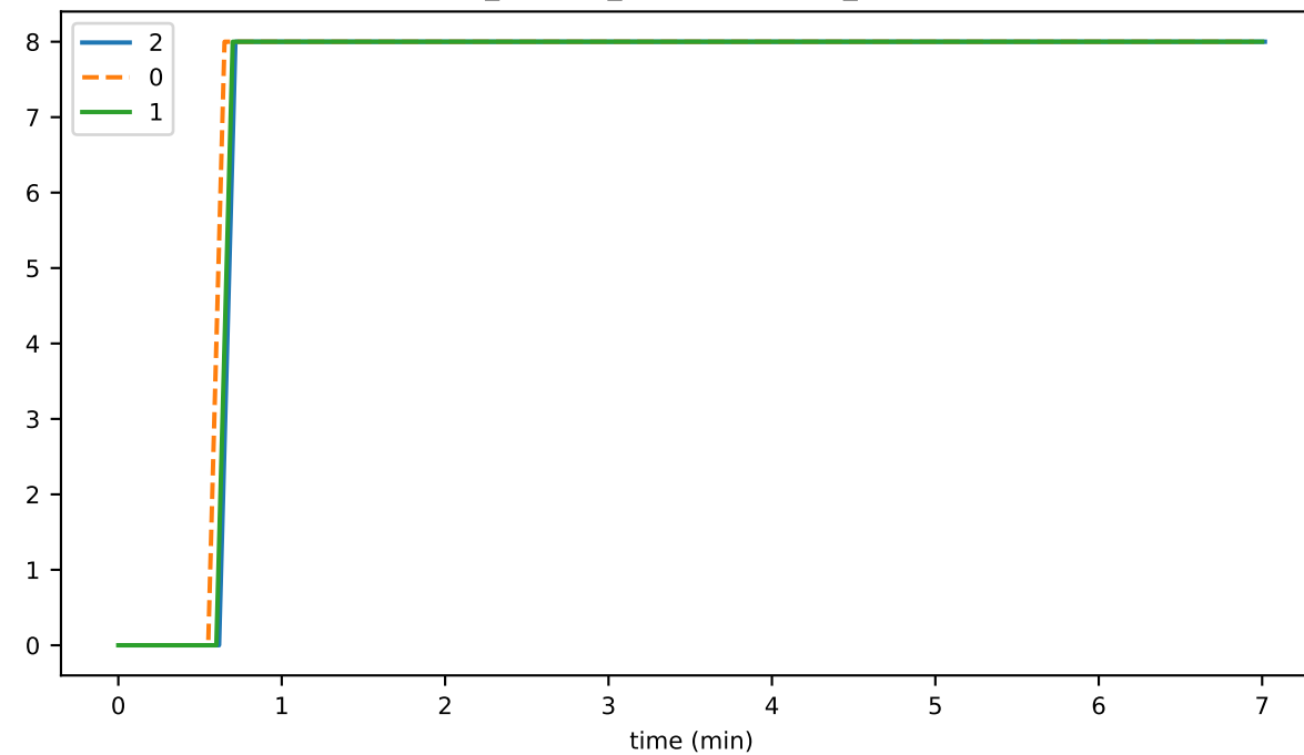
ds_offheap_hashesIndexMb_state
