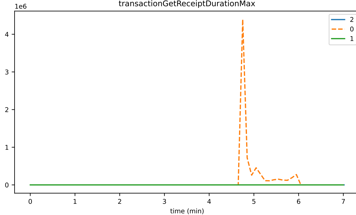
transactionGetReceiptDurationMax
