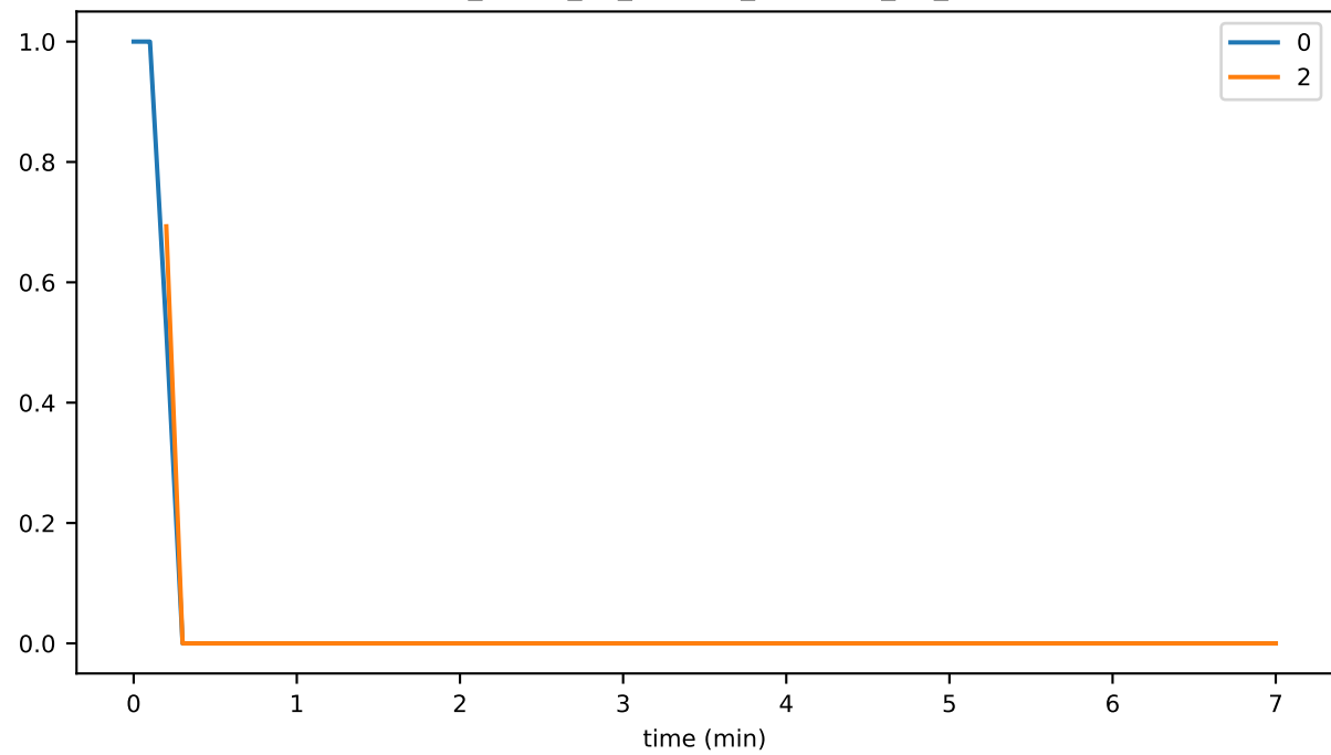
sync_phase_01_fraction_OUTSIDE_OF_RPC
