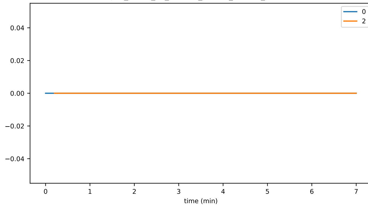
sync_phase_01_fraction_PLATFORM_STATUS_PREVENTING_SYNC
