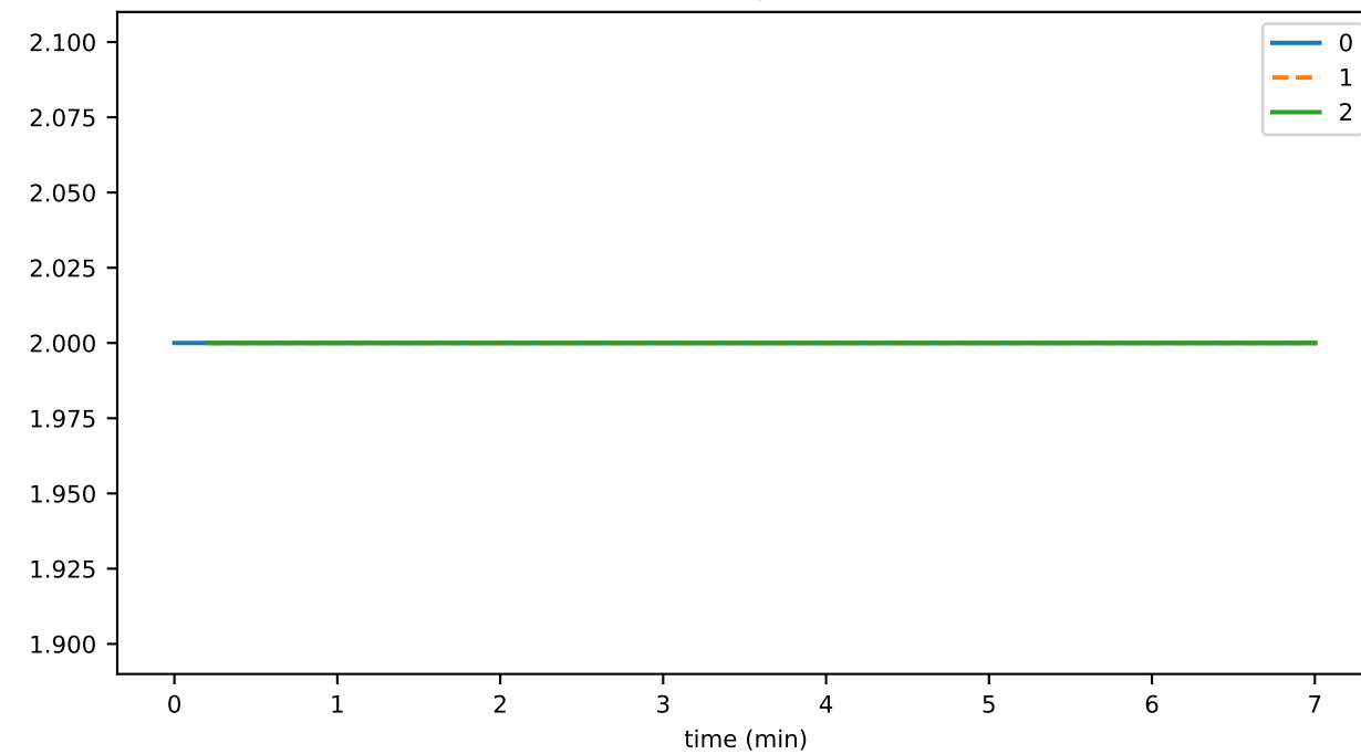
oldestSignedStateSeconds
