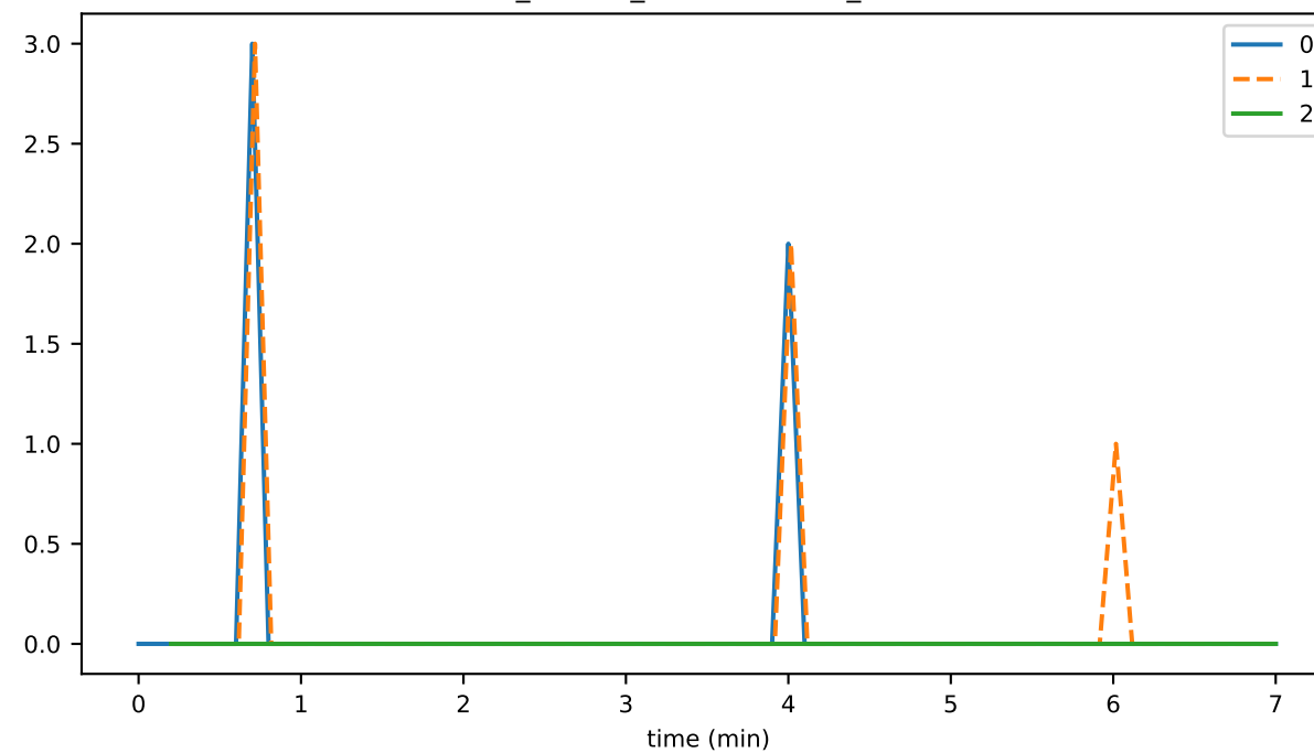
ds_flushes_leavesDeleted_state
