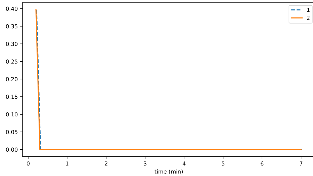
sync_phase_00_fraction_OUTSIDE_OF_RPC
