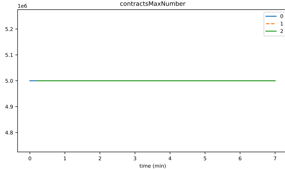
contractsMaxNumber
