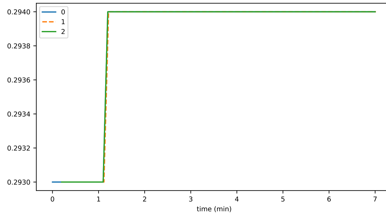
preconsensusEventFileTotalSizeGB
