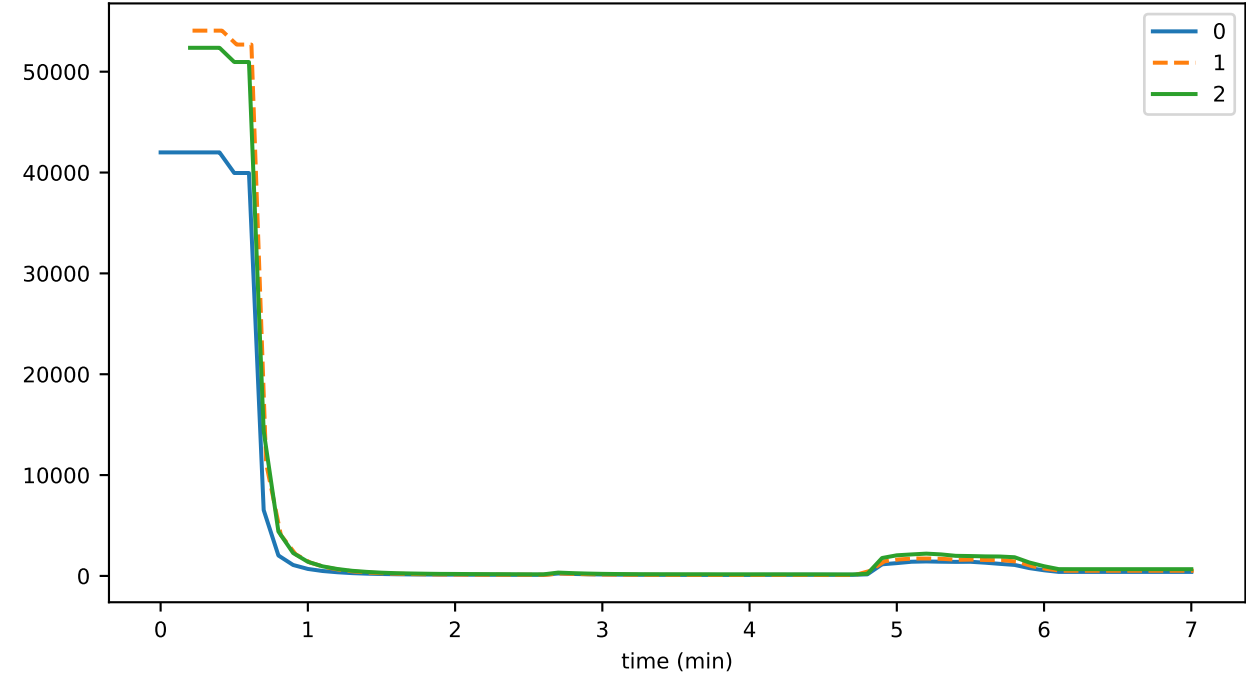
consensus_time_HANDLING_CONSENSUS_ROUND
