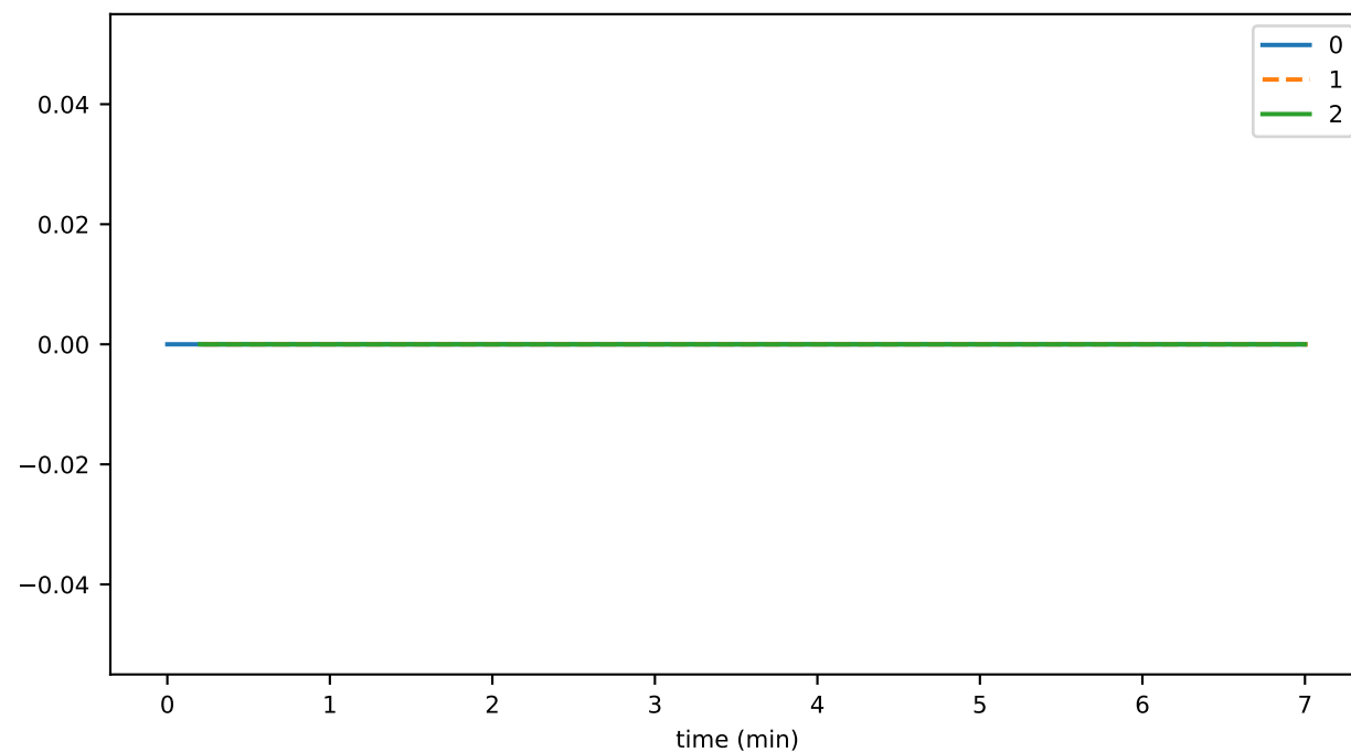
contractsMaxNumber
