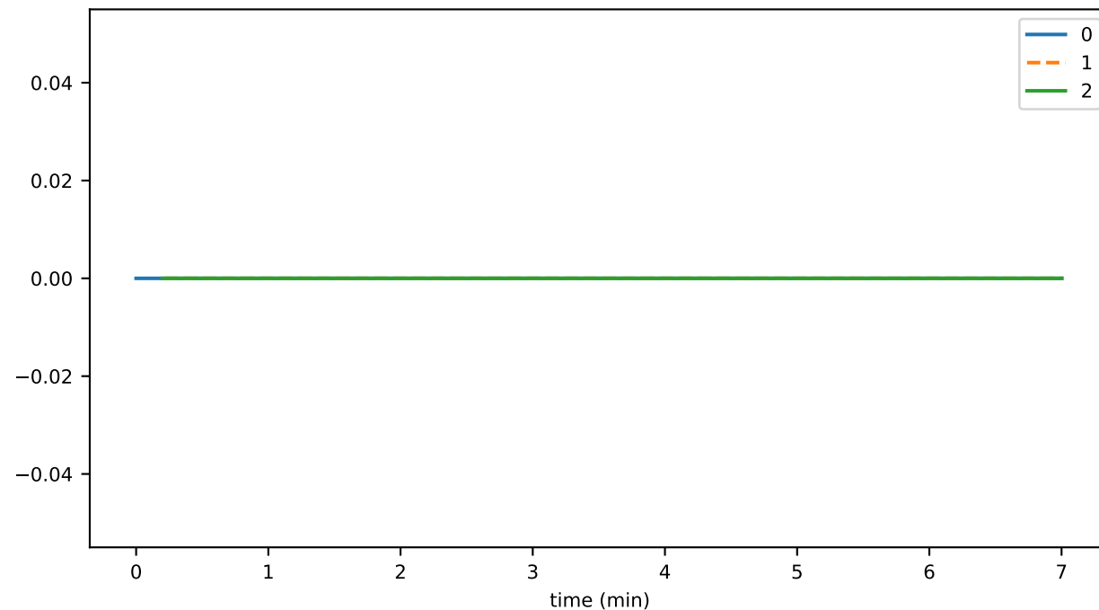
stateSignatureTransactionThrottledTxns
