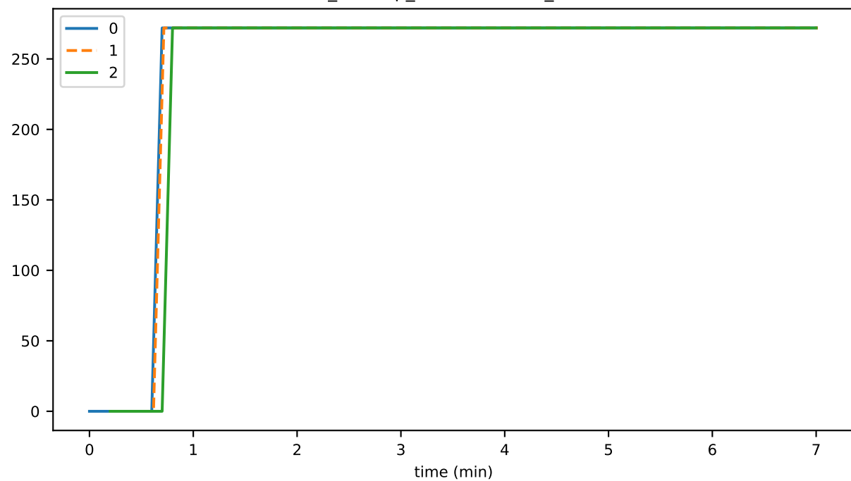
ds_offheap_dataSourceMb_state
