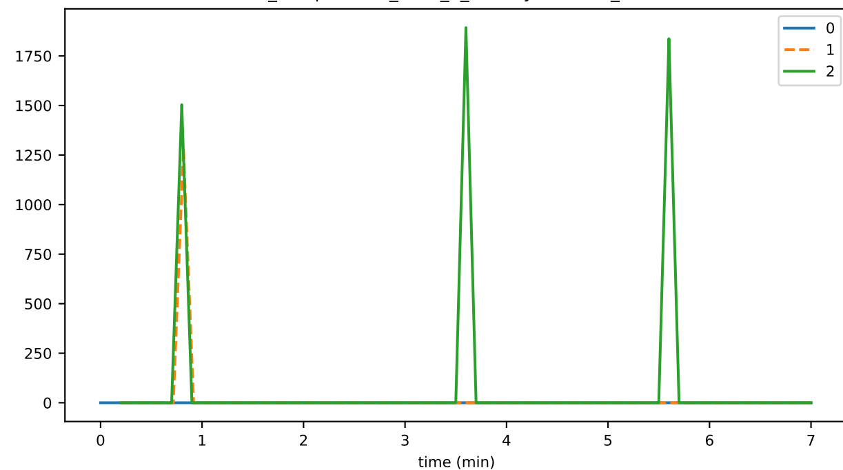
ds_compactions_level_1_leavesTimeMs_state
