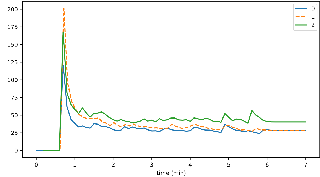
consensus_time_HANDLING_CONSENSUS_ROUND
