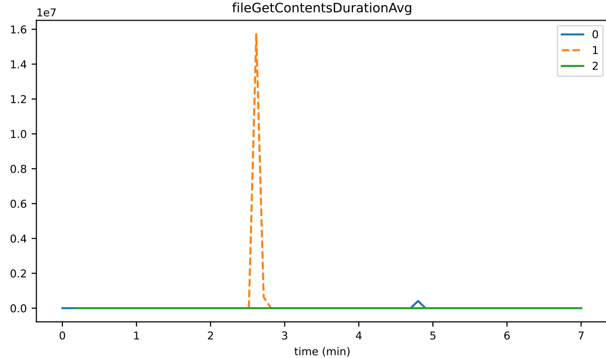
fileGetContentsDurationAvg
