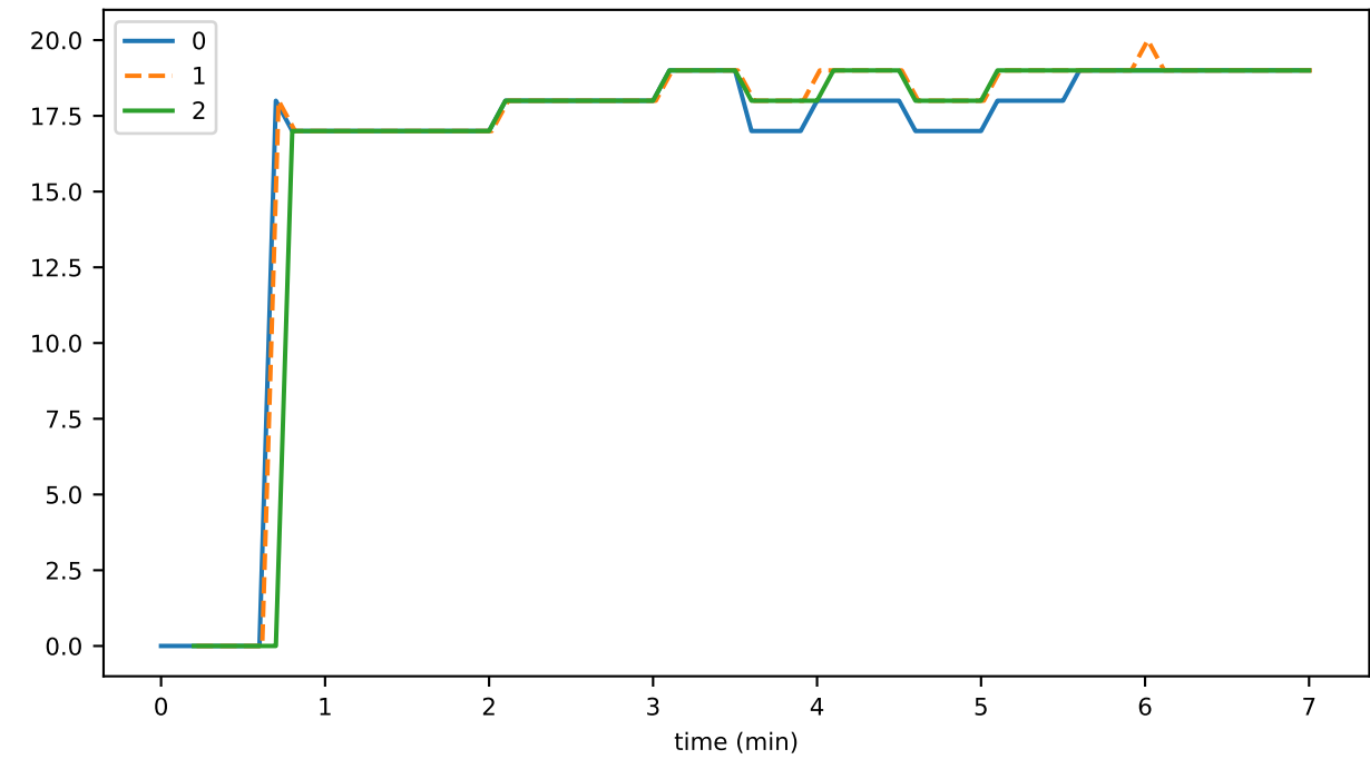
ds_files_leavesStoreFileCount_state
