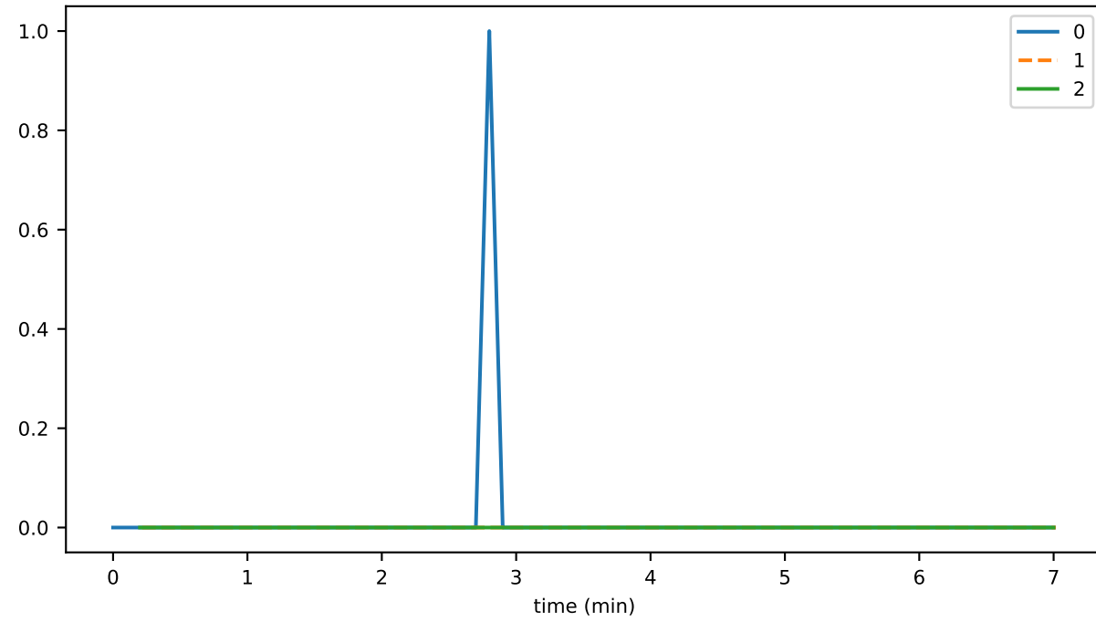
broadcastDisabledDueToOverload
