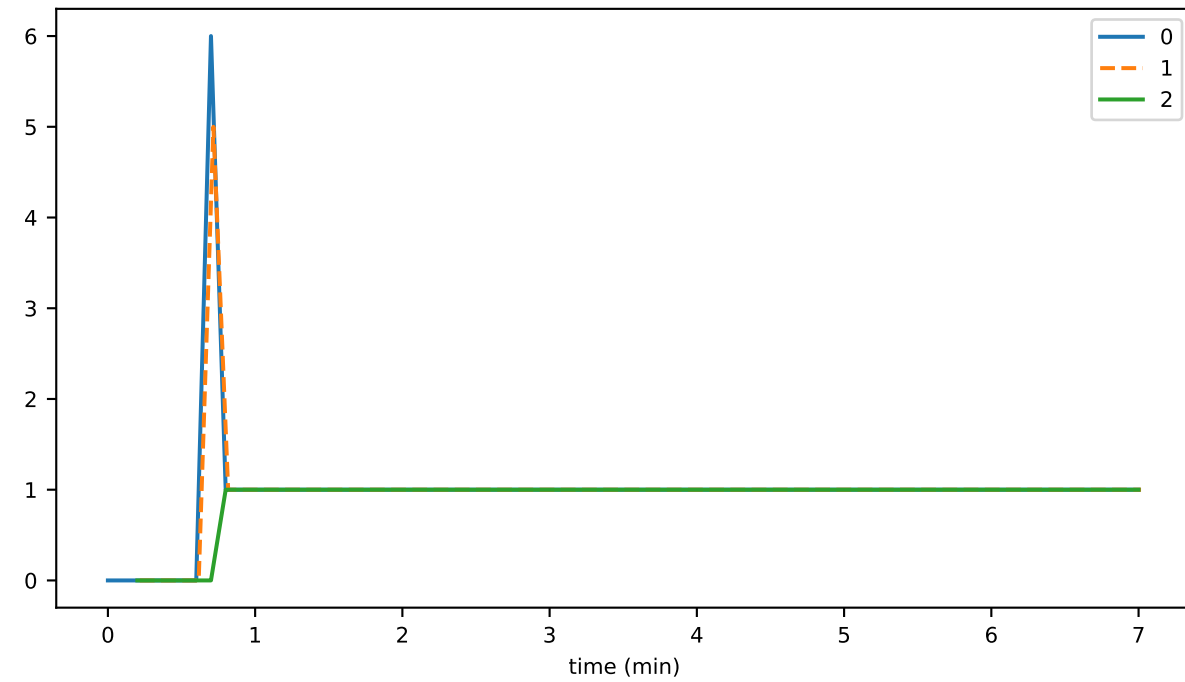
ds_files_leafKeysStoreFileSizeMb_state
