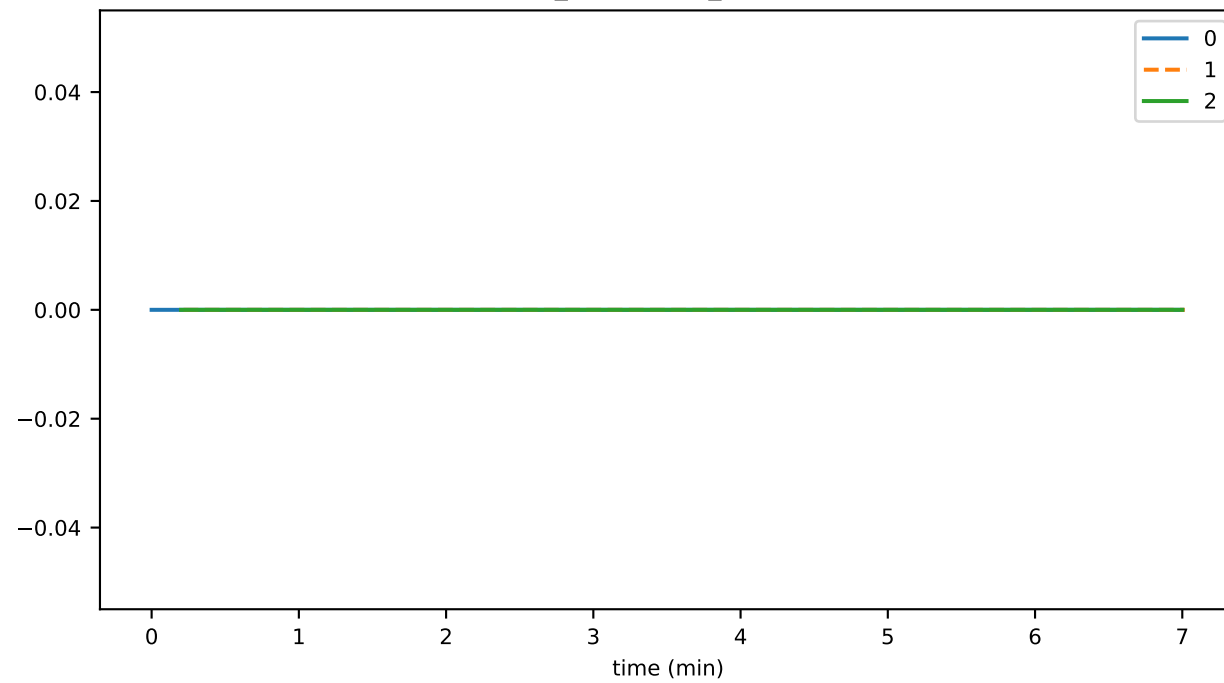
connRecv_endStream_badBlockProof
