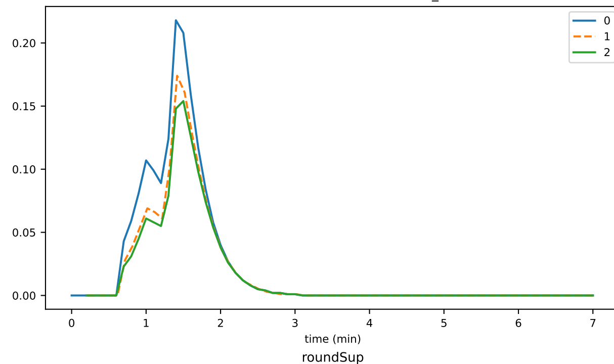
roundsSinceLastConsensusEvent_1
