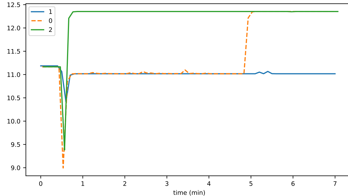
numIndirectProofs
