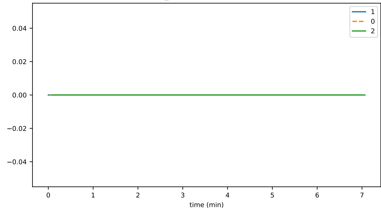
conn_headerSentToAckLatency
