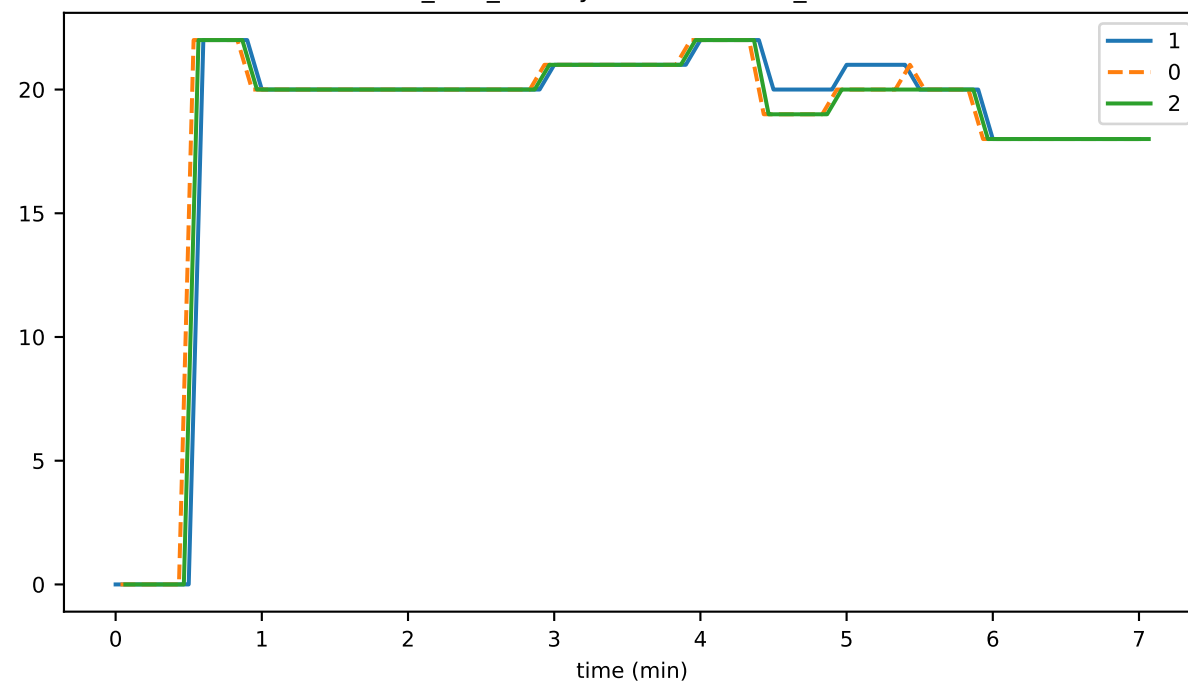
ds_files_leavesStoreFileCount_state
