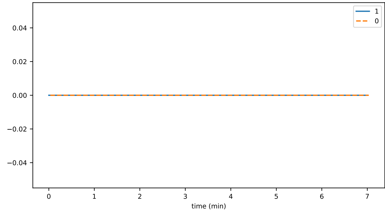
disconnects_per_sec_02
