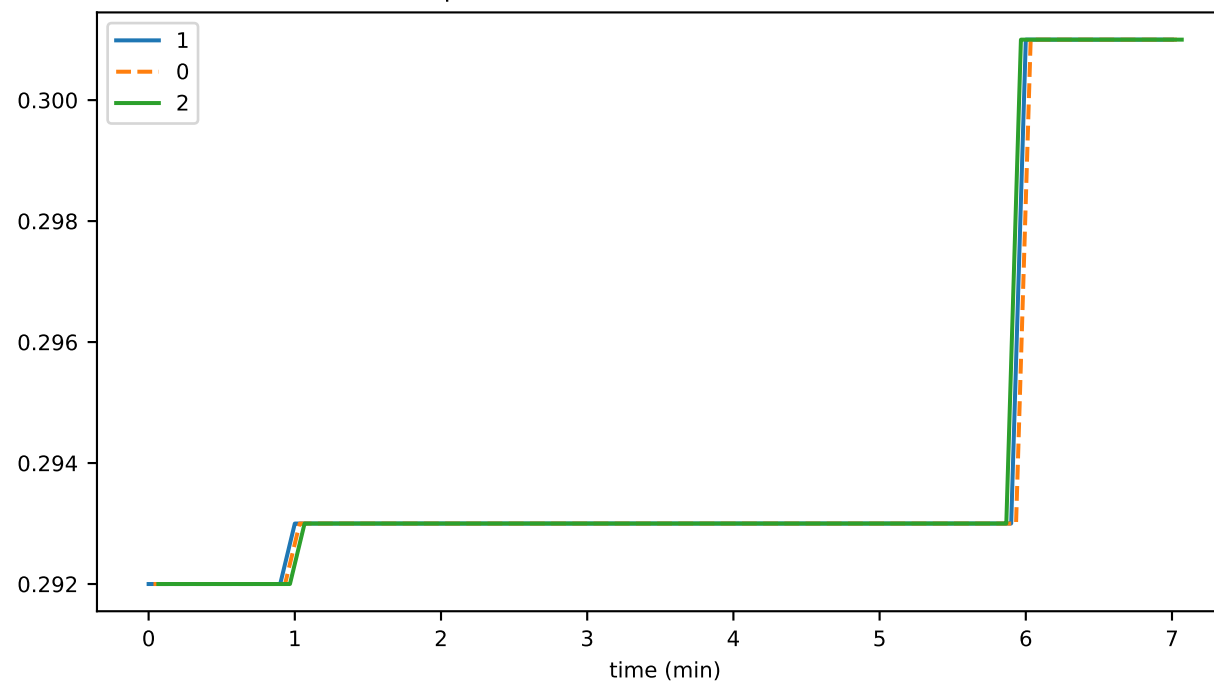
preconsensusEventFileTotalSizeGB
