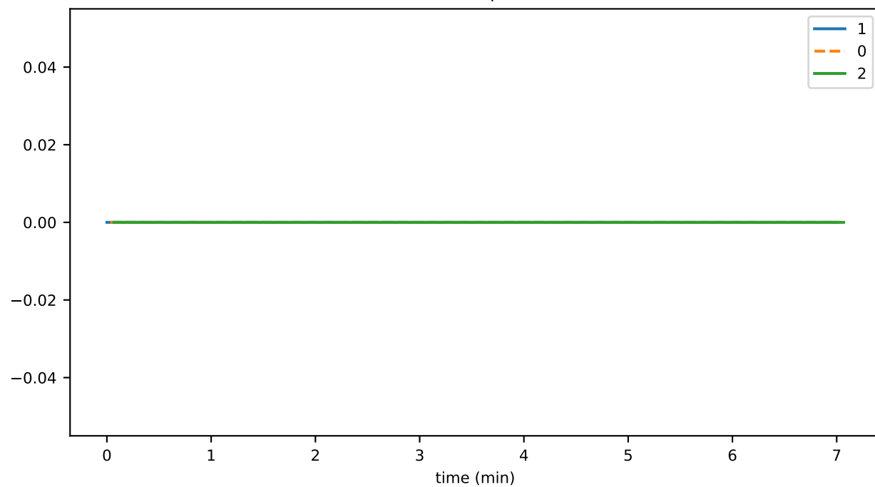
tokenCancelAirdropThrottledTxns
