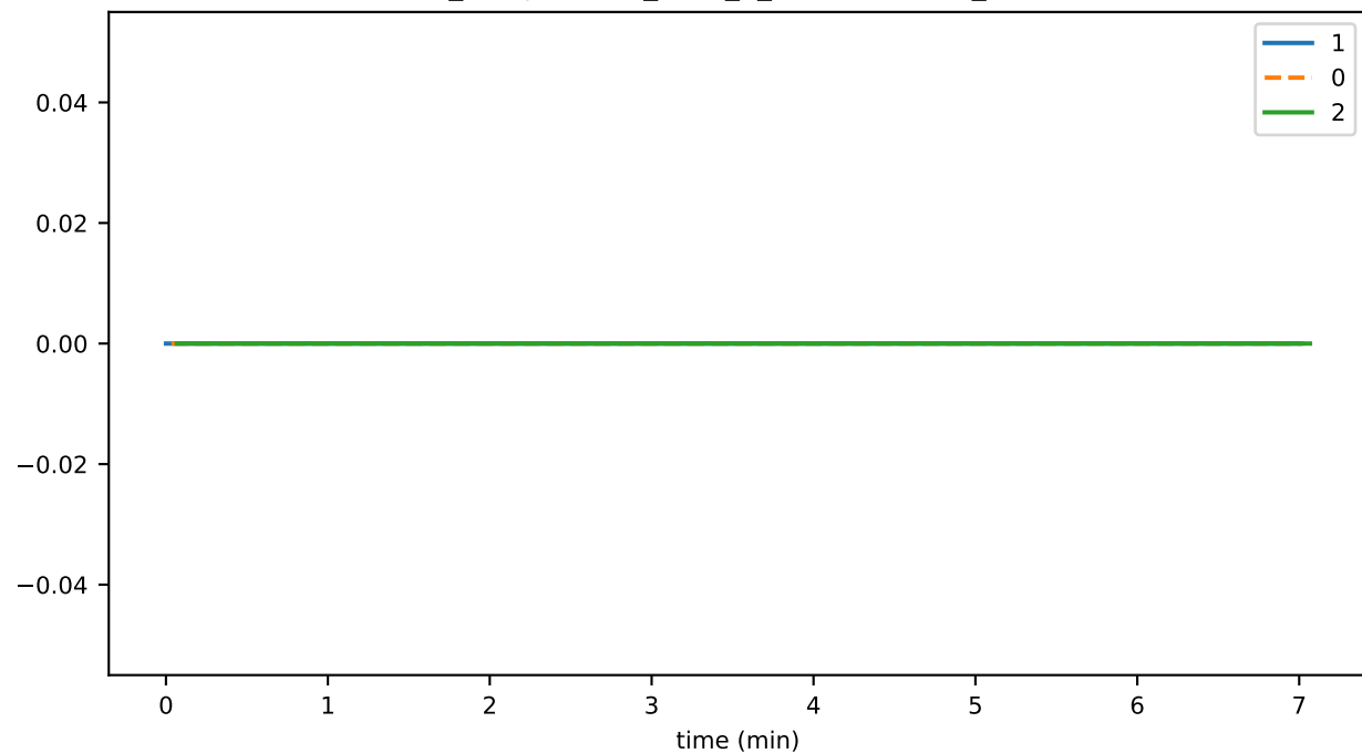
ds_compactions_level_5_hashesTimeMs_state
