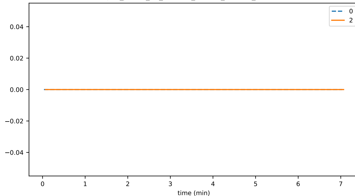
sync_phase_01_fraction_PLATFORM_STATUS_PREVENTING_SYNC
