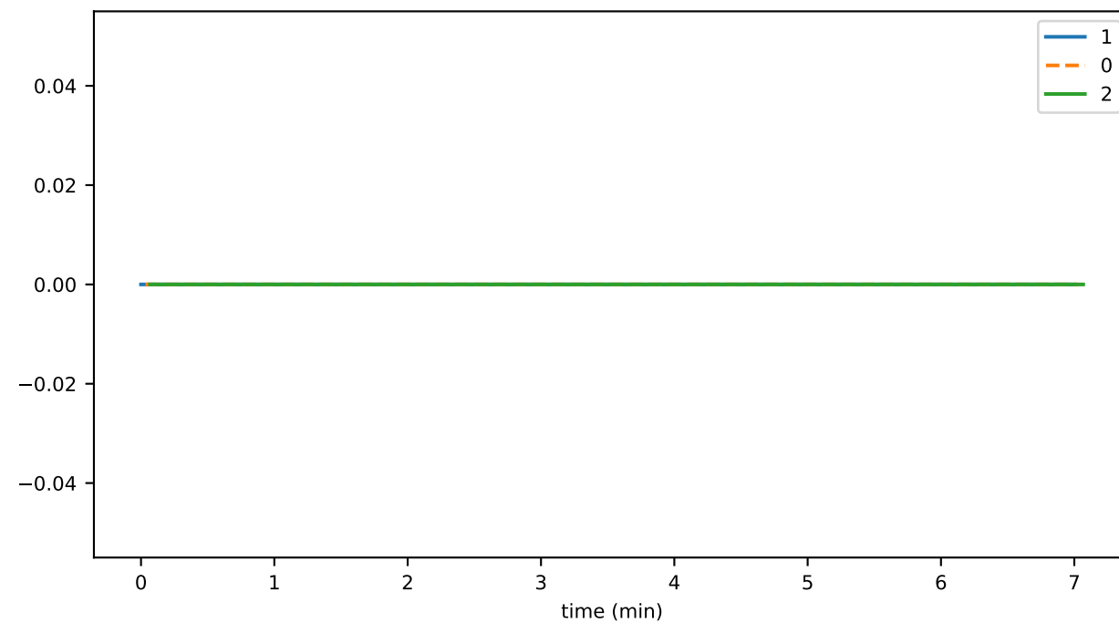
tokenCreateDurationMax
