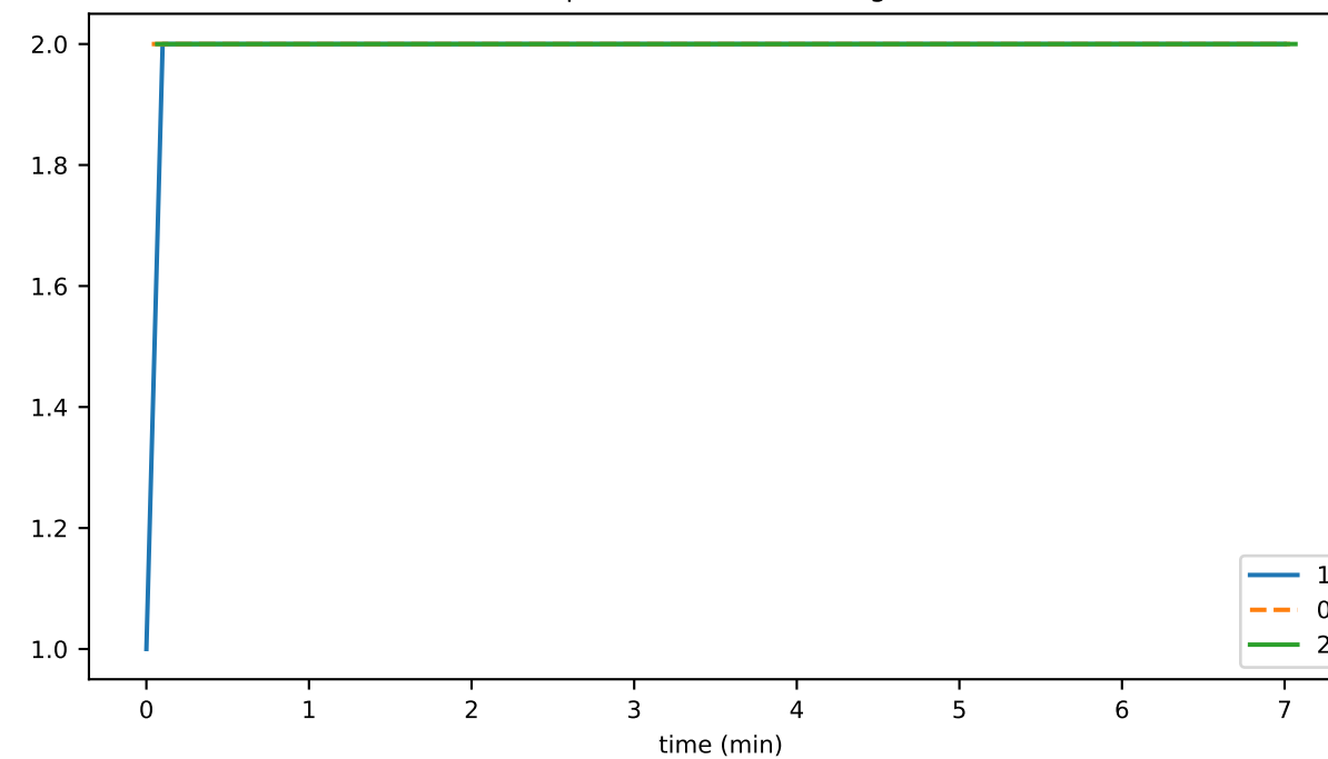
rpcReadThreadRunning
