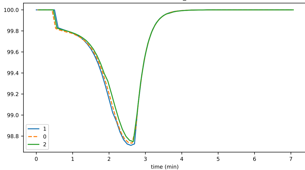
nodeActivePercent_node2
