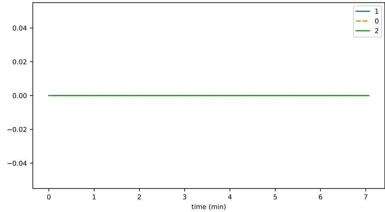
staleTransactions
