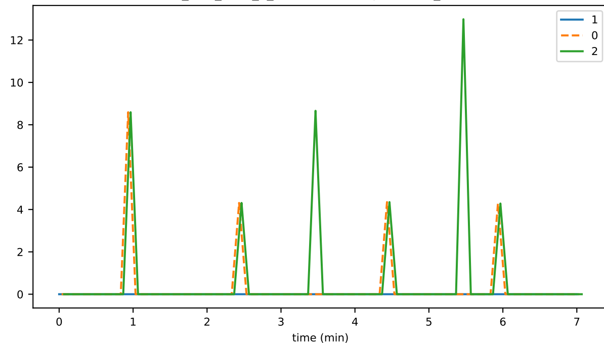
ds_files_level_3_leafKeysFileSizeByLevelMb_state
