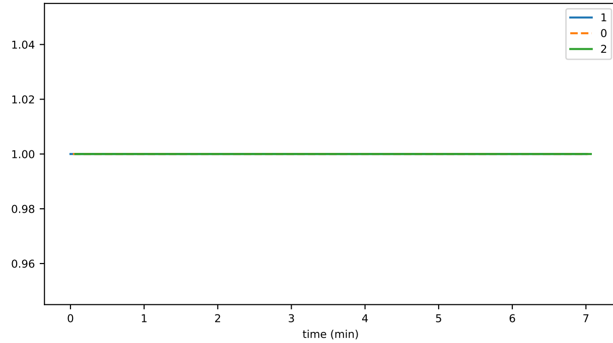
hintsKeyPublicationDurationAvg
