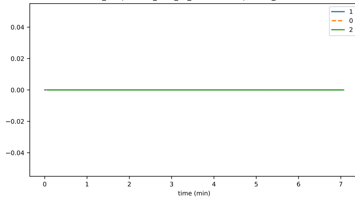
ds_compactions_level_10_leavesSavedSpaceMb_state
