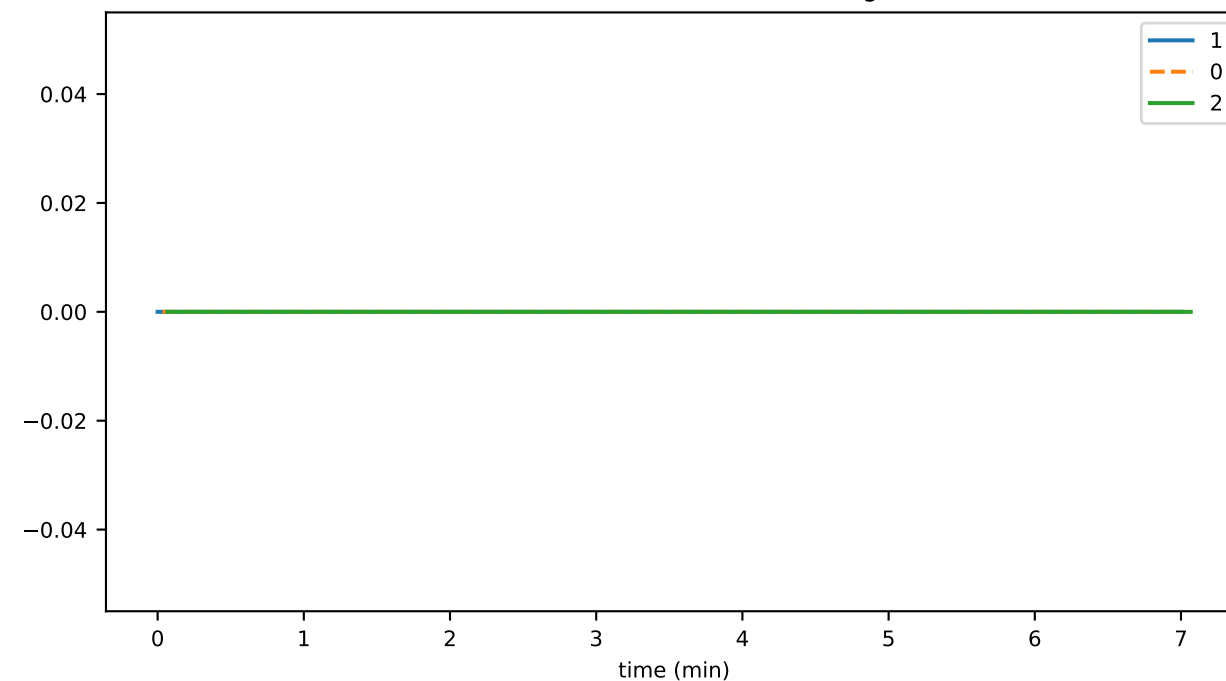
contractAutoRenewDurationAvg
