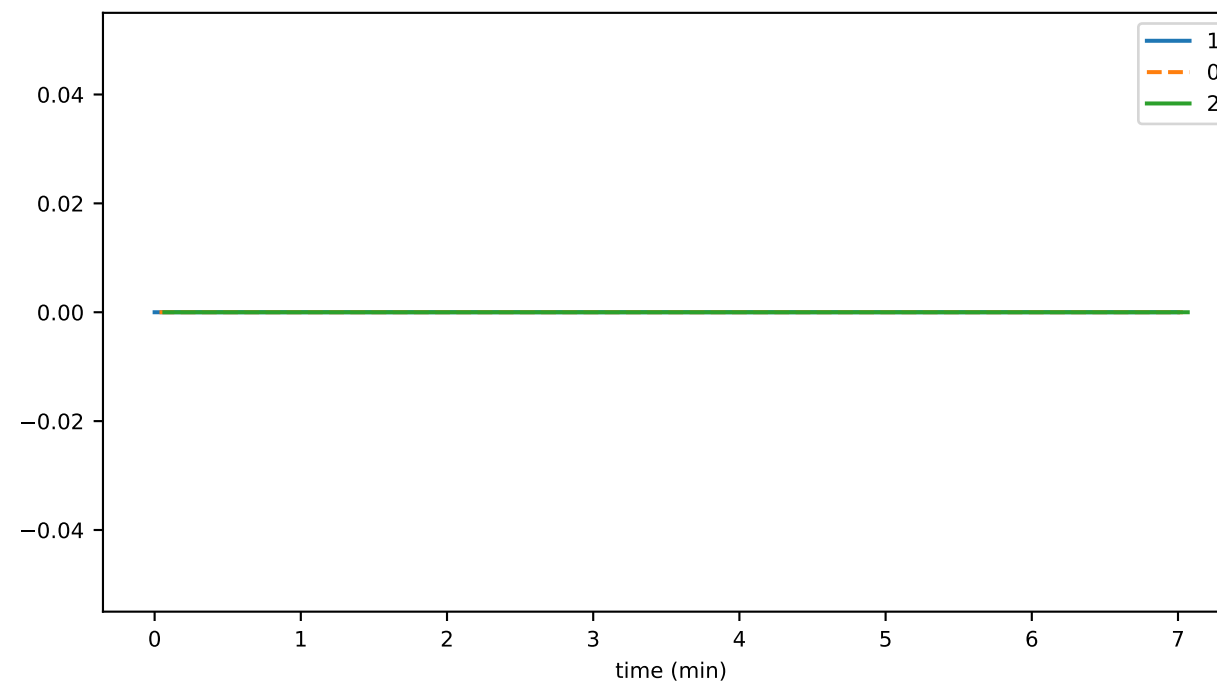
SigBatches_per_sec
