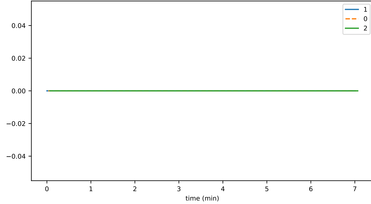
contractGetRecordsThrottledTxns
