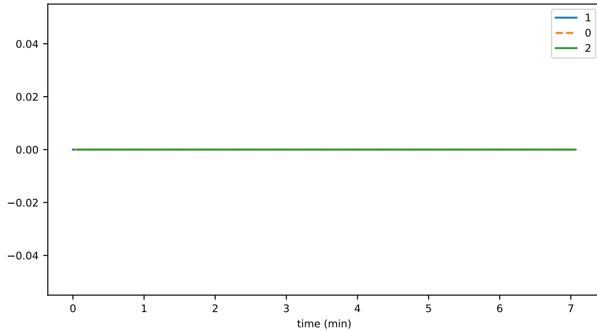
conn_connClose_newConnection
