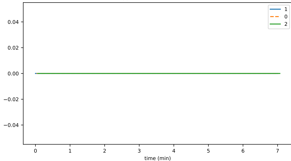
cryptoDeleteAllowanceDurationMax
