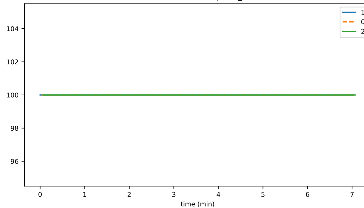
nodeActivePercentSnapshot_node0
