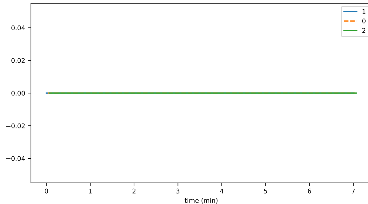
crsPublicationDurationMax
