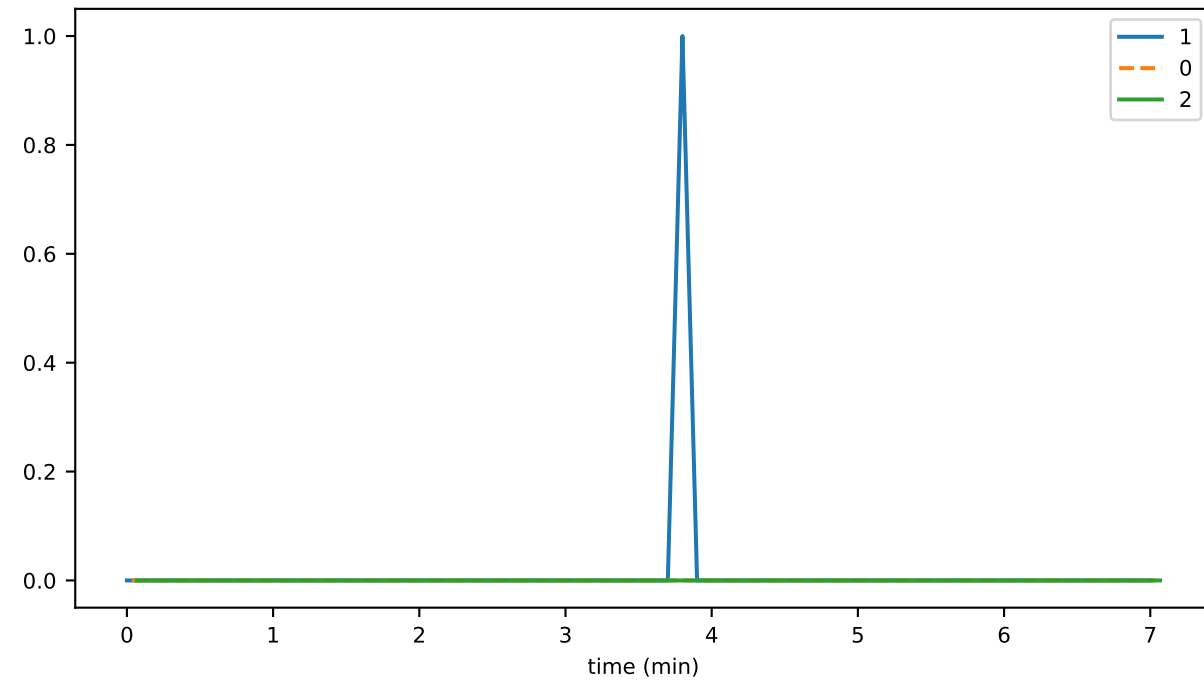
branchingNodeCount
