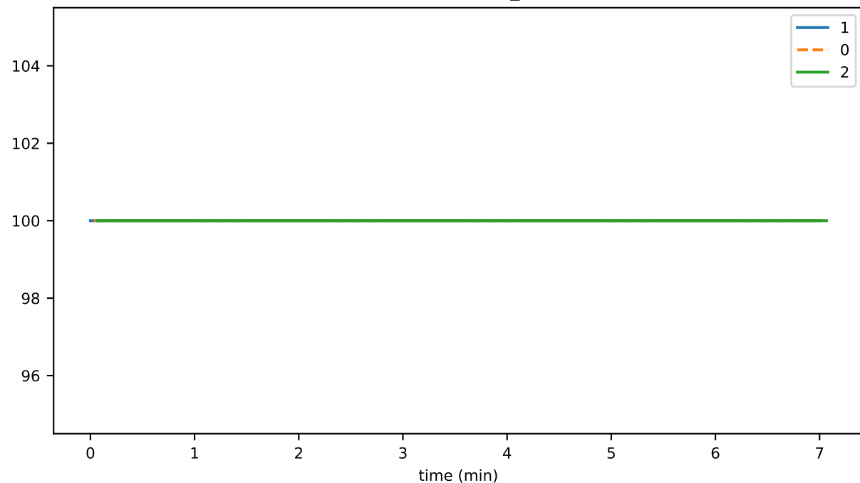
nodeActivePercent_node2
