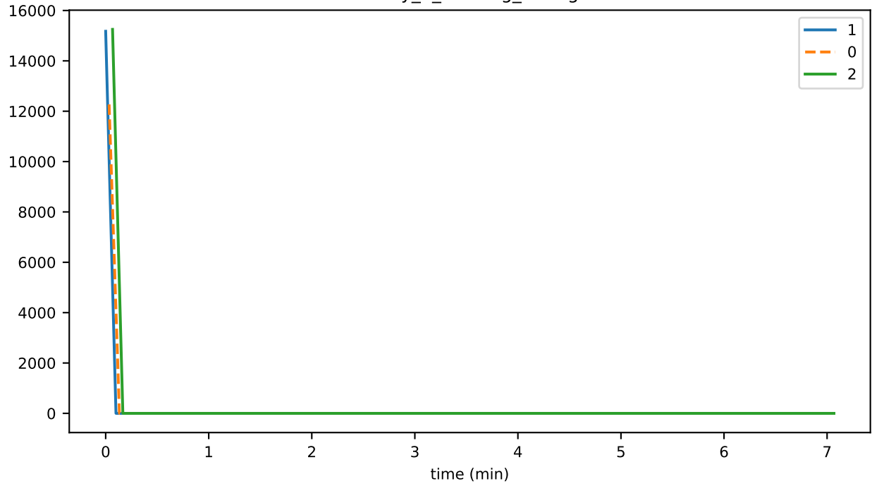
eventDelay_1_hashing_storageMAX
