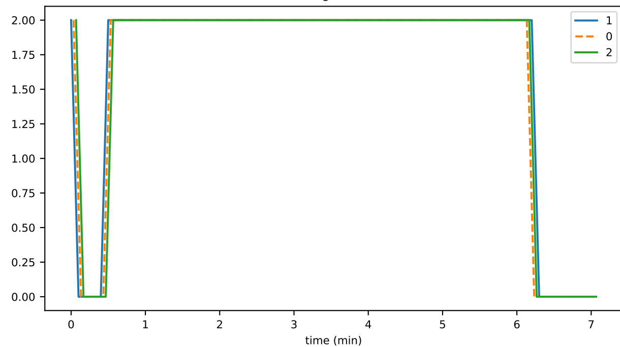
numVotingRoundsMAX
