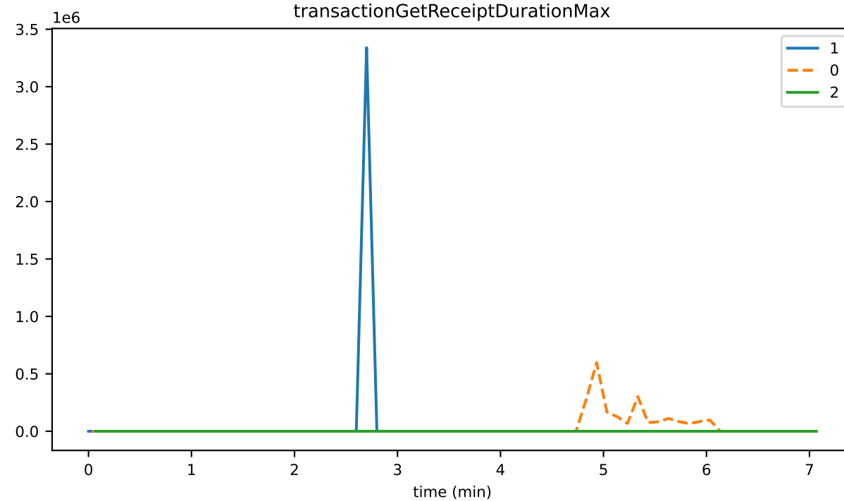
transactionGetReceiptDurationMax
