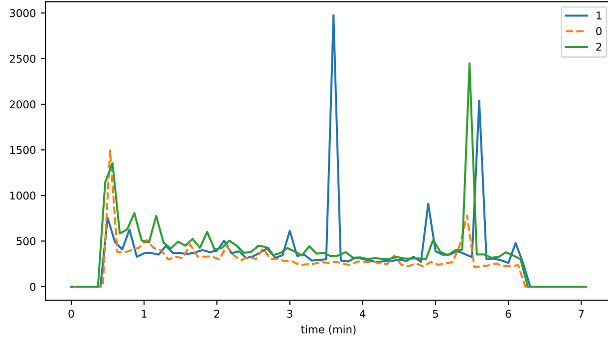
eventDelay_5_orphanBuffer_gossipMAX
