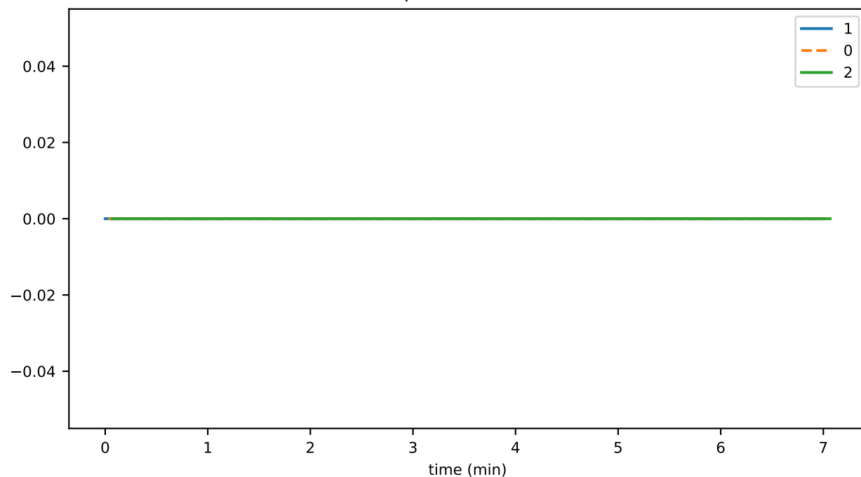
freezeDurationAvg
