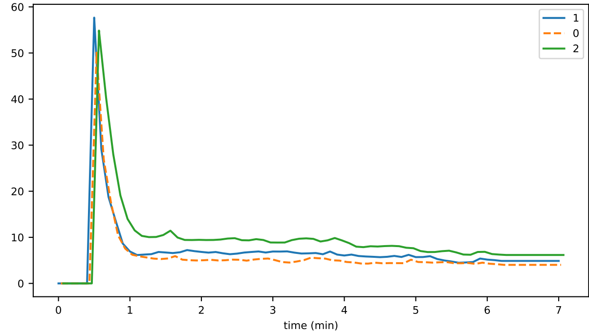
eventDelay_1_hashing_gossip
