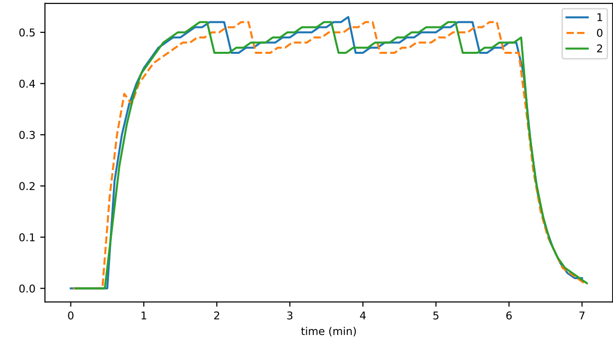
staleTransactions
