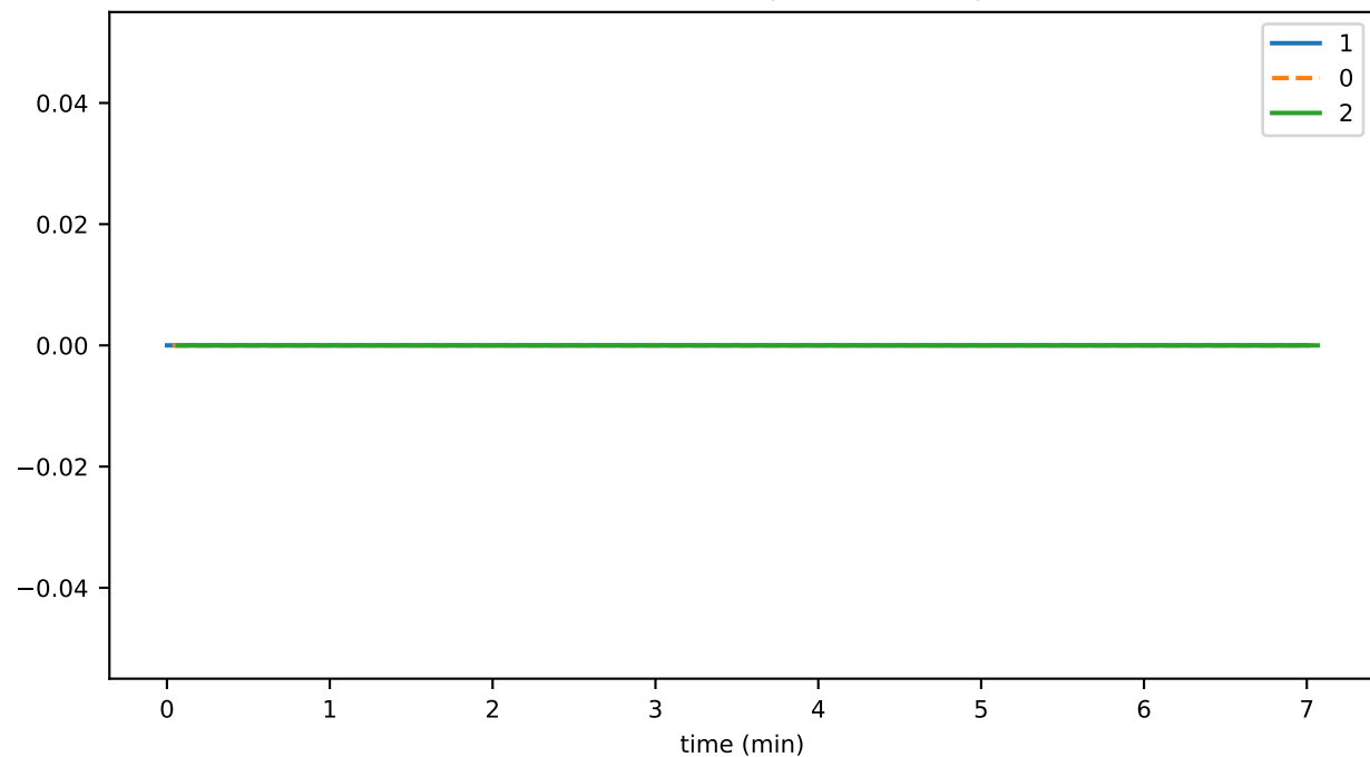
consensusDeleteTopicThrottledTxns
