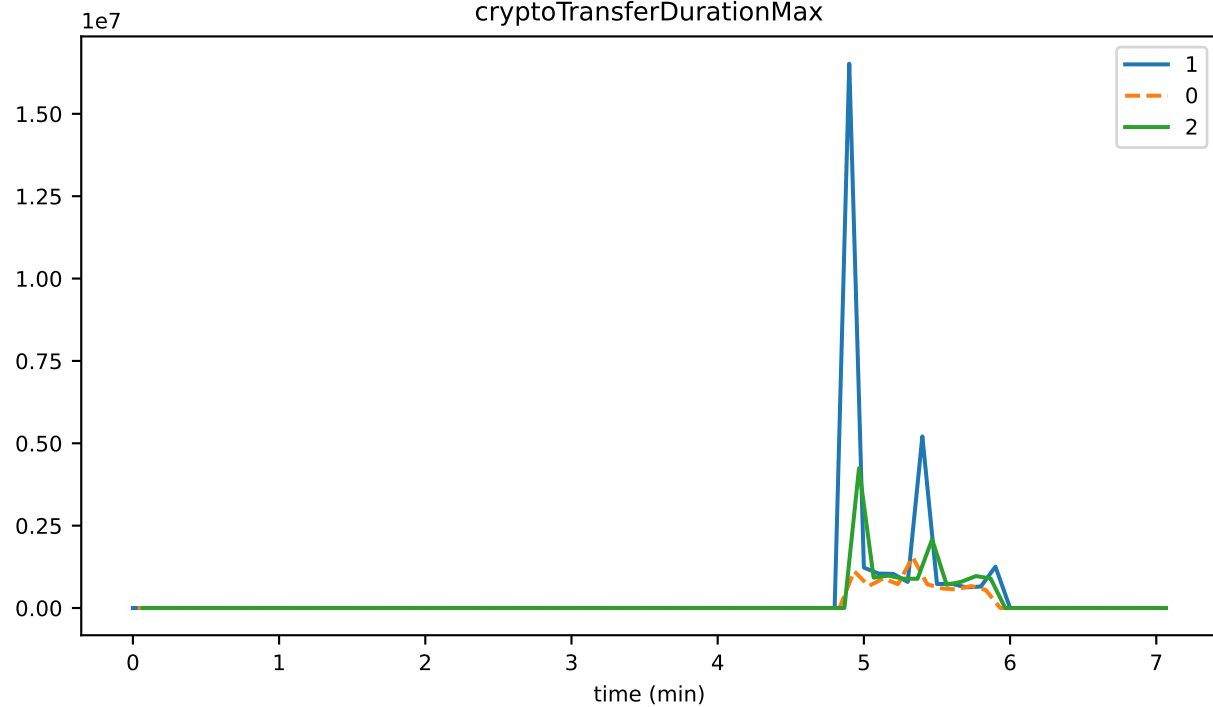
cryptoTransferDurationMax
