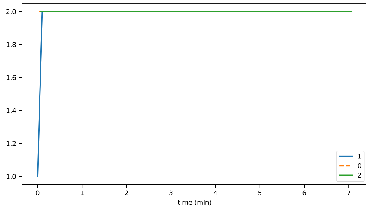
scheduleCreateDurationMax
