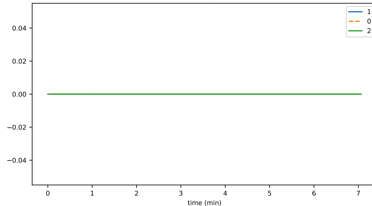
tokenClaimAirdropDurationAvg
