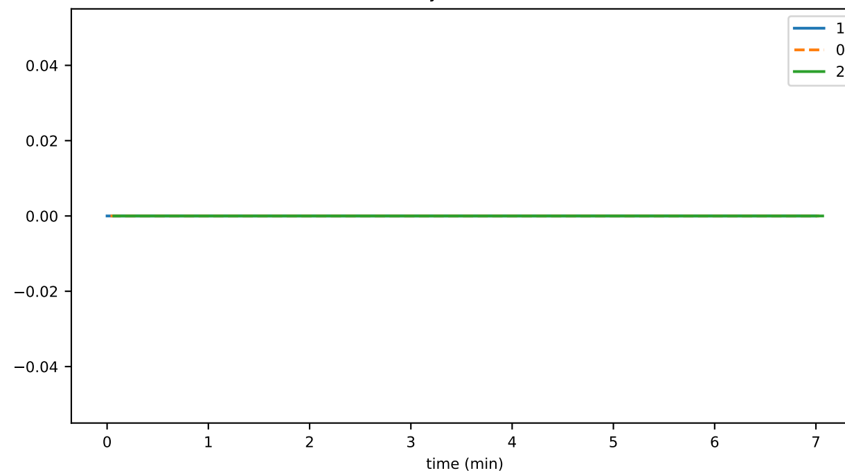
doNotSyncHalted
