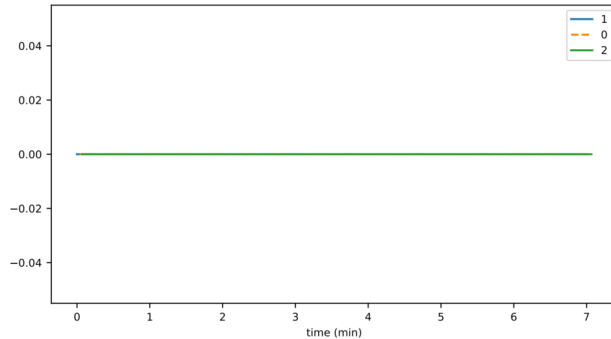
cryptoTransferThrottledTxns
