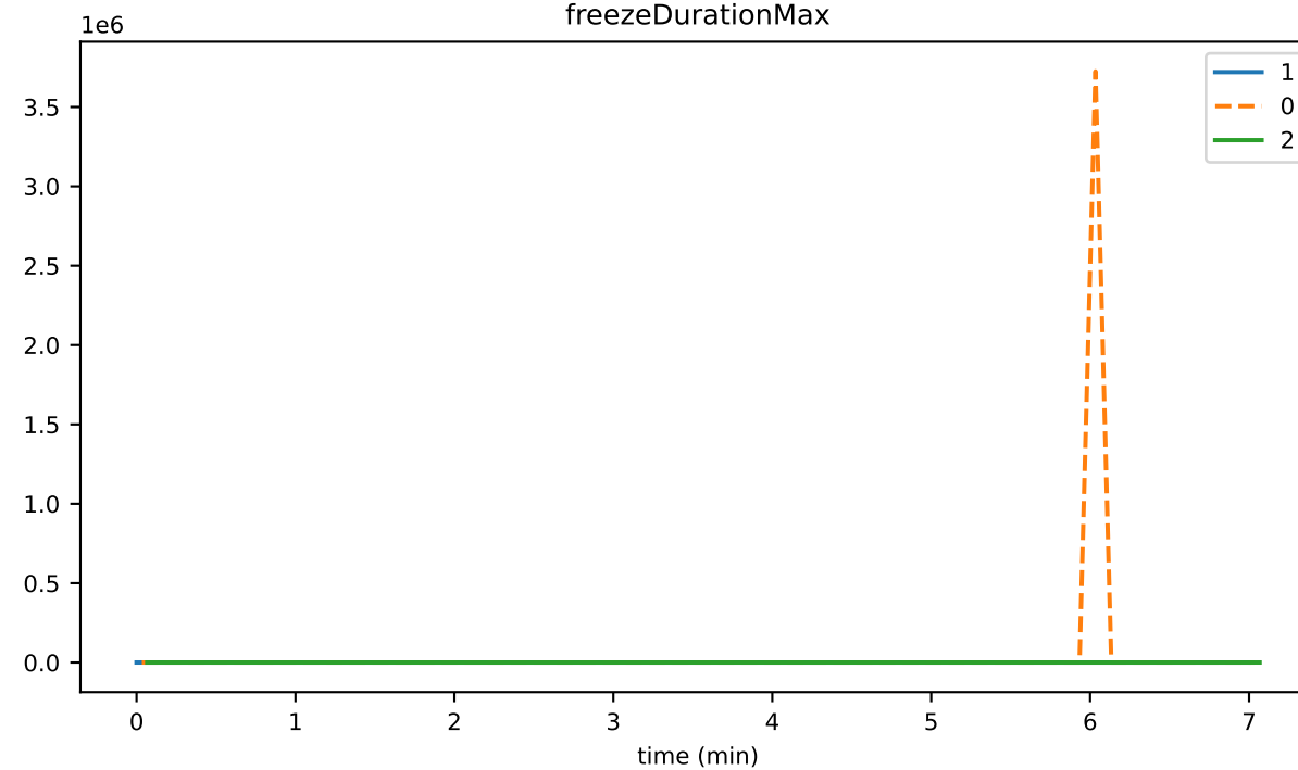
freezeDurationMax
