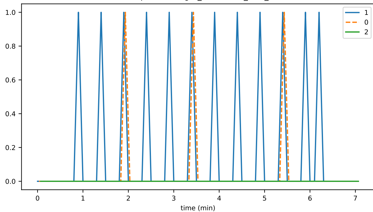
StateSnapshotManager_unhandled_task_count
