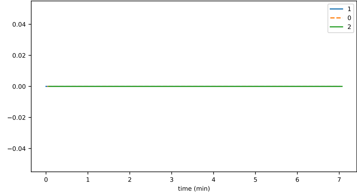
hintsKeyPublicationDurationMax
