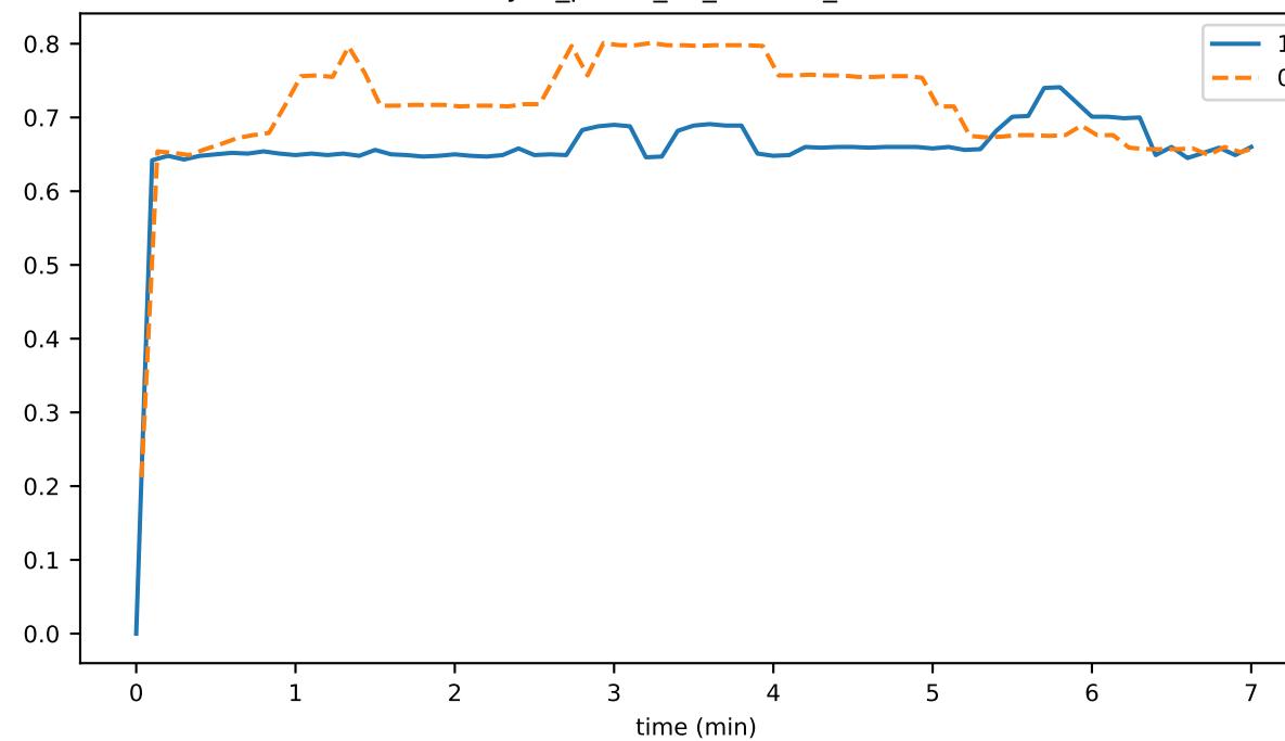
sync_phase_02_fraction_IDLE
