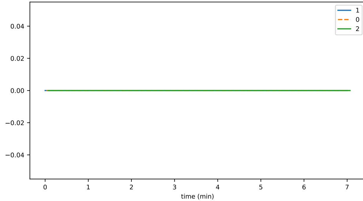
cryptoAddLiveHashThrottledTxns
