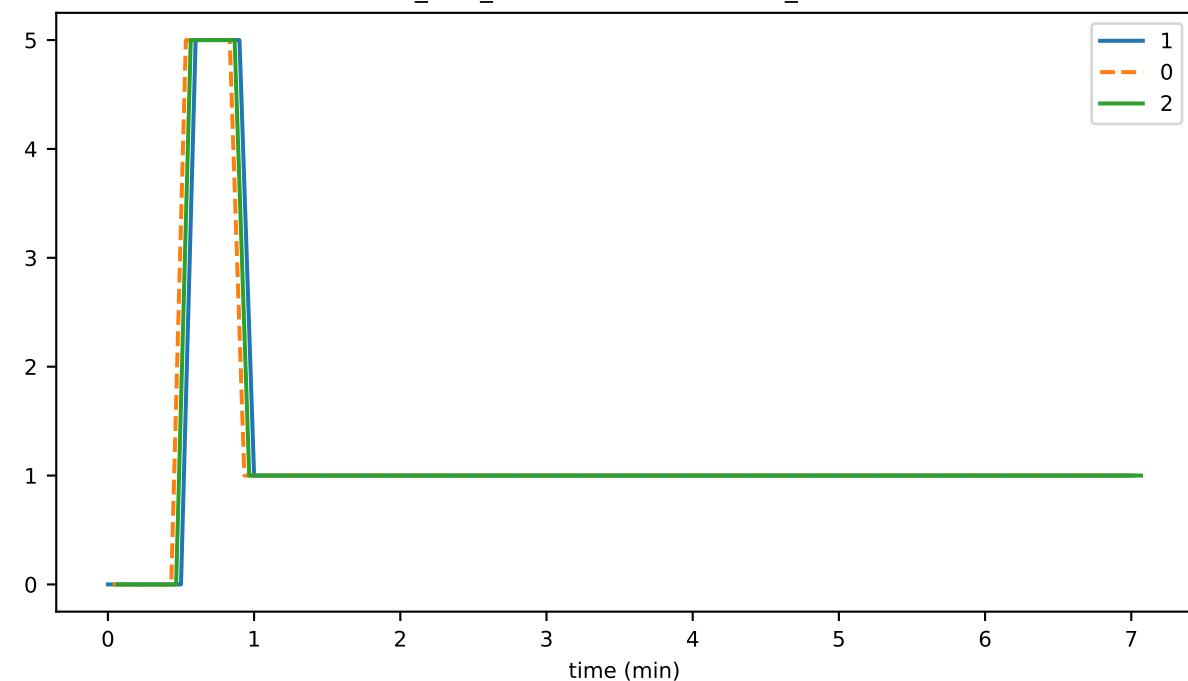
ds_files_leafKeysStoreFileSizeMb_state
