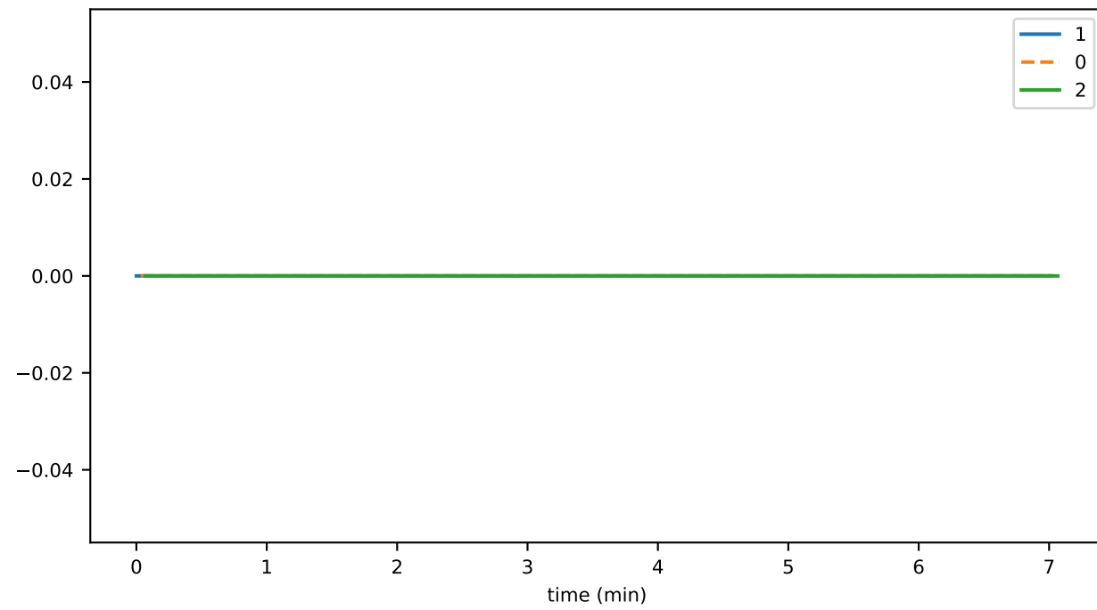
networkGetExecutionTimeDurationAvg
