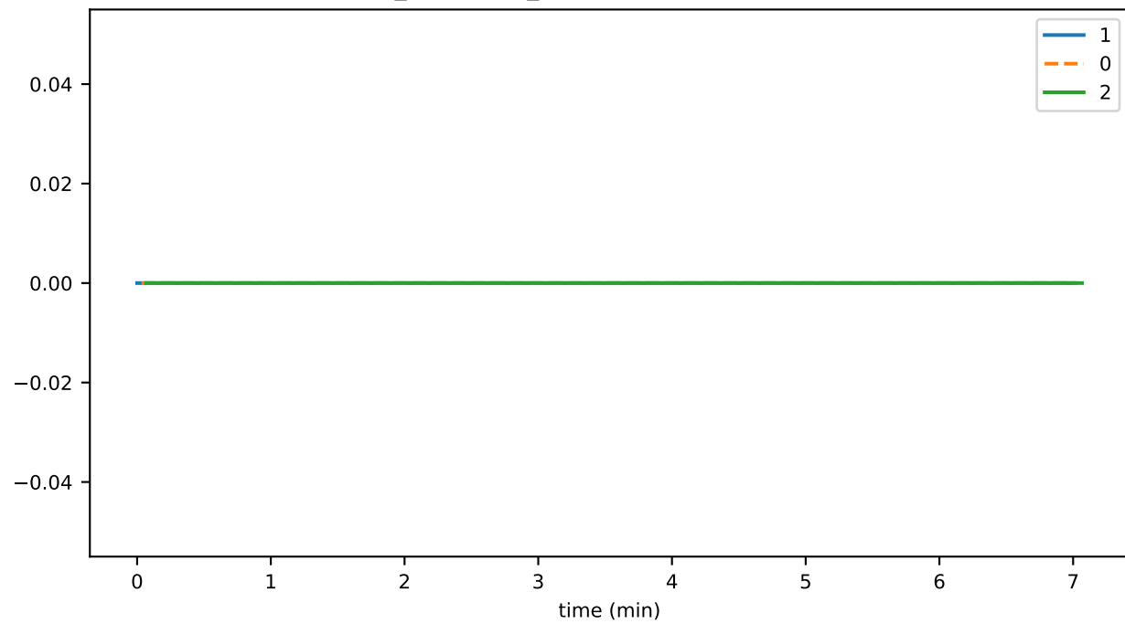
conn_connClose_transientEndStreamReceived
