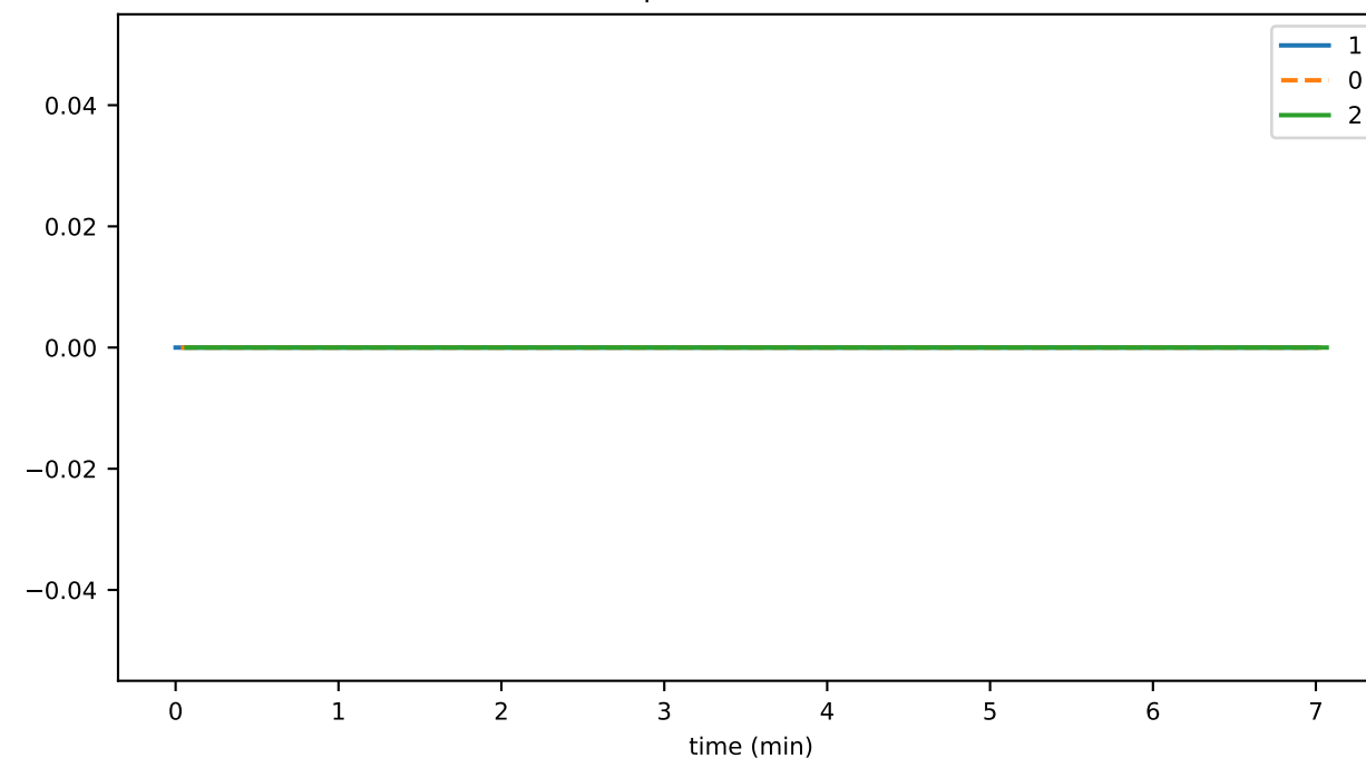
freezeDurationMax
