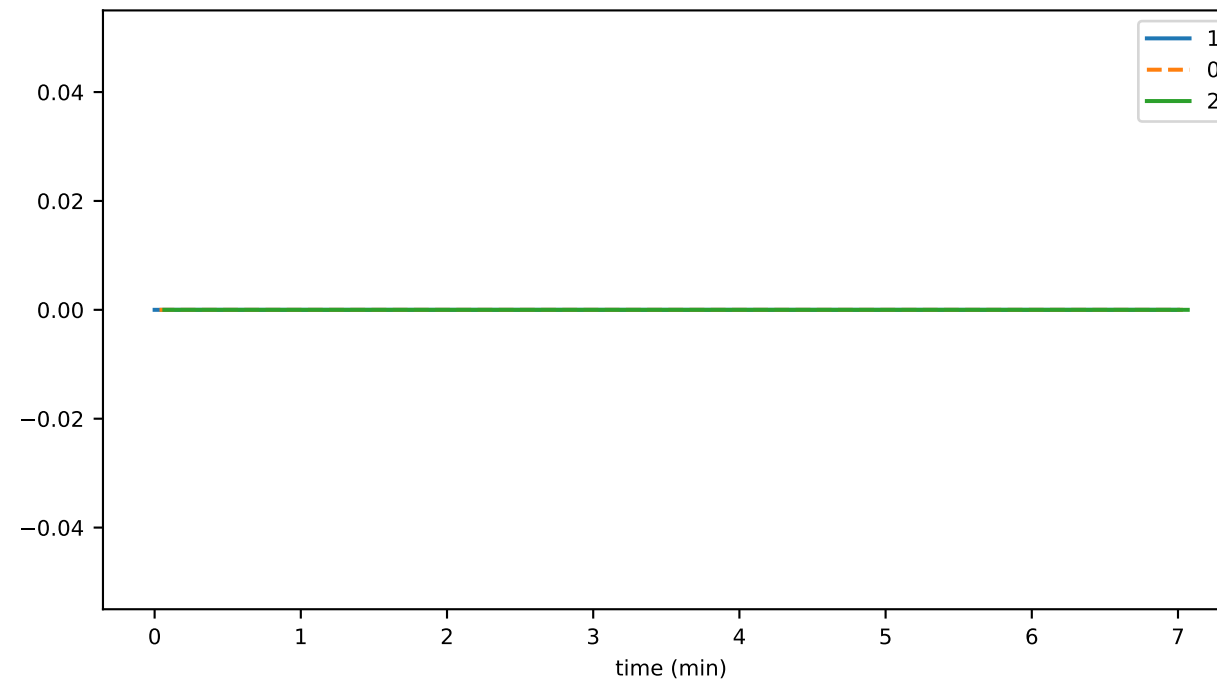
queriedAccountBalances
