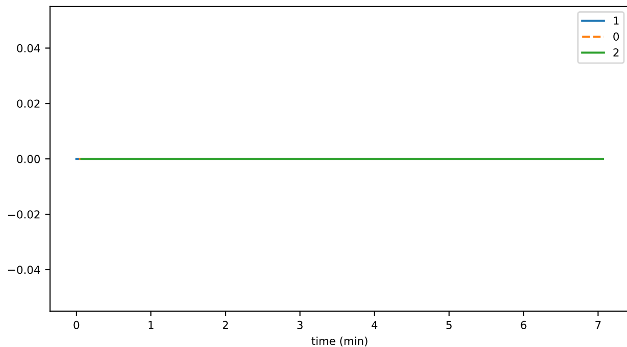
numEventsAddedUntilConsensusMAX
