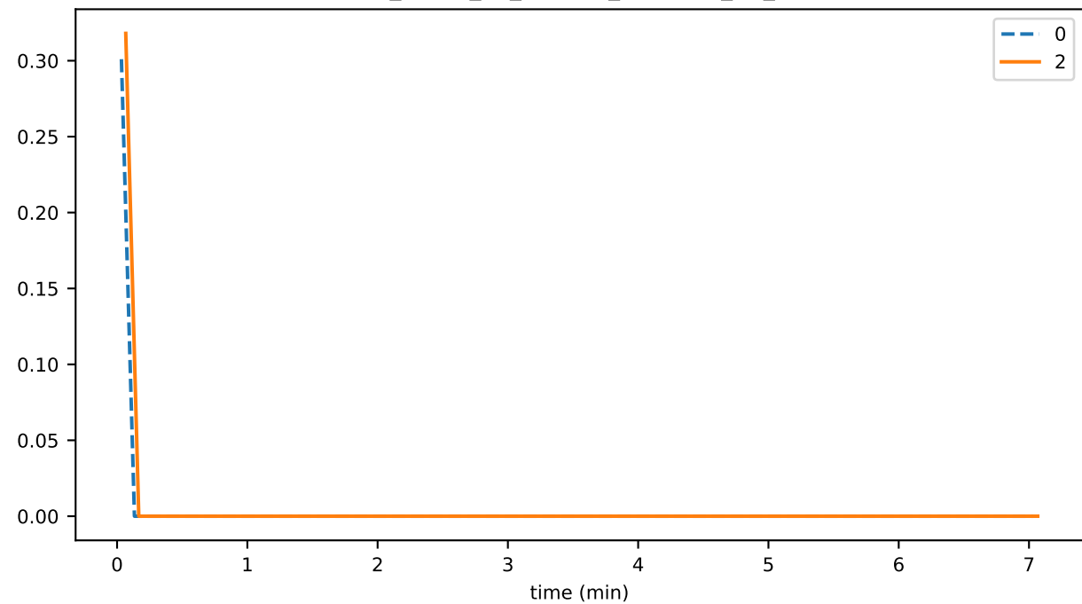
sync_phase_01_fraction_OUTSIDE_OF_RPC
