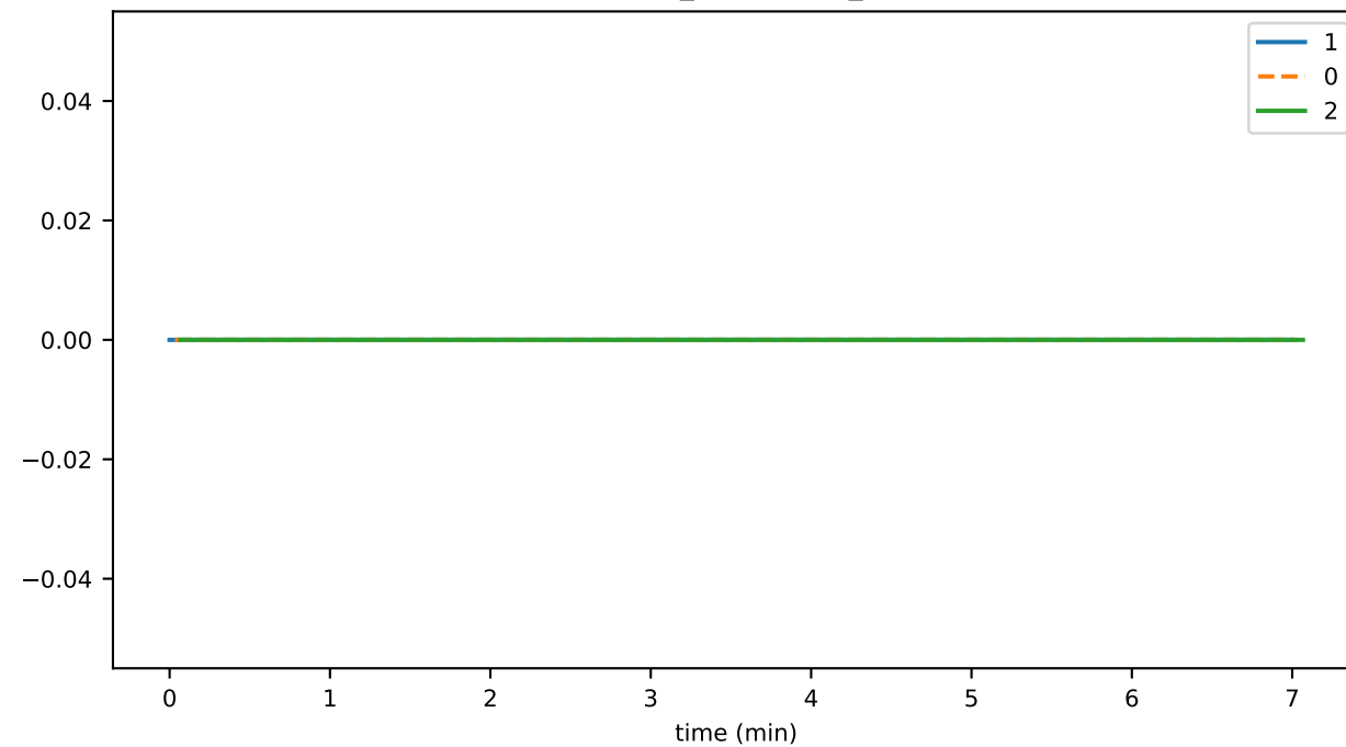
connSend_endStream_error
