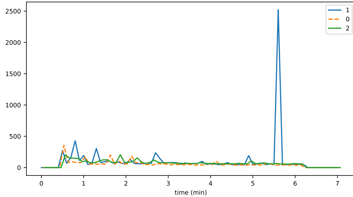
eventDelay_3_deduplication_storageMAX
