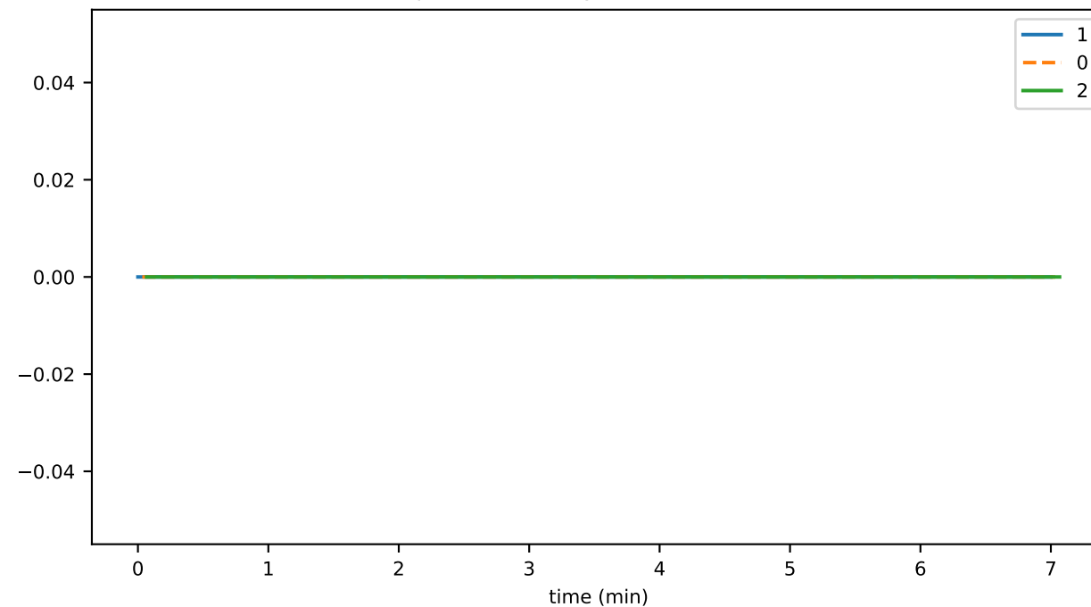
hapiCreationLimitsPercentUsed
