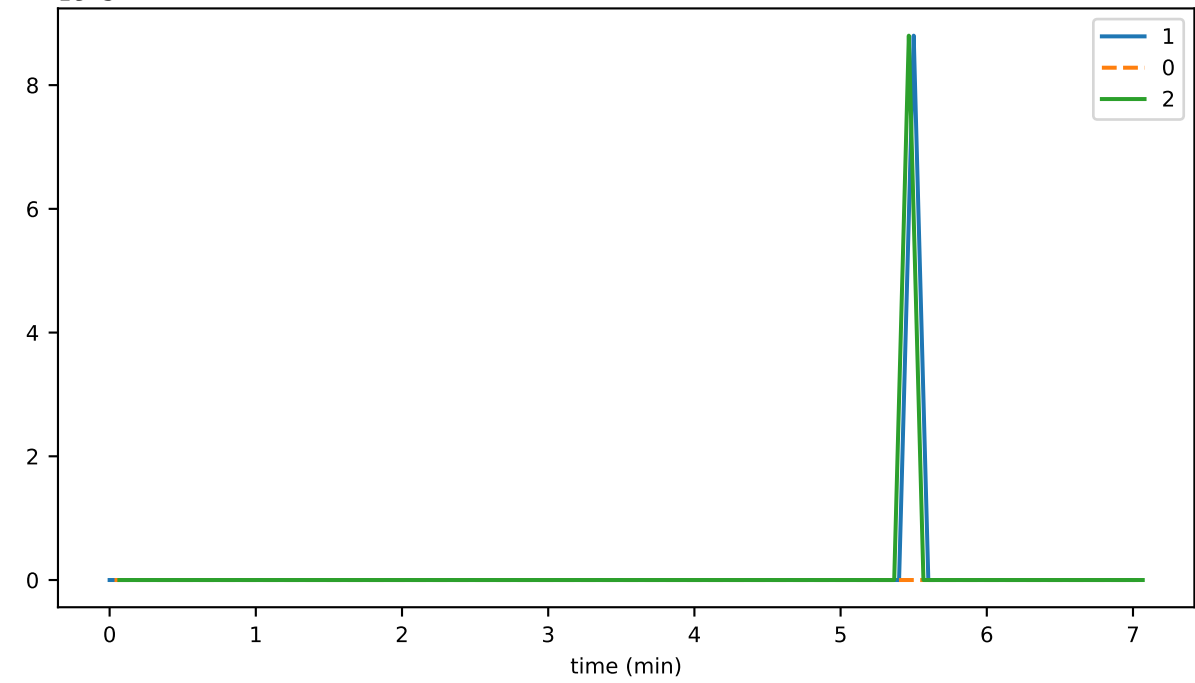
ds_compactions_level_3_leafKeysSavedSpaceMb_state
