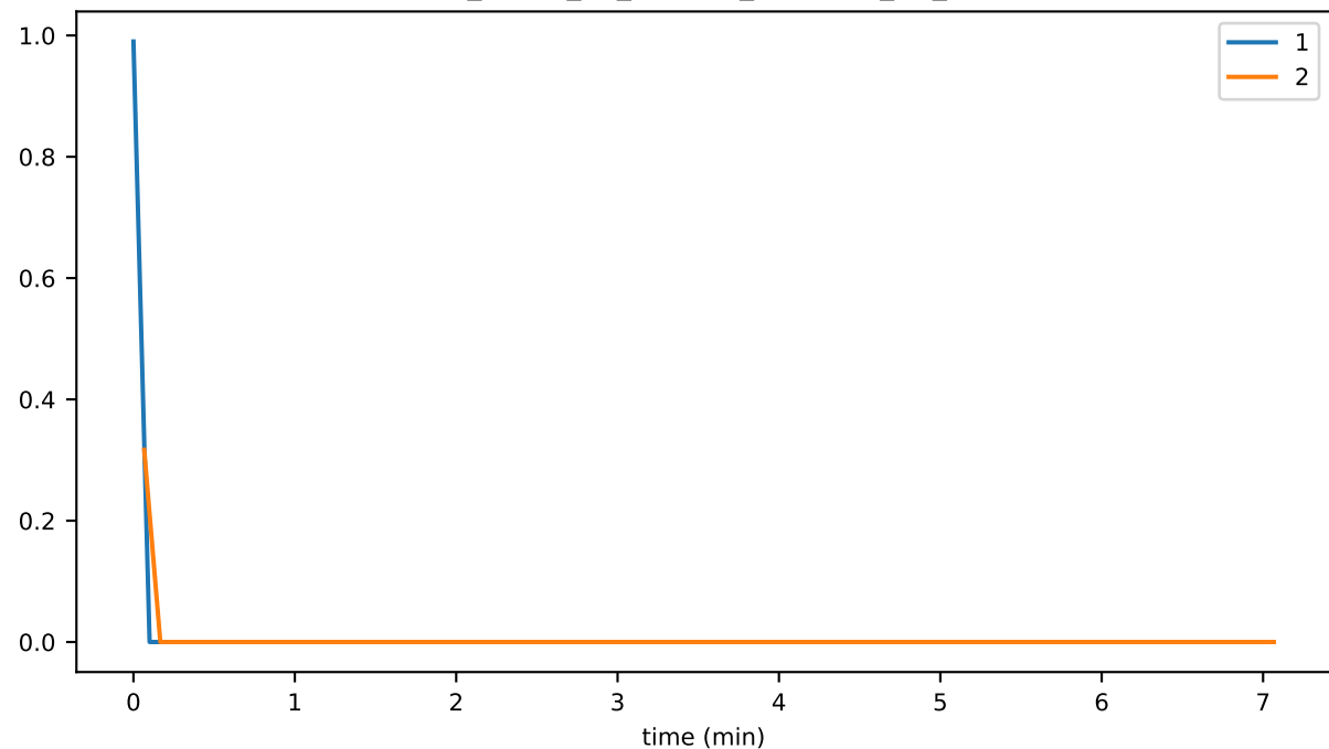
sync_phase_00_fraction_OUTSIDE_OF_RPC
