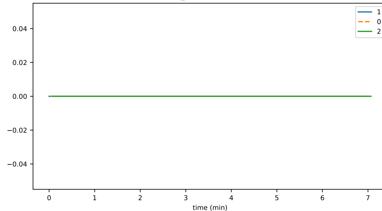
connSend_streamingBlockNumber
