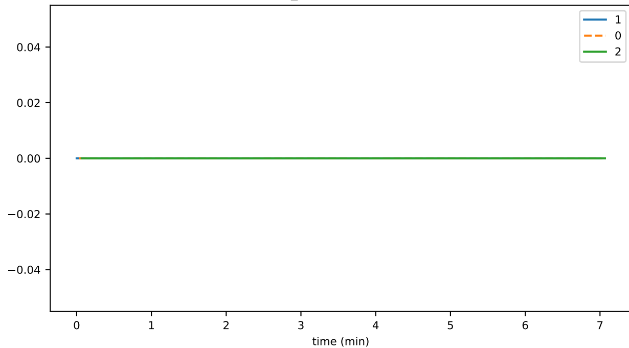
connRecv_latestBlockResendBlock
