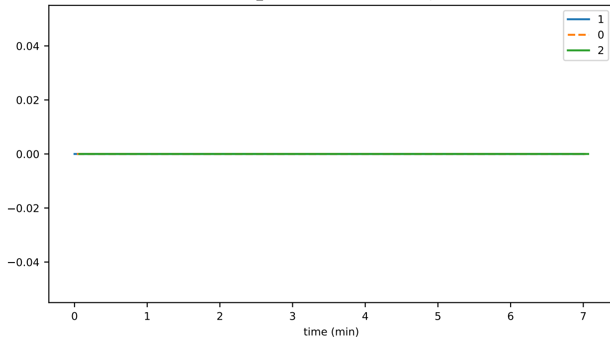
conn_connClose_blockNodeBehind
