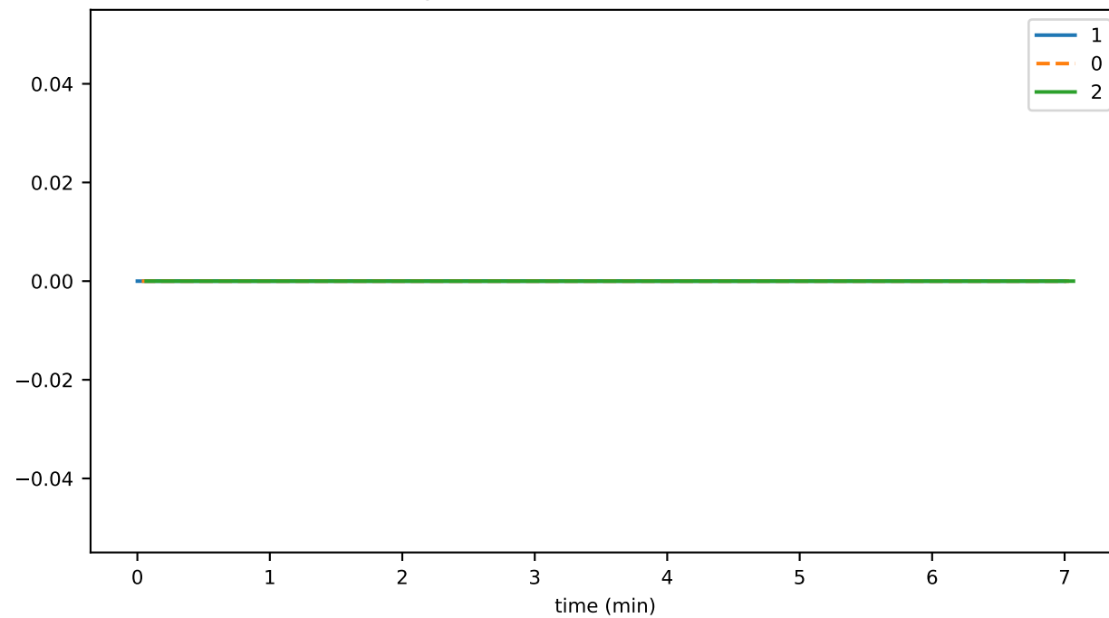
registeredNodeUpdateDurationMax
