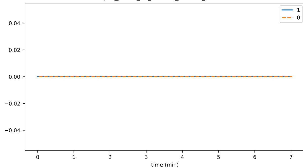
sync_phase_02_fraction_GOSSIP_HALTED
