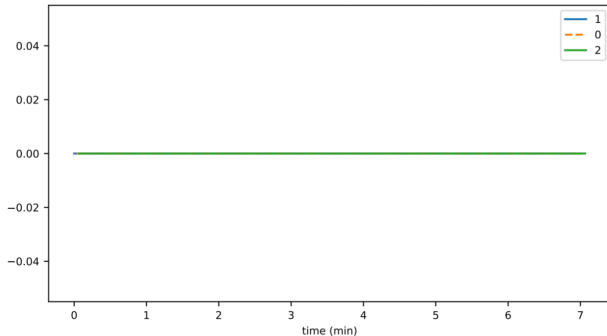
tokenCancelAirdropThrottledTxns
