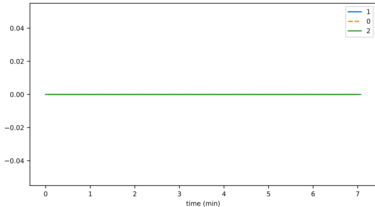
crsPublicationDurationAvg
