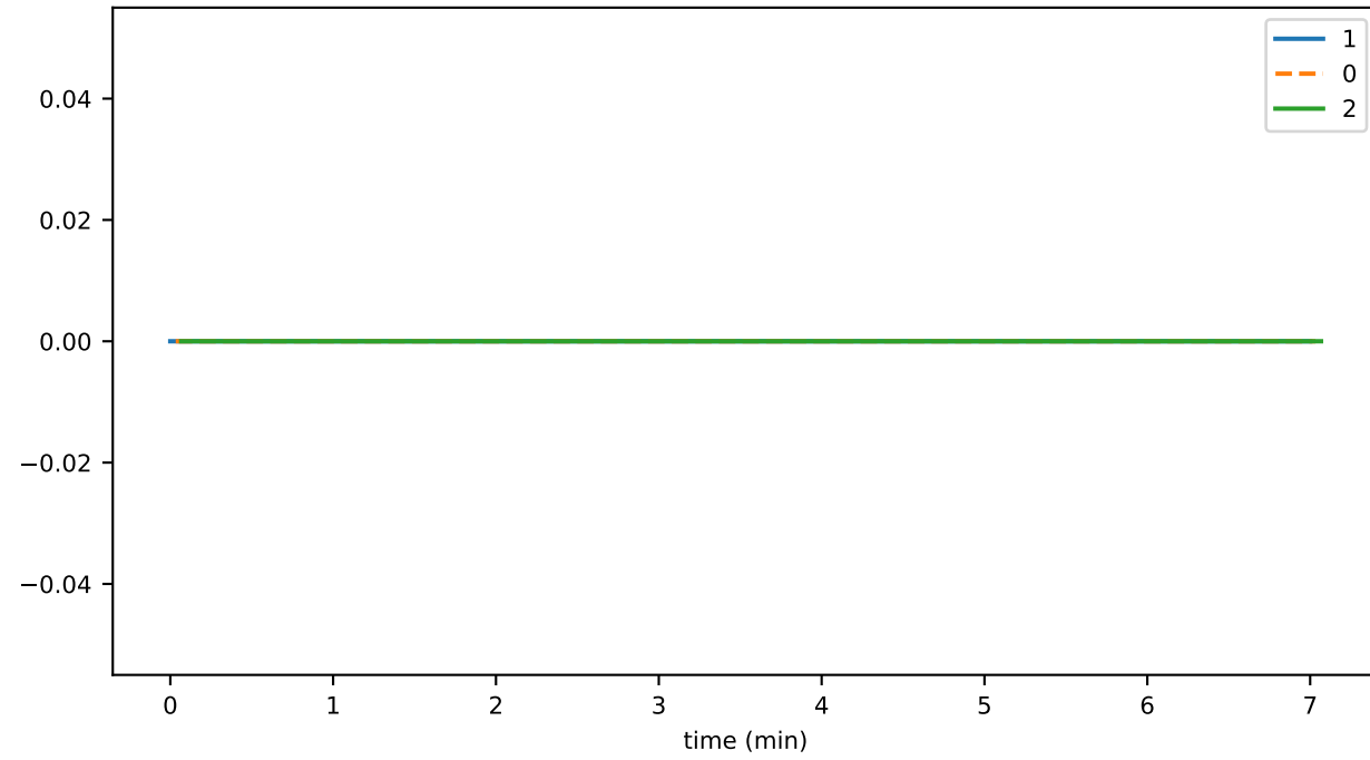
cryptoGetAccountBalanceDurationAvg
