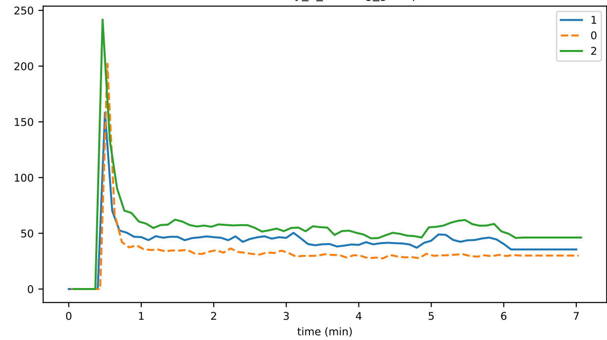
eventDelay_1_hashing_gossip
