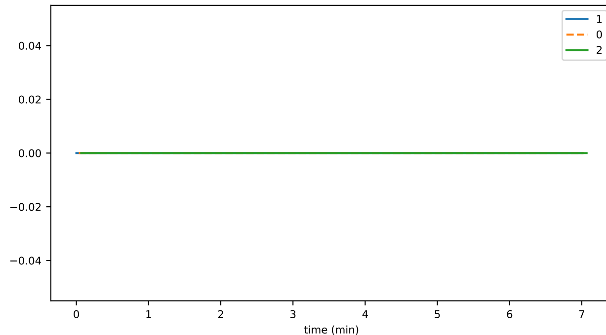
contractDeleteDurationAvg
