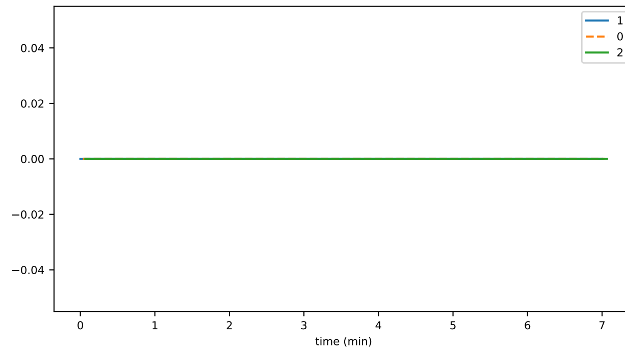
numIndirectProofs
