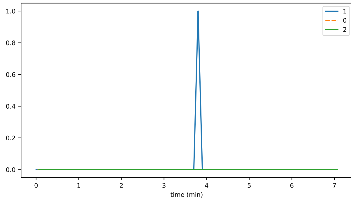
broadcastDisabledDueToOverload
