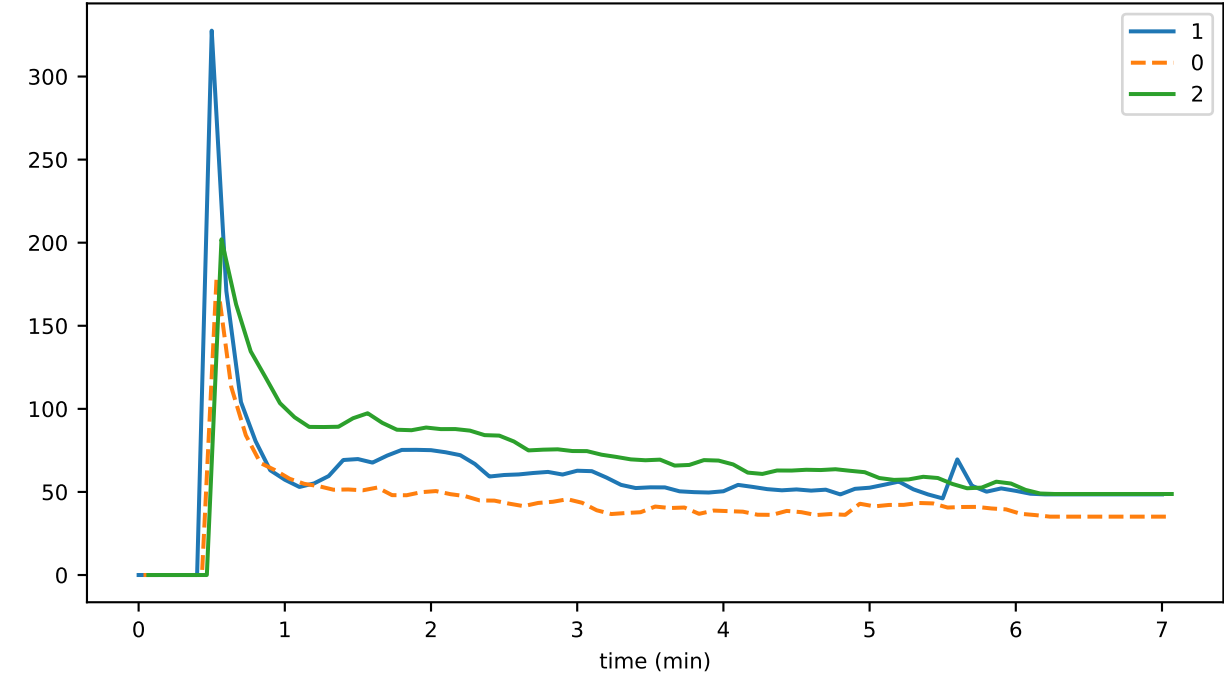
eventDelay_5_orphanBuffer_runtime
