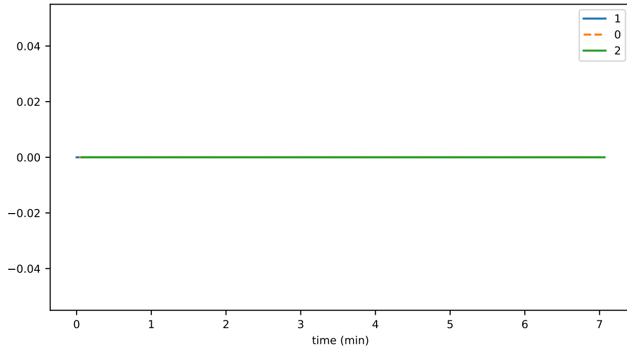
staleEvents
