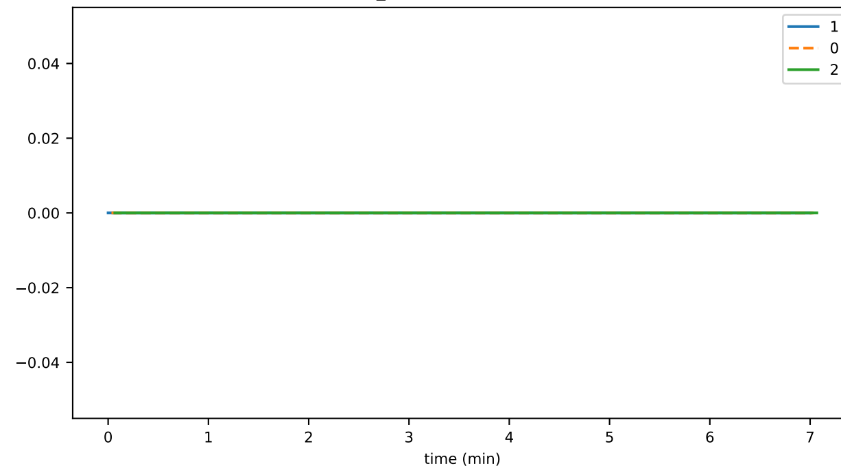
conn_blockClosedToAckLatency
