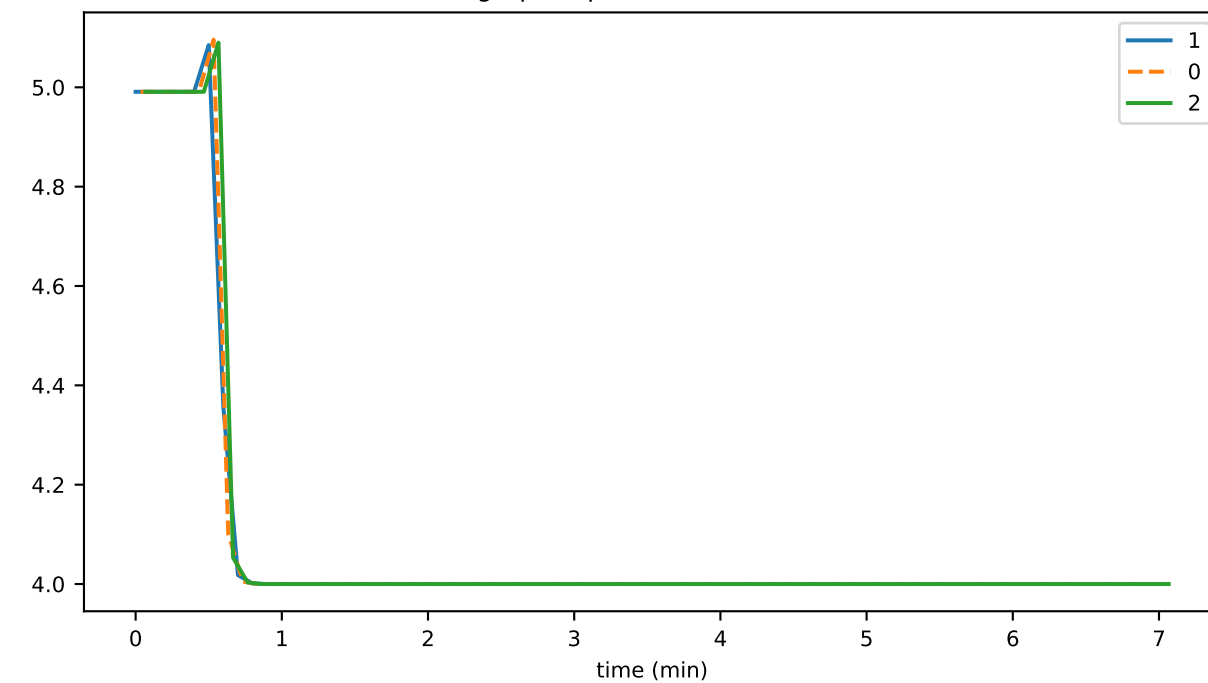
graphDepthUntilConsensus
