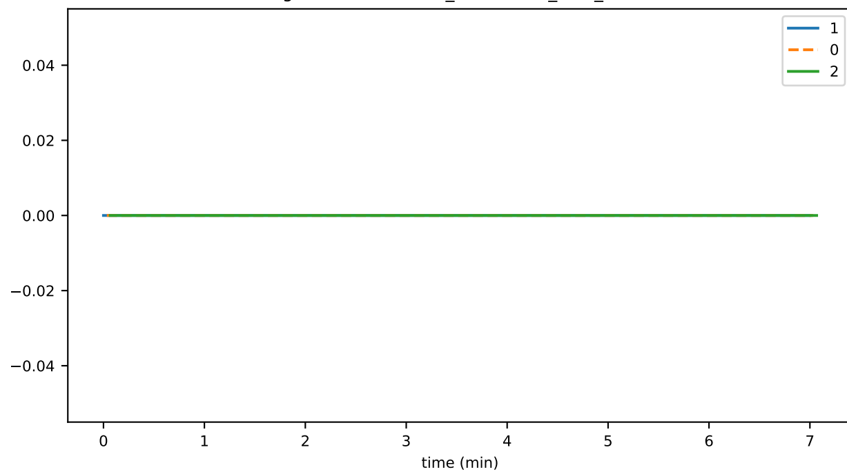
SigQuDepth
