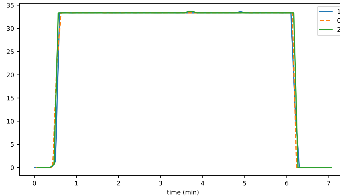
broadcastEventsReceived
