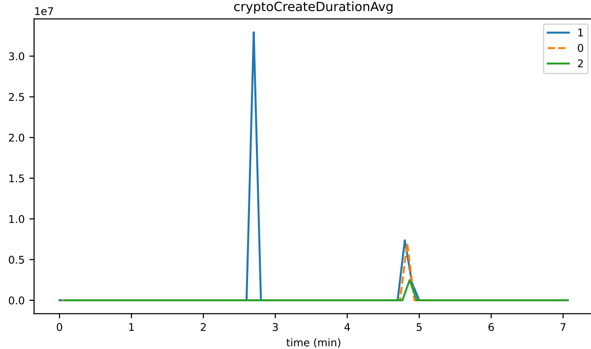
cryptoCreateDurationAvg
