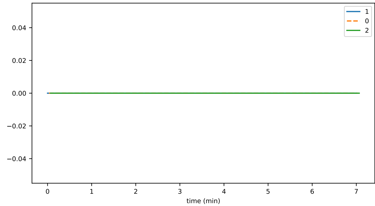
historyProofTransR2ToFailCnt
