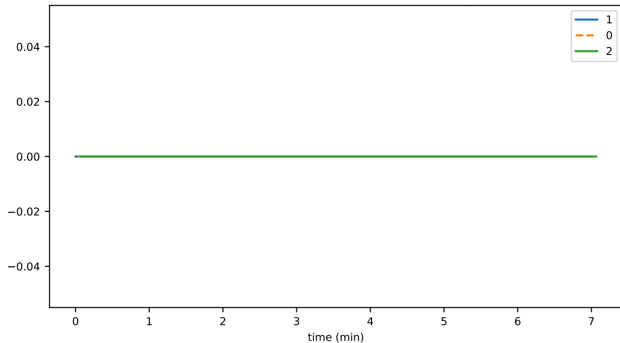
tokenDissociateFromAccountThrottledTxns
