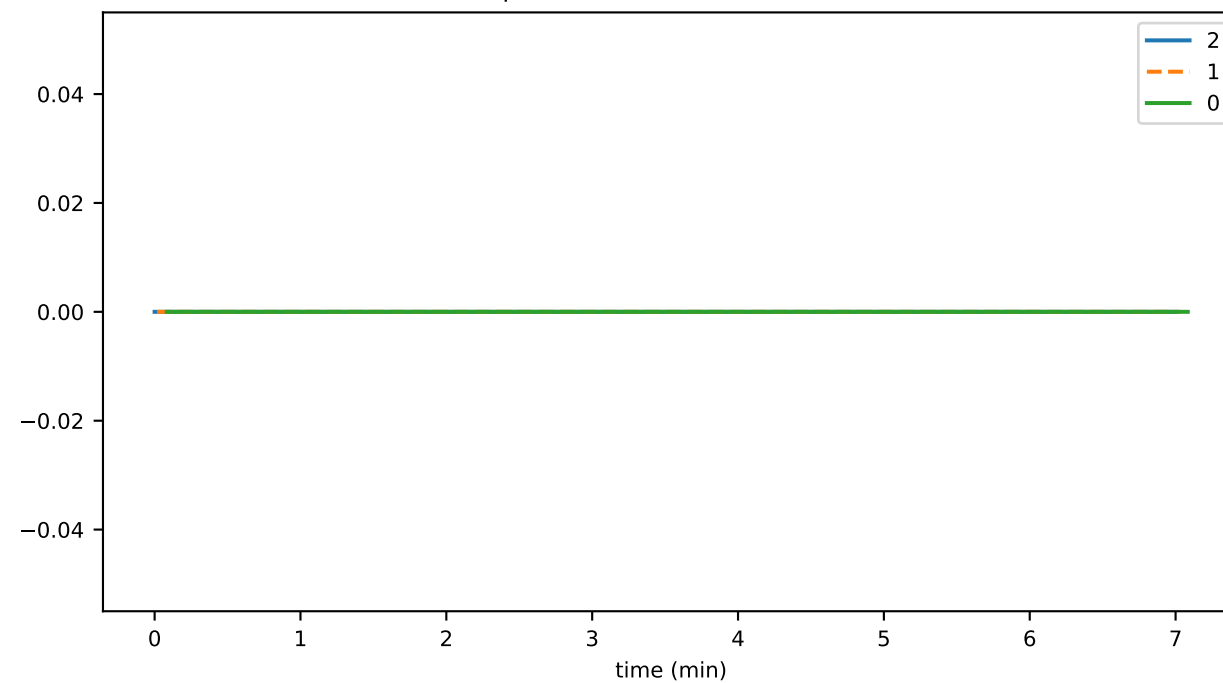
hapiCreationLimitsPercentUsed
