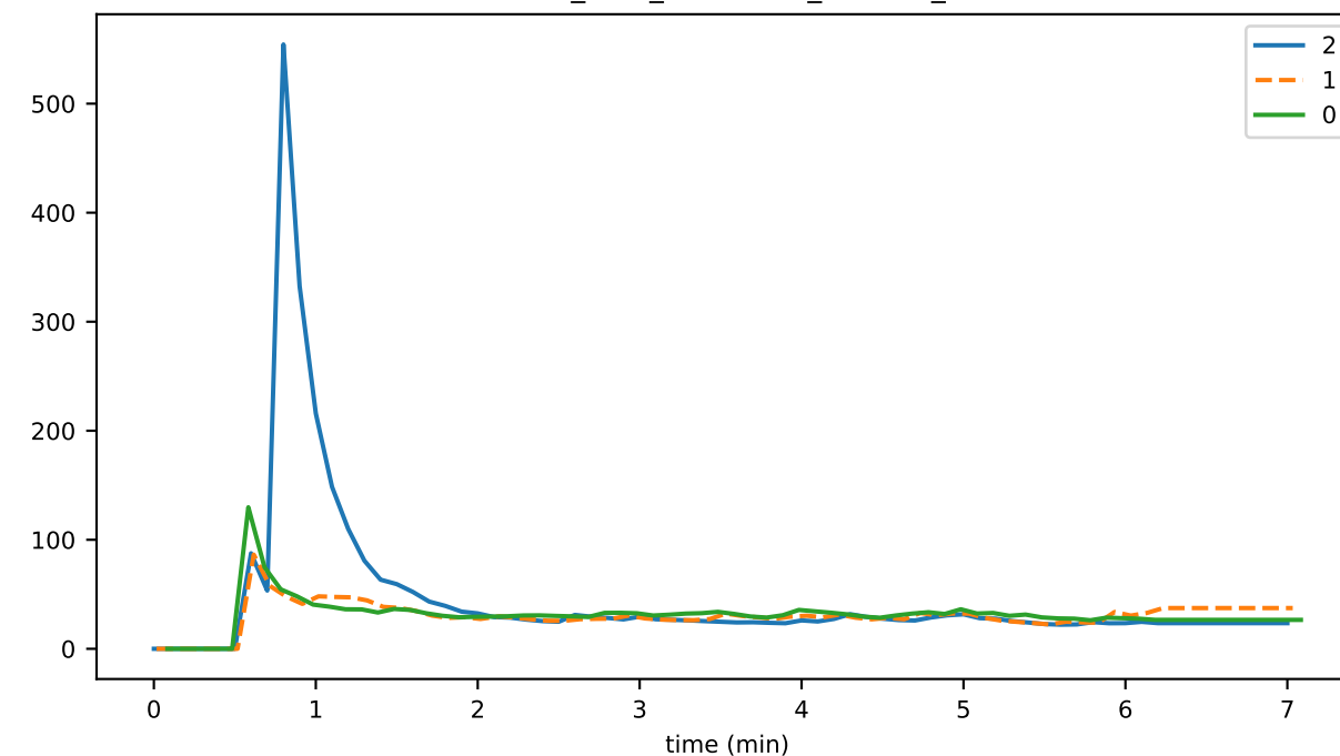
consensus_time_HANDLING_CONSENSUS_ROUND
