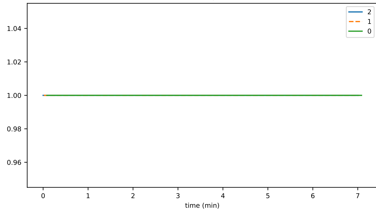
hintsKeyPublicationDurationAvg
