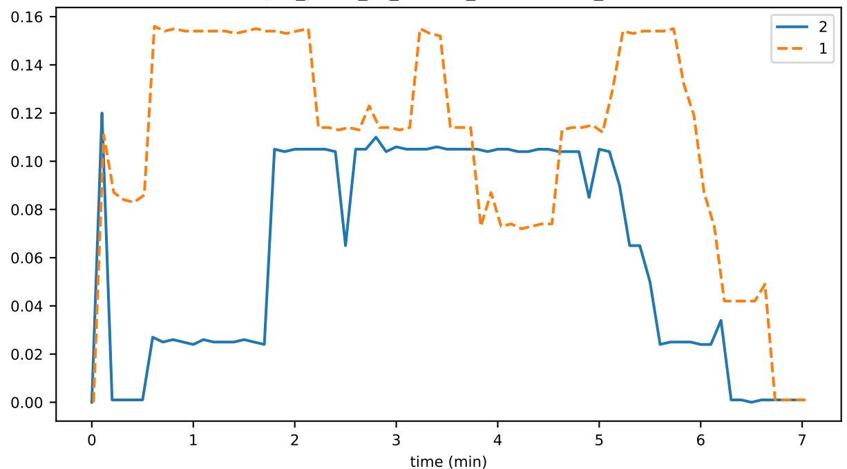
sync_phase_00_fraction_GOSSIP_HALTED
