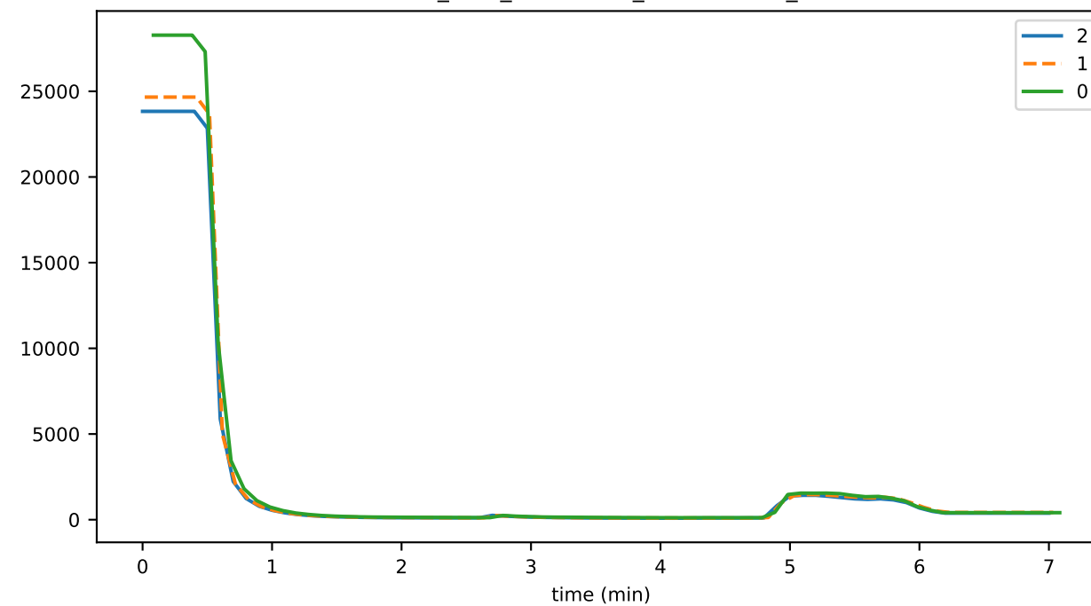
consensus_time_HANDLING_CONSENSUS_ROUND
