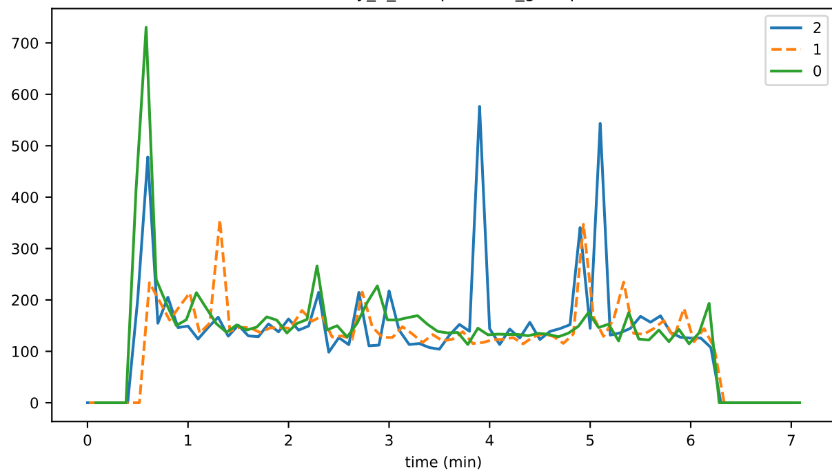
eventDelay_3_deduplication_gossipMAX
