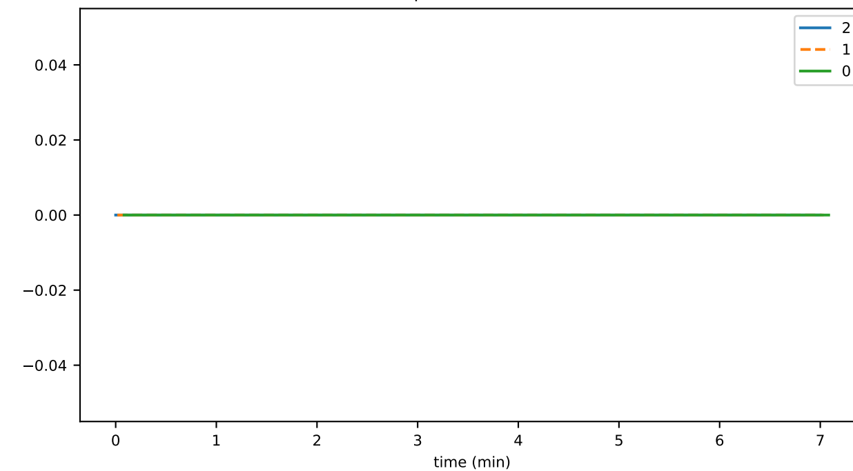
orphanBufferSize
