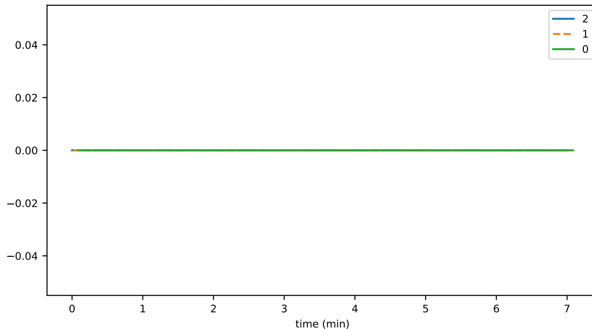
cryptoCreateDurationMax
