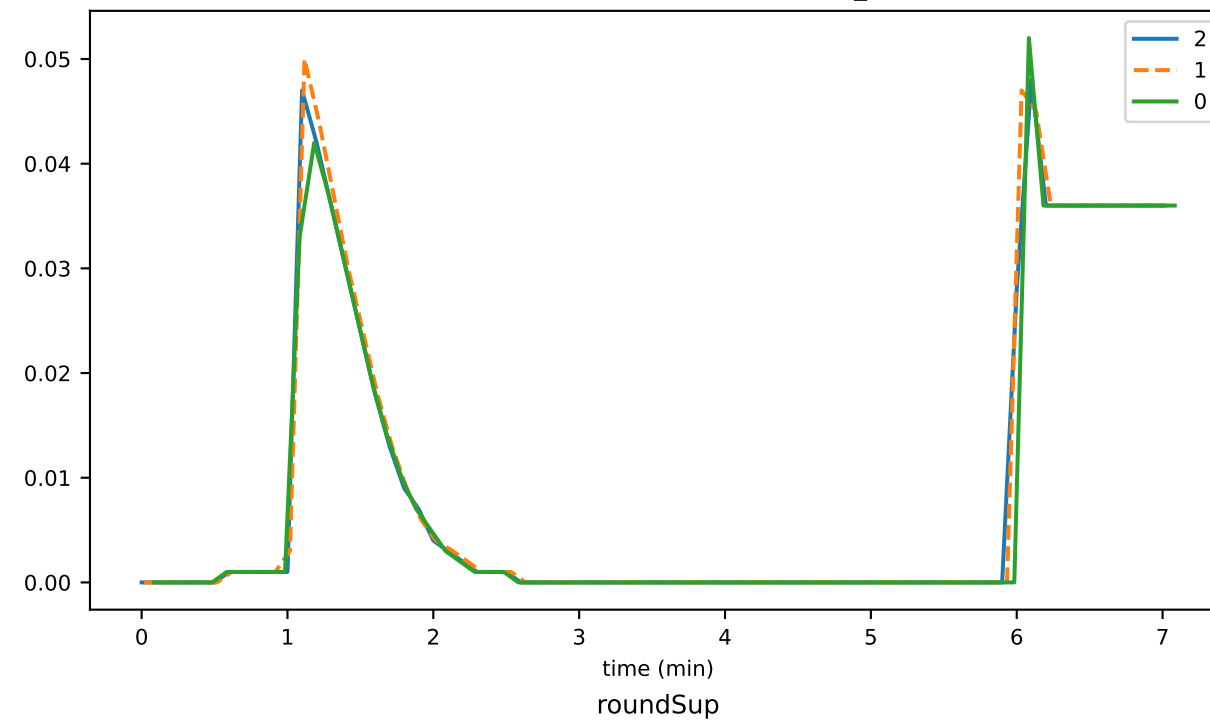
roundsSinceLastConsensusEvent_1
