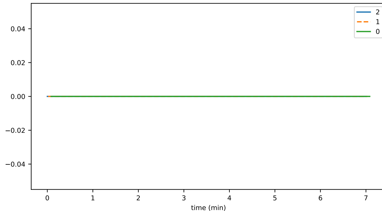
contractDeleteDurationAvg
