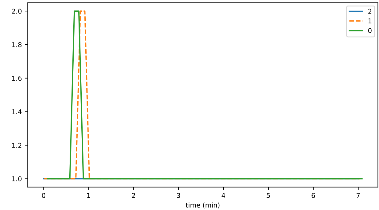
createTransactionRecordDurationAvg
