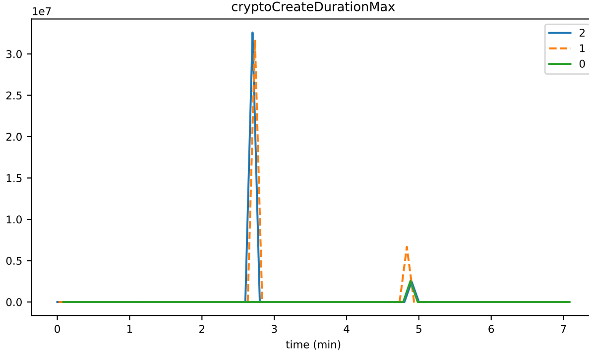
cryptoCreateDurationMax
