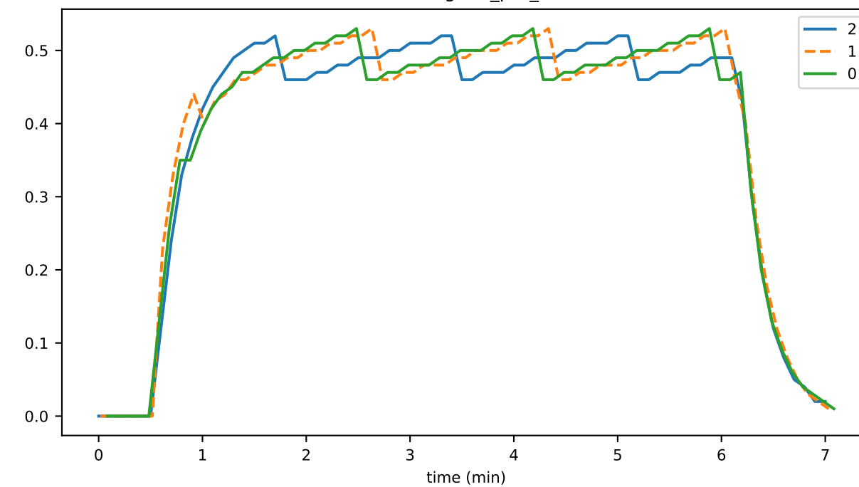
staleTransactions
