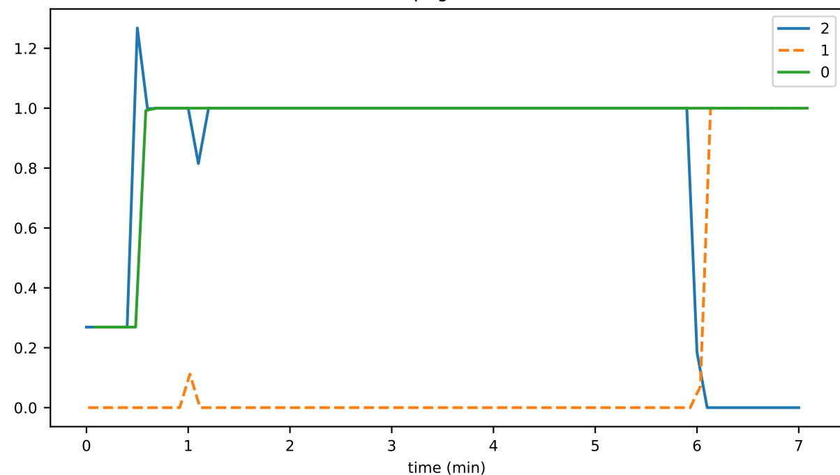
OrphanBuffer_unhandled_task_count
