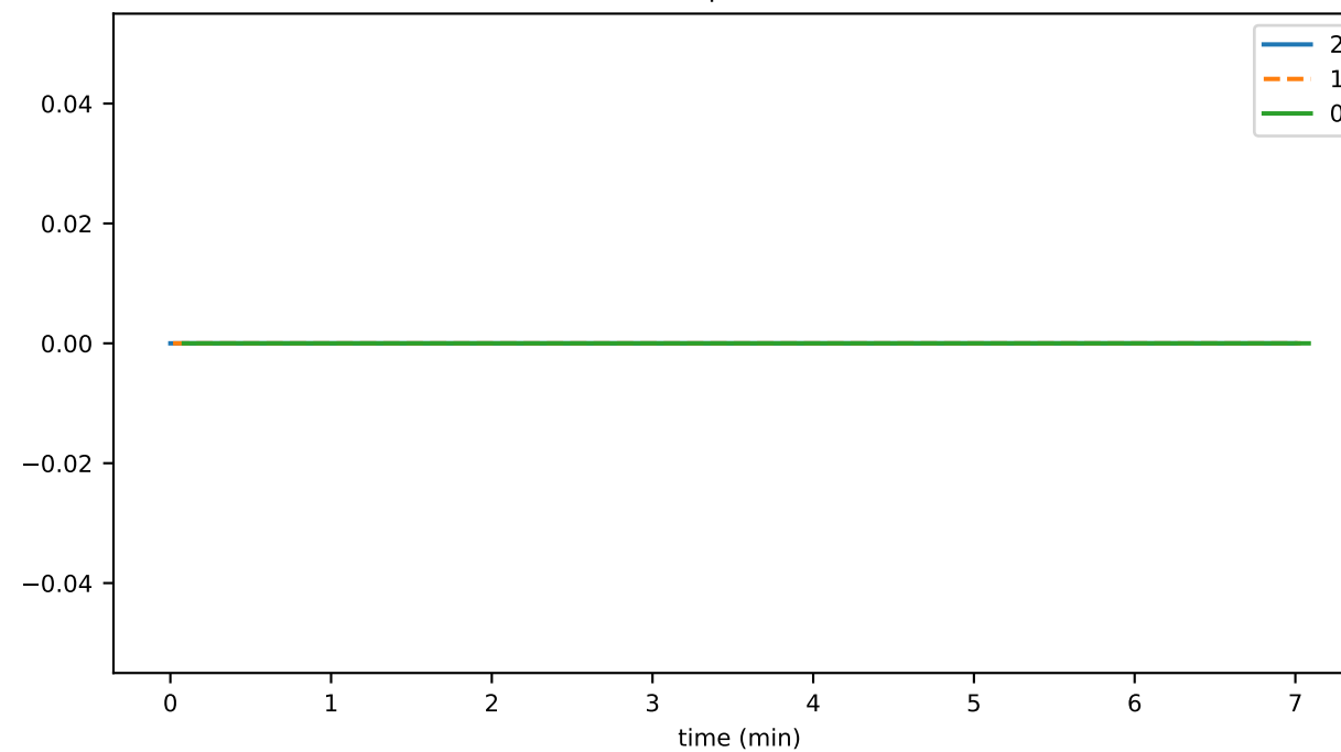
consensusGetTopicInfoThrottledTxns
