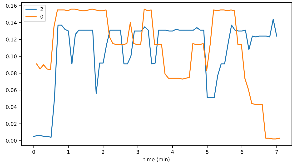
sync_phase_01_fraction_IDLE
