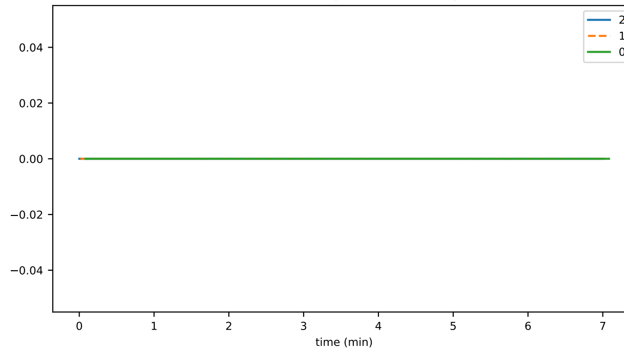
consensusGetTopicInfoThrottledTxns
