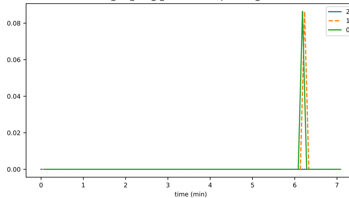
ds_files_level_3_leavesFileSizeByLevelMb_state
