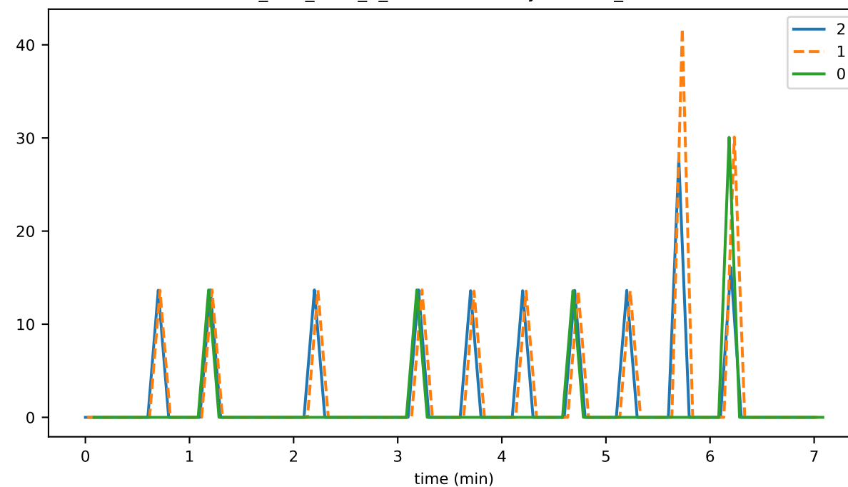
ds_files_level_2_leafKeysFileSizeByLevelMb_state
