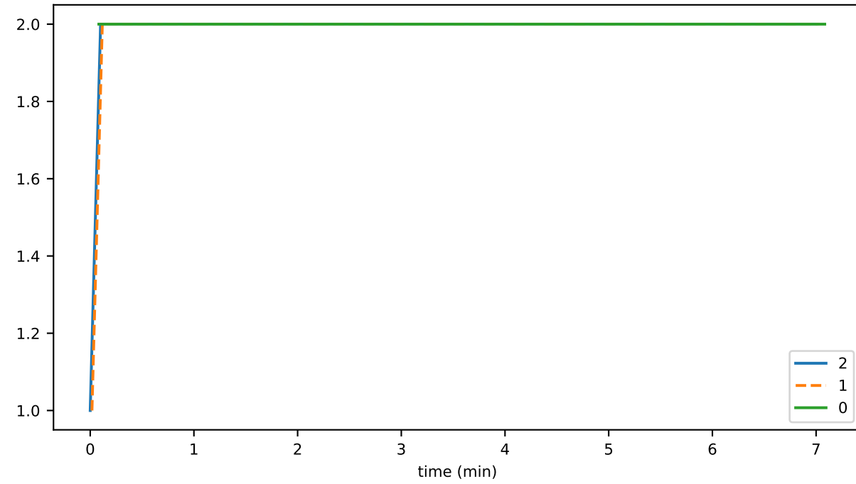
scheduleCreateDurationMax
