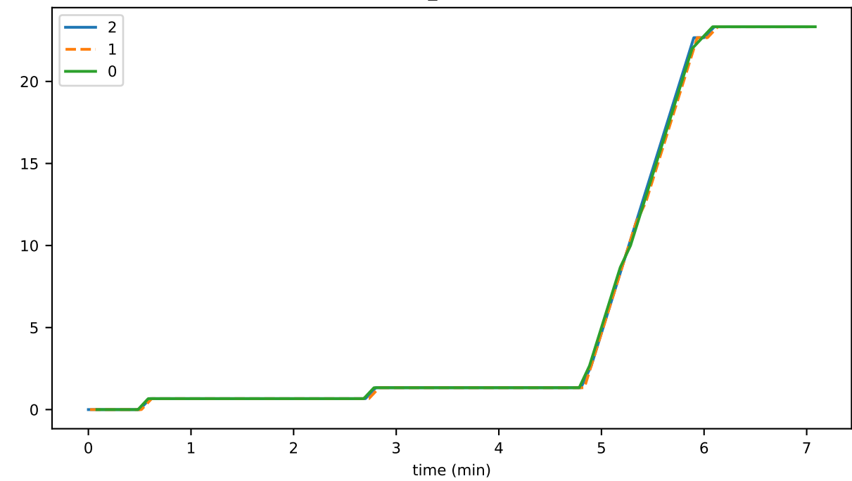
bufferedTransactions
