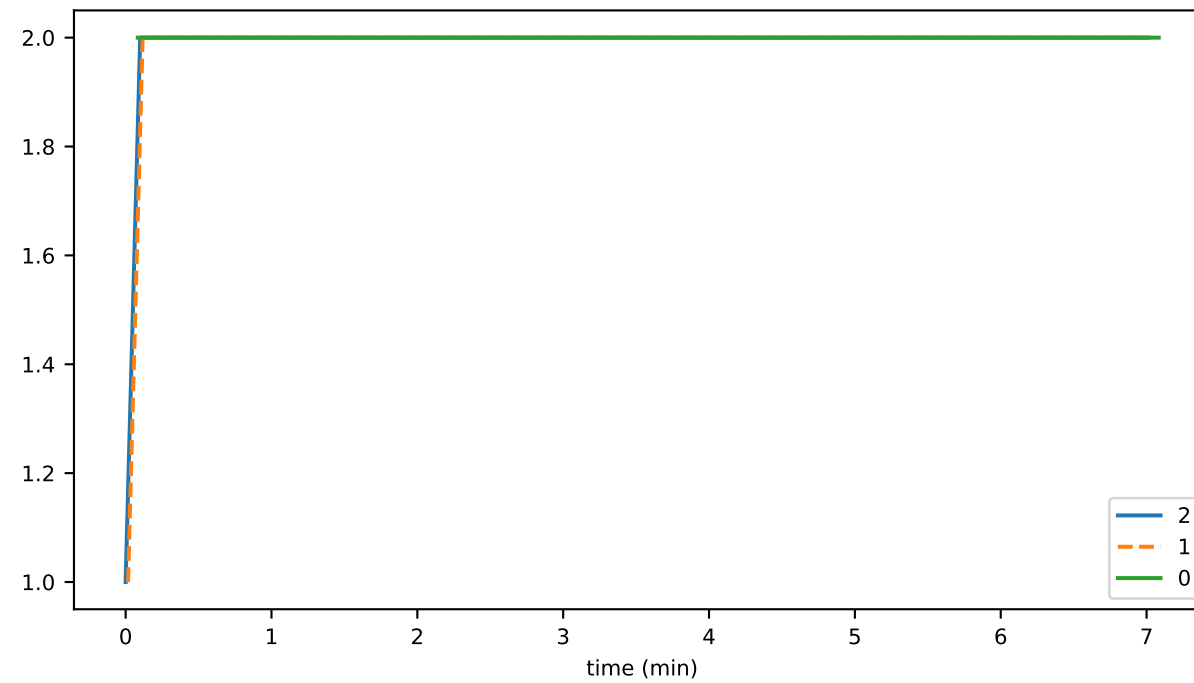
syncPermitsUtilized
