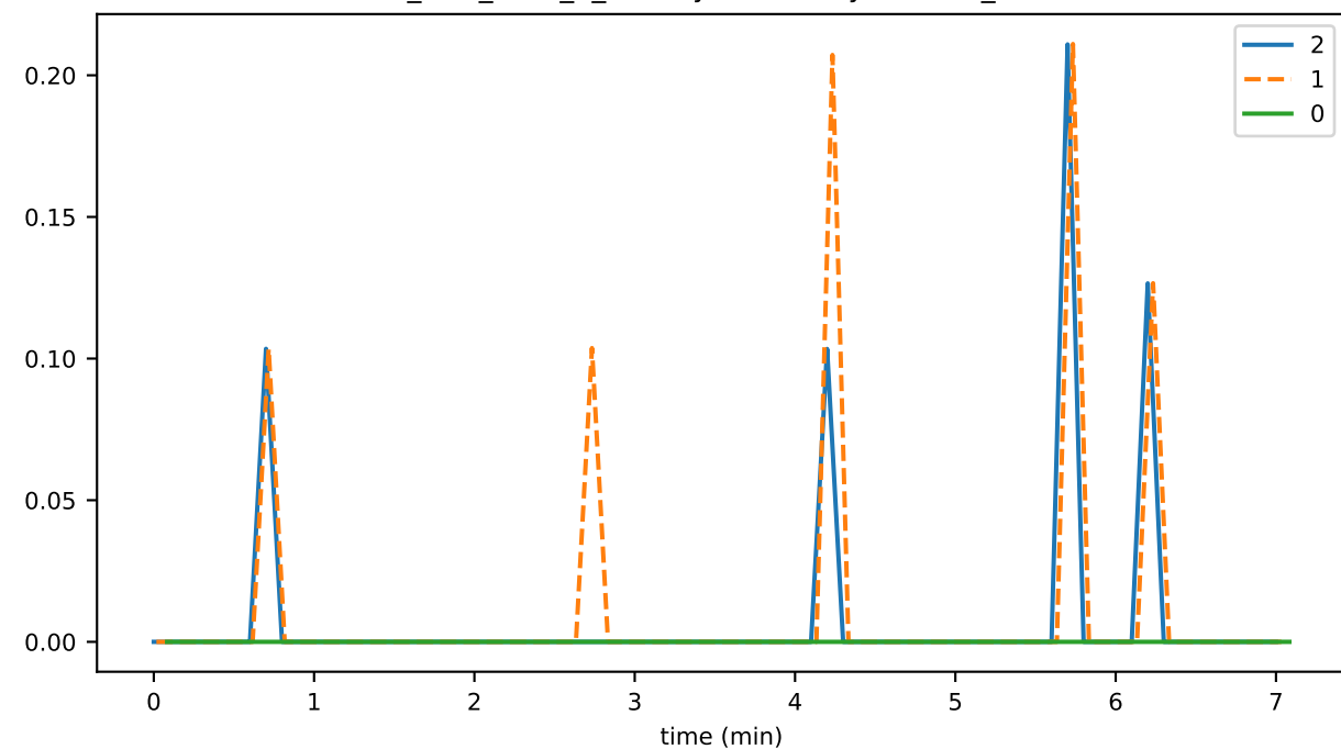
ds_files_level_2_hashesFileSizeByLevelMb_state
