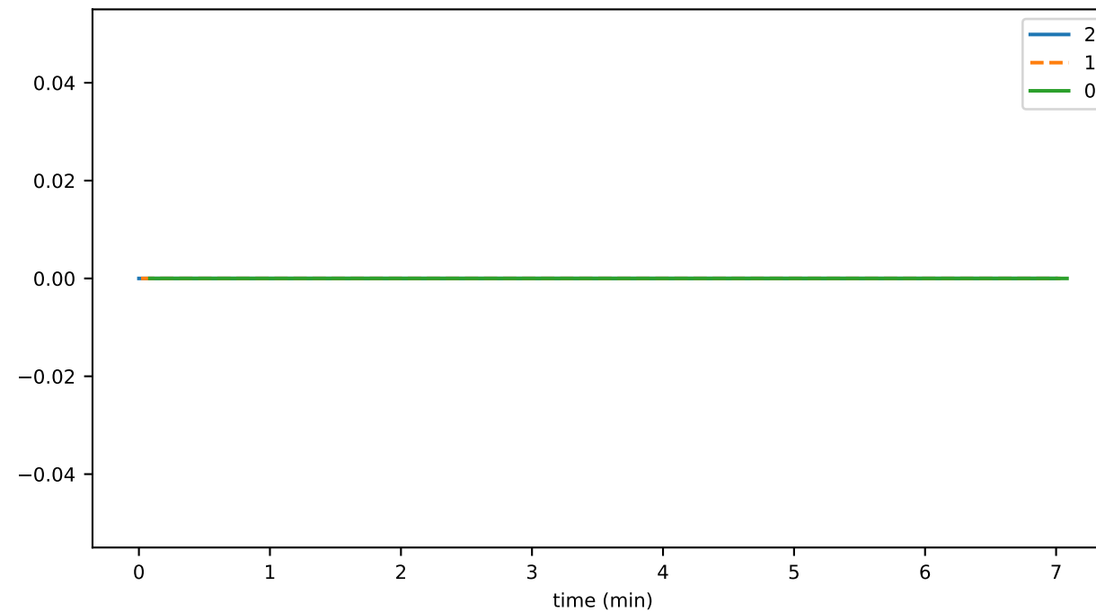
hintsKeyPublicationDurationMax
