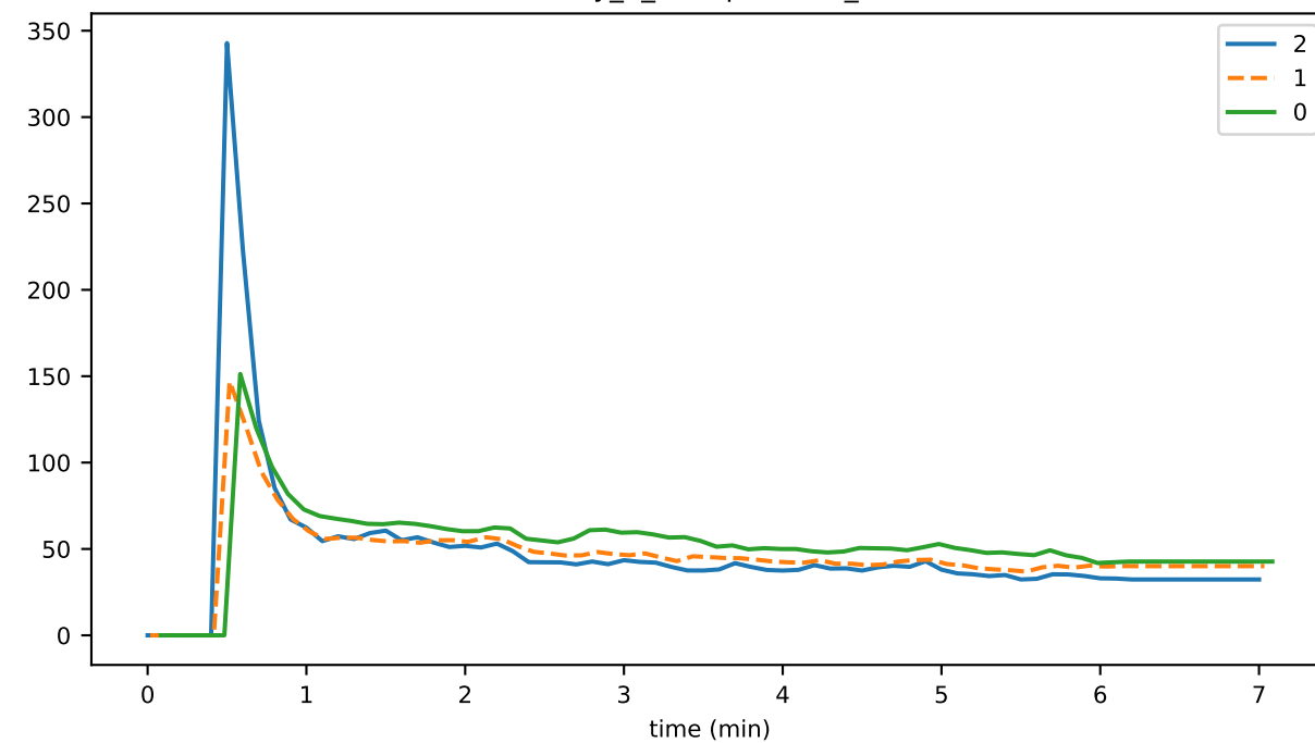
eventDelay_3_deduplication_runtime
