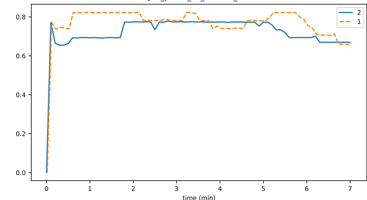
sync_phase_00_fraction_IDLE
