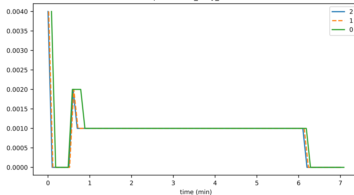
orphanBufferSize
