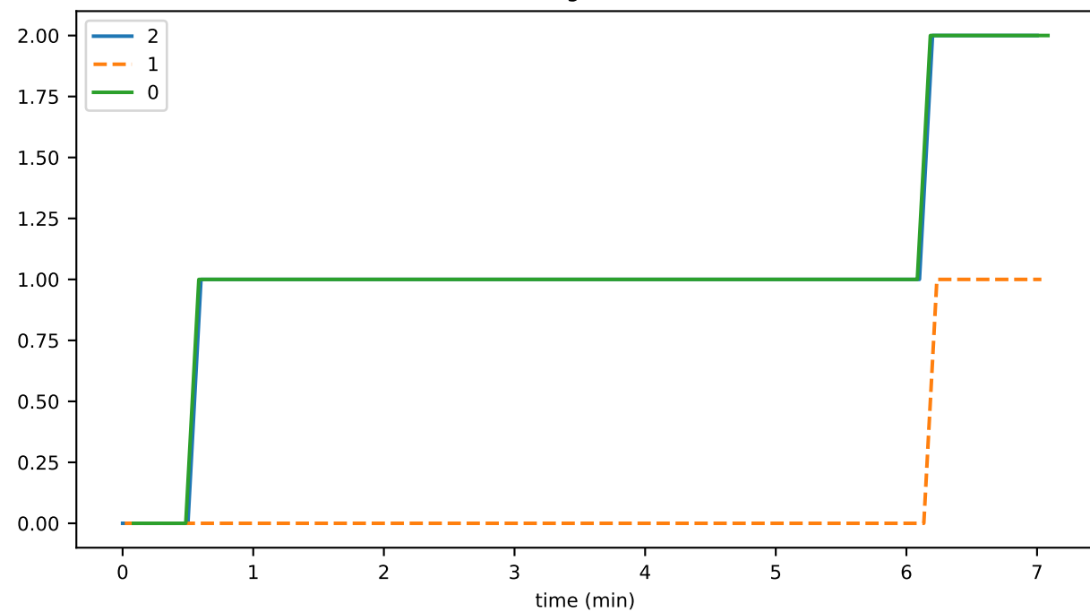
totalNeverSignedDiskStates
