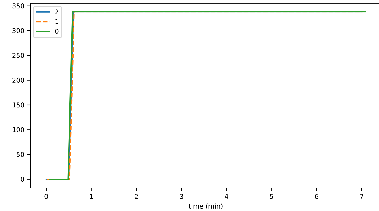
bufferedPriorityTransactions
