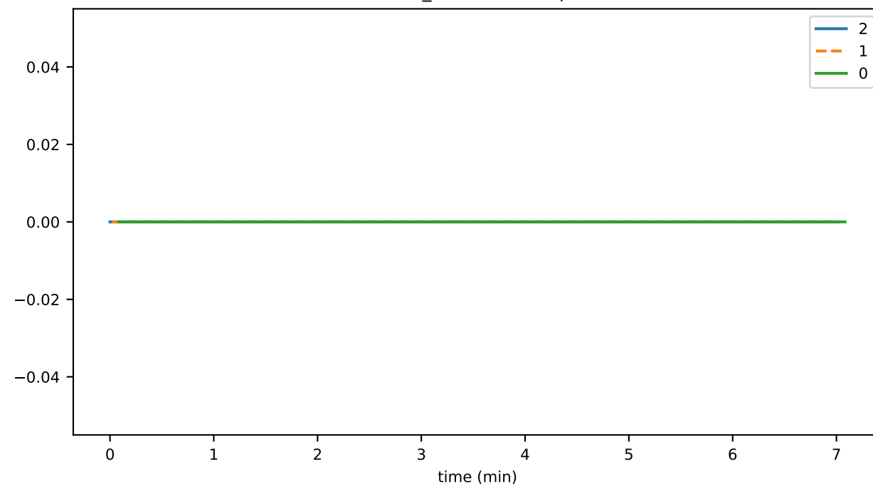
connRecv_latestBlockSkipBlock
