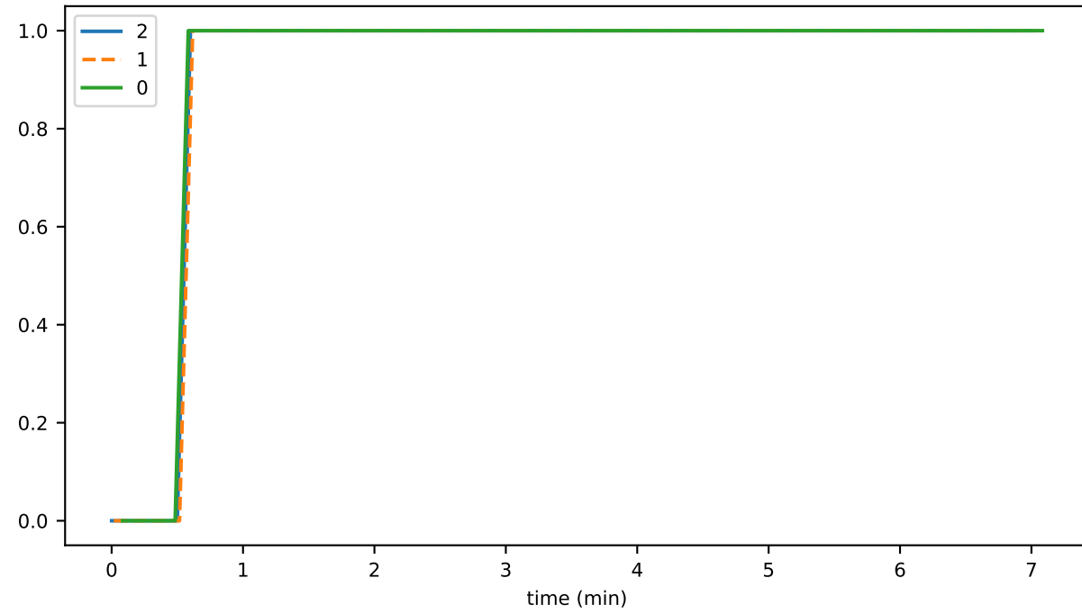
conn_activeConnlp
