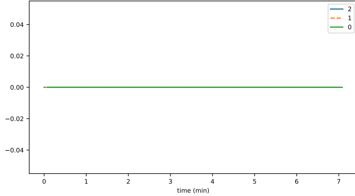
conn_activeConnlp
