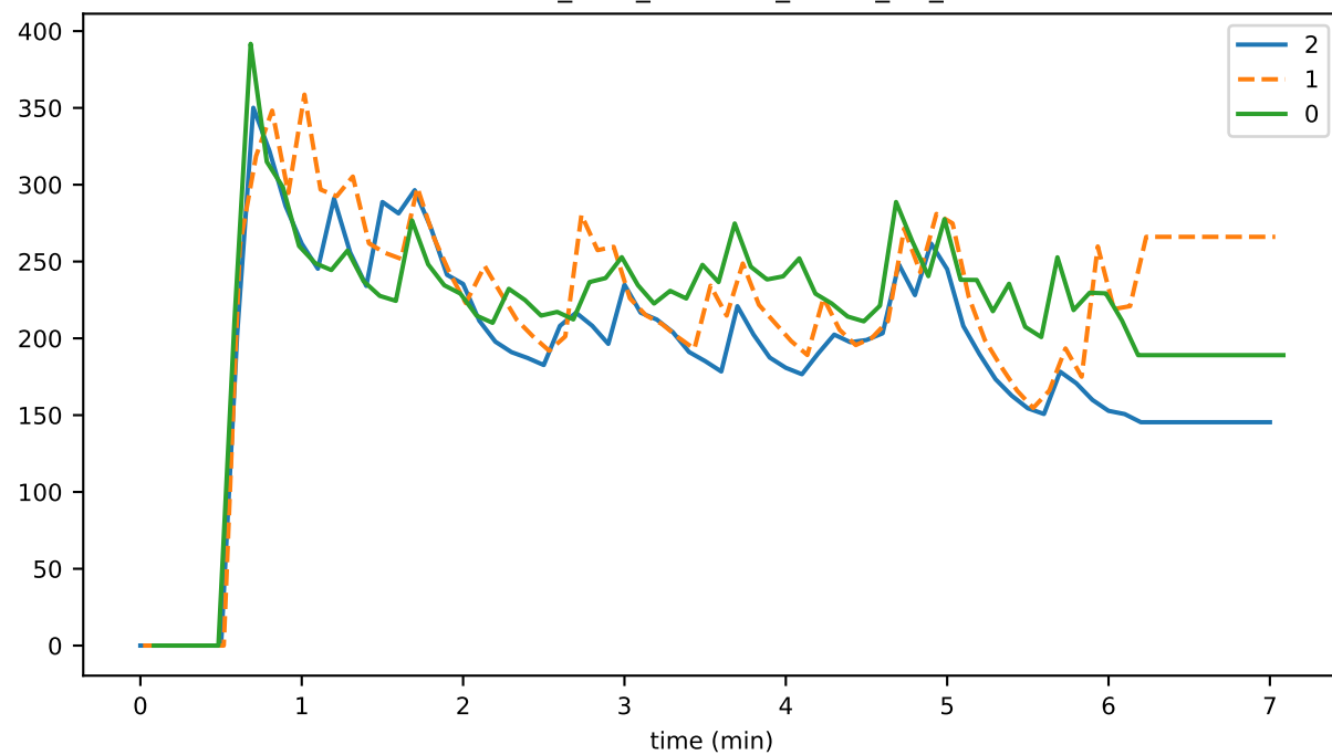
consensus_time_GETTING_STATE_TO_SIGN
