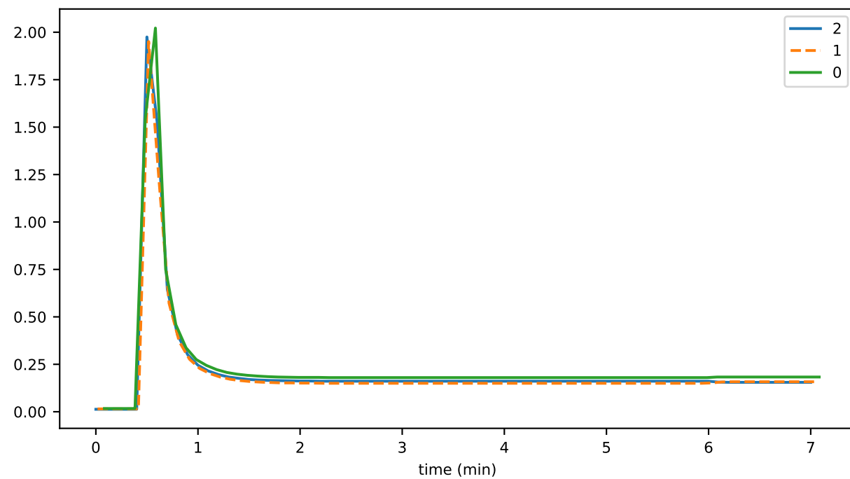
secR2nR
