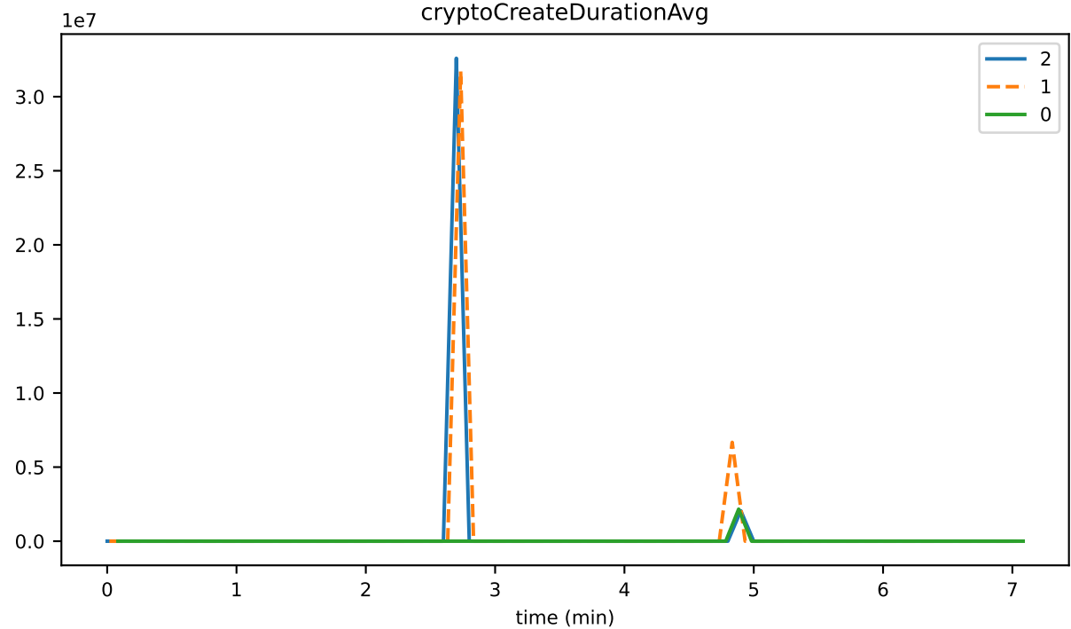
cryptoCreateDurationAvg
