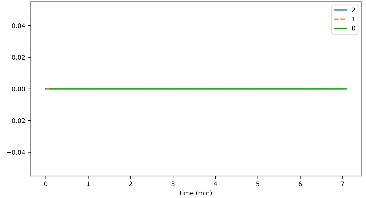
numIndirectProofs
