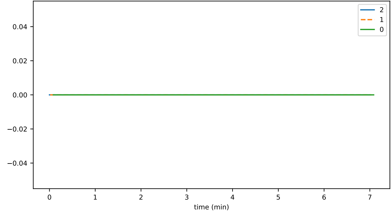
createTransactionRecordDurationAvg
