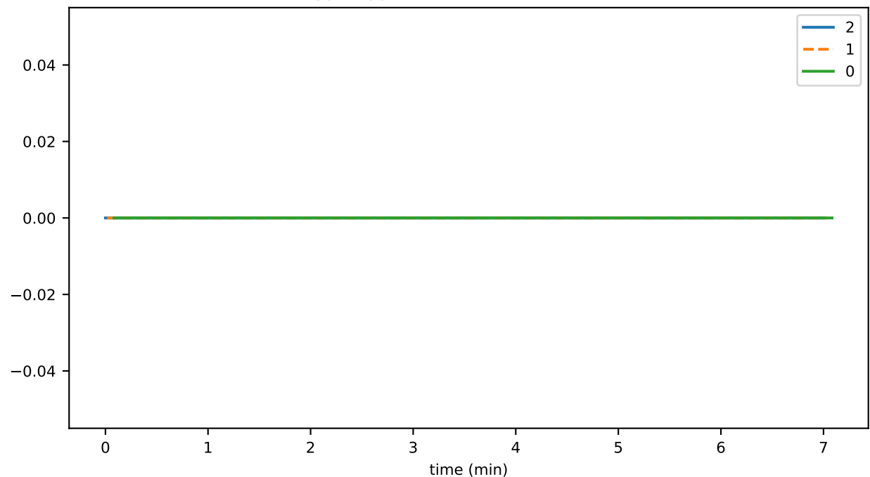
cryptoCreateDurationAvg
