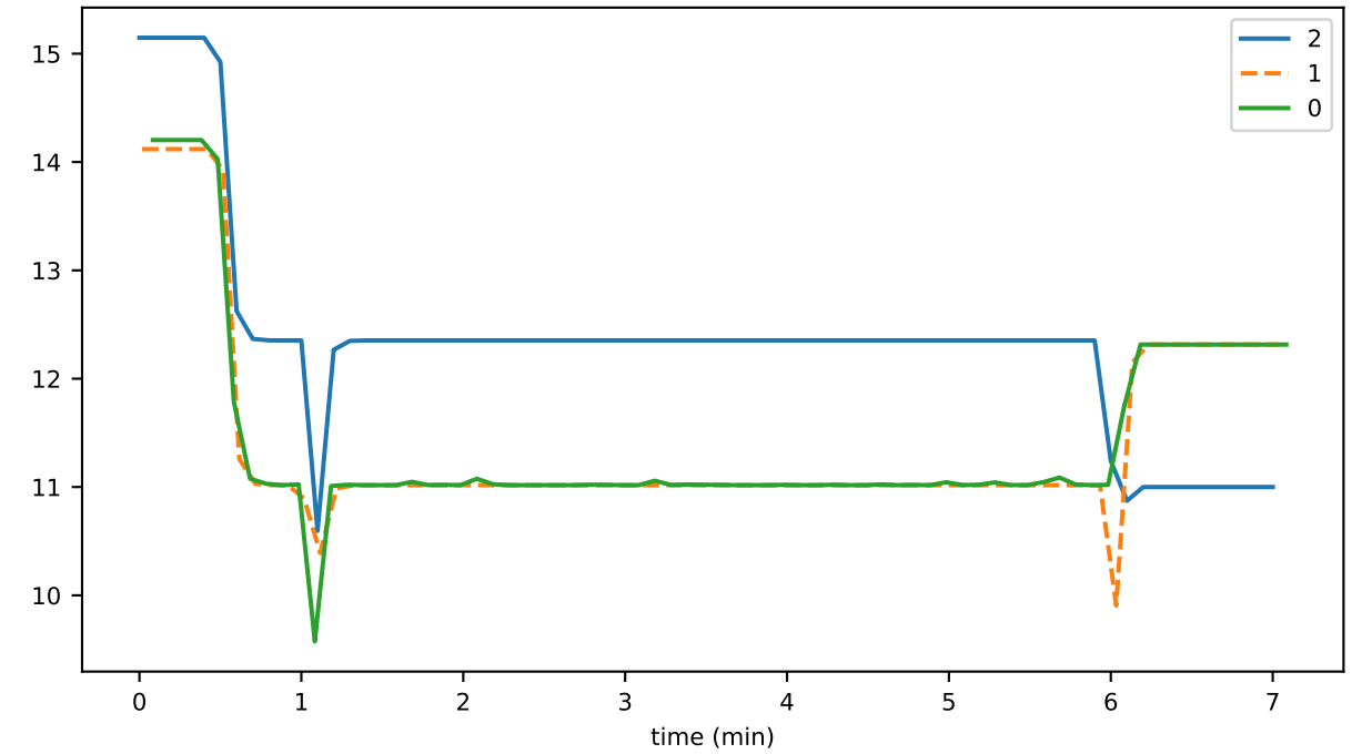
numIndirectProofs
