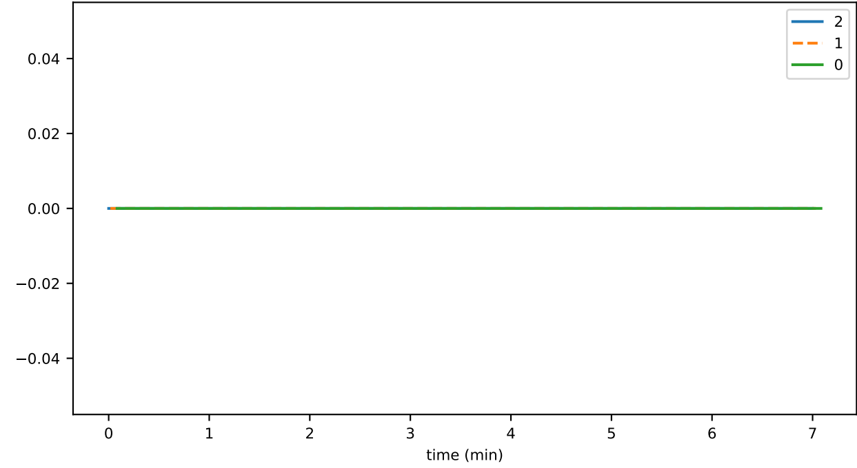
fileDeleteDurationAvg
