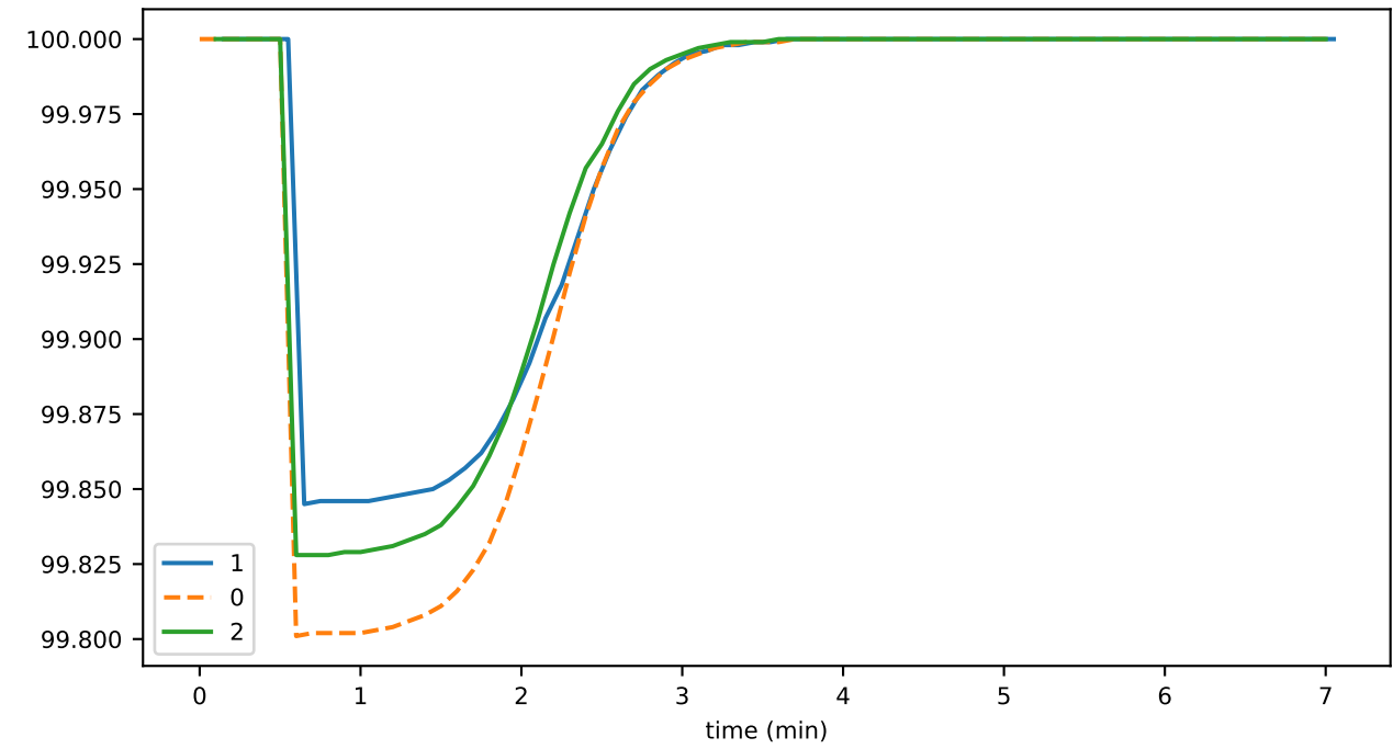
nodeActivePercent_node2
