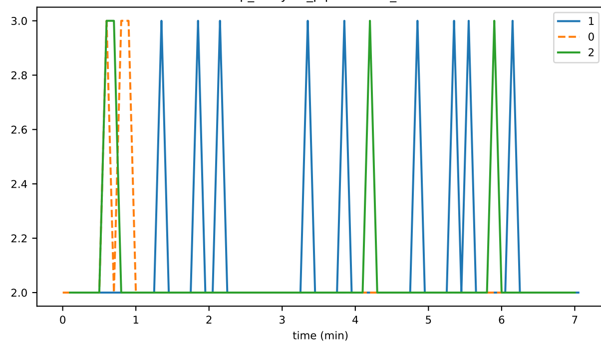
vmap_lifecycle_pipelineSize_state
