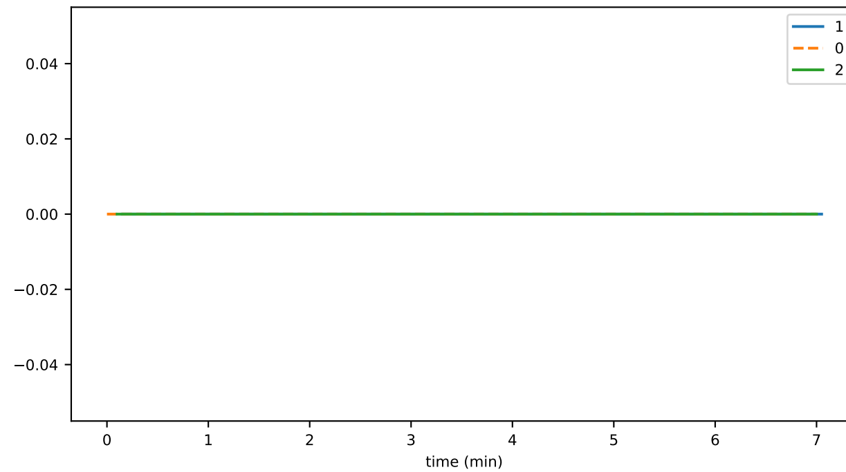
queriedAccountBalances
