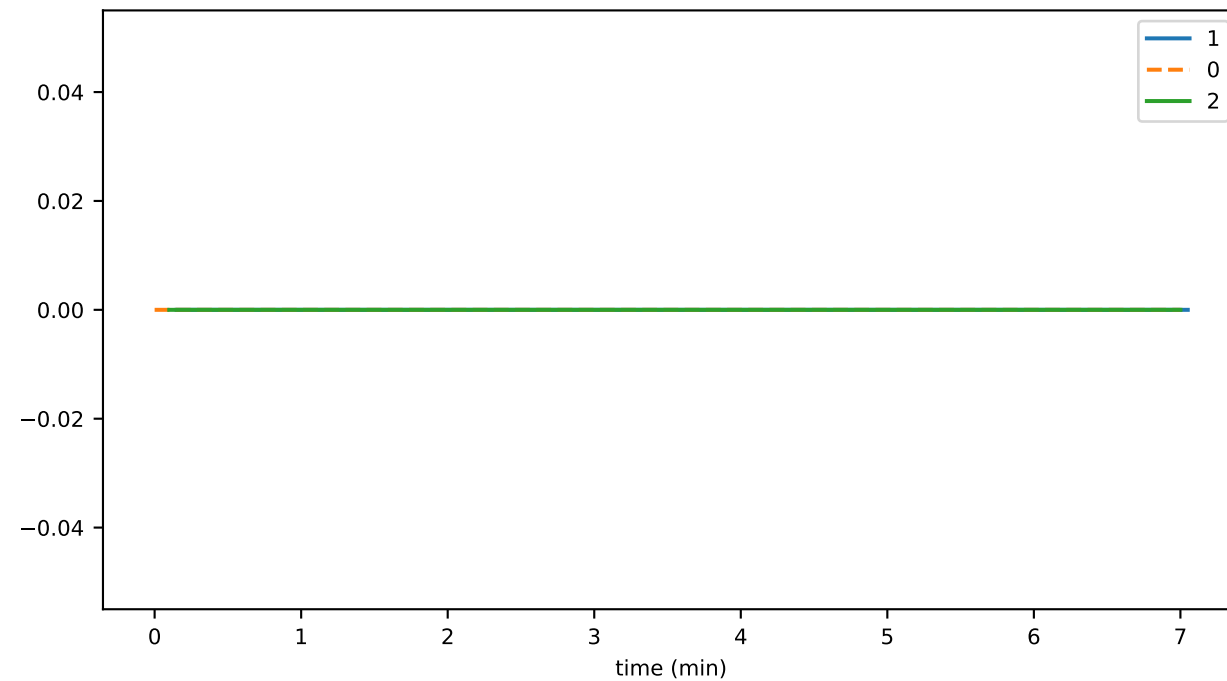
utilPngThrottledTxns
