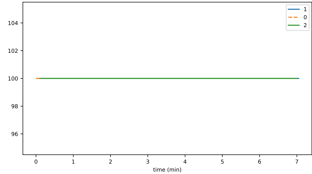
nodeActivePercentSnapshot_node0
