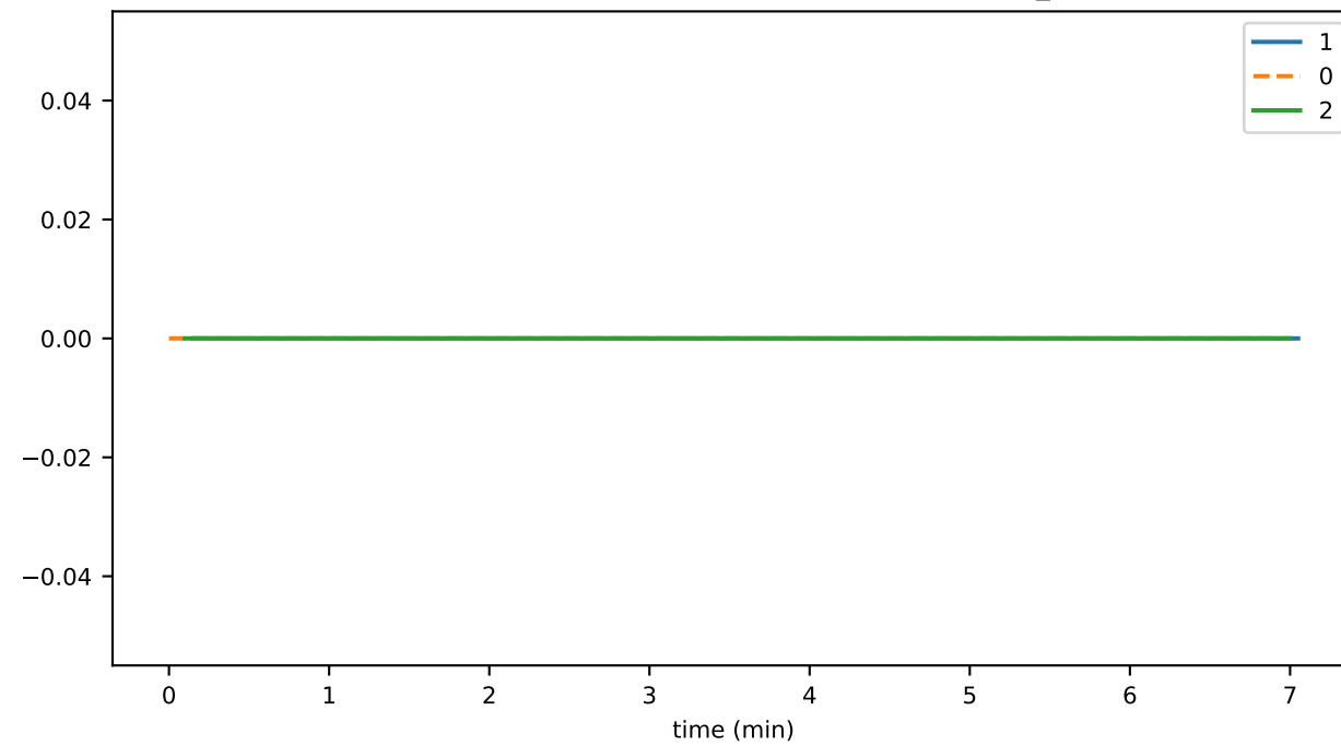
SmartContractService:FailedTransactionDuration_sum
