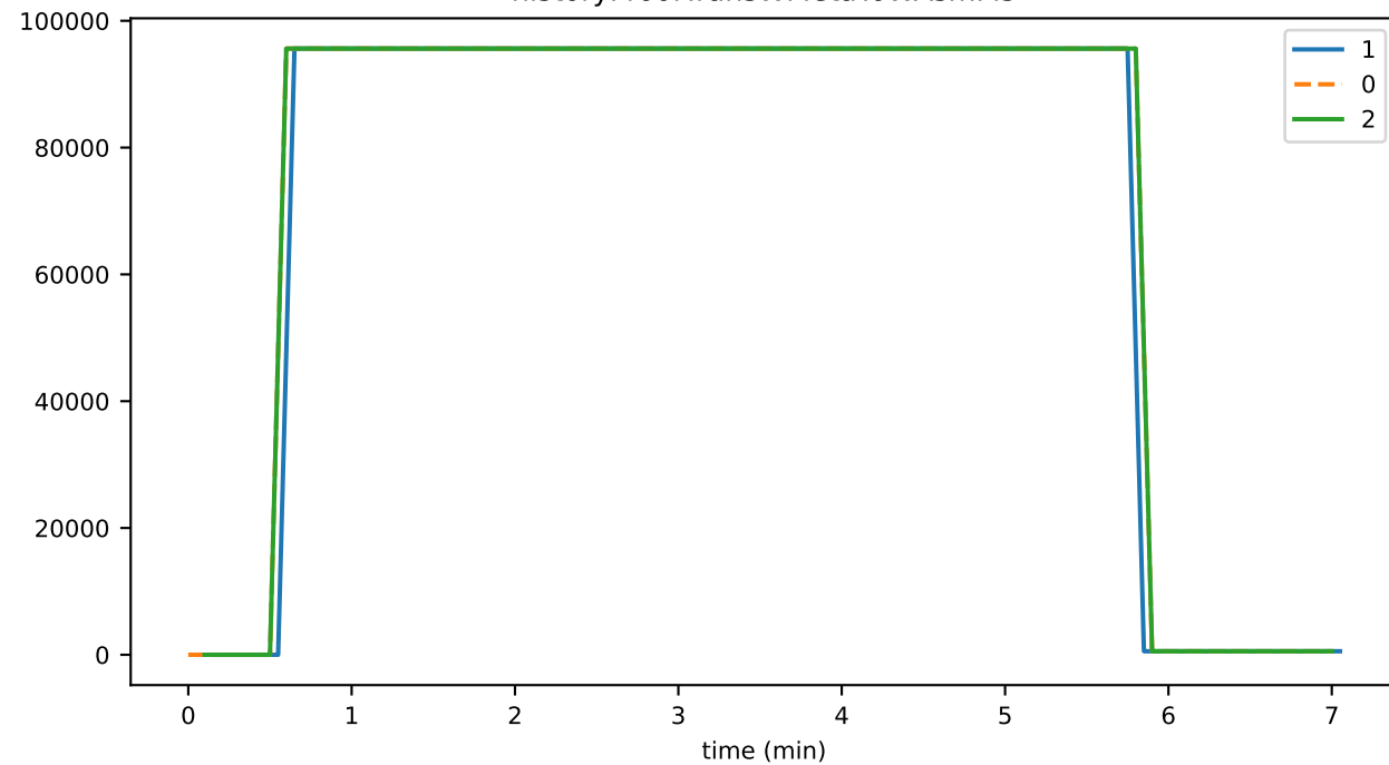
historyProofTransWMetaToWasmMs
