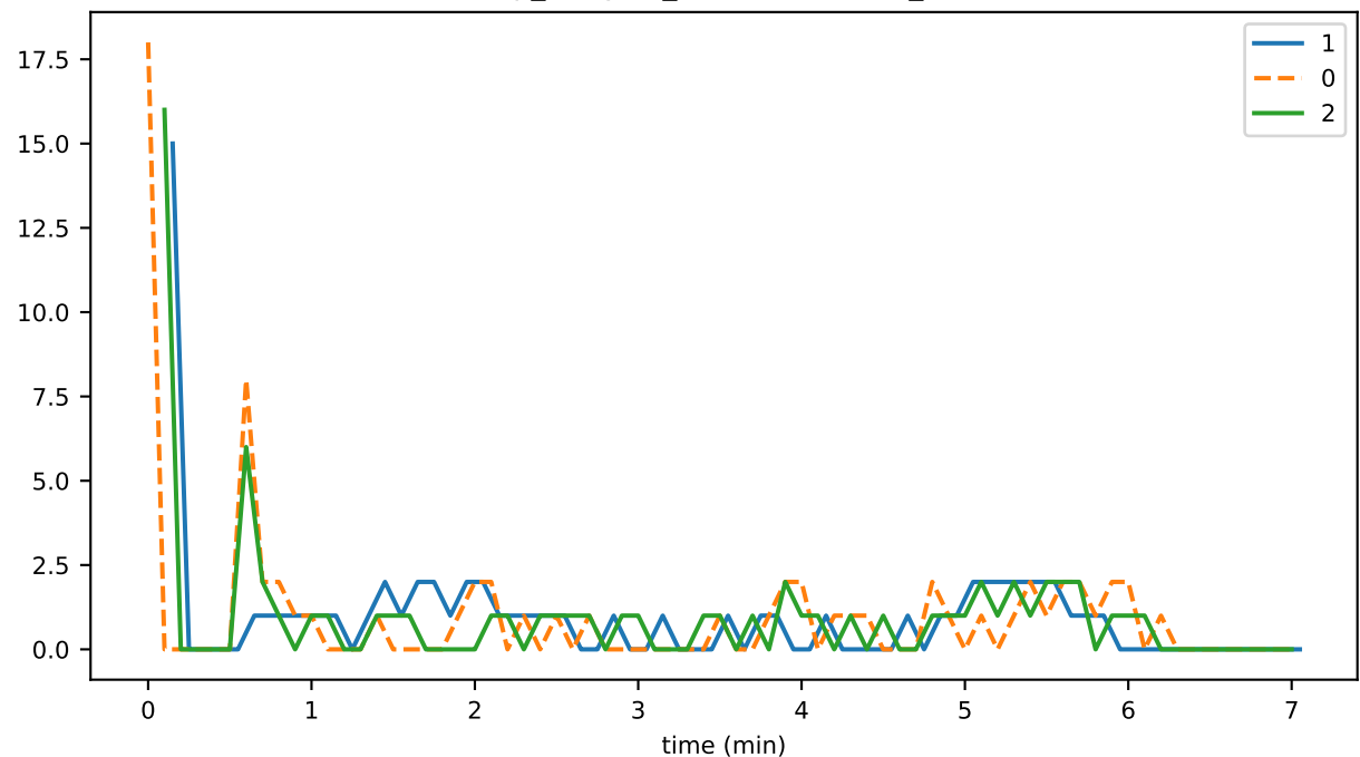
vmap_lifecycle_nodeCacheSizeB_state
