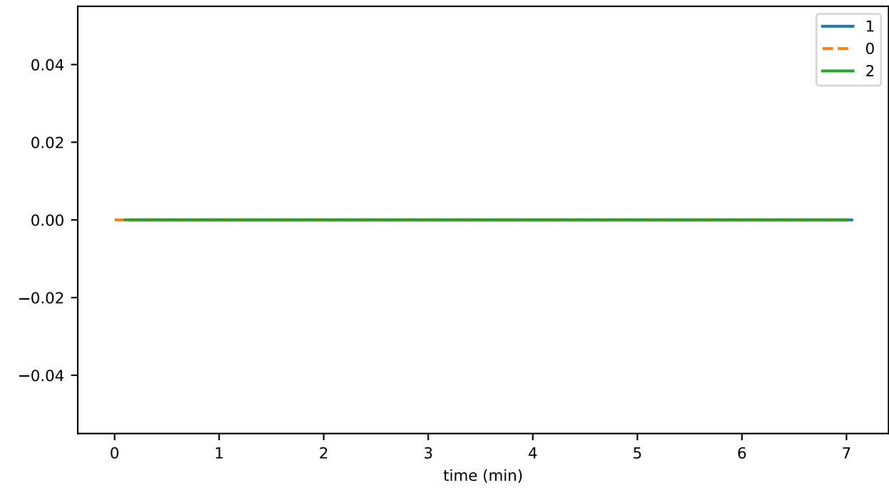
cryptoGetAccountRecordsThrottledTxns
