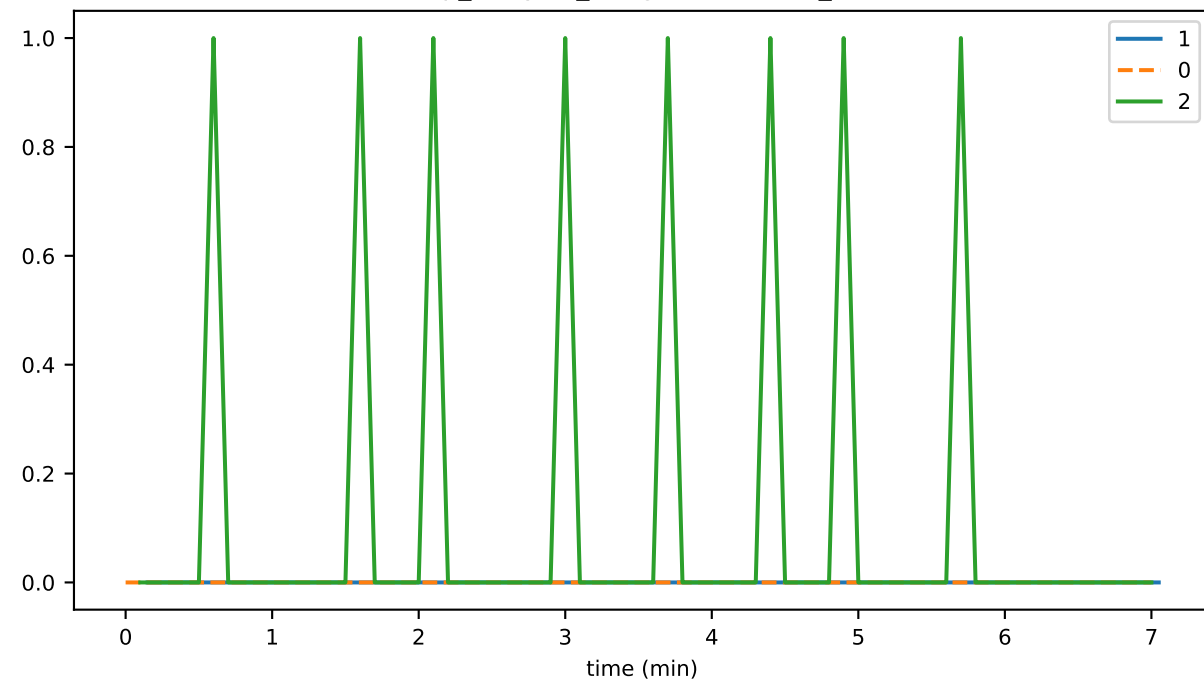
vmap_lifecycle_pipelineSize_state
