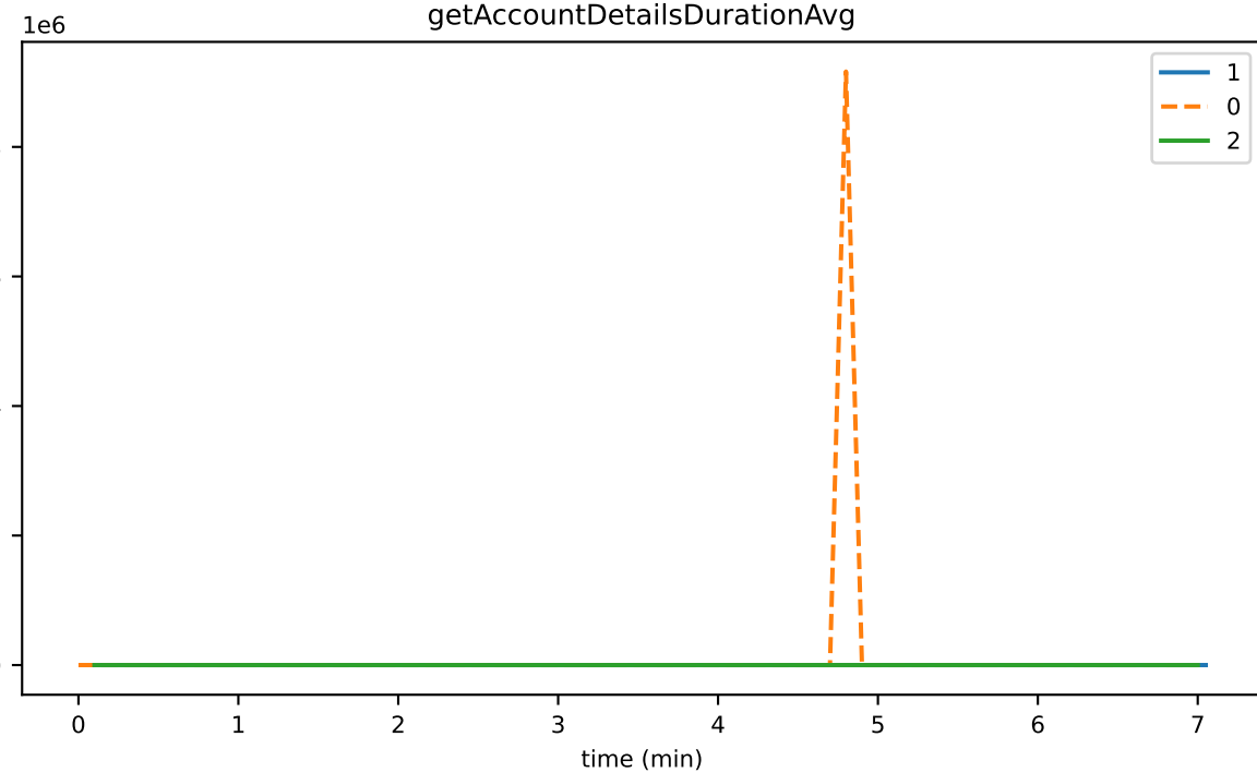
getAccountDetailsDurationAvg
