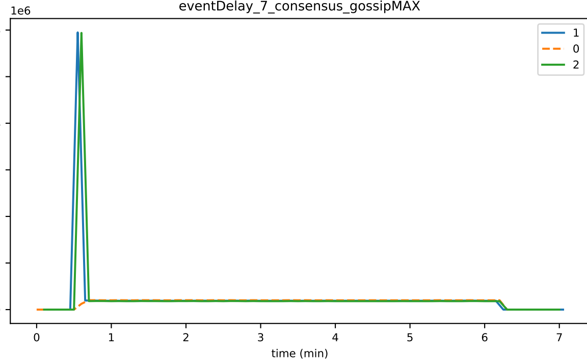
eventDelay_7_consensus_gossipMAX
