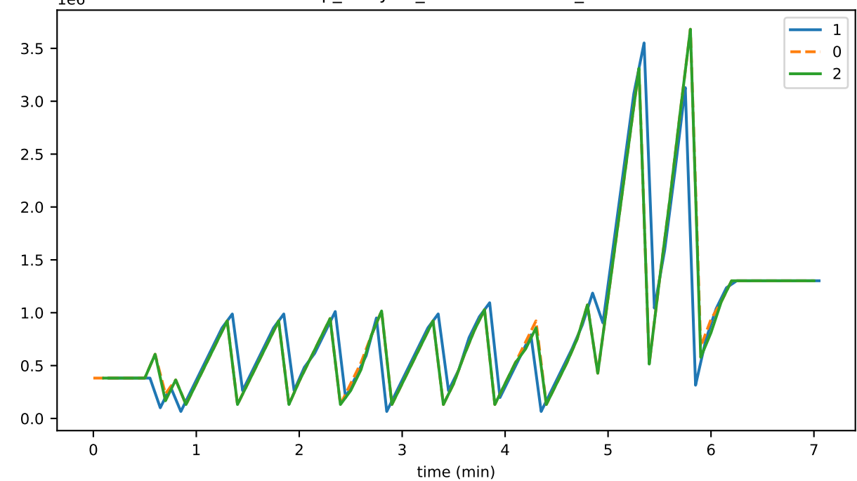
vmap_lifecycle_nodeCacheSizeB_state
