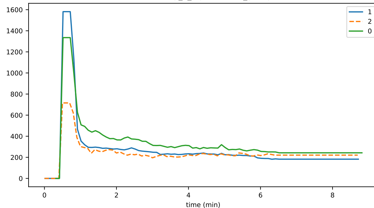
eventDelay_5_orphanBuffer_runtime
