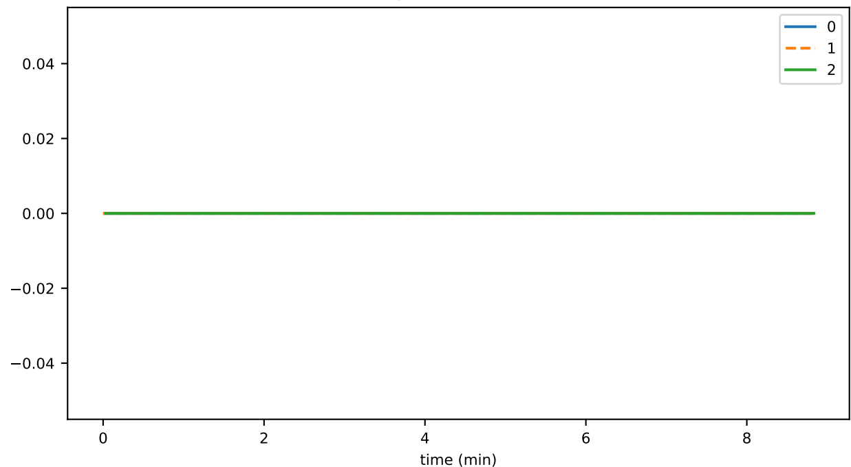
freezeDurationAvg
