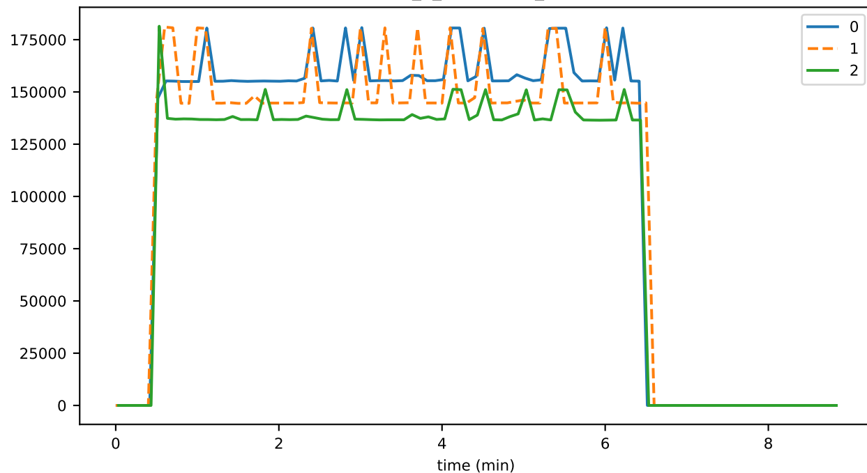
eventDelay_7_consensus_gossipMAX
