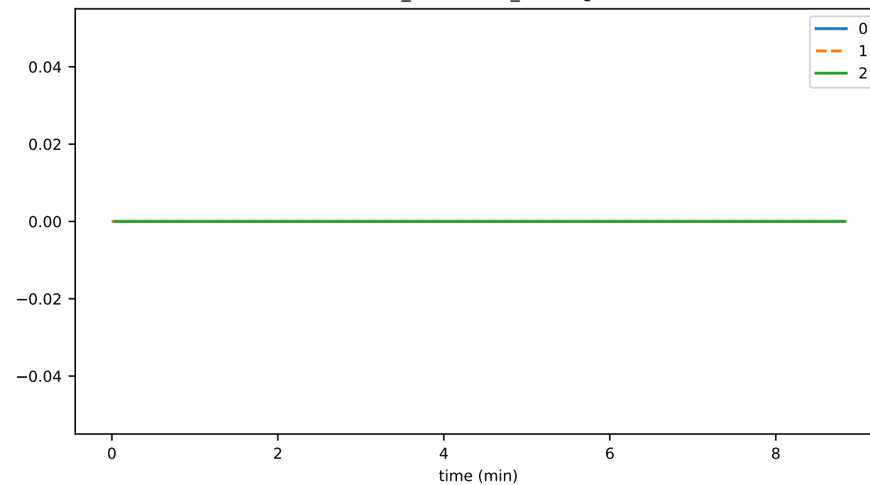
connRecv_endStream_unrecognized
