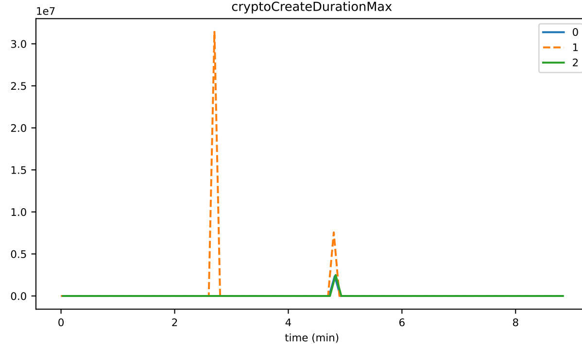
cryptoCreateDurationMax
