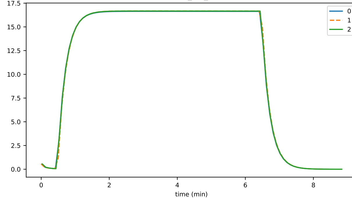
rounds_per_sec
