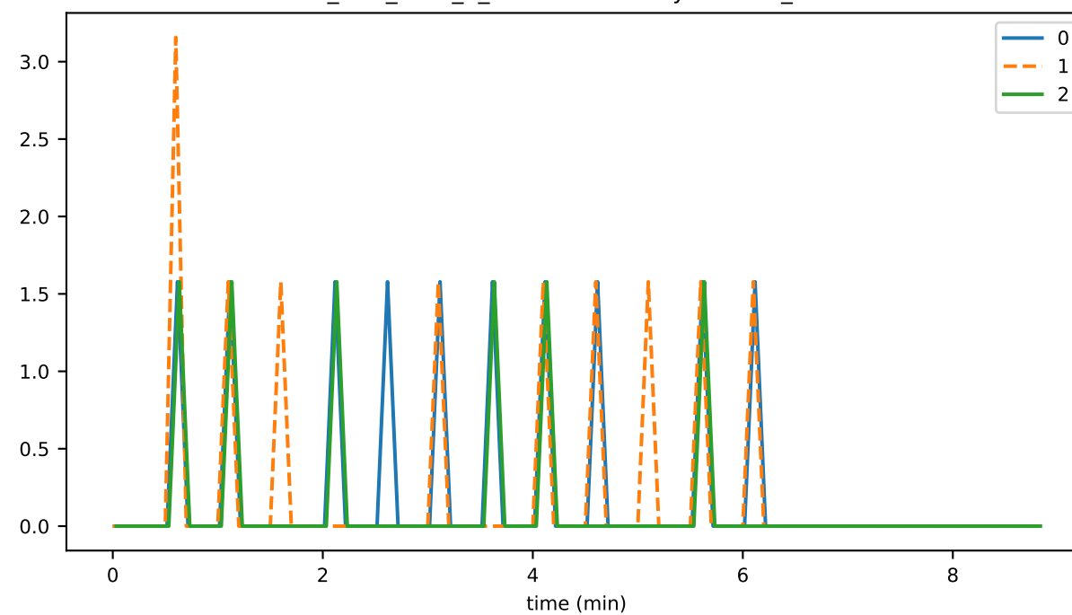
ds_files_level_1_hashesFileSizeByLevelMb_state
