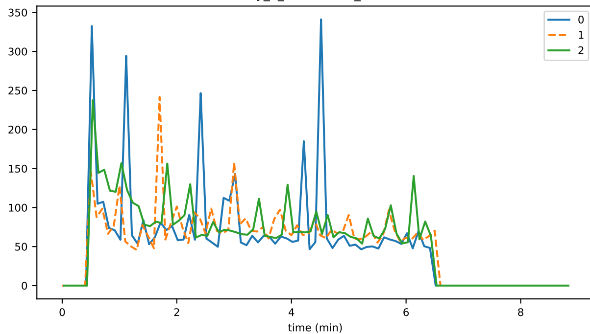
eventDelay_4_verification_runtimeMAX
