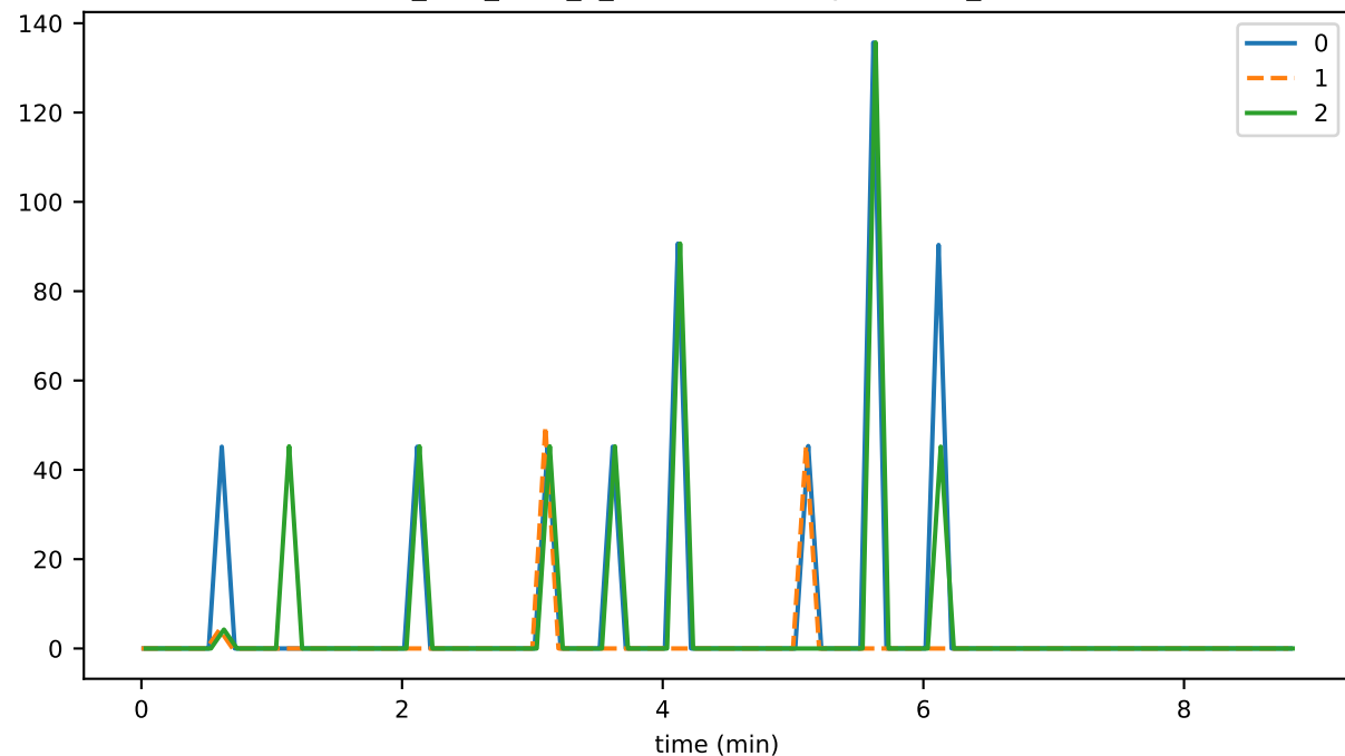
ds_files_level_3_leafKeysFileSizeByLevelMb_state
