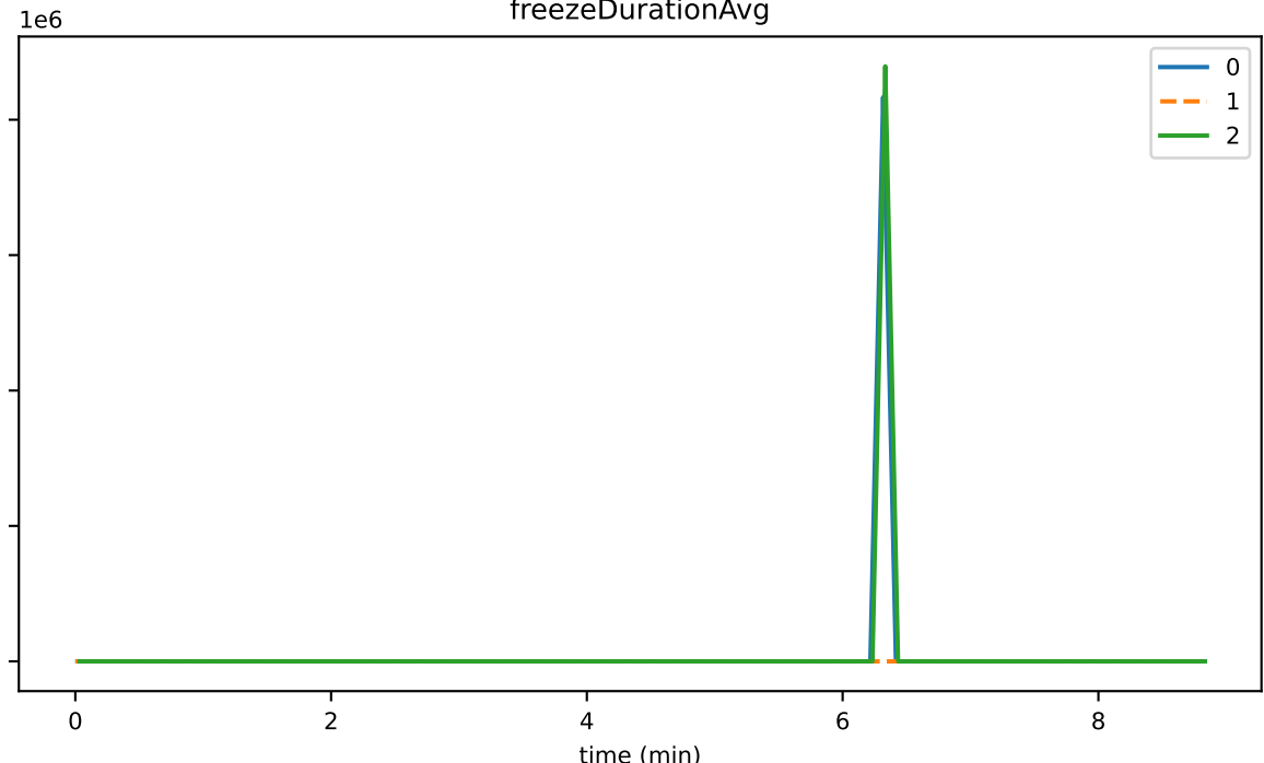
freezeDurationAvg
