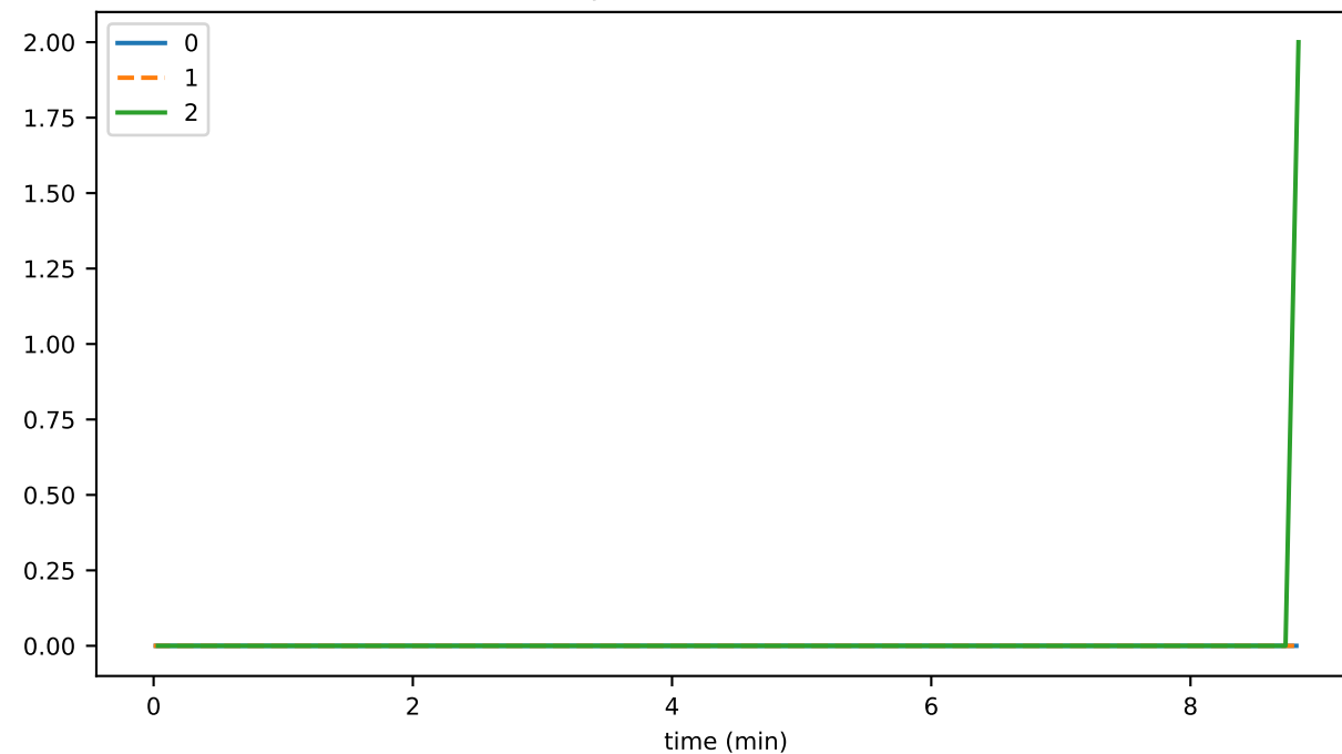
syncPermitsUtilized
