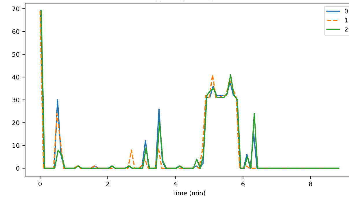
dupEvPercent
