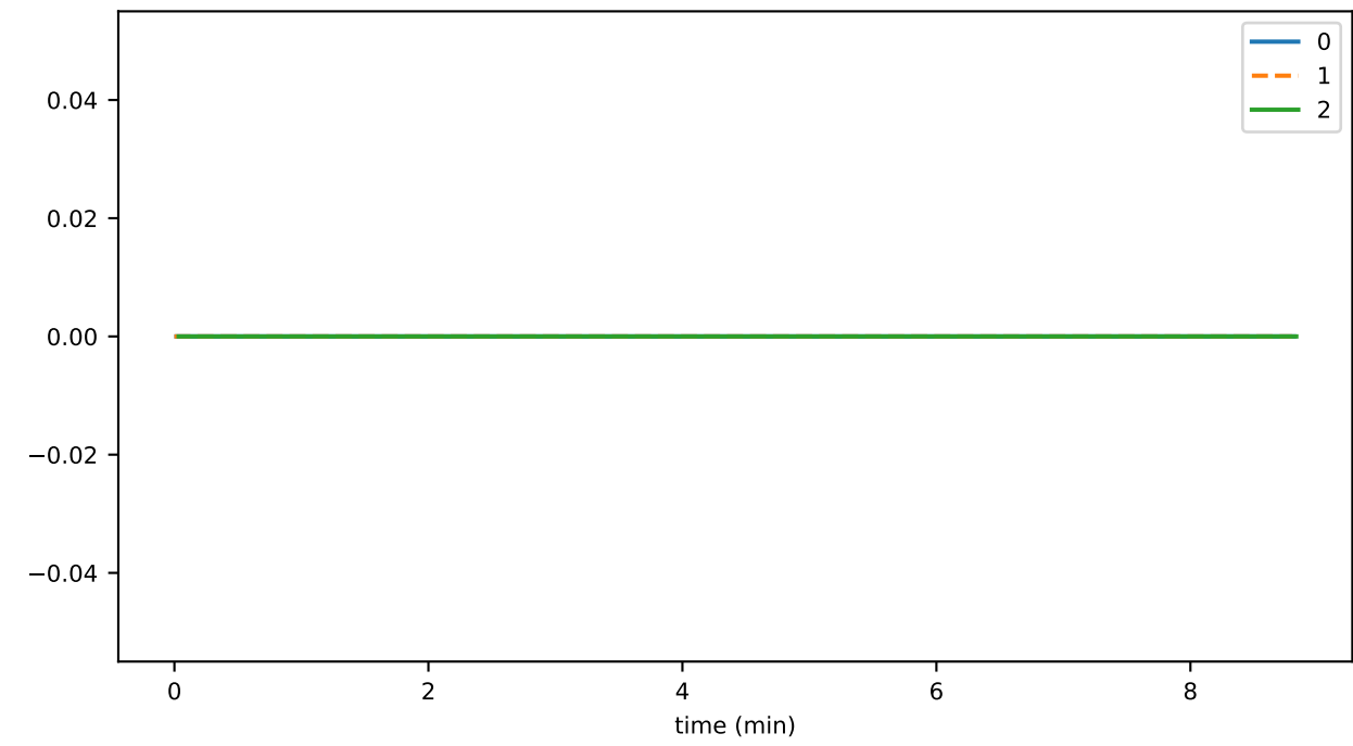
queriedAccountBalances
