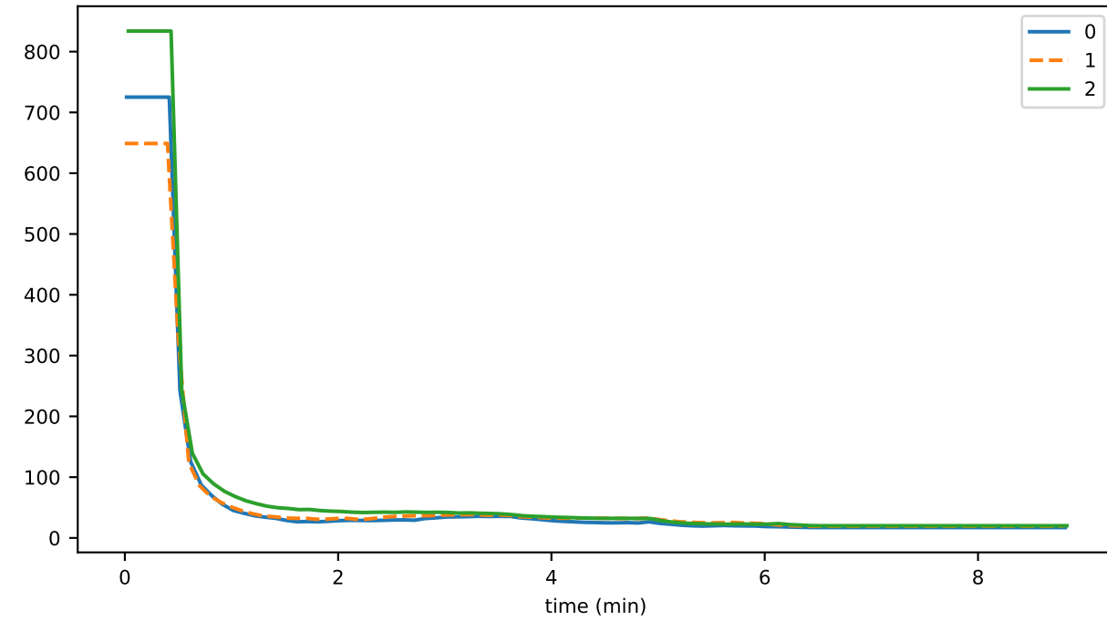
utilPrngDurationMax
