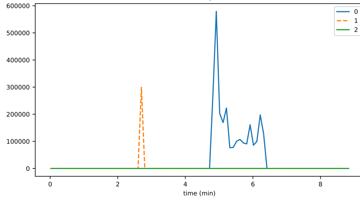
transactionGetReceiptDurationMax
