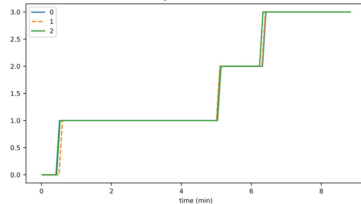
historyProofTransR2ToFailCnt
