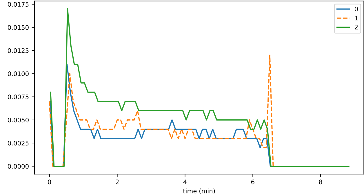
ConsensusEngine_busy_fraction
