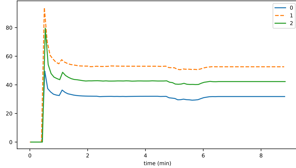
averageTimeToFullySignState
