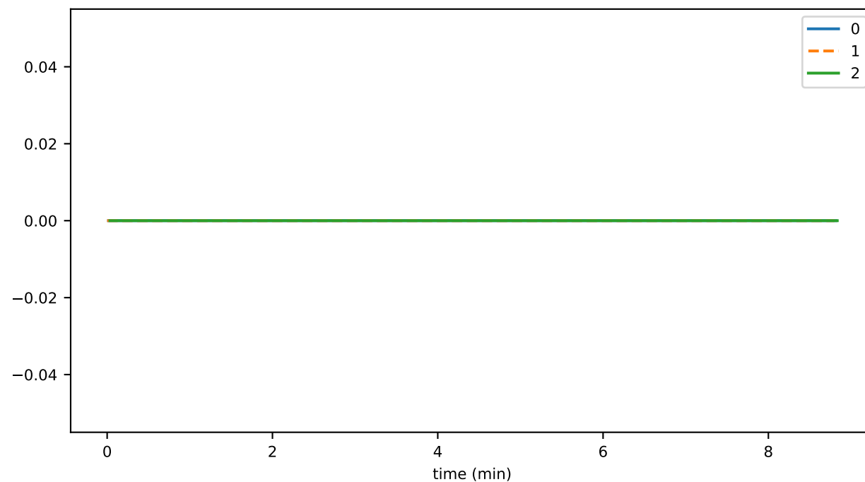
contractUpdateDurationMax
