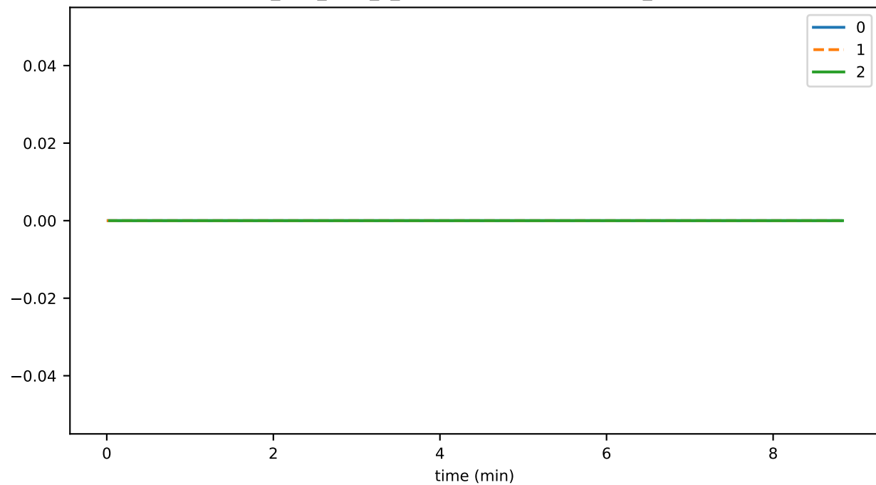
ds_files_level_3_leafKeysFileSizeByLevelMb_state
