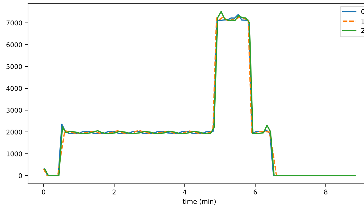
vmap_queries_updatedEntities_state
