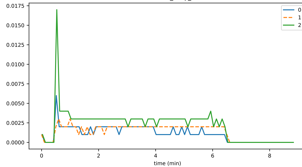
InlinePcesWriter_busy_fraction
