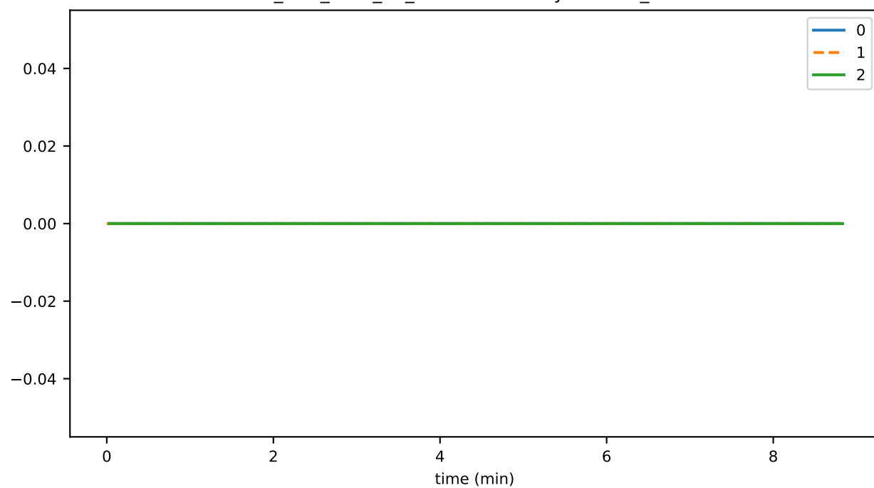
ds_files_level_10_leavesFileSizeByLevelMb_state
