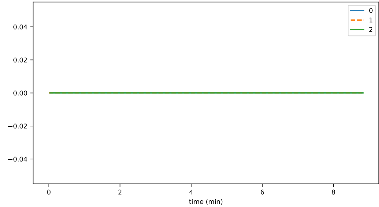
SmartContractService:SystemContractMethodCall_KYC_failed
