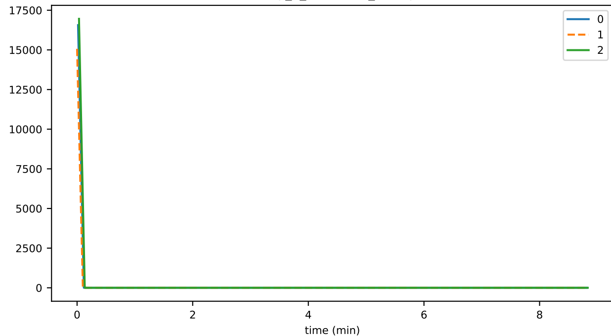
eventDelay_3_deduplication_gossipMAX
