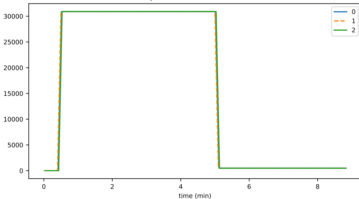
historyProofTransWMetaToWasmMs
