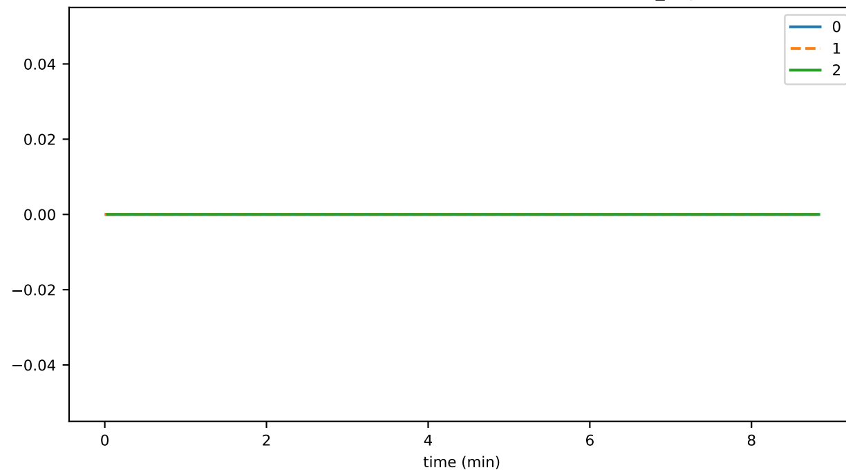
SmartContractService:FailedTransactionDuration_sum
