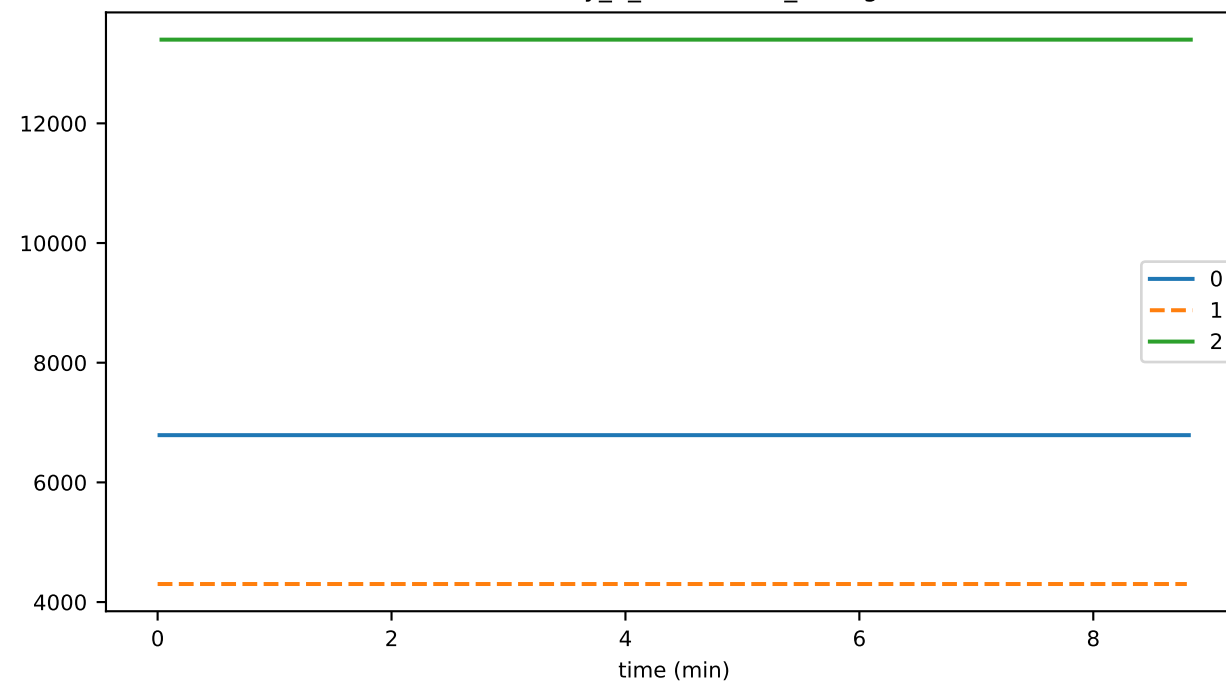
eventDelay_4_verification_storage
