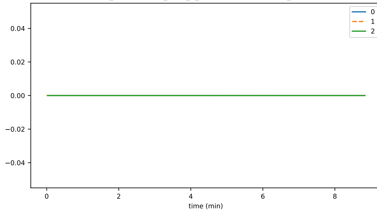
ds_compactions_level_4_hashesSavedSpaceMb_state
