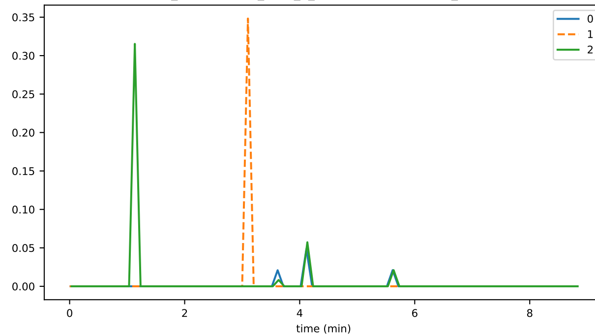
ds_compactions_level_2_leavesSavedSpaceMb_state
