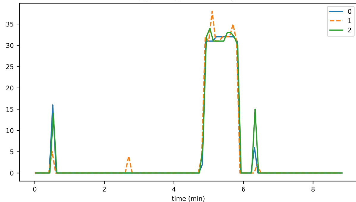
vmap_queries_removedEntities_state
