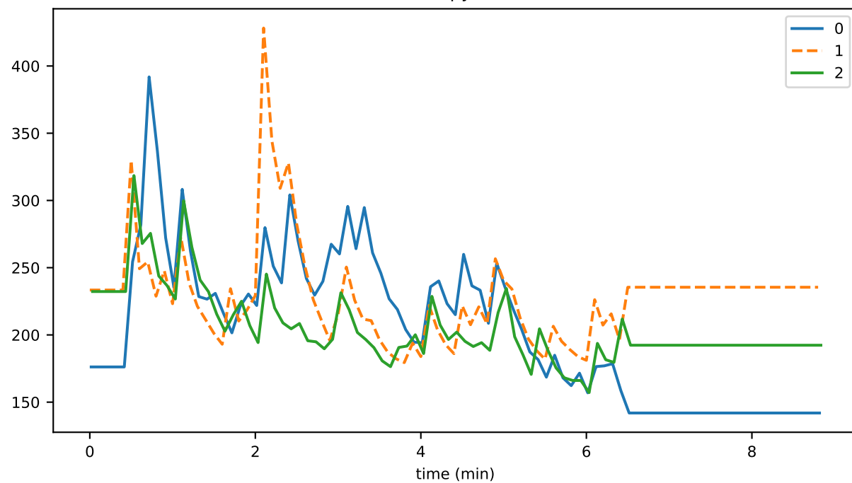
stateCopyMicros
