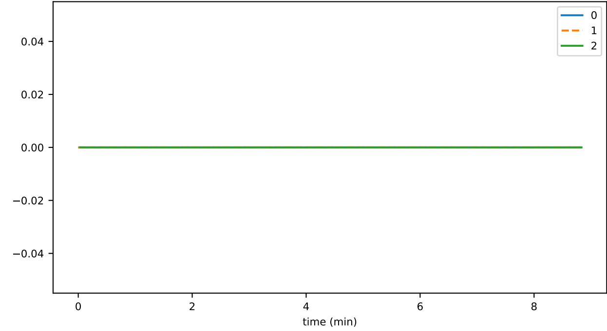
SmartContractService:SystemContractMethodCall_KYC_failed
