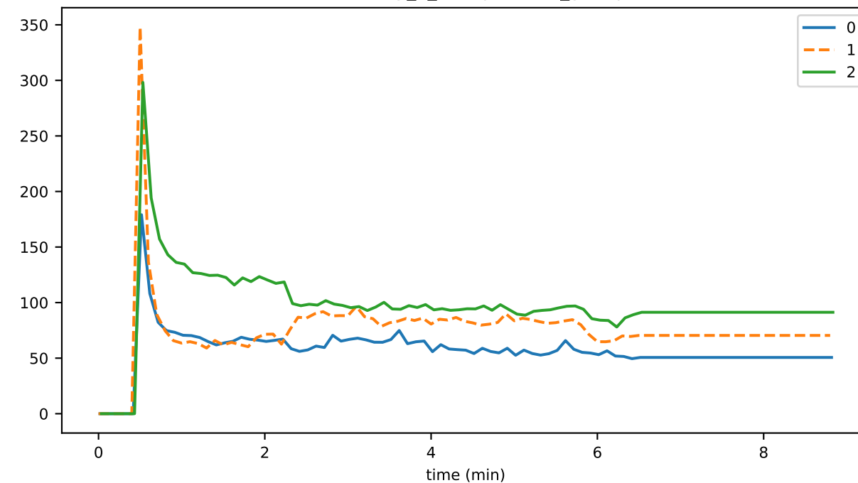
eventDelay_3_deduplication_runtime
