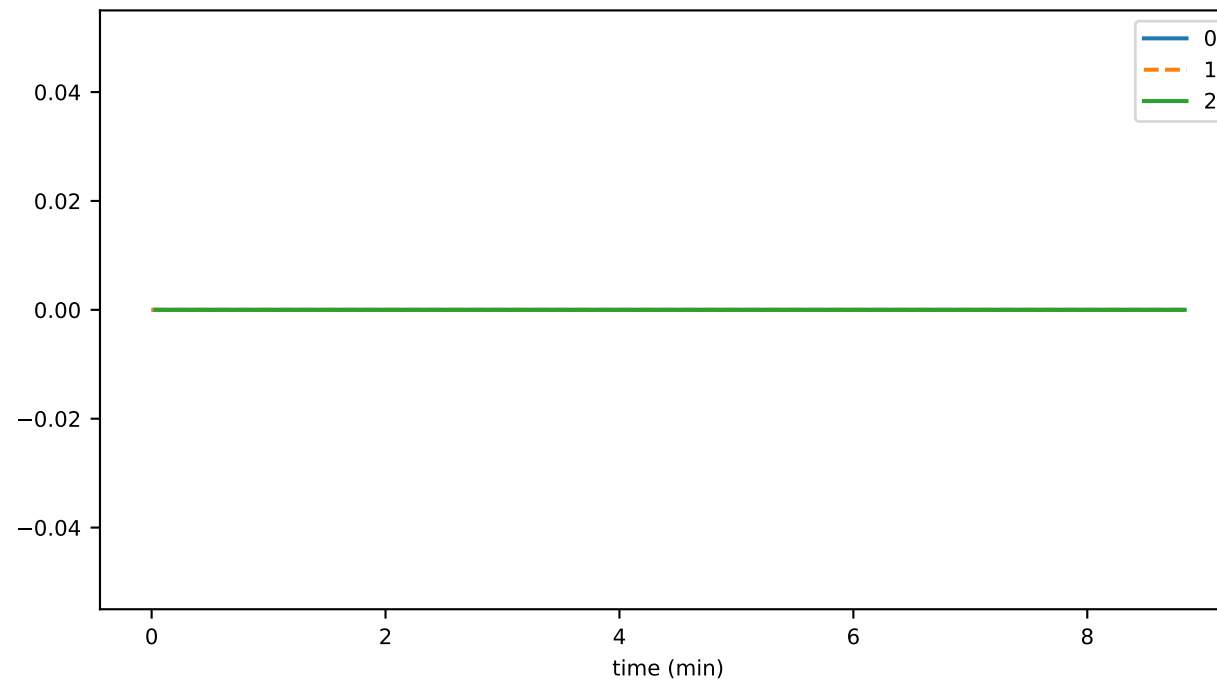
eventsWithDisparateSignature
