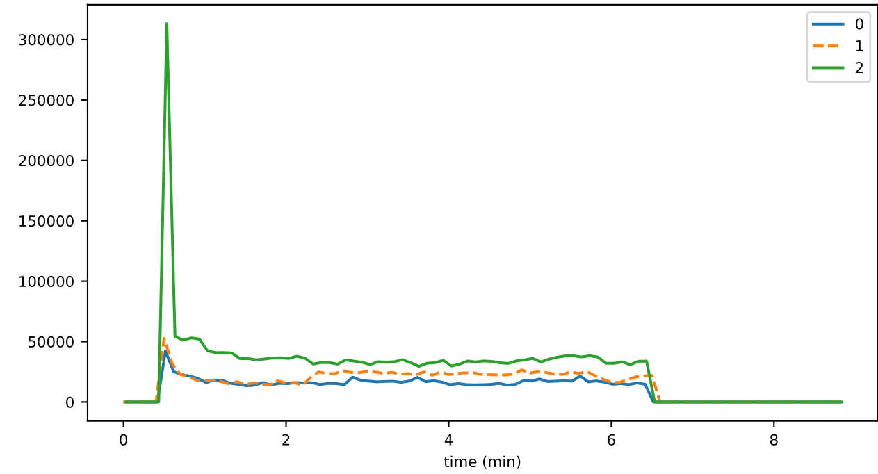
ping_us_00
