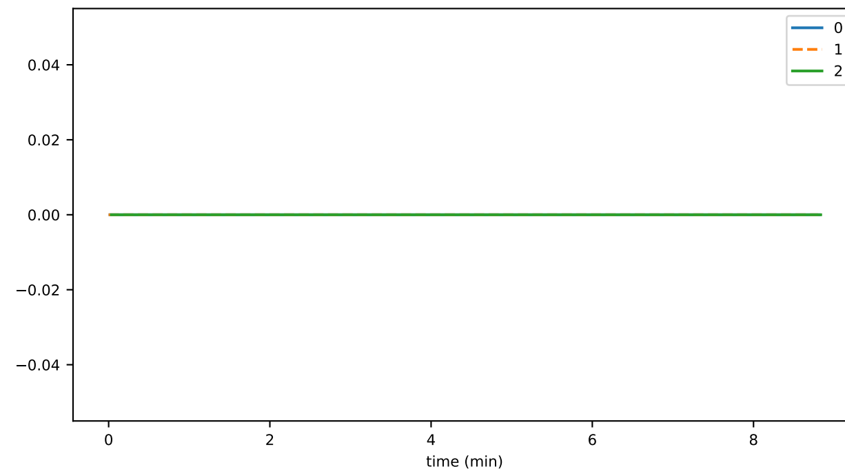
staleTransactions
