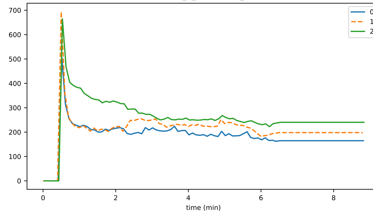
eventDelay_4_verification_gossip
