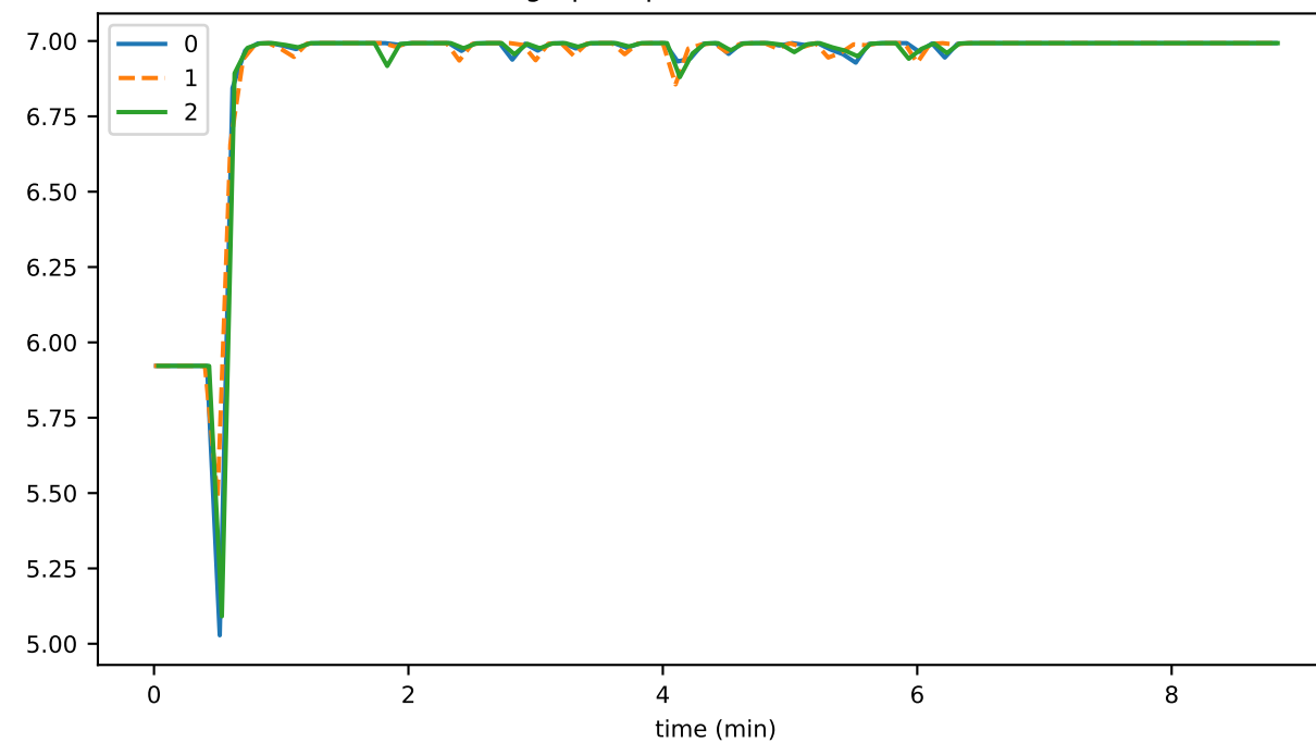
graphDepthUntilConsensus
