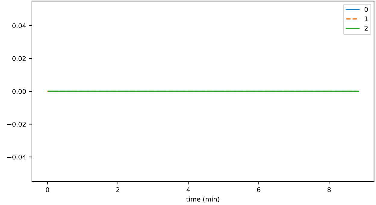
numIndirectProofs
