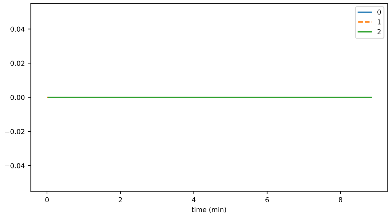
tokenUpdateDurationMax
