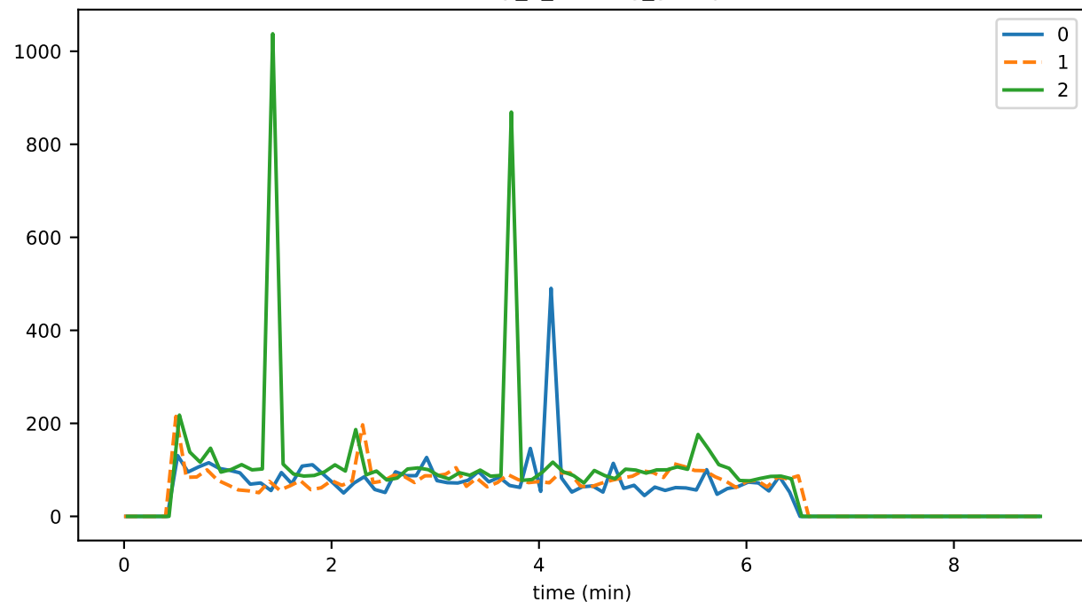
eventDelay_1_hashing_storageMAX
