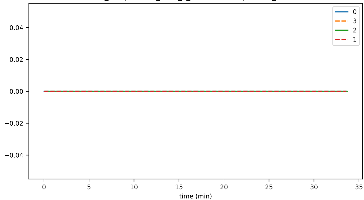
ds_compactions_level_8_leavesSavedSpaceMb_state
