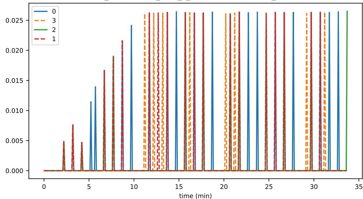
ds_compactions_level_2_hashesSavedSpaceMb_state
