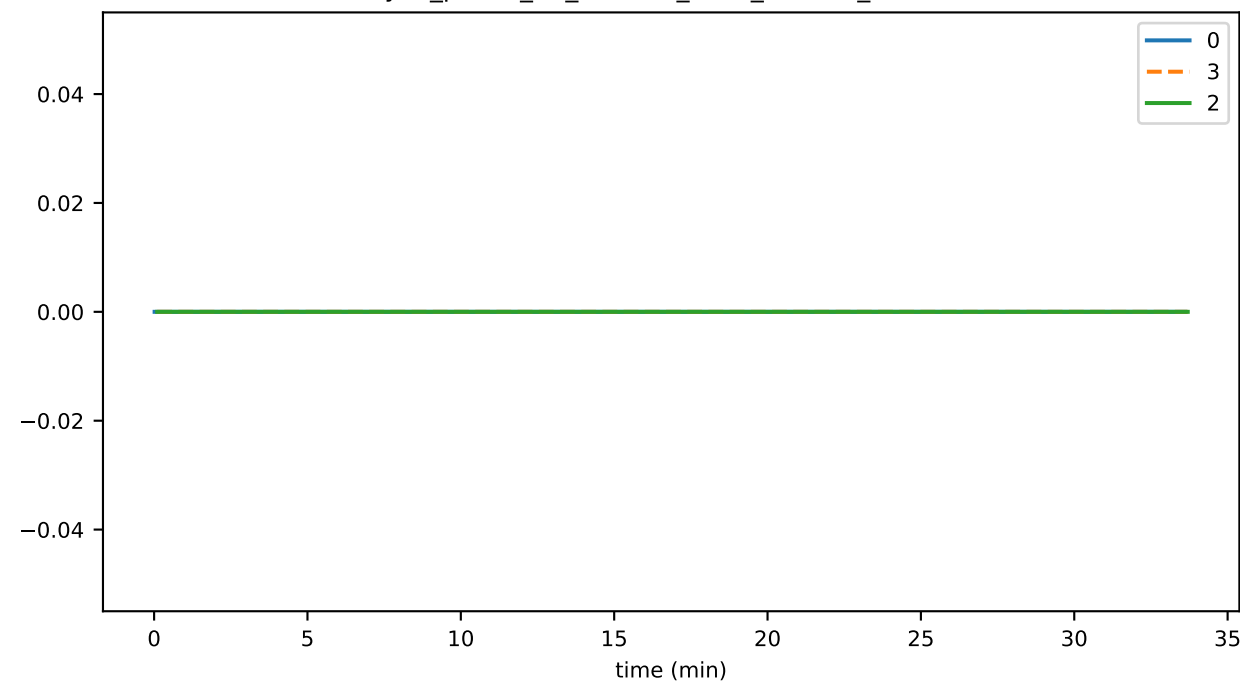
sync_phase_01_fraction_SELF_FALLEN_BEHIND
