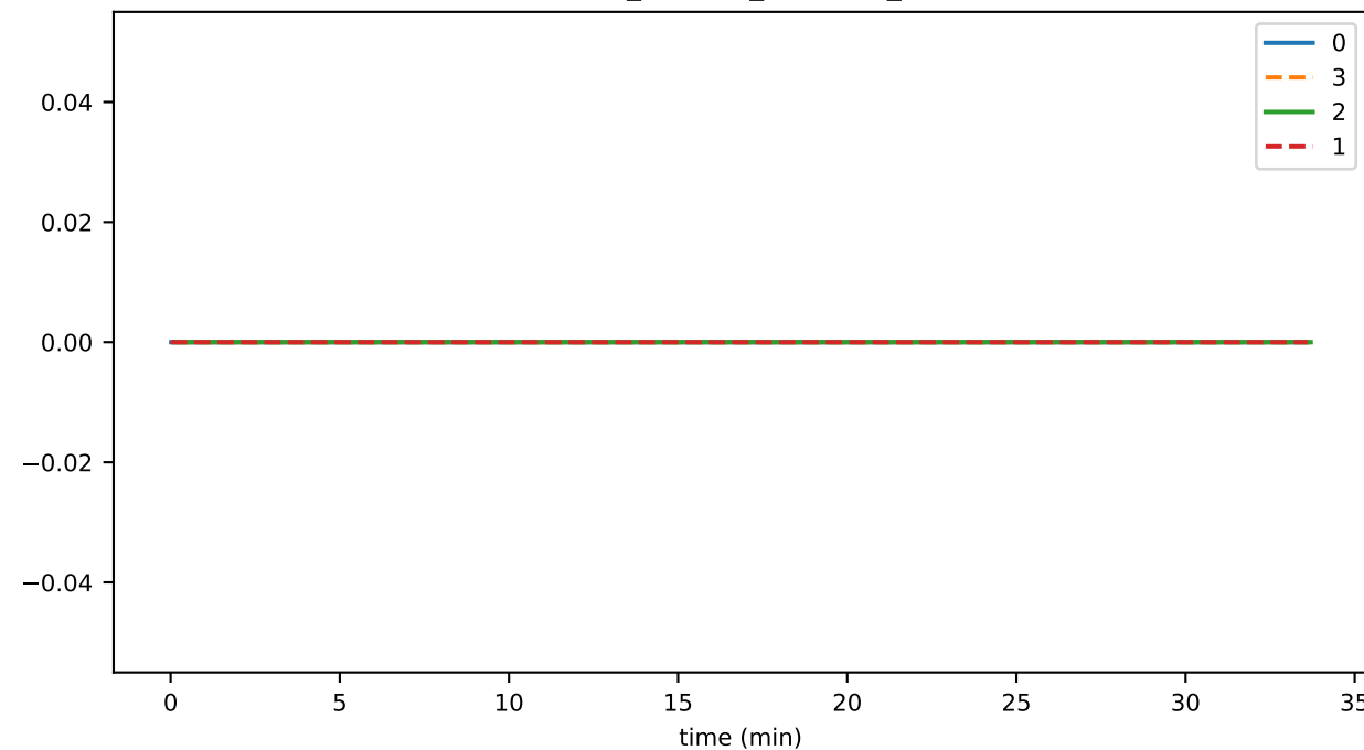
eventCreation_fraction_QUIESCENCE
