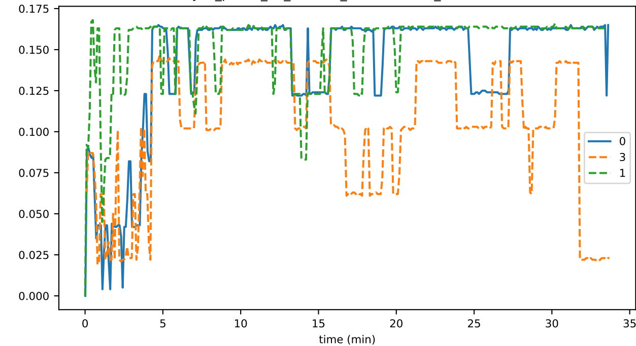
sync_phase_02_fraction_EXCHANGING_WINDOWS
