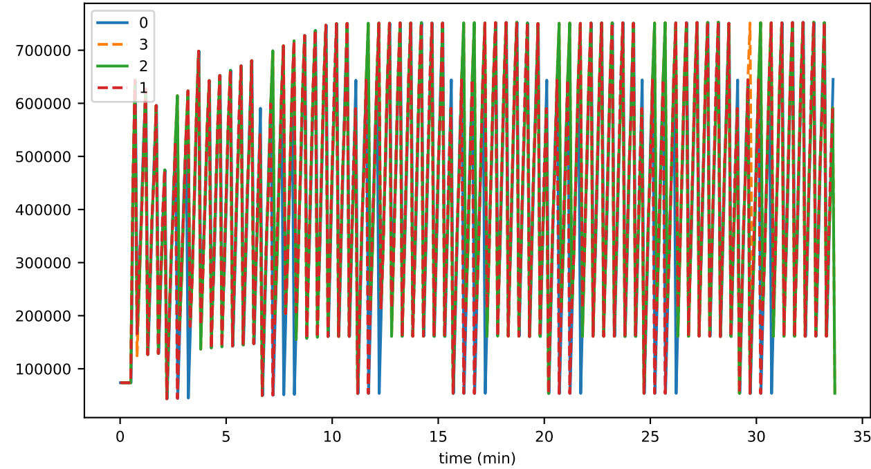
vmap_queries_addedEntities_state
