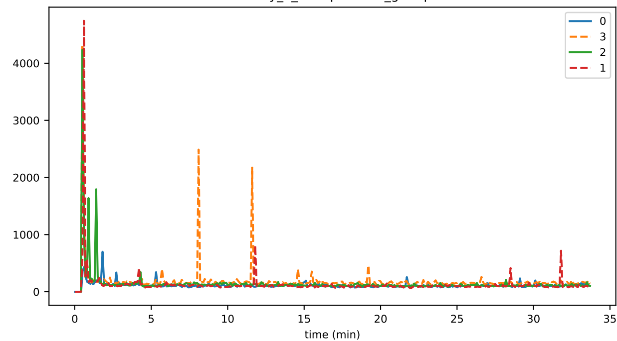
eventDelay_3_deduplication_gossipMAX
