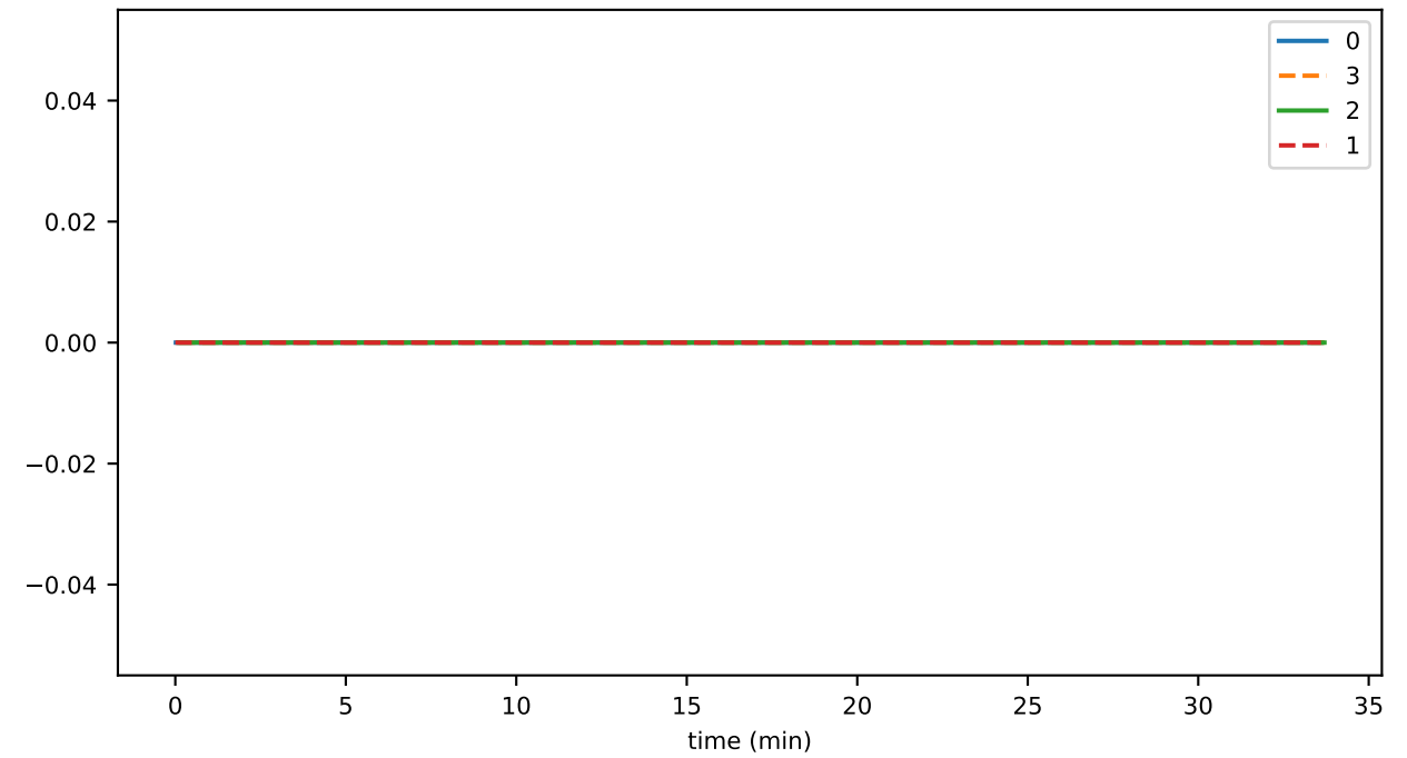
broadcastDisabledDueToOverload
