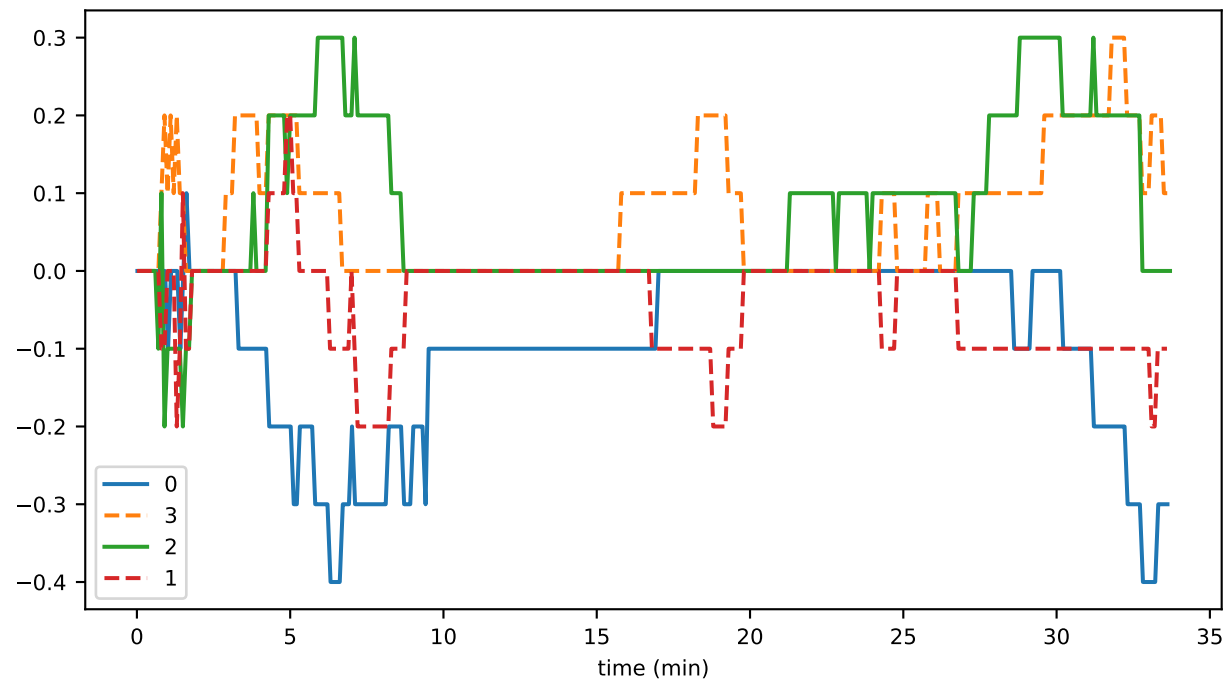
syncIndicatorDiff
