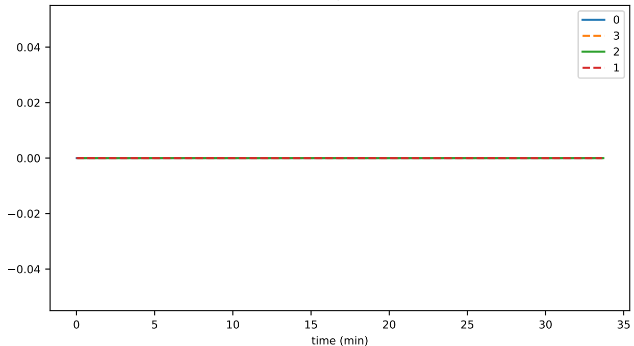
uptimeComputationTime
