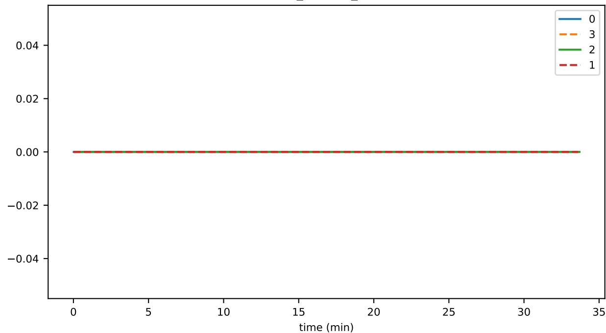
eventCreation_fraction_PLATFORM_STATUS
