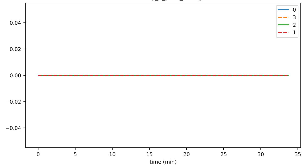
eventDelay_6_pces_storage
