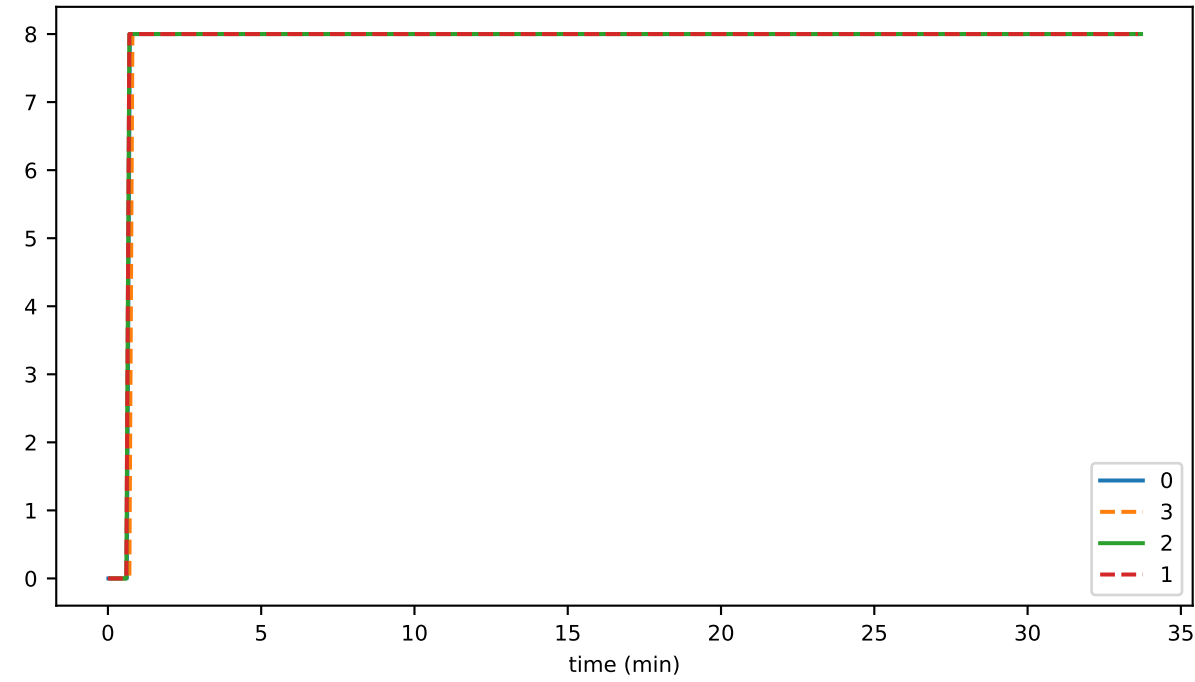
ds_reads_hashes_state
