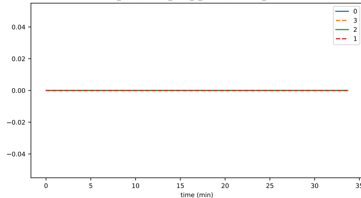
ds_compactions_level_4_leavesTimeMs_state
