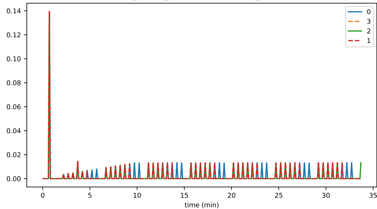
ds_flushes_leavesStoreFileSizeMb_state
