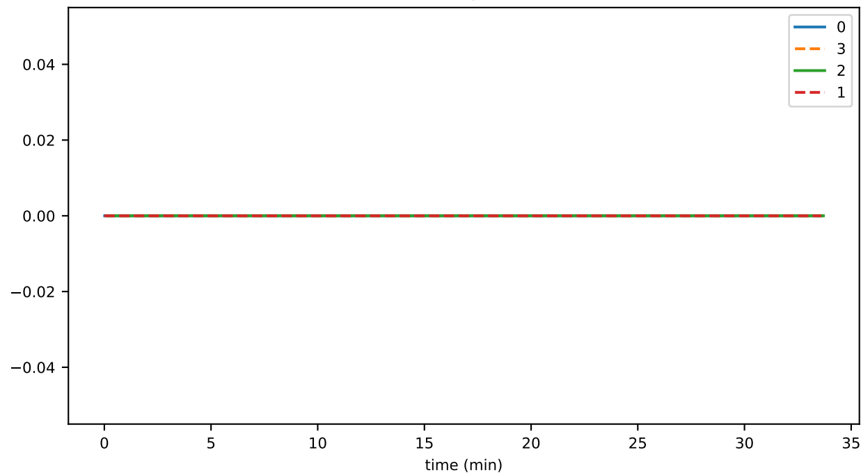
trans_per_event
