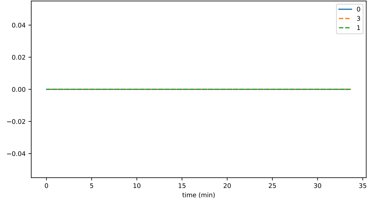
sync_phase_02_fraction_OTHER_FALLEN_BEHIND
