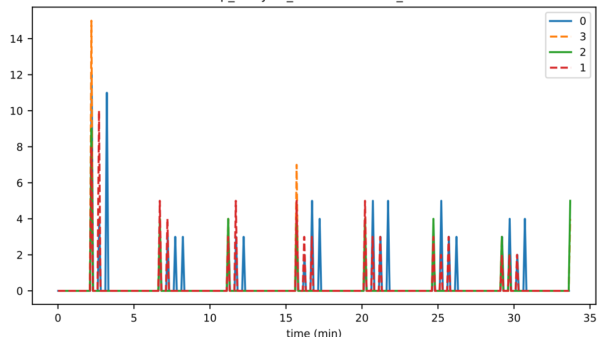
vmap_lifecycle_flushDurationMs_state
