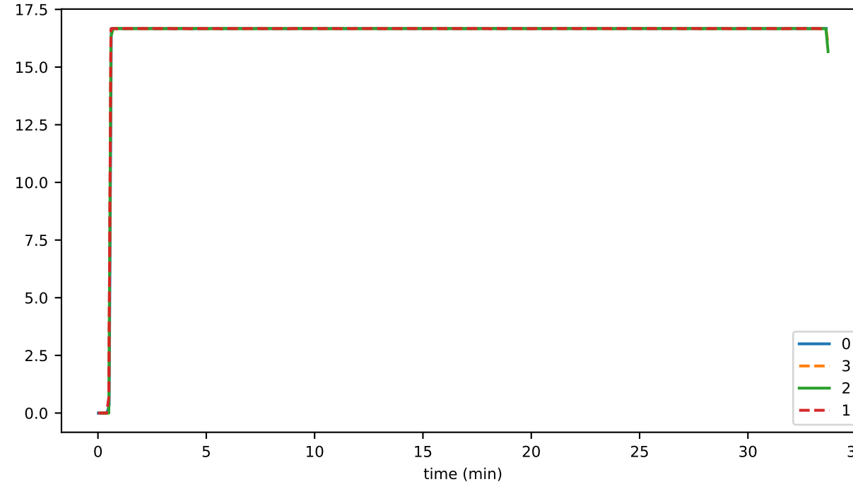
buffer_blockBytes
