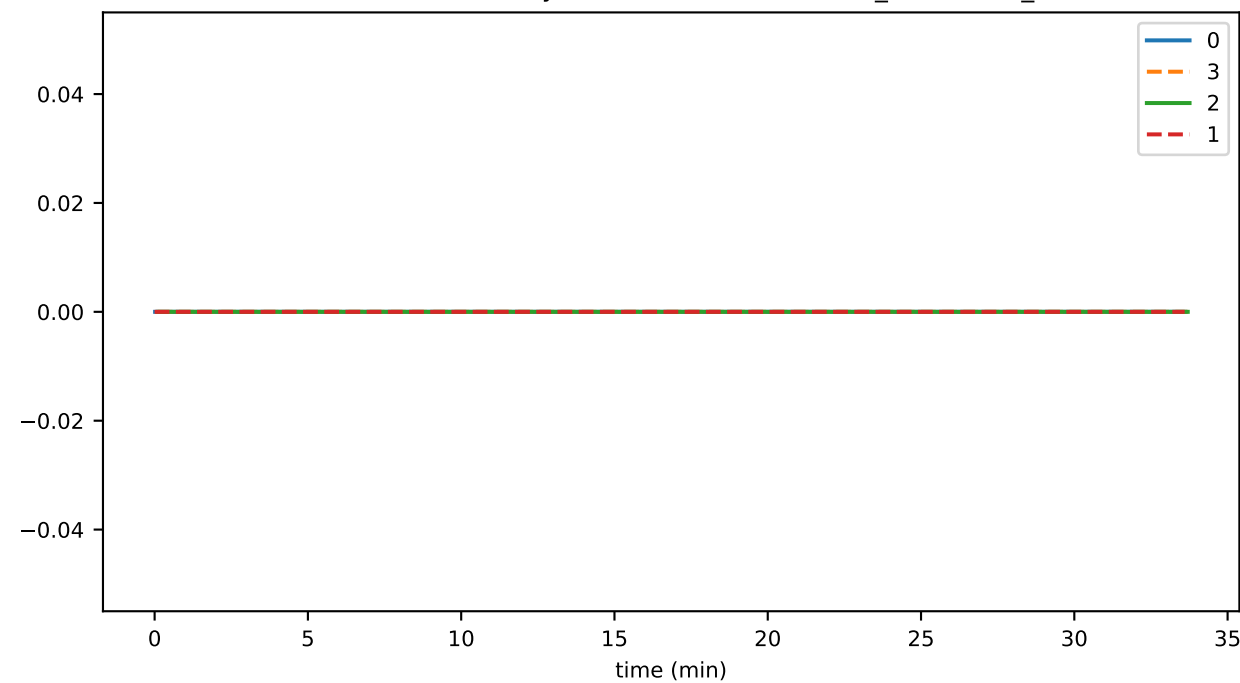
SmartContractService:SystemContractMethodCall_APPROVAL_failed
