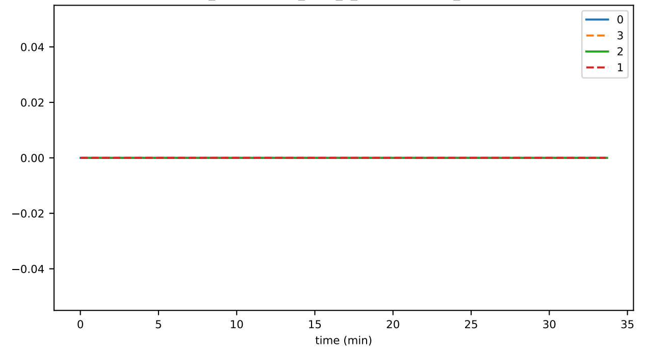
ds_compactions_level_6_hashesTimeMs_state
