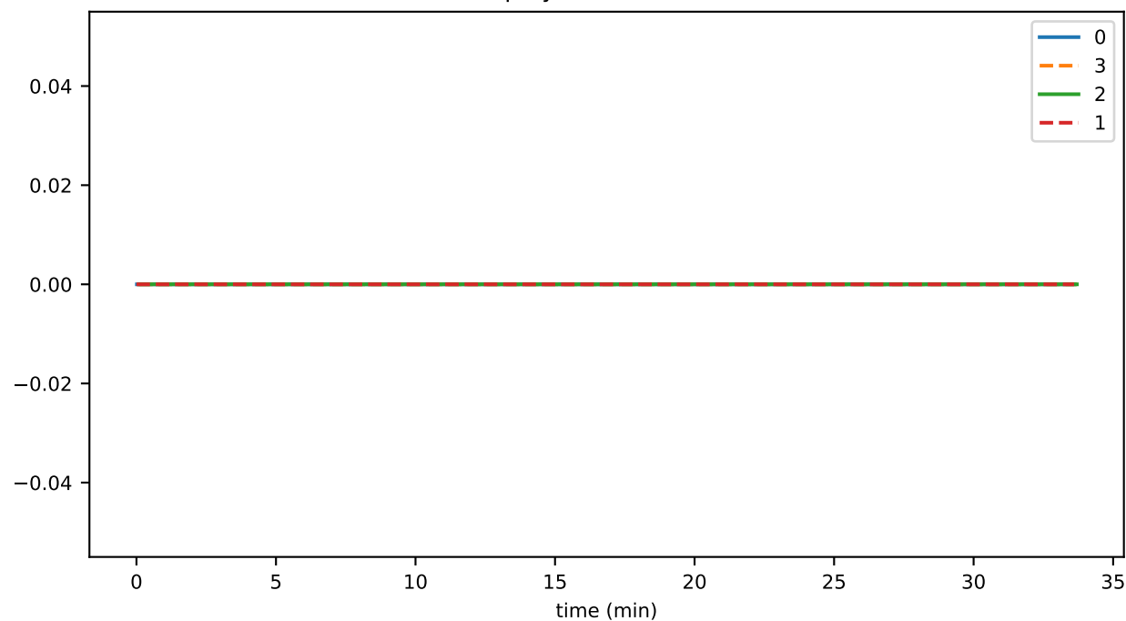
hapiFreeQueryLimitsPercentUsed
