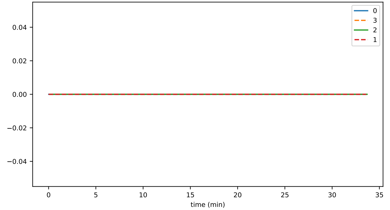
ds_files_level_5_leafKeysFileSizeByLevelMb_state
