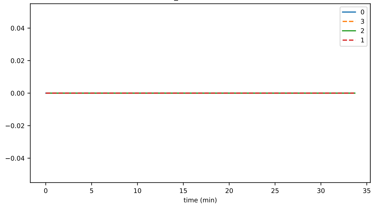
buffer_backPressureState
