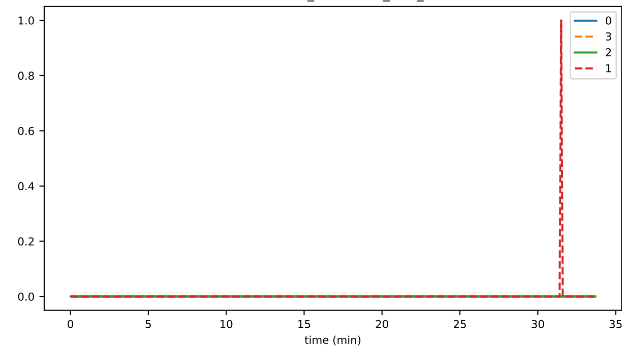
branchingNodeCount
