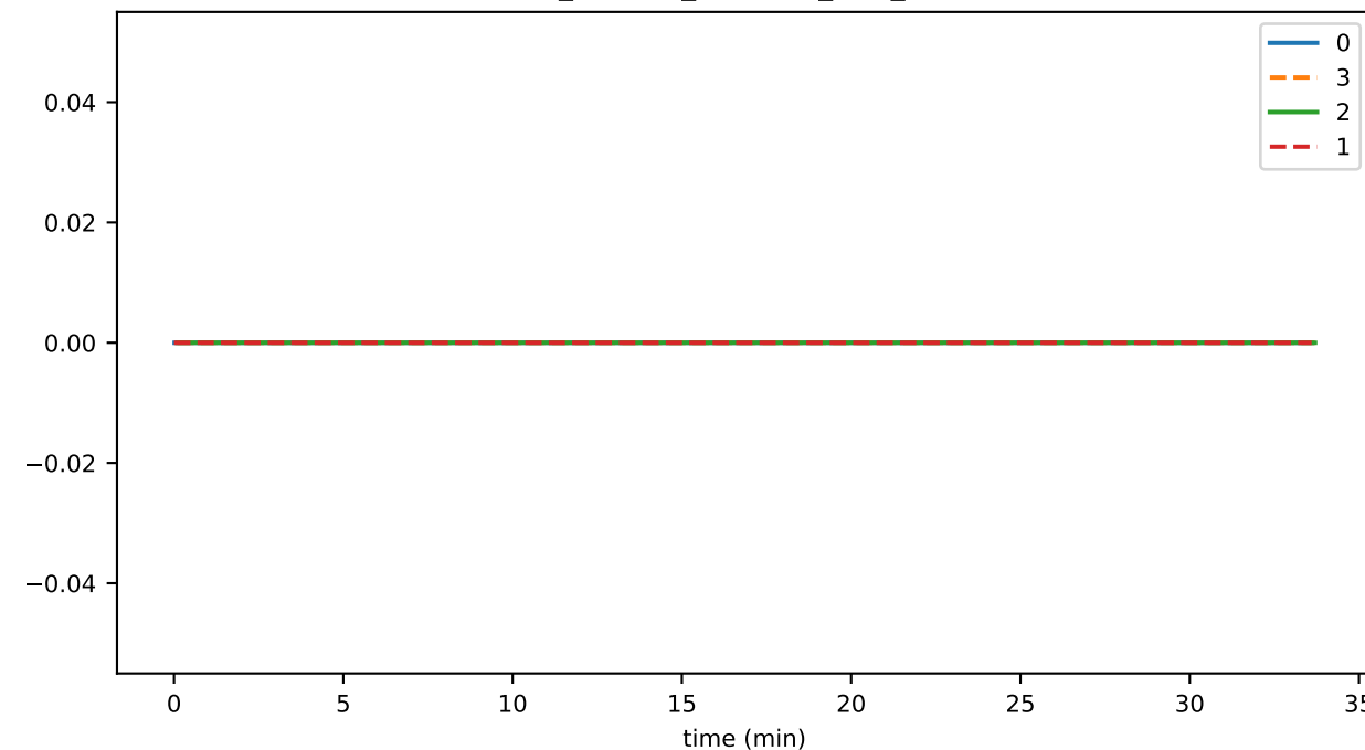
consensus_time_GETTING_STATE_TO_SIGN
