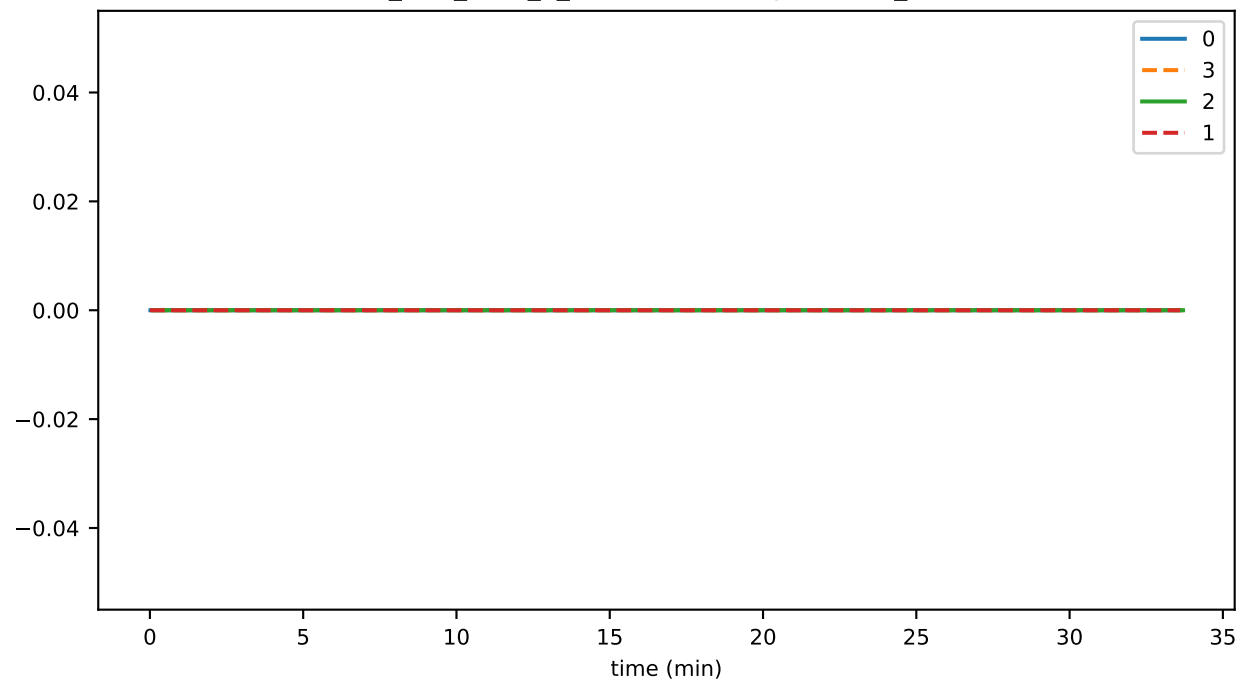
ds_files_level_3_leavesFileSizeByLevelMb_state
