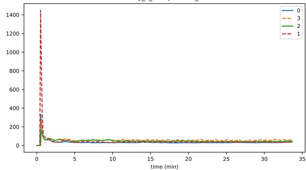
eventDelay_3_deduplication_runtime
