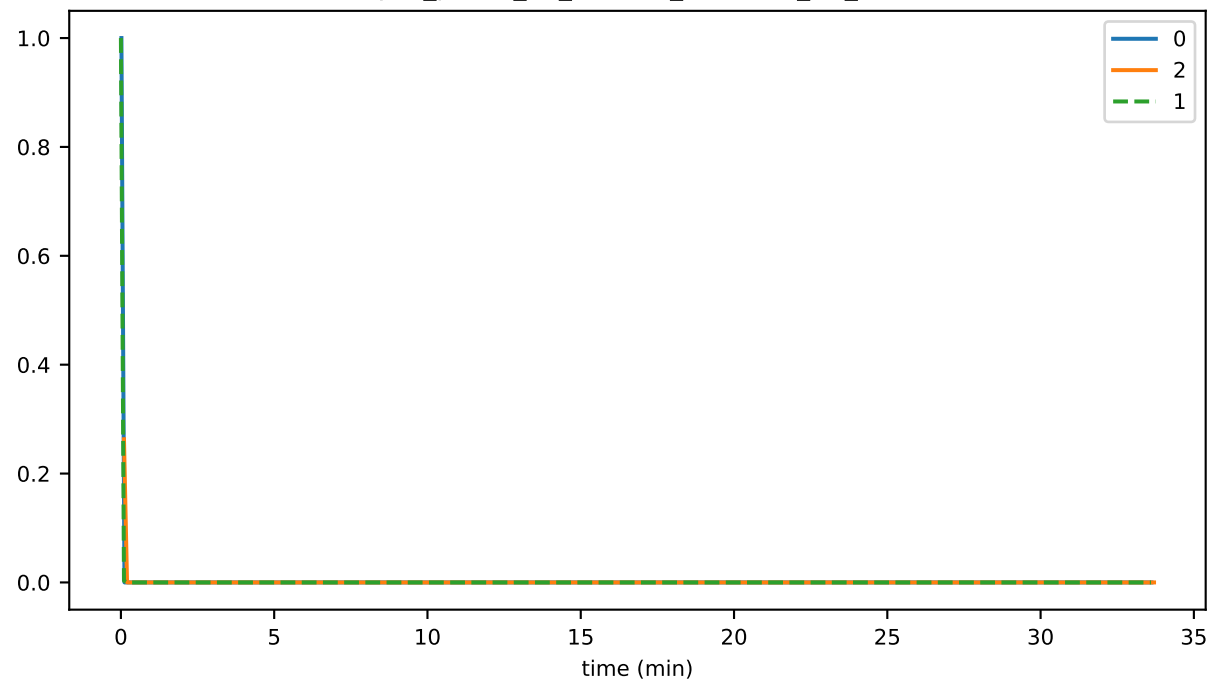
sync_phase_03_fraction_RECEIVING_EVENTS
