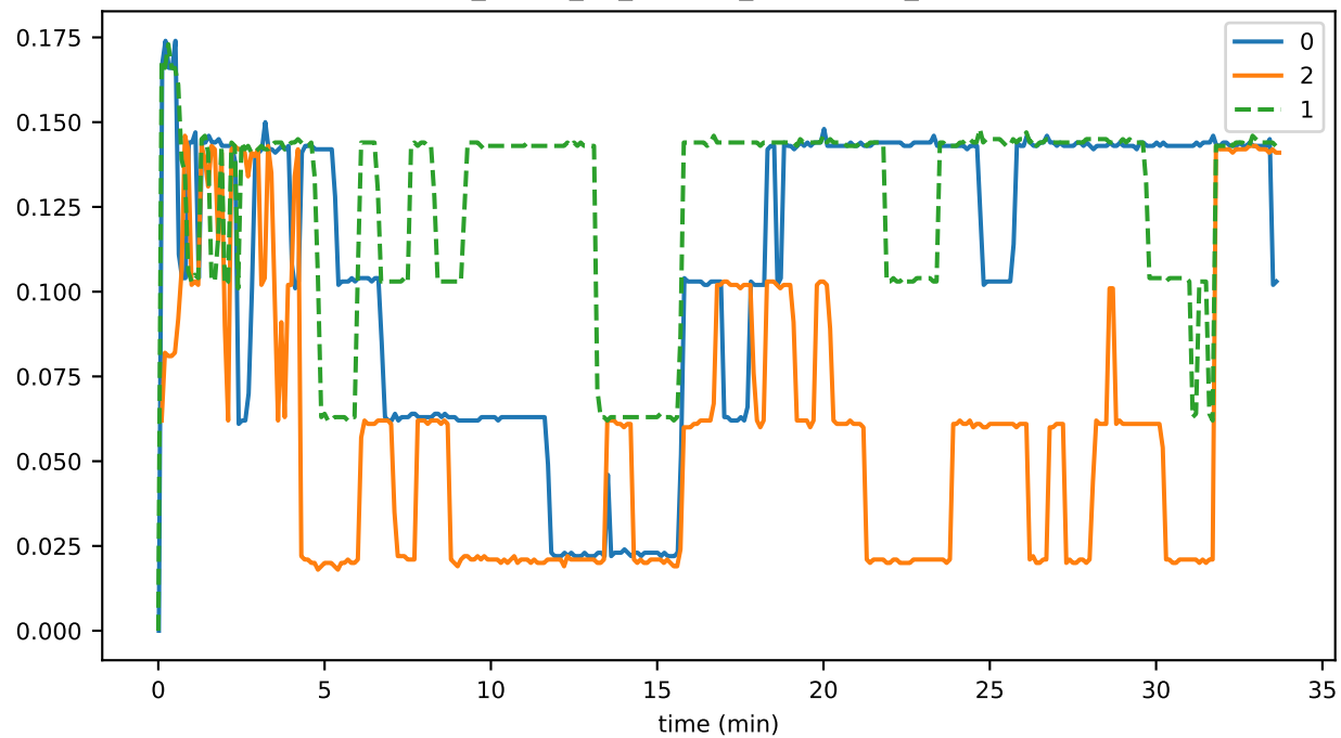
sync_phase_03_fraction_RECEIVING_EVENTS
