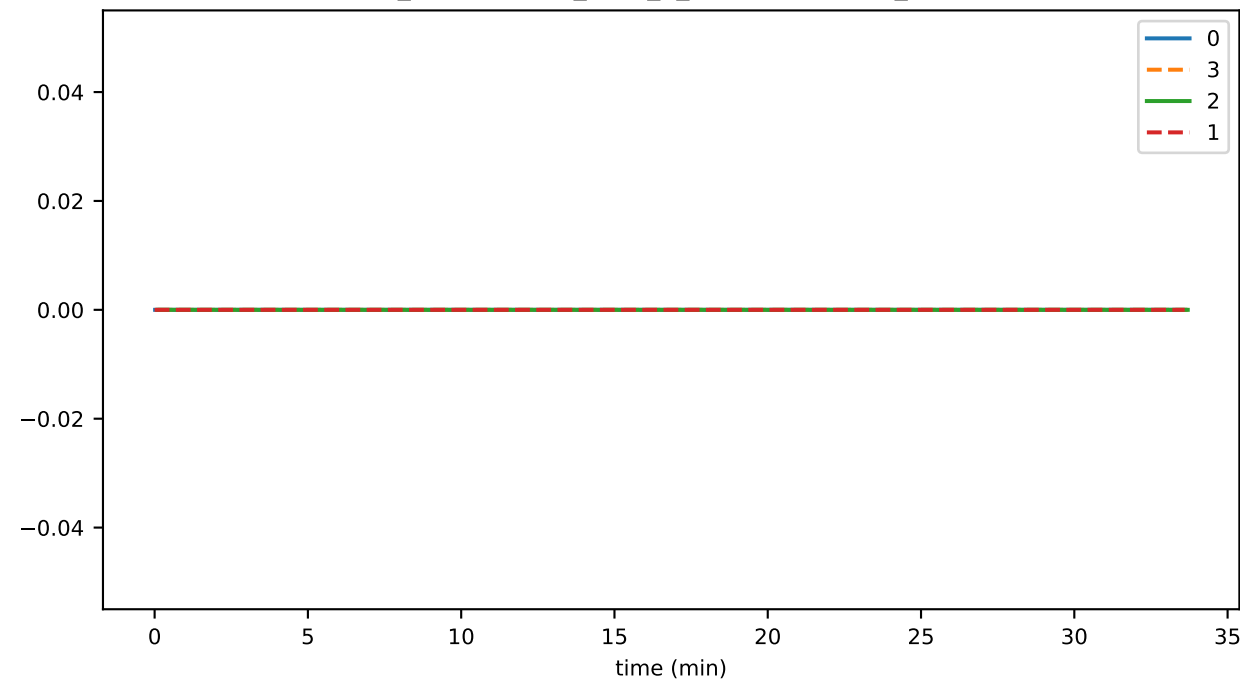
ds_compactions_level_3_leafKeysTimeMs_state
