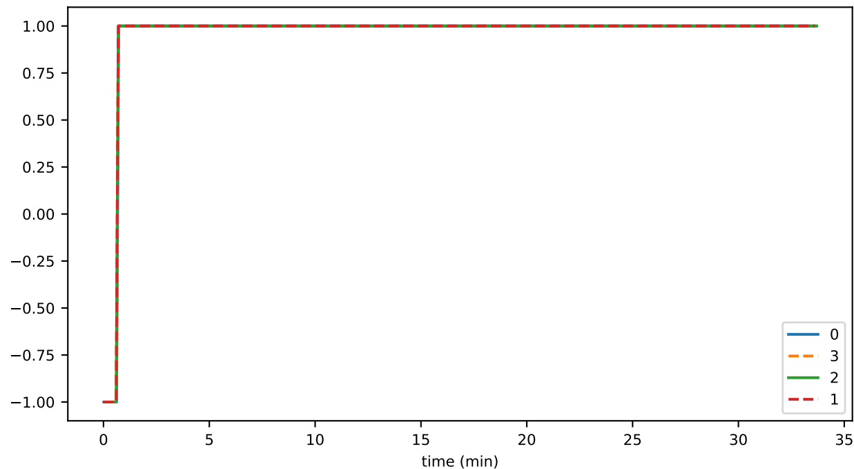
preconsensusEventFileOldestIdentifier
