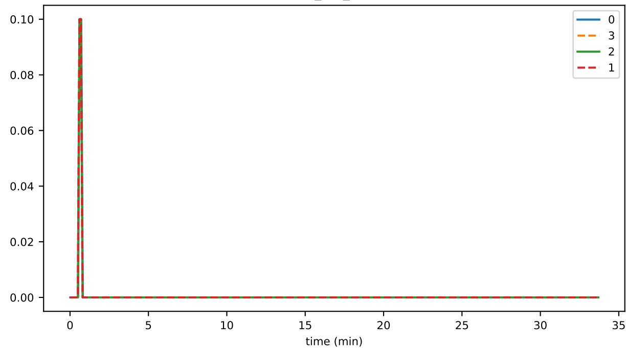
trans_per_event
