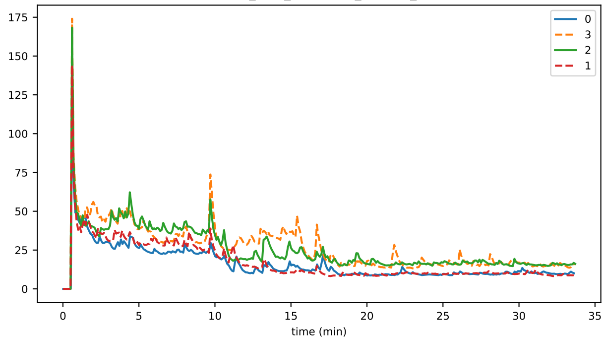
consensus_time_CREATING_SIGNED_STATE
