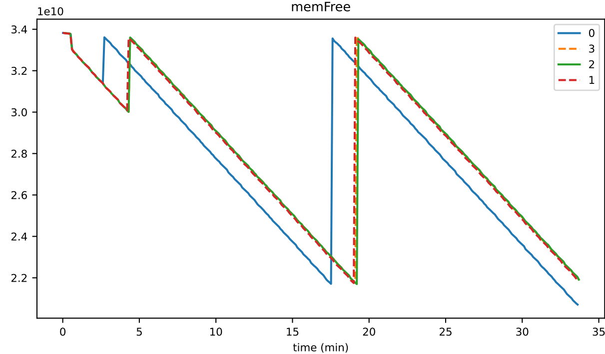
memFree
