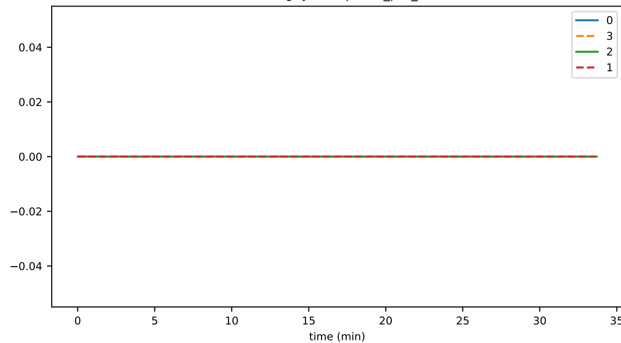
incomingSyncRequests_per_sec
