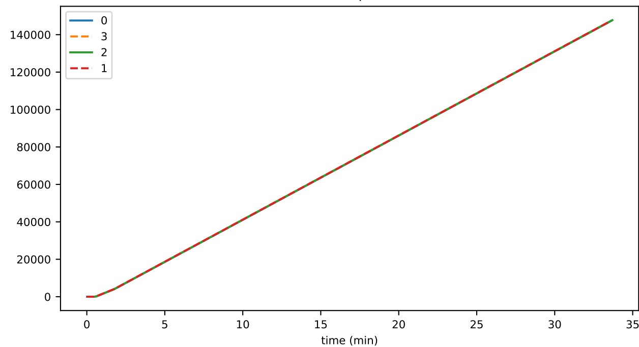
roundIncEqParents
