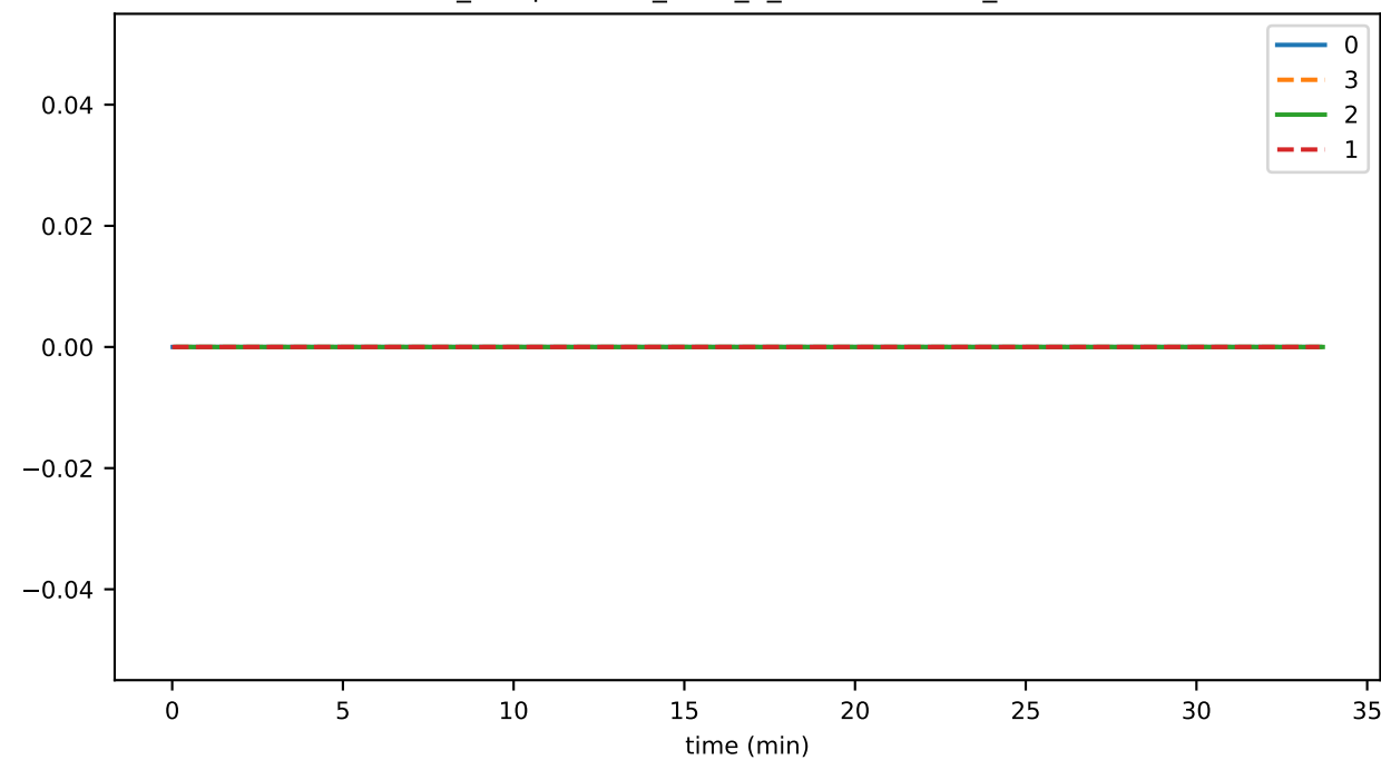
ds_compactions_level_8_leavesTimeMs_state
