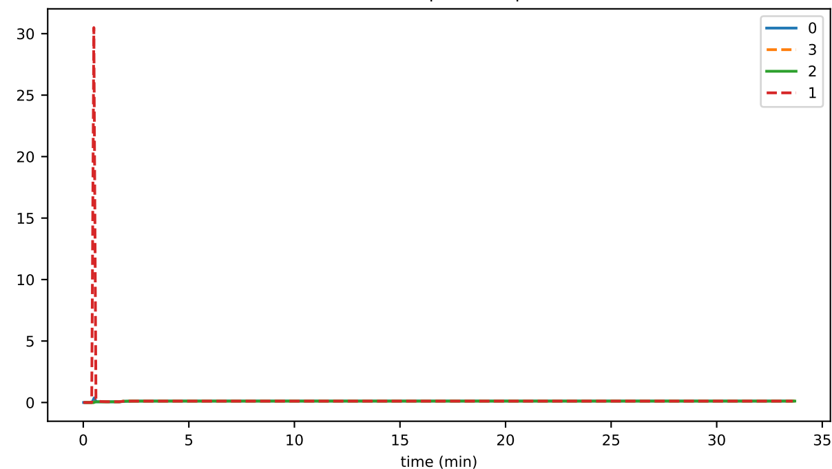
secR2C
