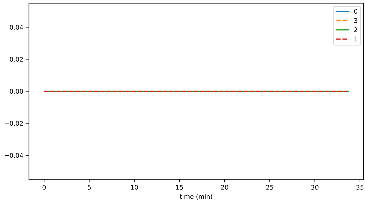
stateSignaturesGathered_per_sec
