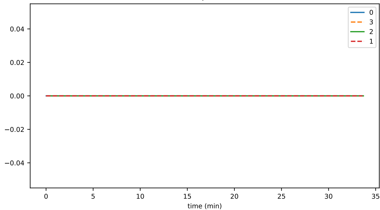
airdropsUsed
