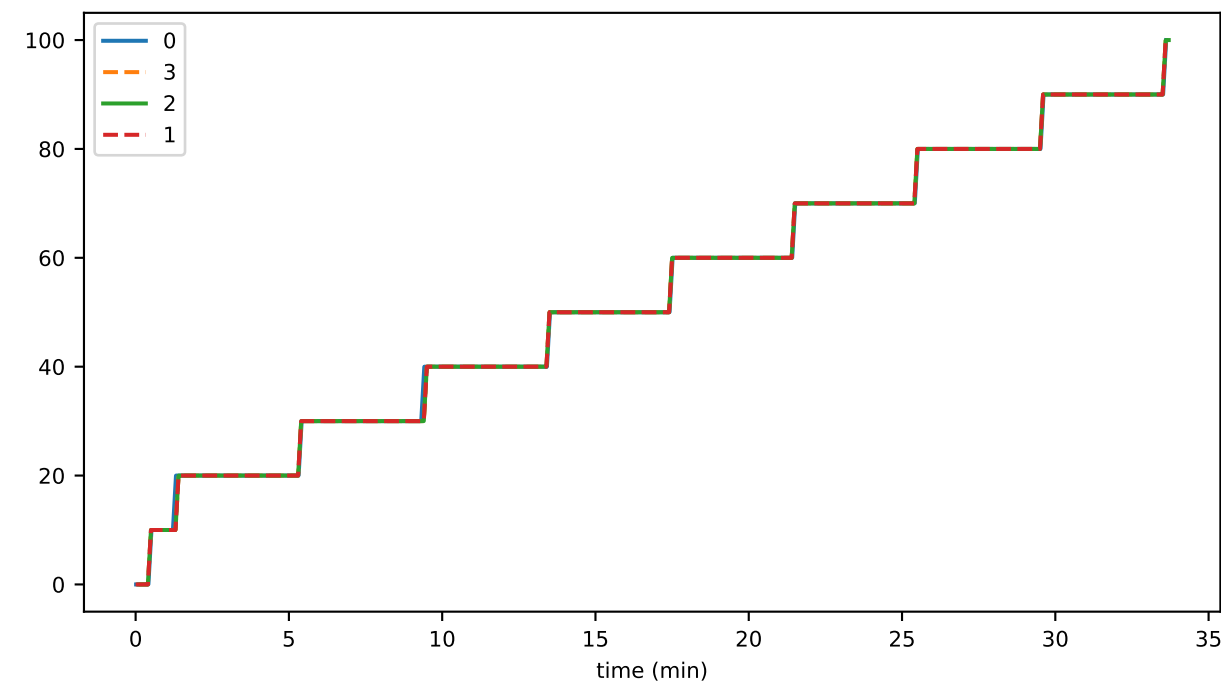
disconnects_per_sec_00
