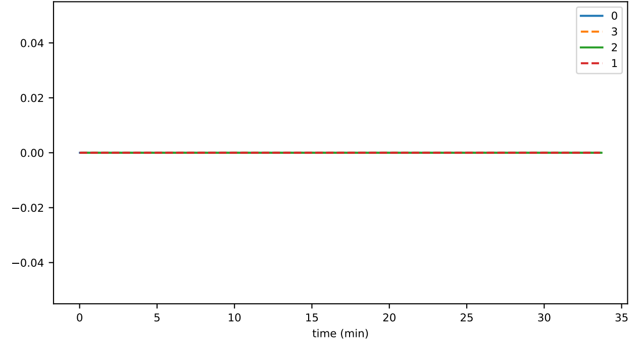
connSend_requestSendLatency
