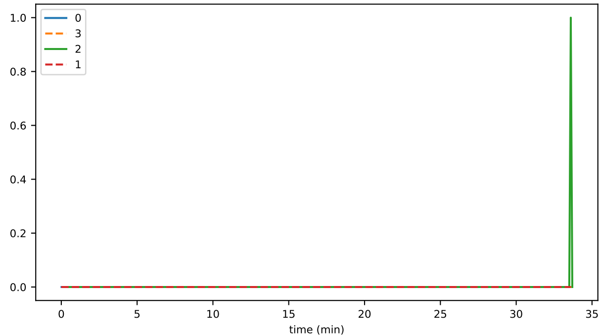
orphanBufferSize
