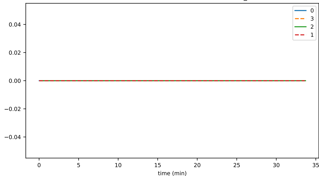
SmartContractService:OpsDuration_PerTxn_avg
