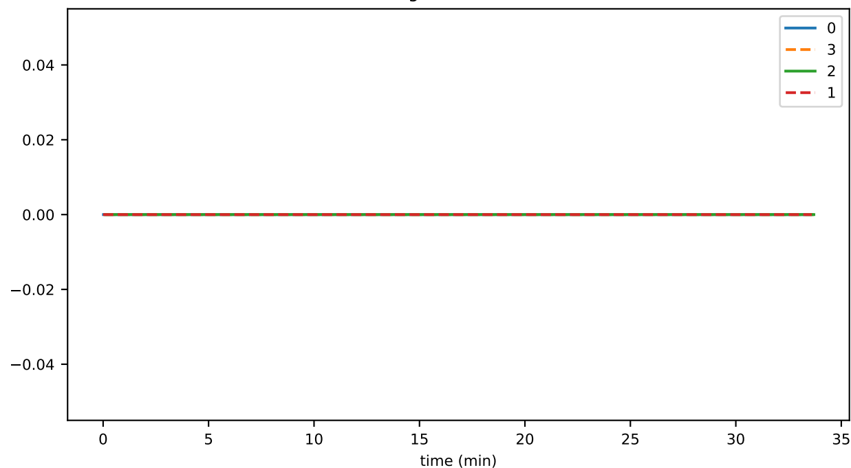
hintsSigningSuccessMsAvg
