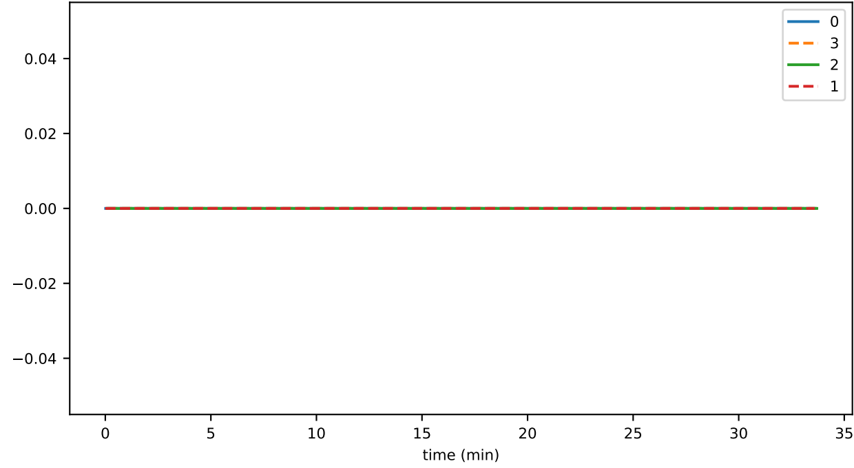
ds_reads_hashes_state
