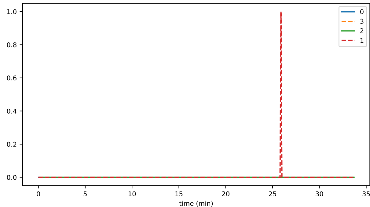
StateSigner_unhandled_task_count
