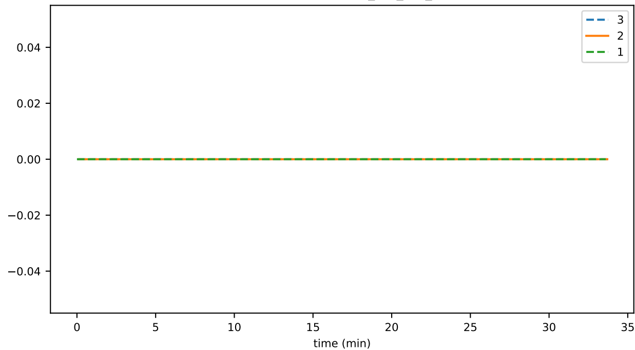
reconnectRejections_per_sec_00
