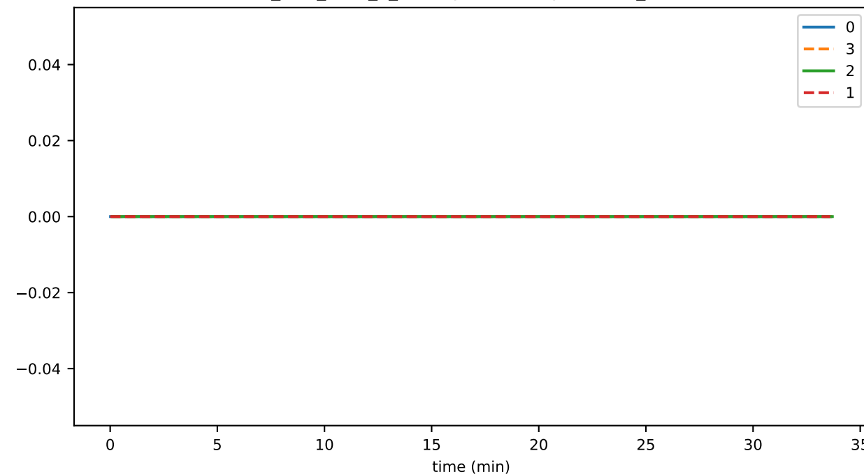
ds_files_level_4_hashesFileSizeByLevelMb_state
