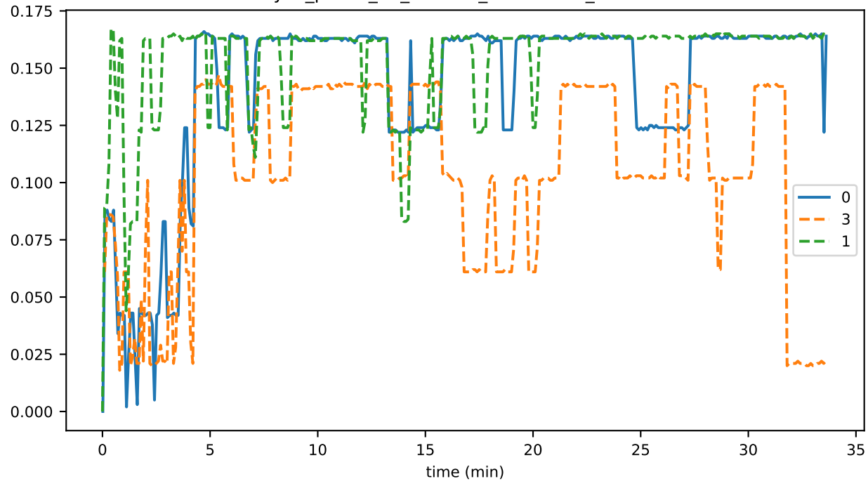
sync_phase_02_fraction_RECEIVING_EVENTS
