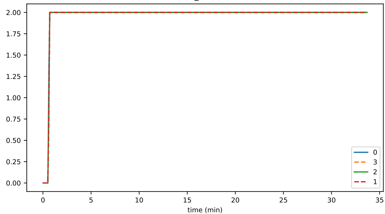
buffer_saturation
