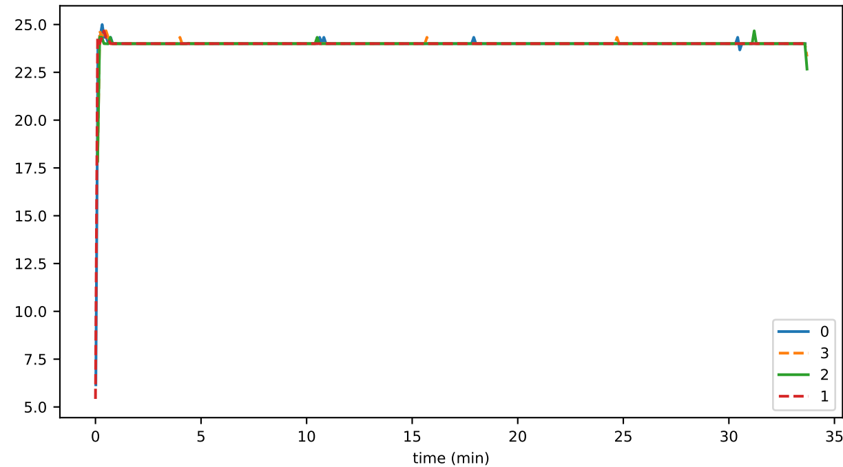
outgoingSyncRequests_per_sec
