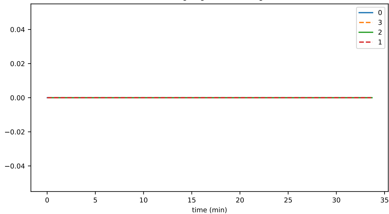
hintsSigningSuccessMsAvg
