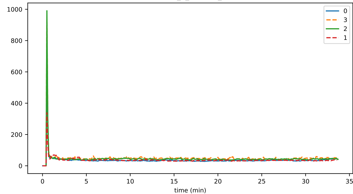
eventDelay_1_hashing_gossip
