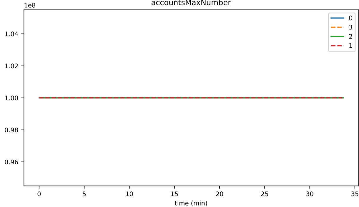
accountsMaxNumber
