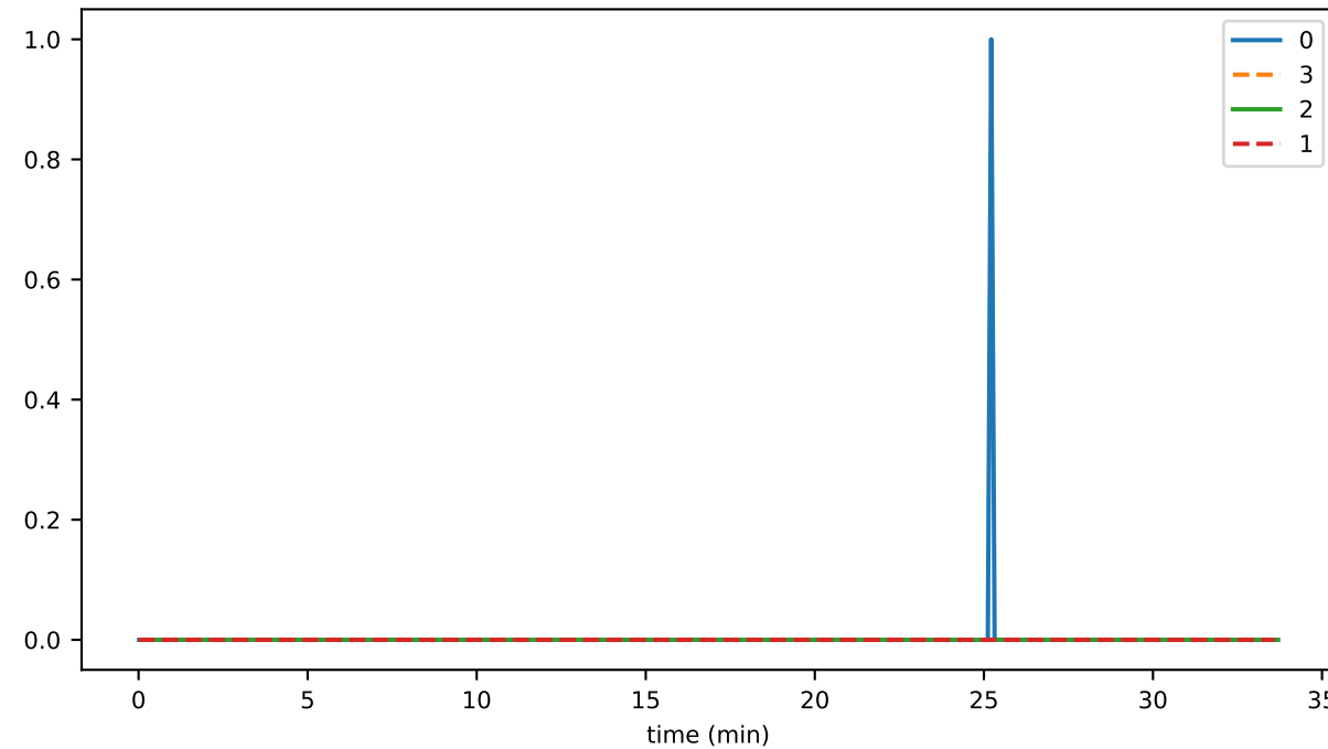
ds_compactions_level_2_leavesTimeMs_state
