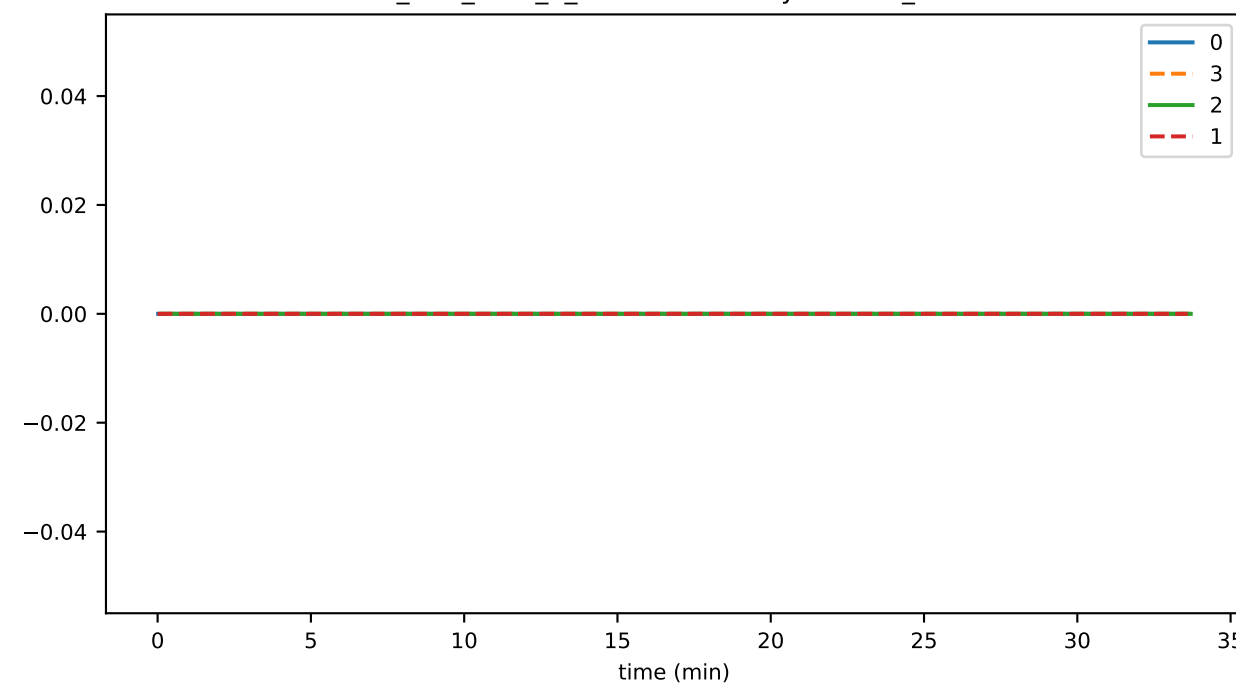
ds_files_level_4_hashesFileSizeByLevelMb_state
