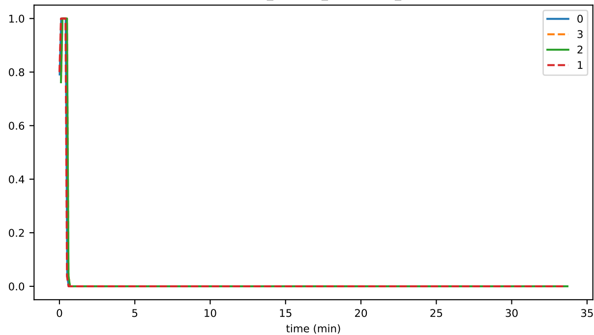
eventCreation_fraction_PLATFORM_STATUS
