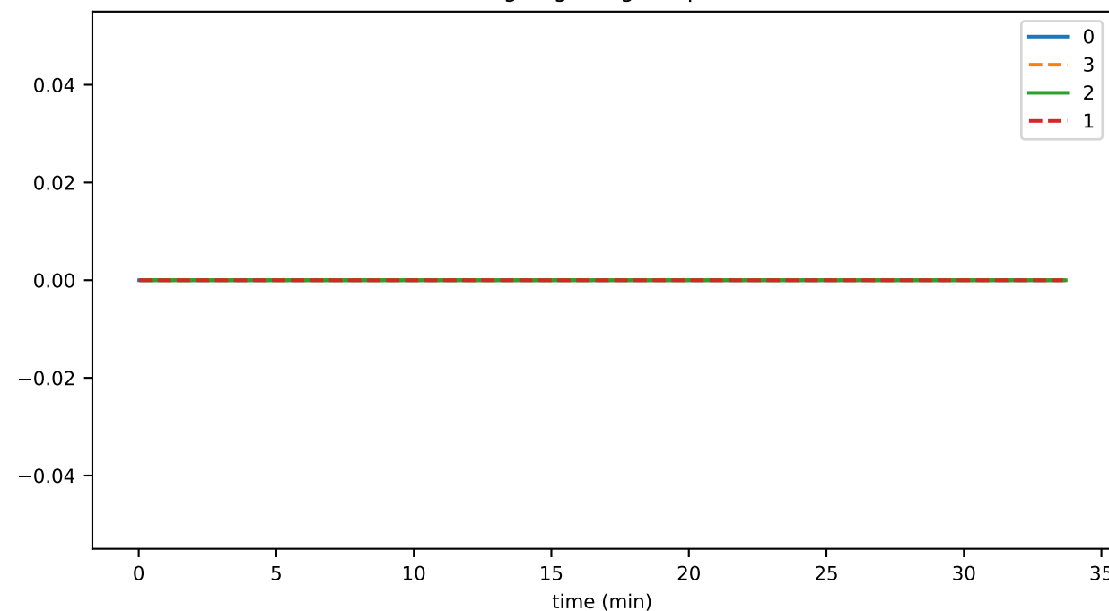
incomingSyncRequests_per_sec
