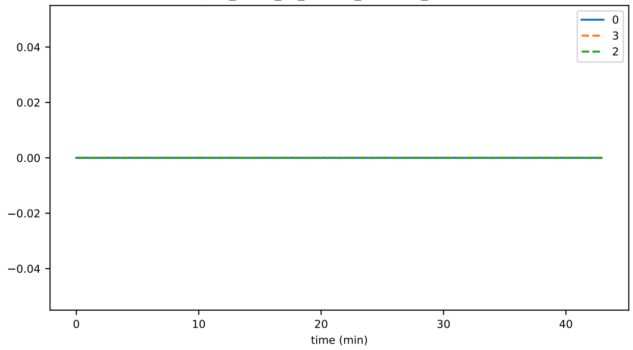
sync_phase_02_fraction_EXCHANGING_TIPS
