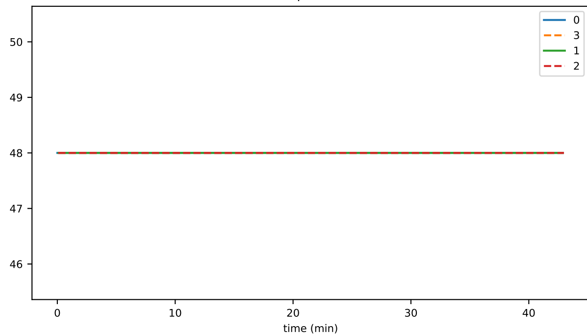
reconnectRejections_per_sec_00
