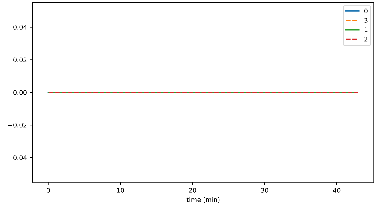
doNotSyncIntakeCounter
