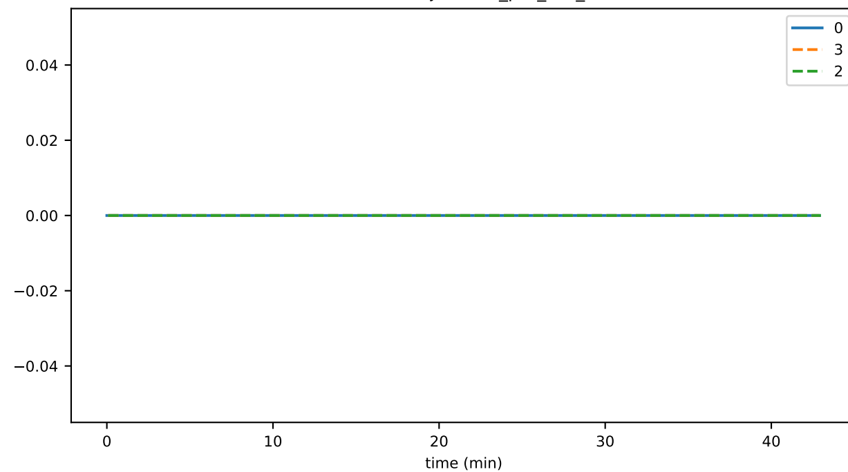
reconnectRejections_per_sec_01
