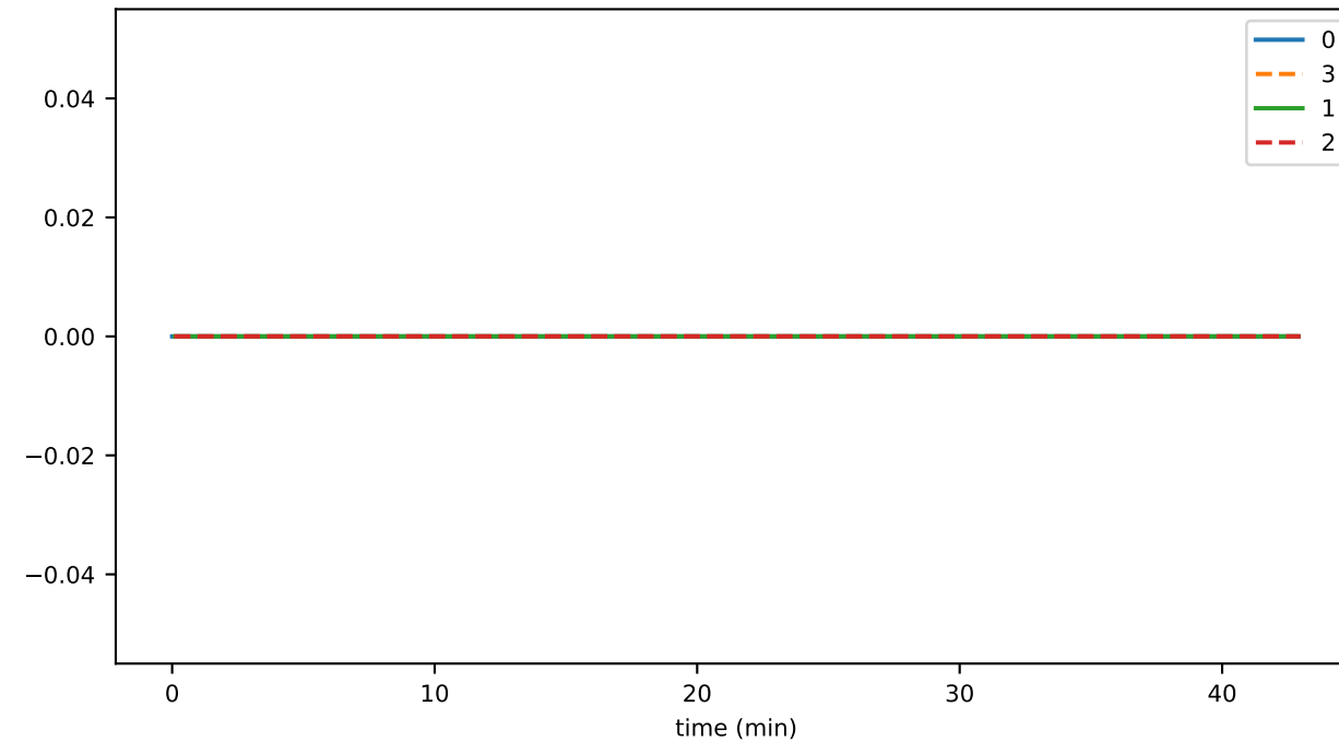
SmartContractService:SystemContractMethodCall_TRANSFER_failed
