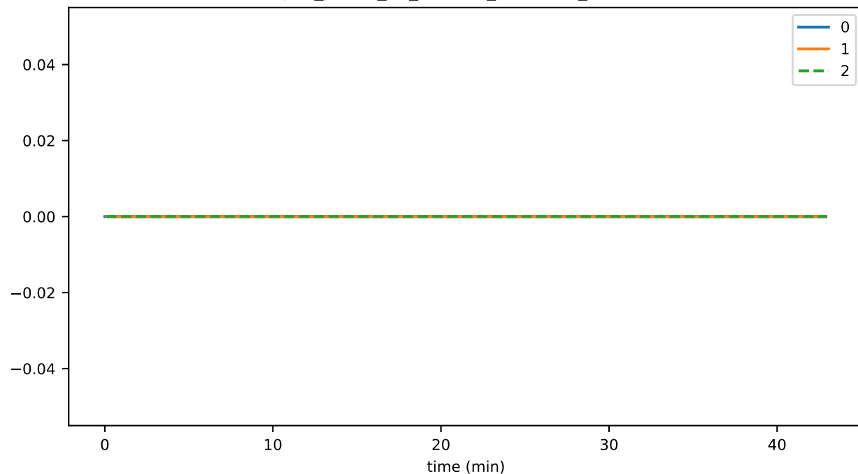
syncIndicatorDiff
