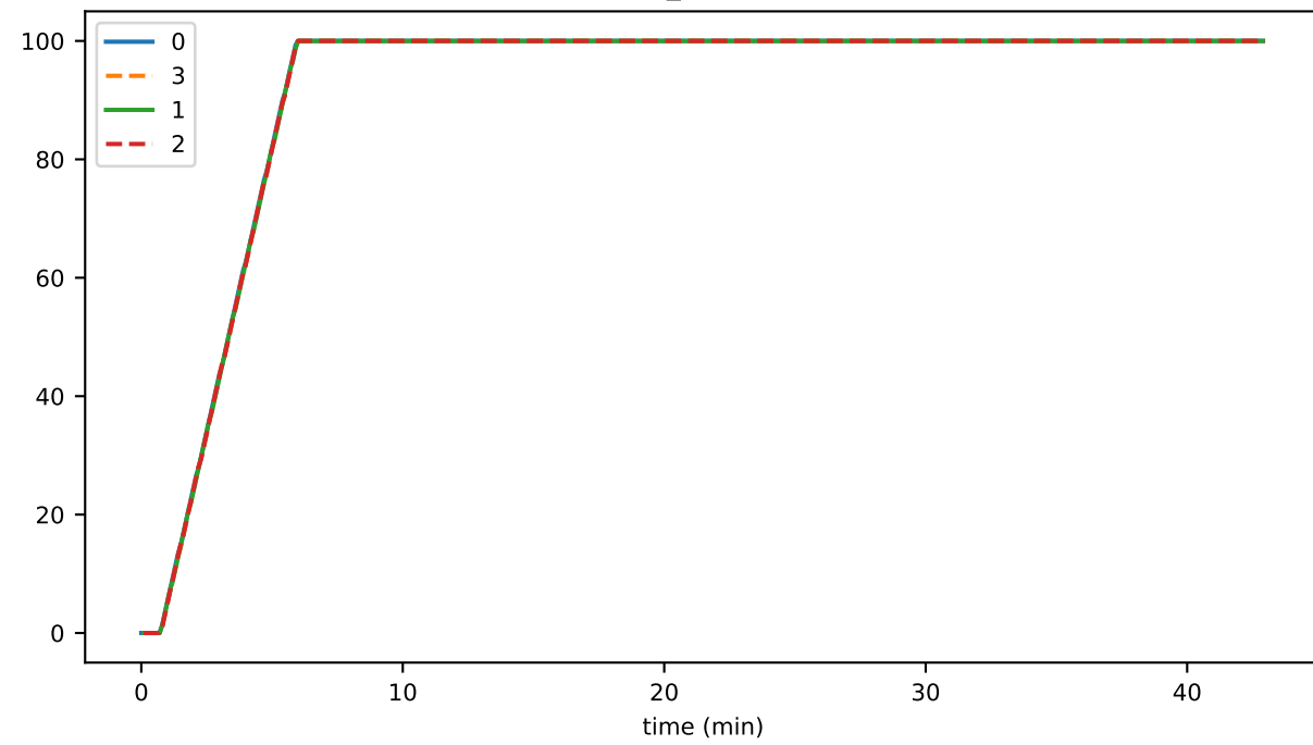
buffer_saturation
