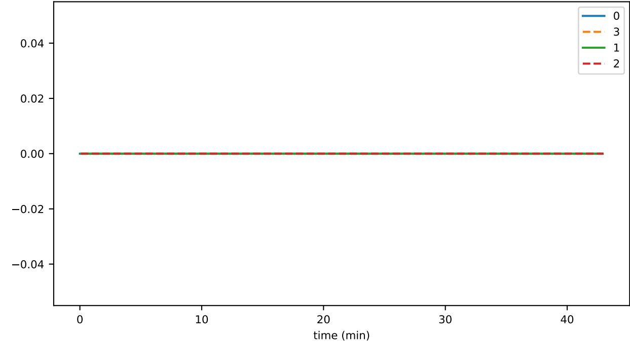
SmartContractService:SystemContractMethodCall_APPROVAL_failed
