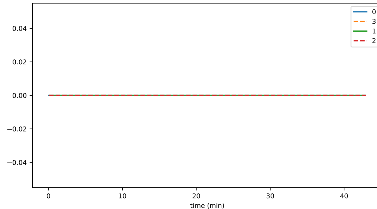
ds_files_level_9_leafKeysFileSizeByLevelMb_state
