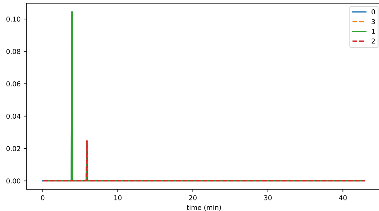
ds_compactions_level_2_leavesSavedSpaceMb_state
