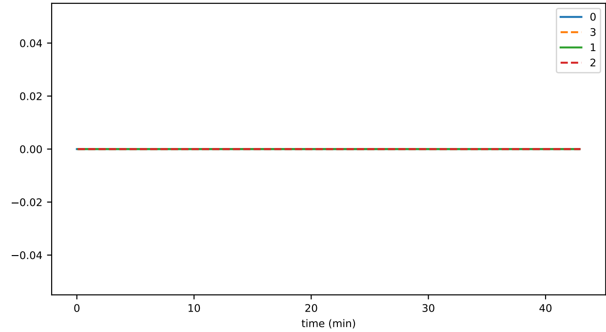
connSend_endStream_tooFarBehind
