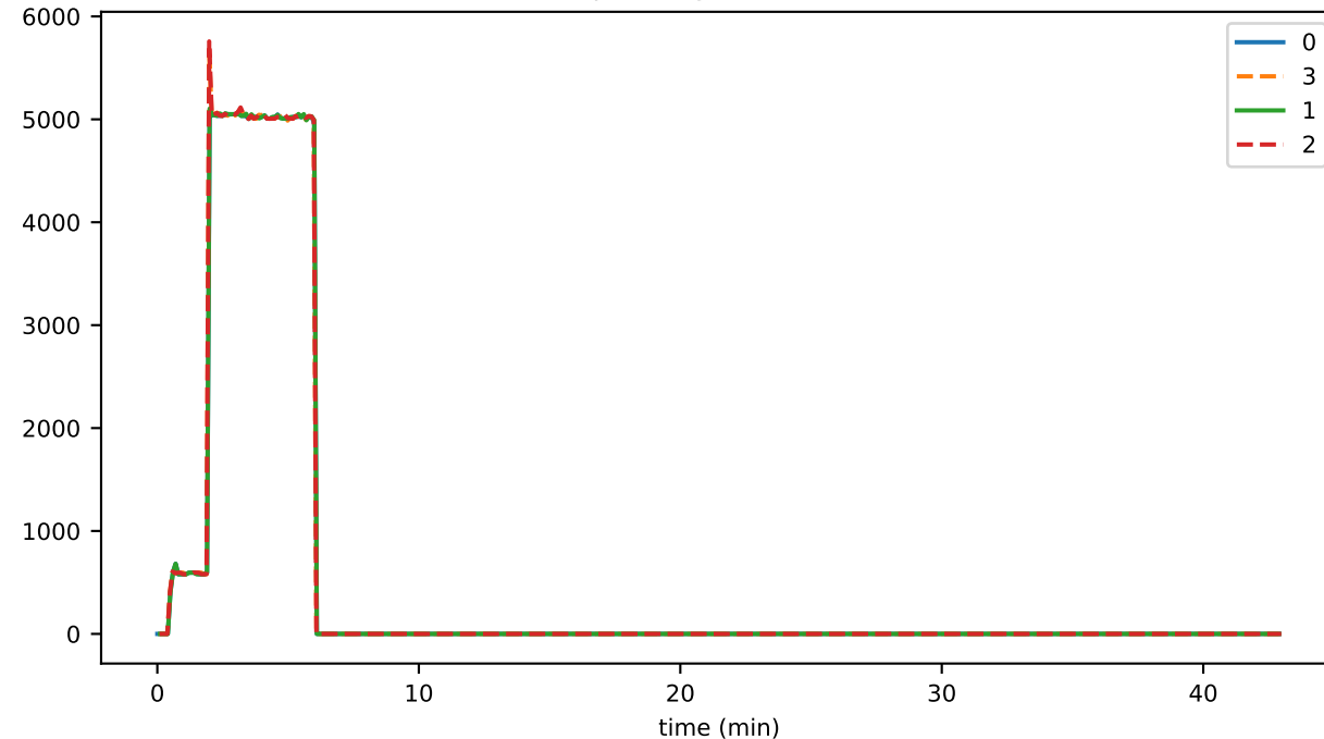
pcesAvgTotalWriteDuration
