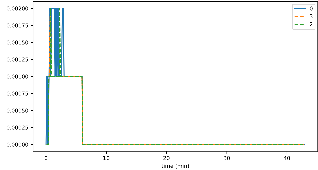
sync_phase_01_fraction_EXCHANGING_WINDOWS
