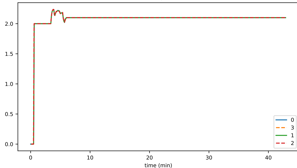
oldestSignedStateSeconds
