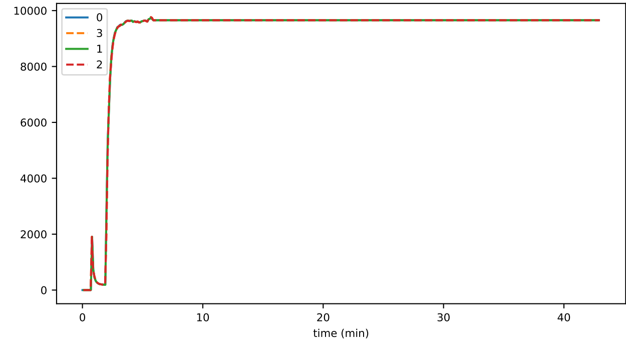
buffer_latestBlockOpened
