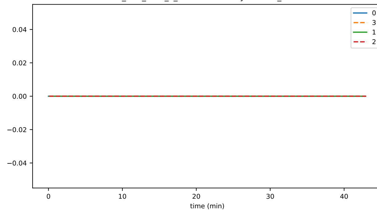
ds_files_level_4_hashesFileSizeByLevelMb_state
