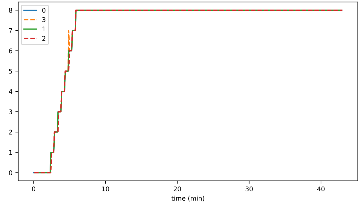
ds_flushes_hashesWritten_state
