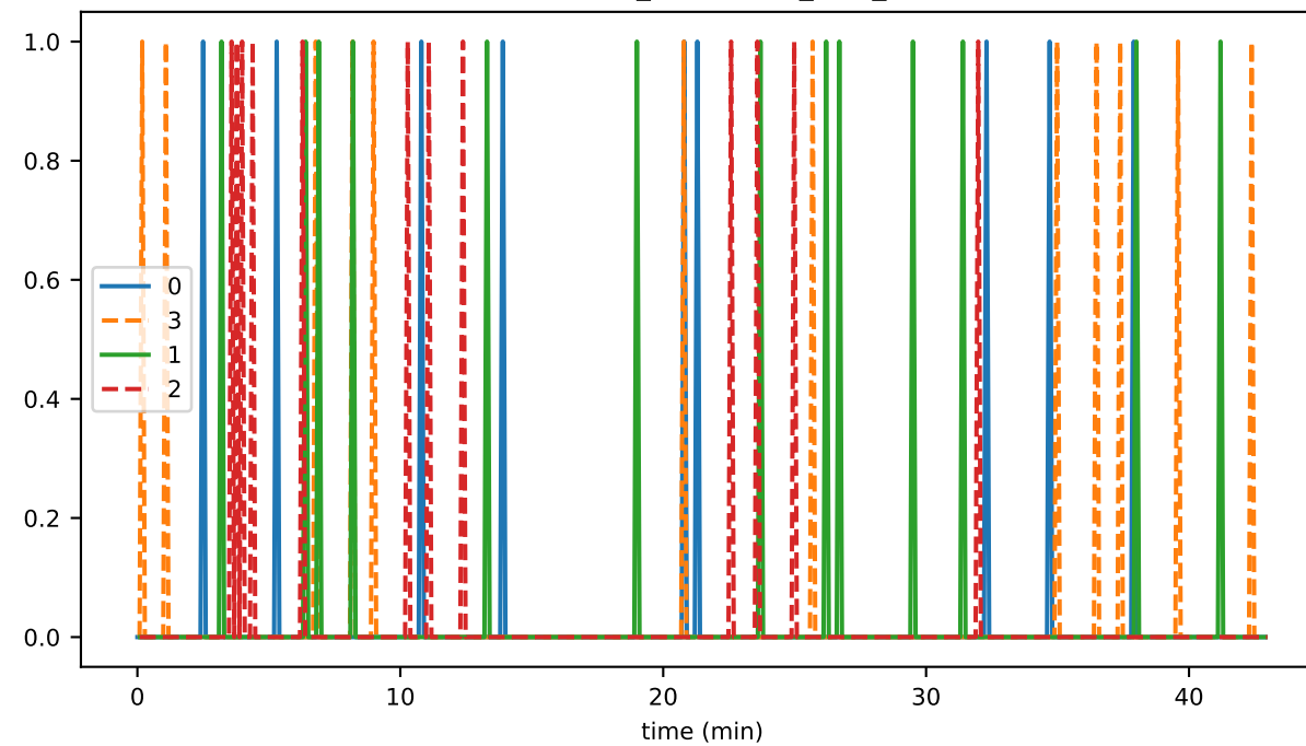
healthyNetworkFraction
