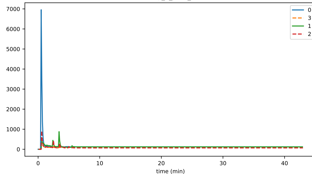
eventDelay_6_pces_storage
