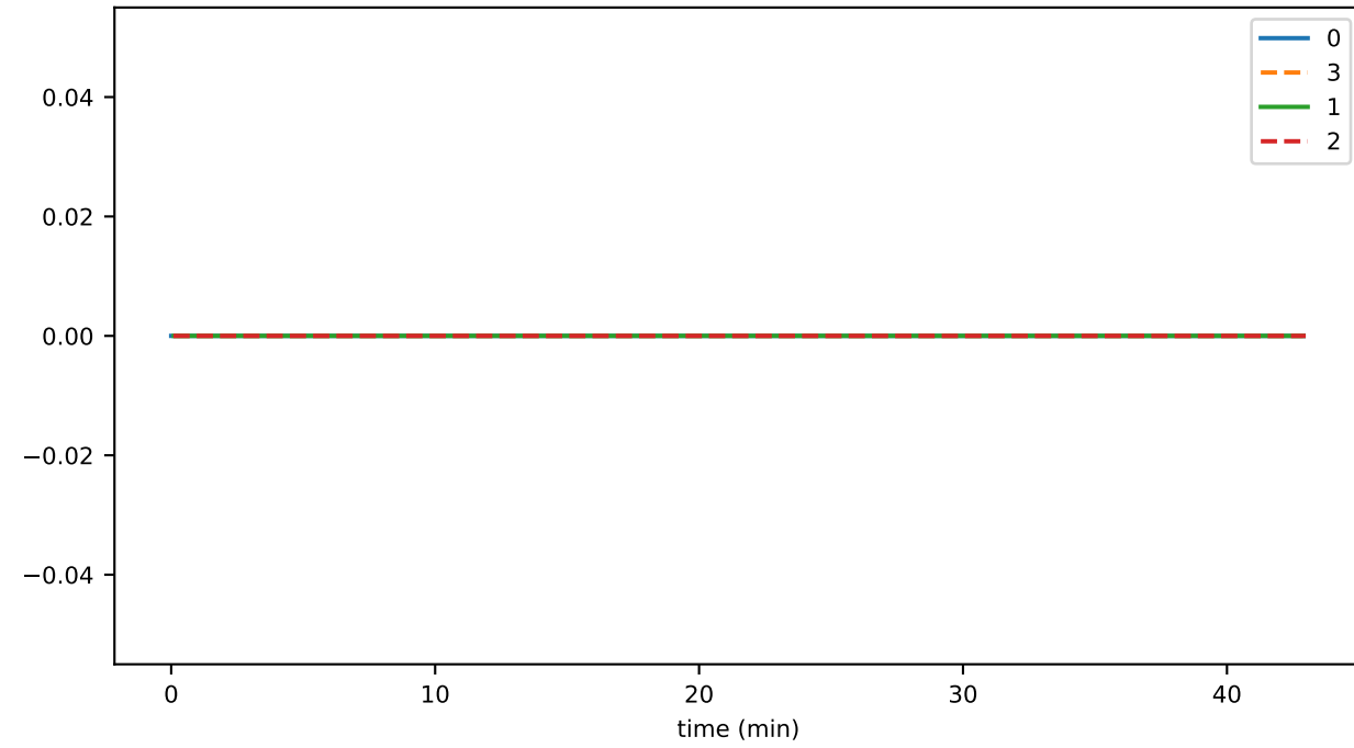
connSend_blockItems
