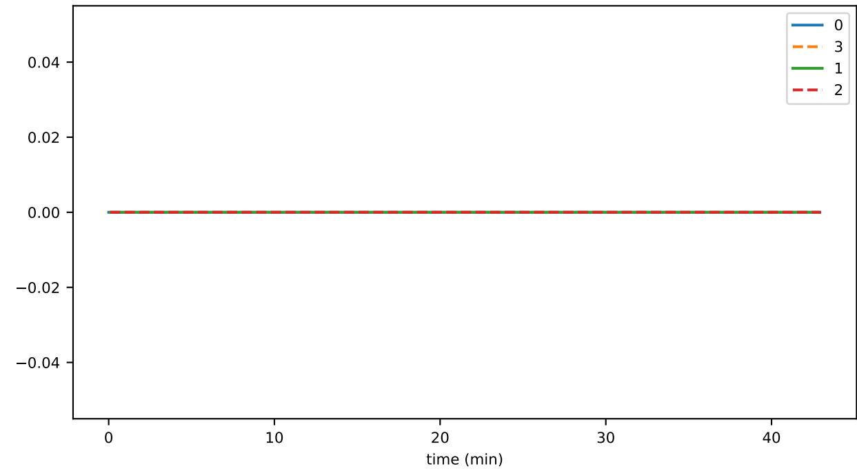
connSend_requestSendLatency
