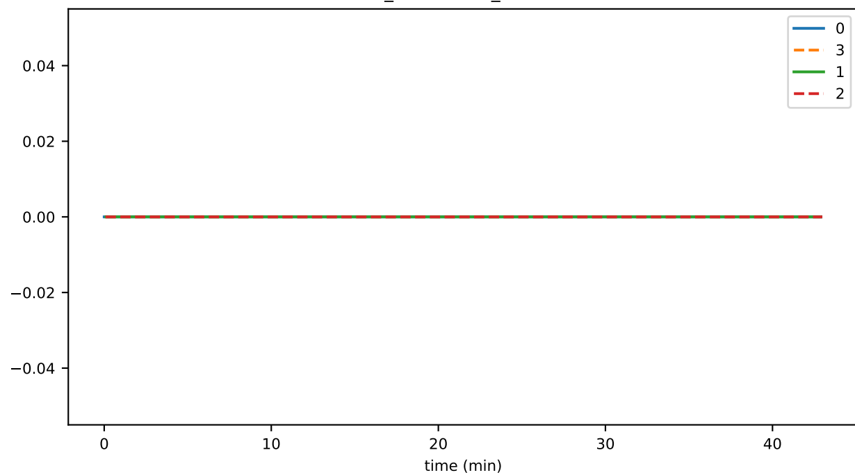
connRecv_endStream_error
