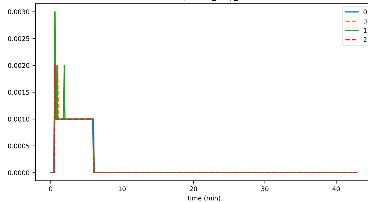
EventDeduplicator_busy_fraction
