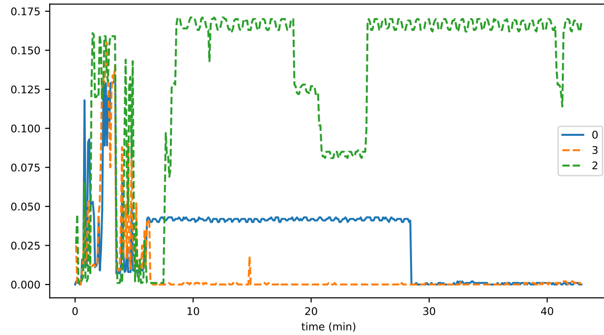
sync_phase_01_fraction_EXCHANGING_TIPS
