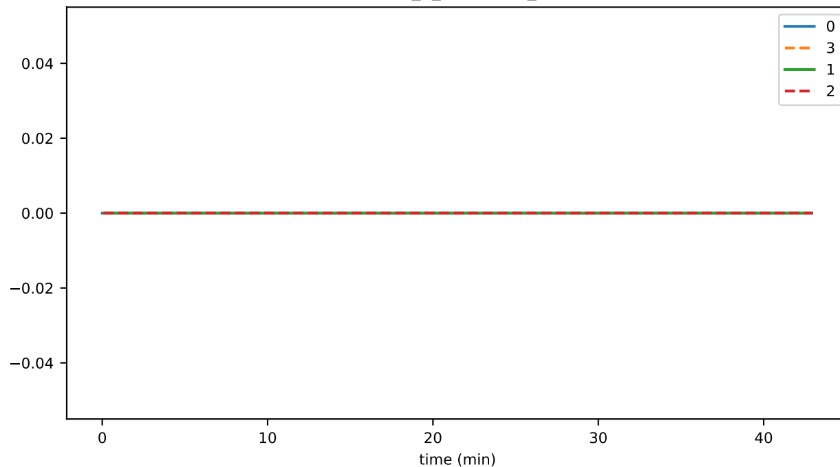
eventDelay_2_validation_storage
