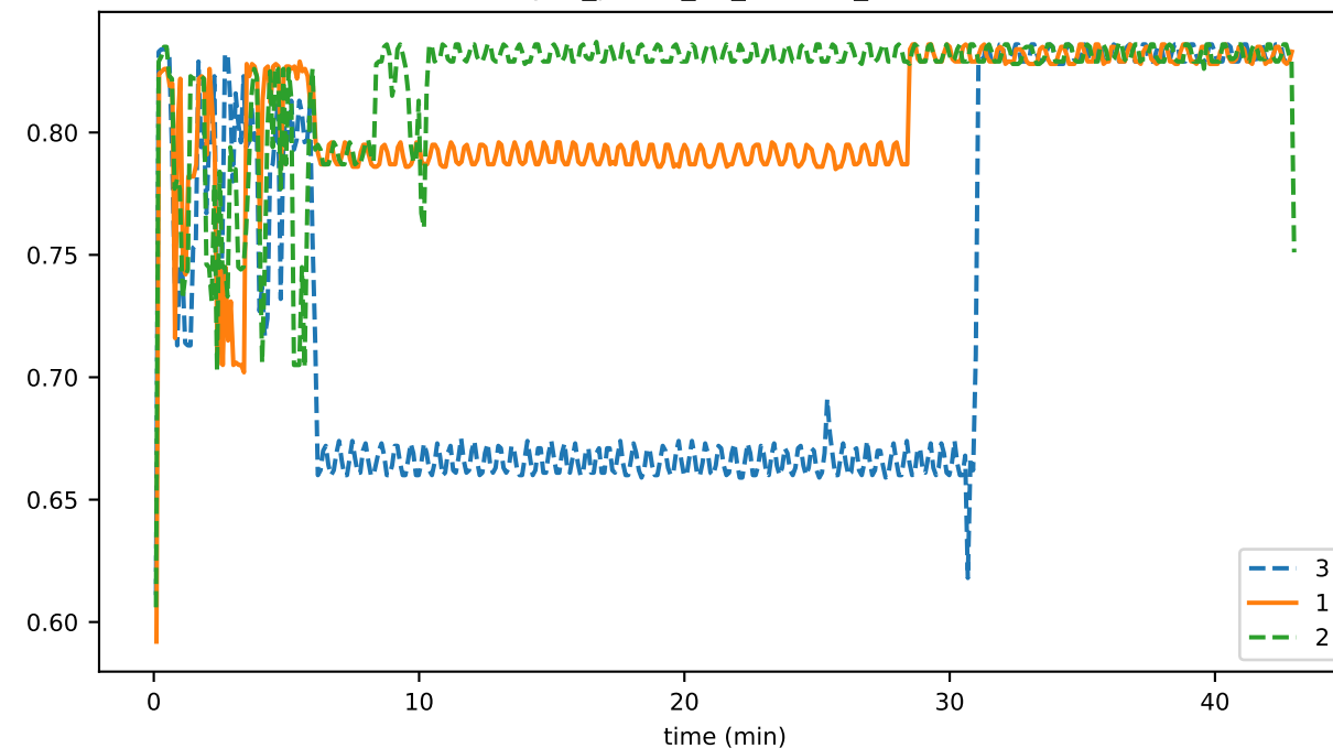
sync_phase_00_fraction_OTHER_FALLEN_BEHIND
