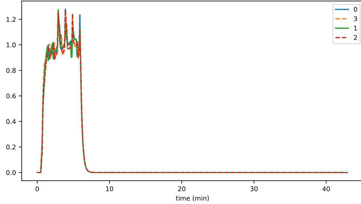
submittedPlatformTransactions
