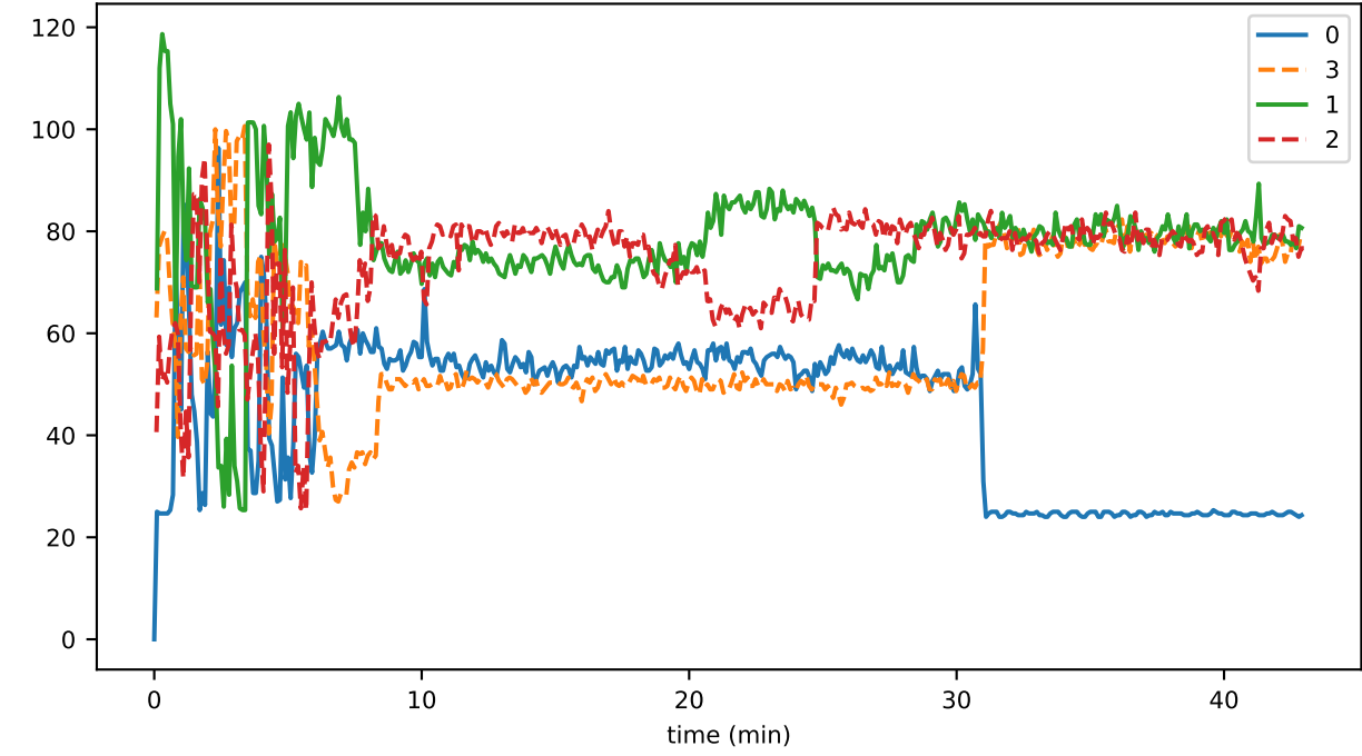
doNotSyncRemoteProcessingEvents
