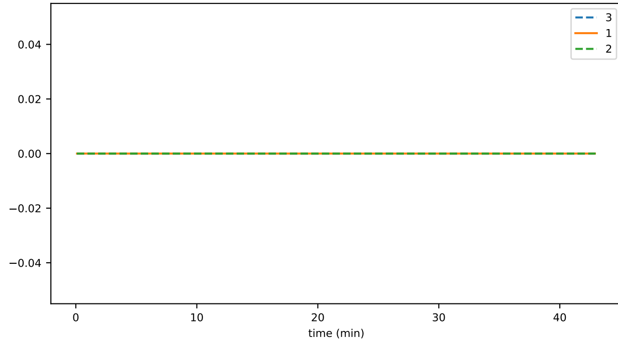
sync_phase_01_fraction_EXCHANGING_TIPS
