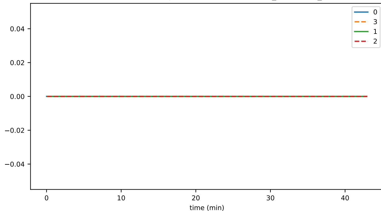
SmartContractService:SystemContractMethodCall_ASSOCIATION_total
