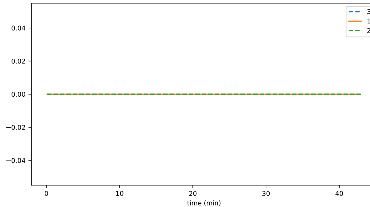
sync_phase_00_fraction_SELF_FALLEN_BEHIND
