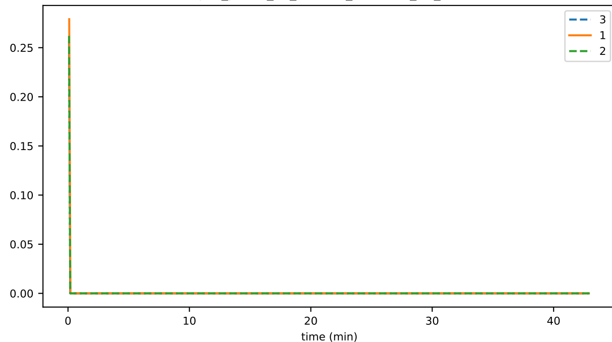
sync_phase_00_fraction_RECEIVING_EVENTS
