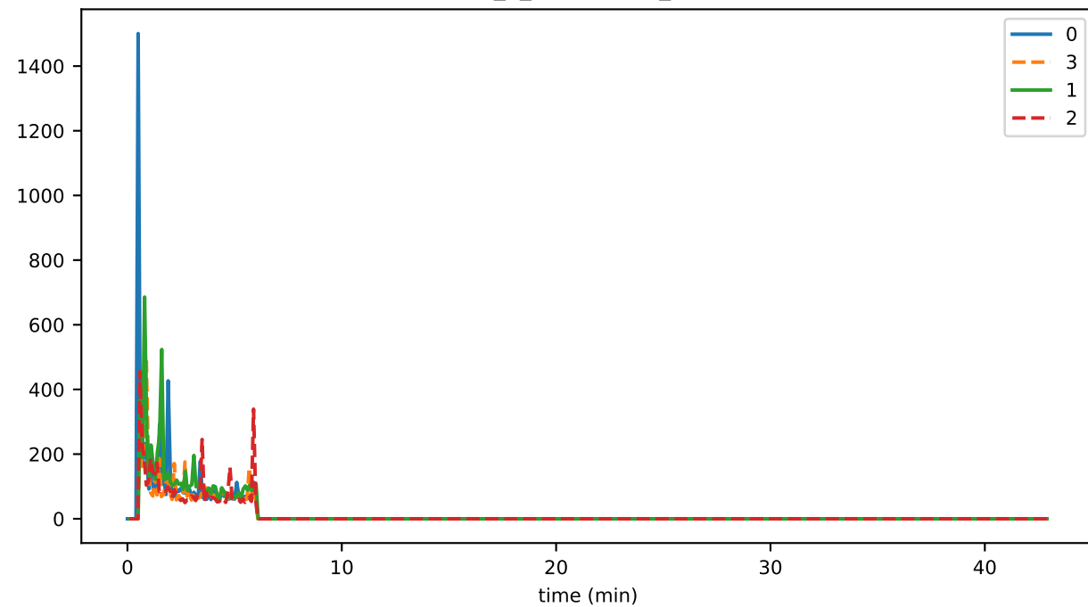
eventDelay_4_verification_runtimeMAX
