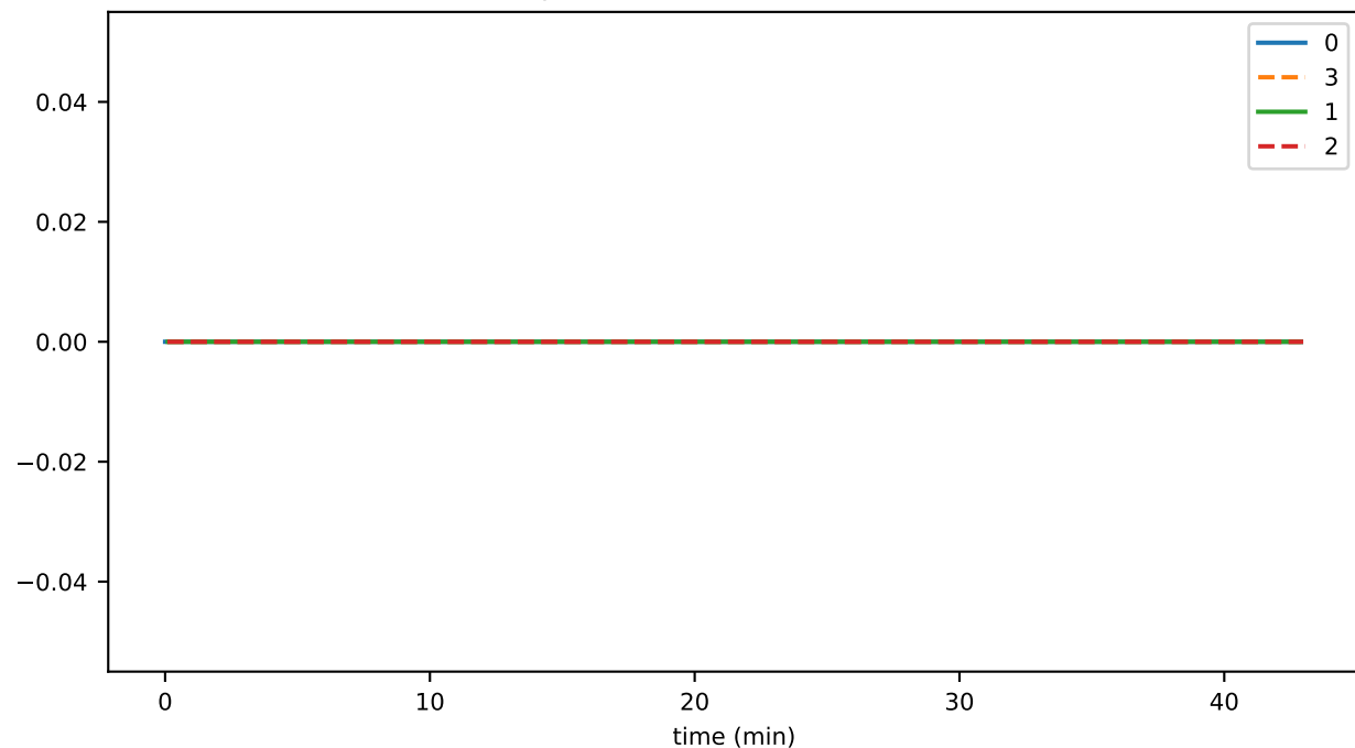
pcesAvgSyncDuration
