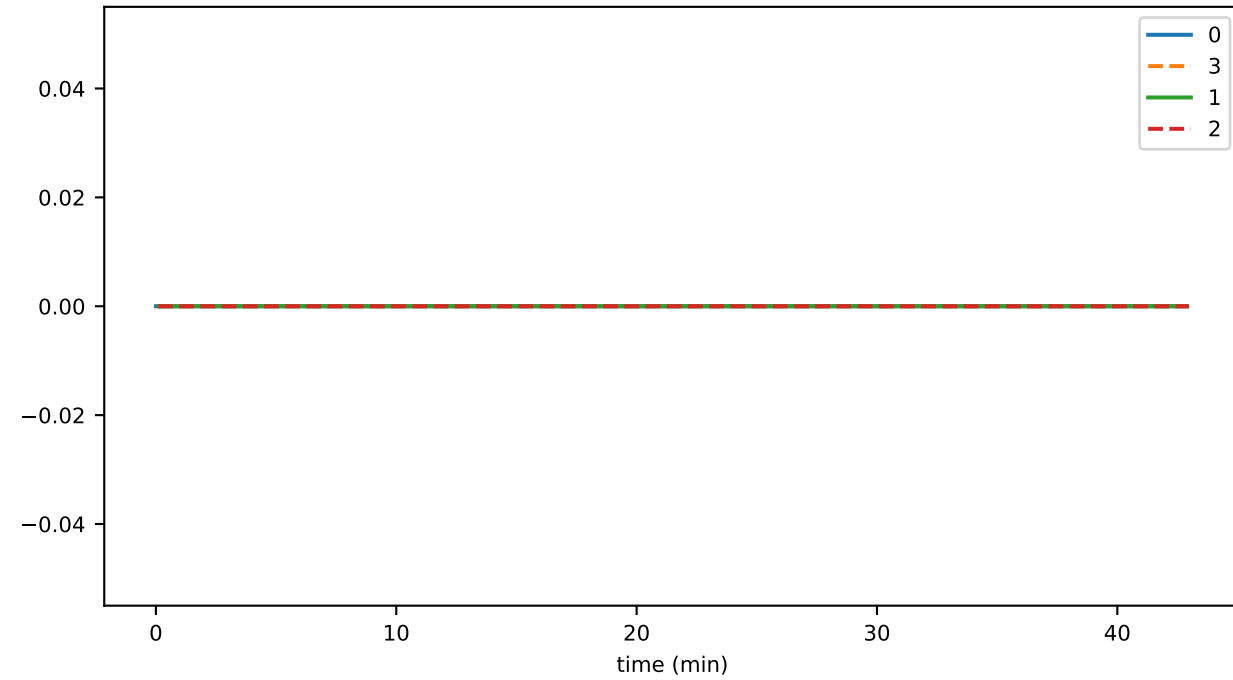
submittedPlatformTransactions
