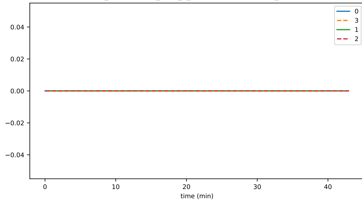
ds_compactions_level_6_hashesSavedSpaceMb_state
