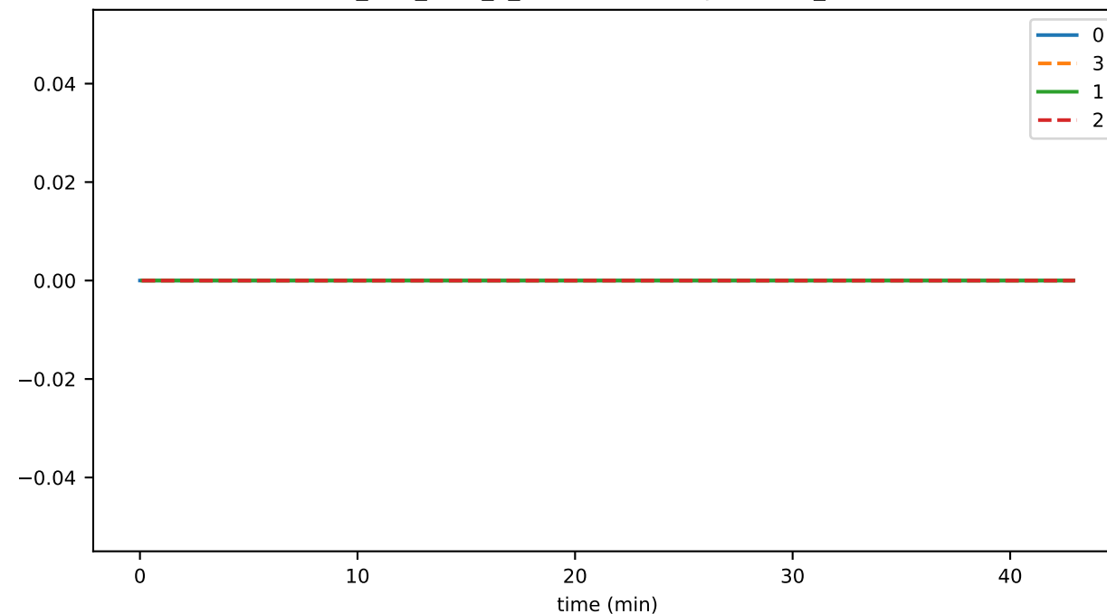
ds_files_level_2_leavesFileSizeByLevelMb_state
