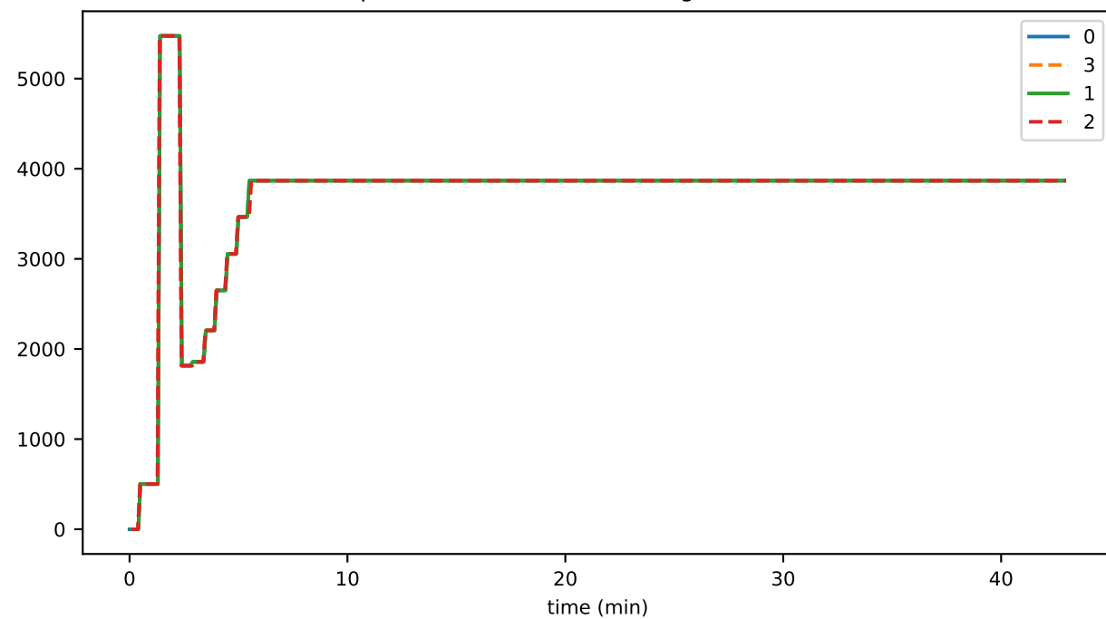
preconsensusEventFileYoungestIdentifier
