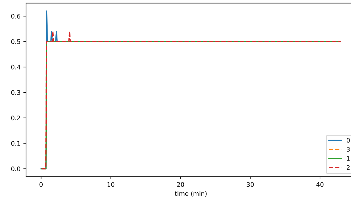
vmap_lifecycle_familySizeBackpressureMs_state
