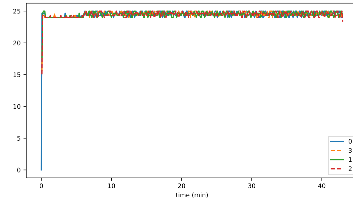
accountsPercentUsed
