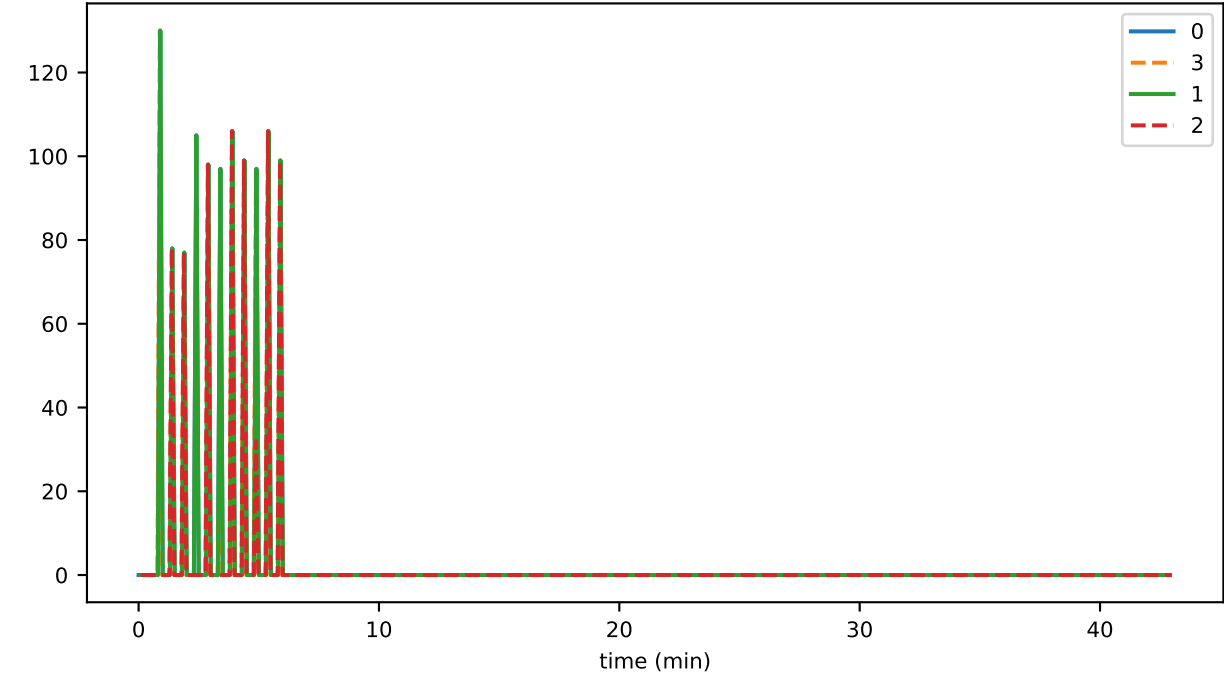
ds_flushes_hashesWritten_state
