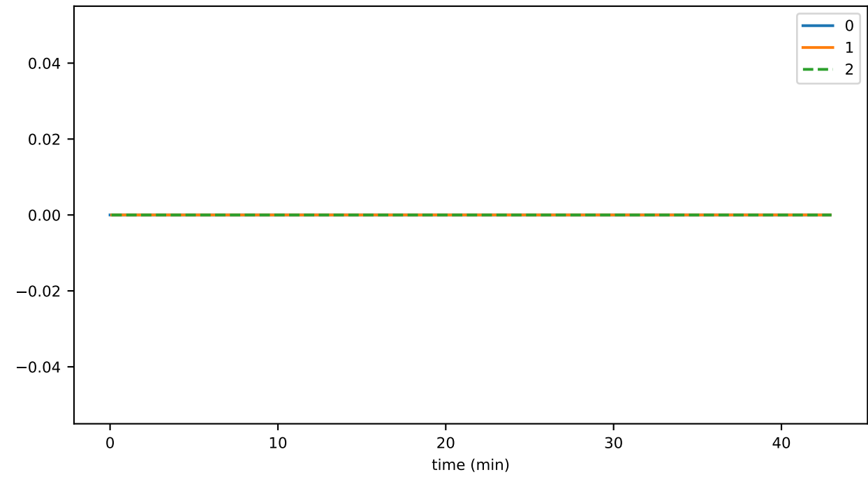
recordHashes_highestBlock
