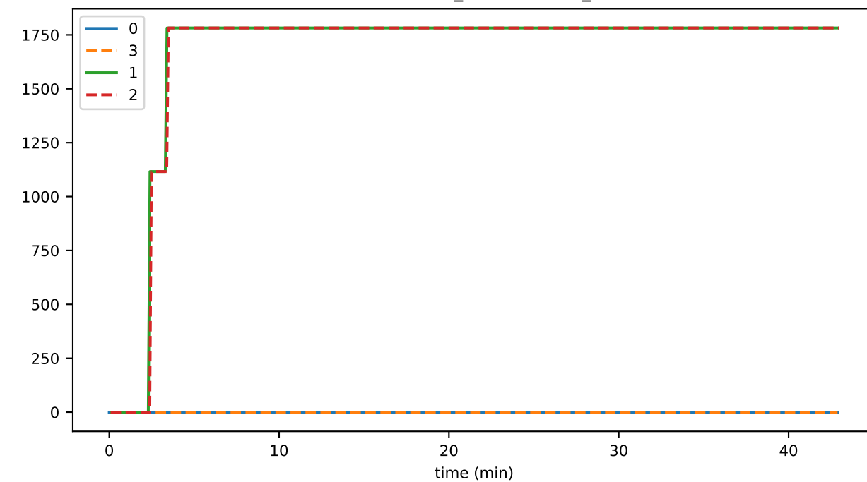
futureEventBuffer_eventCreator_maxBR
