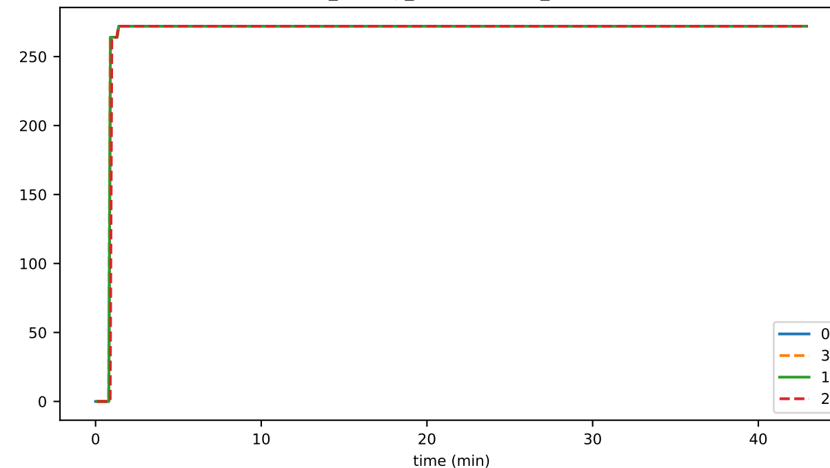
ds_offheap_hashesListMb_state
