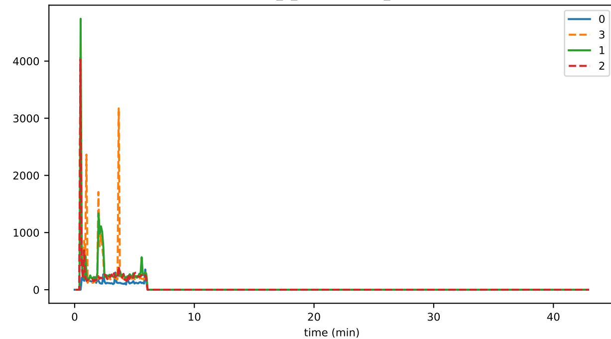
eventDelay_3_deduplication_gossipMAX
