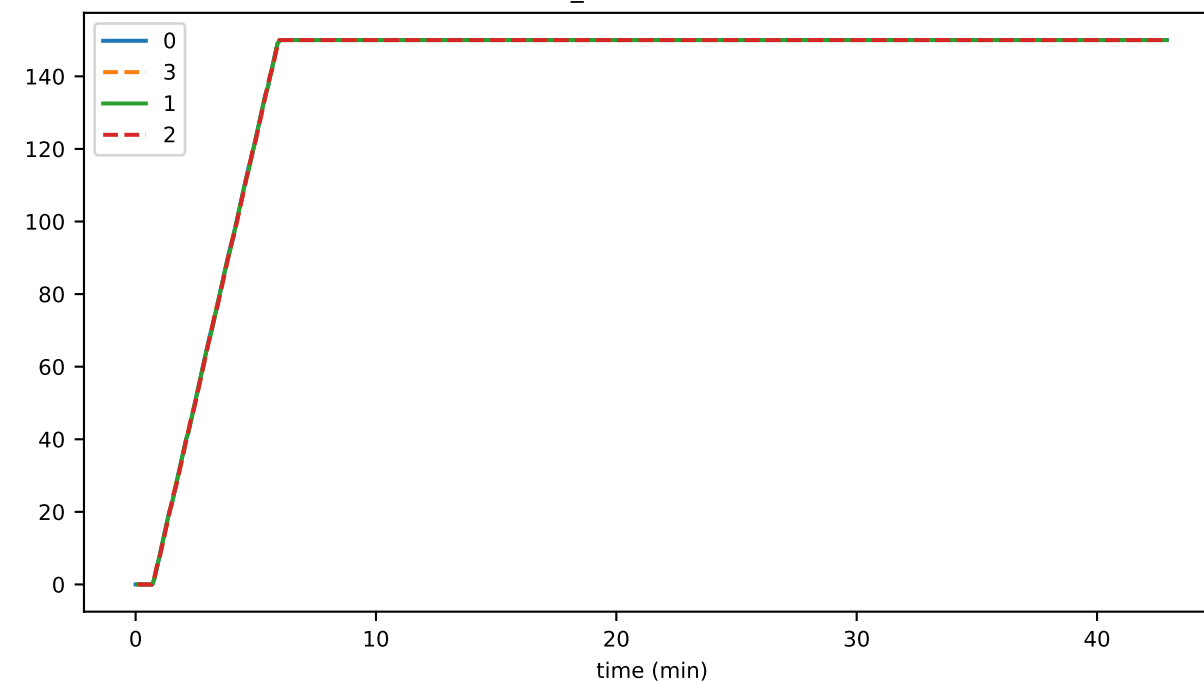
buffer_numBlocksOpened
