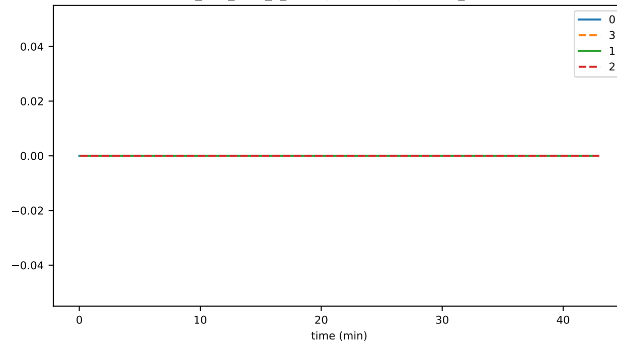
ds_files_level_4_hashesFileSizeByLevelMb_state
