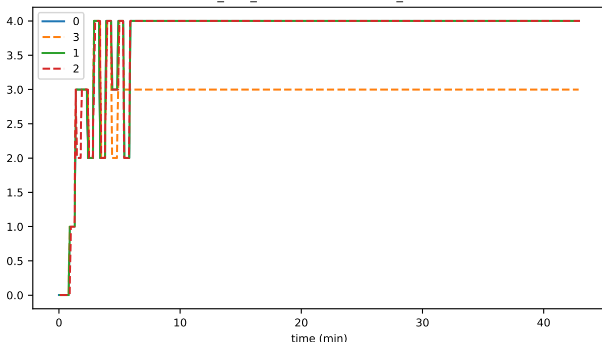
ds_files_hashesStoreFileCount_state
