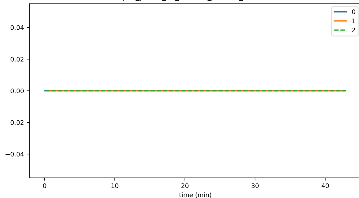
sync_phase_03_fraction_NO_PERMIT
