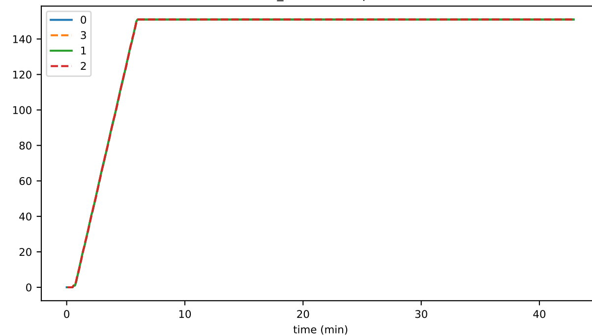
buffer_numBlocksOpened
