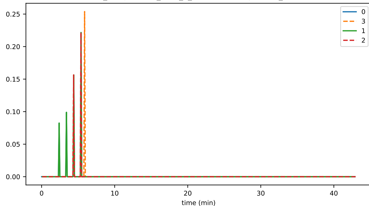
ds_compactions_level_1_leafKeysSavedSpaceMb_state
