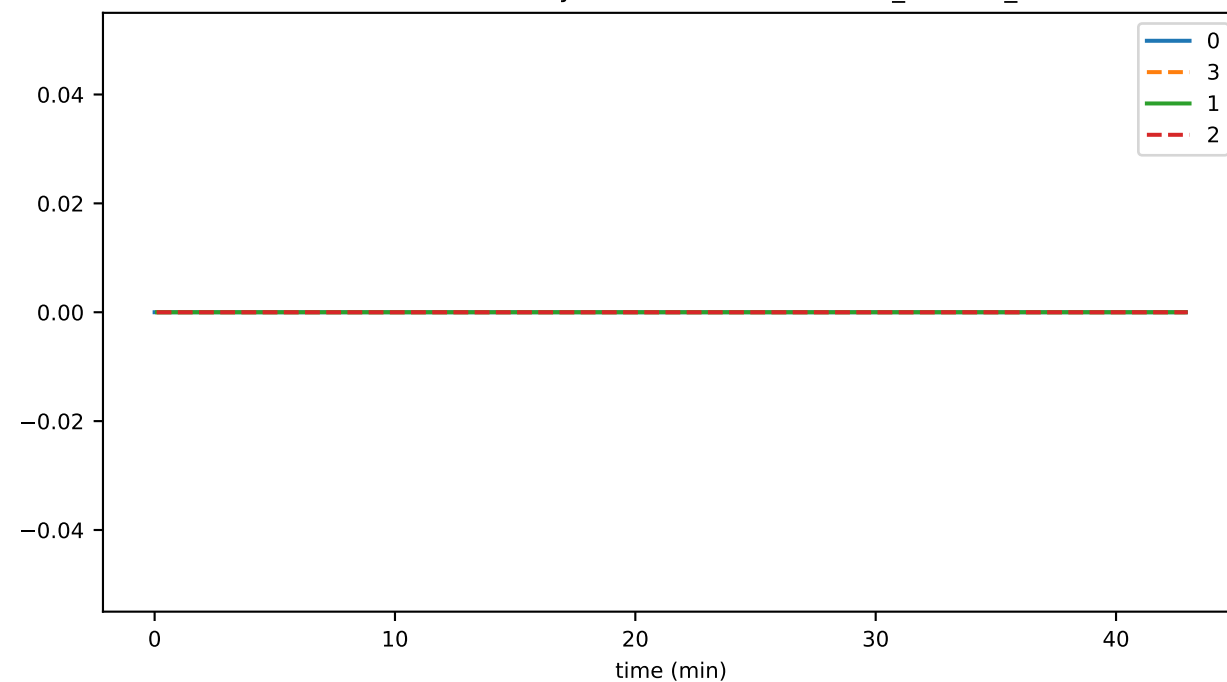
SmartContractService:SystemContractMethodCall_FREEZE_UNFREEZE_failed
