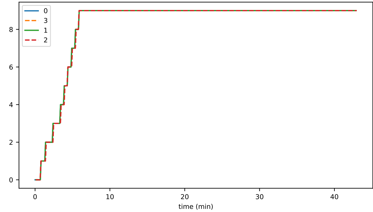
preconsensusEventFileOldestSeconds
