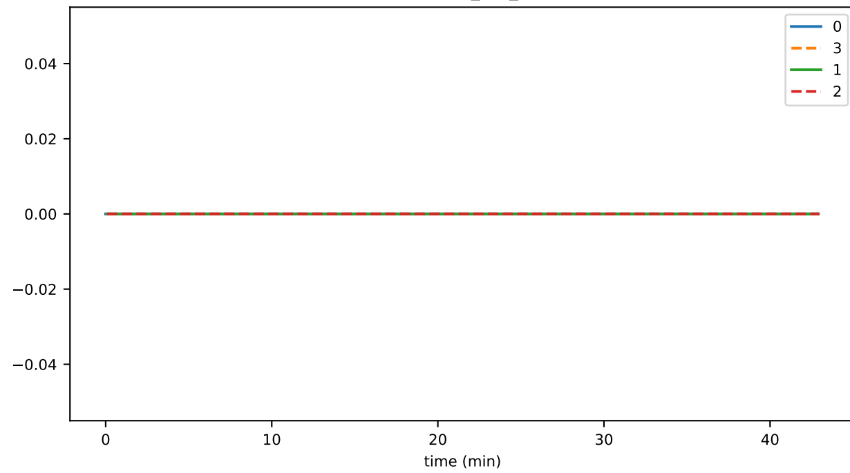
DigLockUp_per_sec
