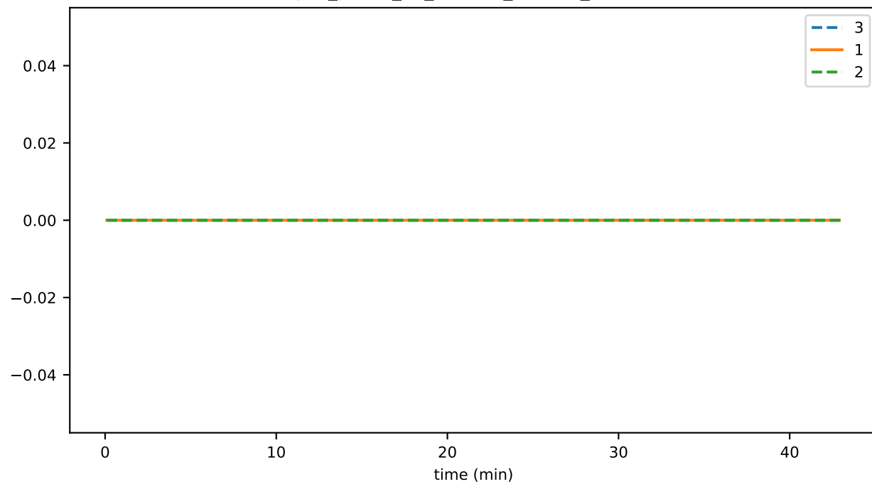
sync_phase_00_fraction_NO_PERMIT
