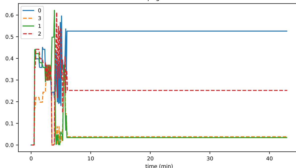
opAgeDiff
