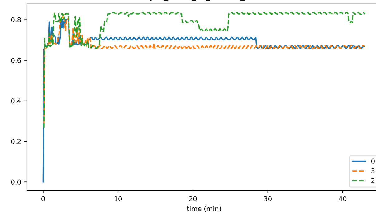
sync_phase_01_fraction_OTHER_FALLEN_BEHIND
