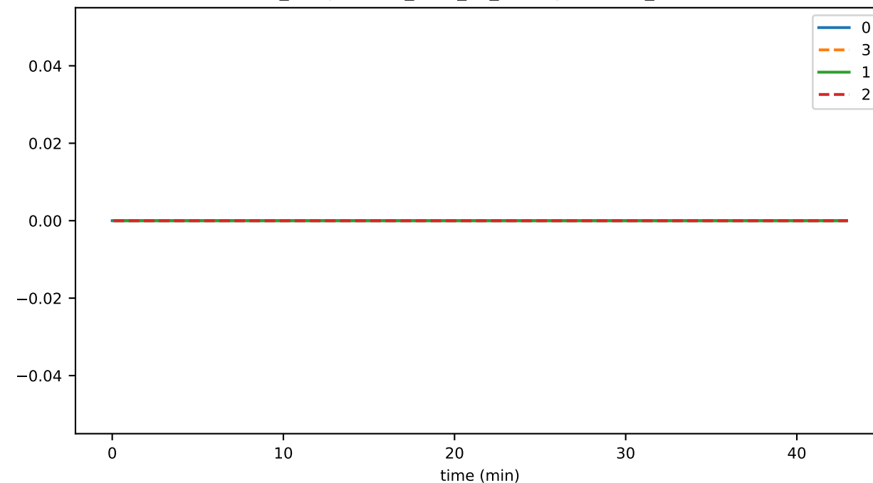
ds_compactions_level_10_leavesTimeMs_state
