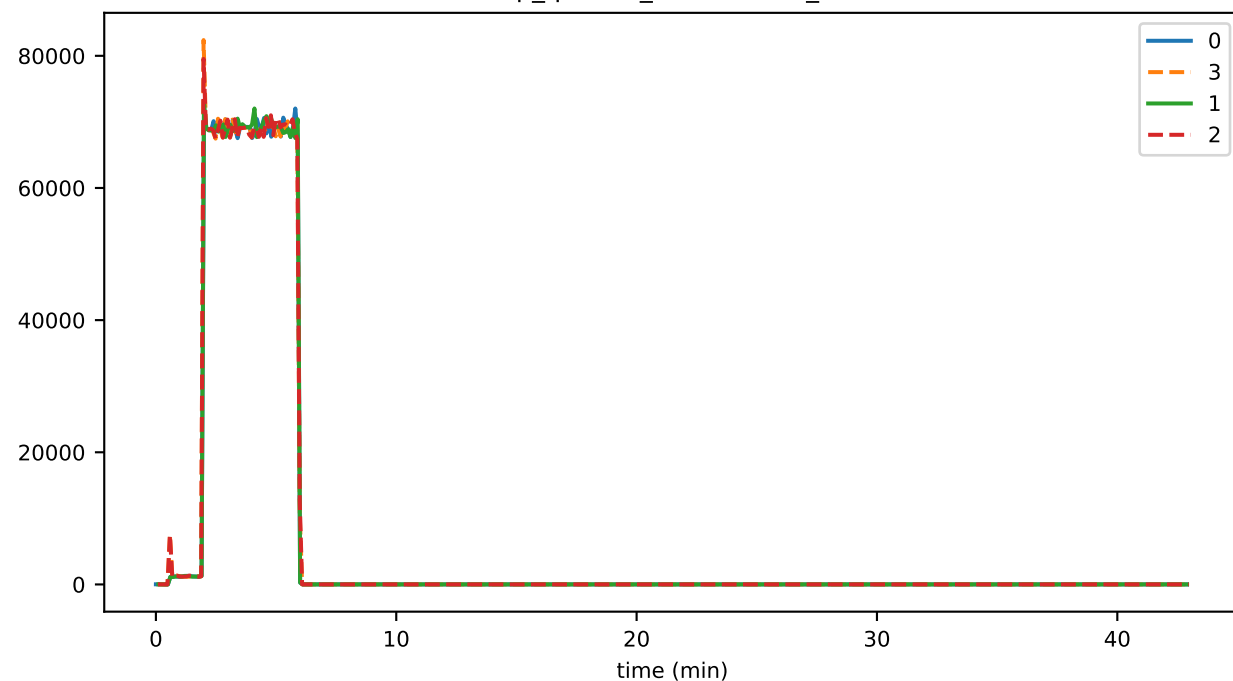
vmap_queries_updatedEntities_state
