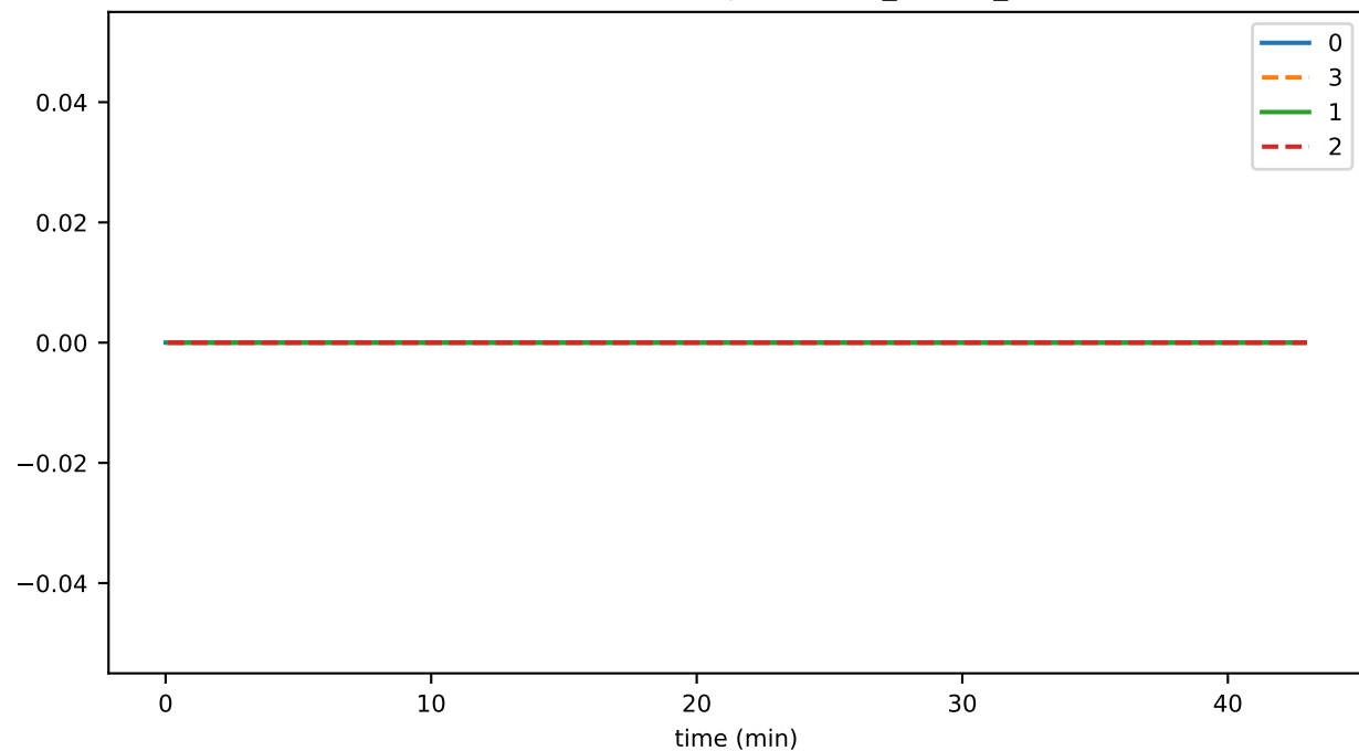
SmartContractService:OpsDuration_TxnsThrottled
