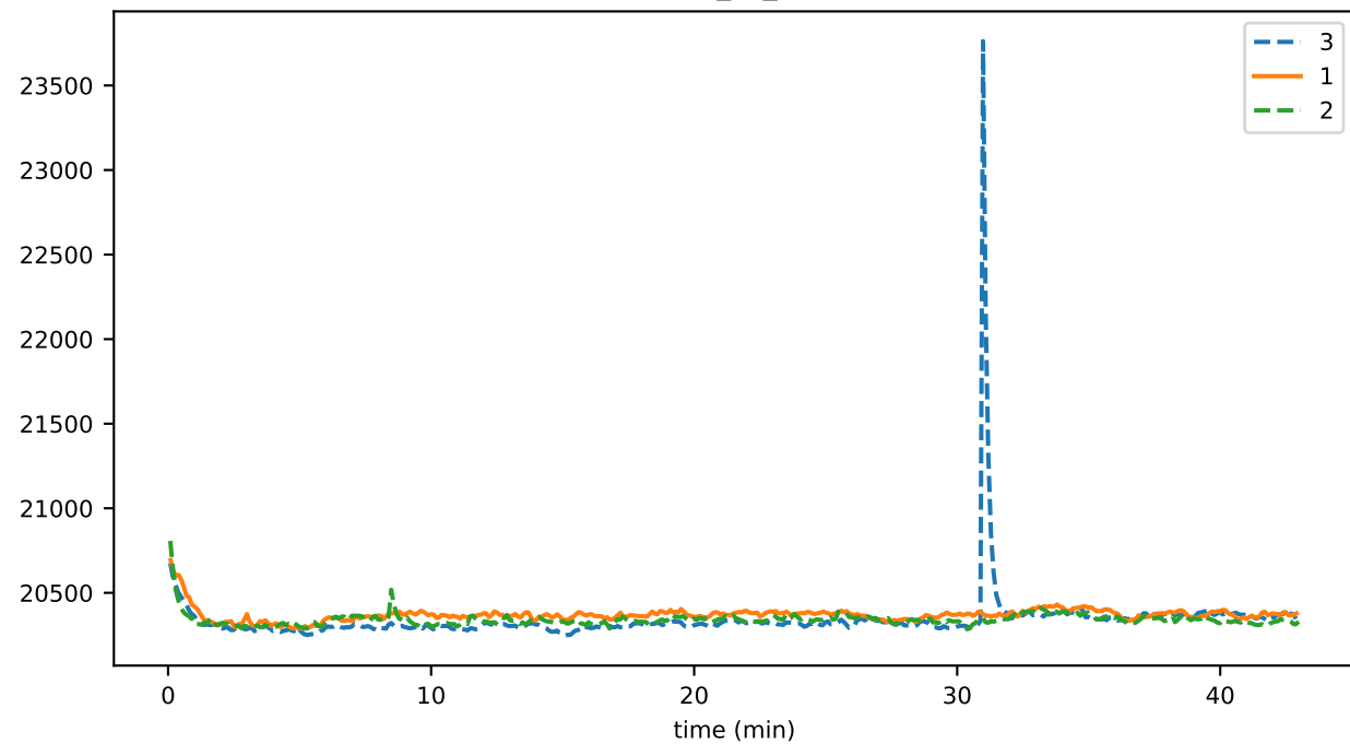
ping_us_00
