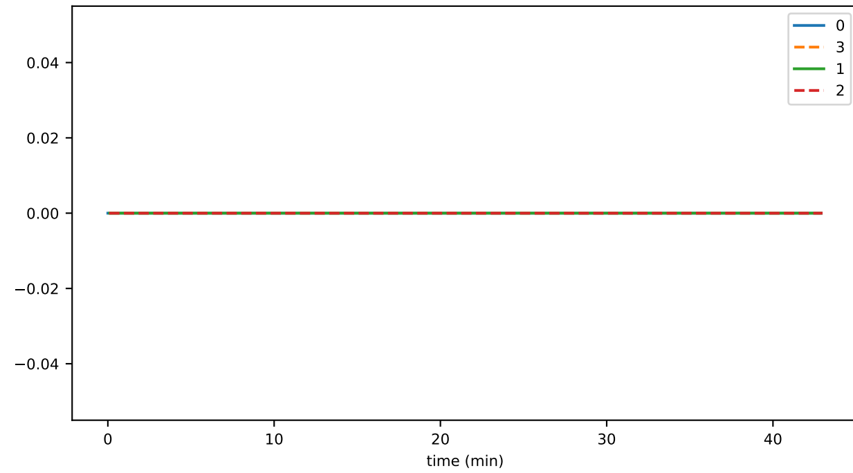
SigSpans_per_sec
