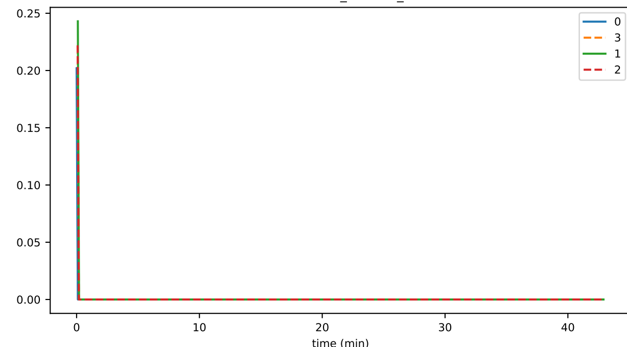
eventCreation_fraction_IDLE
