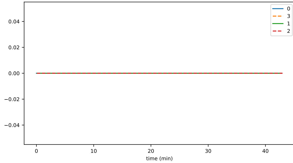
doNotSyncHalted
