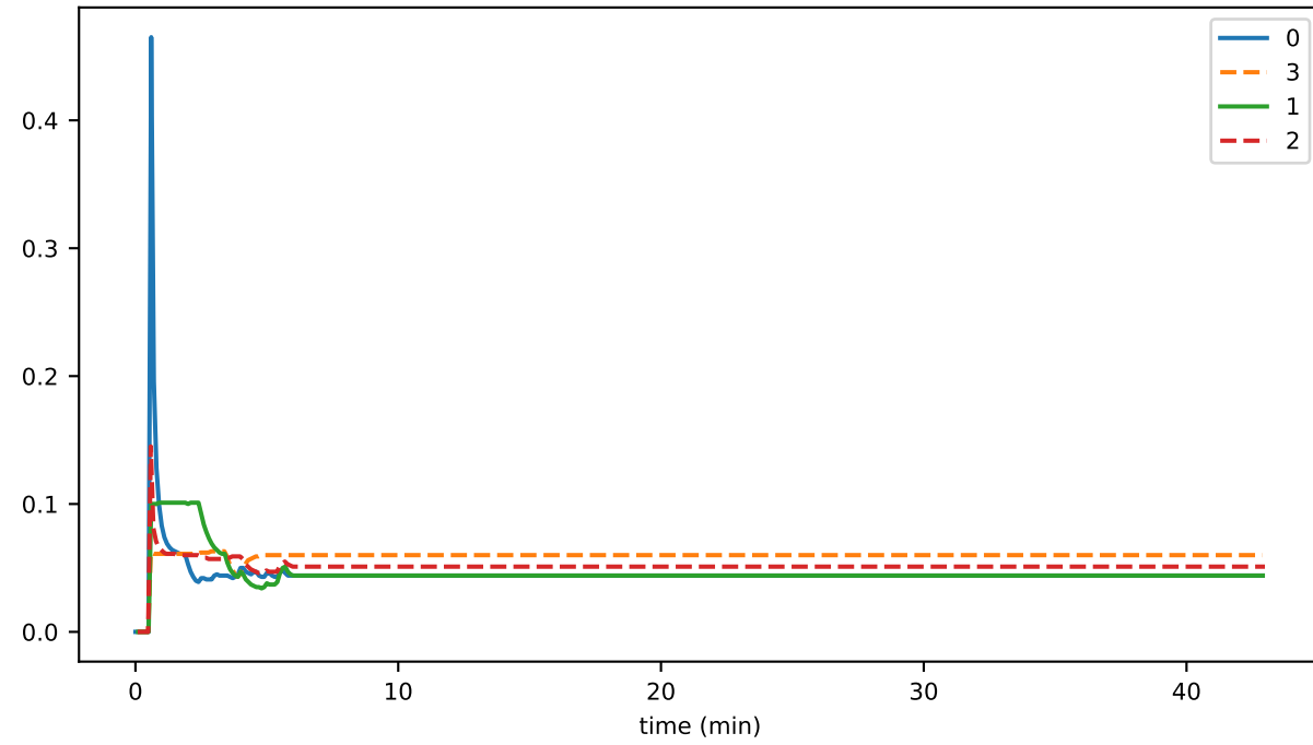
secR2C
