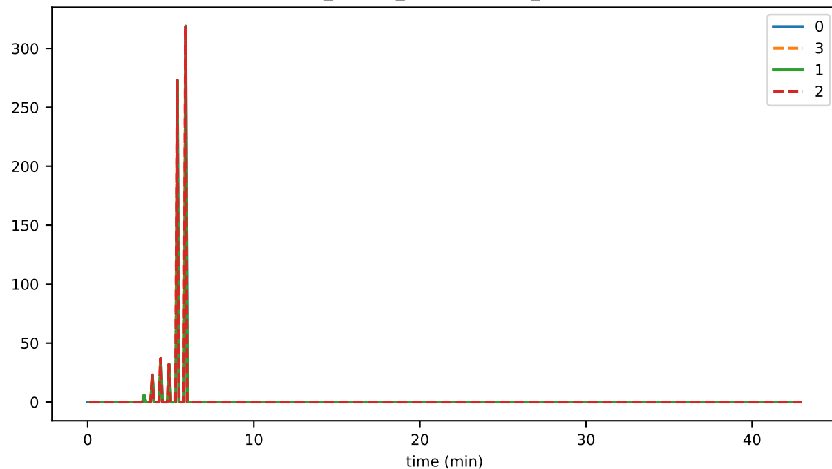
ds_flushes_leavesDeleted_state
