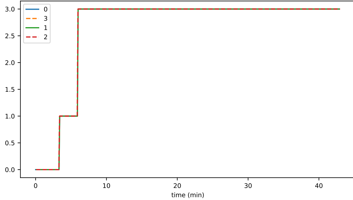
buffer_backPressureState
