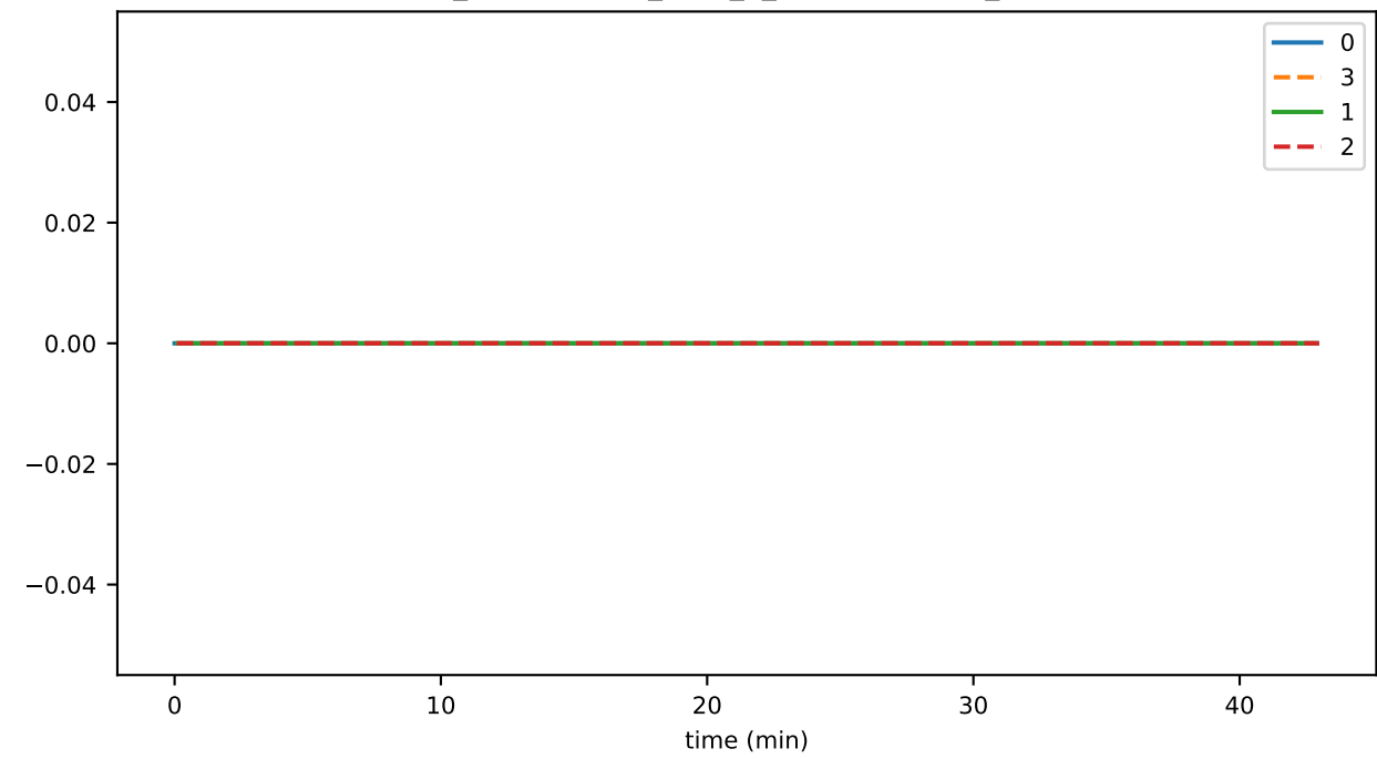
ds_compactions_level_6_hashesTimeMs_state
