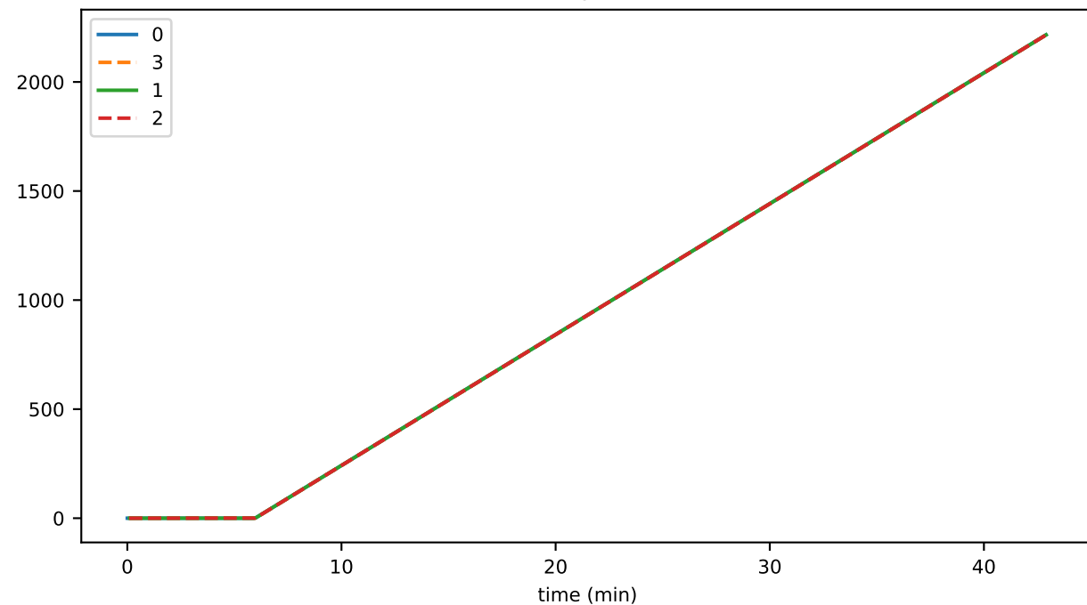
uptimeComputationTime
