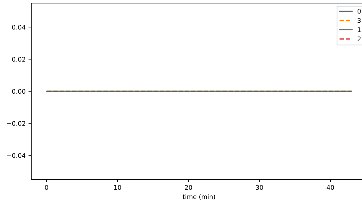
ds_files_level_6_leavesFileSizeByLevelMb_state
