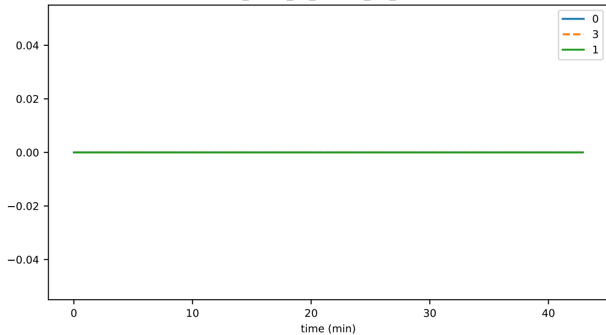
sync_phase_02_fraction_NO_PERMIT
