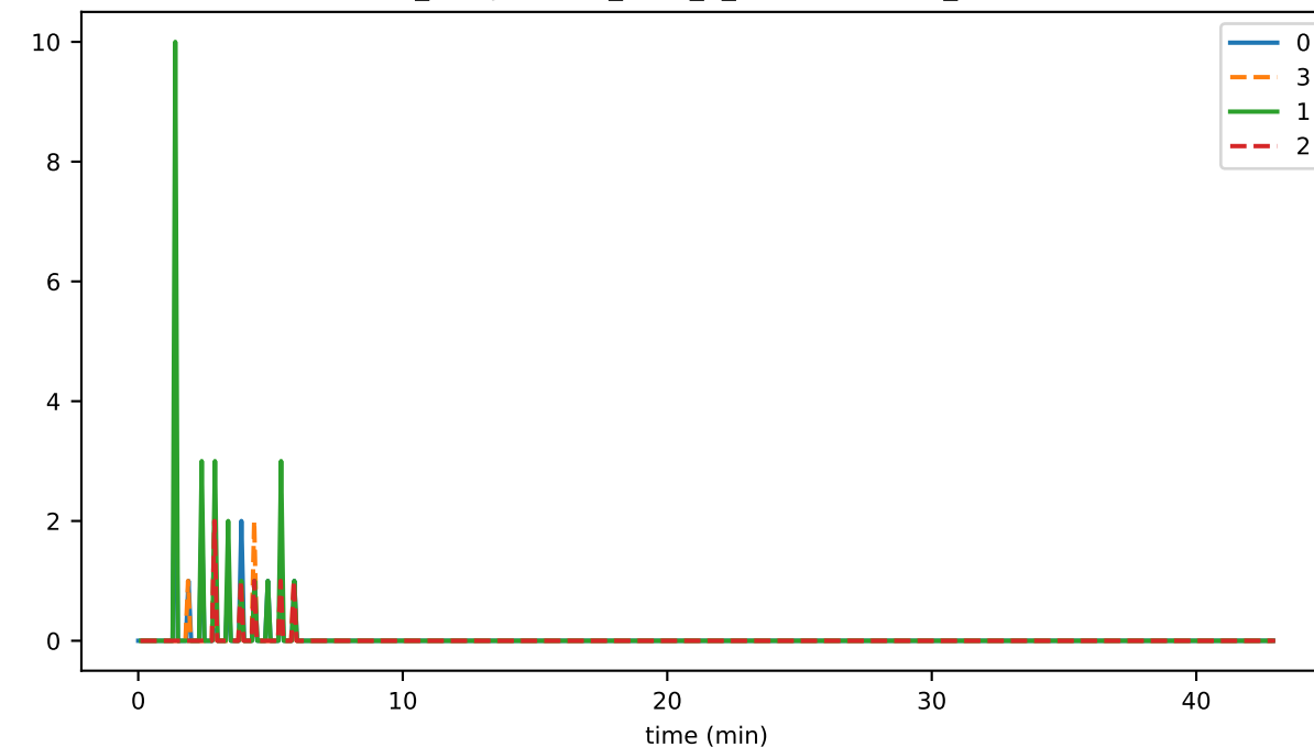
ds_compactions_level_1_leafKeysTimeMs_state
