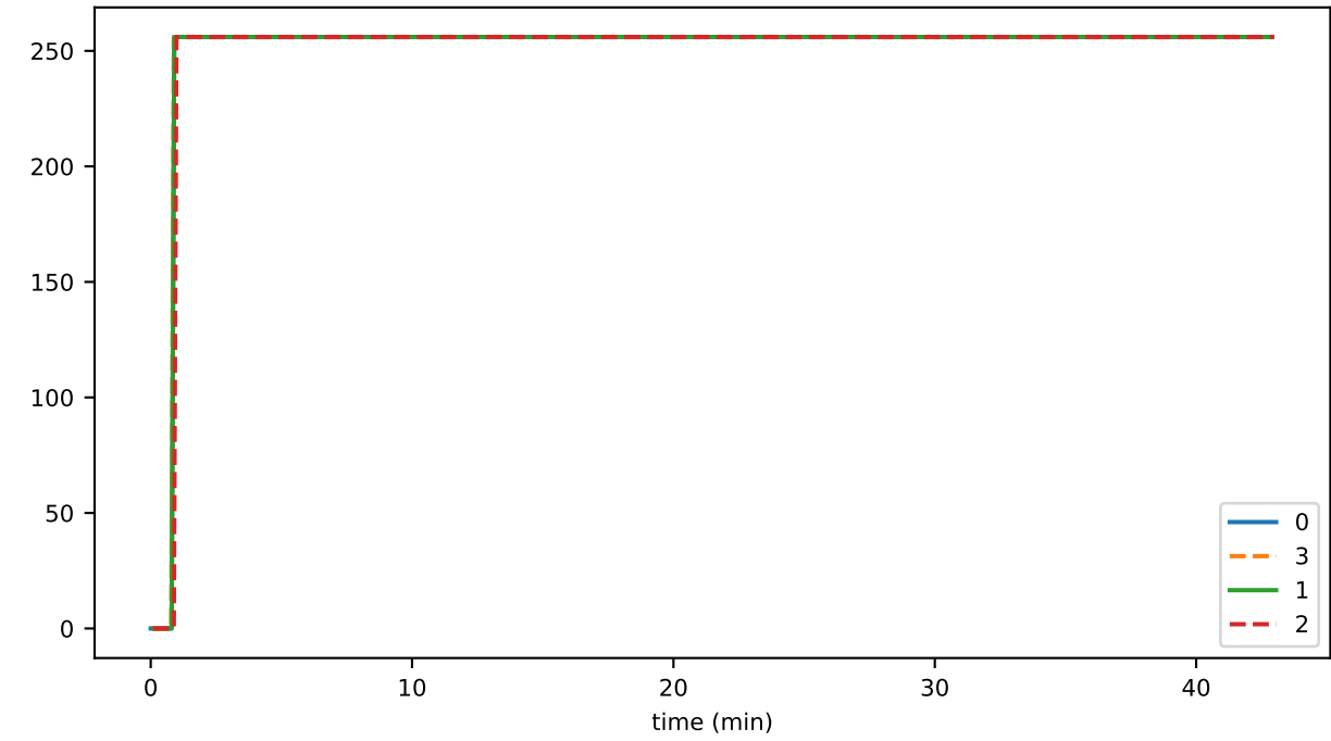
ds_reads_leafKeys_state
