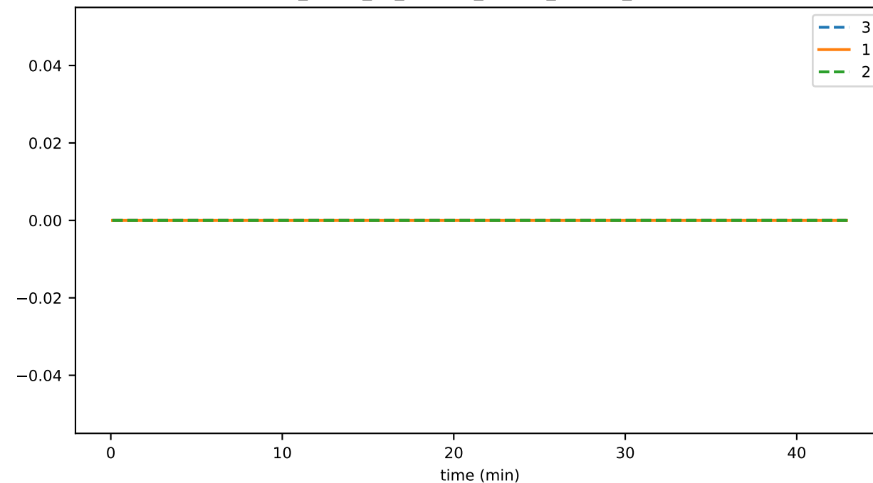
sync_phase_00_fraction_OTHER_FALLEN_BEHIND
