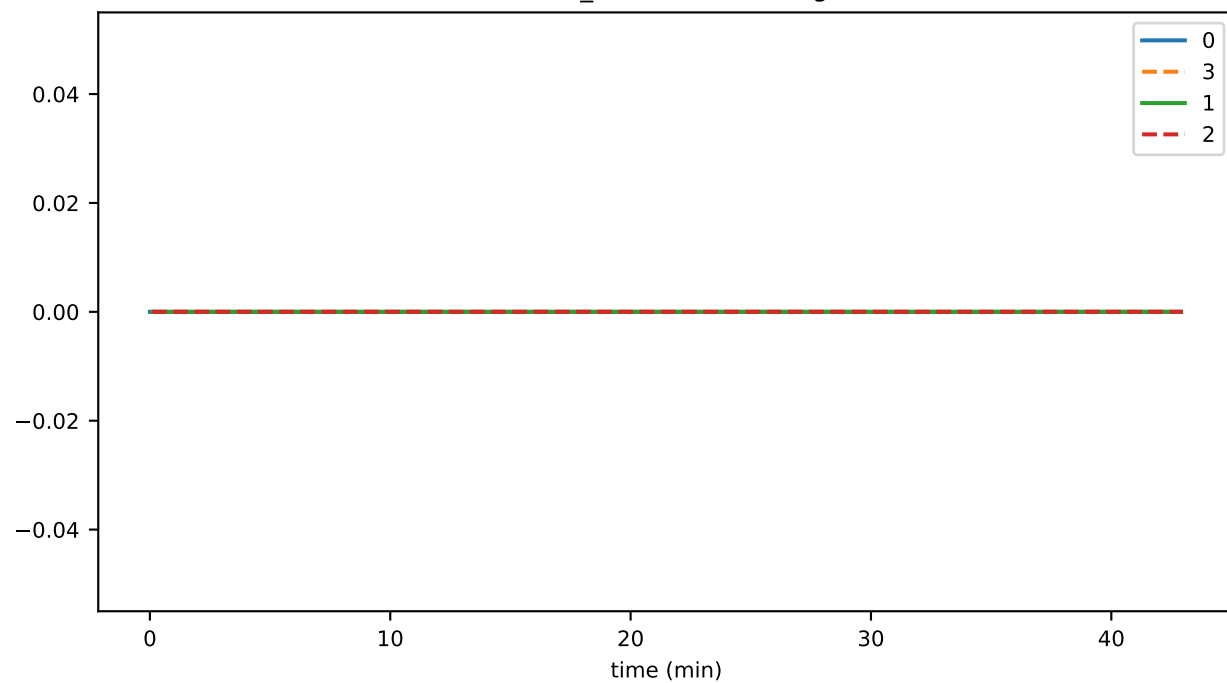
buffer_numBlocksMissing
