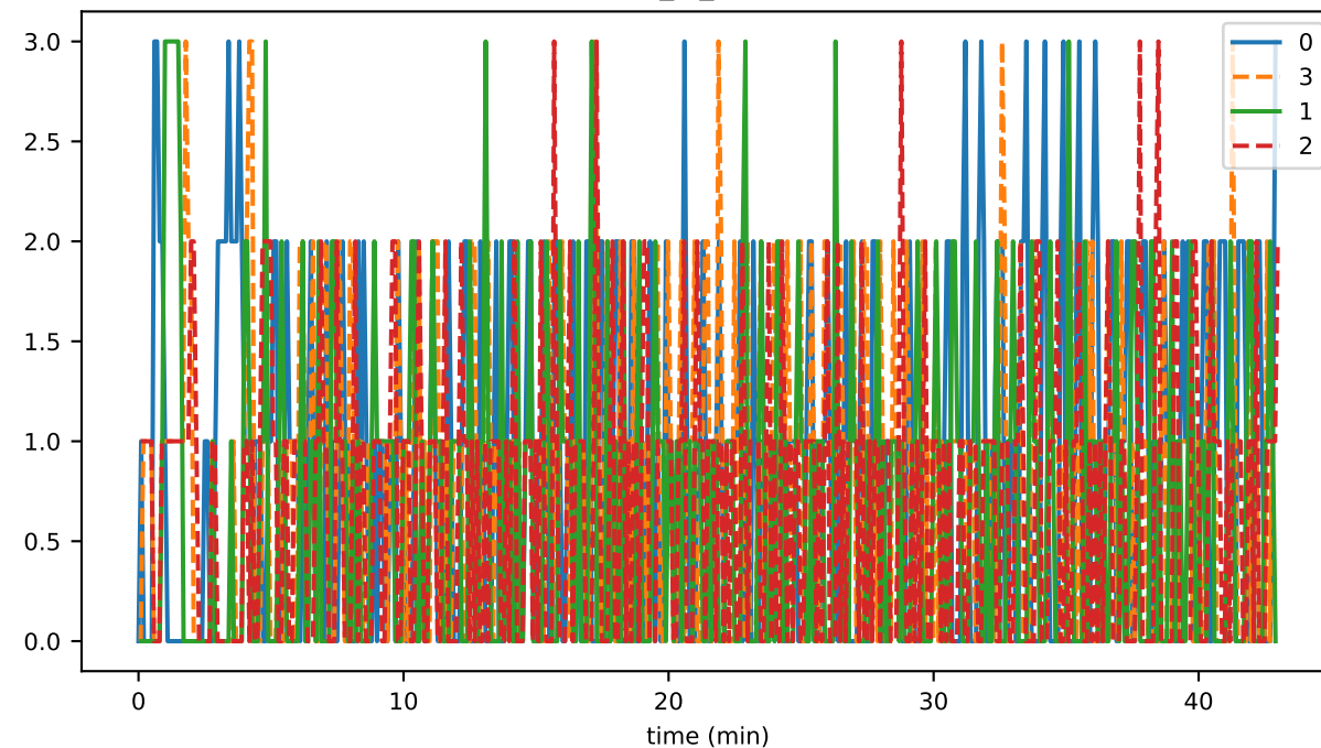
syncs_in_progress
