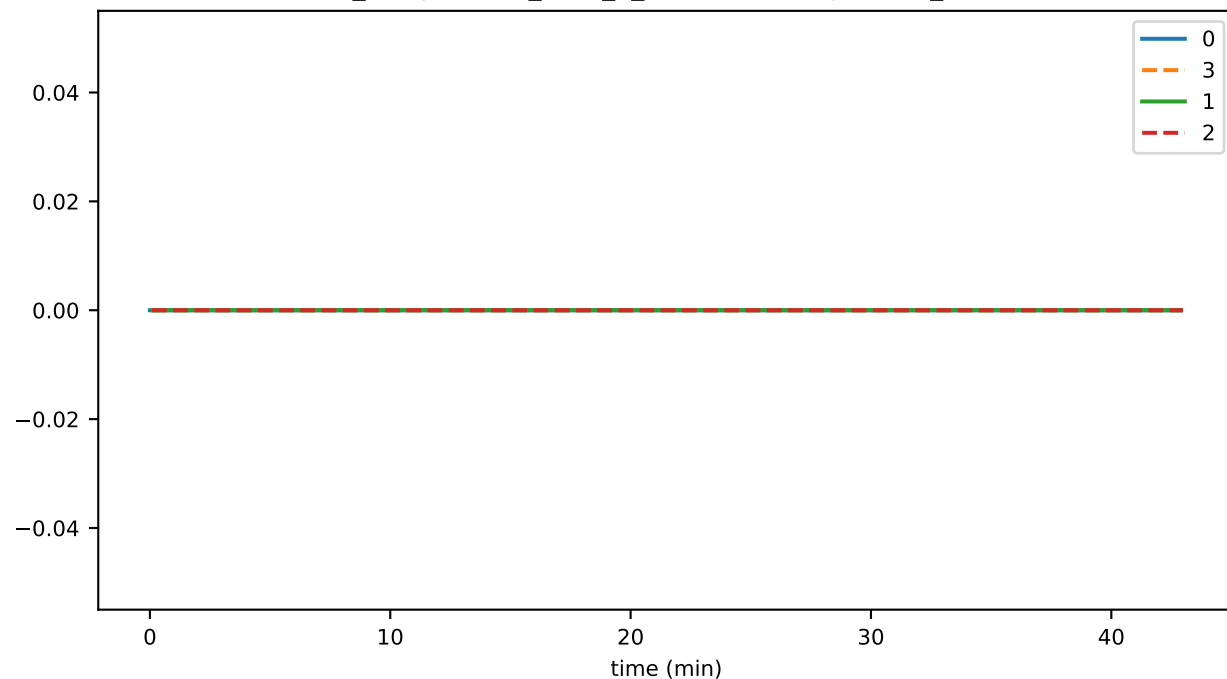
ds_compactions_level_0_leafKeysSavedSpaceMb_state
