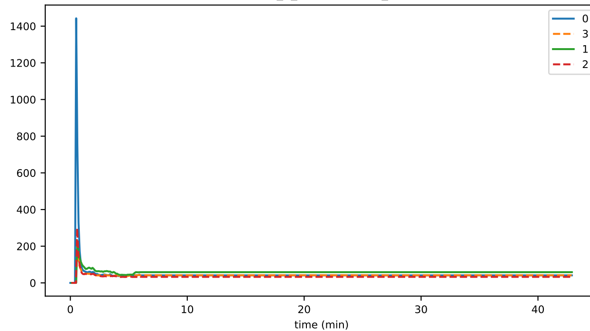
eventDelay_3_deduplication_runtime
