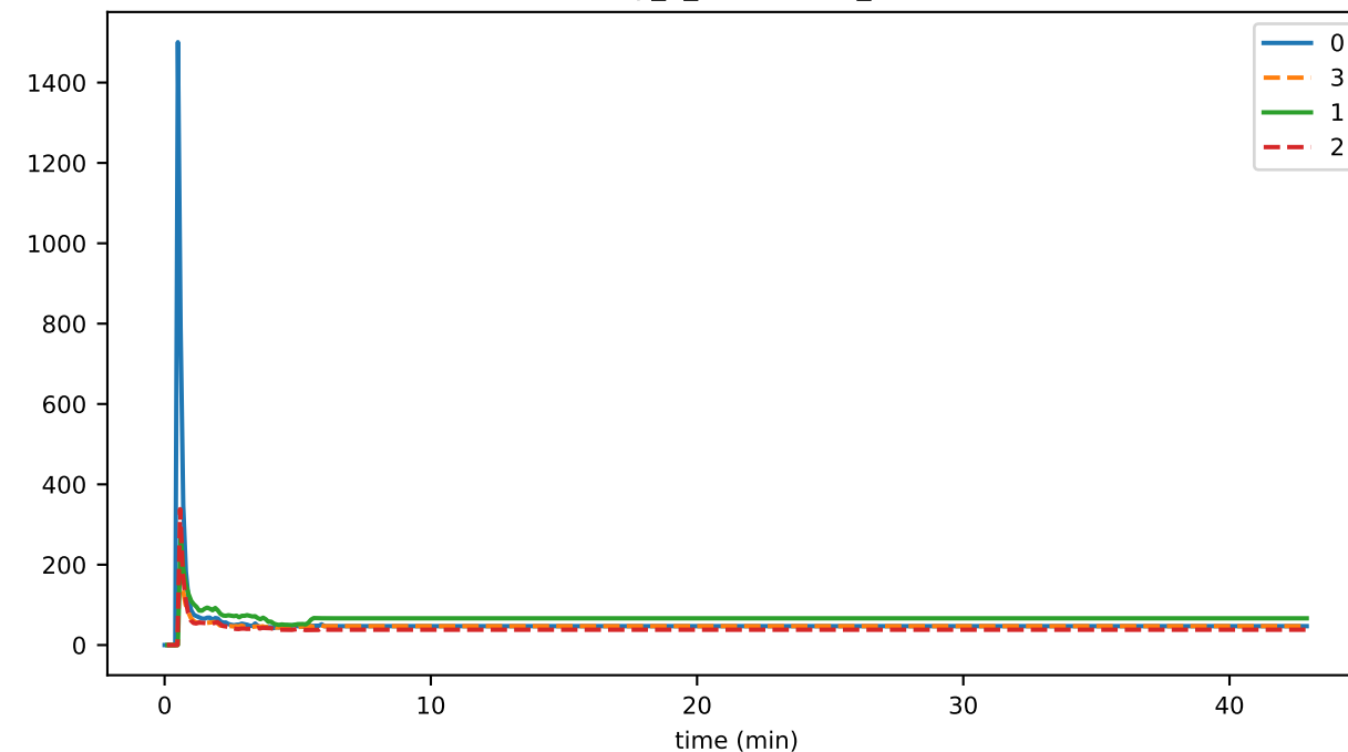
eventDelay_4_verification_storage
