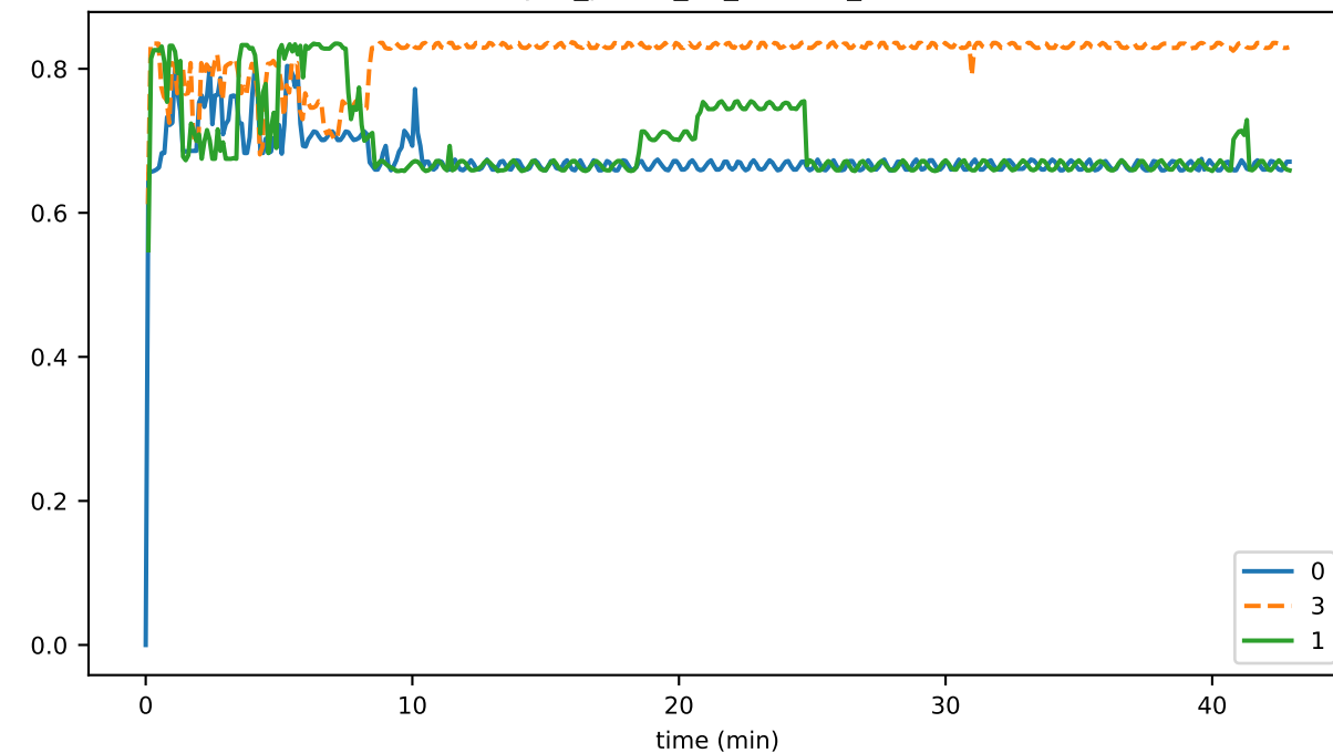
sync_phase_02_fraction_OTHER_FALLEN_BEHIND
