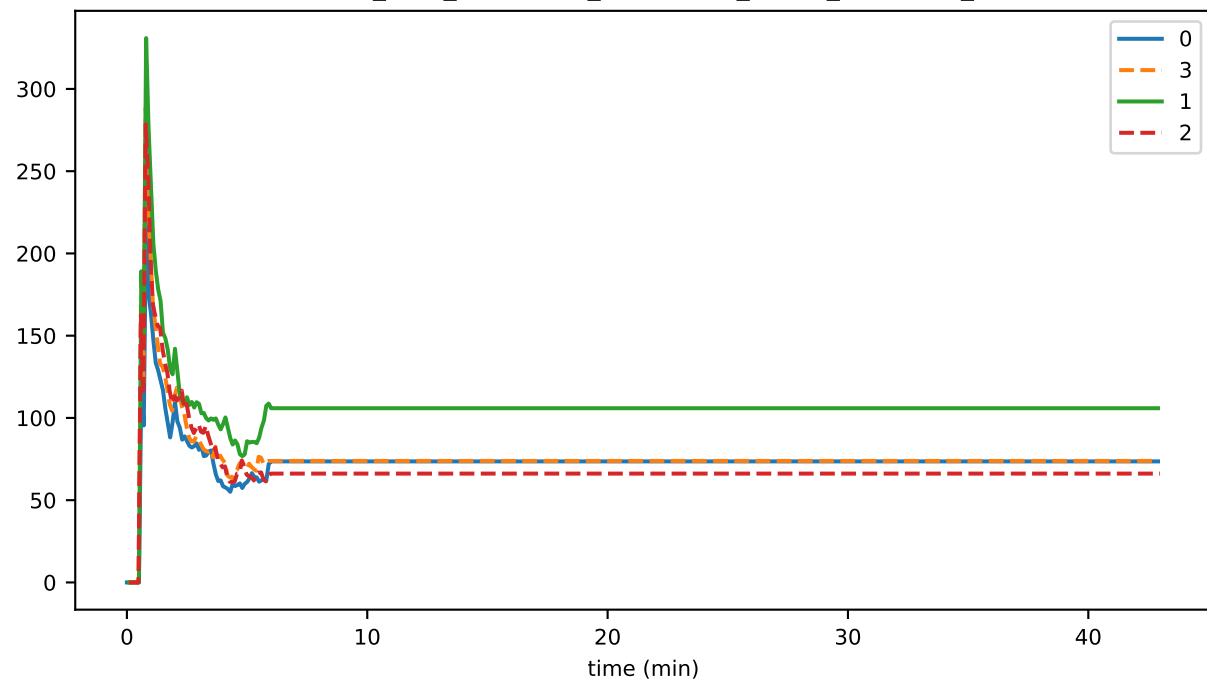
ConsensusEngine_busy_fraction
