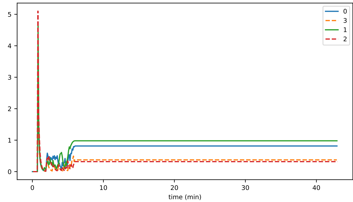
sigStateHash
