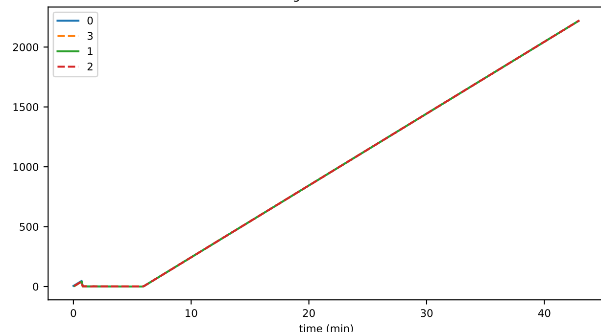
oldestSignedStateSeconds
