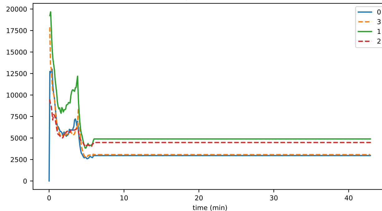
syncPermitsAvailable
