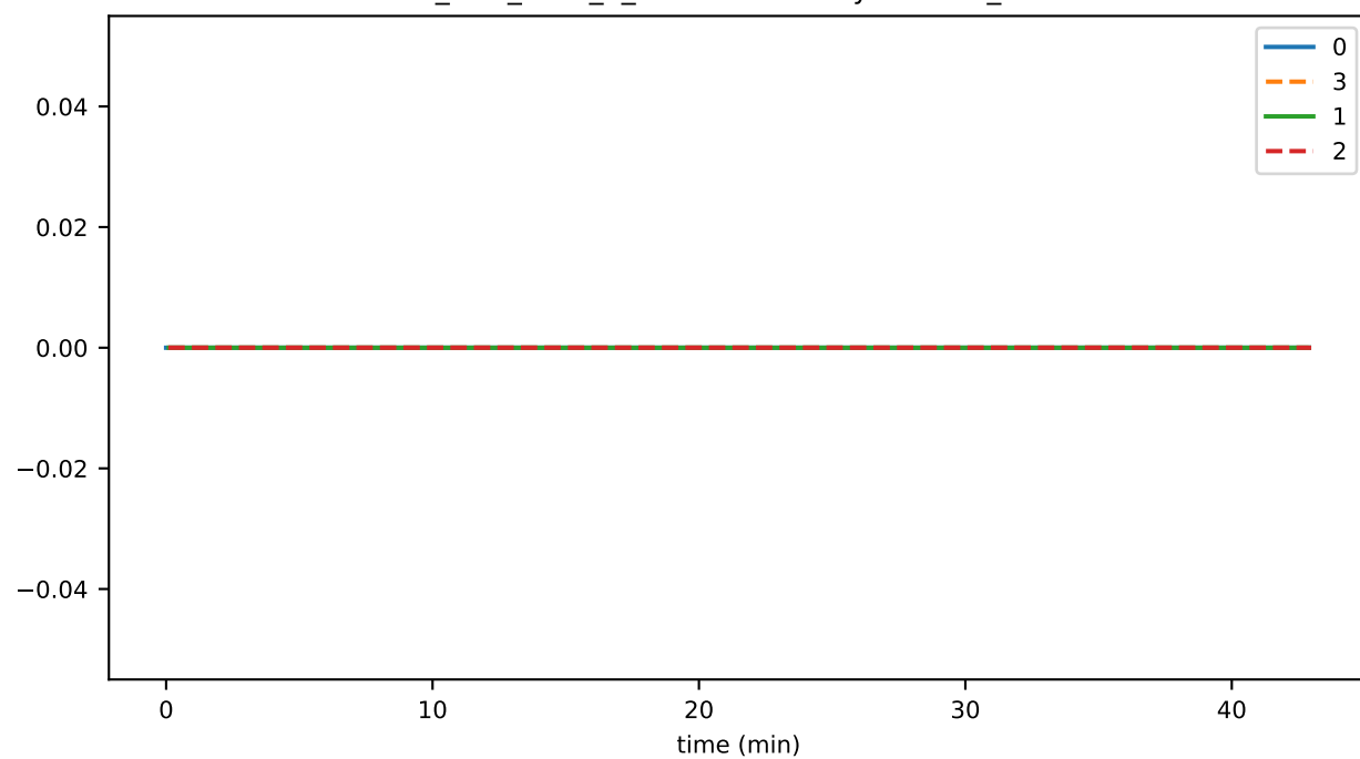
ds_files_level_3_leavesFileSizeByLevelMb_state
