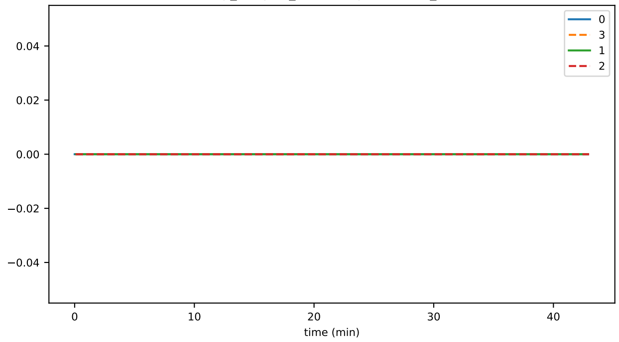
vmap_lifecycle_flushDurationMs_state
