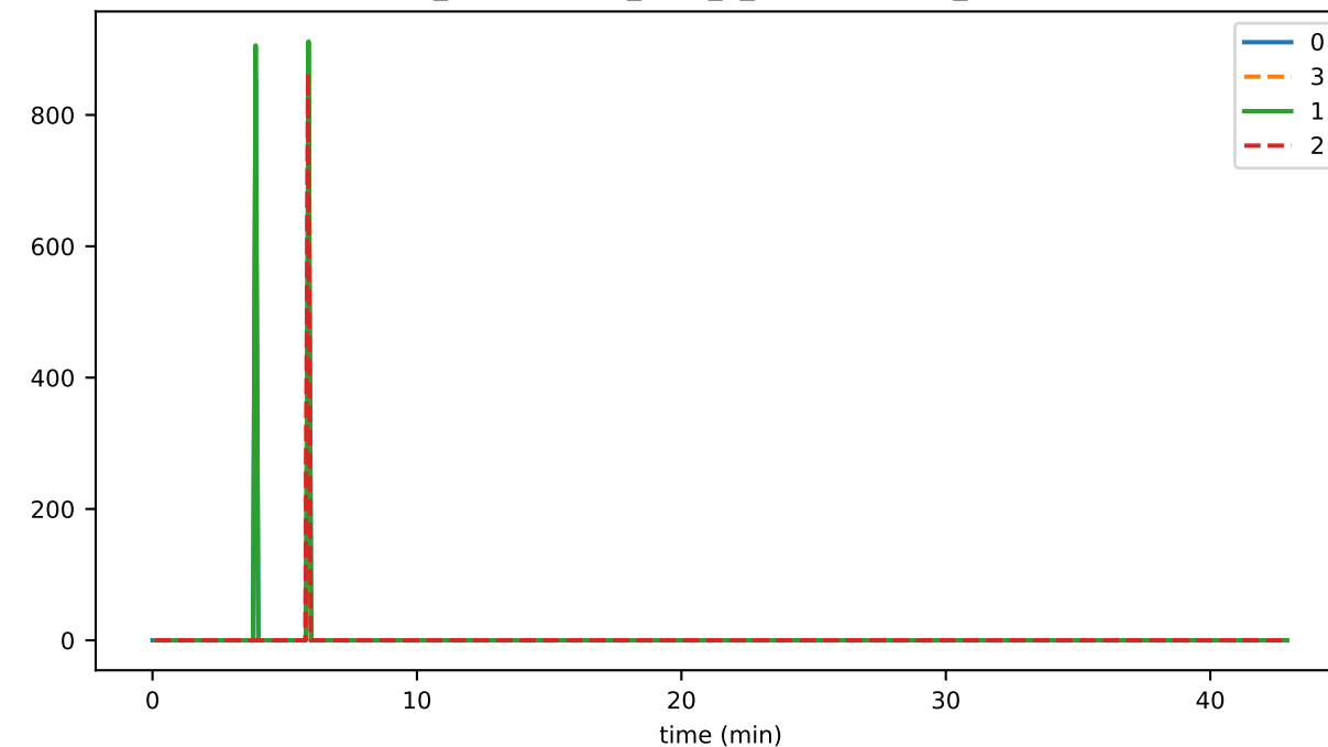
ds_compactions_level_2_leavesTimeMs_state
