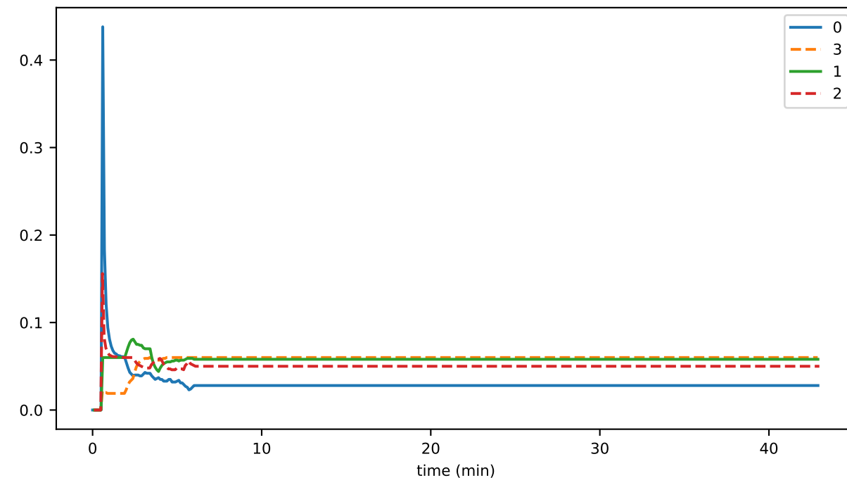
senderReconnectDurationSeconds
