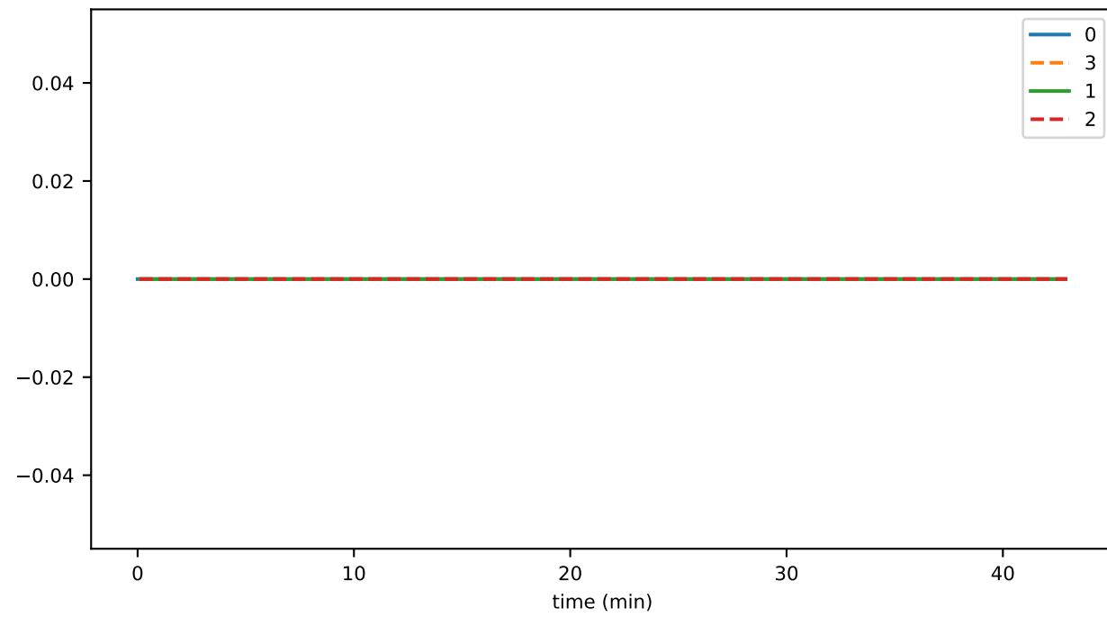
filesPercentUsed
