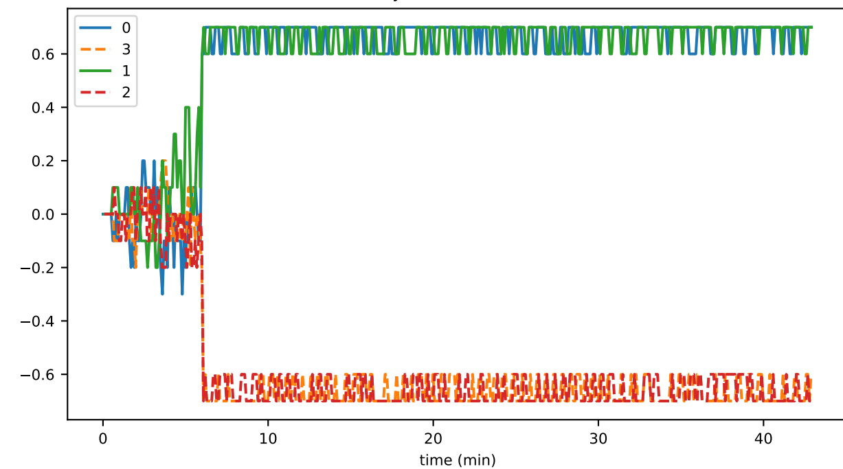
syncIndicatorDiff
