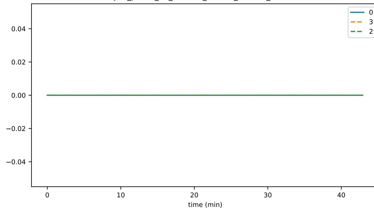
sync_phase_01_fraction_OTHER_FALLEN_BEHIND
