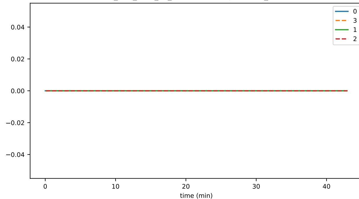
ds_files_level_1_leafKeysFileSizeByLevelMb_state
