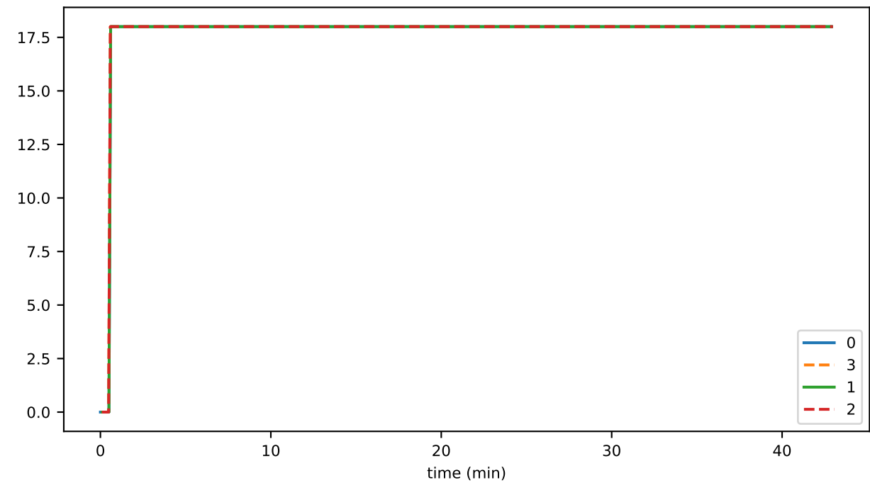
filesUsed
