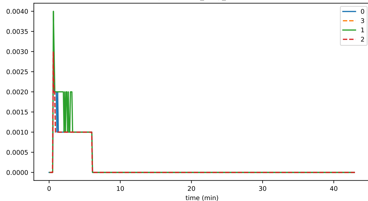
orphanBufferSize
