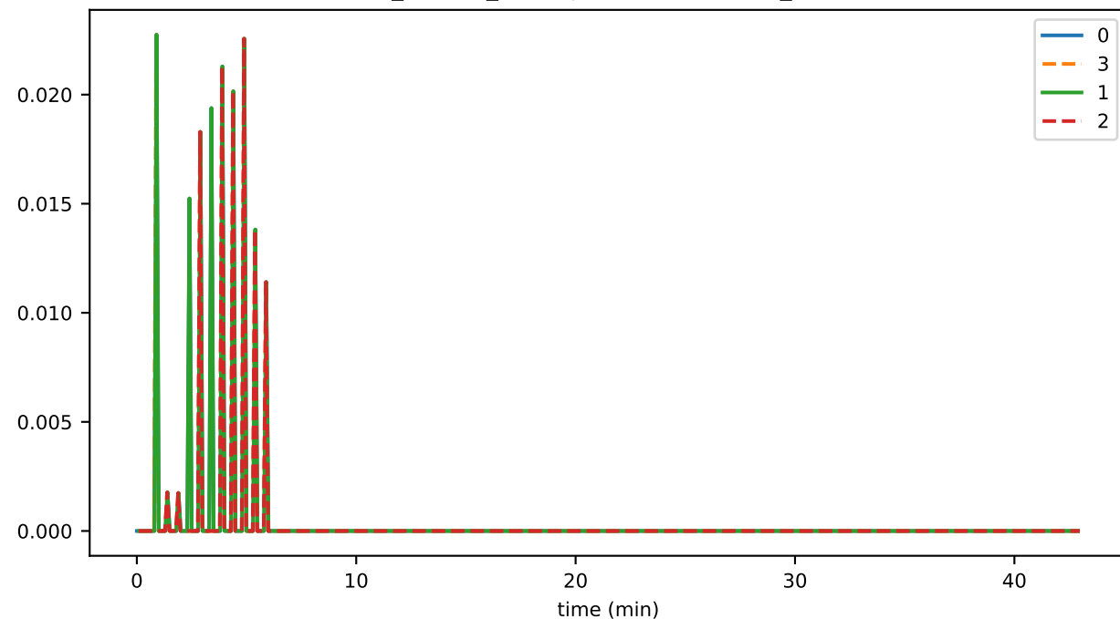
ds_flushes_leavesDeleted_state
