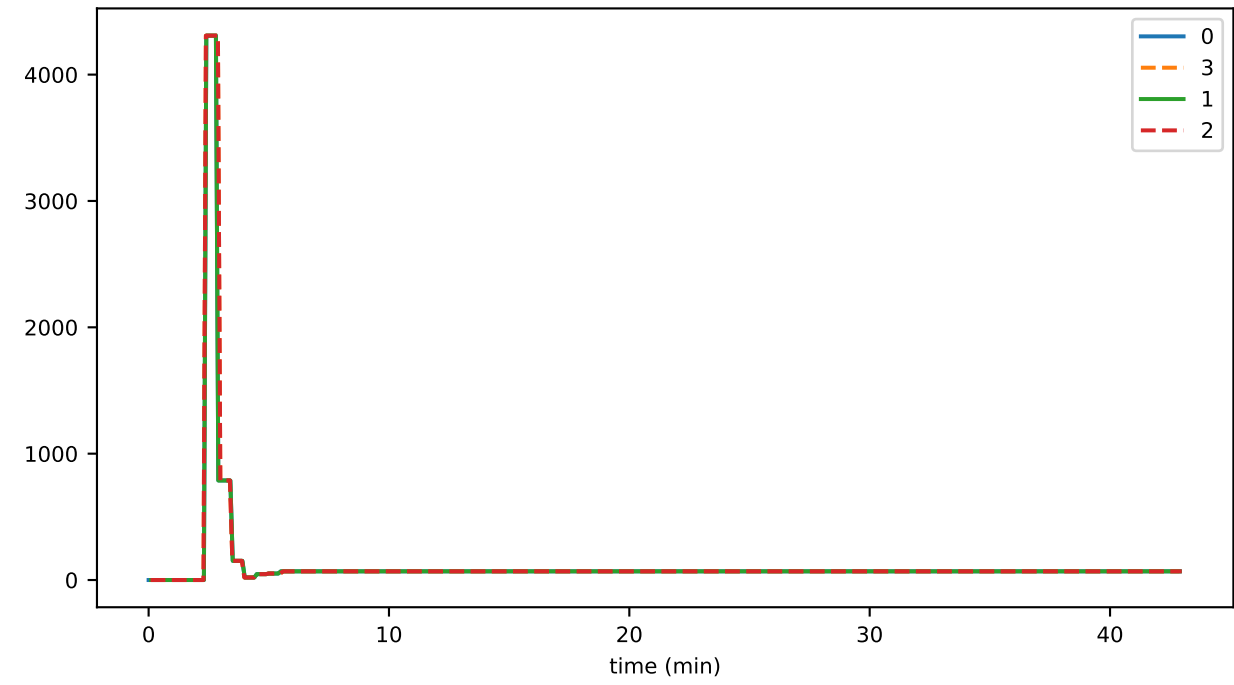
preconsensusEventAverageUnutilizedFileSpan
