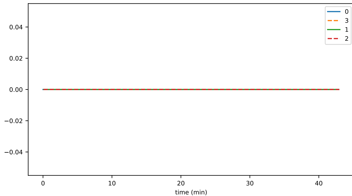
startsReconnectAsReceiver
