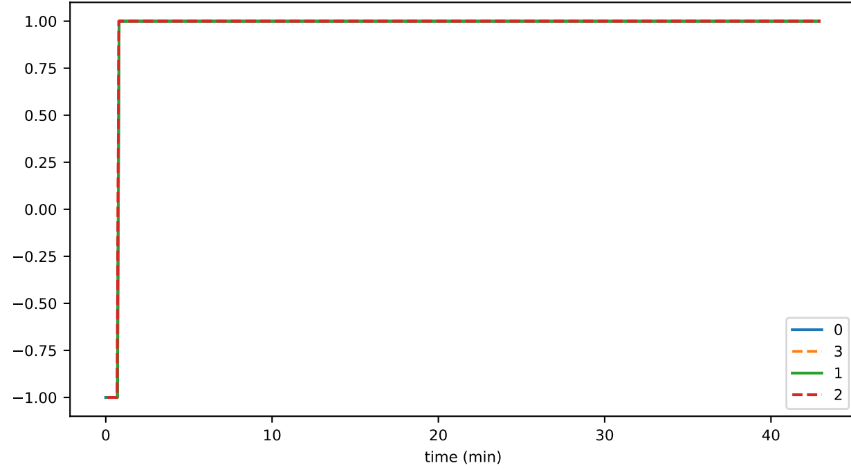
preconsensusEventFileOldestIdentifier
