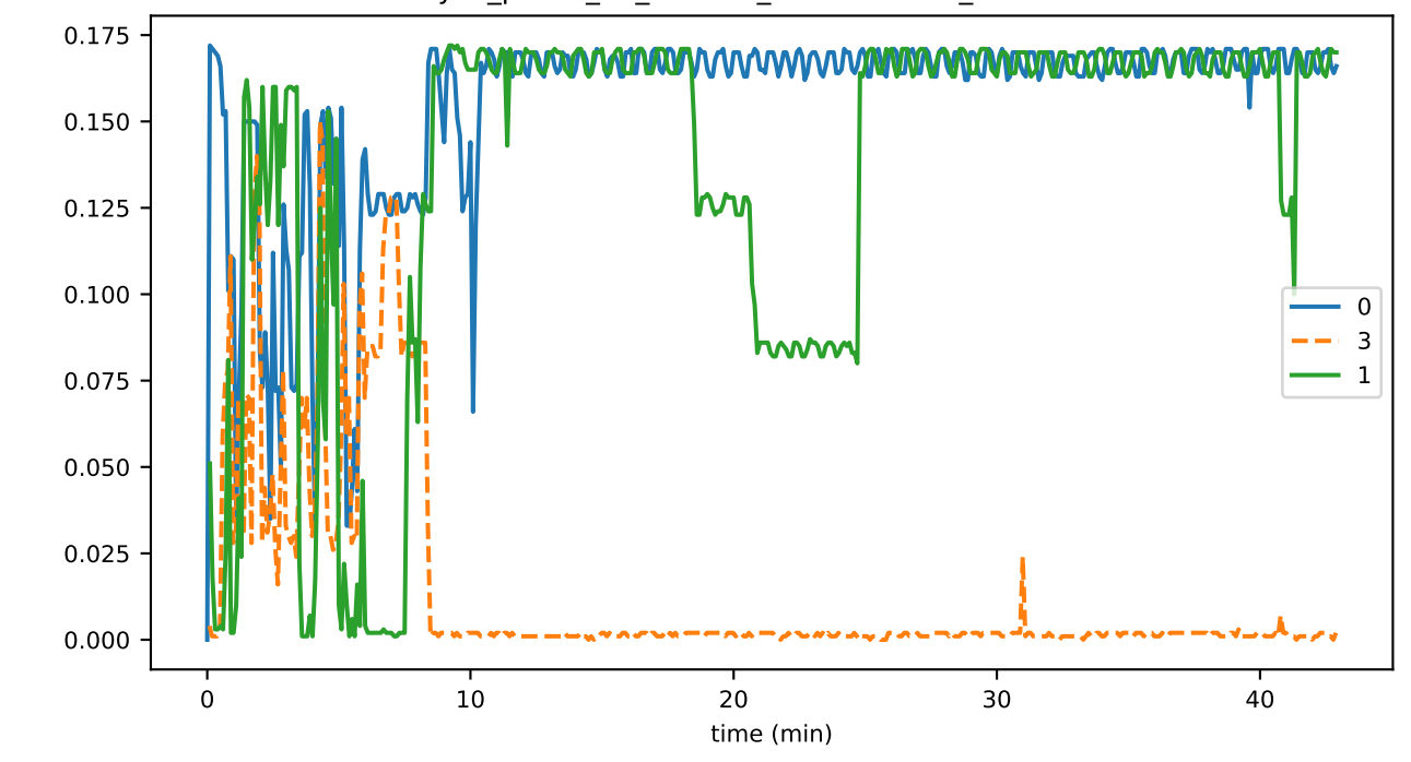
sync_phase_02_fraction_EXCHANGING_WINDOWS
