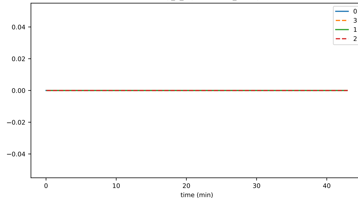
eventDelay_6_pces_gossip
