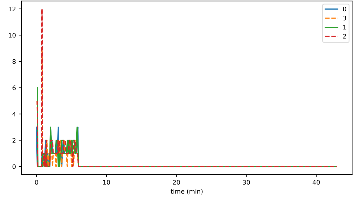
vmap_lifecycle_hashDurationMs_state
