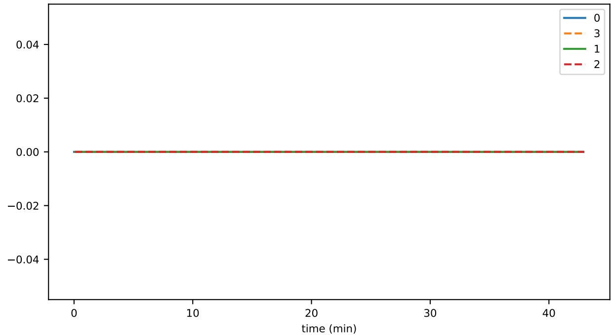
ds_compactions_level_8_leavesSavedSpaceMb_state
