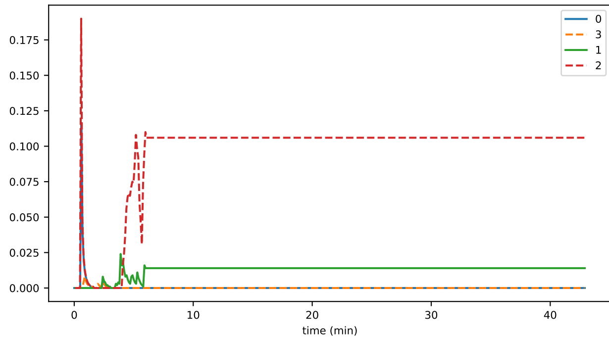
selfishness
