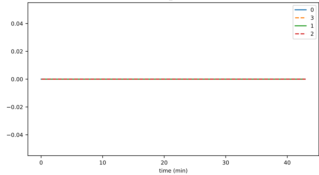
connSend_endOfBlock
