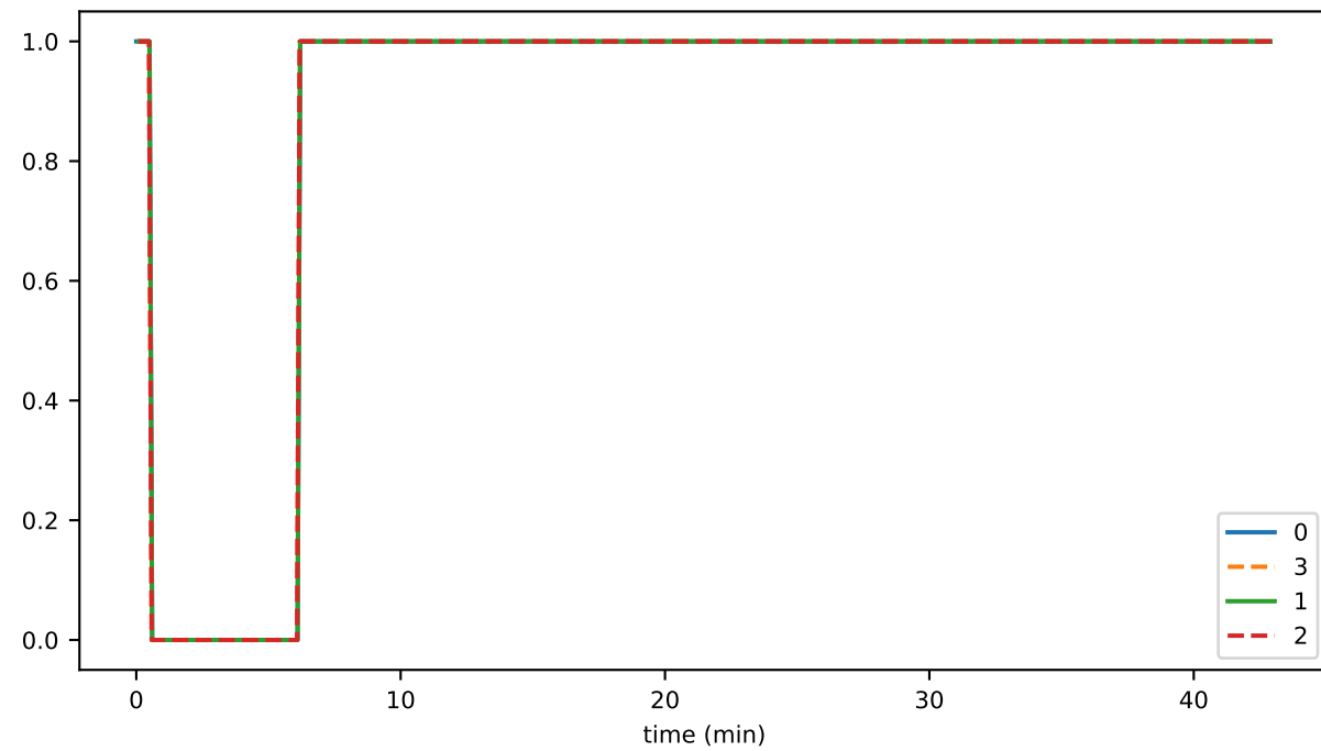
degraded
