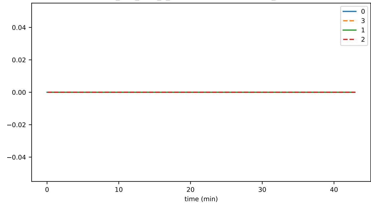
ds_files_level_5_leafKeysFileSizeByLevelMb_state
