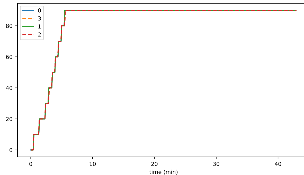
disconnects_per_sec_00
