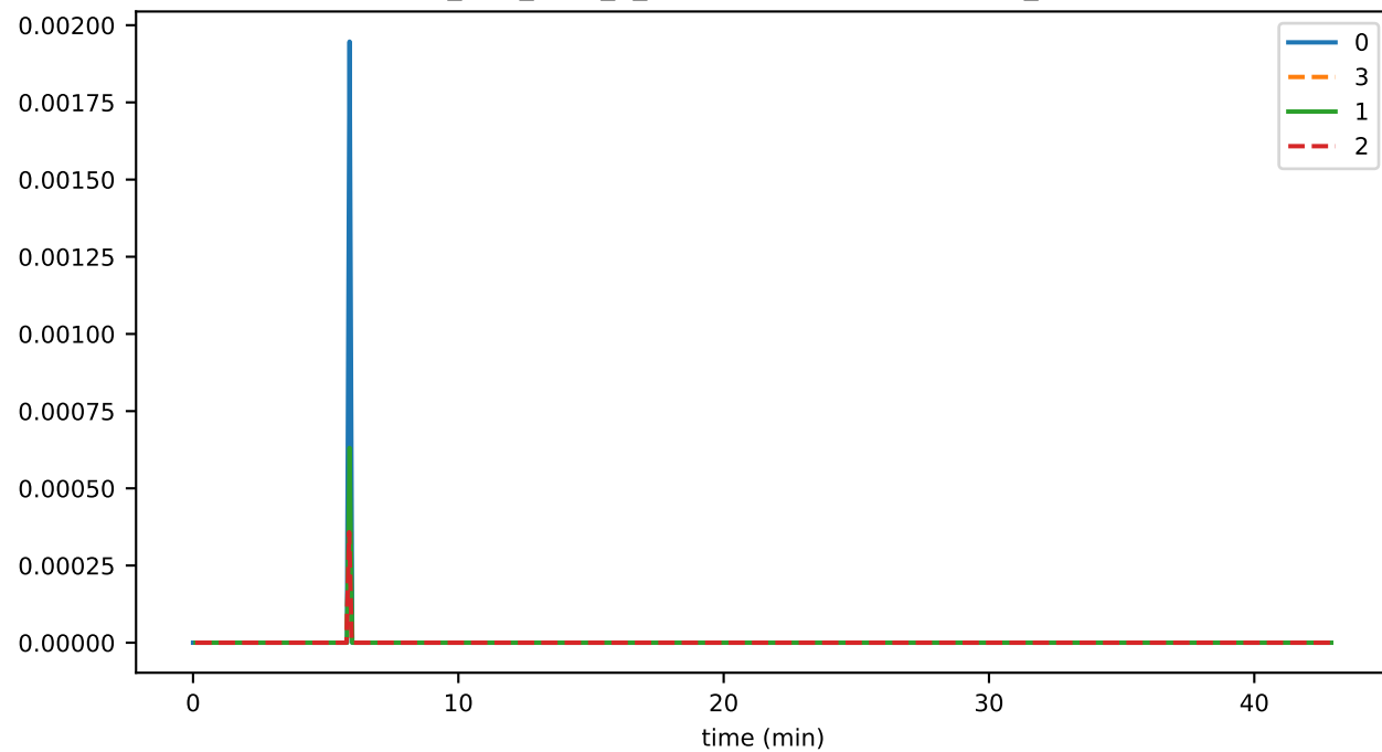
ds_files_level_2_leafKeysFileSizeByLevelMb_state
