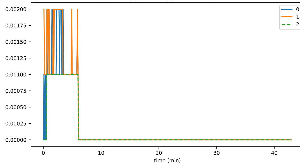
sync_phase_03_fraction_EXCHANGING_WINDOWS
