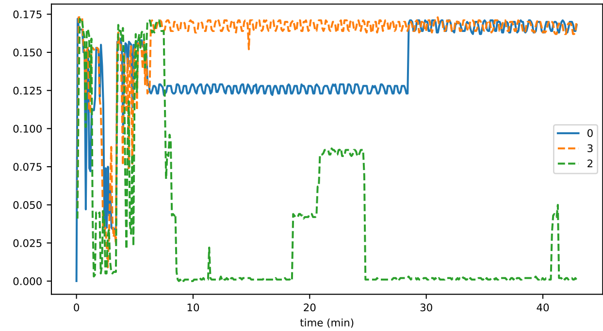
sync_phase_01_fraction_EXCHANGING_WINDOWS
