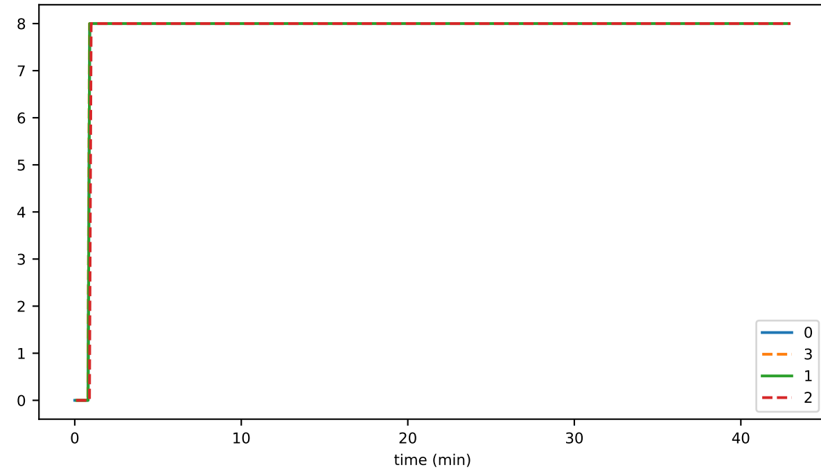
ds_reads_hashes_state
