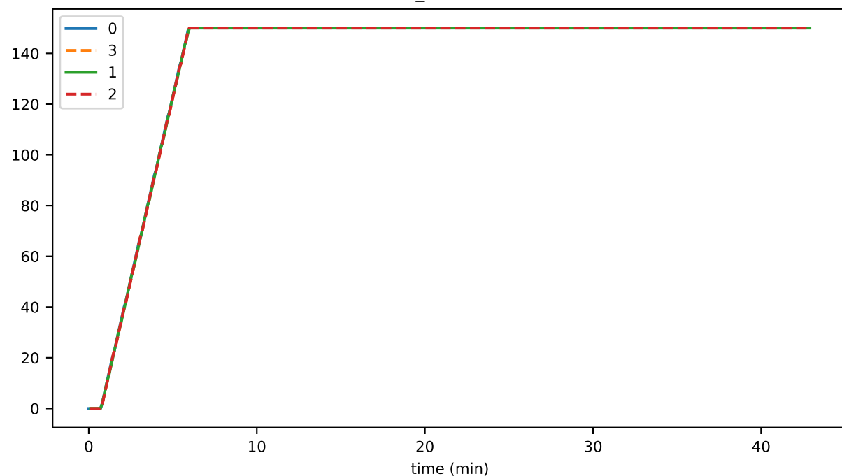
buffer_numBlocksMissing
