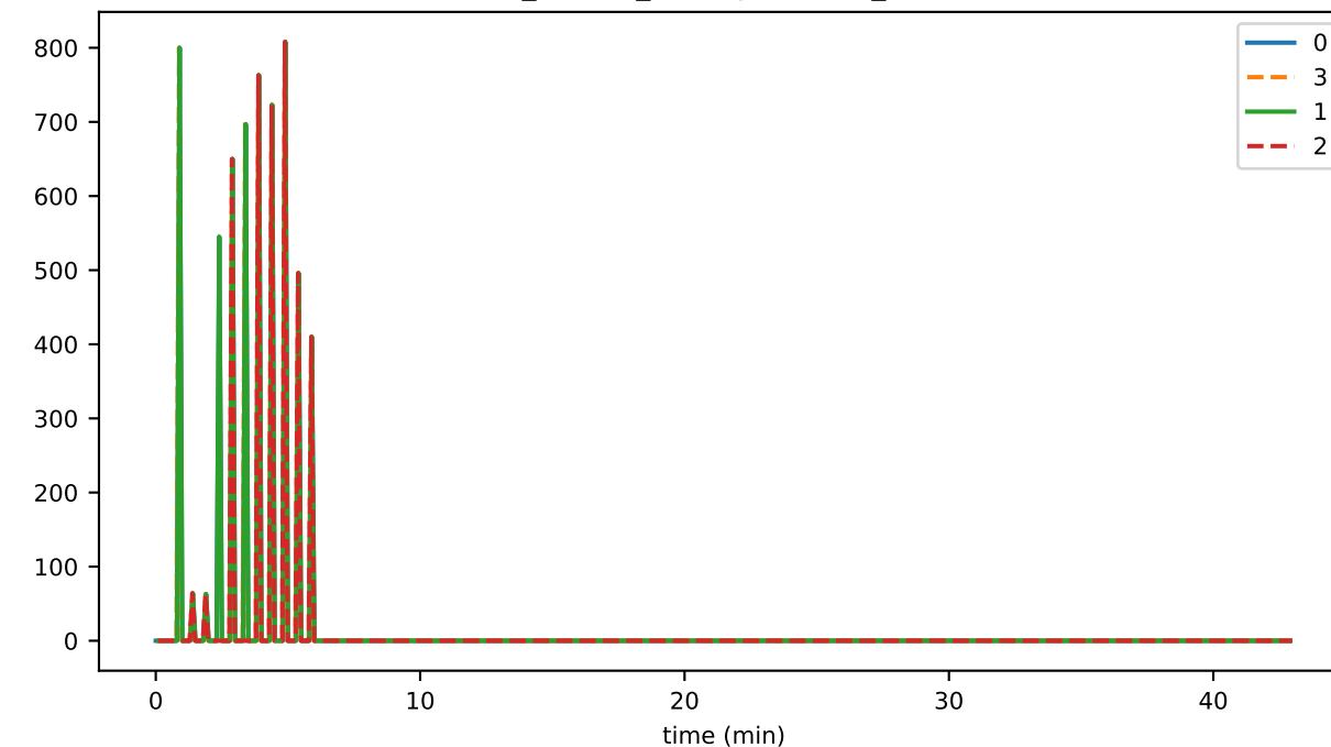
ds_flushes_leavesStoreFileSizeMb_state
