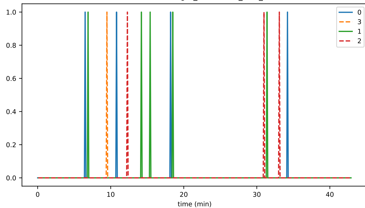
EventManager_unhandled_task_count
