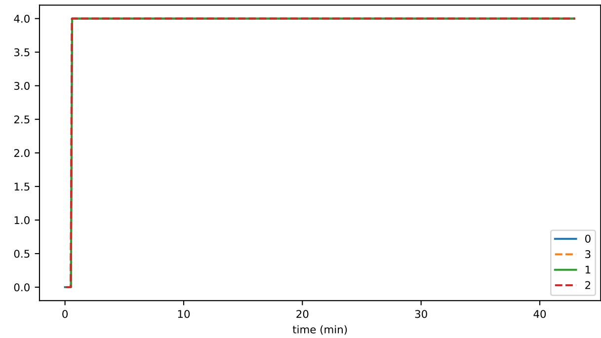
nodesUsed
