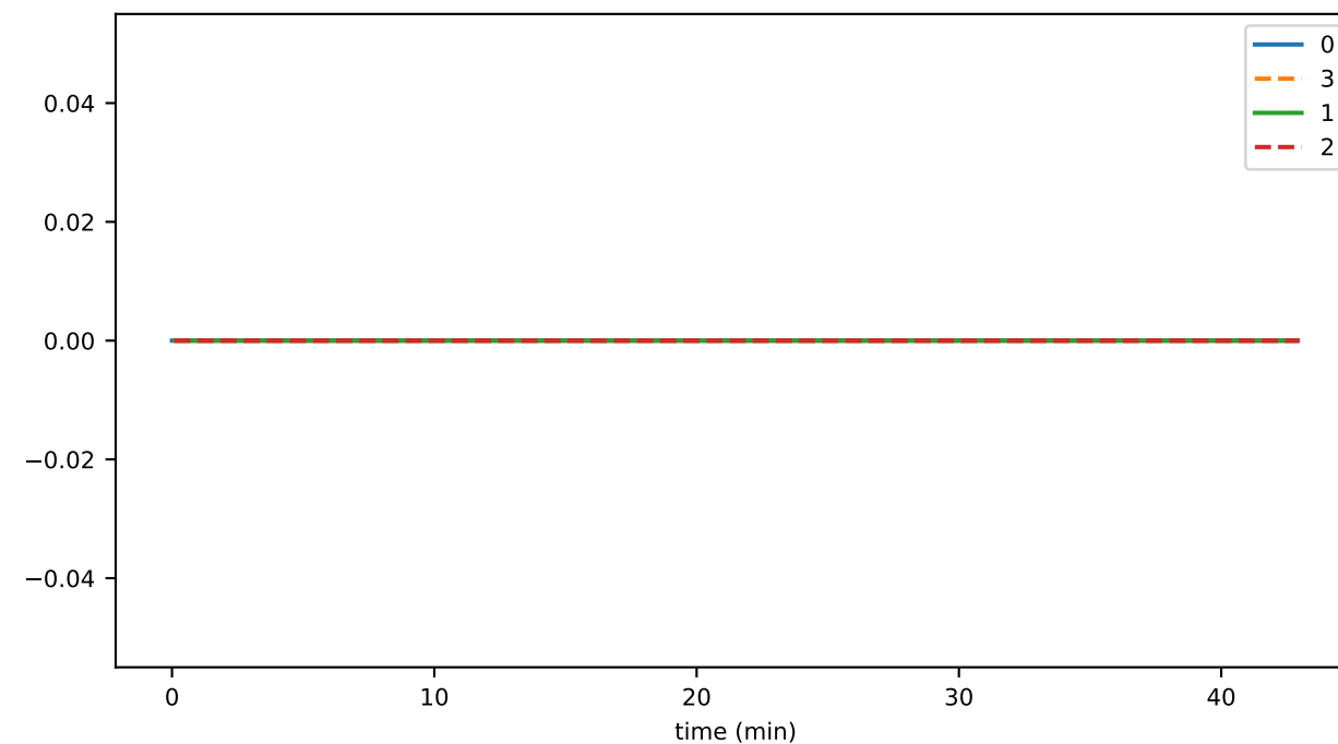
startsReconnectAsSender
