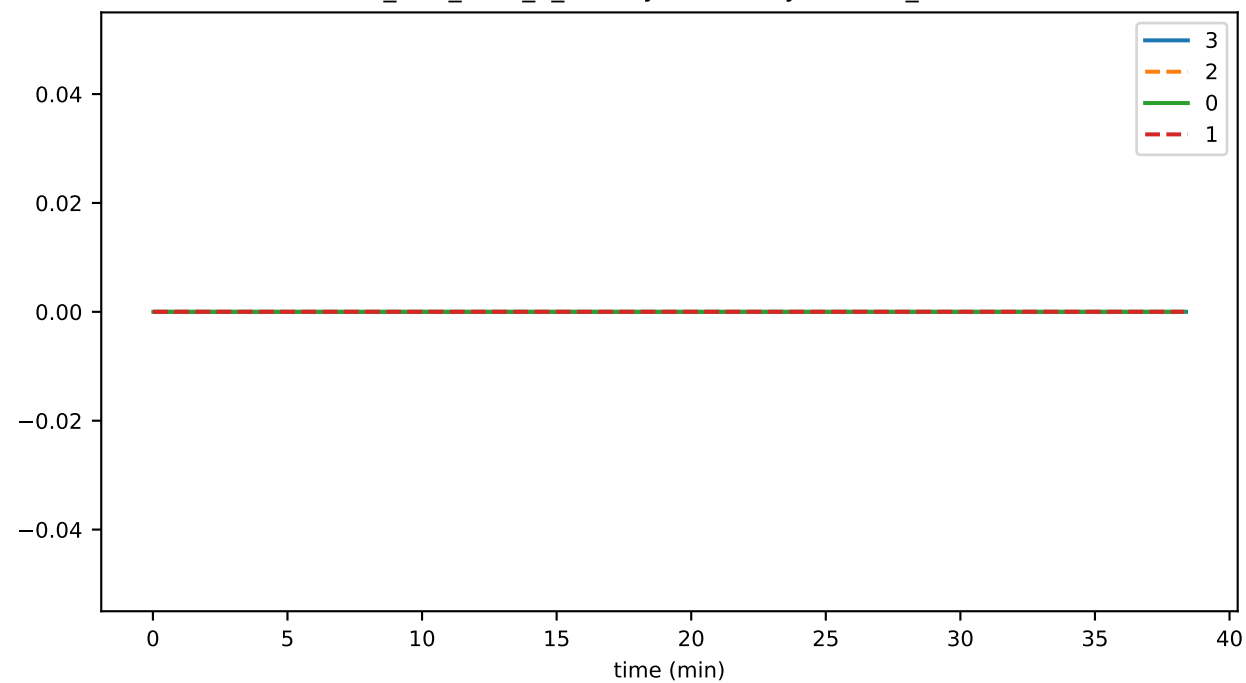
ds_files_level_2_leafKeysFileSizeByLevelMb_state
