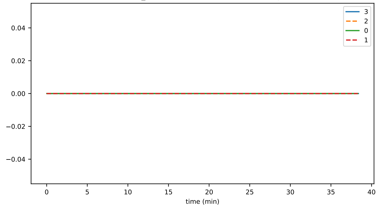
conn_onComplete
