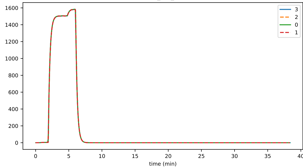
trans_per_sec
