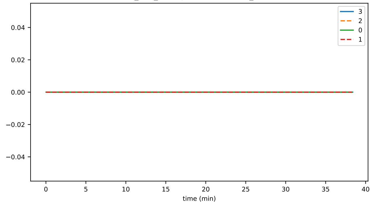
ds_files_leavesStoreFileSizeMb_state
