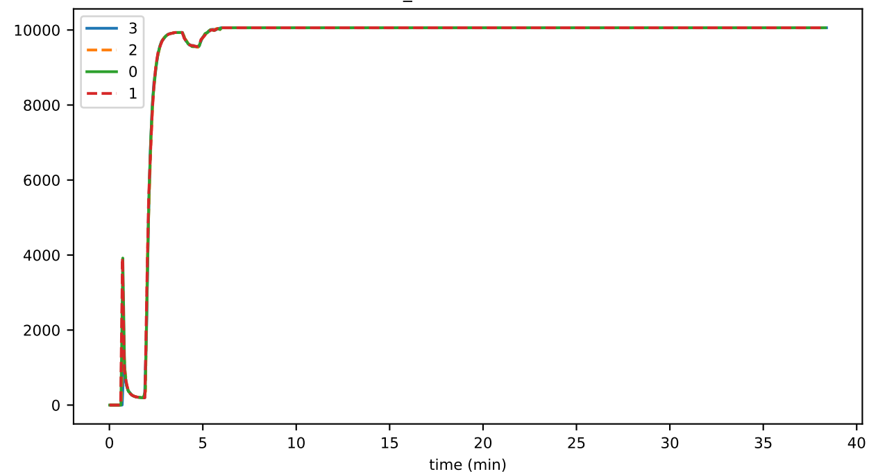
buffer_latestBlockOpened
