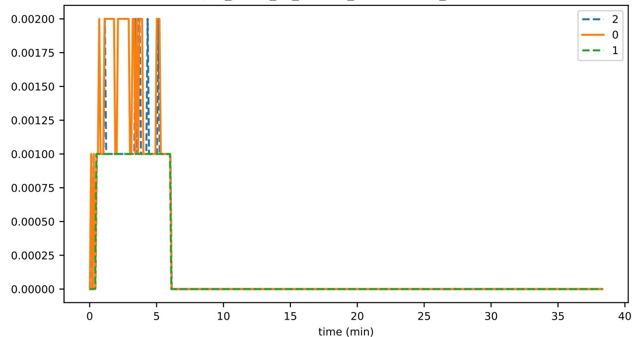
sync_phase_03_fraction_EXCHANGING_WINDOWS
