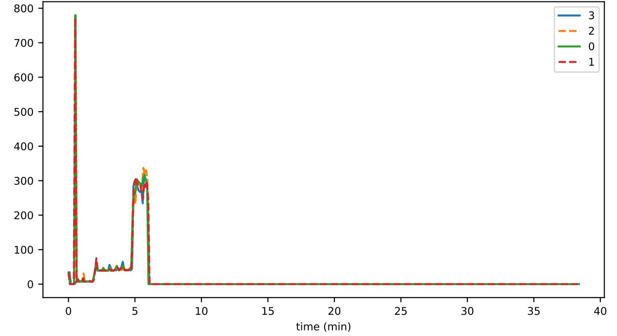
ds_reads_leafKeys_state
