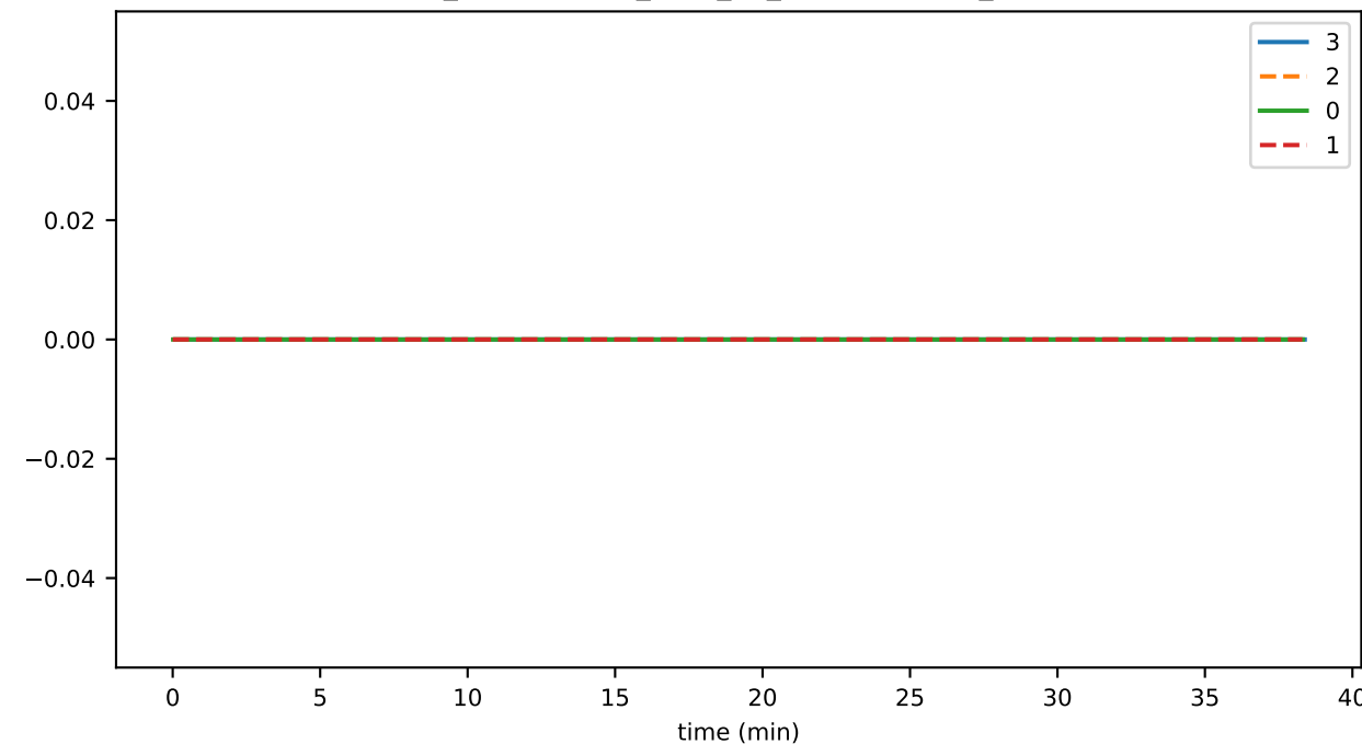
ds_compactions_level_10_leavesTimeMs_state
