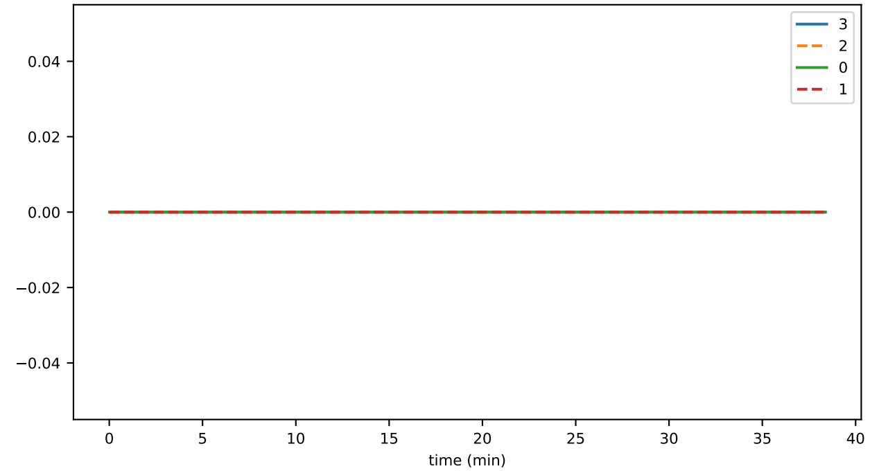
sync_per_secC
