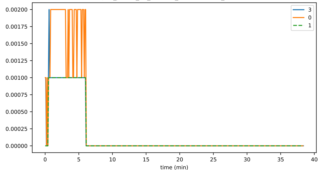
sync_phase_02_fraction_EXCHANGING_WINDOWS
