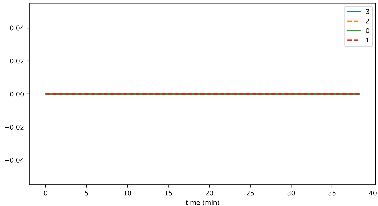
ds_files_level_6_leafKeysFileSizeByLevelMb_state
