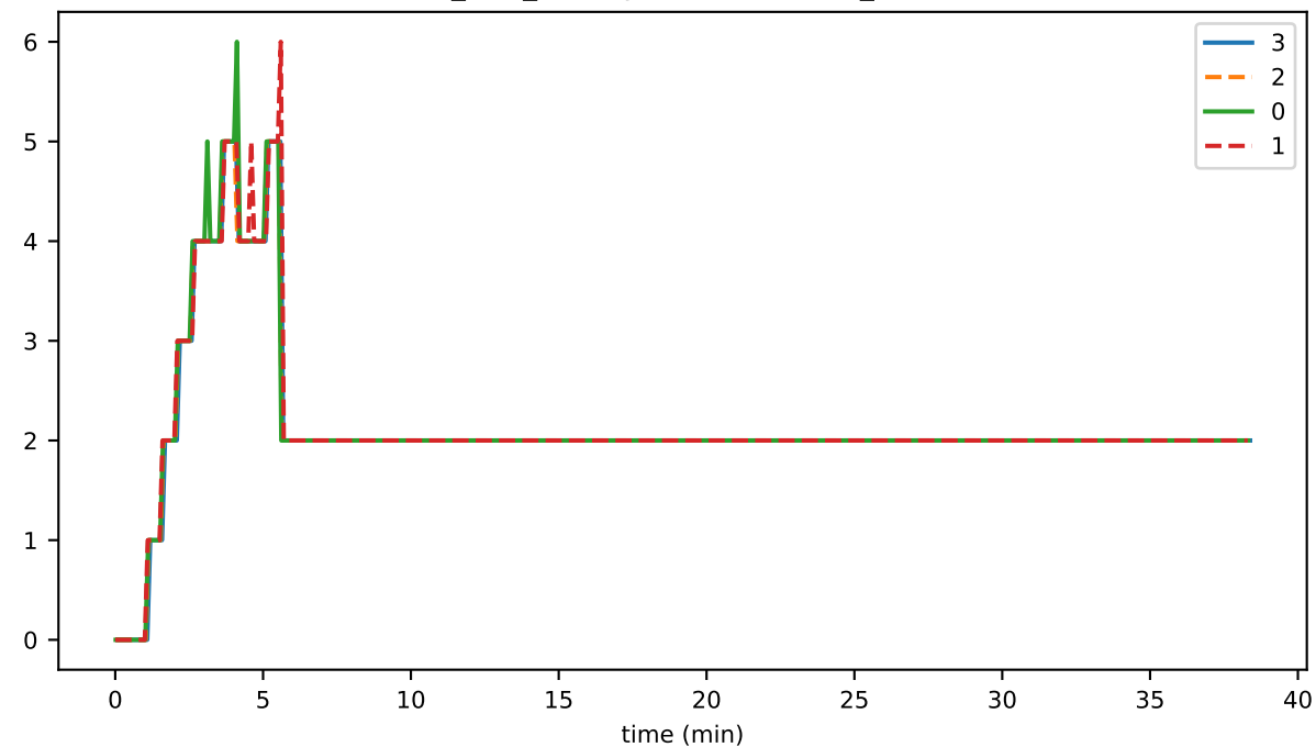
ds_files_leavesStoreFileCount_state
