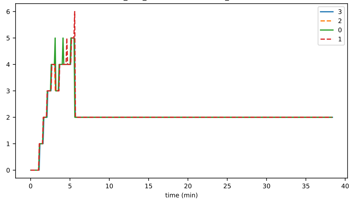
ds_files_leavesStoreFileCount_state
