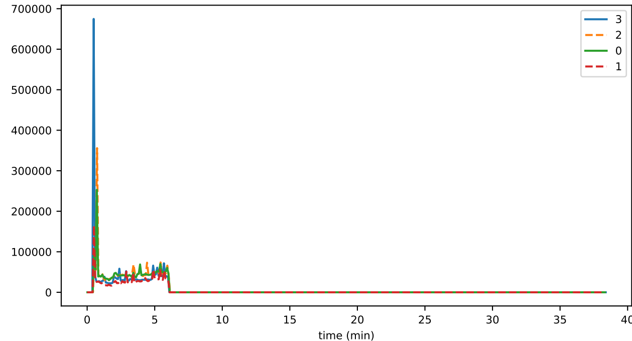
pcesAvgTotalWriteDuration
