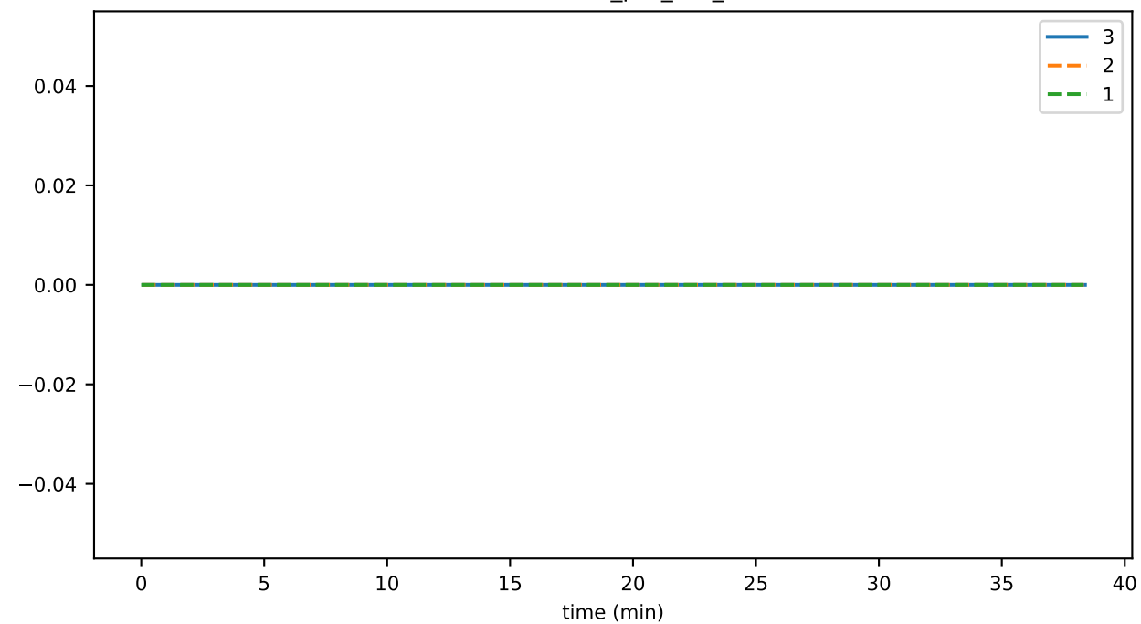
disconnects_per_sec_00
