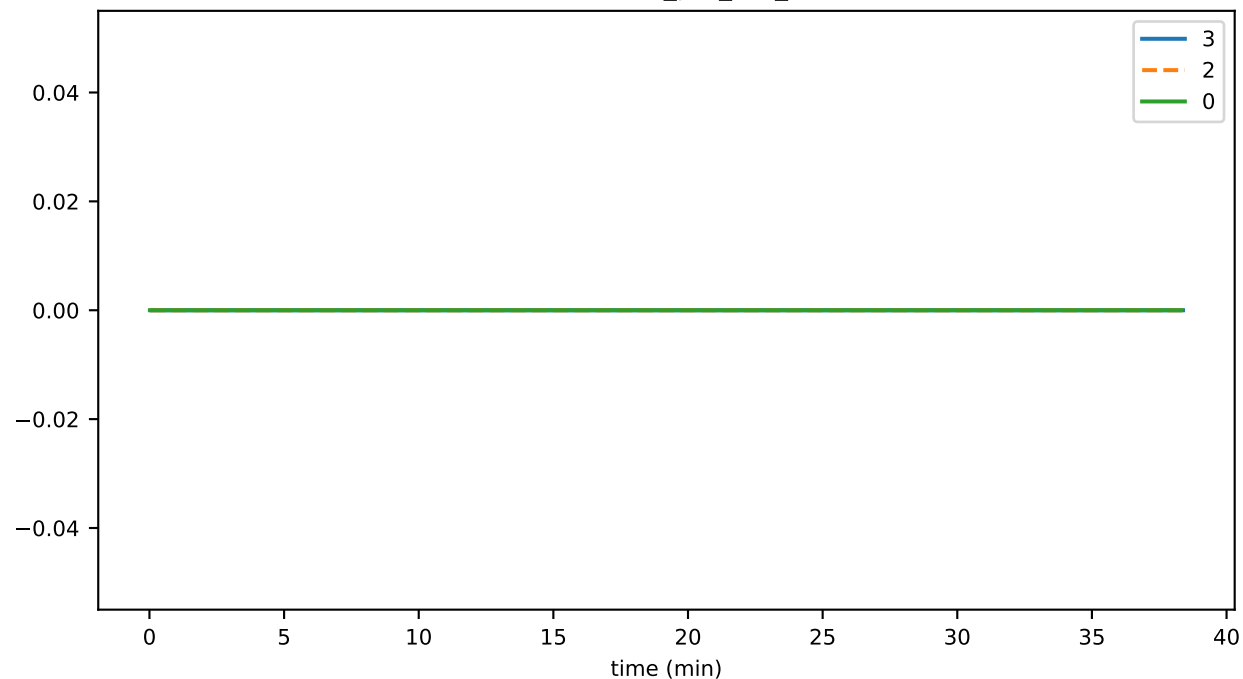
disconnects_per_sec_03
