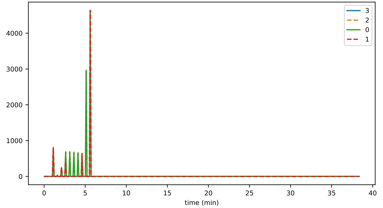
ds_flushes_leavesStoreFileSizeMb_state
