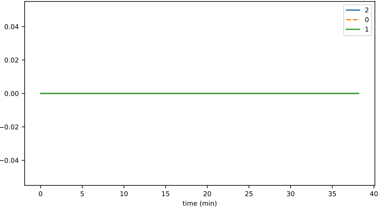
SmartContractService:SystemContractMethodCall_DIRECT_total
