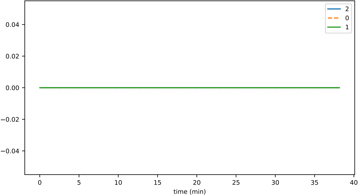
SmartContractService:SystemContractMethodCall_KYC_failed
