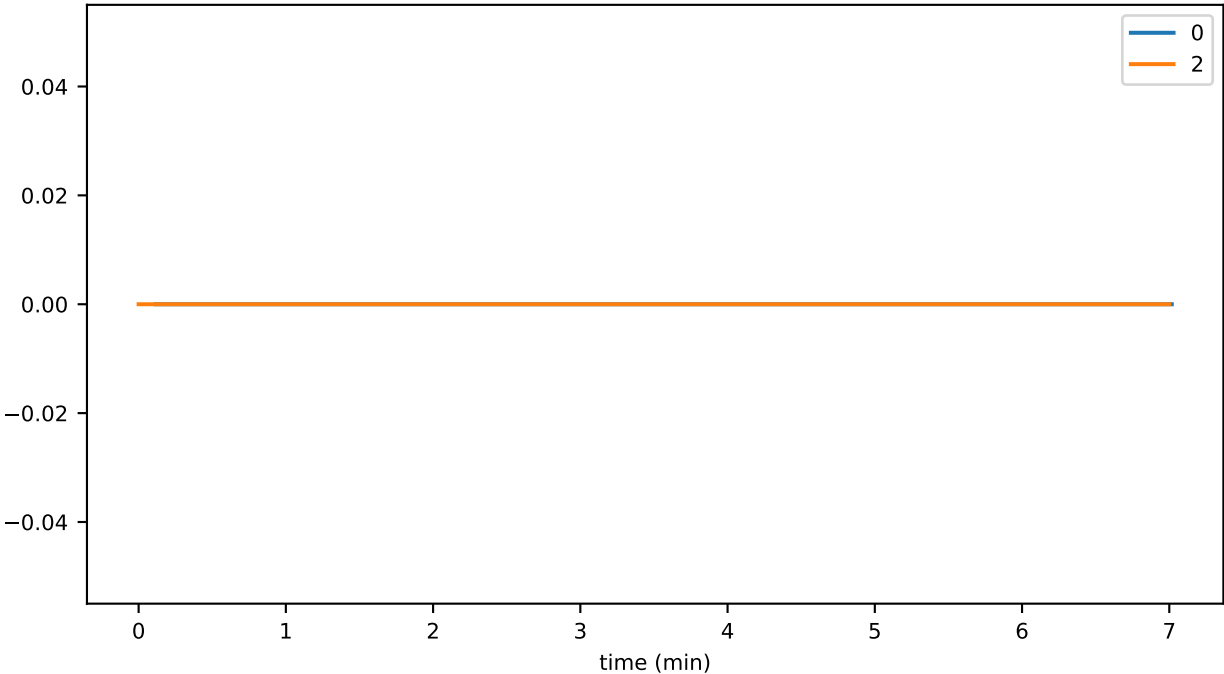
sync_phase_02_fraction_EXCHANGING_TIPS
