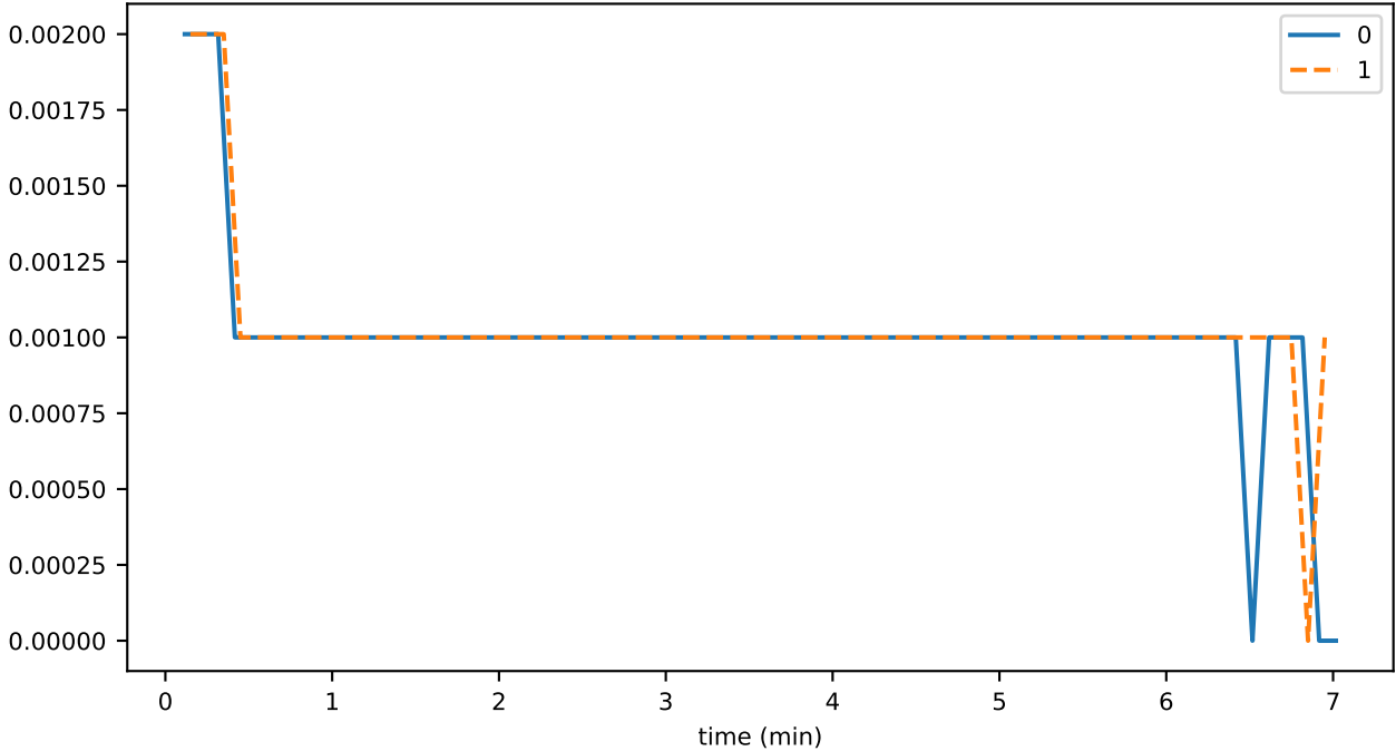
sync_phase_02_fraction_EXCHANGING_EVENTS
