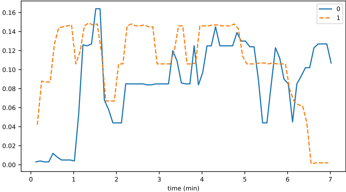
sync_phase_02_fraction_EXCHANGING_TIPS
