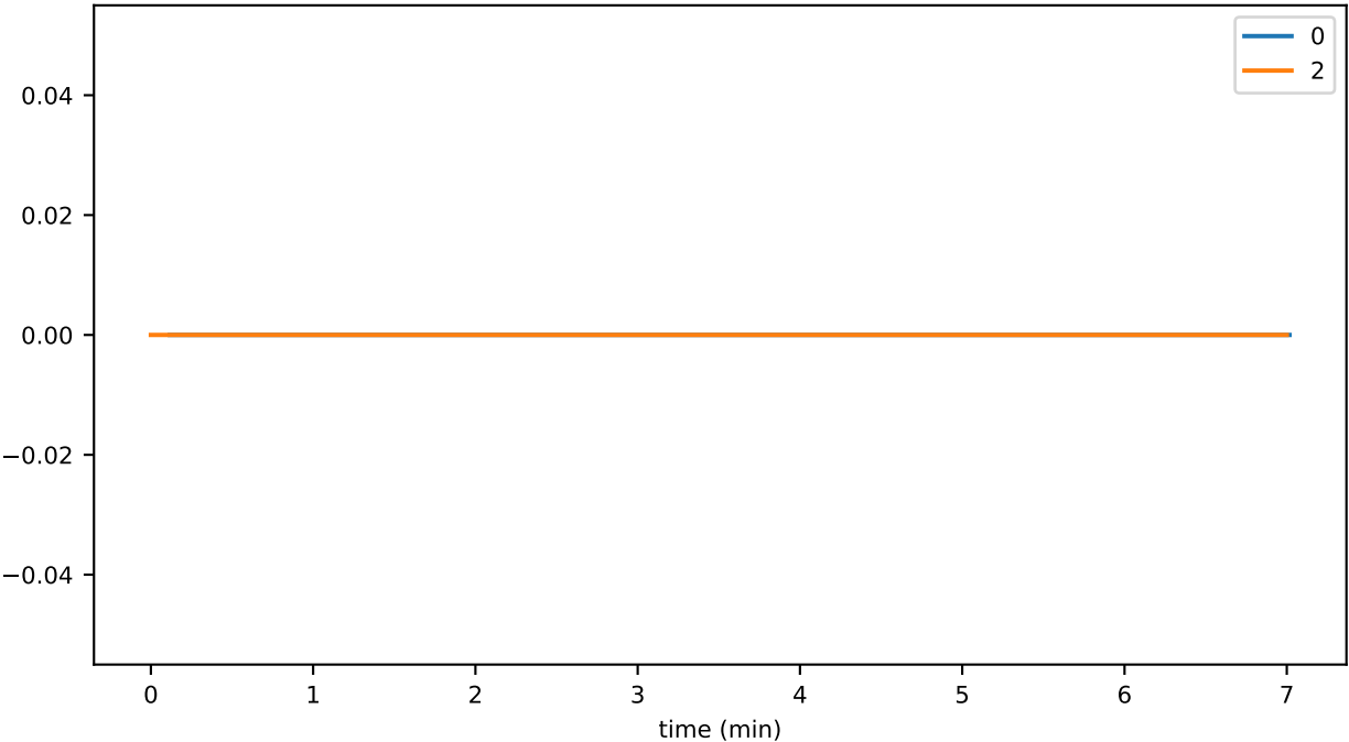
sync_phase_02_fraction_EXCHANGING_EVENTS
