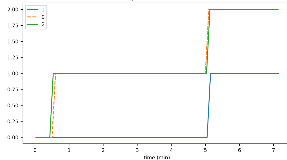
historyProofTransR2ToFailCnt
