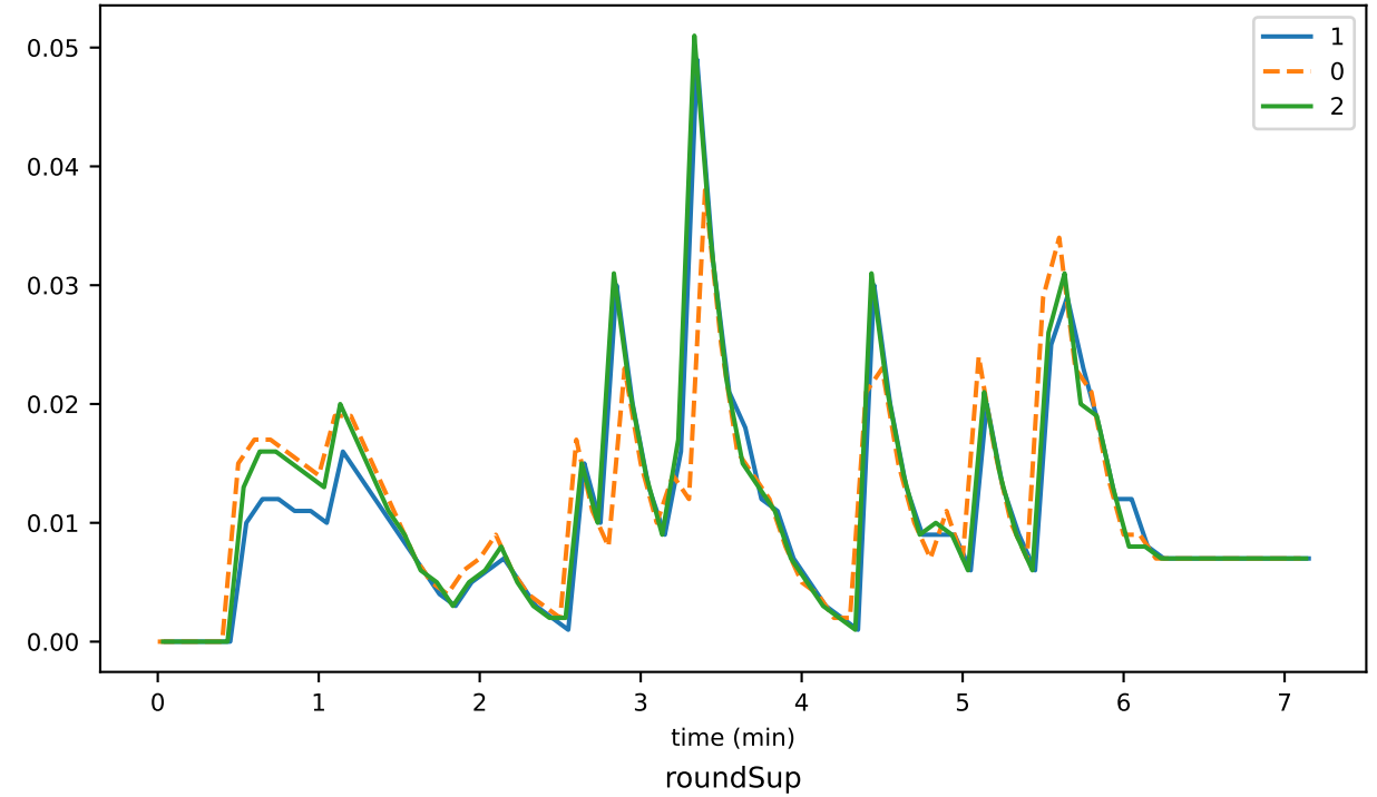
roundsSinceLastConsensusEvent_1
