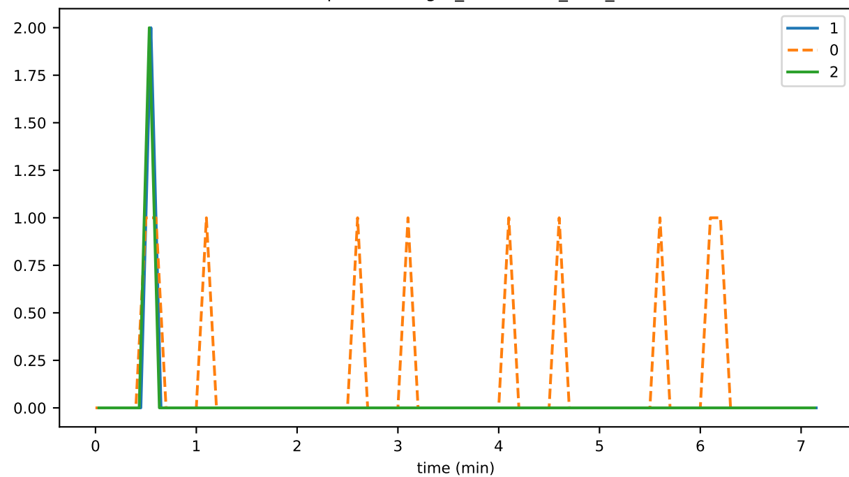
StateSnapshotManager_unhandled_task_count
