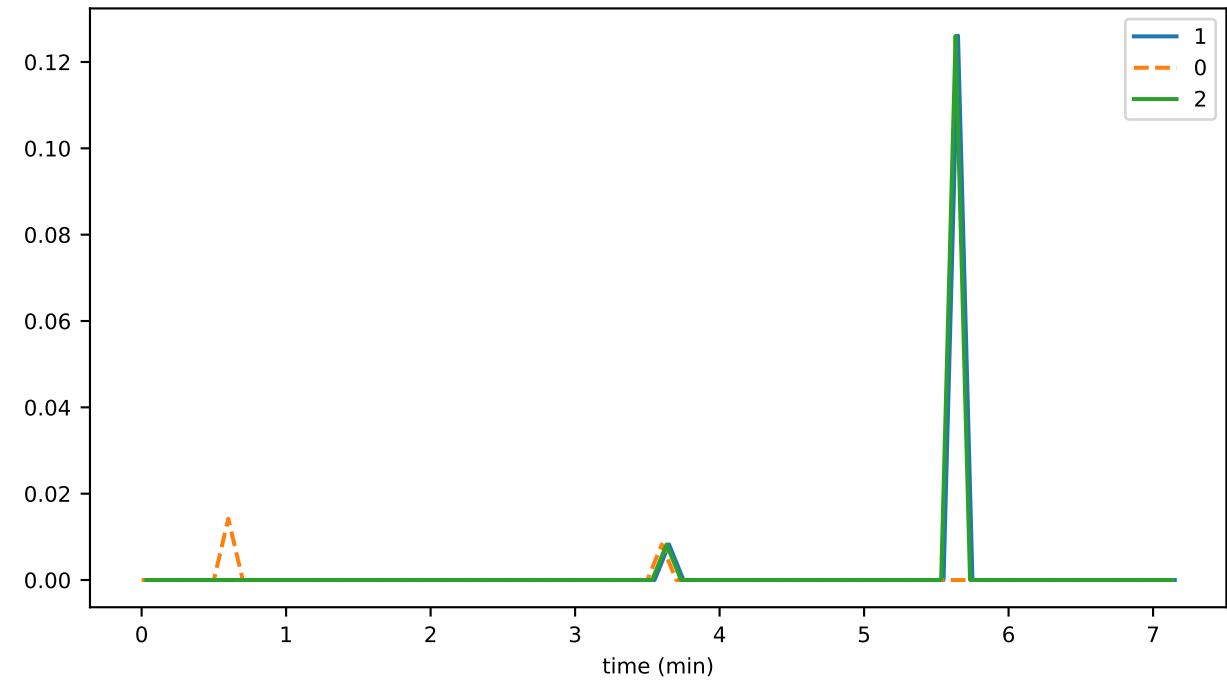
ds_compactions_level_2_leavesSavedSpaceMb_state
