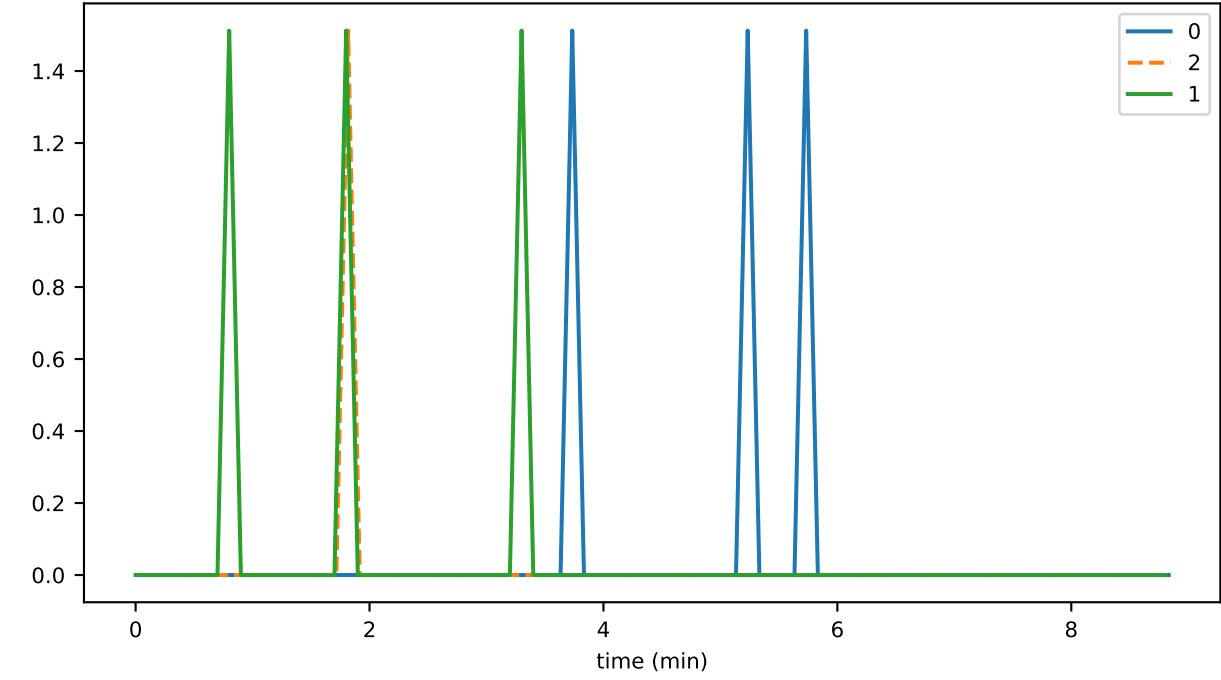
ds_files_level_1_hashesFileSizeByLevelMb_state
