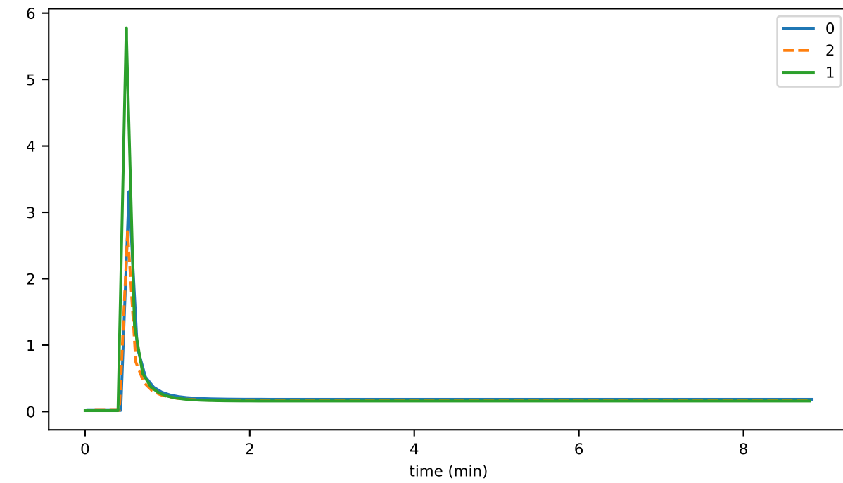
secR2C
