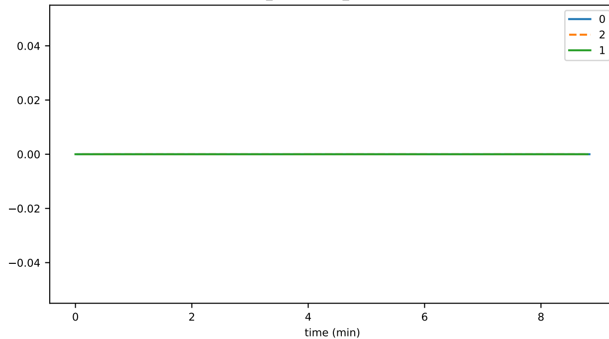
connRecv_endStream_persistenceFailed
