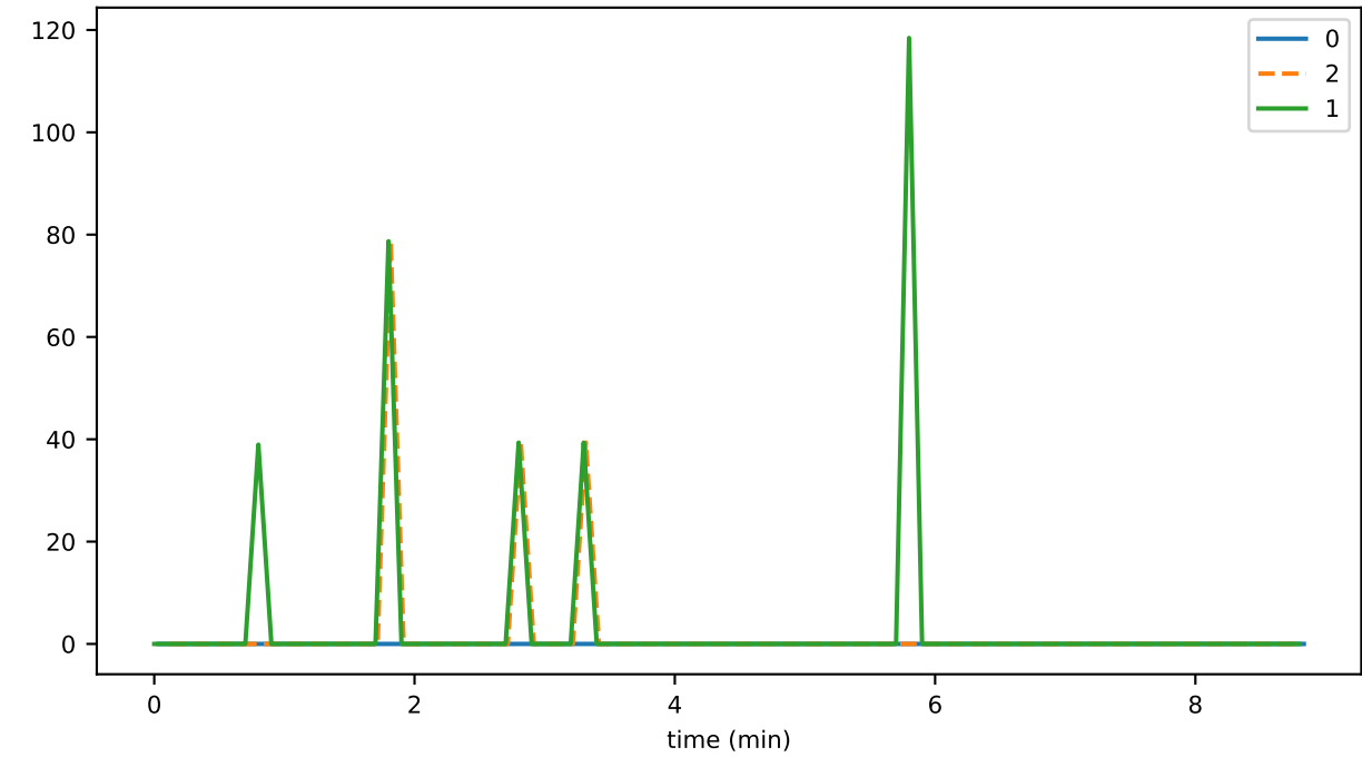
ds_files_level_2_leafKeysFileSizeByLevelMb_state
