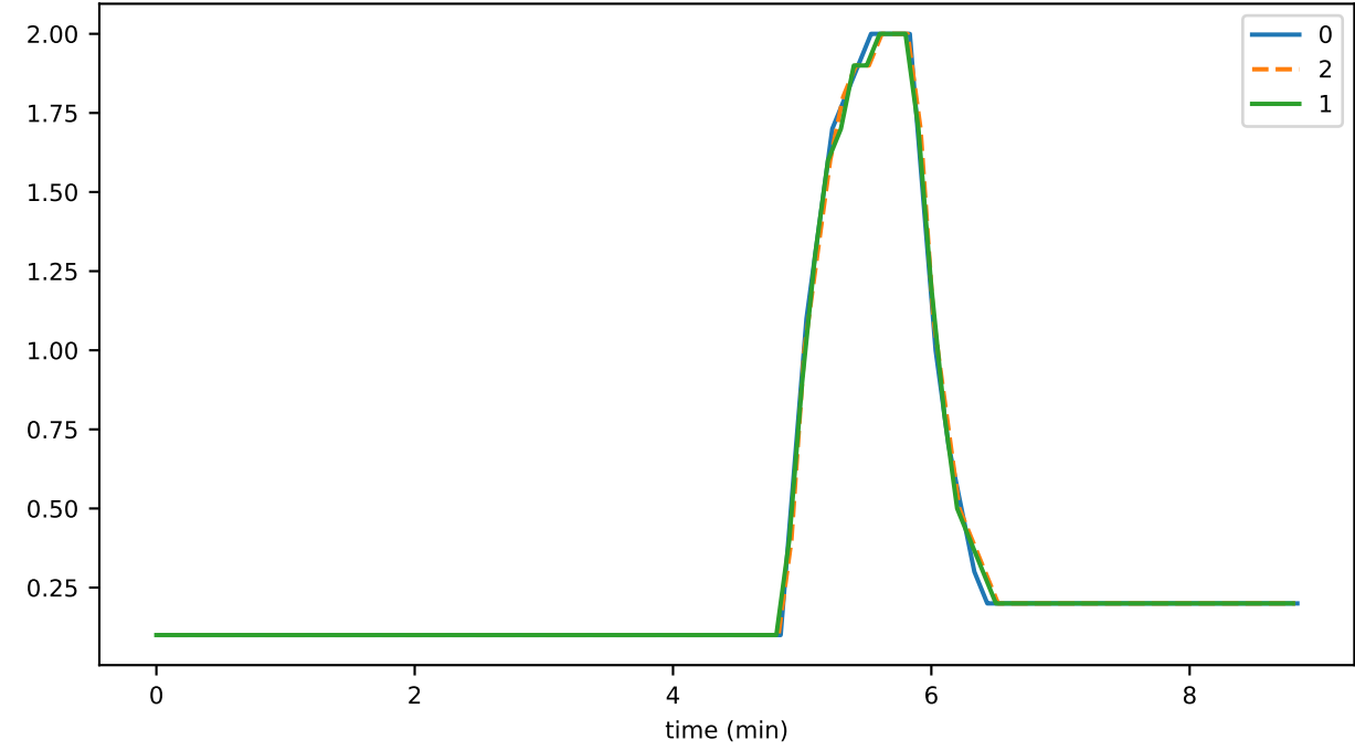
trans_per_event
