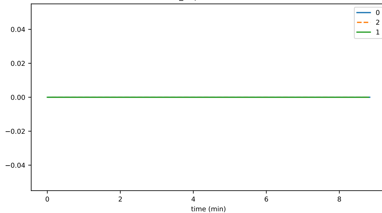
connSend_requestBlockItemCount
