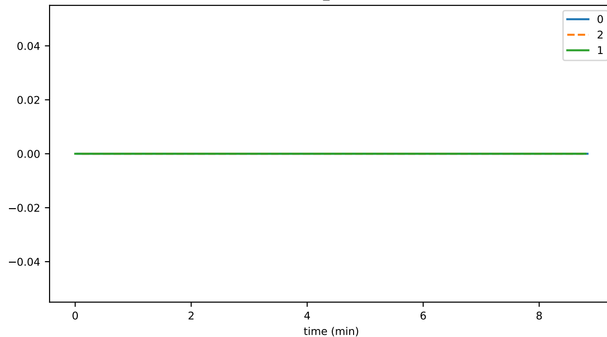
conn_connClose_blockNodeHighLatency
