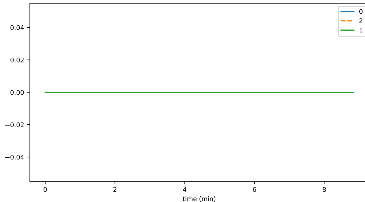
ds_files_level_7_leavesFileSizeByLevelMb_state
