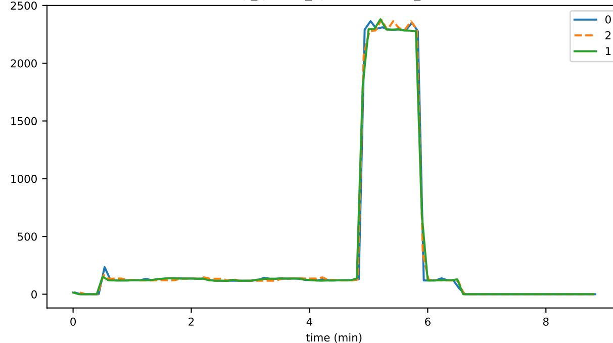
witnessesSeen
