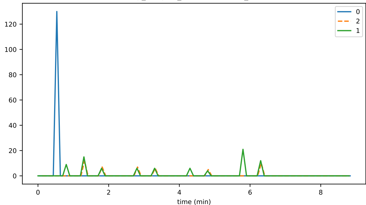
vmap_lifecycle_mergeDurationMs_state
