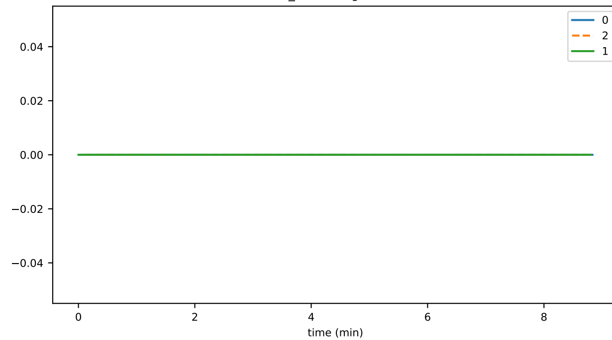
connSend_streamingBlockNumber
