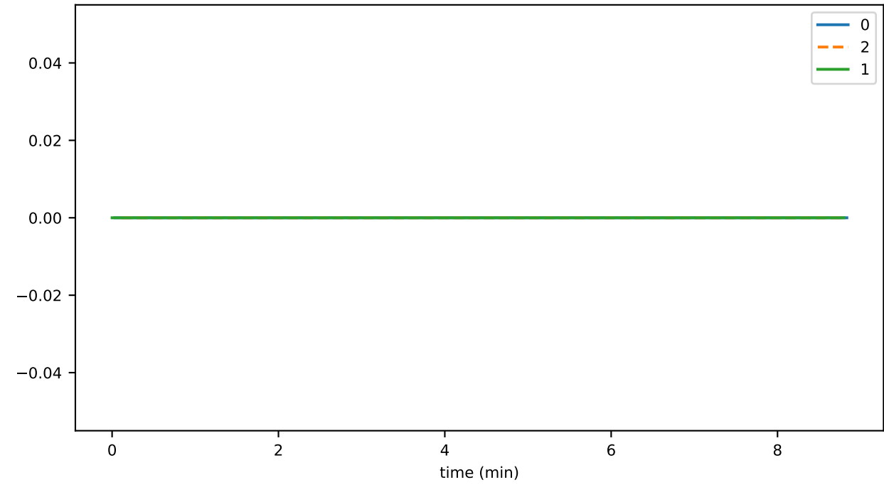
numEventsAddedUntilConsensus
