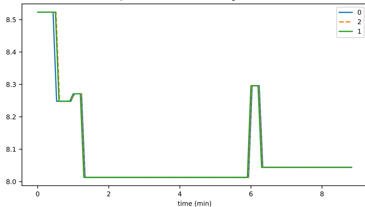
preconsensusEventFileOldestIdentifier
