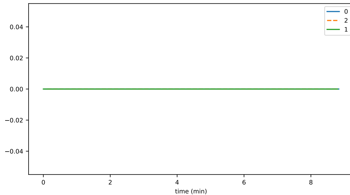
uNRECOGNIZEDDurationMax
