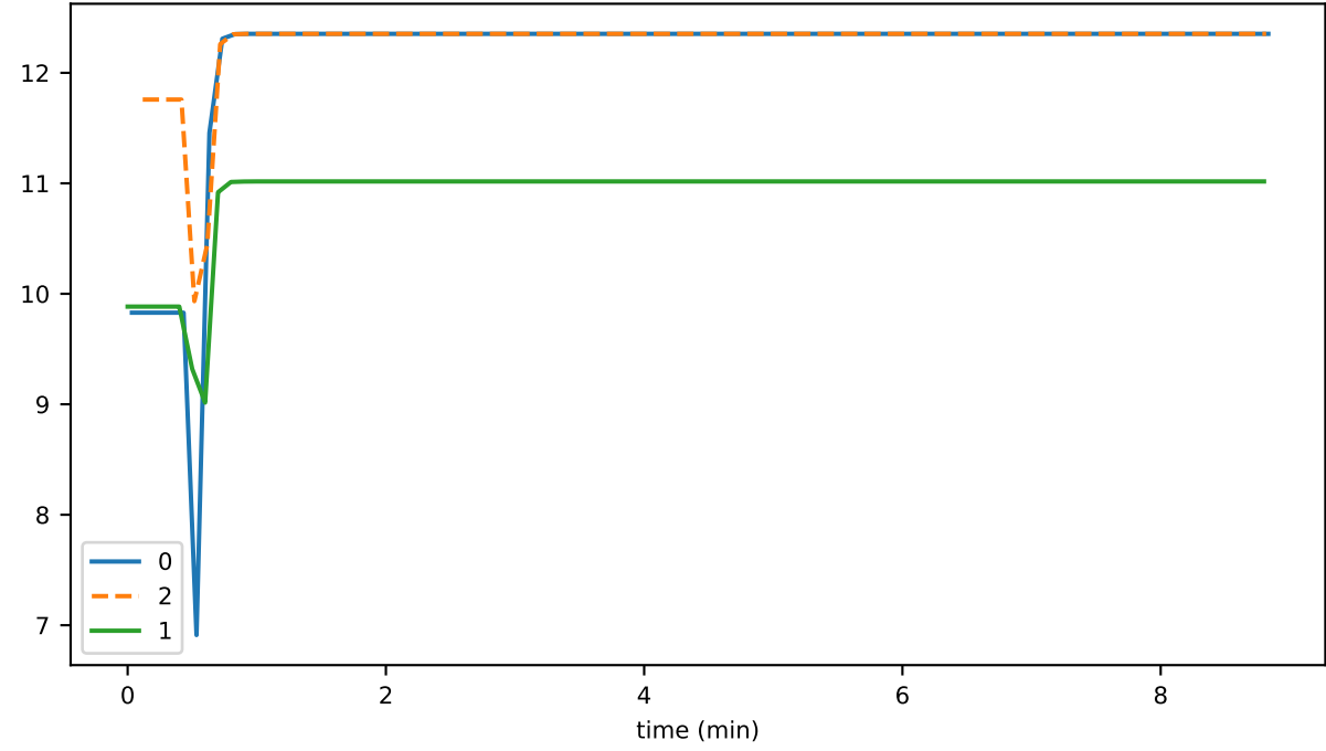
numEventsAddedUntilConsensus
