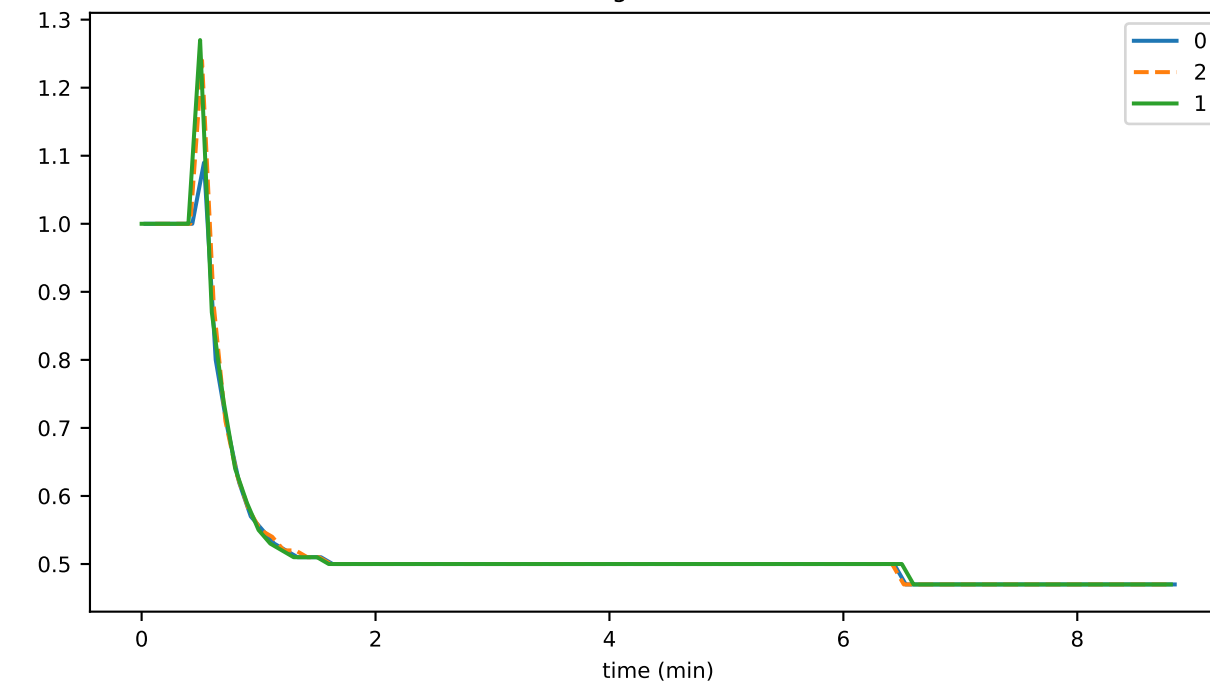
utilPrngDurationAvg
