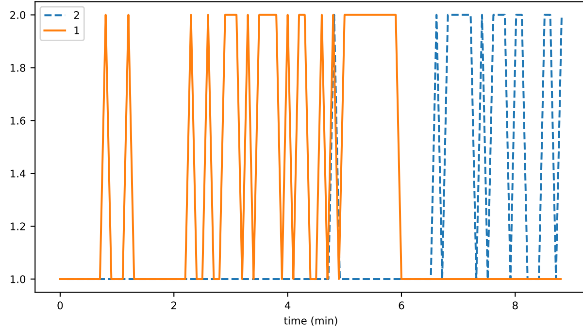
rpc_input_00_queueMaxSize
