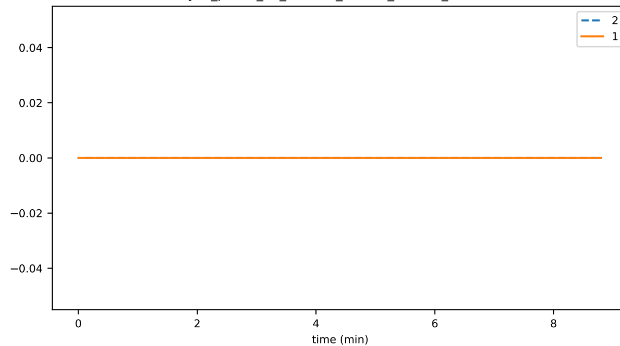
sync_phase_00_fraction_OTHER_FALLEN_BEHIND
