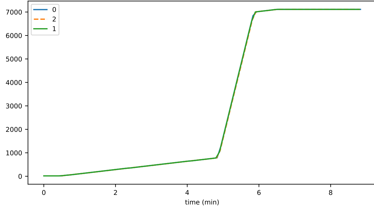
trans
