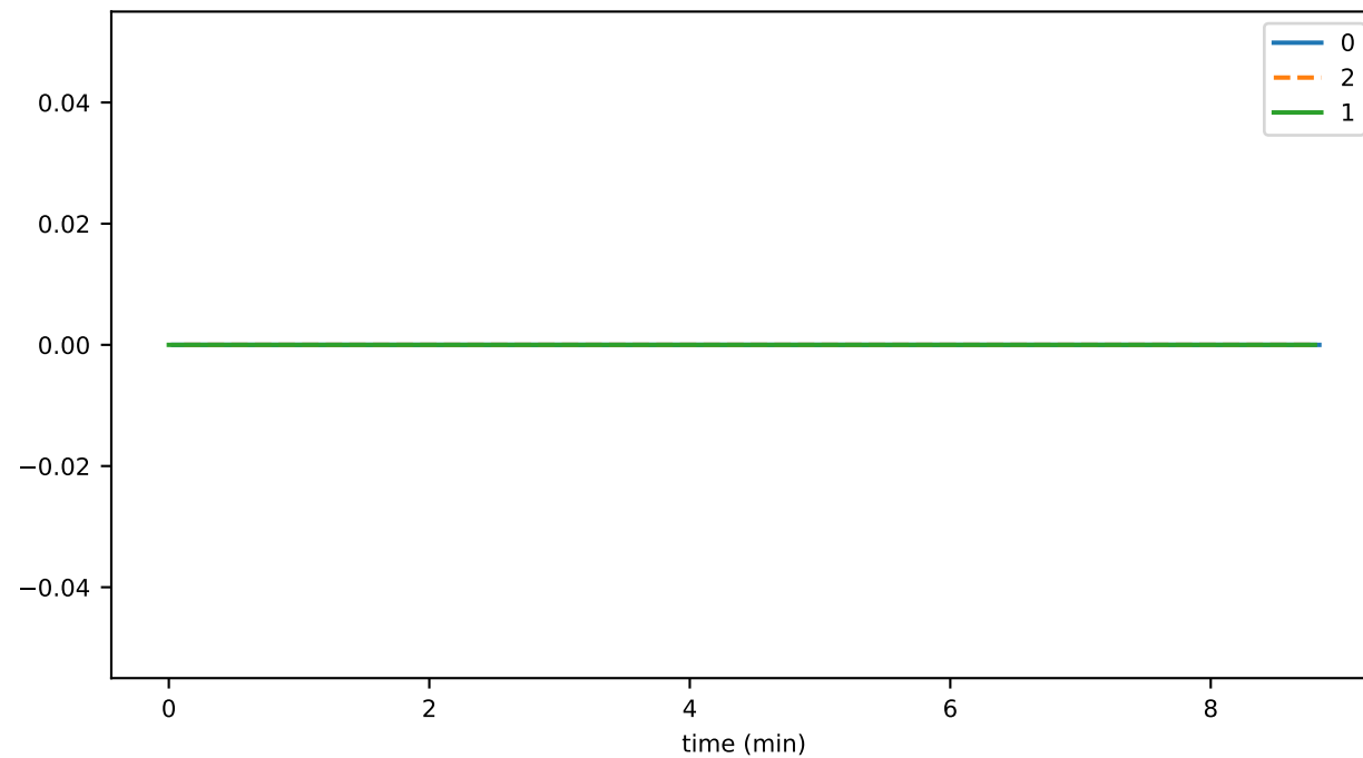
historyProofKeyPublicationThrottledTxns
