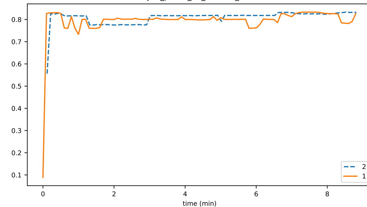
sync_phase_00_fraction_OTHER_FALLEN_BEHIND
