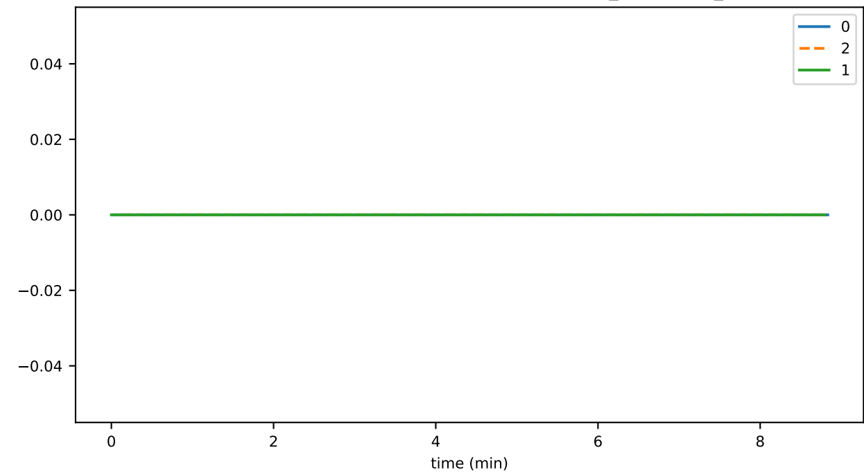
SmartContractService:SystemContractMethodCall_SCHEDULE_failed
