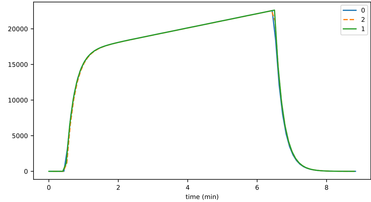
rpc_input_00_queueMinSize
