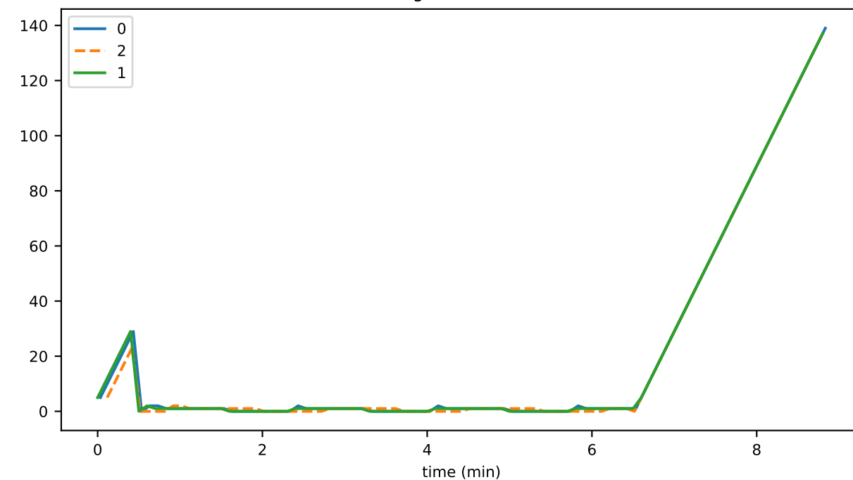
OrphanBuffer_busy_fraction
