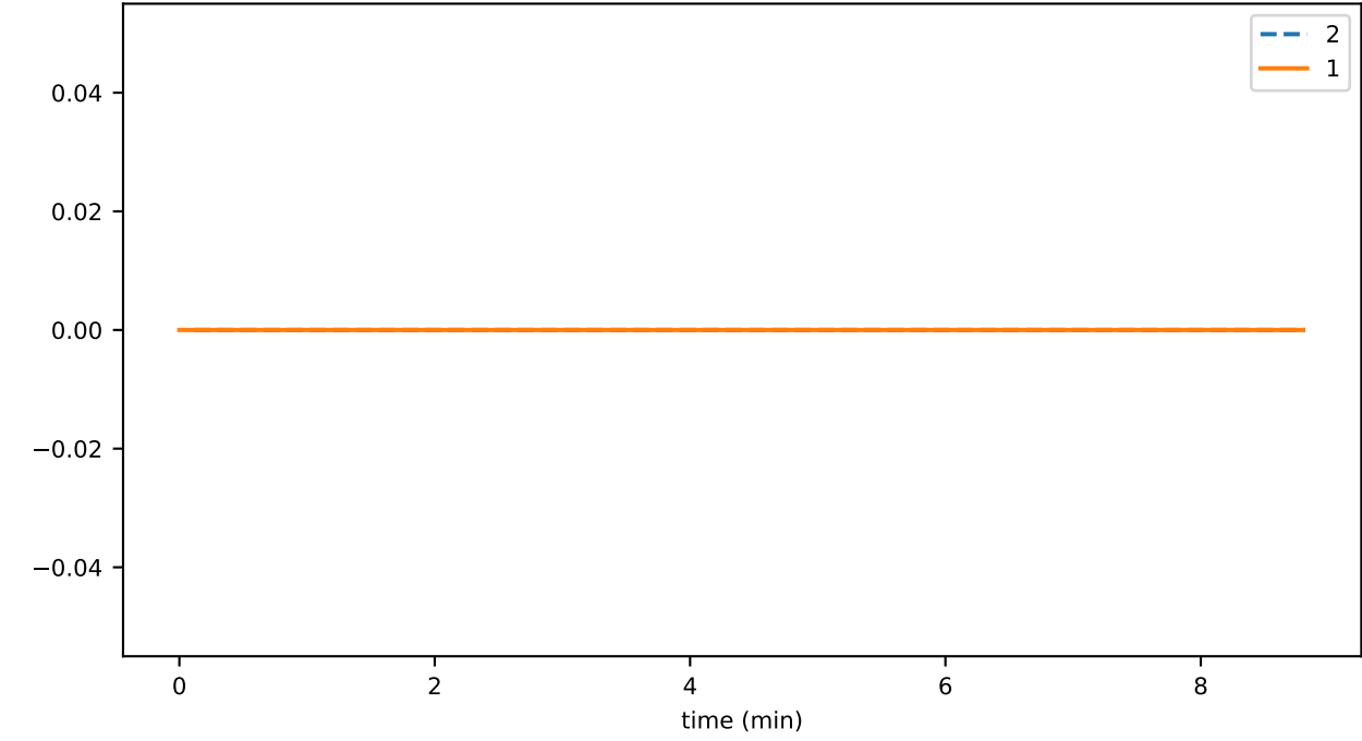
rpc_input_00_queueMinSize
