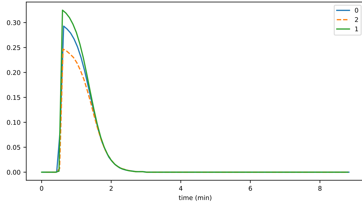
rpc_input_00_queueMaxSize
