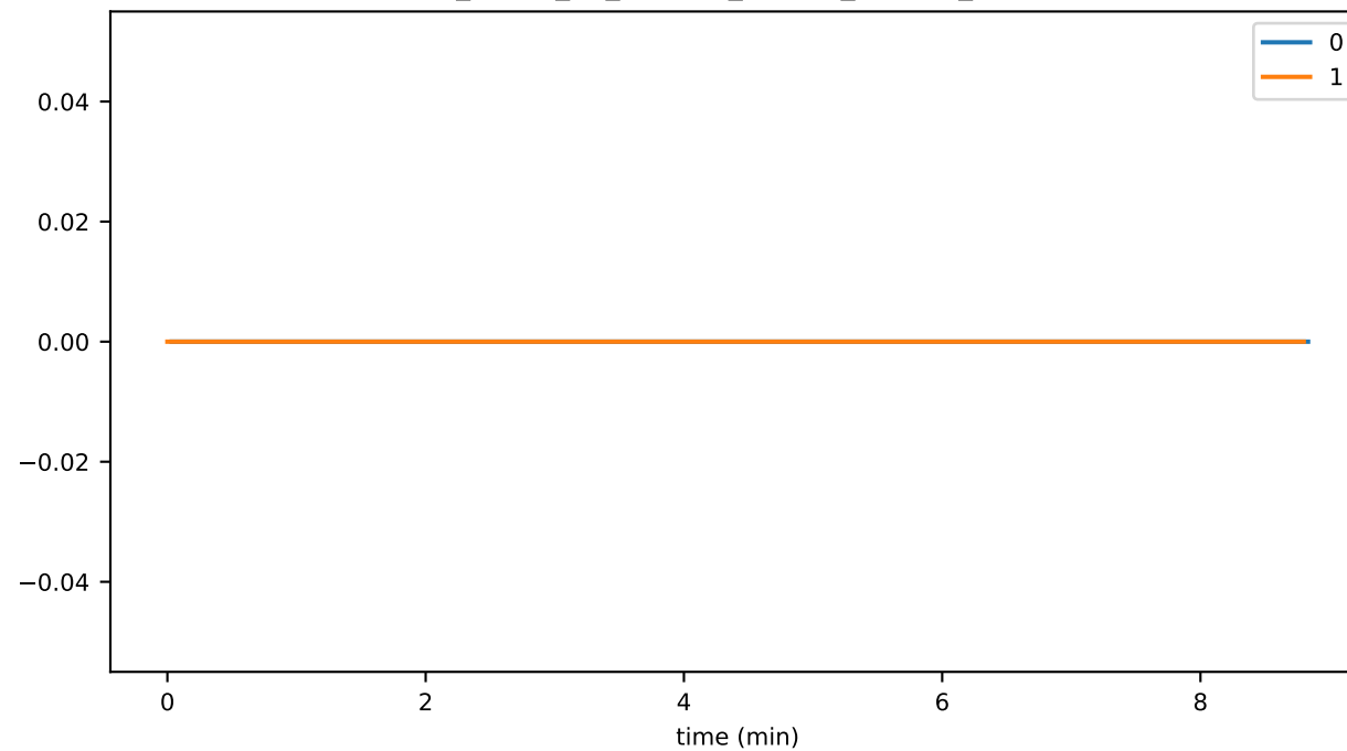
sync_phase_02_fraction_OTHER_FALLEN_BEHIND
