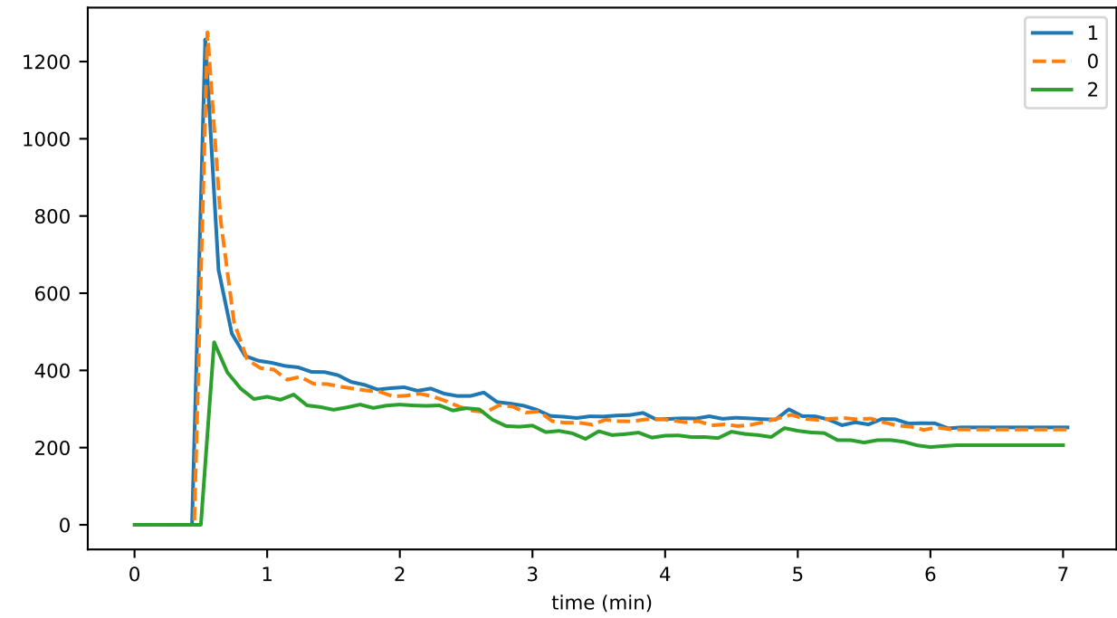
eventDelay_4_verification_gossip
