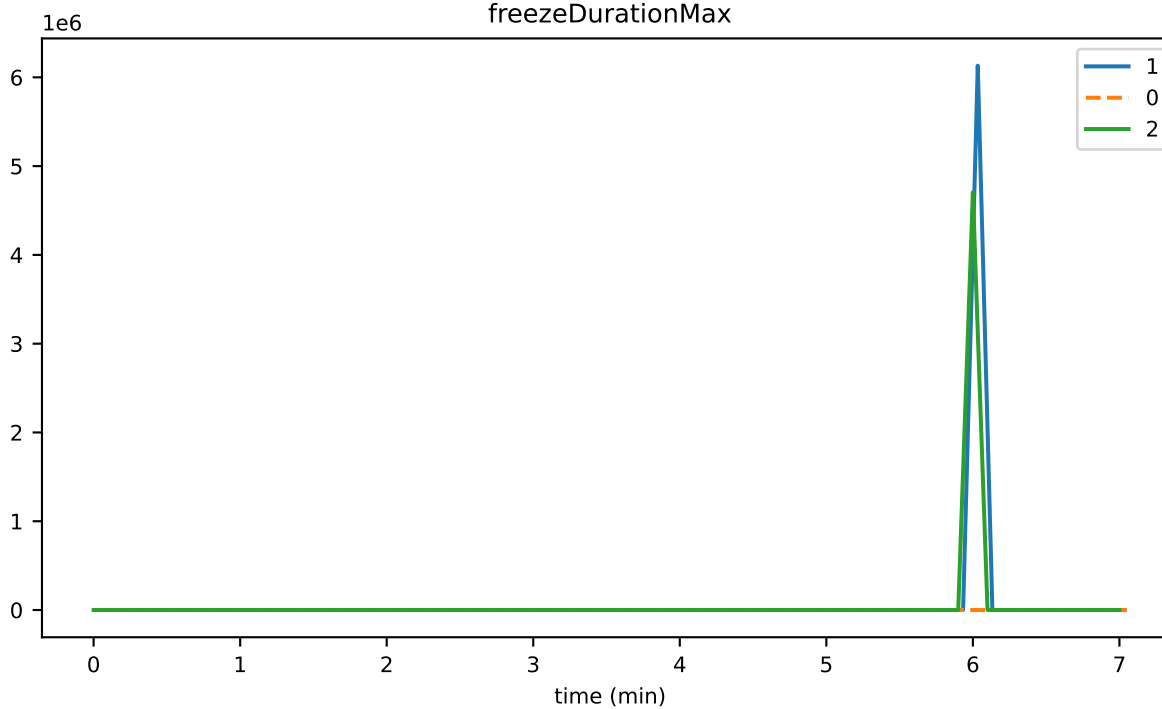
freezeDurationMax
