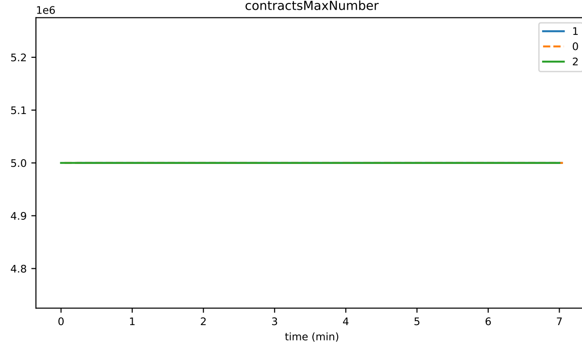
contractsMaxNumber
