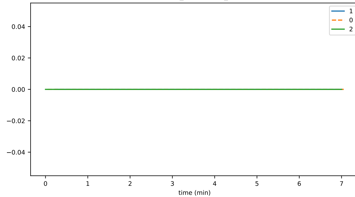
connSend_endStream_error
