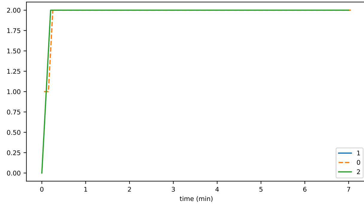
scheduleCreateDurationMax
