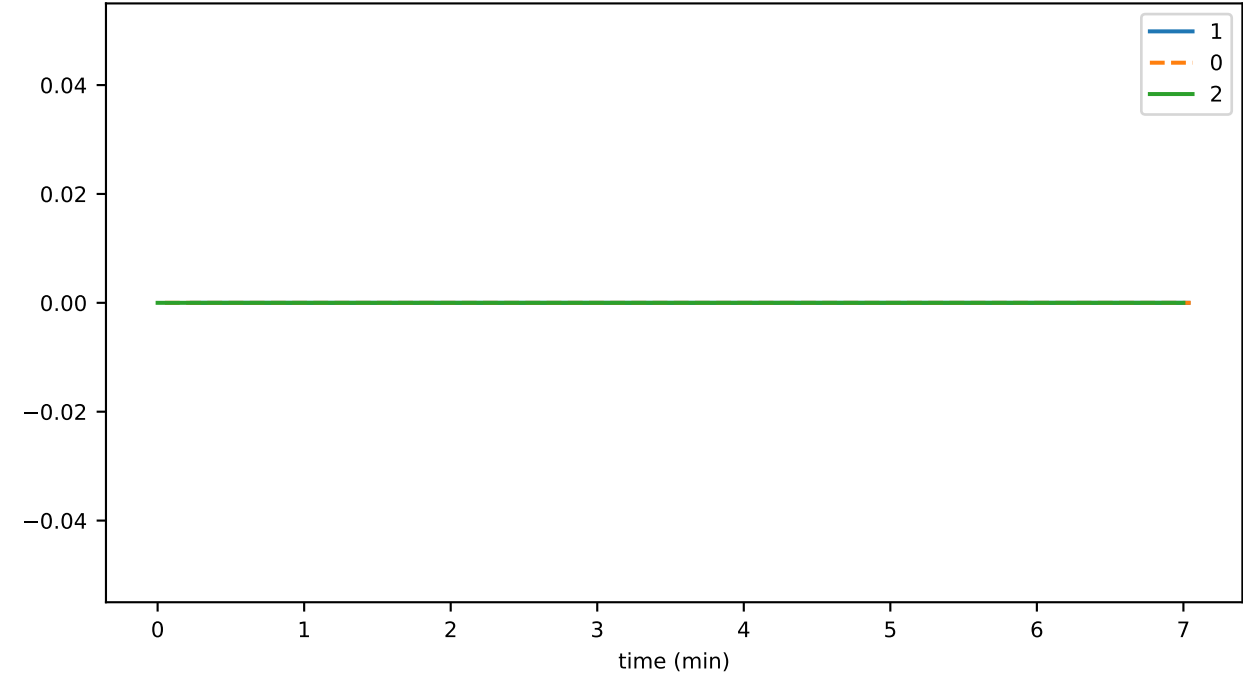
nodeCreateDurationMax
