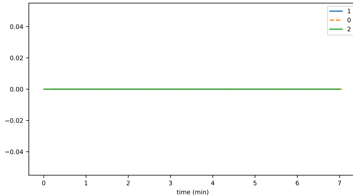
hintsSignaturesProduced
