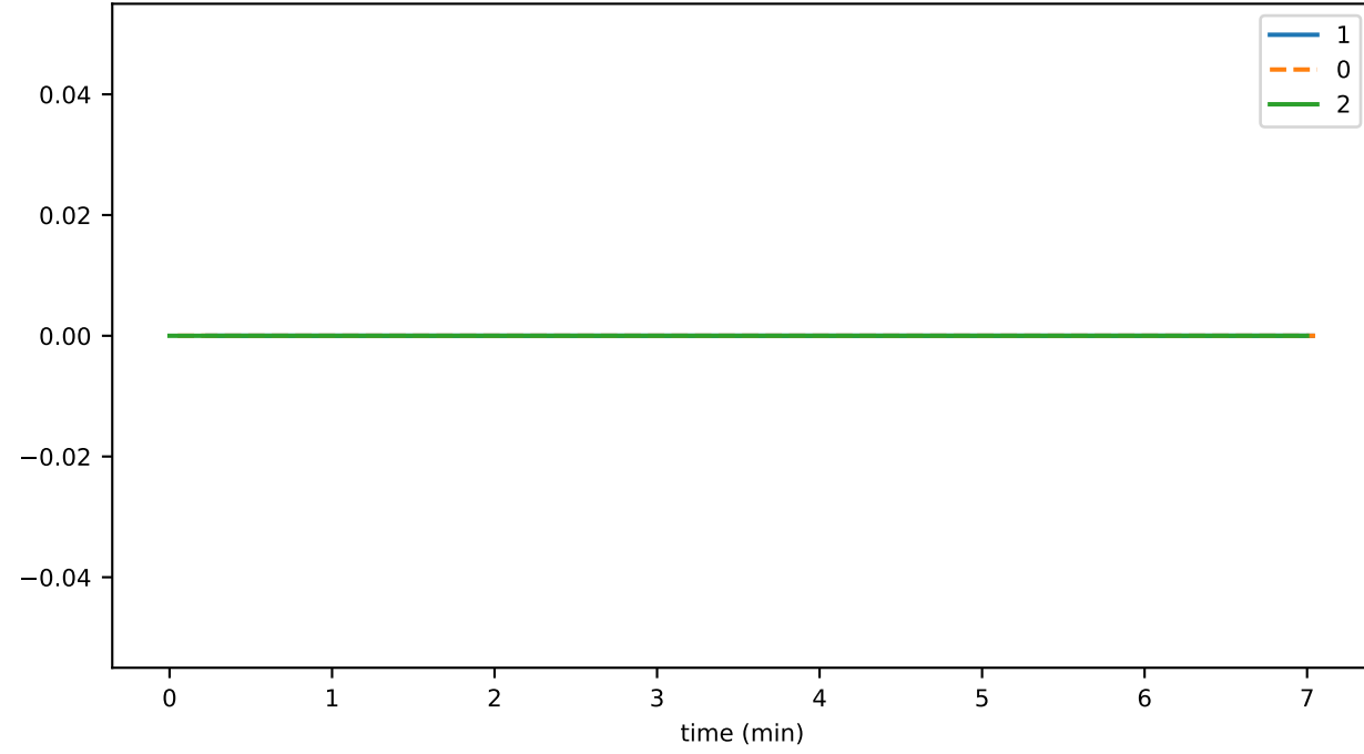
nodeCreateDurationAvg
