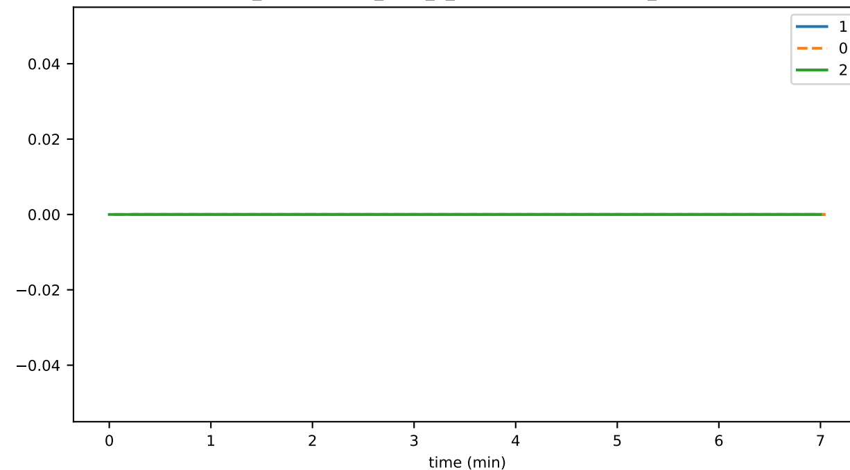
ds_compactions_level_6_leavesSavedSpaceMb_state
