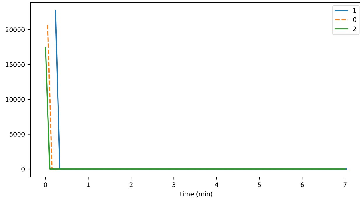
eventDelay_3_deduplication_storageMAX
