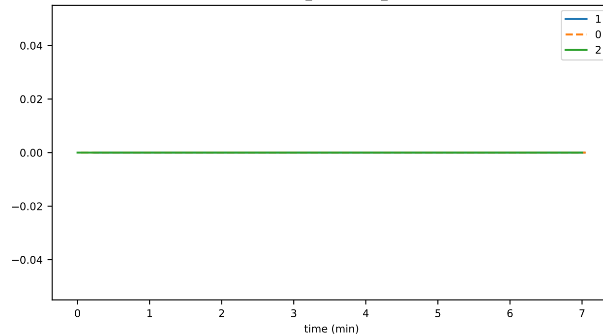
connRecv_endStream_persistenceFailed
