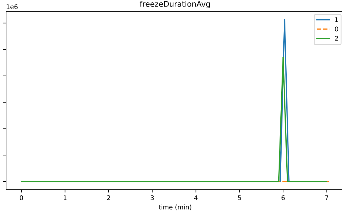
freezeDurationAvg
