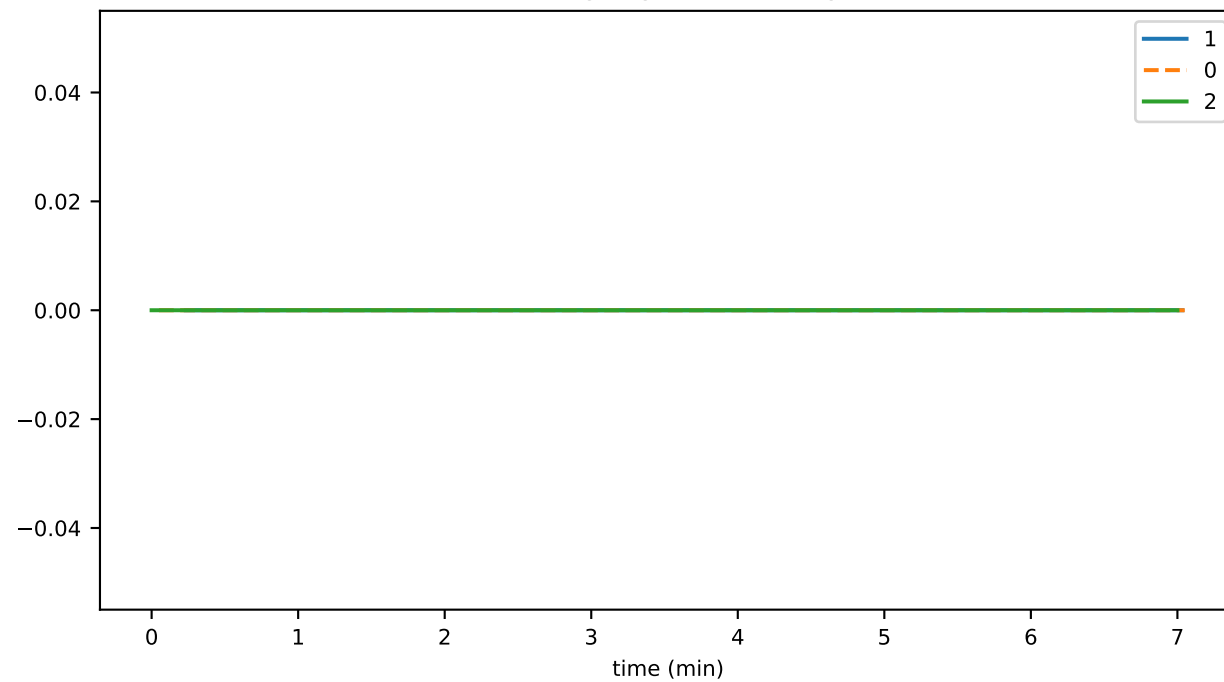
historyAssemblySignatureDurationMax
