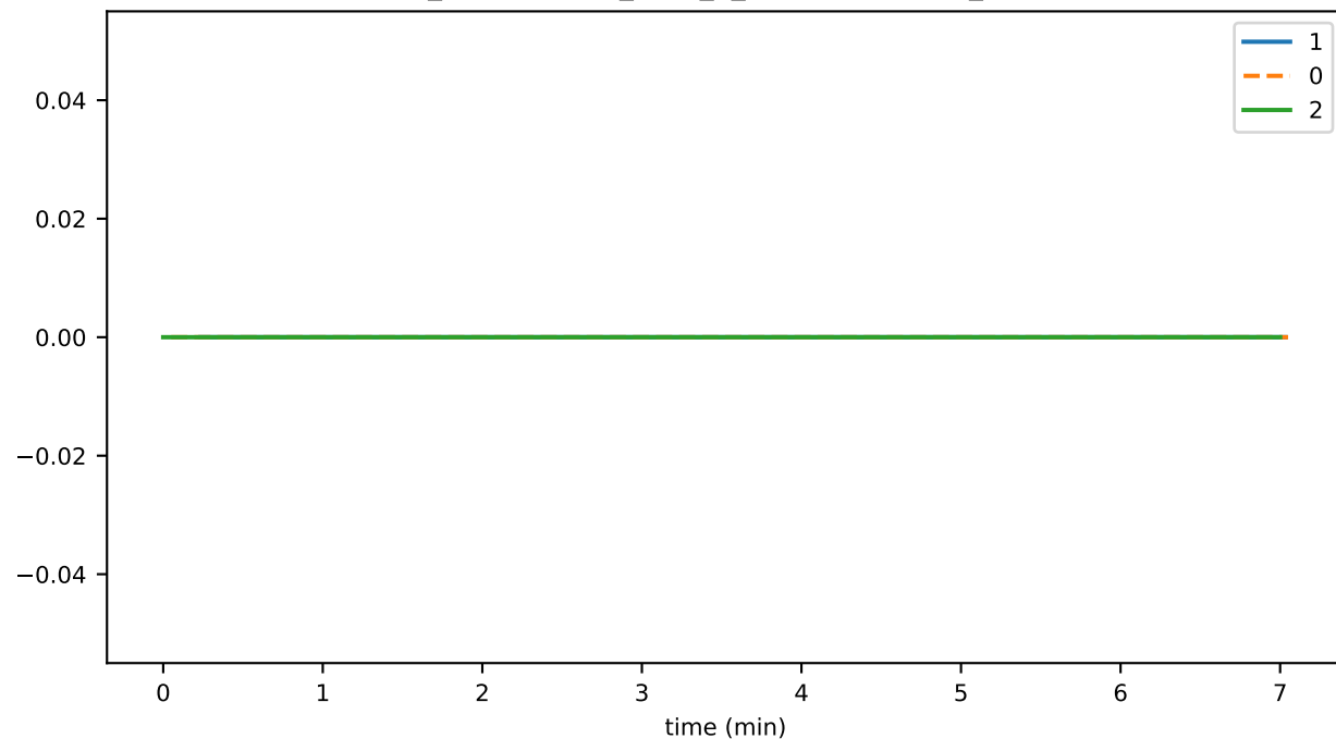
ds_compactions_level_6_leafKeysTimeMs_state
