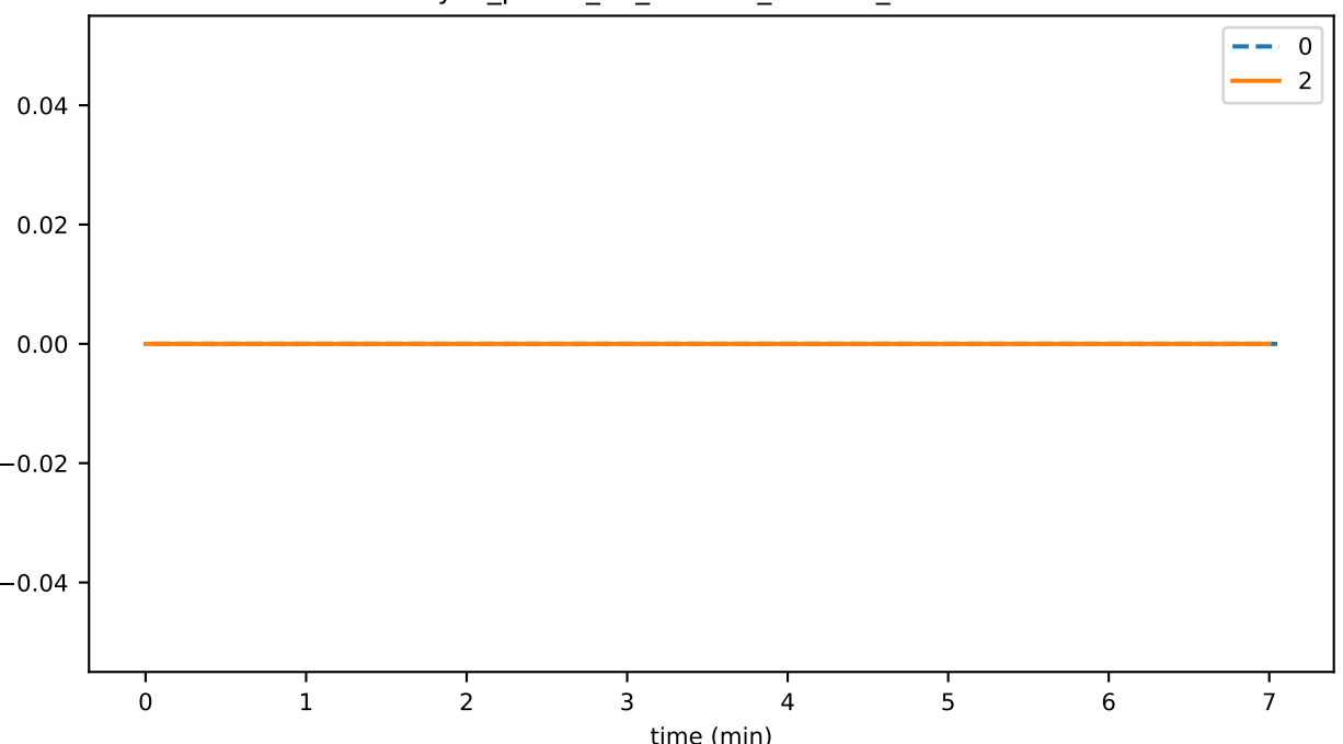
sync_phase_01_fraction_GOSSIP_HALTED
