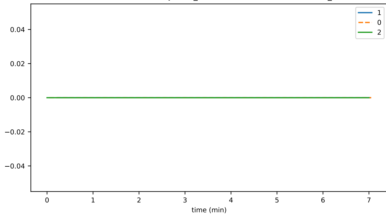
SmartContractService:Rejected_contractCallTxDueToIntrinsicGas_total
