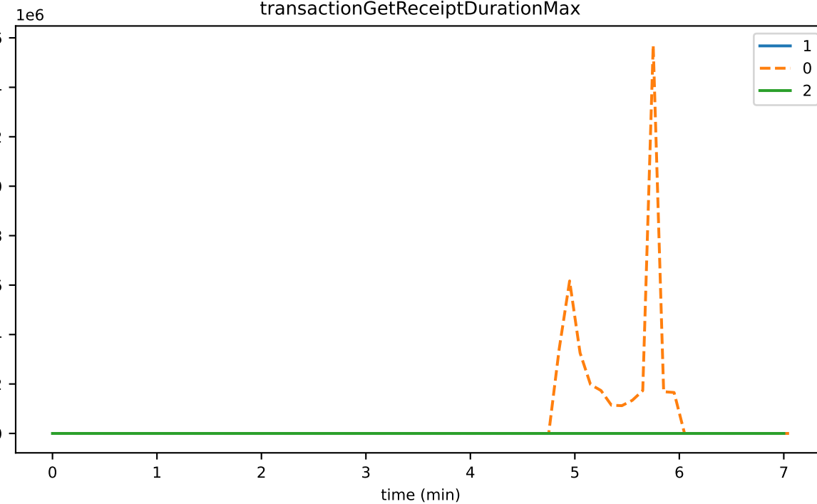
transactionGetReceiptDurationMax
