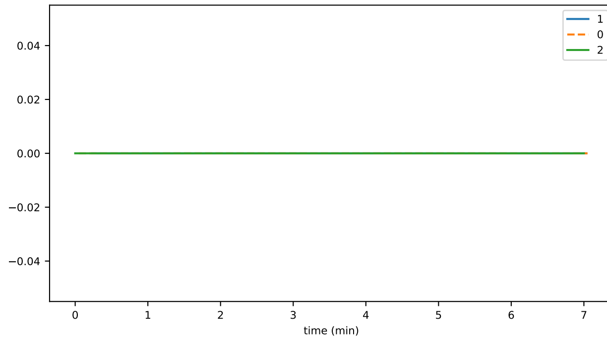
ethereumTransactionDurationMax
