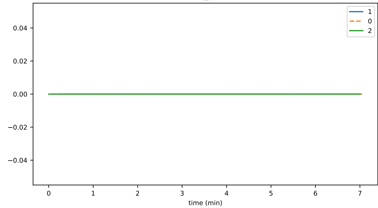
connRecv_unknown
