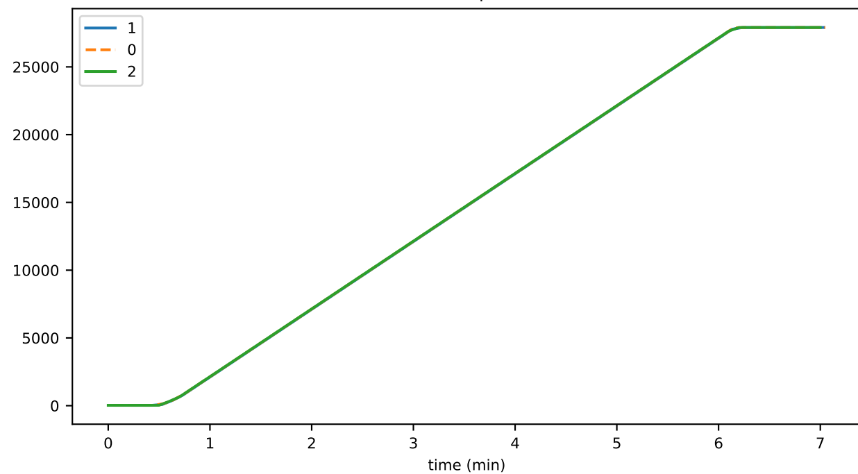
roundIncEqParents
