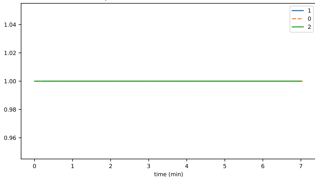
preconsensusEventFileRate
