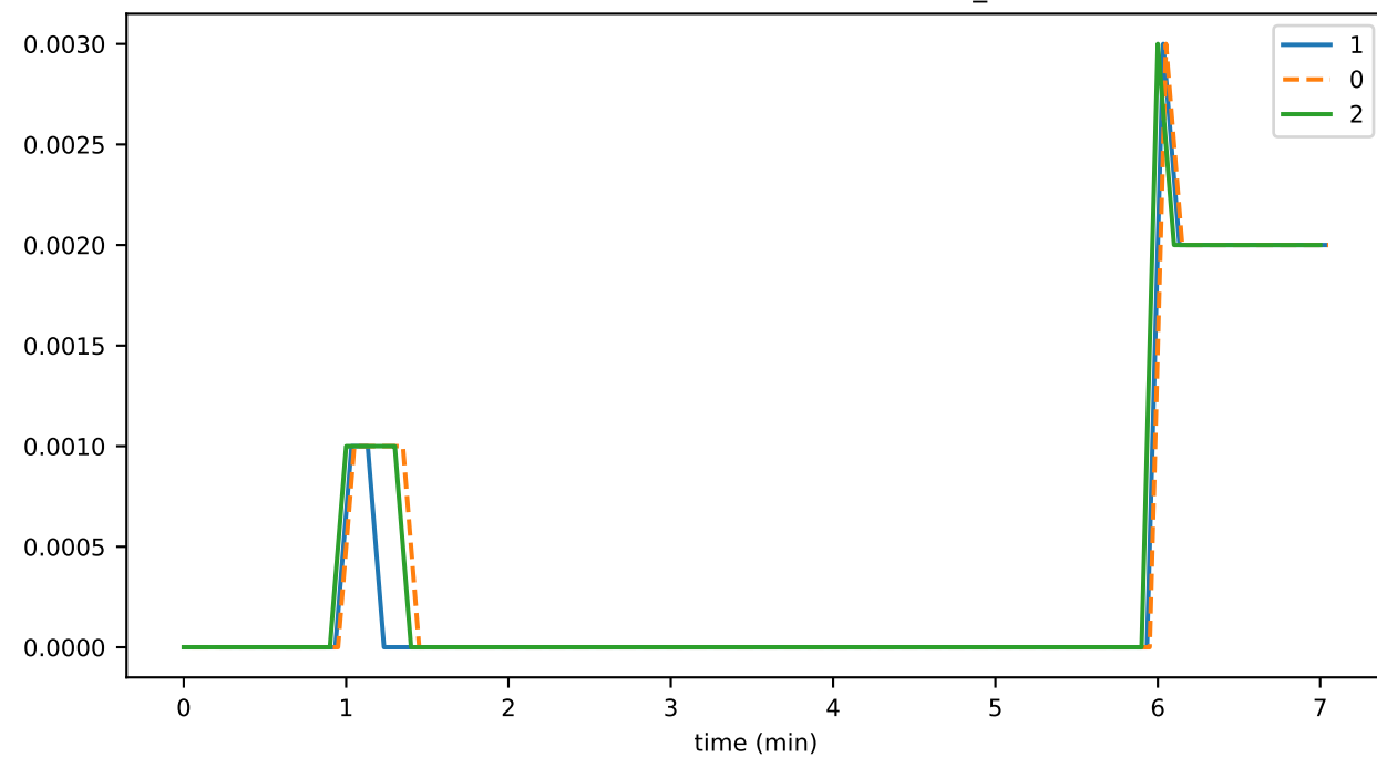
roundsSinceLastConsensusEvent_2
