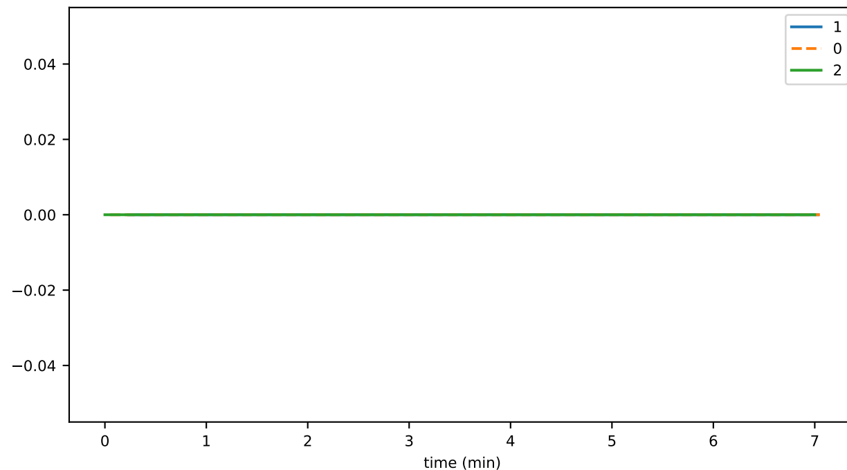
contractsMaxNumber
