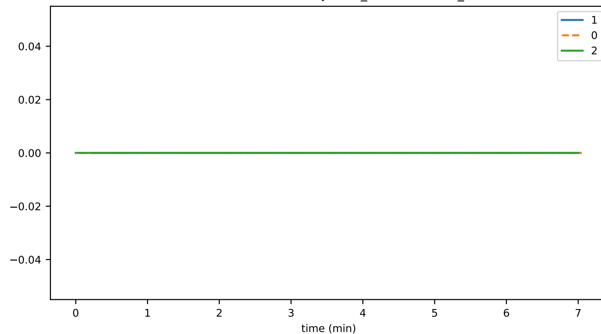
SmartContractService:Rejected_contractCreateTx_total
