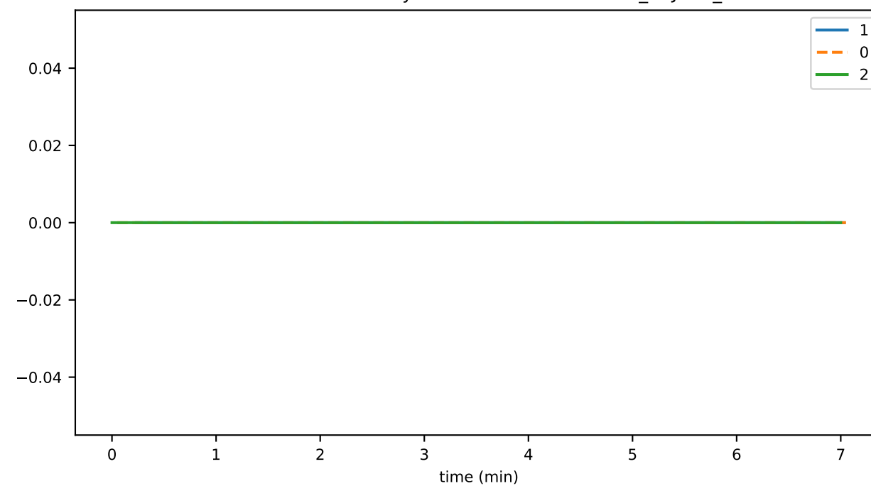
SmartContractService:SystemContractMethodCall_REJECT_failed
