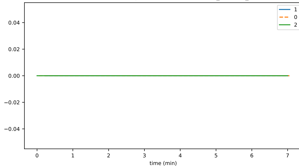
SmartContractService:SystemContractMethodCall_ALLOWANCE_failed
