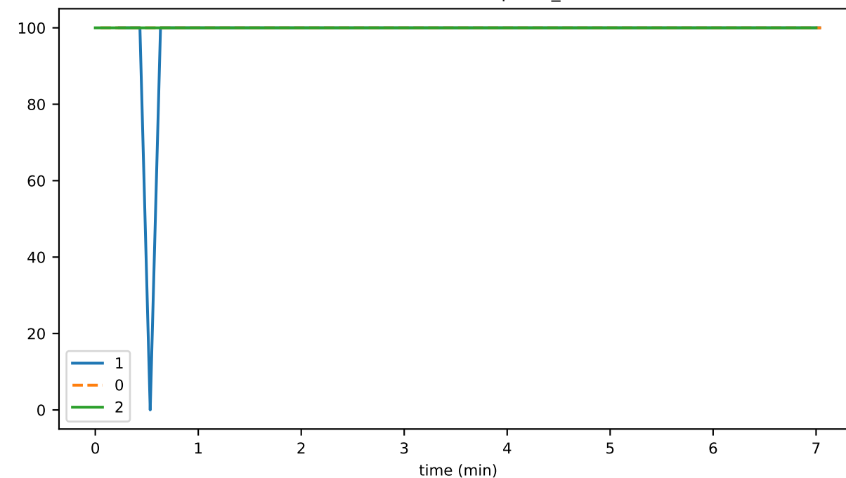
nodeActivePercentSnapshot_node0
