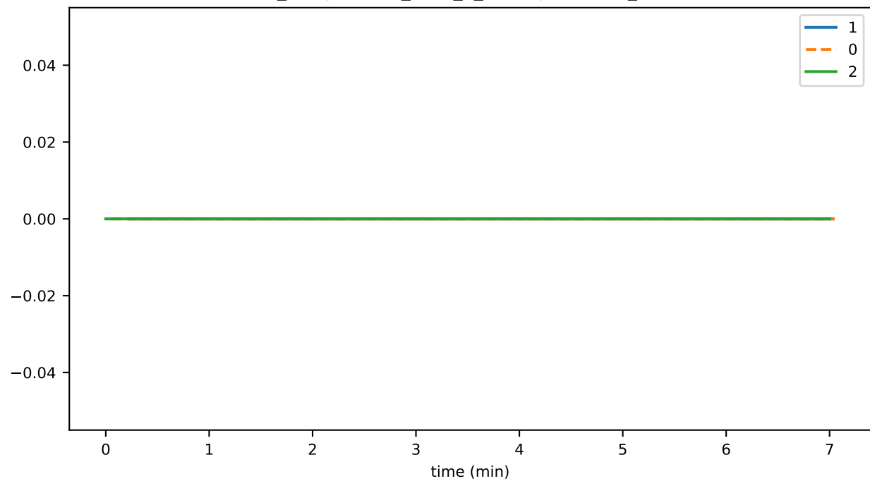
ds_compactions_level_9_leavesTimeMs_state
