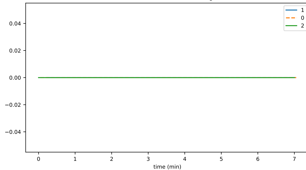
scheduleGetInfoDurationAvg
