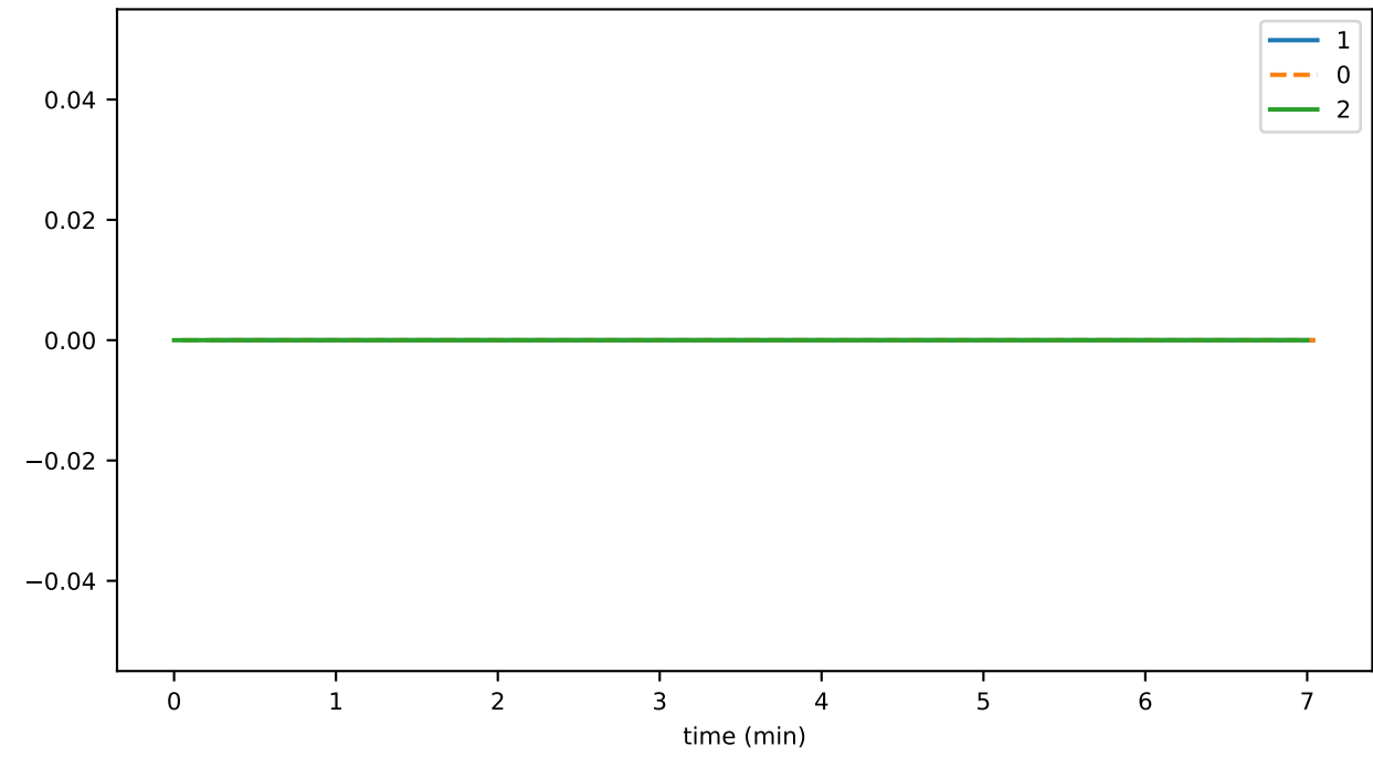
futureEventBuffer_eventCreator_count
