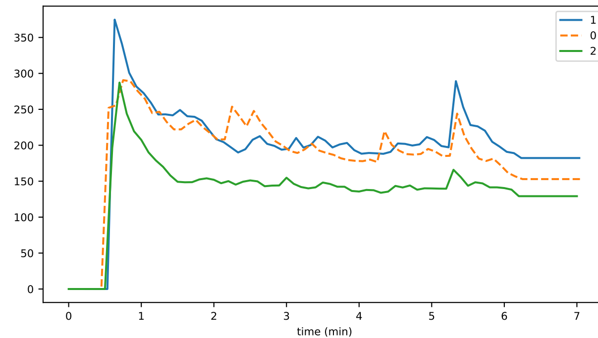
timeToDeleteState
