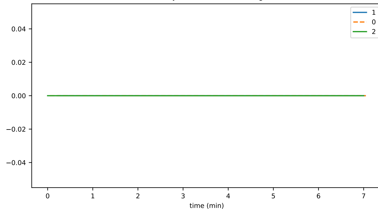
historyProofVoteDurationAvg
