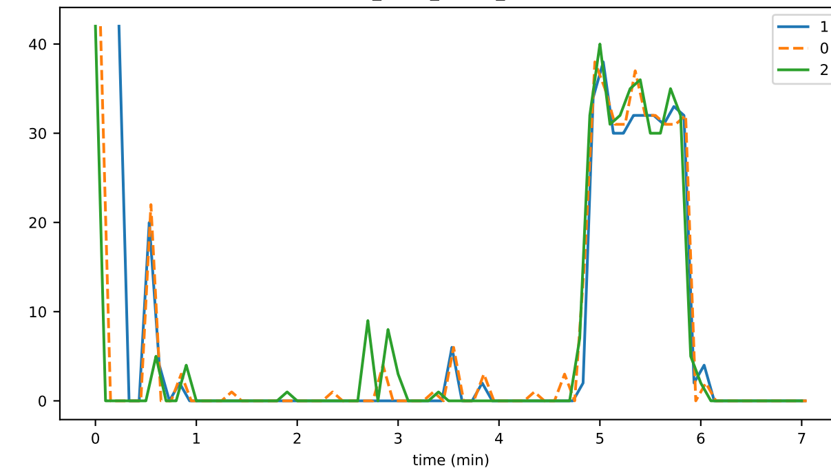
dupEvPercent
