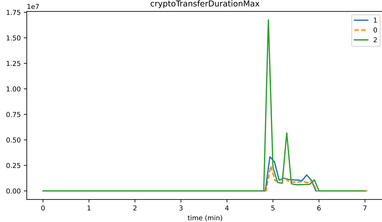
cryptoTransferDurationMax
