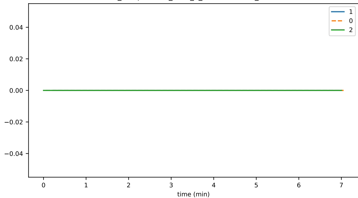
ds_compactions_level_9_leavesTimeMs_state
