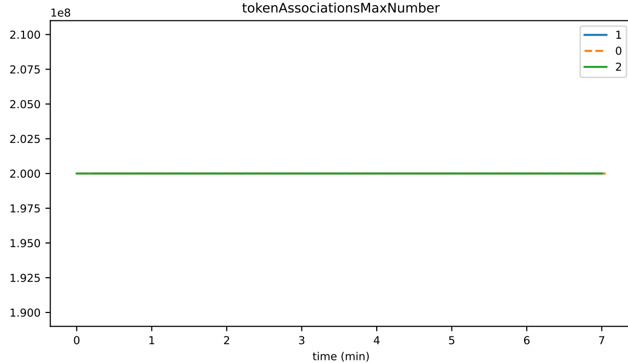
tokenAssociationsMaxNumber
