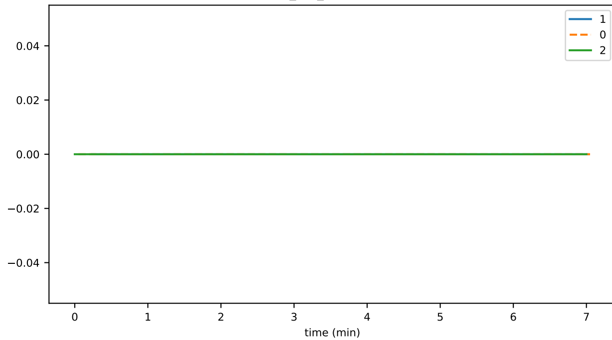
ev_per_syncRMAX
