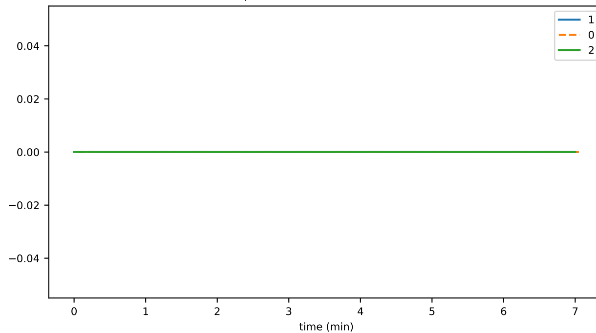
hapiCreationLimitsPercentUsed
