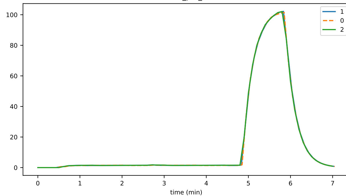
transH_per_sec
