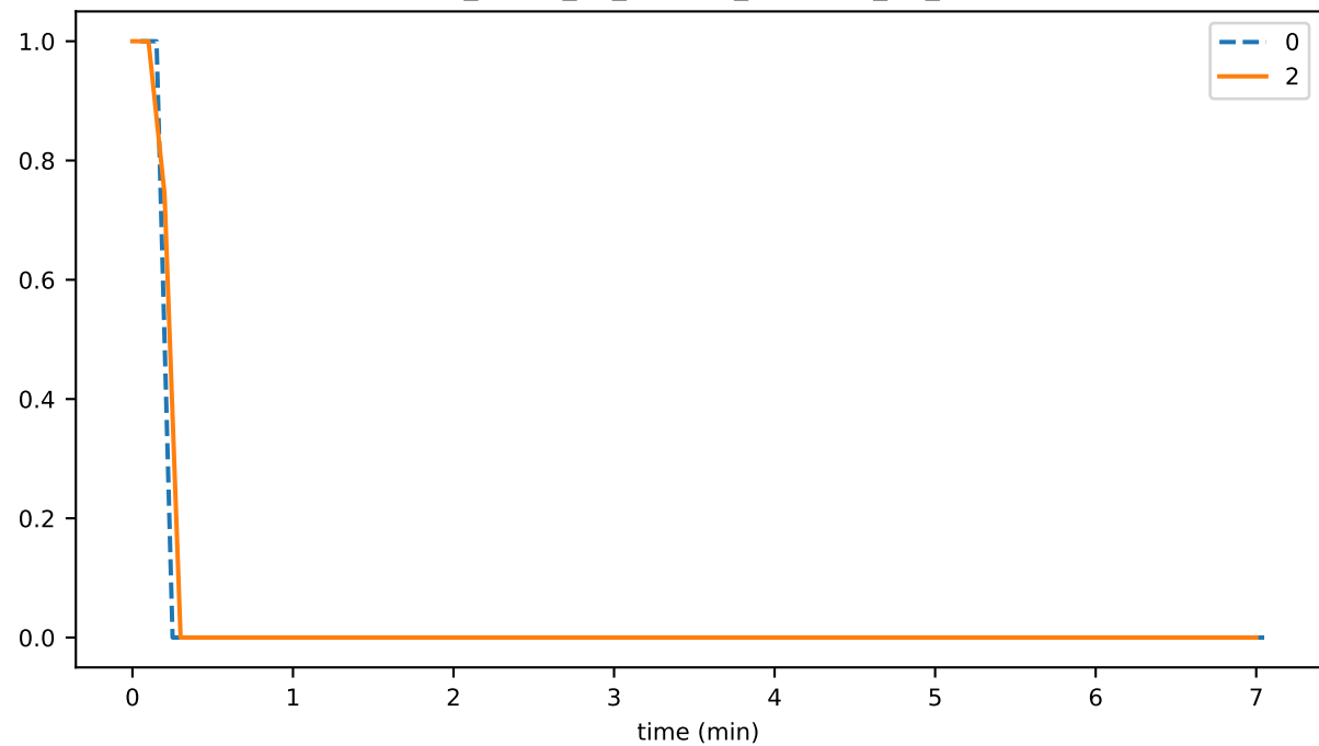
sync_phase_01_fraction_OUTSIDE_OF_RPC
