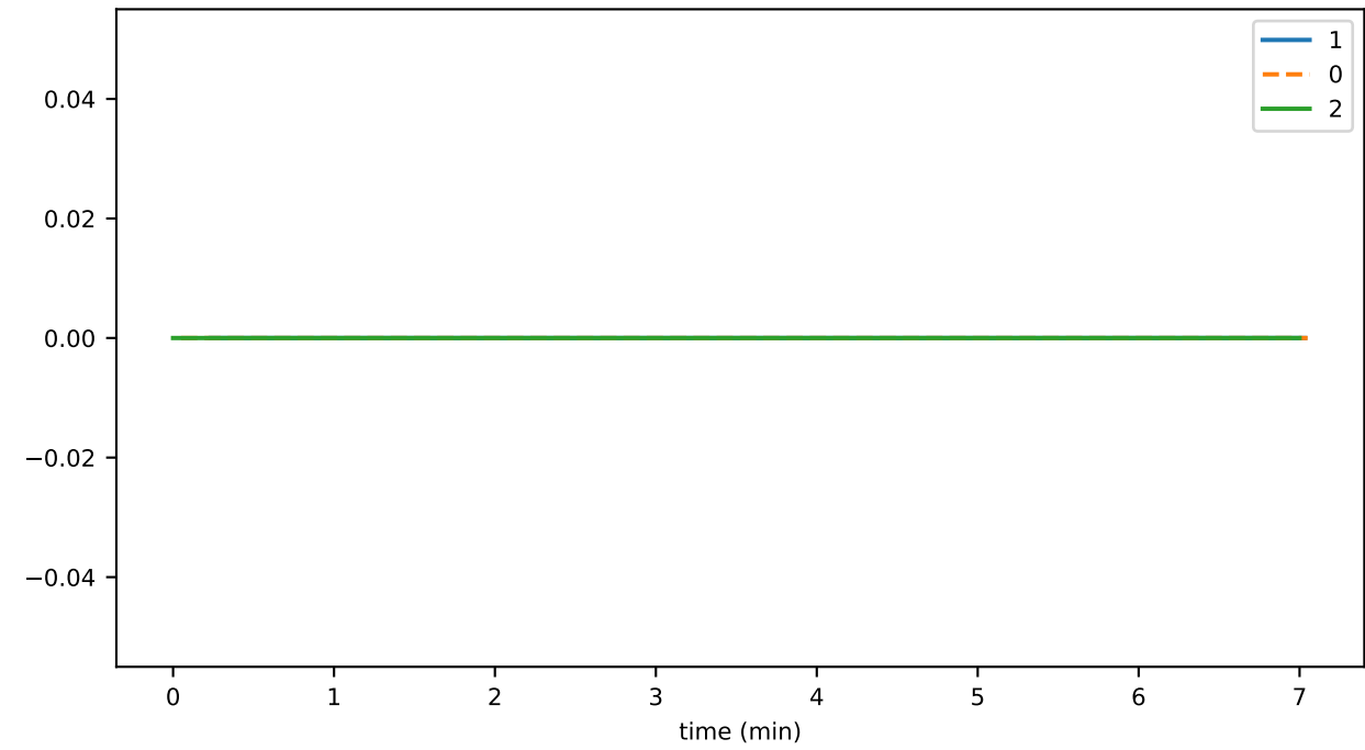
cryptoGetLiveHashDurationAvg
