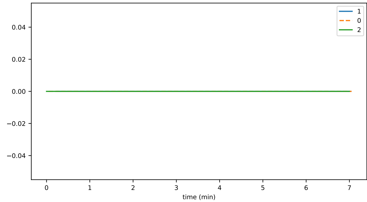
fileDeleteDurationAvg
