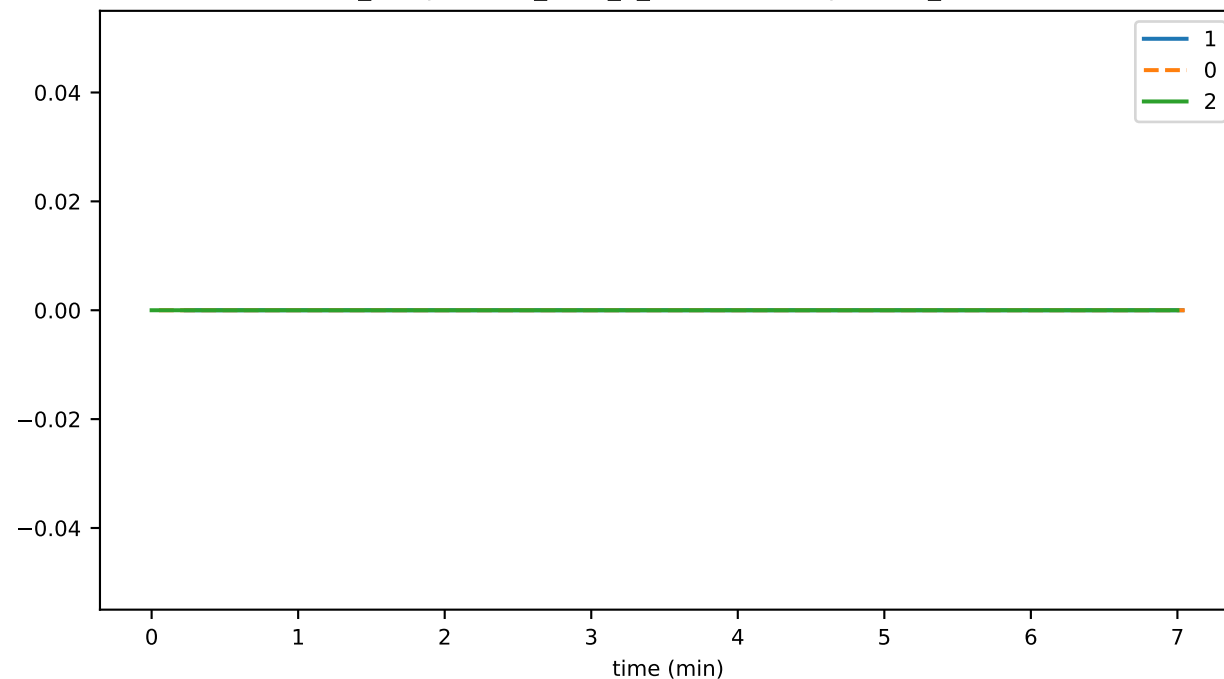
ds_files_hashesStoreFileCount_state
