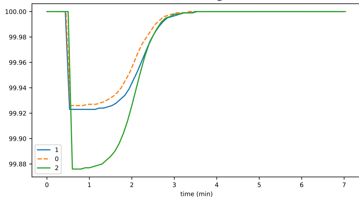
nodeActivePercent_node2
