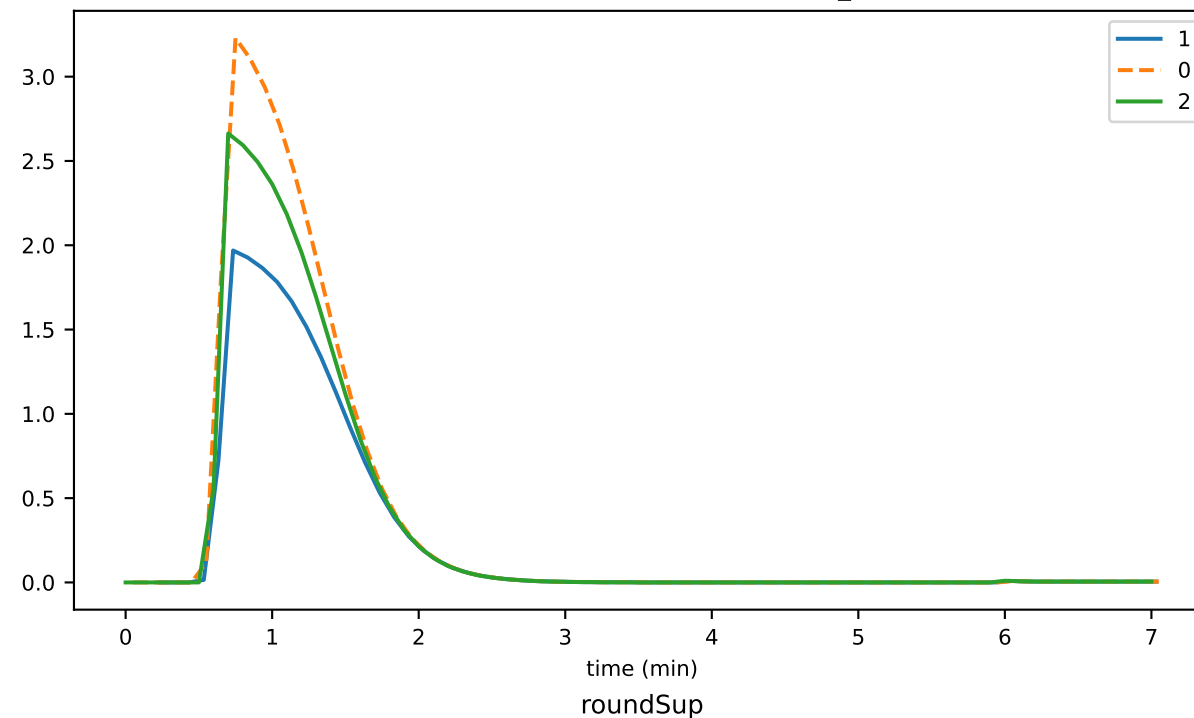
roundsSinceLastConsensusEvent_1
