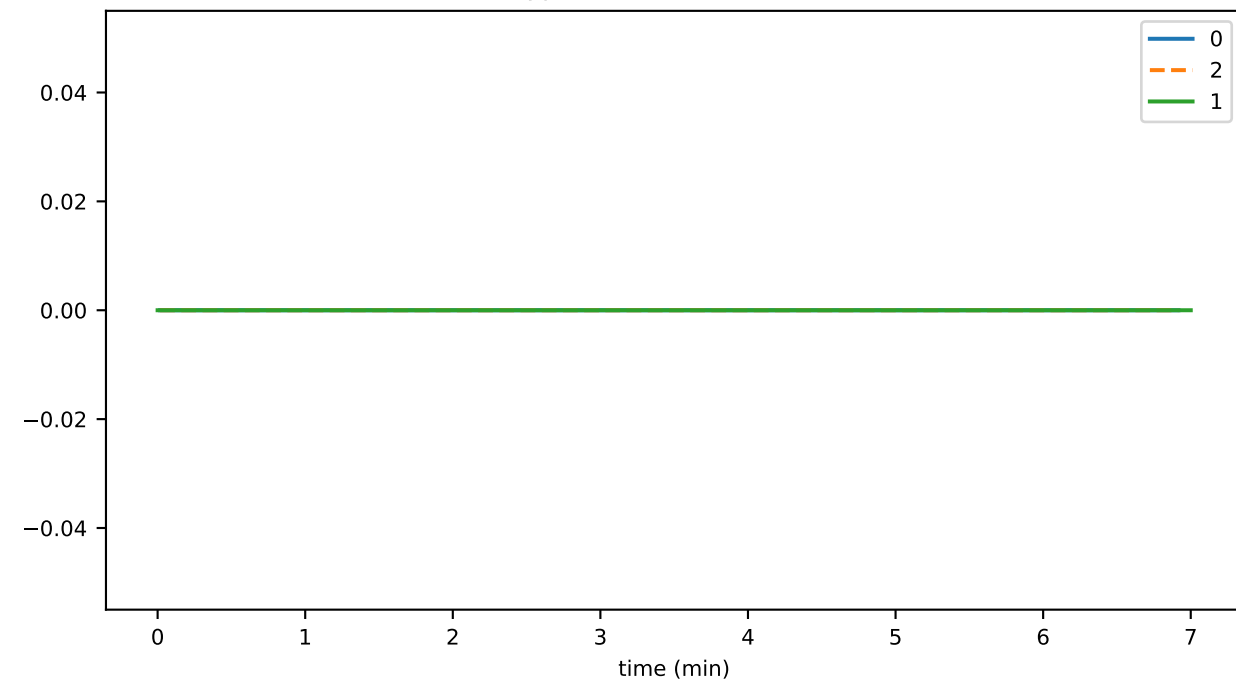
cryptoGetAccountBalanceDurationMax
