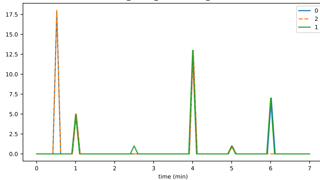
ds_flushes_leavesDeleted_state
