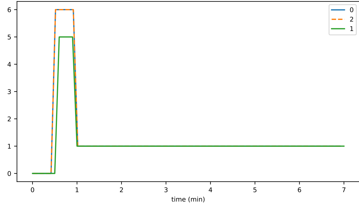
ds_files_leafKeysStoreFileSizeMb_state
