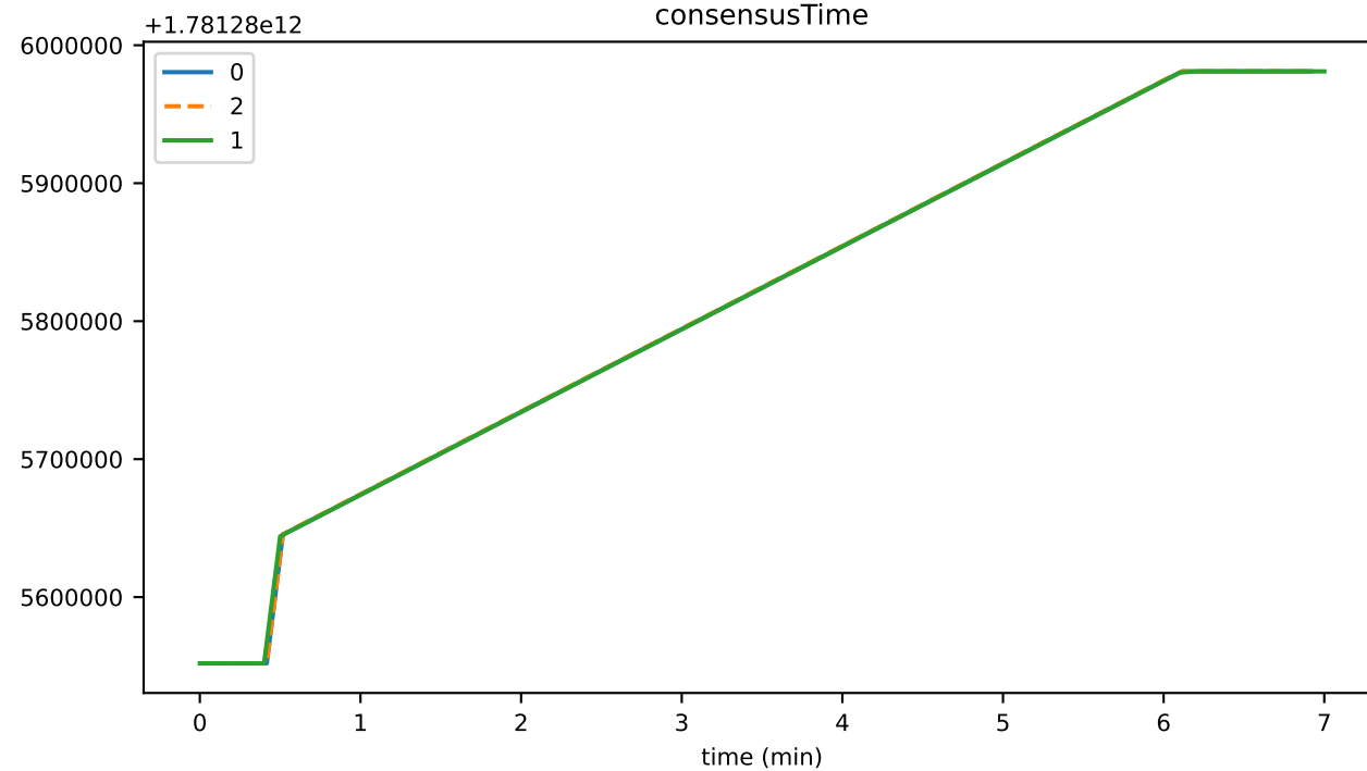
consensusTime
