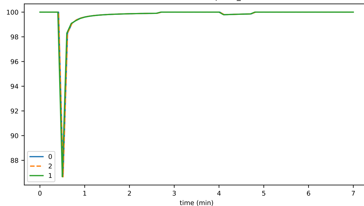
nodeCreateDurationMax
