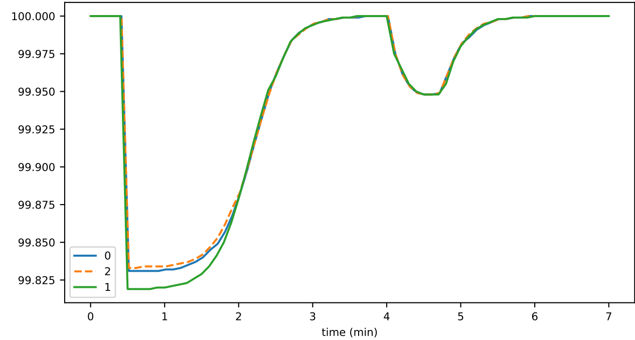
nodeActivePercentSnapshot_node0
