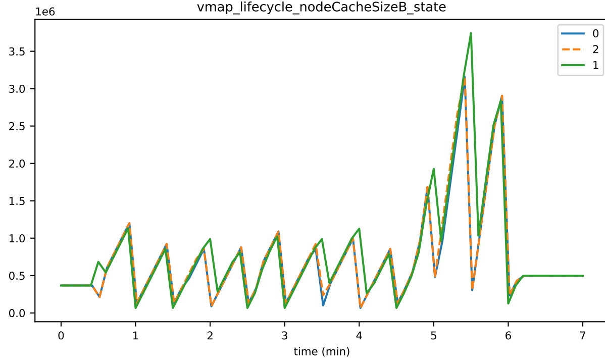
vmap_lifecycle_nodeCacheSizeB_state
