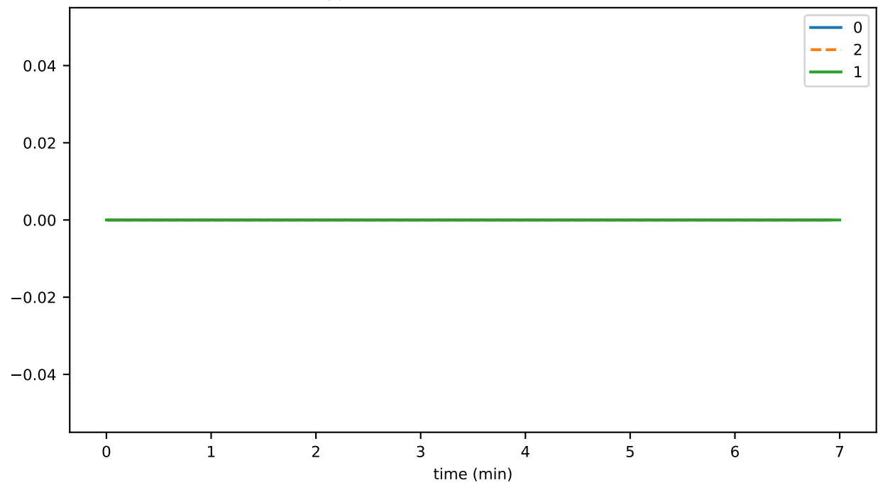
cryptoGetAccountBalanceDurationAvg
