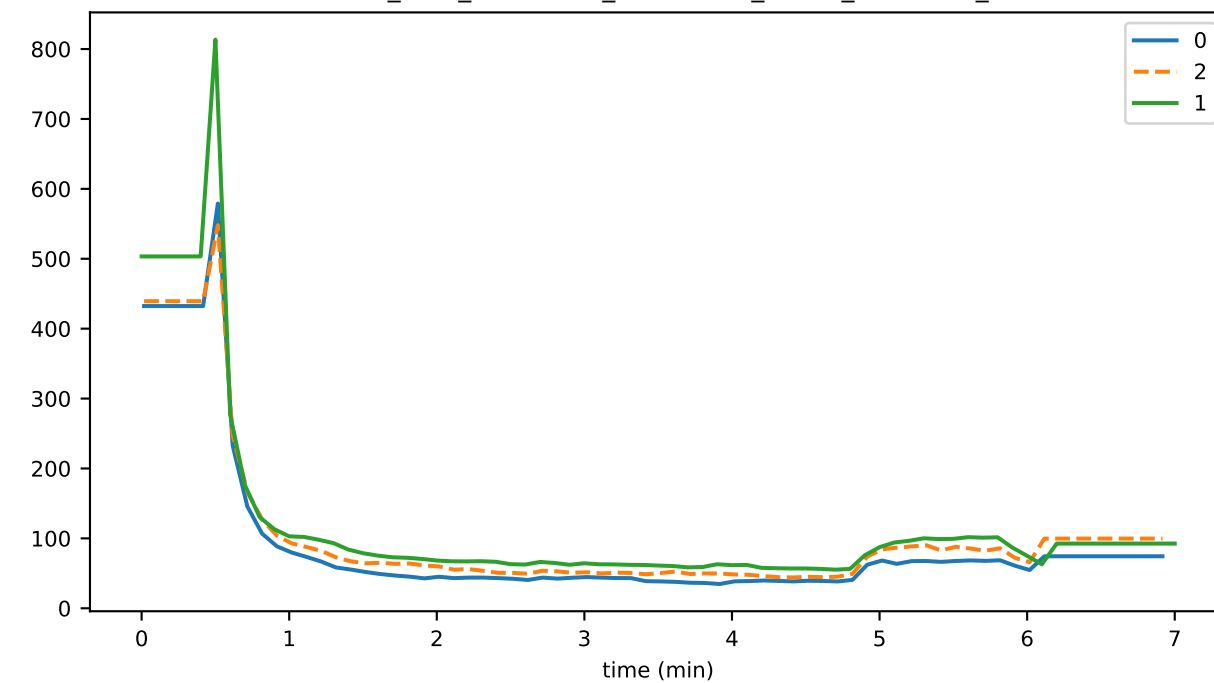
consensus_time_UPDATING_PLATFORM_STATE_RUNNING_HASH
