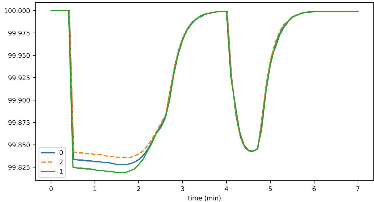
nodeActivePercent_node2
