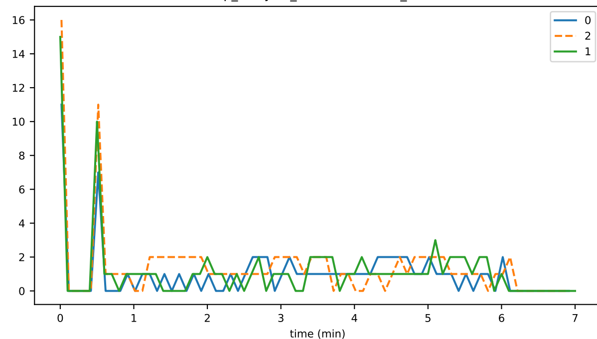
vmap_lifecycle_nodeCacheSizeB_state
