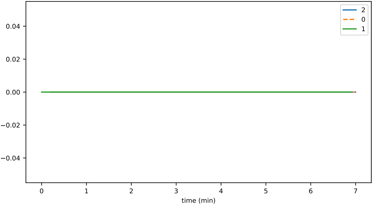
SmartContractService:SuccessfulTransactionDuration_sum
