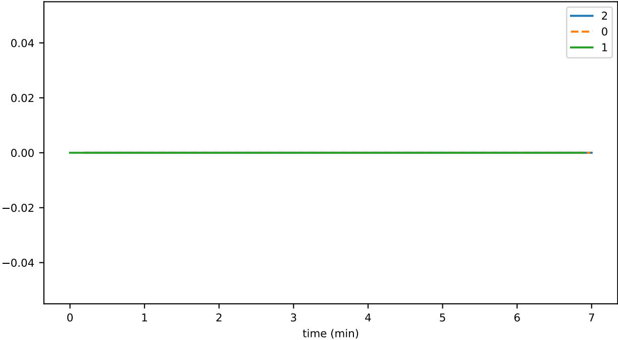
SmartContractService:SystemContractMethodCall_AIRDROP_failed
