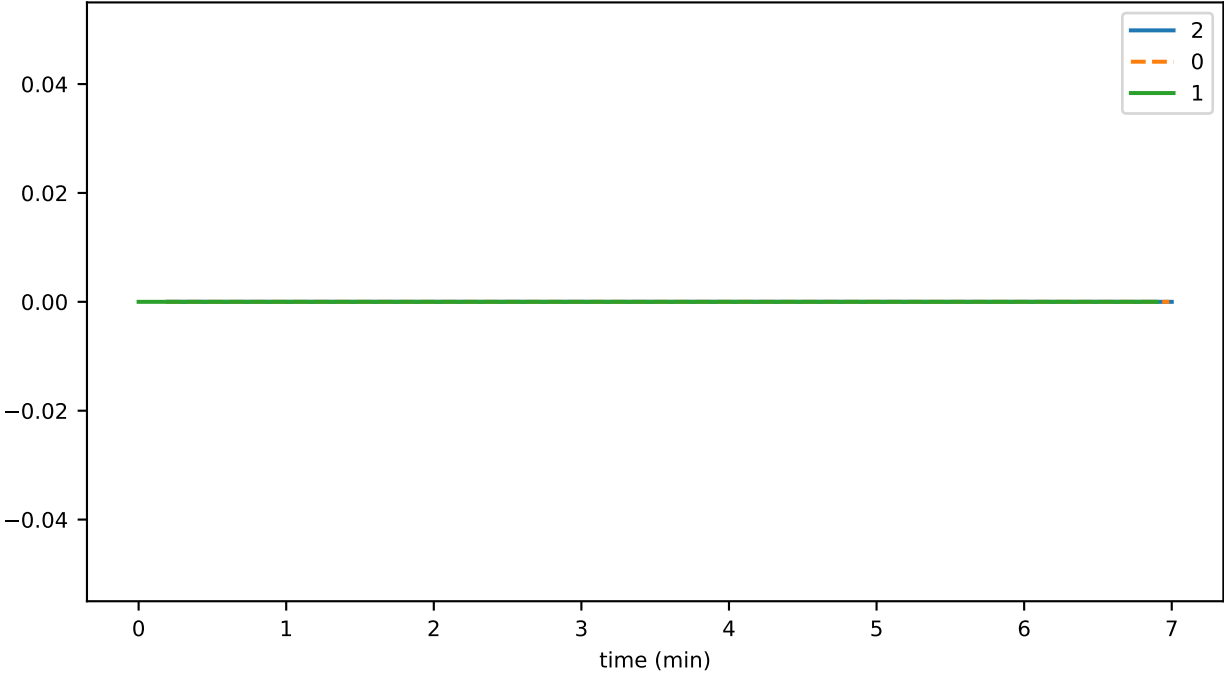
SmartContractService:SystemContractMethodCall_REJECT_failed
