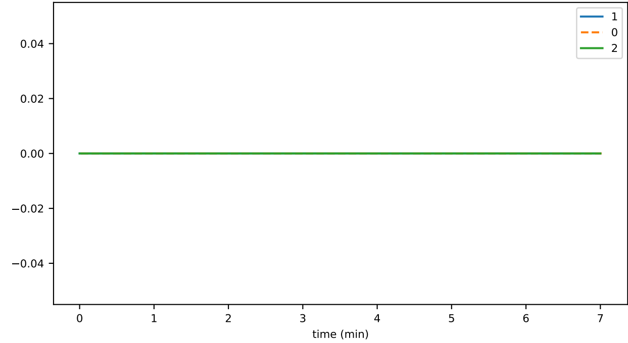
stateSignatureTransactionThrottledTxns
