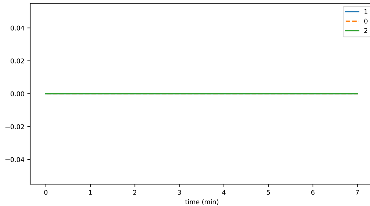
atomicBatchDurationAvg
