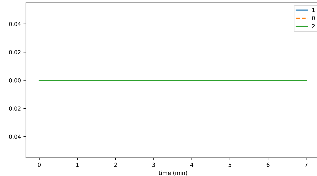
connRecv_latestBlockSkipBlock
