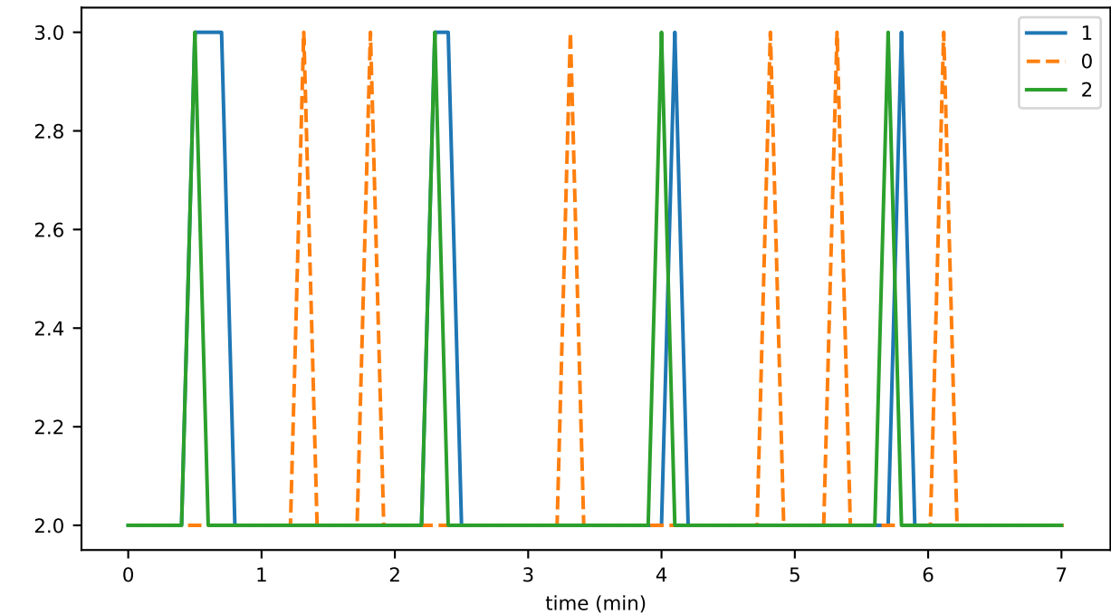
vmap_lifecycle_pipelineSize_state
