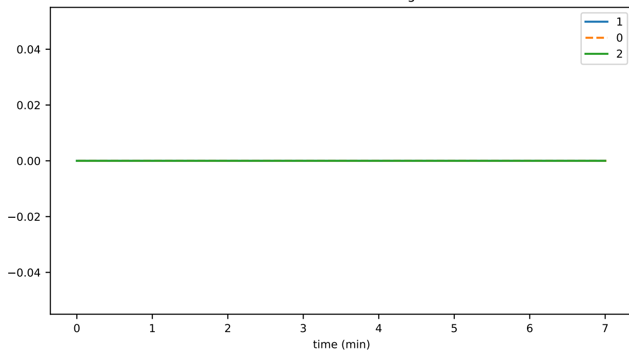
hookStoreDurationAvg
