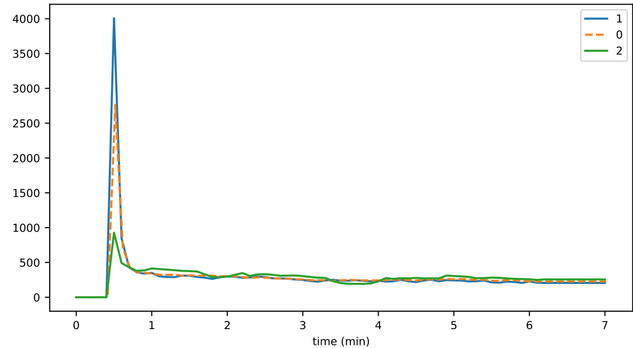
eventDelay_6_pces_gossip
