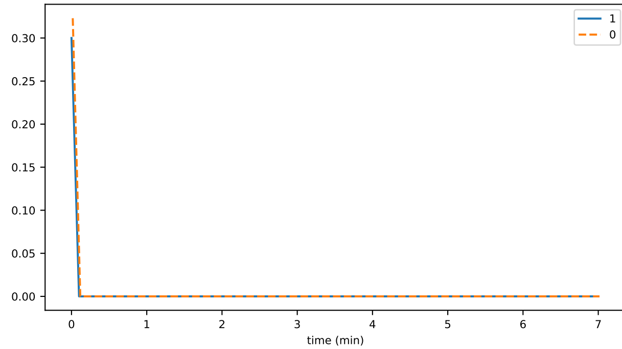
sync_phase_02_fraction_OUTSIDE_OF_RPC
