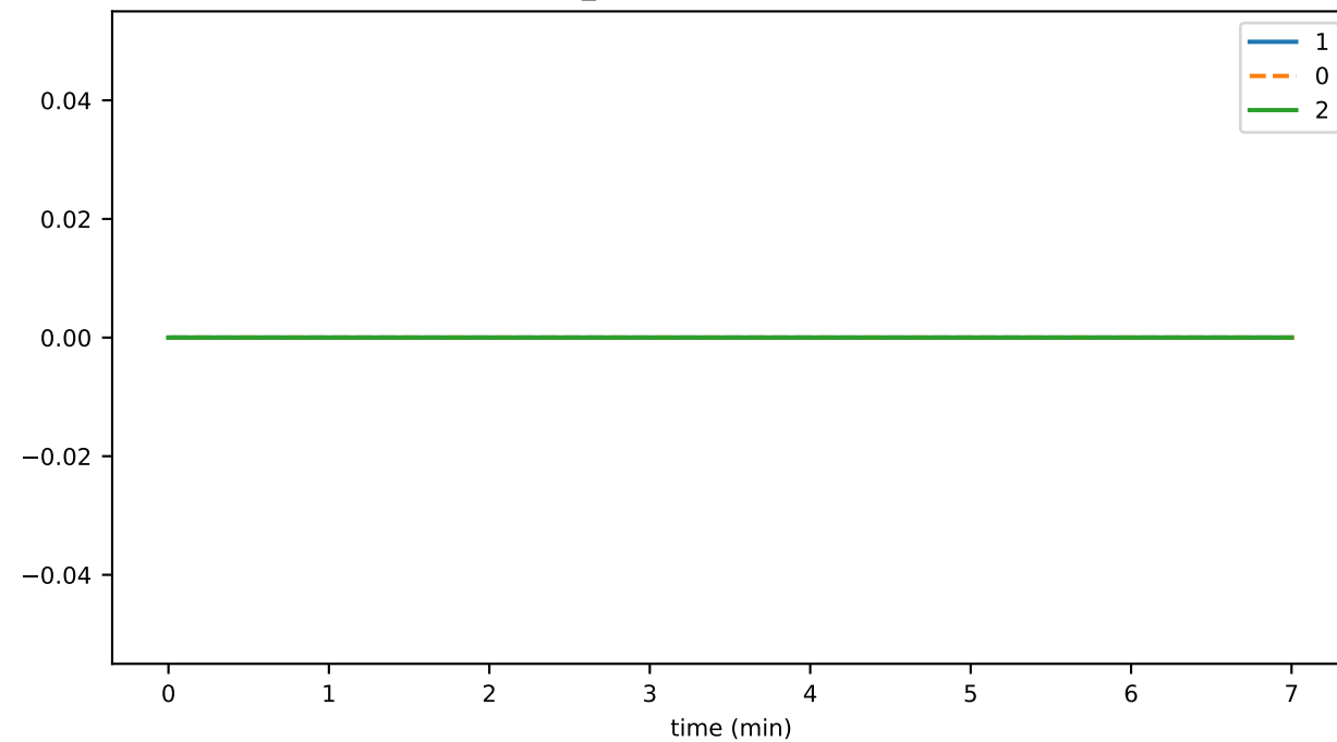
conn_headerSentToAckLatency
