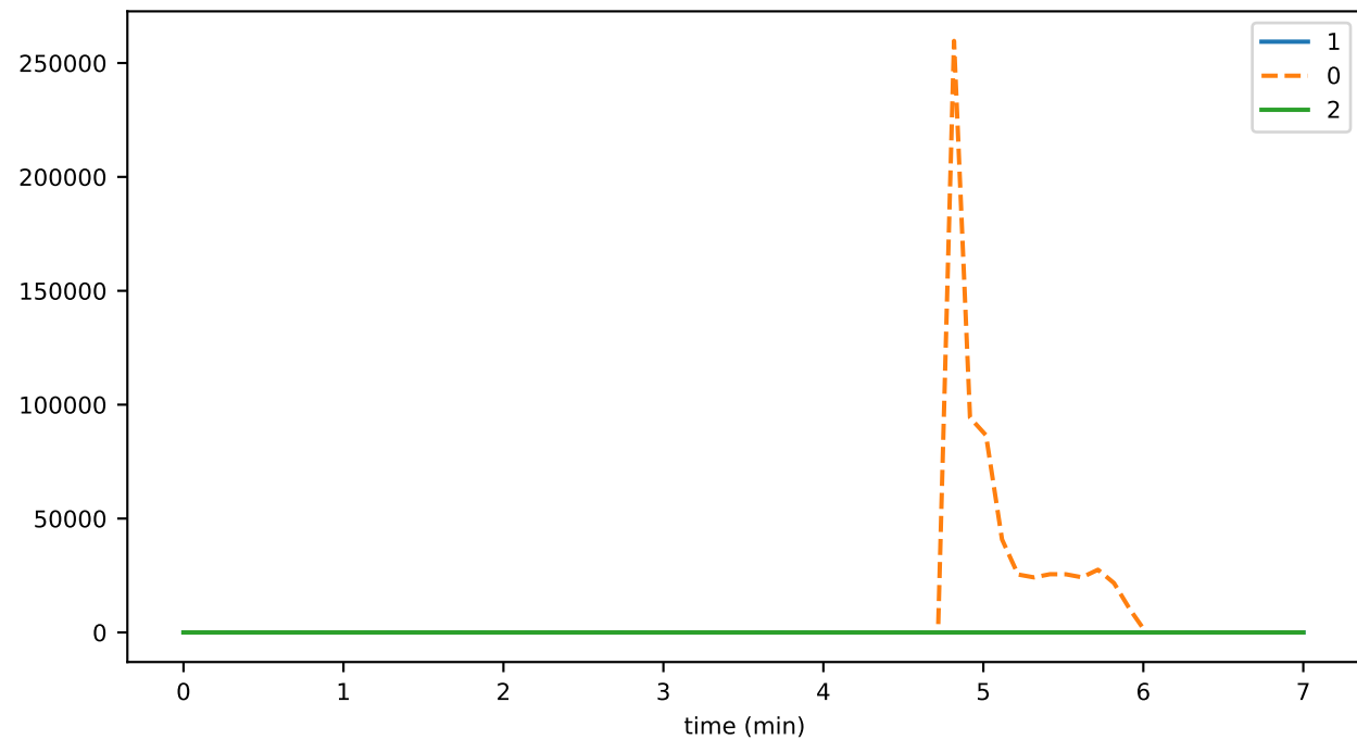
transactionGetReceiptDurationAvg
