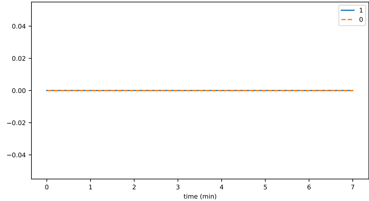
sync_phase_02_fraction_PLATFORM_STATUS_PREVENTING_SYNC
