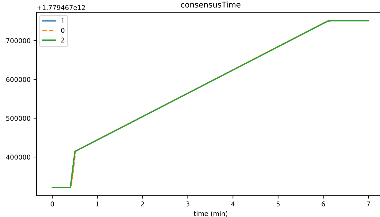
consensusTime
