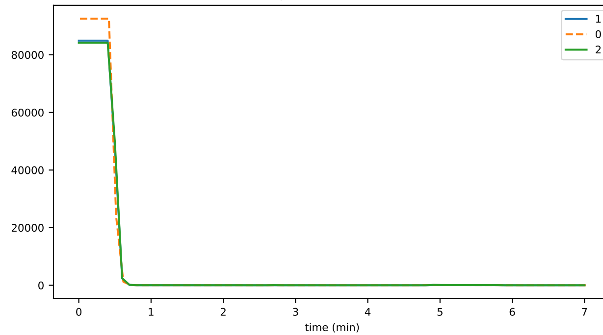
queriedAccountBalances
