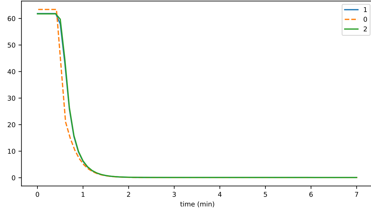
secGossipRoundtrip
