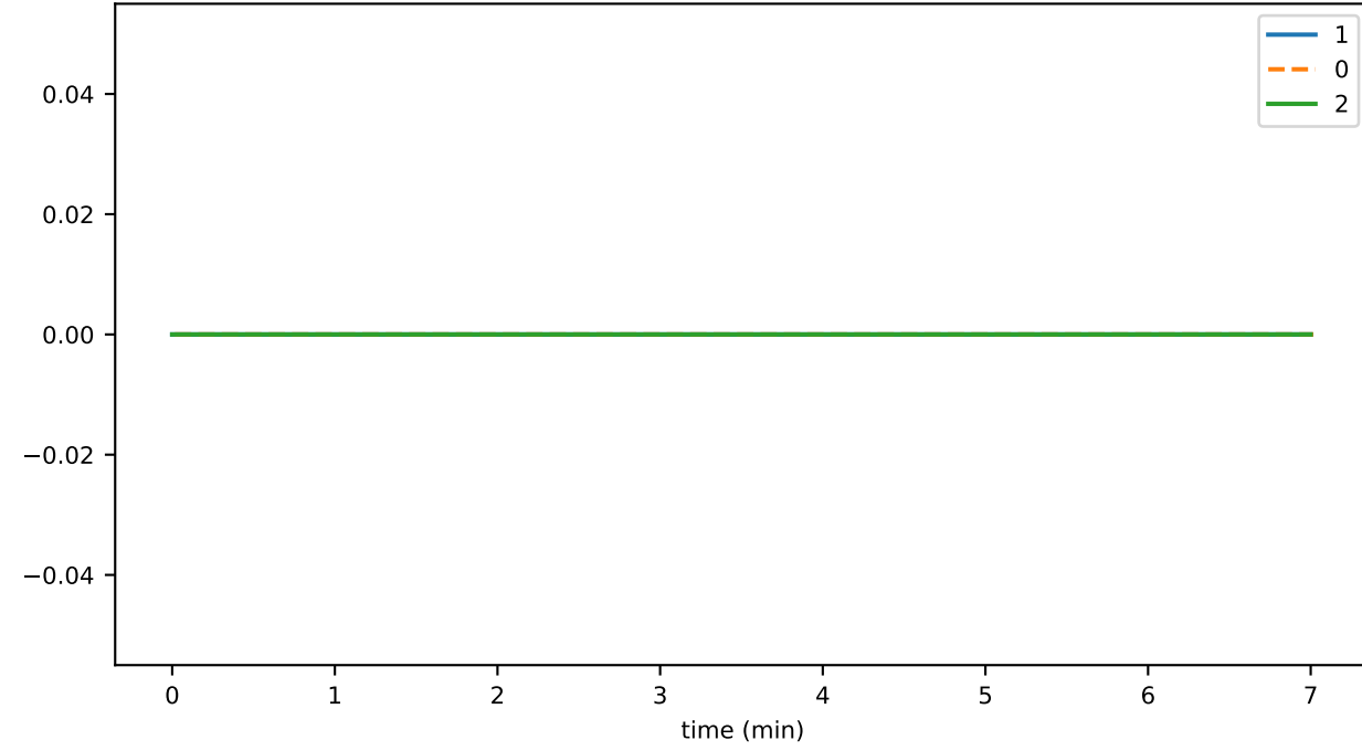
consensusCreateTopicDurationMax
