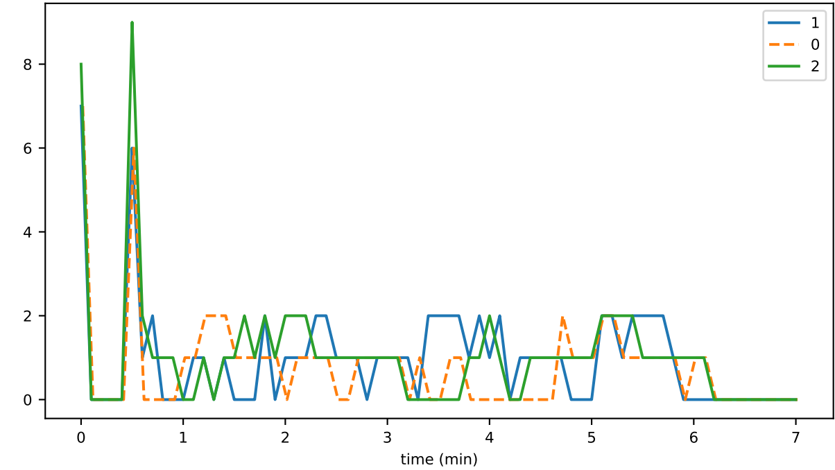
vmap_lifecycle_nodeCacheSizeB_state
