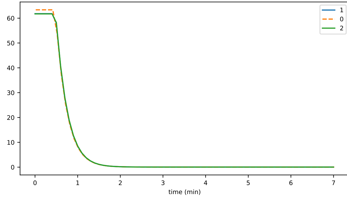
secGossipRoundtrip
