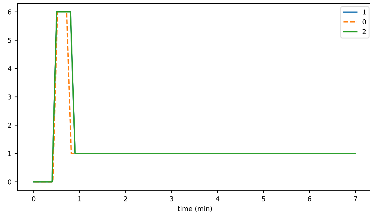
ds_files_leafKeysStoreFileSizeMb_state
