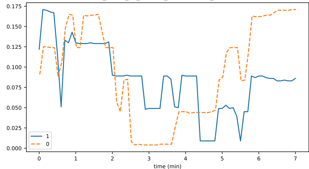
sync_phase_02_fraction_IDLE
