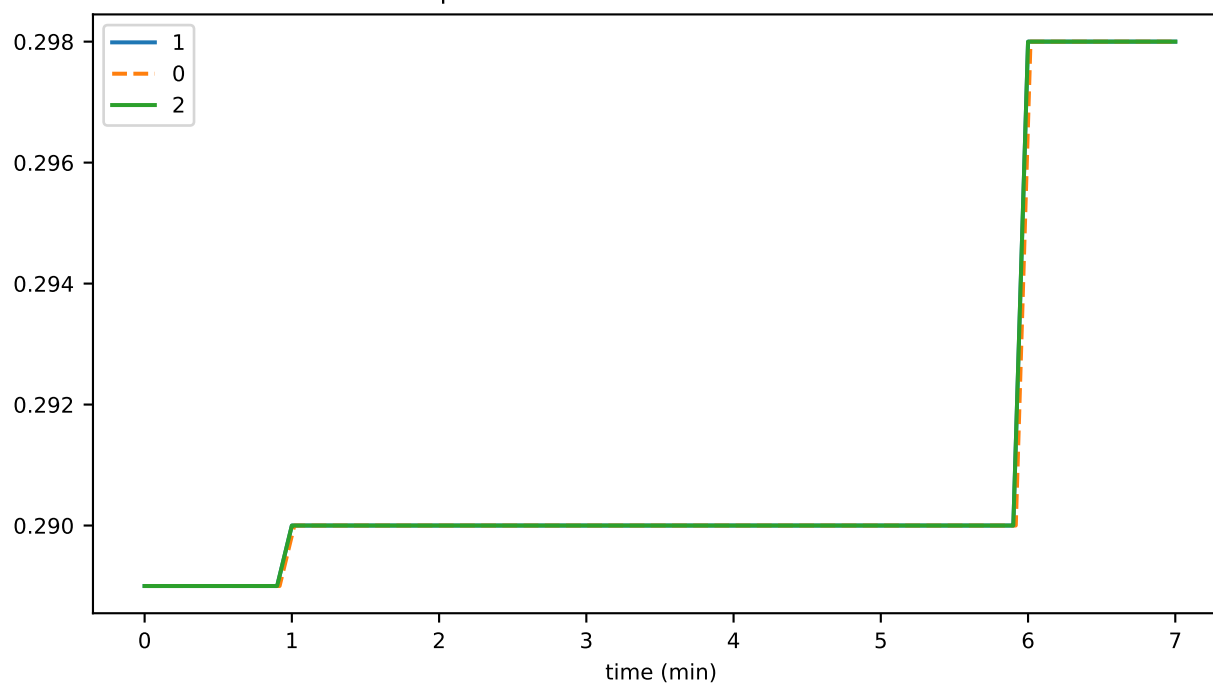
preconsensusEventFileTotalSizeGB
