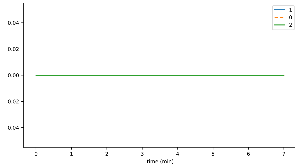
crsPublicationDurationAvg
