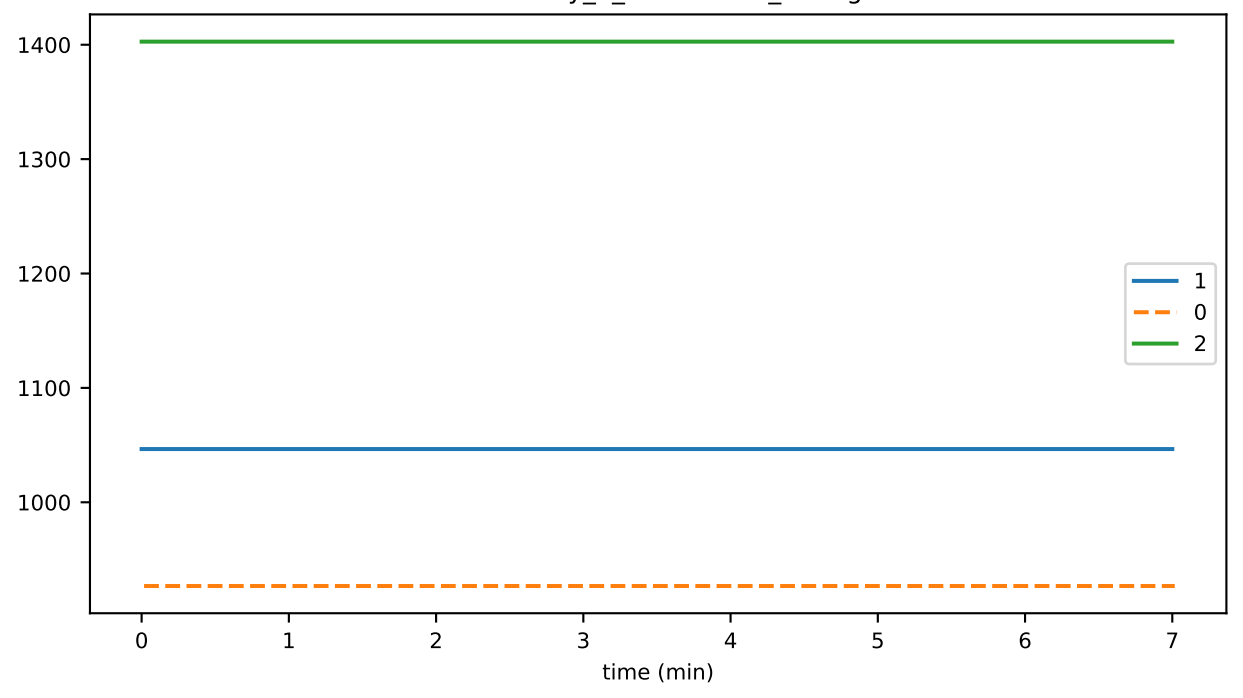
eventDelay_4_verification_storage
