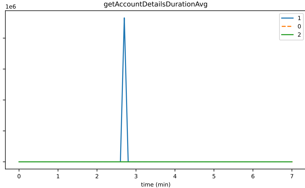
getAccountDetailsDurationAvg
