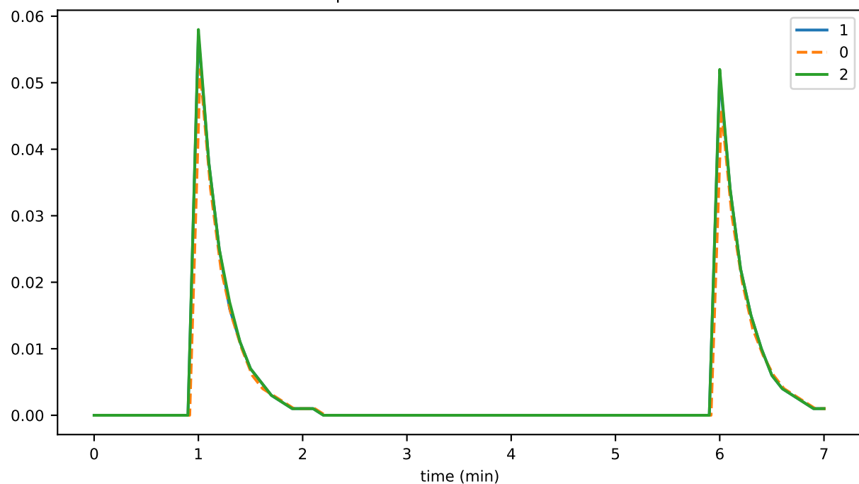
preconsensusEventFileRate
