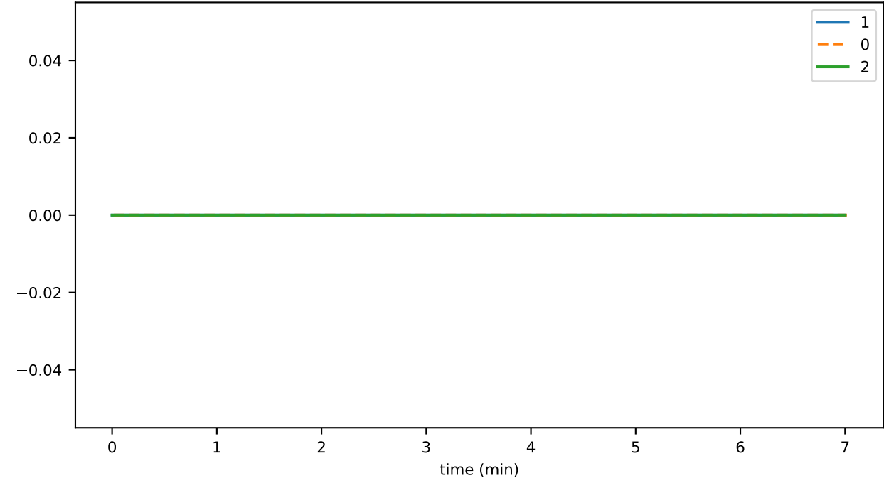
connRecv_endStream_badBlockProof
