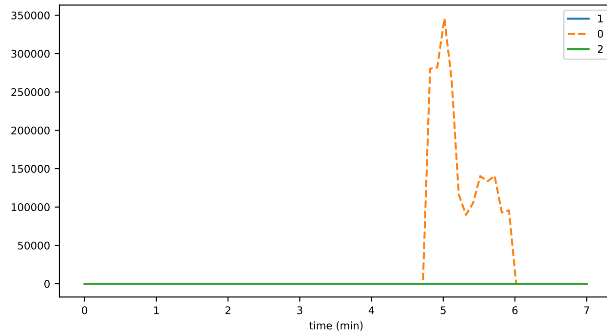
transactionGetReceiptDurationMax
