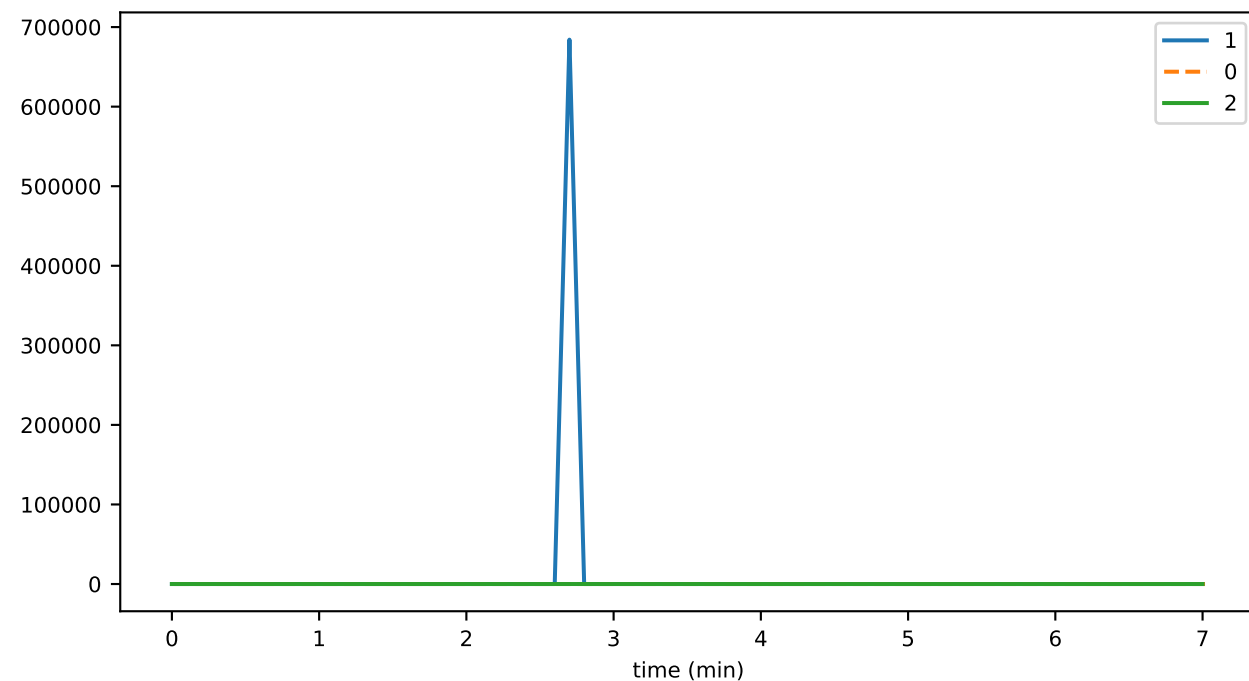
transactionGetRecordDurationMax
