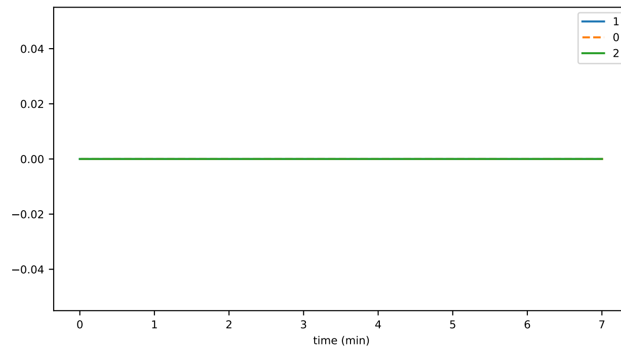
hookStoreDurationMax
