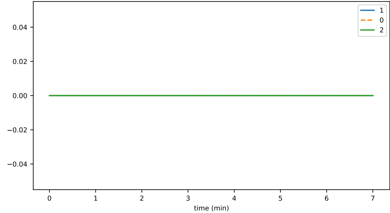
ConsensusEngine_busy_fraction
