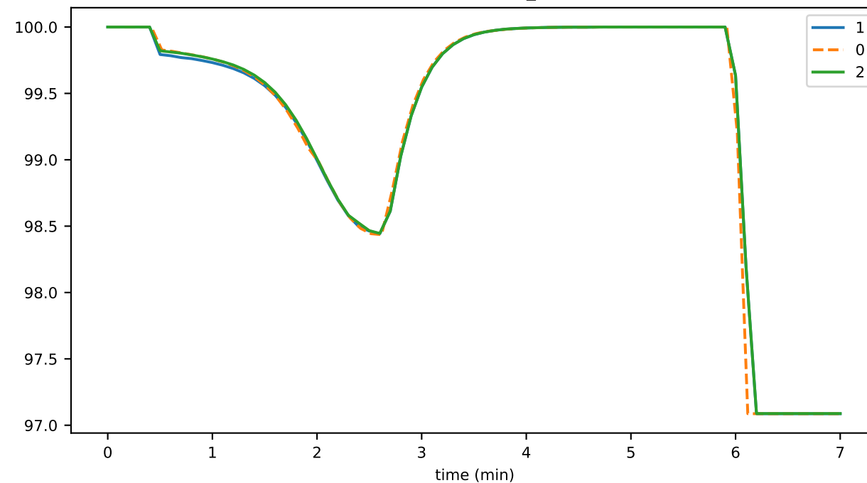
nodeActivePercentSnapshot_node0
