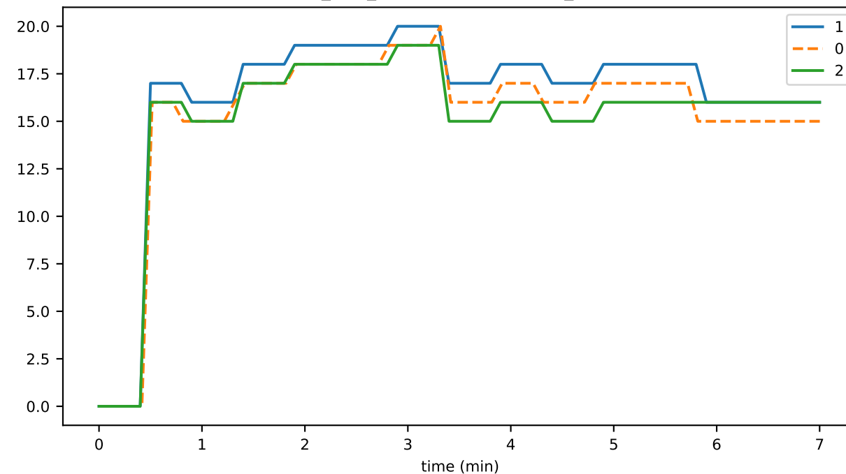
ds_files_leavesStoreFileCount_state
