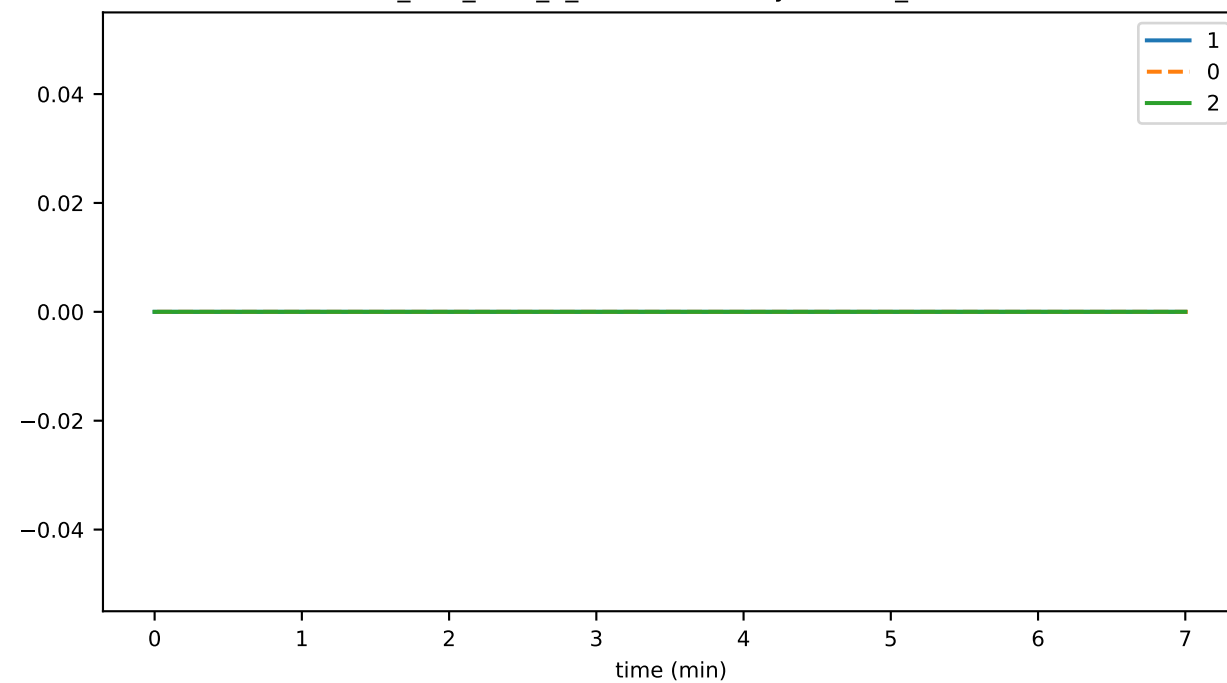
ds_files_level_7_leavesFileSizeByLevelMb_state
