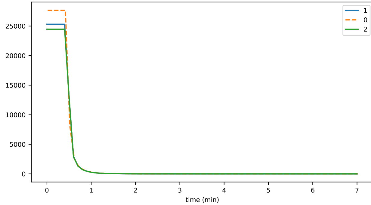
consensusCreateTopicDurationMax
