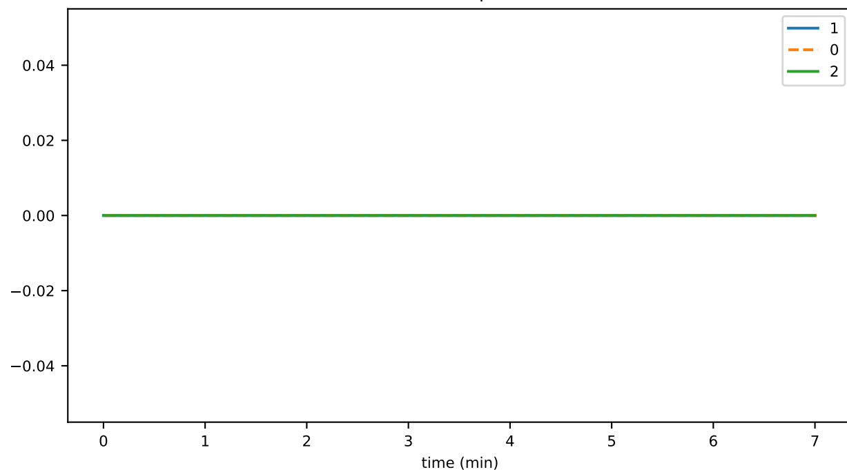
transactionGetRecordDurationMax
