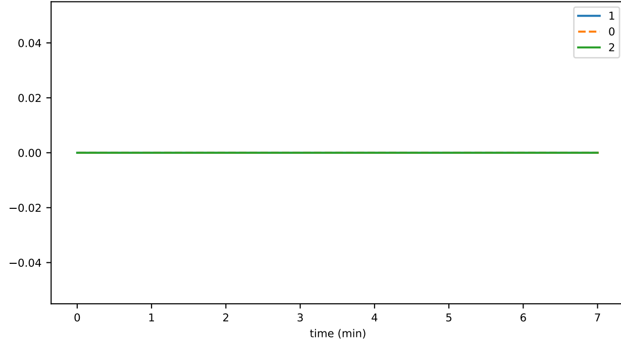
connRecv_acknowledgement
