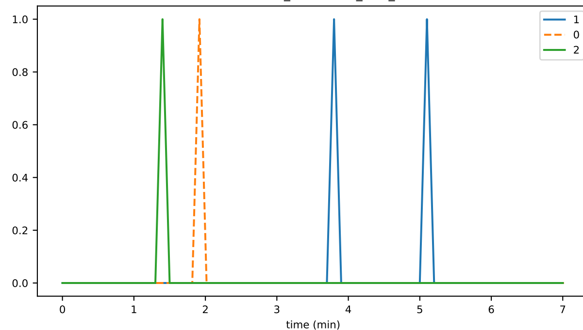
HealthMonitor_unhandled_task_count
