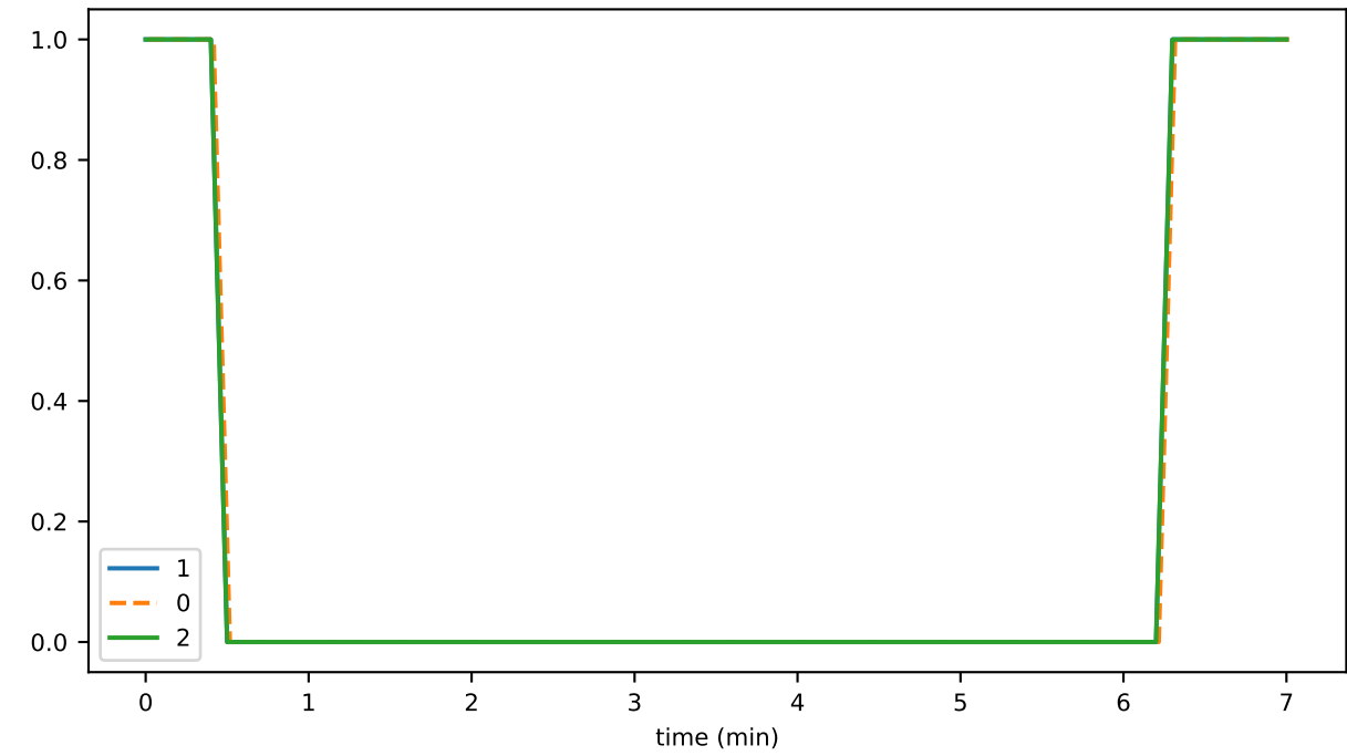
degraded
