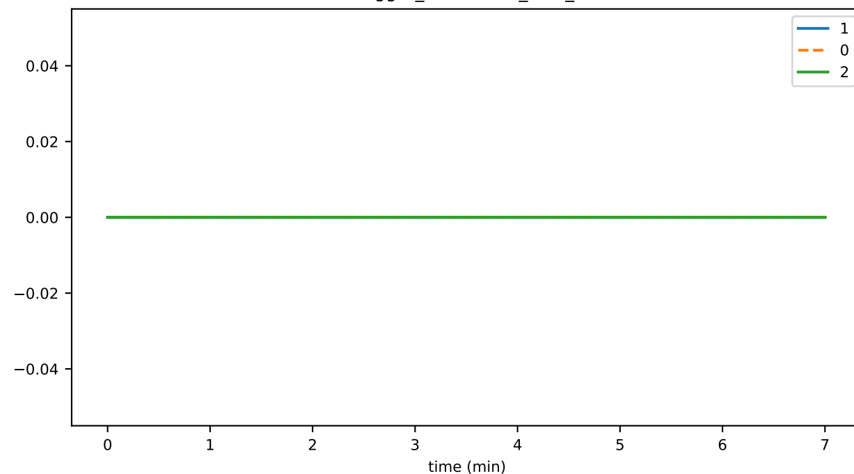
HealthMonitor_unhandled_task_count
