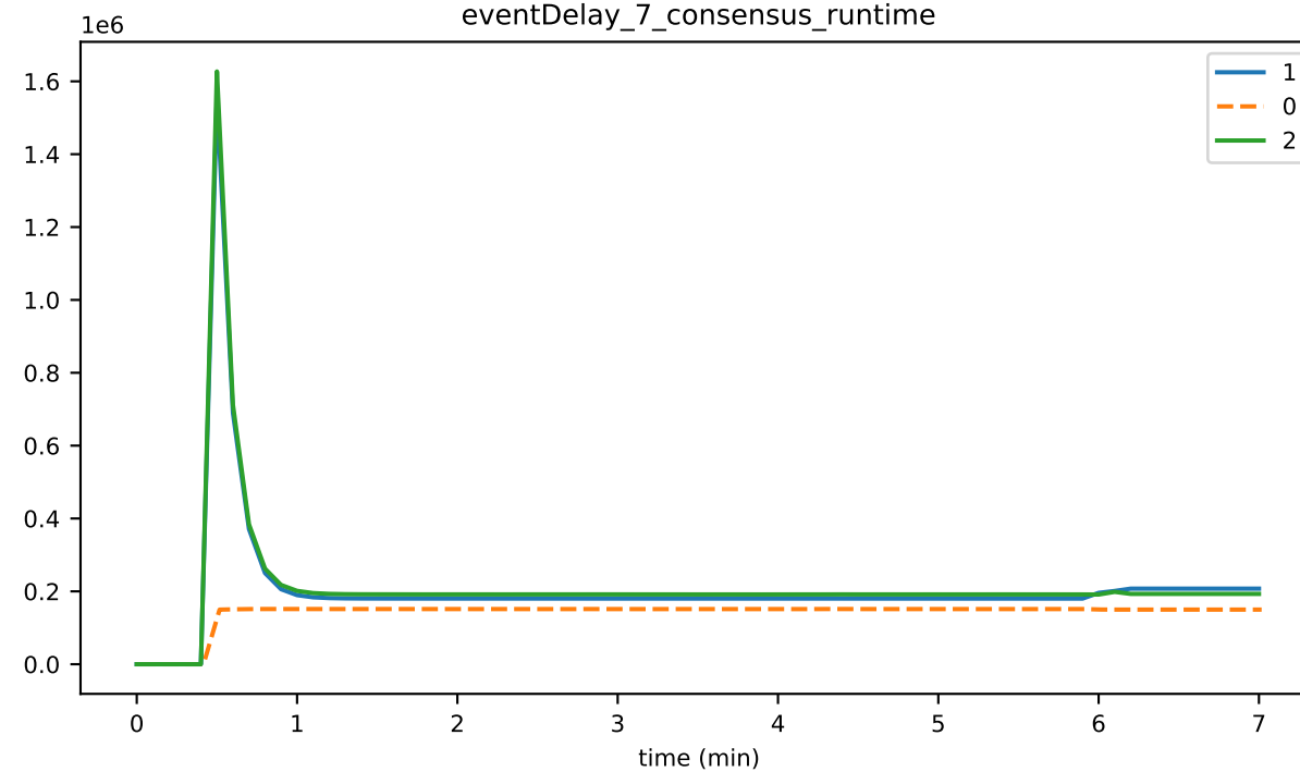
eventDelay_7_consensus_runtime
