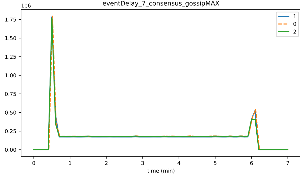
eventDelay_7_consensus_gossipMAX
