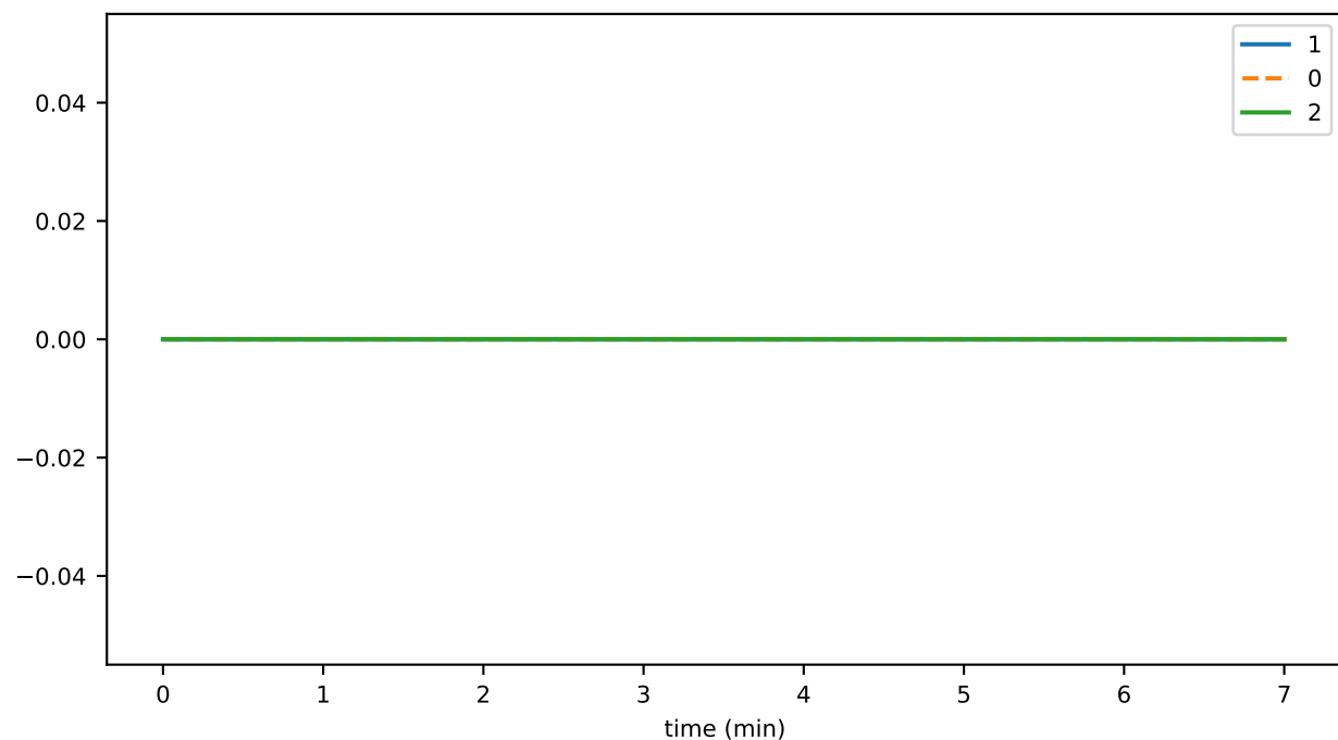
fileGetContentsDurationAvg
