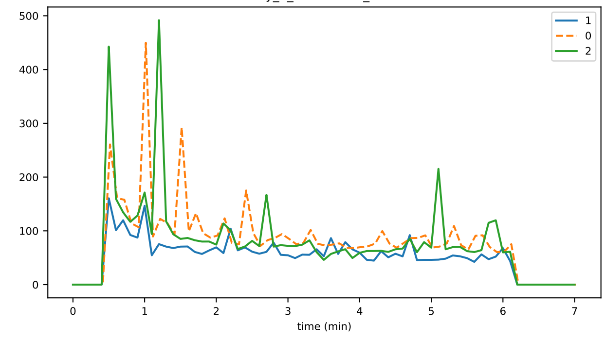
eventDelay_4_verification_runtimeMAX
