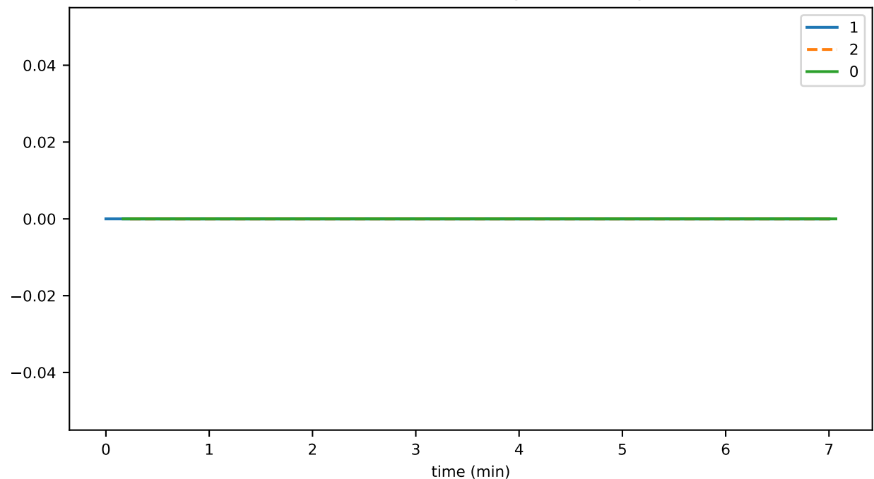
consensusSubmitMessageThrottledTxns
