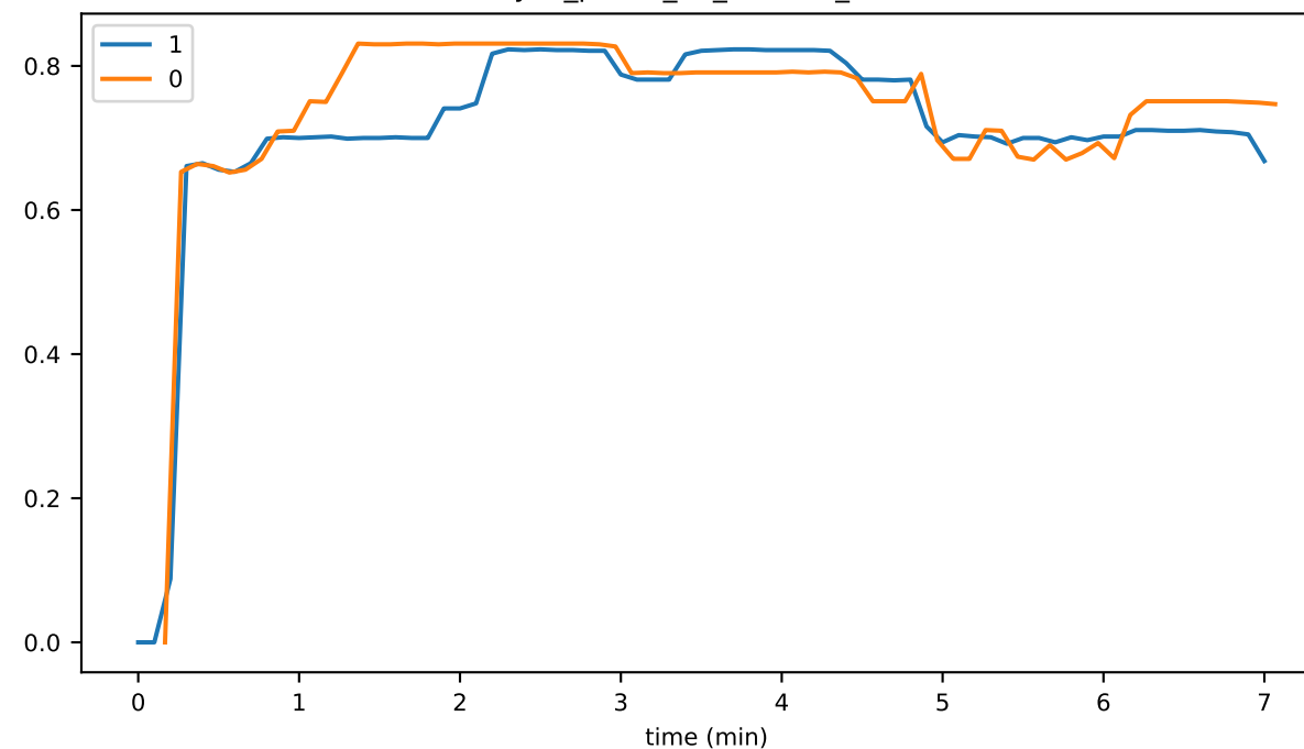
sync_phase_02_fraction_IDLE
