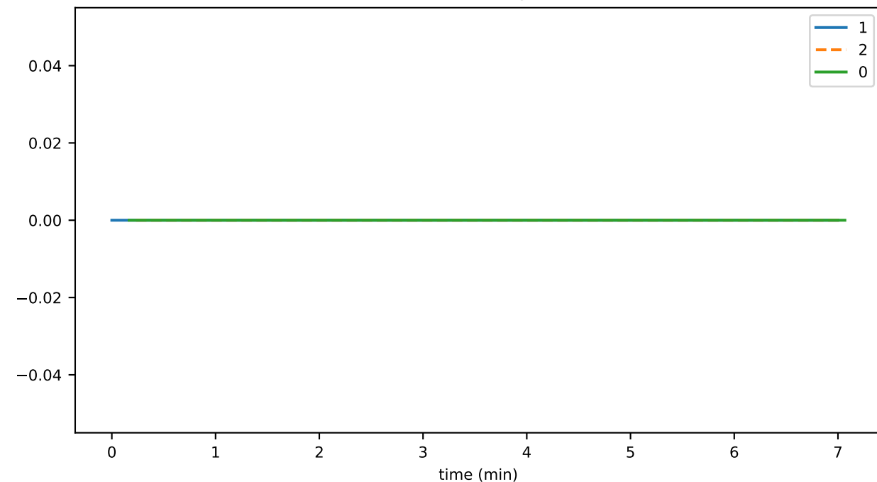
consensusTime
