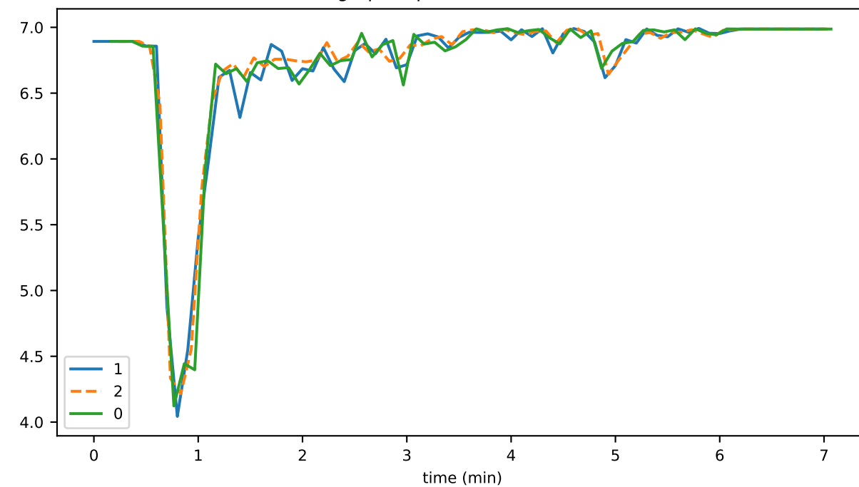
graphDepthUntilConsensus
