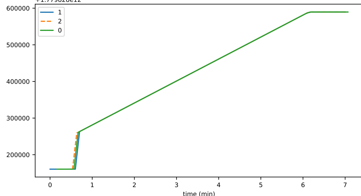
consensusTime
