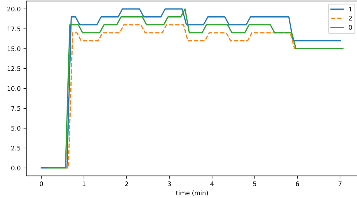
ds_files_leavesStoreFileCount_state
