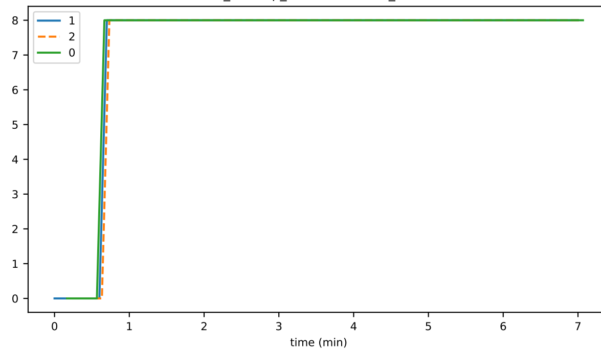
ds_offheap_hashesIndexMb_state
