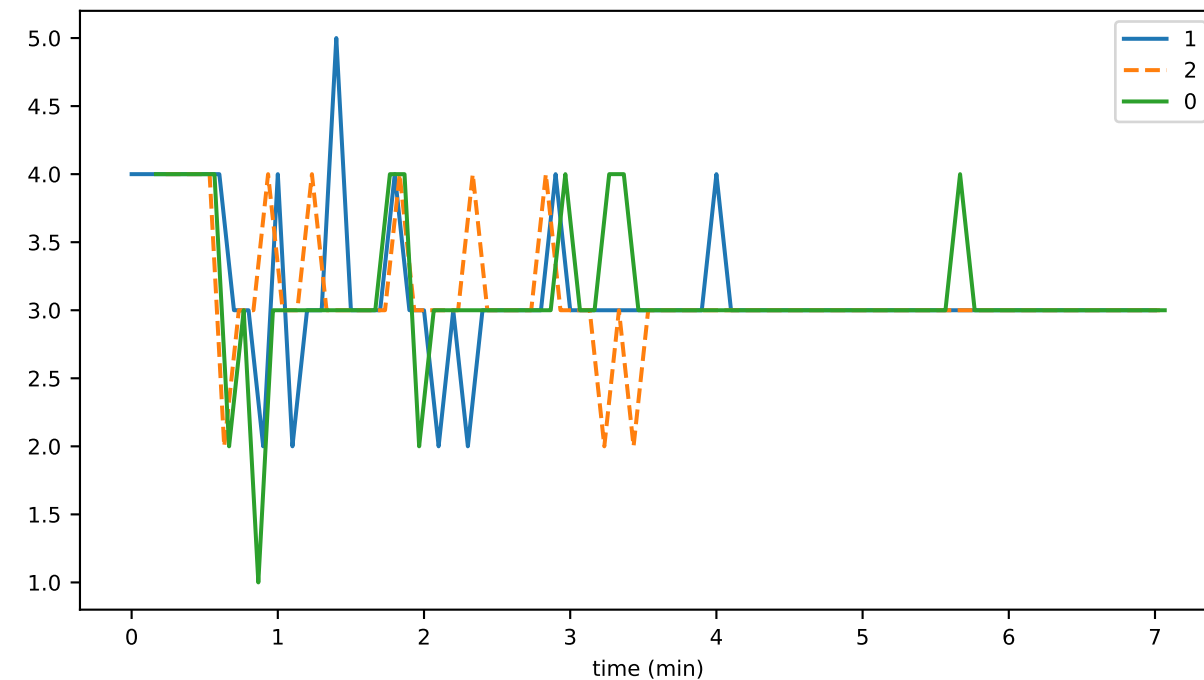
eventsWithDisparateSignature
